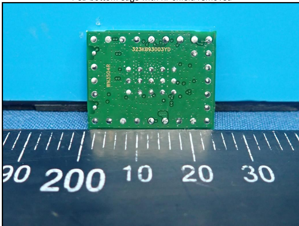
PCB bottom edge with RF shield removed
