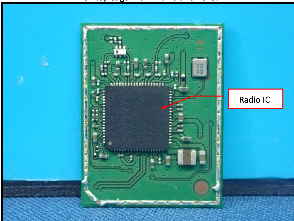
PCB top edge with RF shield removed
