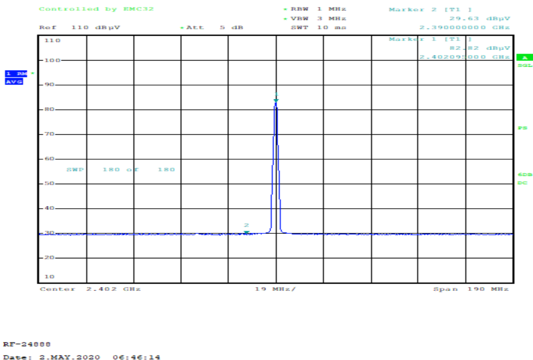
Figure 9-26 Radiated Restricted Band Edge (Ch. 0) Average
