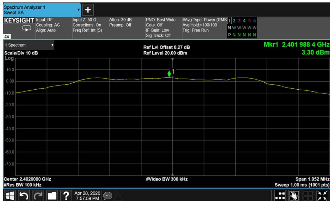
Figure 9-11 Power Spectral Density (Ch. 0)
