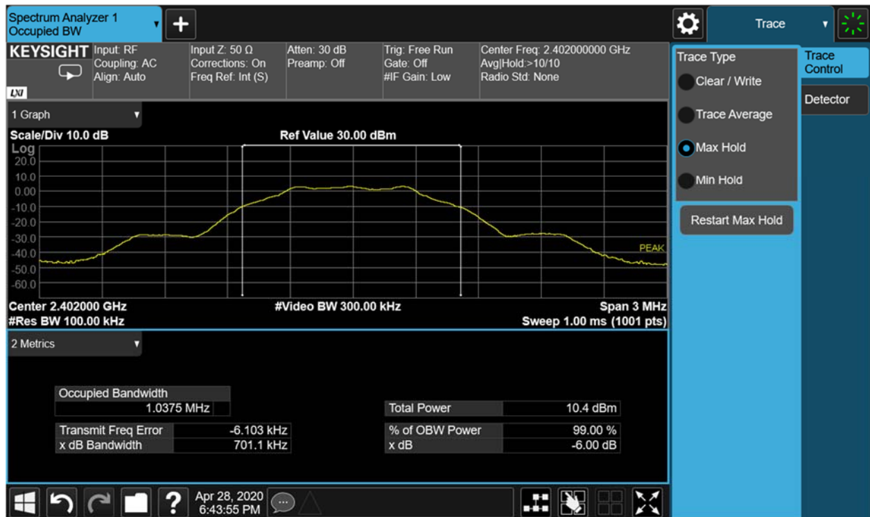
Figure 9-2 6dB Bandwidth (Ch. 0)
