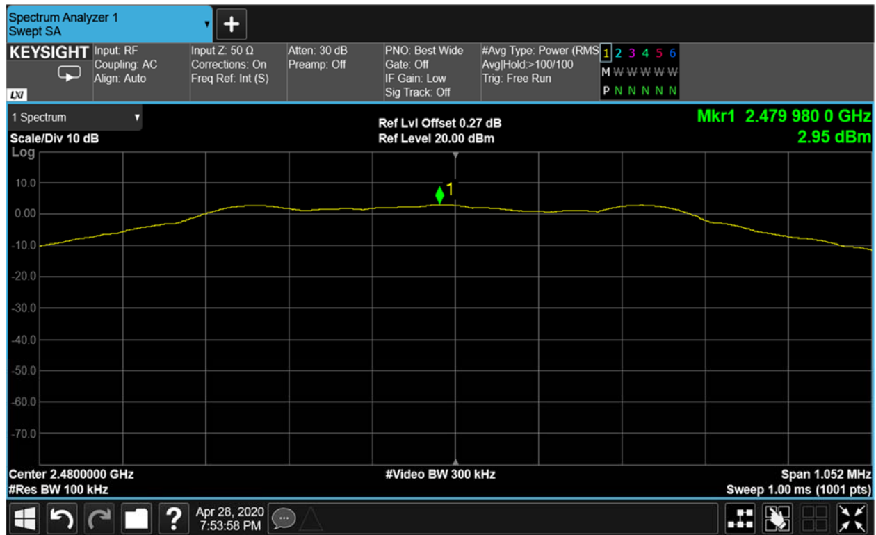
Figure 9-20 Reference Level Measurement (Ch.39)
