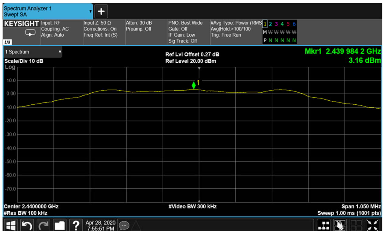
Figure 9-17 Reference Level Measurement (Ch.19)
