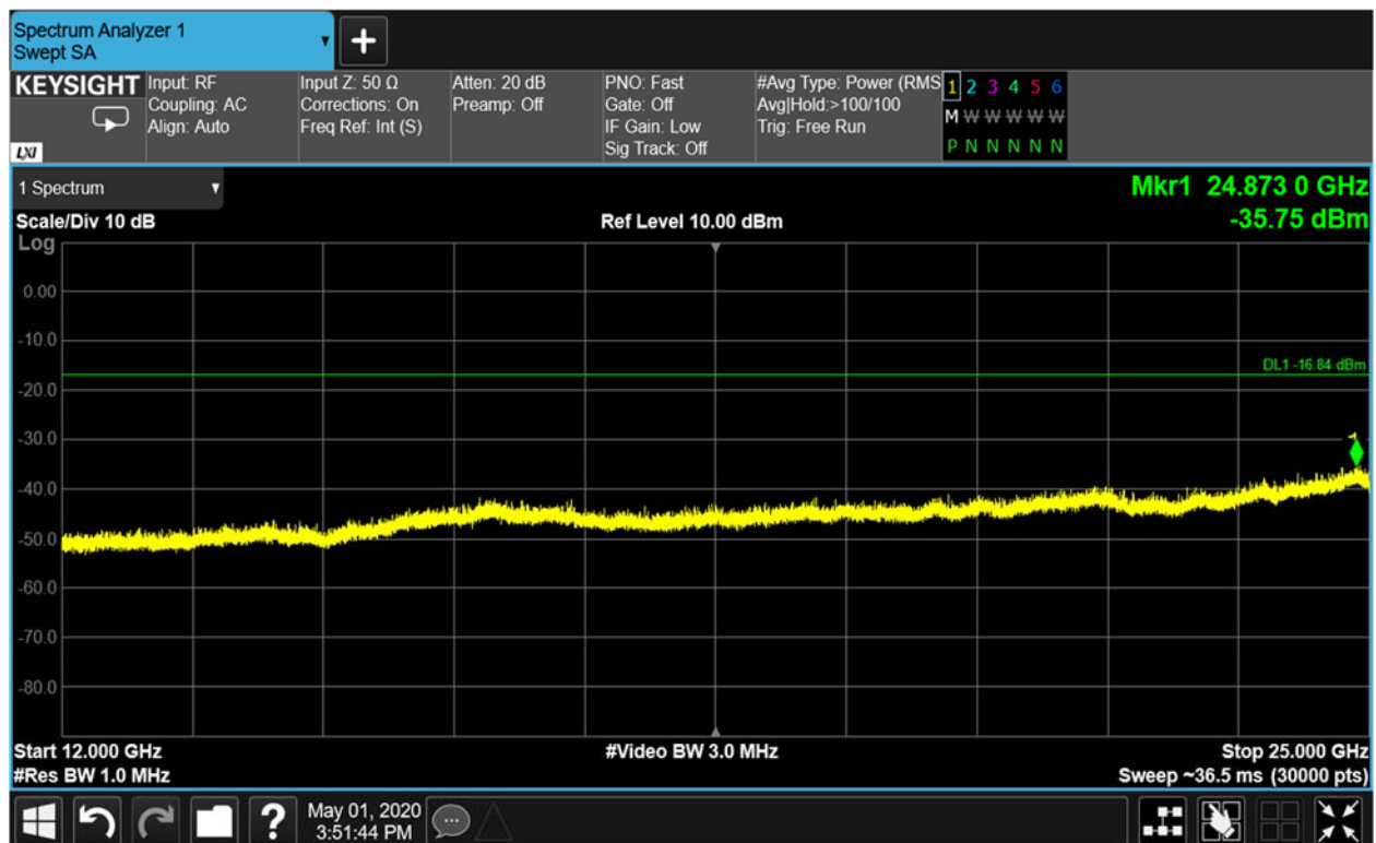
Figure 9-19 Conducted Spurious Emissions 12-25 GHz (Ch. 19)
