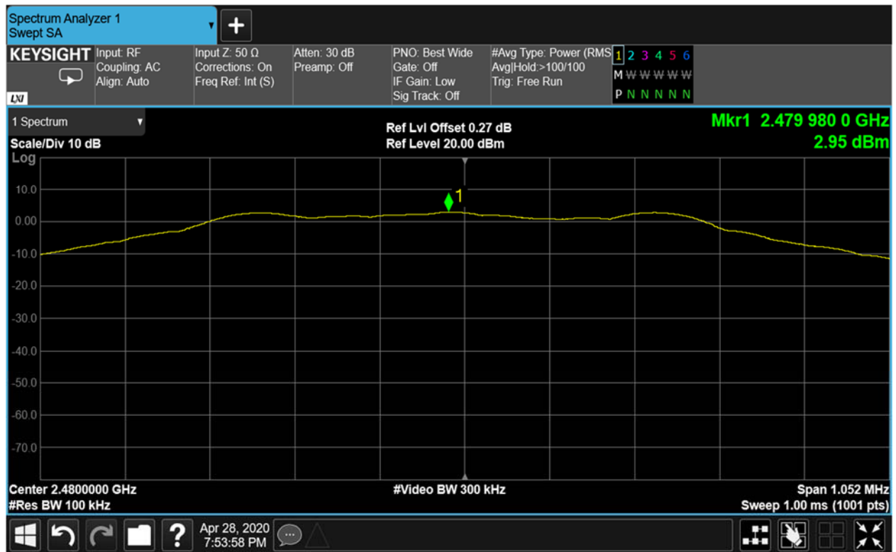
Figure 9-13 Power Spectral Density (Ch. 39)
