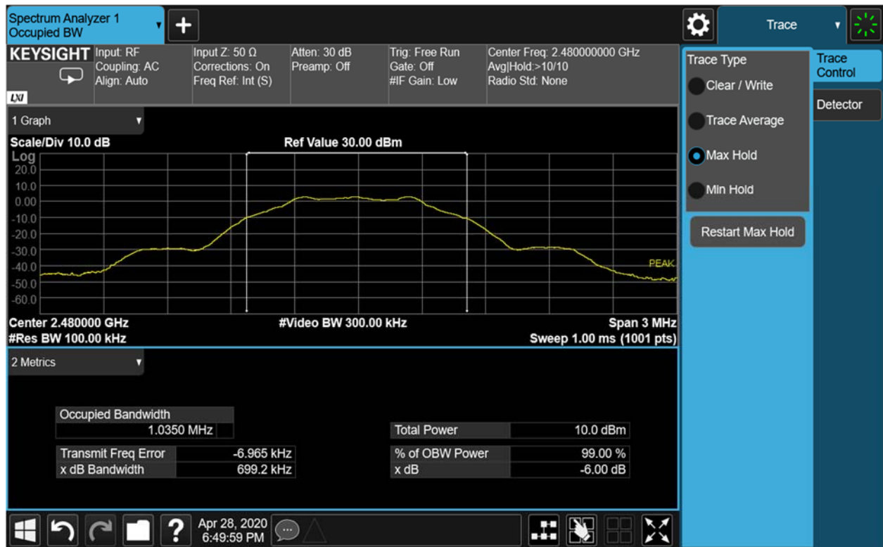
Figure 9-4 6dB Bandwidth (Ch. 39)
