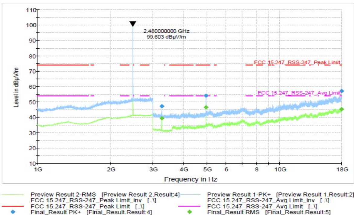
Figure 9-33 Radiated Spurious Emissions 1-18 GHz (Ch. 39)
