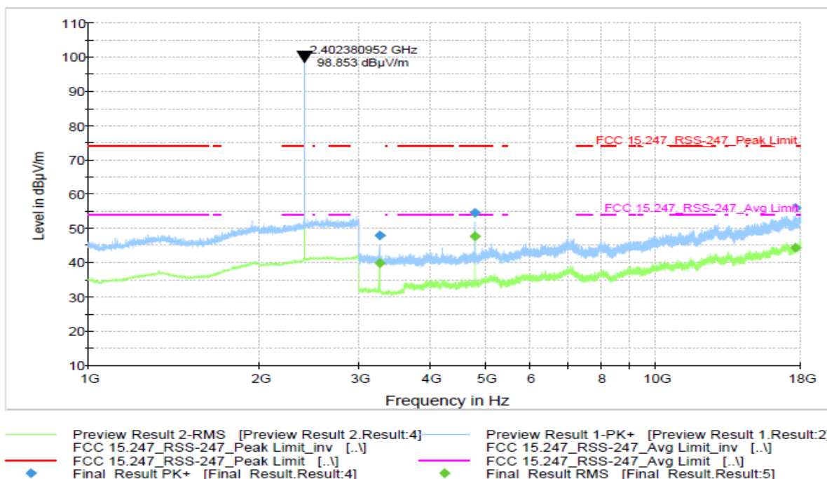
Figure 9-31 Radiated Spurious Emissions 1-18 GHz (Ch. 0)
