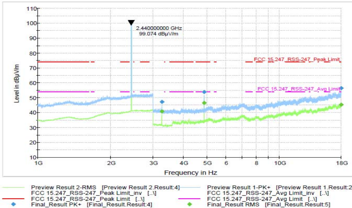
Figure 9-32 Radiated Spurious Emissions 1-18 GHz (Ch. 19)
