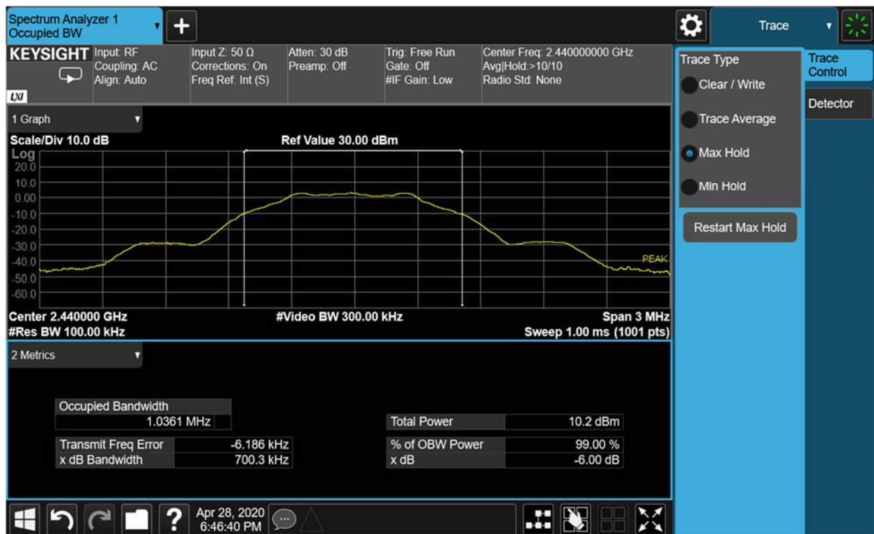
Figure 9-3 6dB Bandwidth (Ch. 19)
