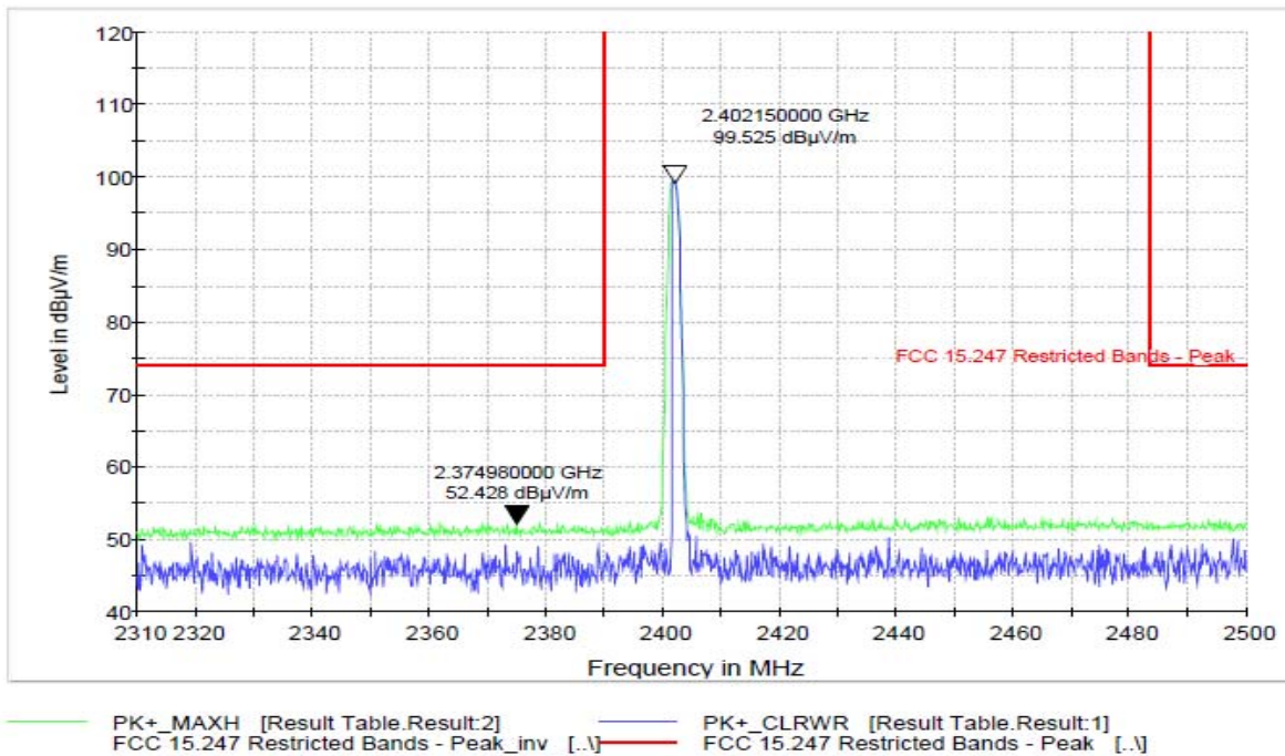
Figure 9-25 Radiated Restricted Band Edge (Ch. 0) Peak
