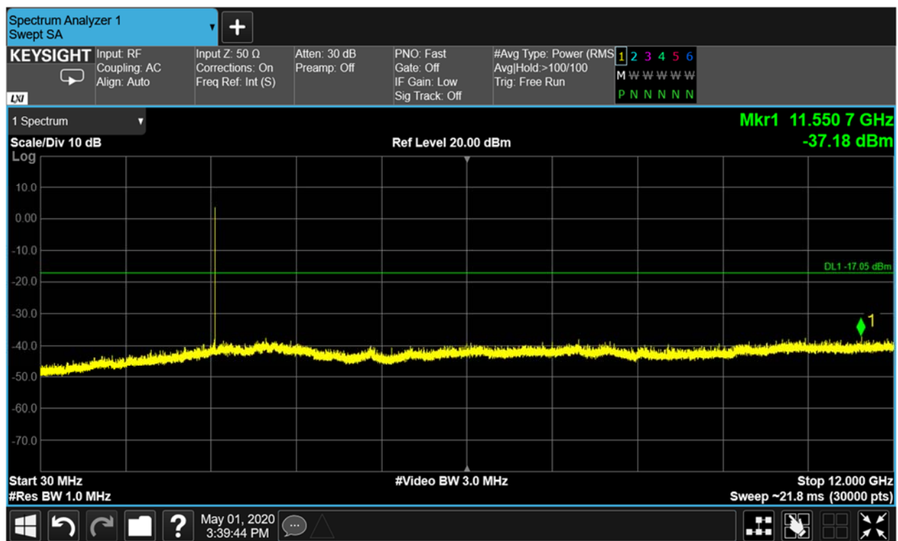
Figure 9-21 Conducted Spurious Emissions 30-12000 MHz (Ch.39)
