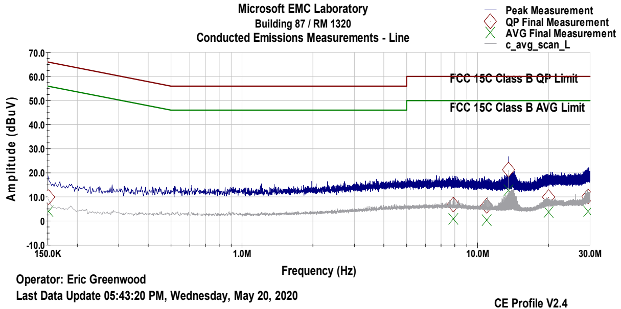
Figure 9-36 AC Line Conducted Emissions- Line (150 kHz- 30 MHz)
