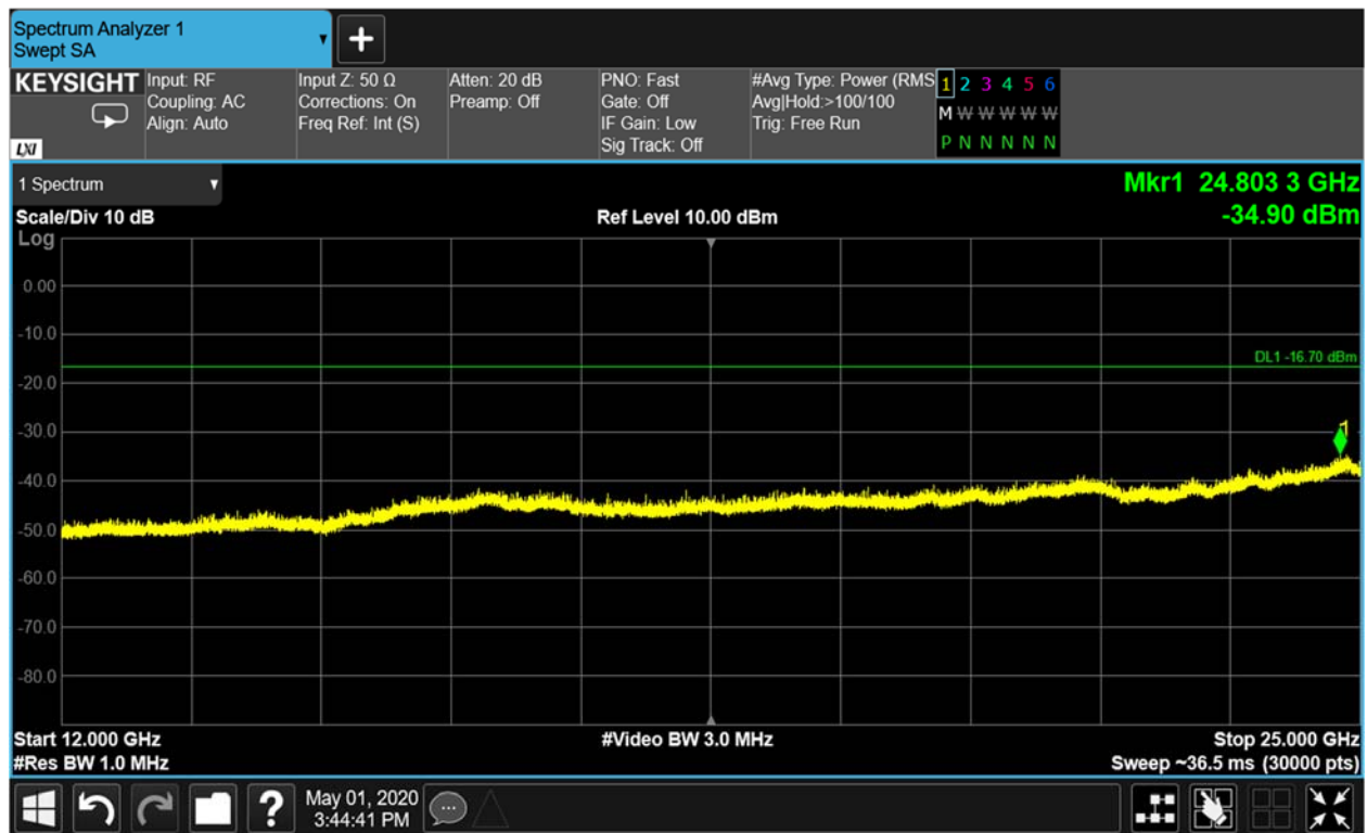
Figure 9-16 Conducted Spurious Emissions 12-25 GHz (Ch.0)
