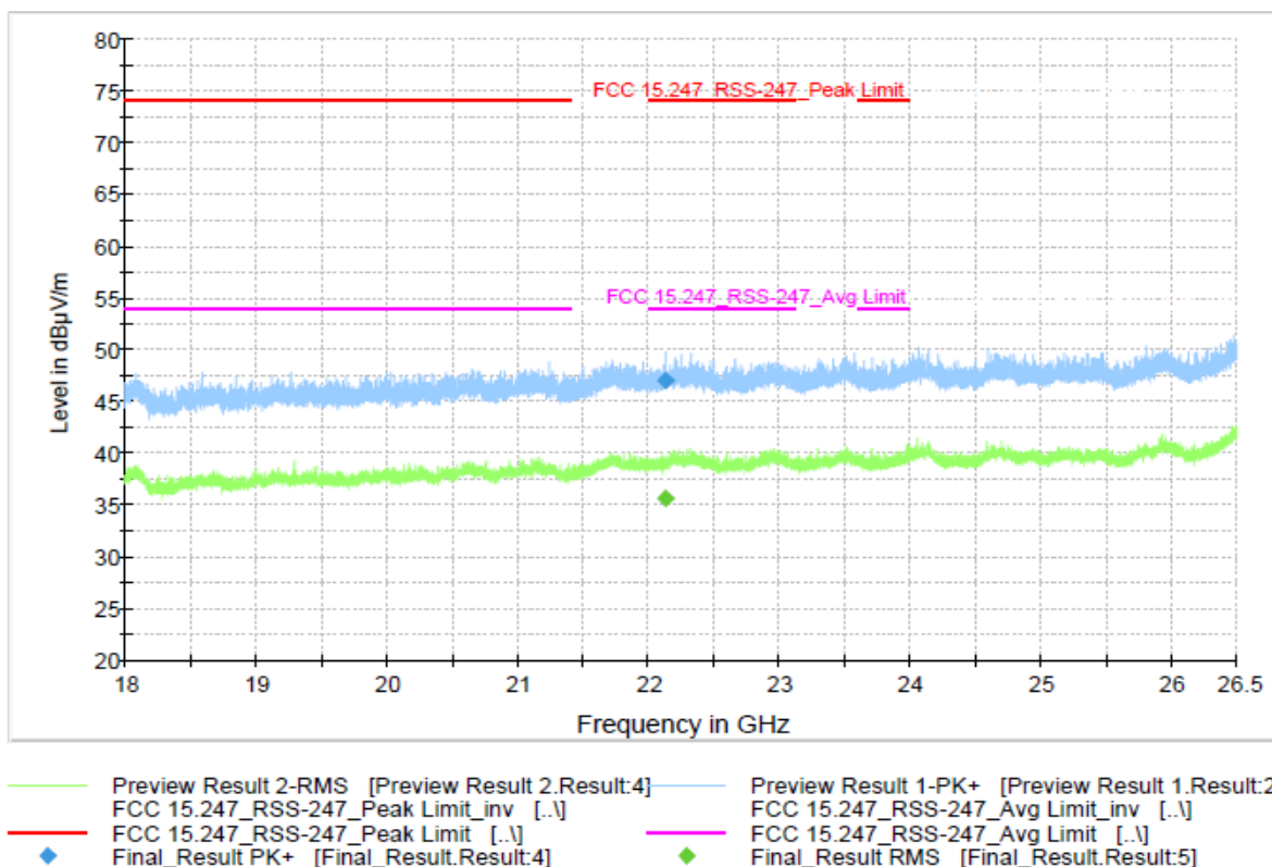
Figure 9-34 Radiated Spurious Emissions (Ch. 19) (18 – 26.5 GHz)
