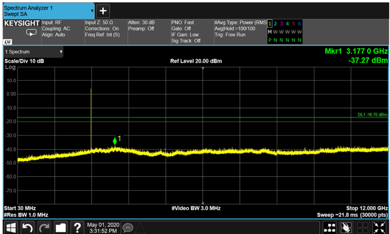
Figure 9-15 Conducted Spurious Emissions 30-12000 MHz (Ch. 0)
