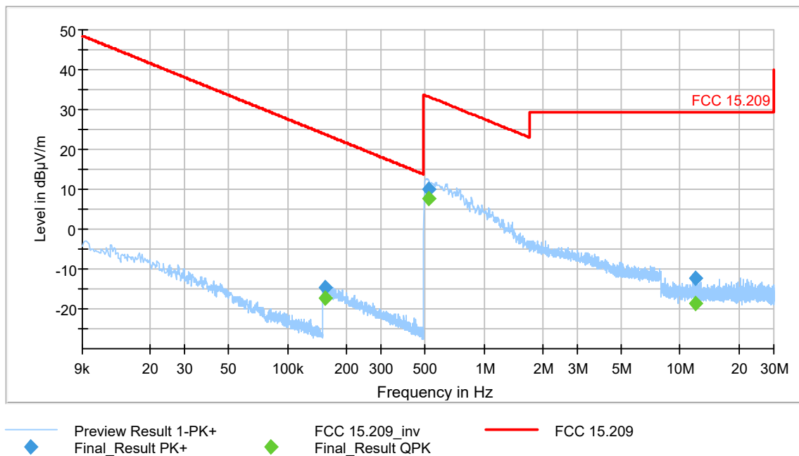
Figure 9-29 Radiated Spurious Emissions (Ch.0) 2440 (9kHz – 30MHz)
