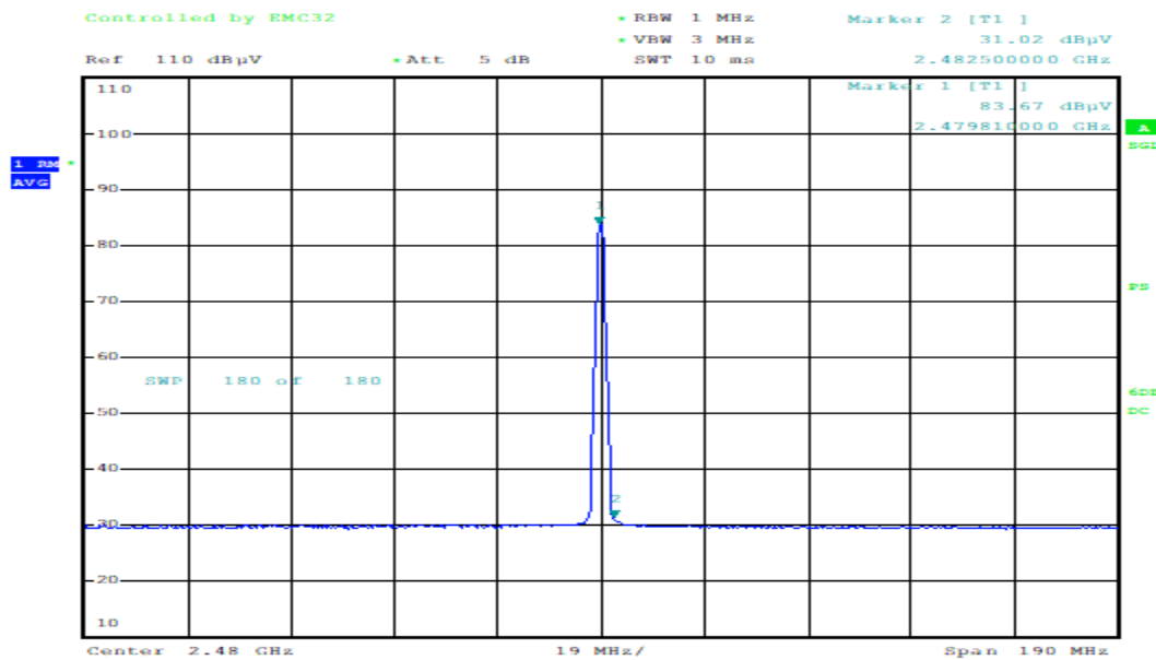
Figure 9-27 Radiated Restricted Band Edge (Ch. 39) Peak
