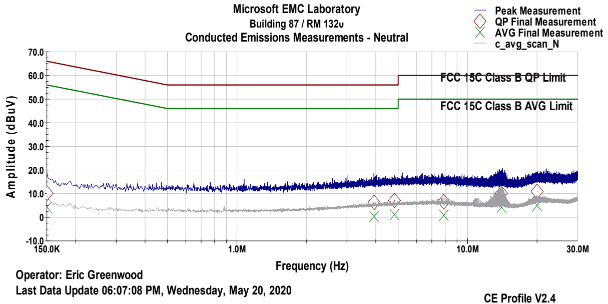
Figure 9-35 AC Line Conducted Emissions- Neutral (150 kHz- 30 MHz)
