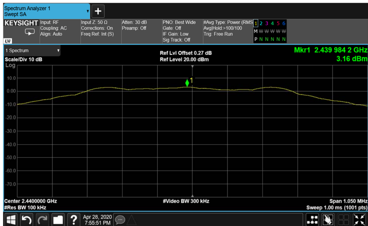
Figure 9-12 Power Spectral Density (Ch. 19)
