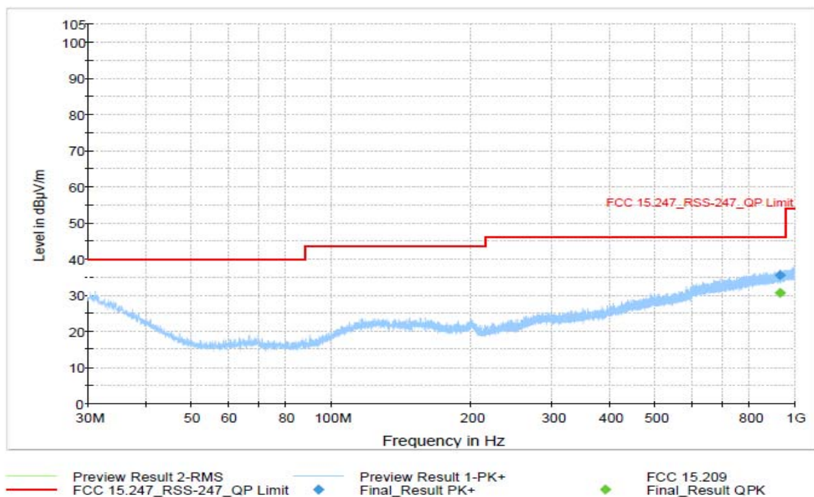
Figure 9-30 Radiated Spurious Emissions (Ch. 19) 2440 (30MHz - 1GHz)
