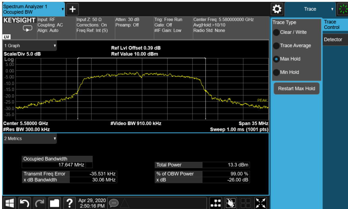
Plot 9-8. 26-dB Emission Bandwidth and 99% OBW Chain A 802.11a (Ch. 116)
