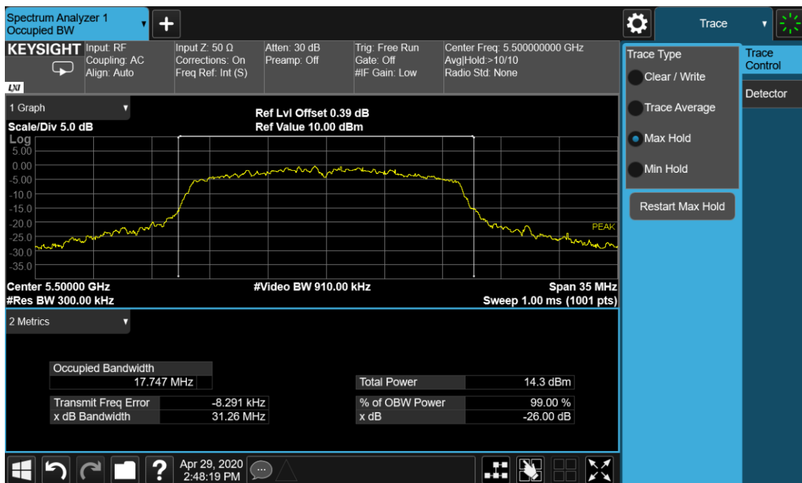
Plot 9-7 . 26-dB Emission Bandwidth and 99% OBW Chain A 802.11a (Ch. 100)
