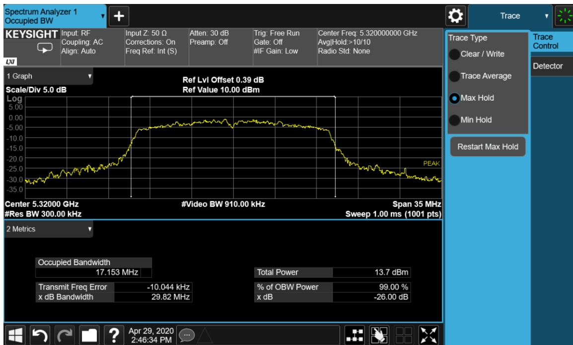
Plot 9-6. 26-dB Emission Bandwidth and 99% OBW Chain A 802.11a (Ch. 64)
