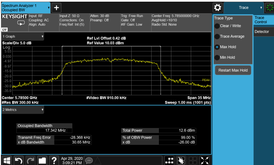
Plot 9-11. 26-dB Emission Bandwidth and 99% OBW Chain A 802.11a (Ch. 157)
