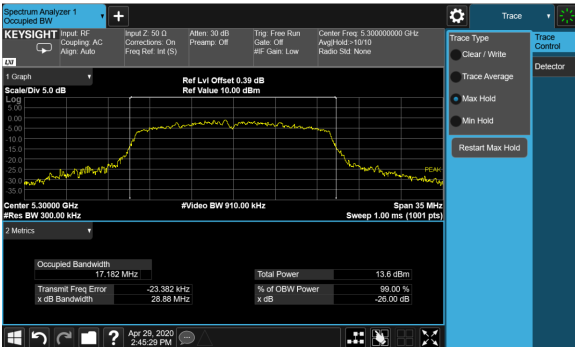
Plot 9-5. 26-dB Emission Bandwidth and 99% OBW Chain A 802.11a (Ch. 60)
