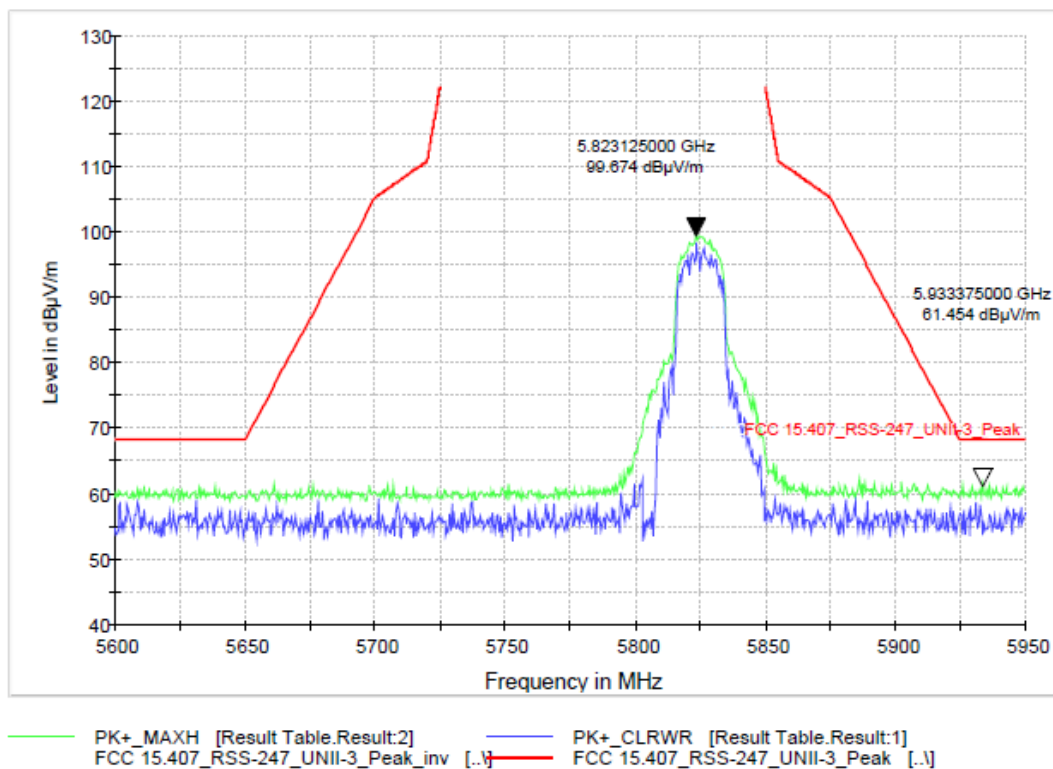
Plot 9-106. Peak Radiated Band Edge Emissions Tx Chains A & B 802.11n HT20 (Ch. 165)
