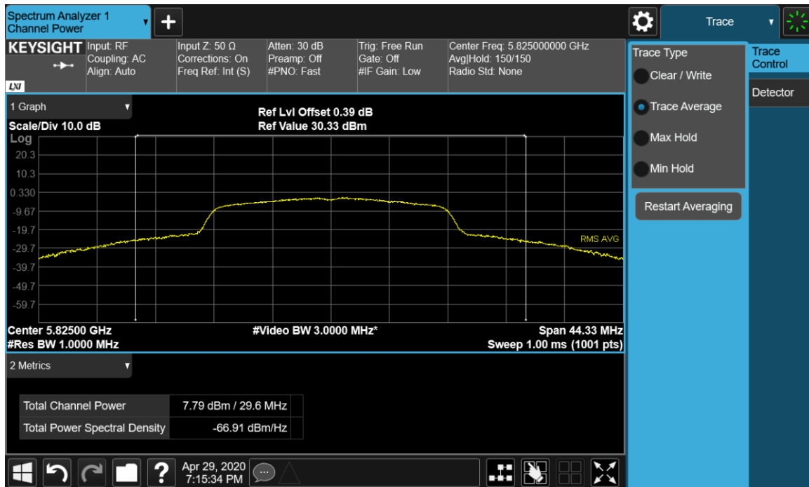
Plot 9-59. Maximum Conducted Output Power Chain A 802.11a (Ch. 165)
