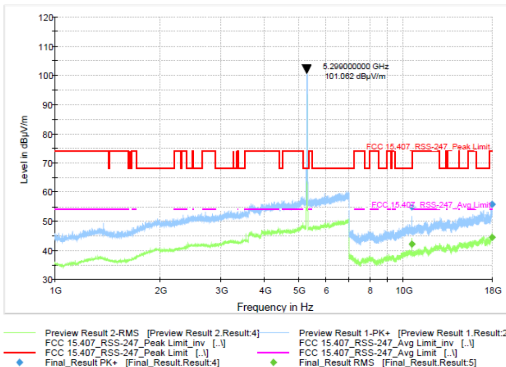
Plot 9-79. Radiated Spurious Emissions 1-18 GHz Tx Chain A 802.11n (Ch. 60)
