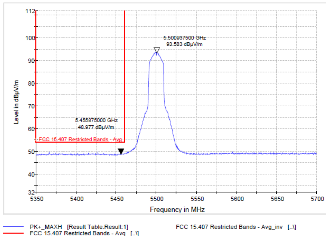
Plot 9-103. Average Radiated Band Edge Emissions Tx Chains A & B 802.11n HT20 (Ch. 100)
