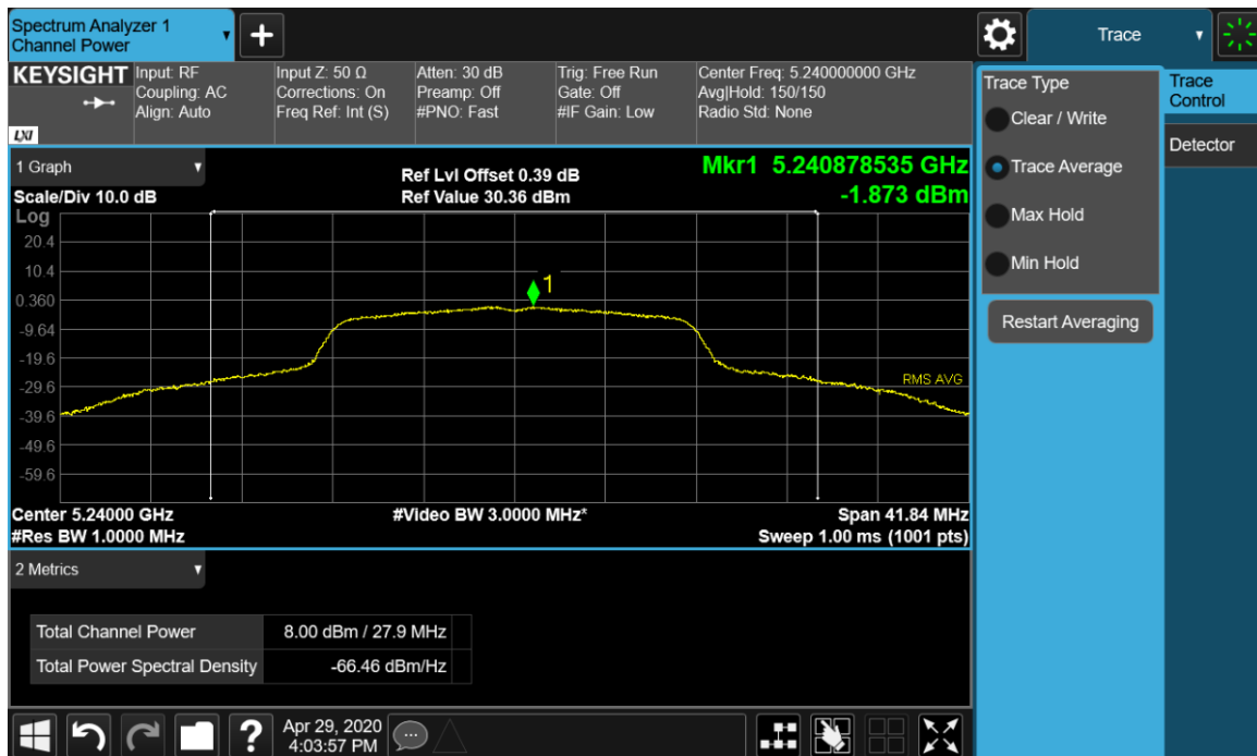
Plot 9-33. Maximum Conducted Output Power and PSD Chain A 802.11a (Ch. 48)
