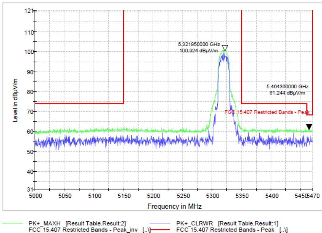
Plot 9-100. Peak Radiated Band Edge Emissions Tx Chains A & B 802.11n HT20 (Ch. 64)
