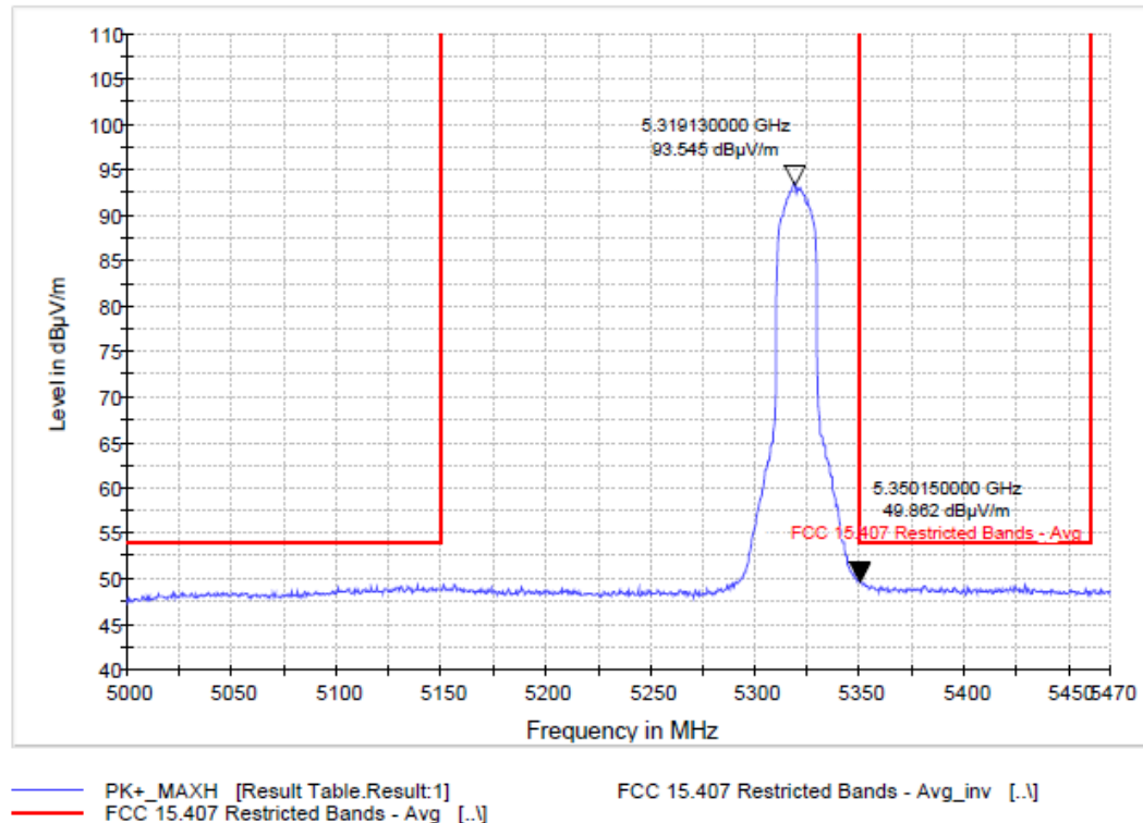
Plot 9-101. Average Radiated Band Edge Emissions Tx Chains A & B 802.11n HT20 (Ch. 64)
