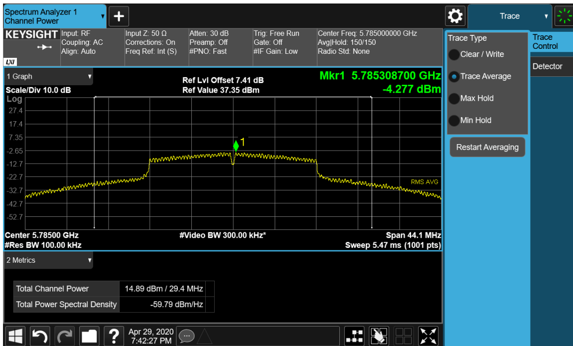
Plot 9-58. Maximum 500KHz PSD Chain A 802.11a (Ch. 157)
