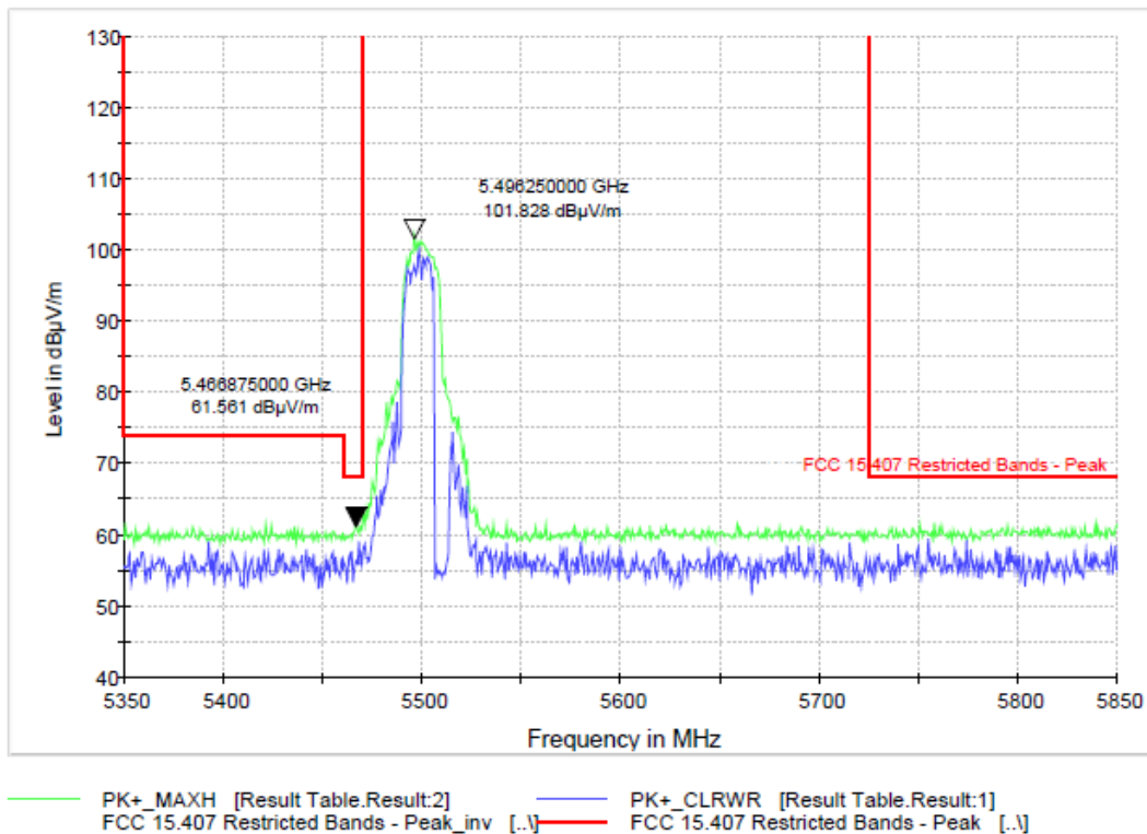
Plot 9-102. Peak Radiated Band Edge Emissions Tx Chains A & B 802.11n HT20 (Ch. 100)
