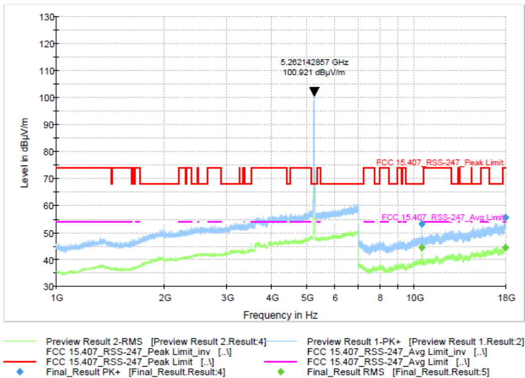
Plot 9-78. Radiated Spurious Emissions 1-18 GHz Tx Chain A 802.11n (Ch. 52)
