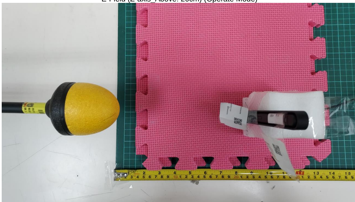
E-Field (Z-axis_Above: 20cm) (Operate Mode)
