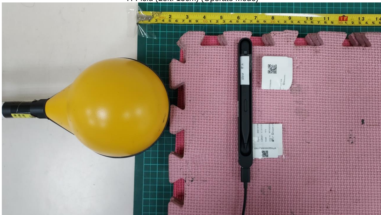
H-Field (Left: 15cm) (Operate Mode)
