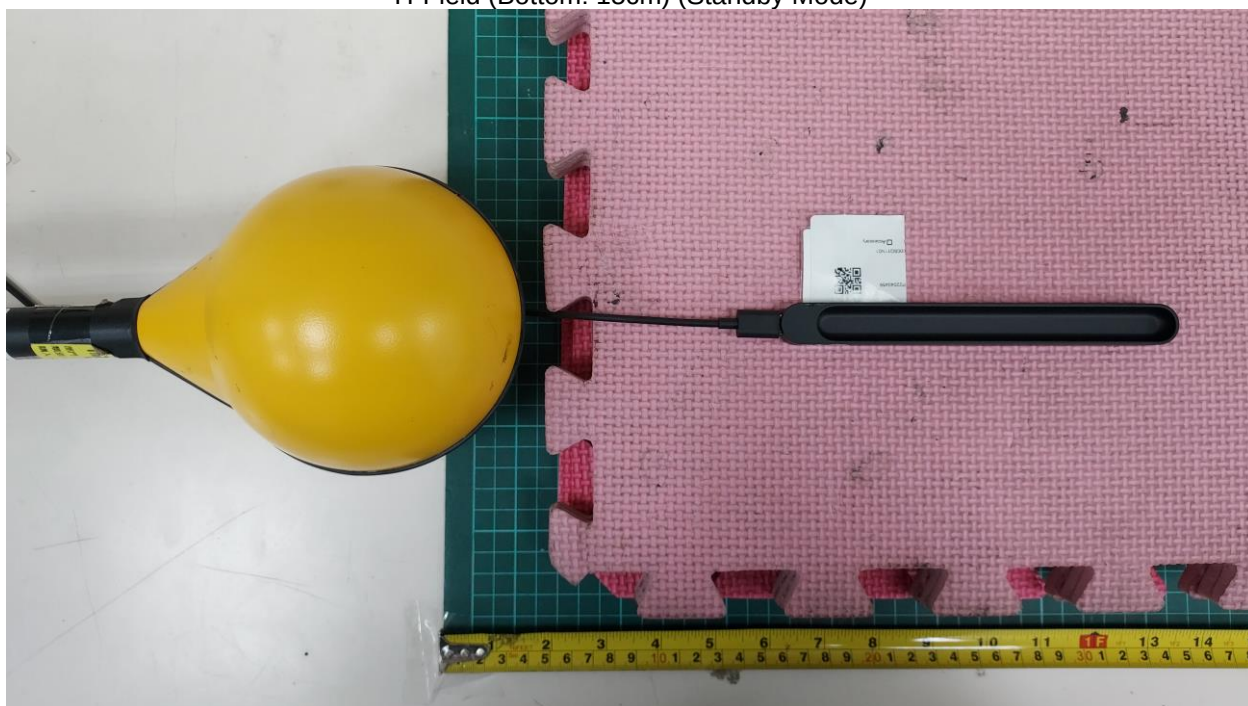
H-Field (Bottom: 15cm) (Standby Mode)
