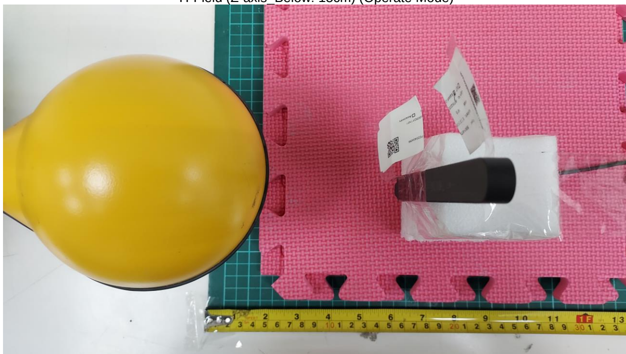
H-Field (Z-axis Below: 15cm) (Operate Mode)
