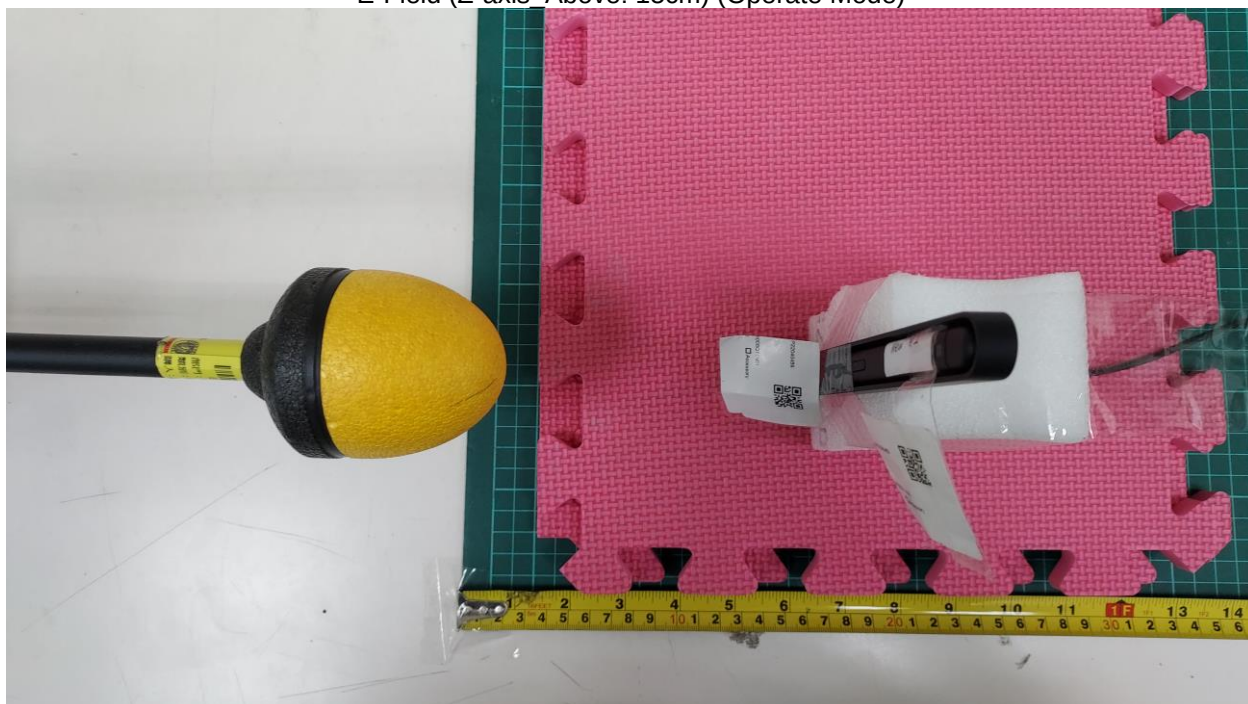
E-Field (Z-axis Above: 15cm) (Operate Mode)
