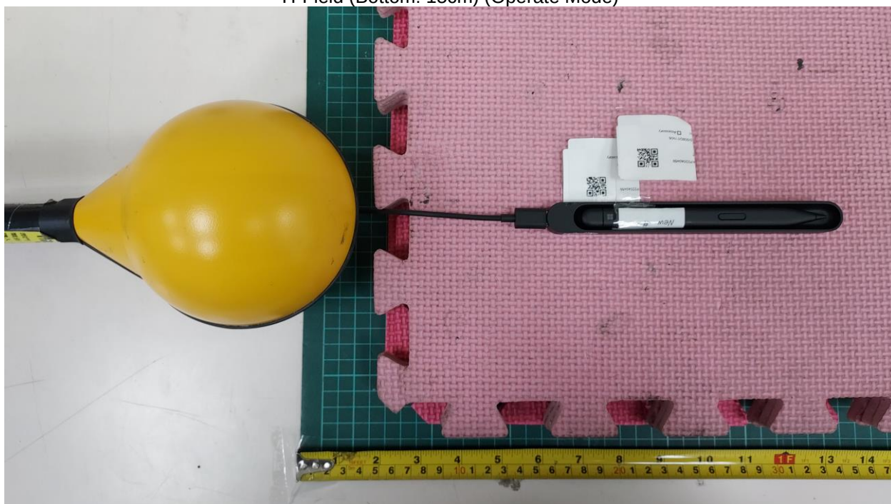
H-Field (Bottom: 15cm) (Operate Mode)
