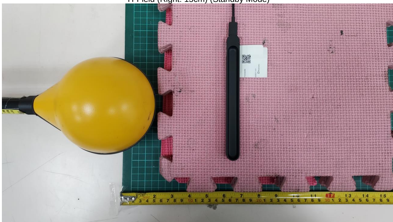
H-Field (Right: 15cm) (Standby Mode)
