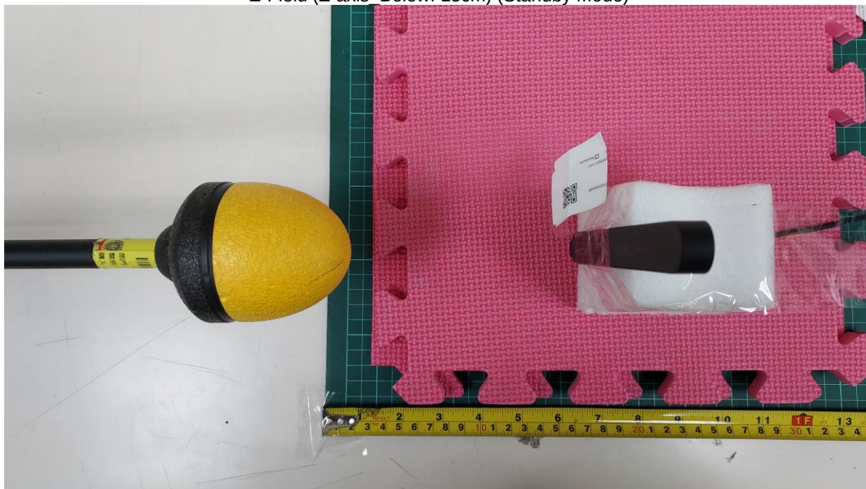
E-Field (Z-axis_Below: 15cm) (Standby Mode)
