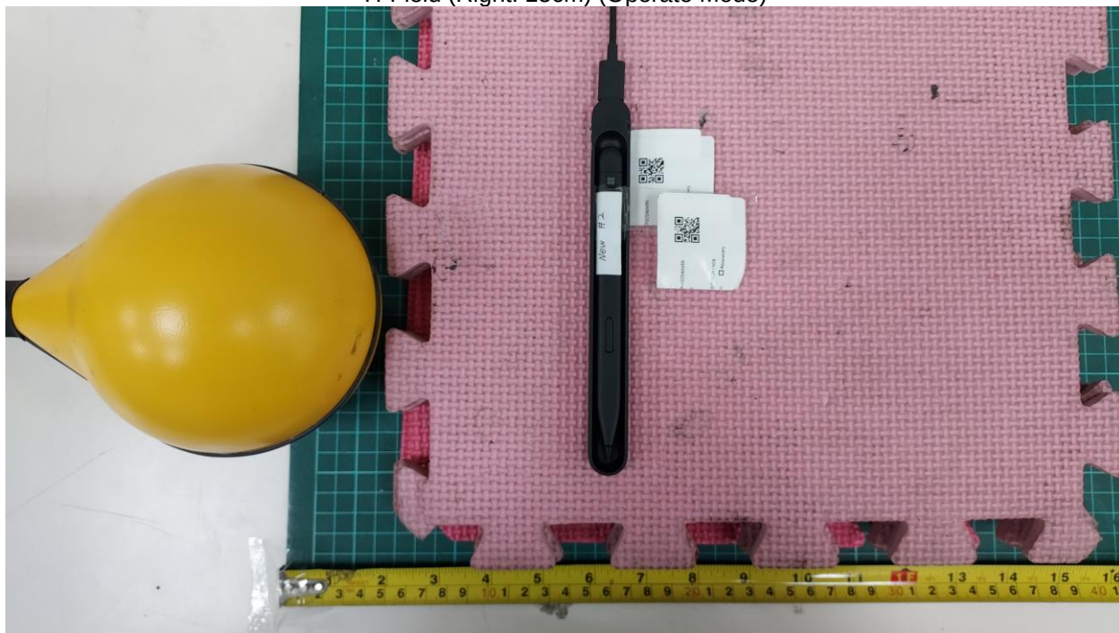
H-Field (Right: 15cm) (Operate Mode)
