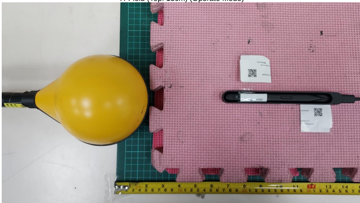
H-Field (Top: 15cm) (Operate Mode)
