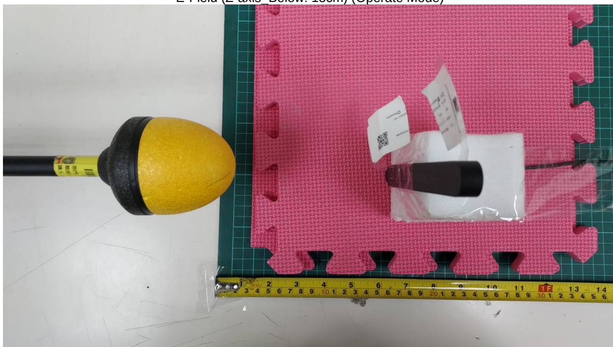
E-Field (Z-axis Below: 15cm) (Operate Mode)
