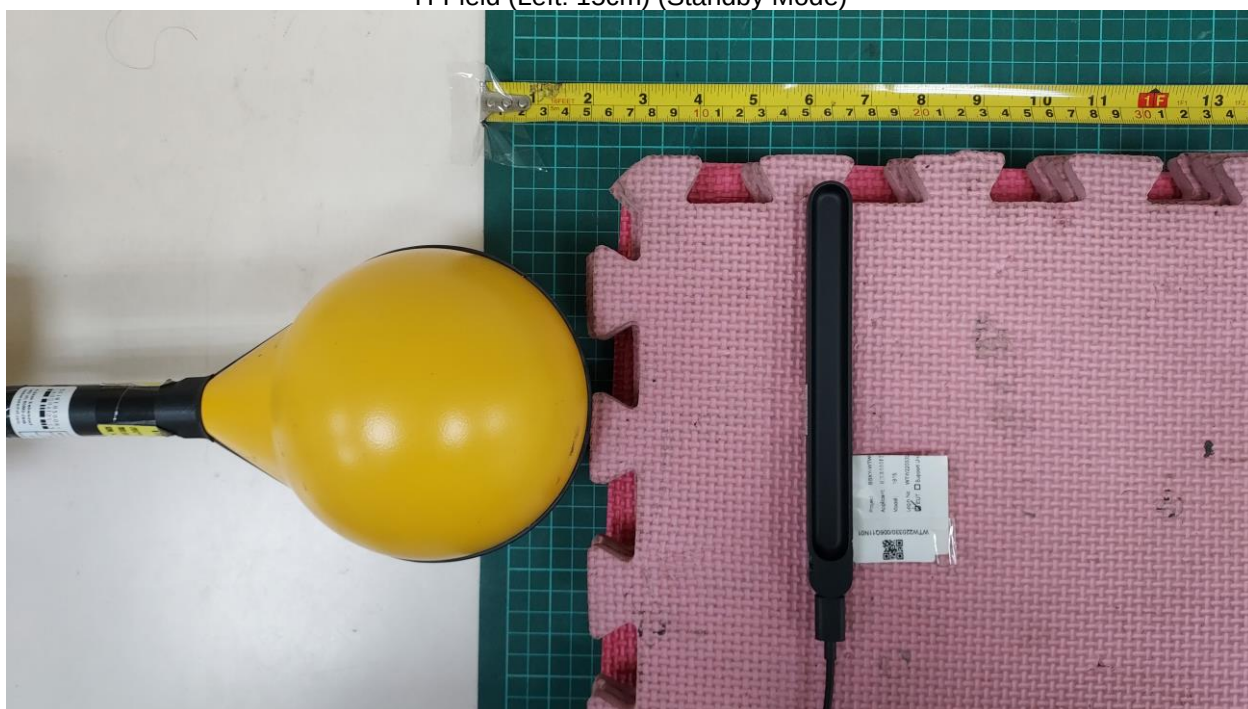
H-Field (Left: 15cm) (Standby Mode)
