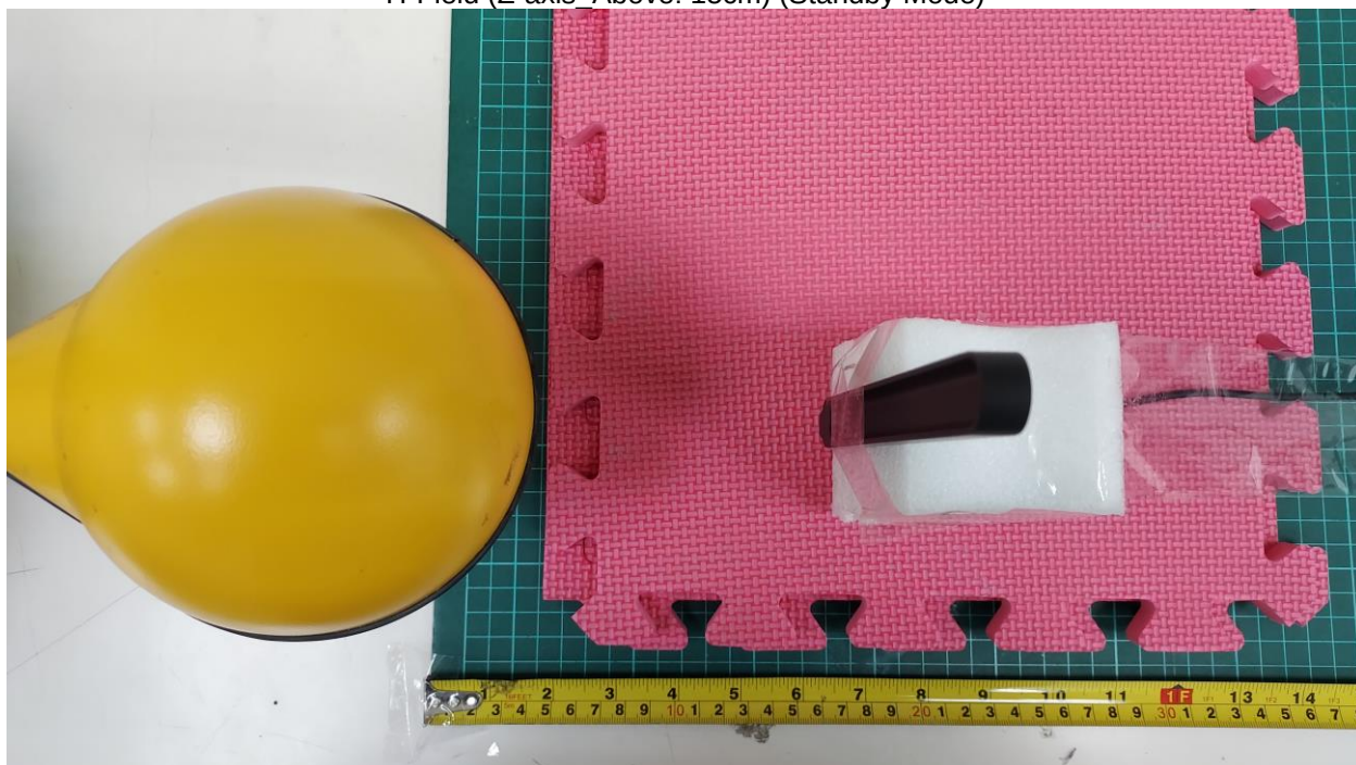
H-Field (Z-axis Above: 15cm) (Standby Mode)
