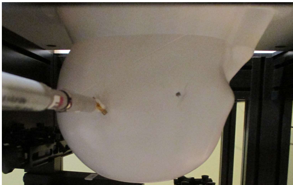
5 GHz Dipole Placed at Location A in 90° Orientation (10mm Spacer)
