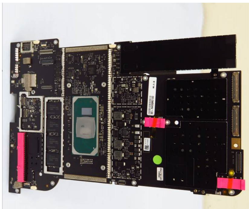
Motherboard with radio shield cans intact
