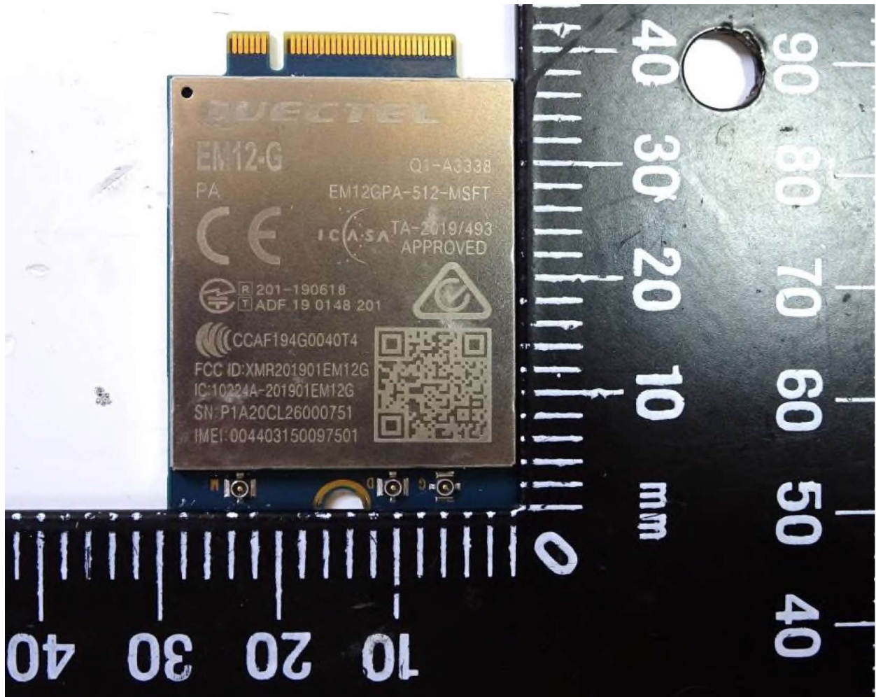
Module - Top View
