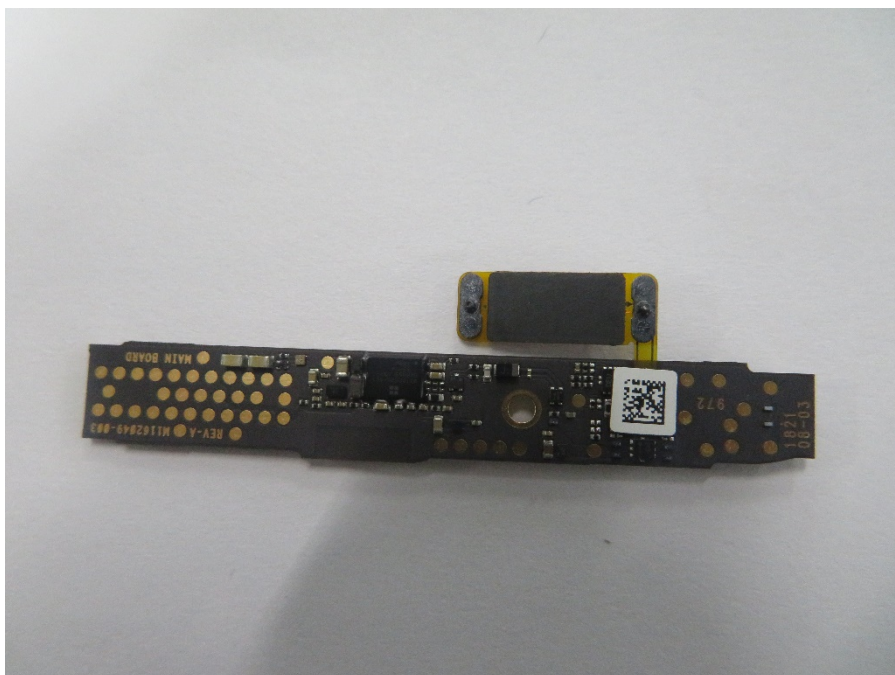
Main PCB + Coil FPC – View 2
