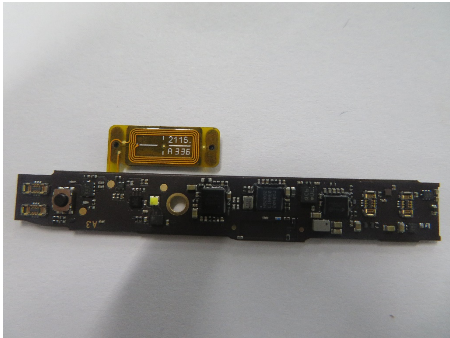
Main PCB + Coil FPC – View 1
