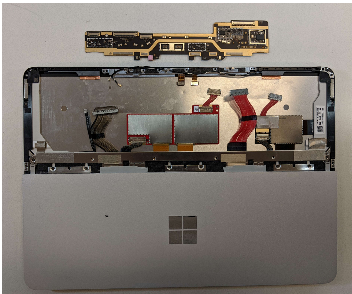
WLAN/BT Radio Board
