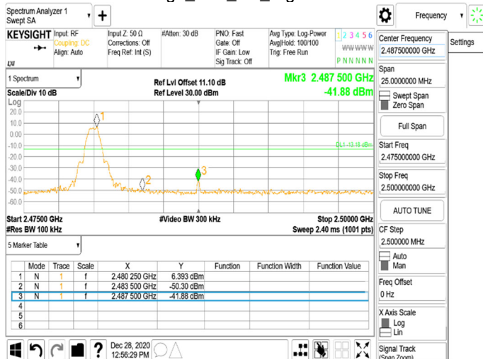
Band Edge_BLE_1M_HighCH39-2480
