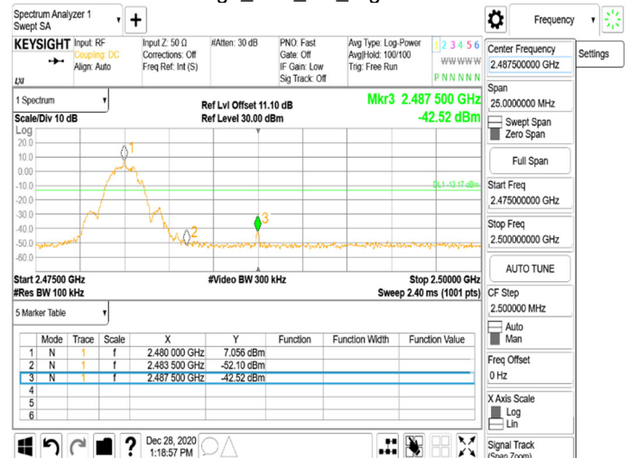
Band Edge_BLE_2M_HighCH39-2480
