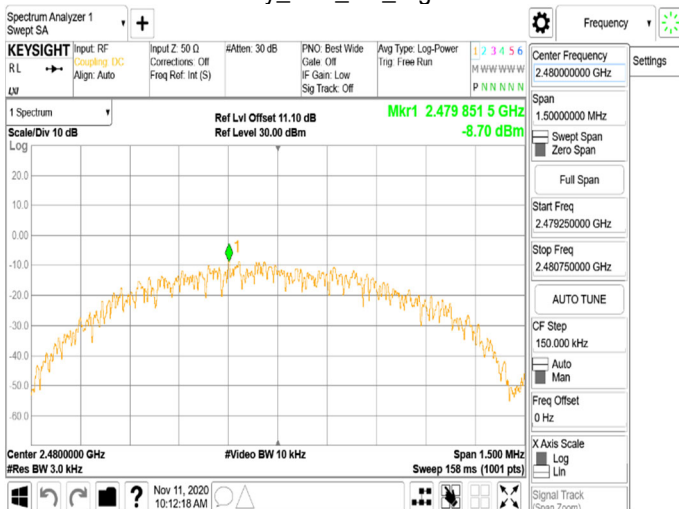
Power Density_BLE_1M_HighCH39-2480
