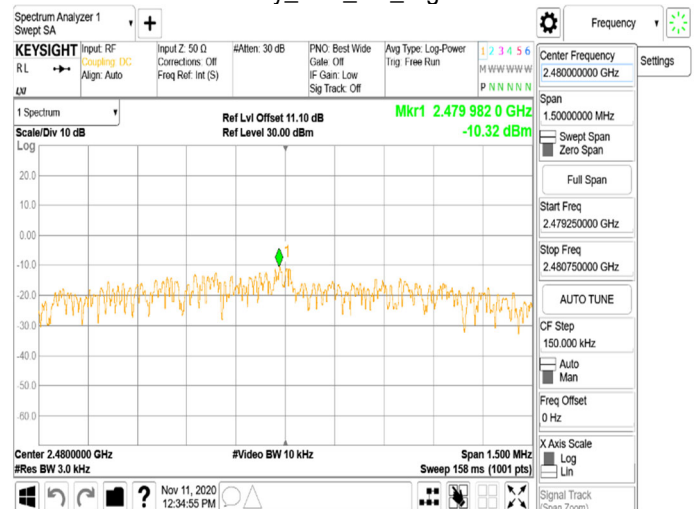
Power Density_BLE_2M_HighCH39-2480
