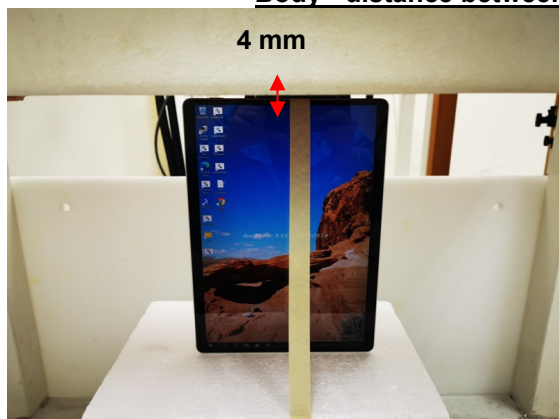
Photograph 21. Body, Right Edge, 4mm
