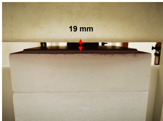
Photograph 15. Body, Back Surface, 19mm
