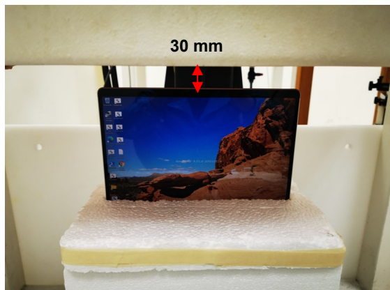
Photograph 17. Body, Top Edge, 30mm
