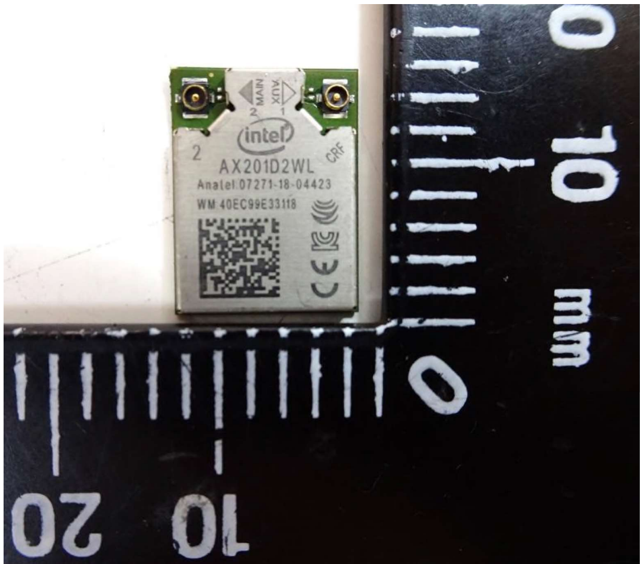
Module - Top View
