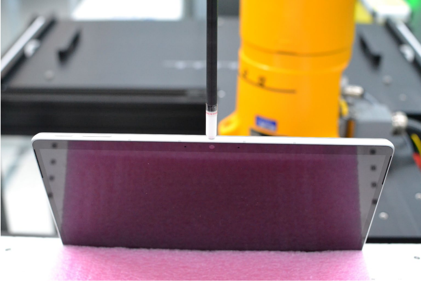
Figure E-5 Near Field Power Density Test Setup Photo – Top Edge at 2mm
