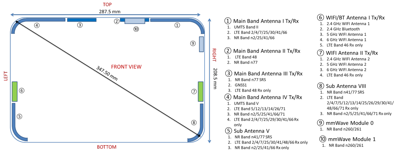
Figure E-1 DUT Antenna Locations
