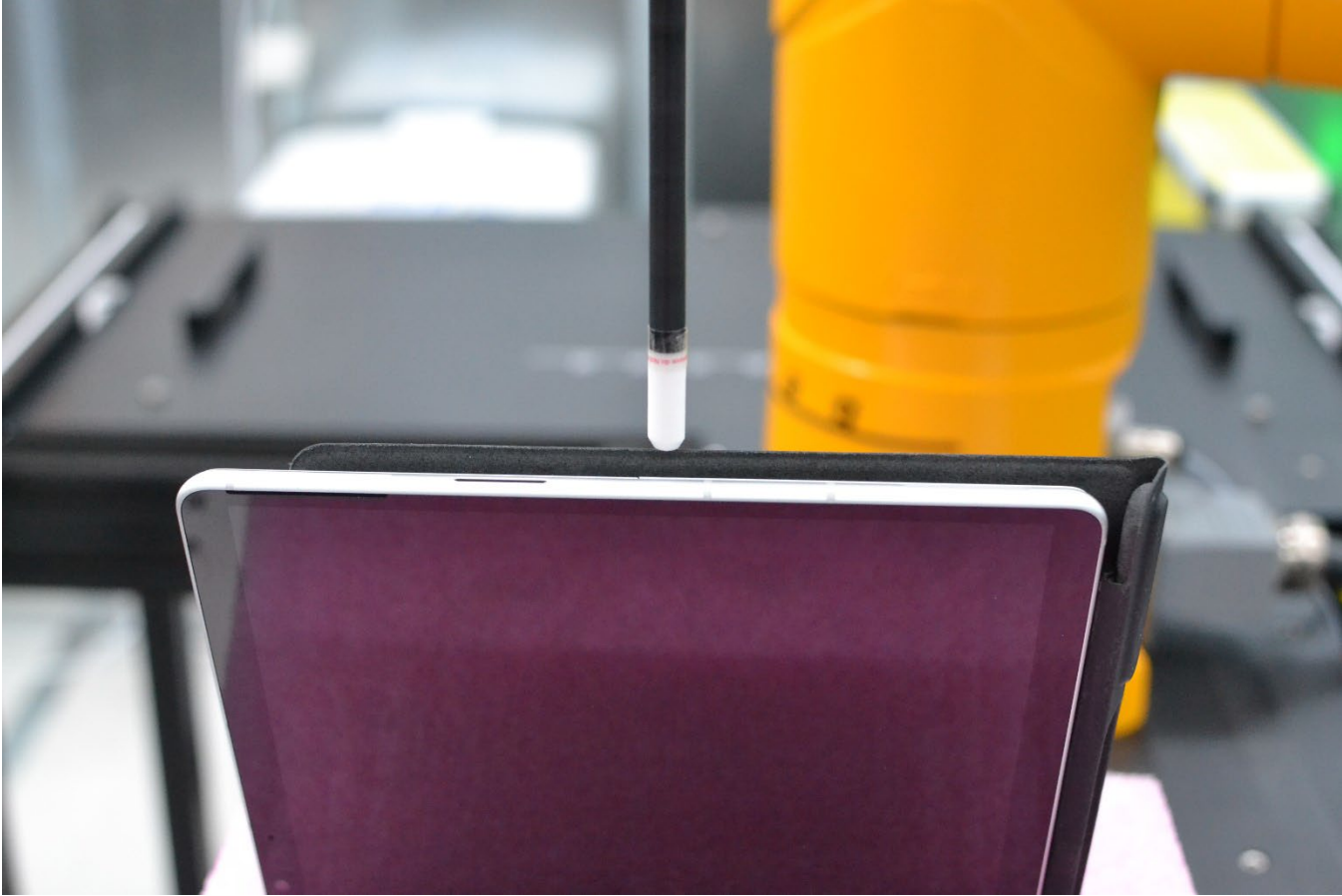
Figure E-7 Near Field Power Density Test Setup Photo – Right Edge at 2mm with Keyboard
