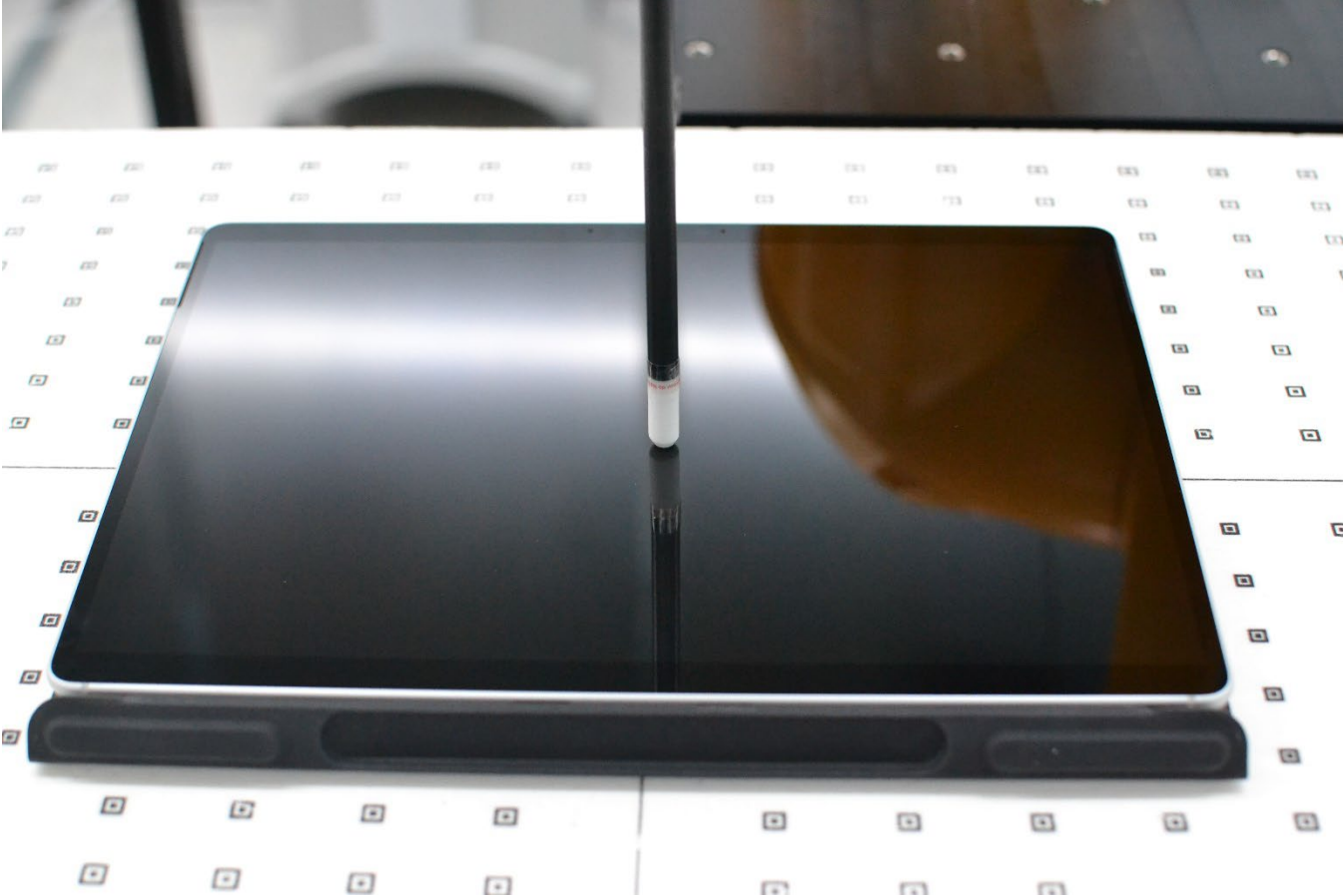
Figure E-4 Near Field Power Density Test Setup Photo – Front Side at 2mm with Keyboard
