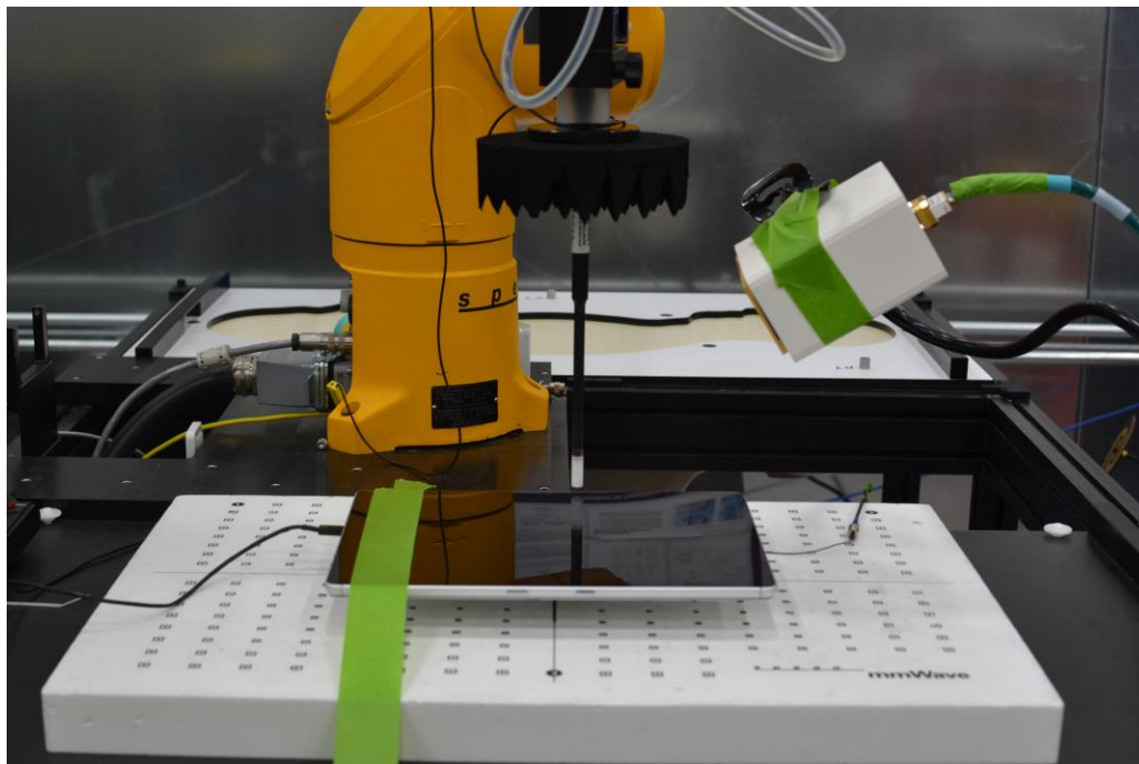
Test Setup Photo 10 – Power Density Setup Front Surface (Figure 7-2)
