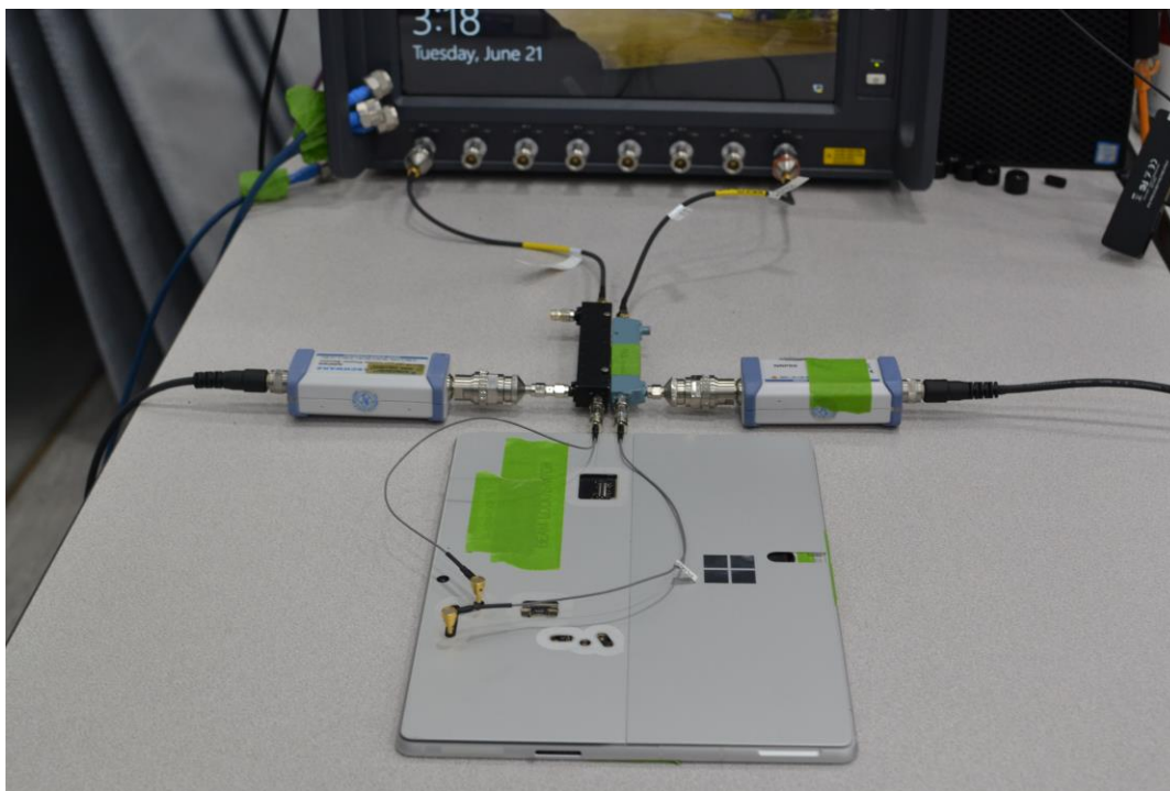
Test Setup Photo 7 – Conducted Test Setup (Figure 6-1c)
