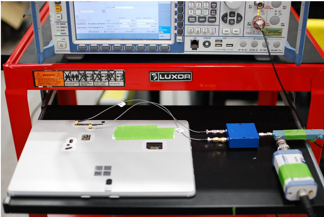
Test Setup Photo 5 - Conducted Test Setup (Figure 6-1b)
