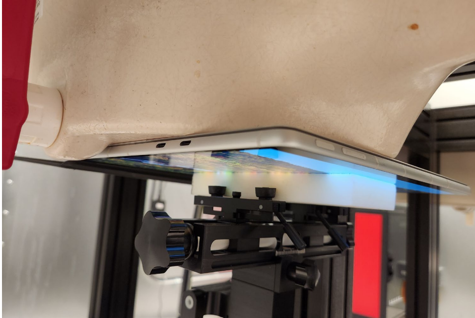
Test Setup Photo 4 – Back Side, Bottom - Left at 0 mm
