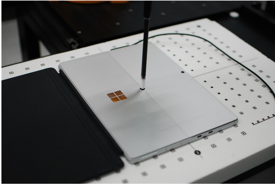
Test Setup Photo 6 – Back Side at 2 mm
