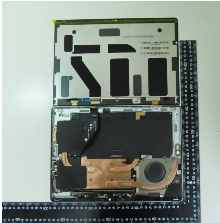
Open View of EUT – 1
