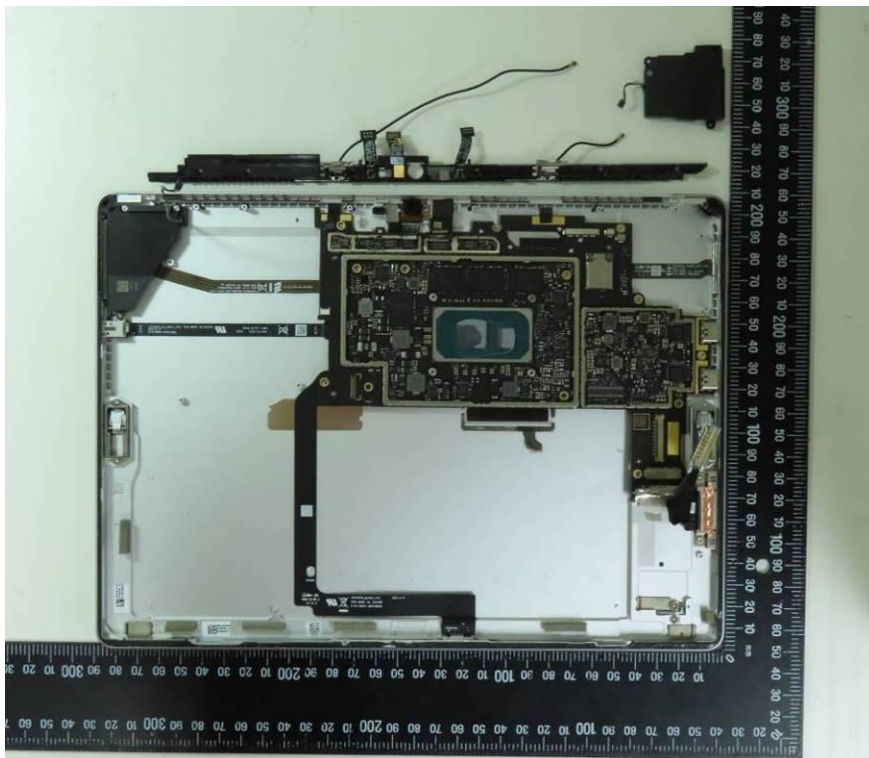
Open View of EUT – 6
