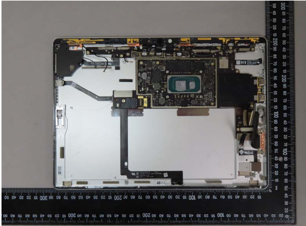
Open View of EUT-9
