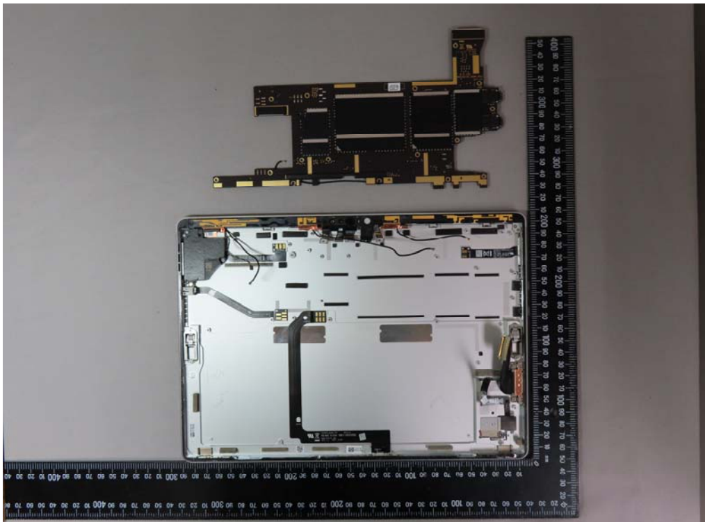
Open View of EUT-10
