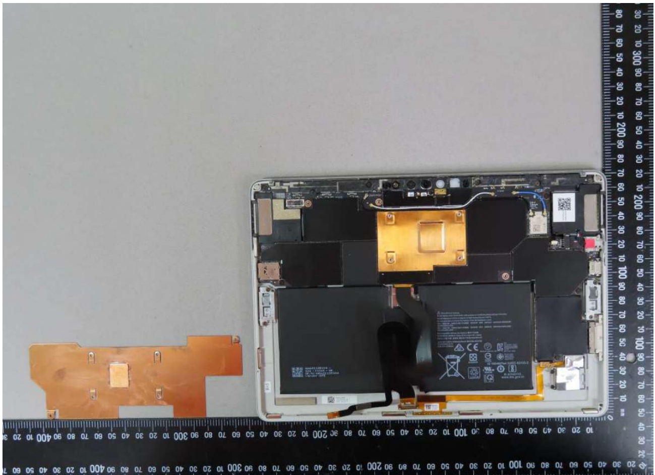
Open view-2
