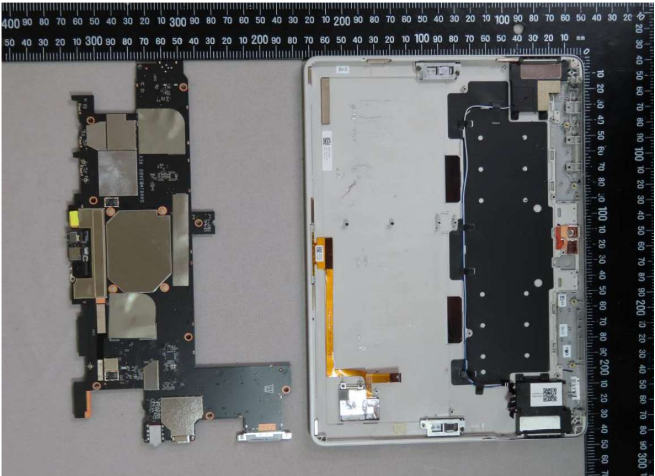
Internal view-1
