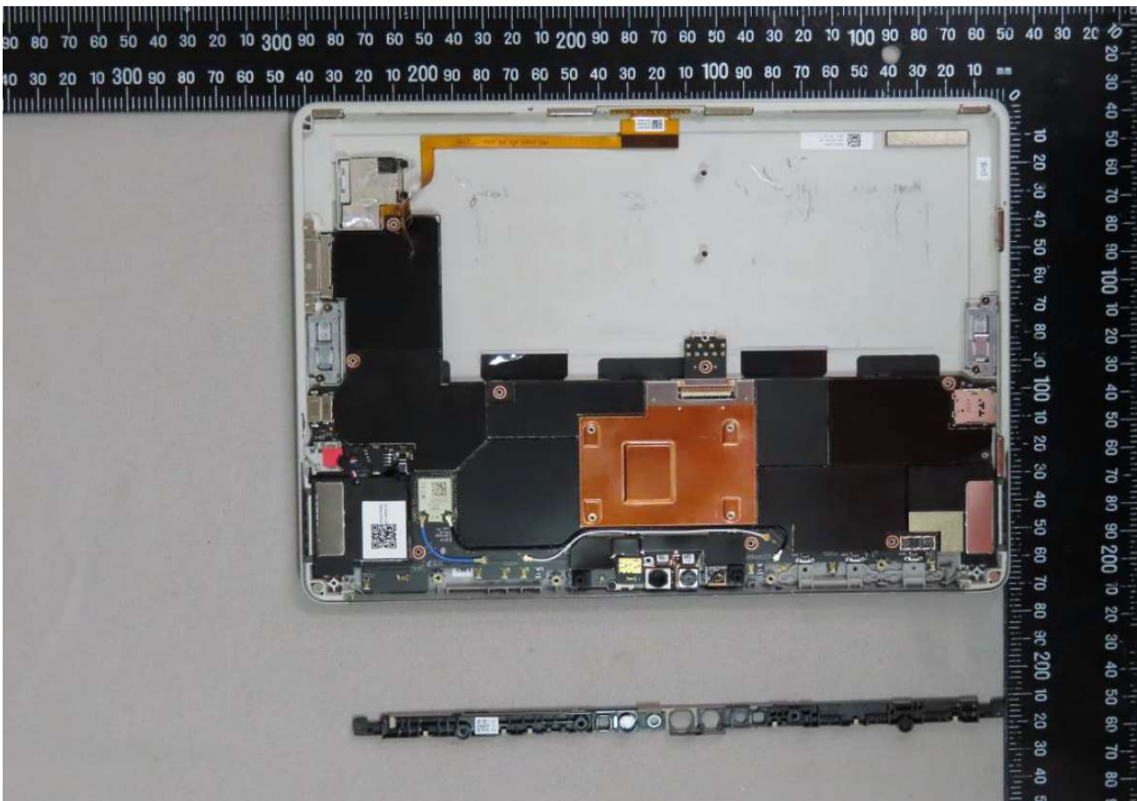
Open view-4
