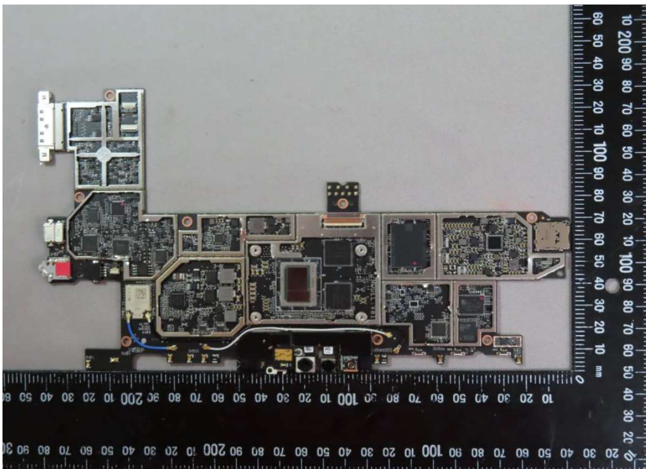
Internal view-3
