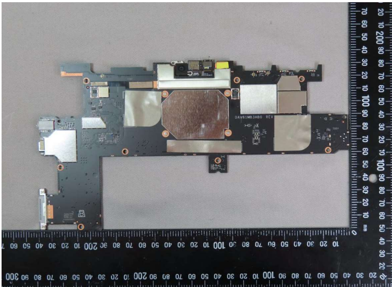
Internal view-3
