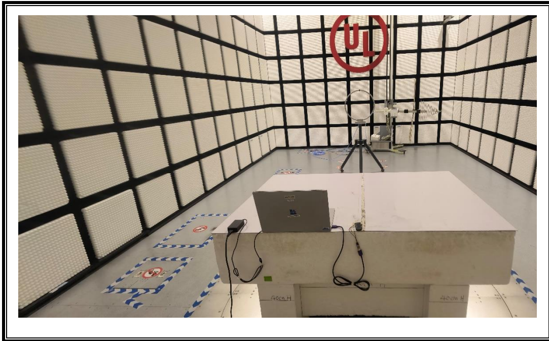
RADIATED RF MEASUREMENT SETUP (Above 1G – X axis)
