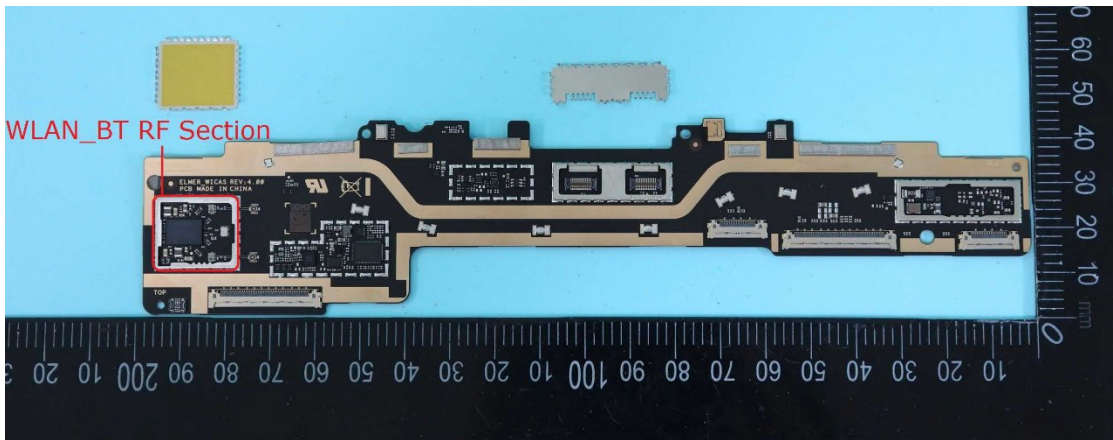
WiFi board – shield removed
