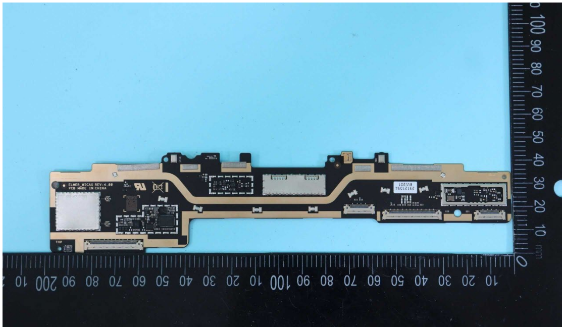
WiFi board
