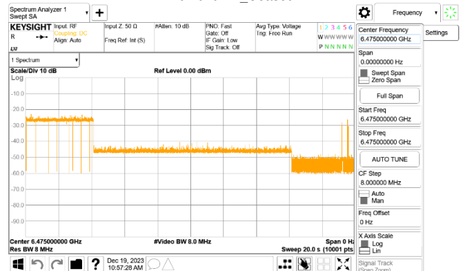
802.11HE_20MHz_CF 6475MHz_Interference_6475MHz_ -71.01dBm_Minimal
