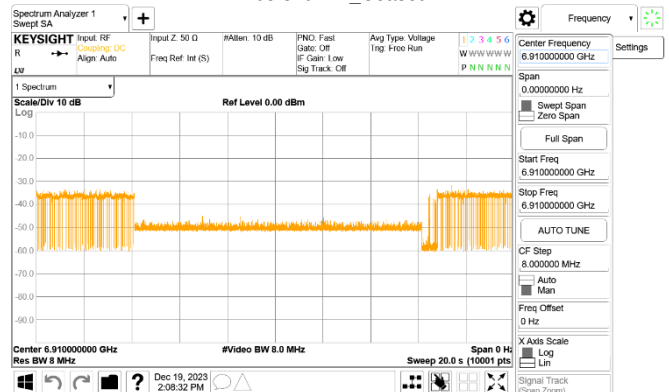
802.11HE_160MHz_CF 6985MHz_Interference_6910MHz_ -68.82dBm_Minimal
