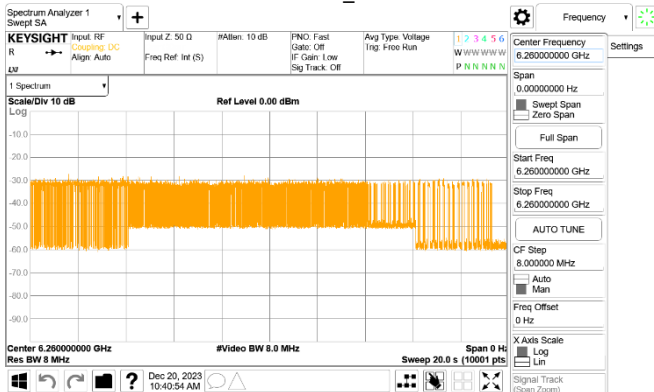
802.11HE_160MHz_CF 6185MHz_Interference_6260MHz_-66.28dBm_Normal
