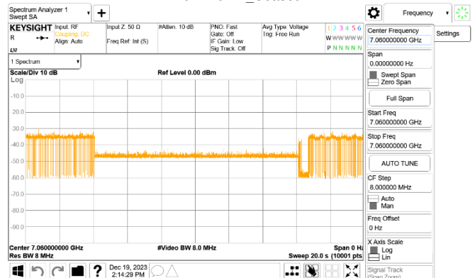
802.11HE_160MHz_CF 6985MHz_Interference_7060MHz_-63.77dBm_Minimal
