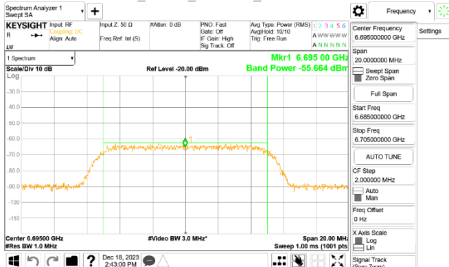
802.11HE_20MHz_6695MHz_AWGN:6695MHz
