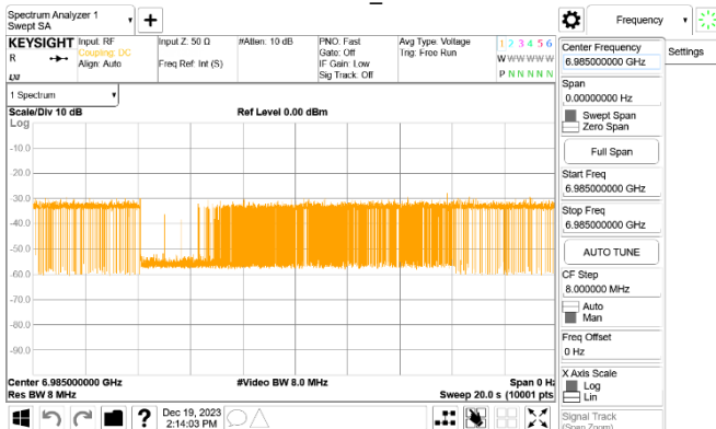
802.11HE_160MHz_CF 6985MHz_Interference_6985MHz_-73.7dBm_Normal
