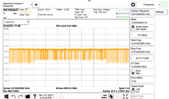
802.11HE_160MHz_CF 6985MHz_Interference_6910MHz_ -70.82dBm_Normal
