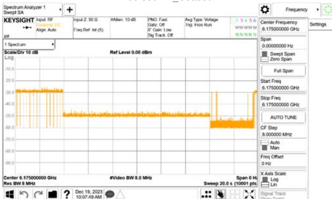
802.11HE_20MHz_CF 6175MHz_Interference_6175MHz_ -74.33dBm_Minimal
