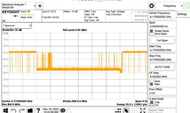
802.11HE_20MHz_CF 6175MHz_Interference_6175MHz_ -77.33dBm_Normal
