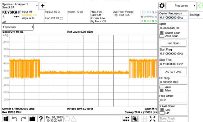
802.11HE_160MHz_CF 6185MHz_Interference_6110MHz_ -71.79dBm_Minimal
