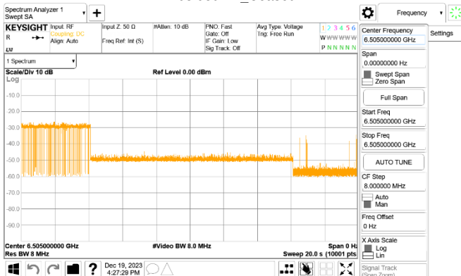
802.11HE_160MHz_CF 6505MHz_Interference_6505MHz_-71.95dBm_Minimal
