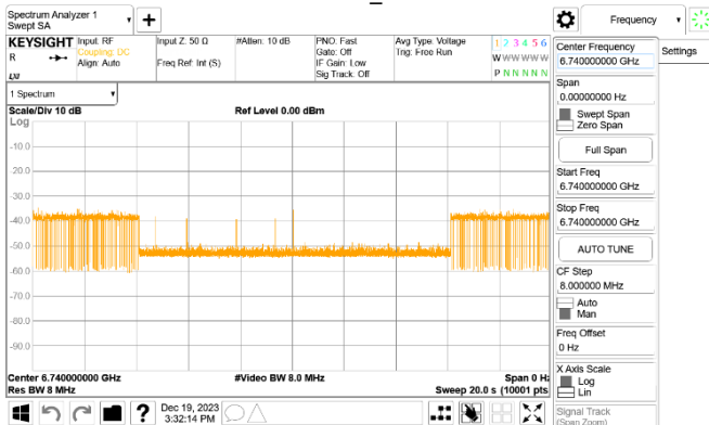
802.11HE_160MHz_CF 6665MHz_Interference_6740MHz_ -73.85dBm_Normal
