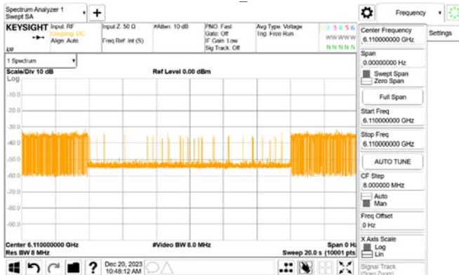
802.11HE_160MHz_CF 6185MHz_Interference_6110MHz_ -73.29dBm_Normal
