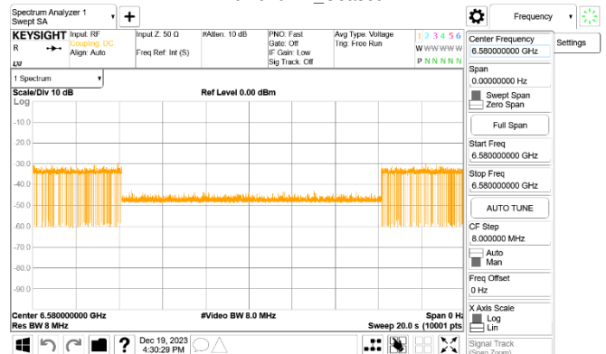
802.11HE_160MHz_CF 6505MHz_Interference_6580MHz_-63.92dBm_Minimal
