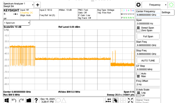
802.11HE_160MHz_CF 6665MHz_Interference_6665MHz_-69.68dBm_Minimal
