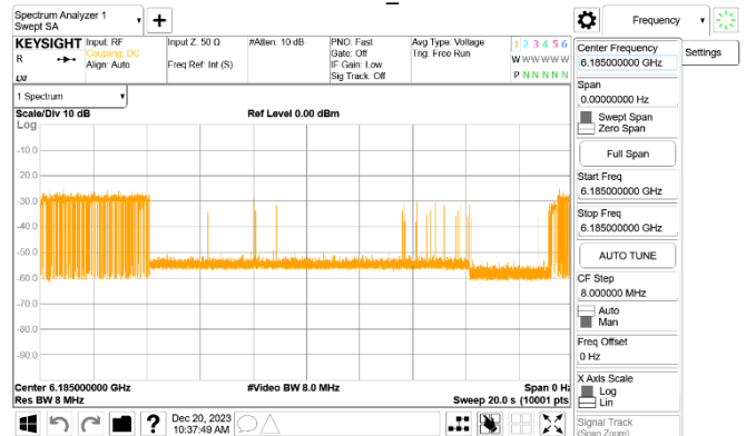
802.11HE_160MHz_CF 6185MHz_Interference_6185MHz_ -76.18dBm_Normal
