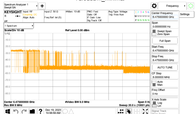
802.11HE_20MHz_CF 6475MHz_Interference_6475MHz_ -74.01dBm_Normal
