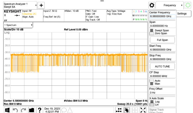
802.11HE_160MHz_CF 6505MHz_Interference_6580MHz_-65.92dBm_Normal
