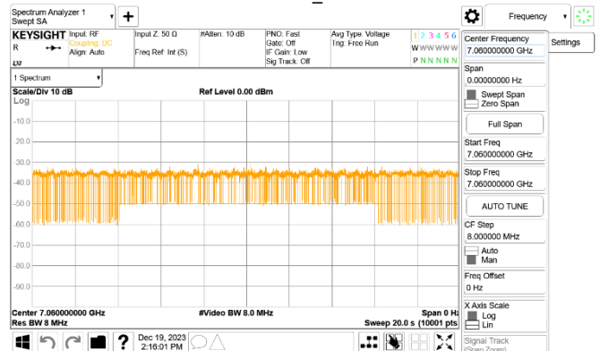
802.11HE_160MHz_CF 6985MHz_Interference_7060MHz_-65.77dBm_Normal
