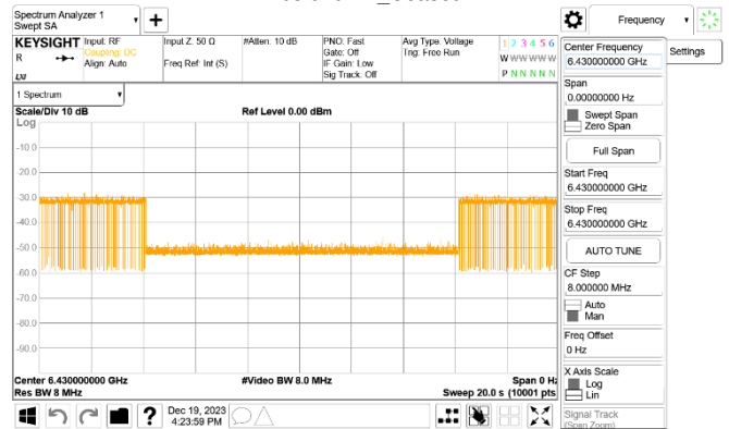
802.11HE_160MHz_CF 6505MHz_Interference_6430MHz_-71.97dBm_Minimal
