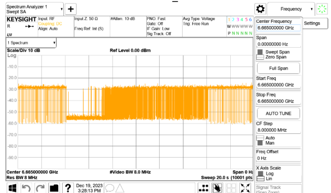
802.11HE_160MHz_CF 6665MHz_Interference_6665MHz_-73.68dBm_Normal
