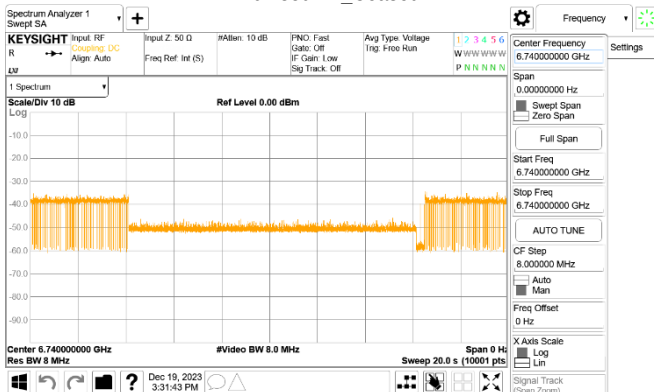
802.11HE_160MHz_CF 6665MHz_Interference_6740MHz_ -70.85dBm_Minimal
