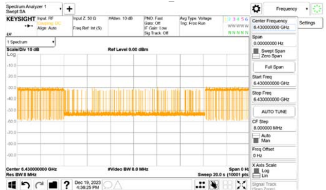
802.11HE_160MHz_CF 6505MHz_Interference_6430MHz_-72.97dBm_Normal
