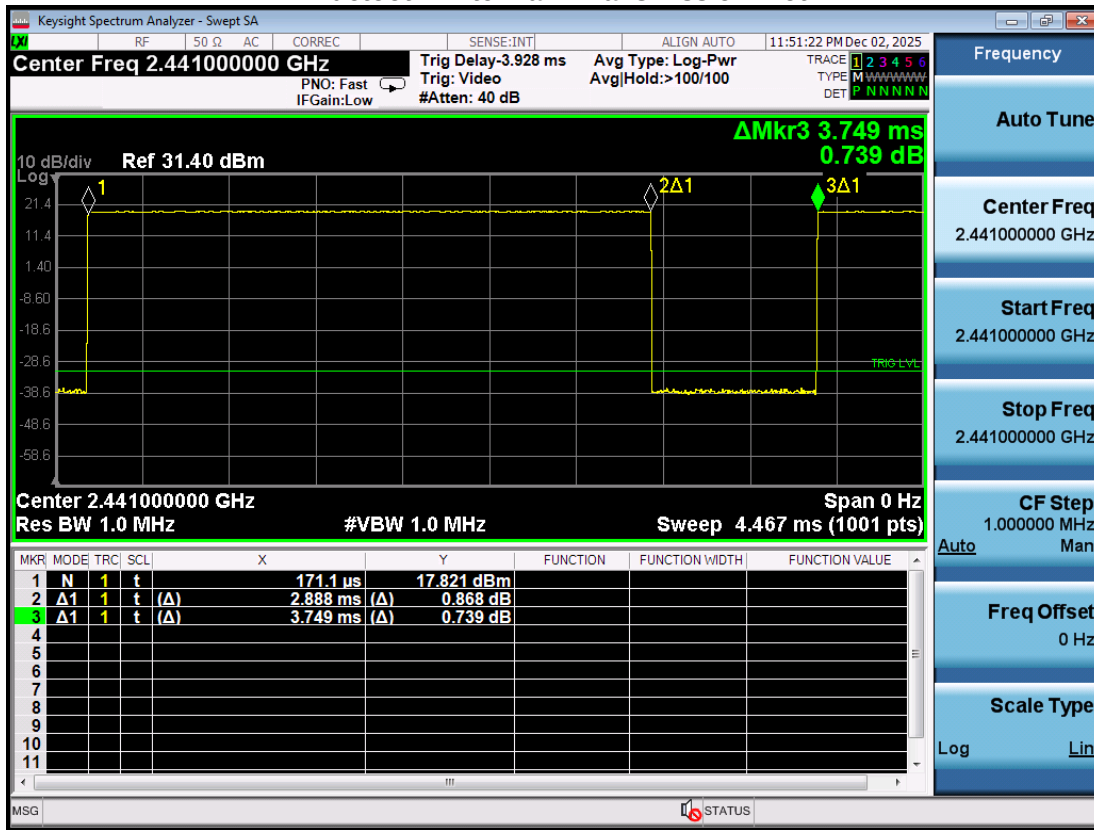
Figure 8-2 Bluetooth Antenna R Transmission Plot
