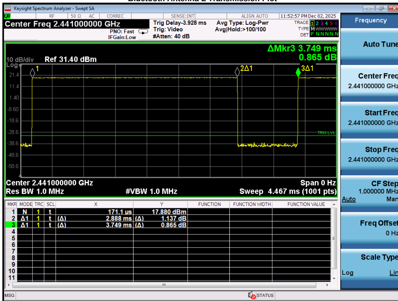
Figure 8-3 Bluetooth Antenna L Transmission Plot
