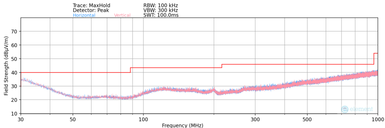
Plot 7-178. Radiated Spurious Plot below 1GHz
