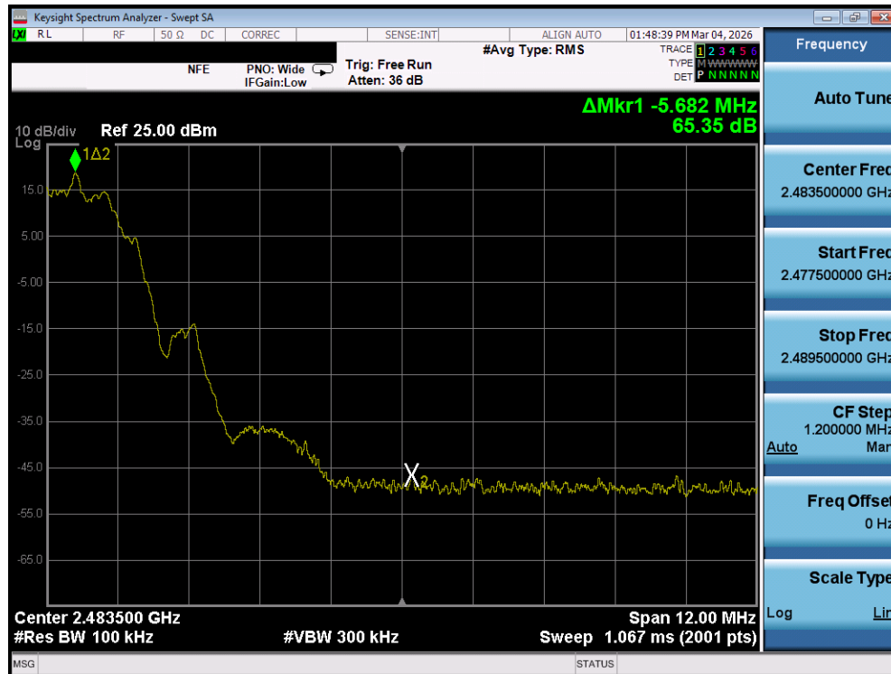
Plot 7-128. Band Edge Plot (Bluetooth (LE), 2Mbps – Ch. 36) – SISO ANT1
