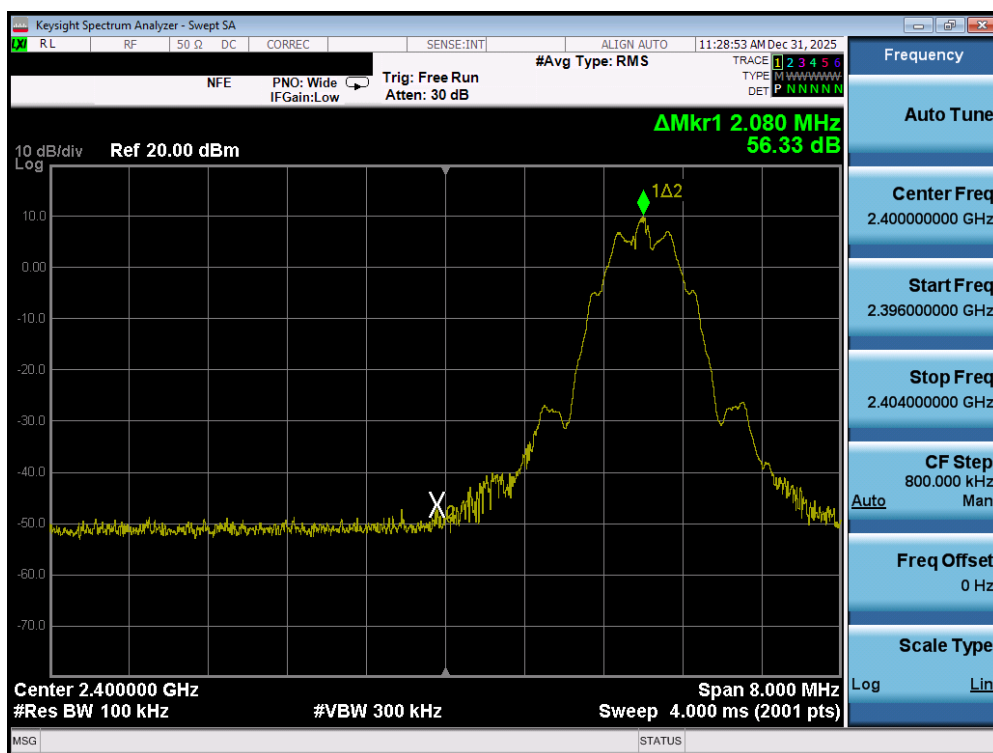
Plot 7-121. Band Edge Plot (Bluetooth (LE), 125kbps – Ch. 37) – SISO ANT1
