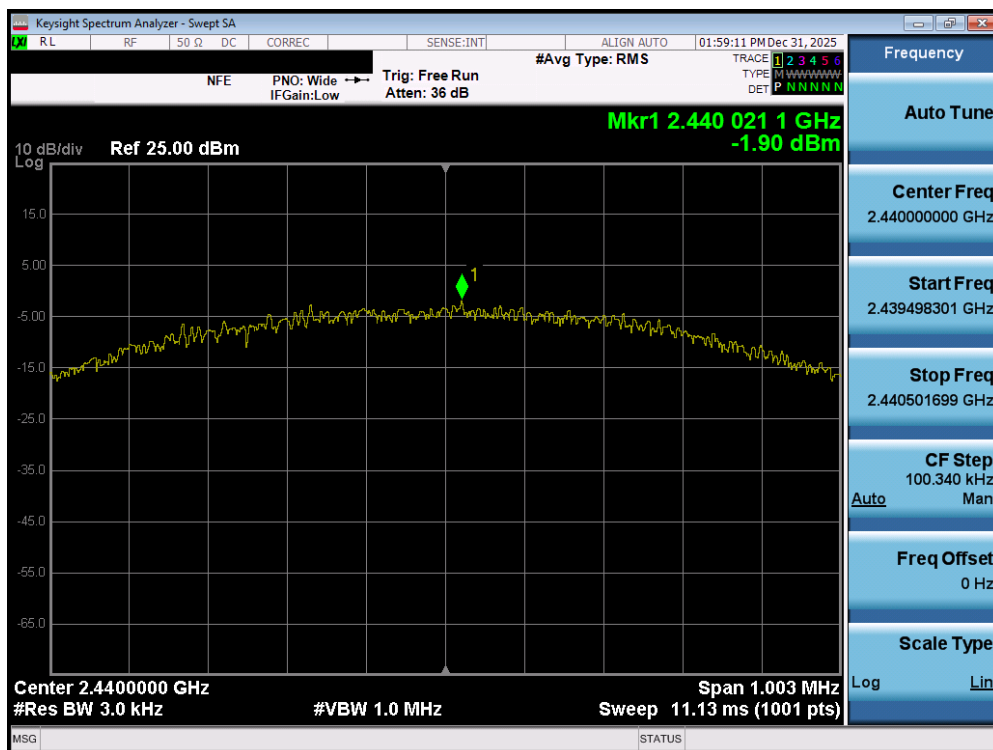
Plot 7-116. Power Spectral Density Plot (Bluetooth (LE), 1Mbps – Ch. 17) – DUAL ANT2
