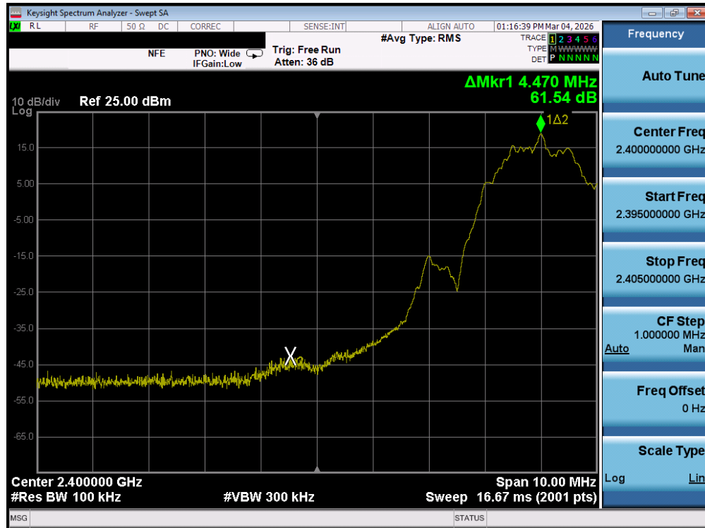
Plot 7-127. Band Edge Plot (Bluetooth (LE), 2Mbps – Ch. 0) – SISO ANT1
