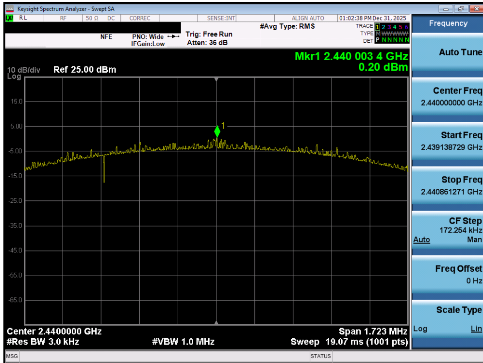
Plot 7-107. Power Spectral Density Plot (Bluetooth (LE), 2Mbps – Ch. 17) – SISO ANT2
