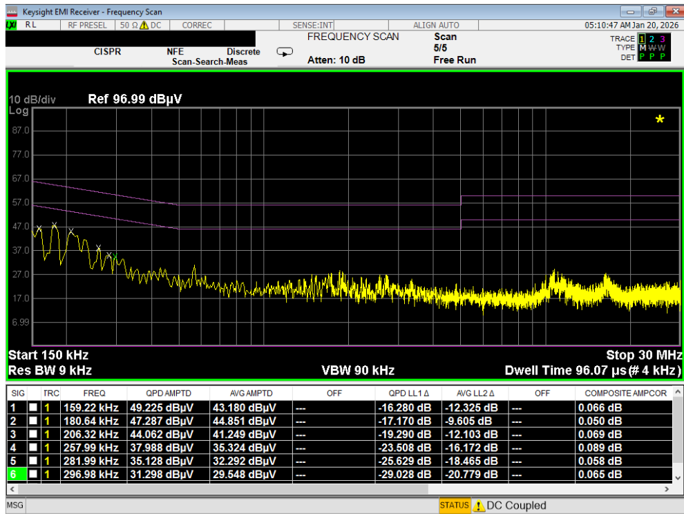
Plot 7-185. Line Conducted Plot with Bluetooth LE (L1)
