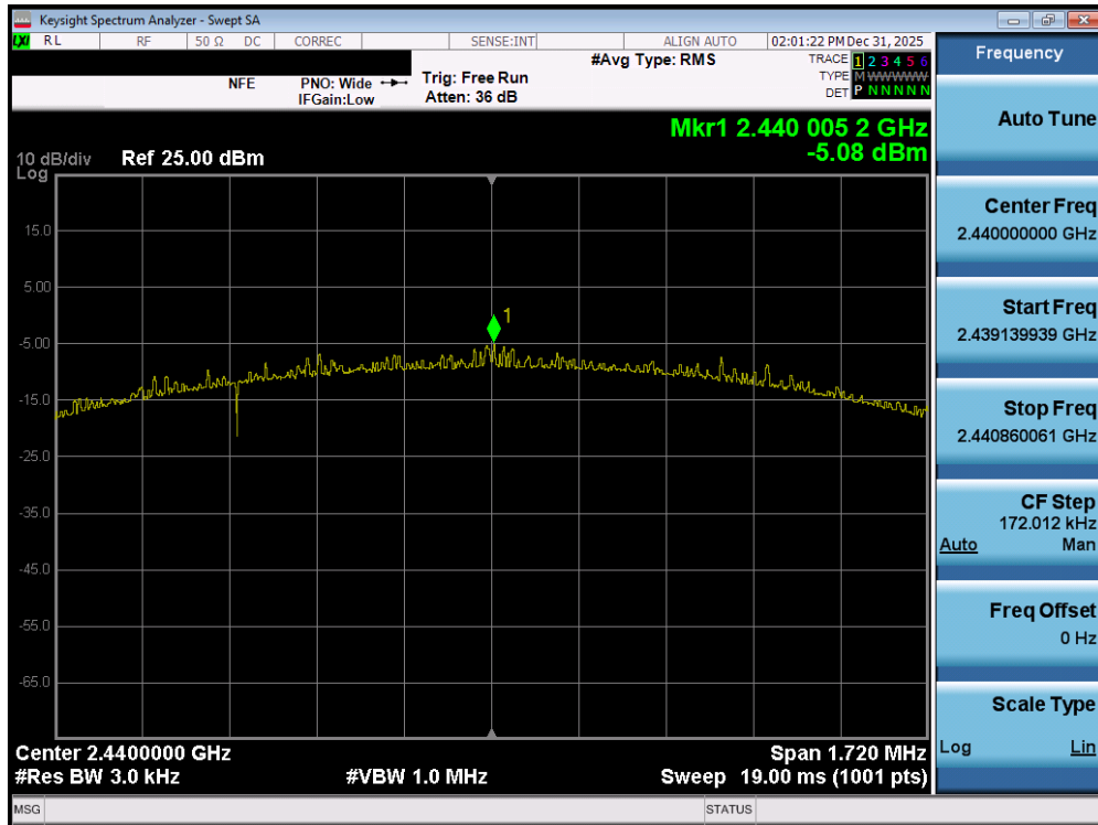
Plot 7-119. Power Spectral Density Plot (Bluetooth (LE), 2Mbps – Ch. 17) – DUAL ANT2
