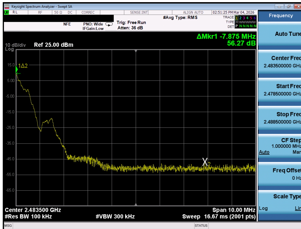
Plot 7-144. Band Edge Plot (Bluetooth (LE), 2Mbps - Ch. 36) - DUAL ANT2
