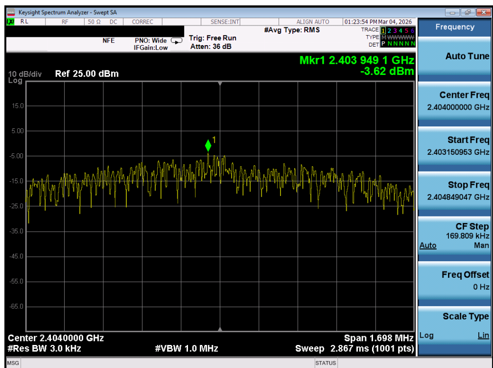
Plot 7-112. Power Spectral Density Plot (Bluetooth (LE), 2Mbps – Ch. 0) – DUAL ANT1
