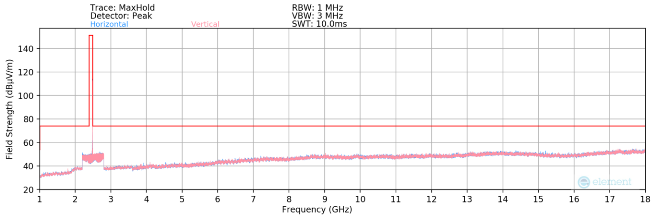
Plot 7-171. Radiated Spurious Plot above 1GHz (Bluetooth (LE) – Ch. 39) – Ant 1
