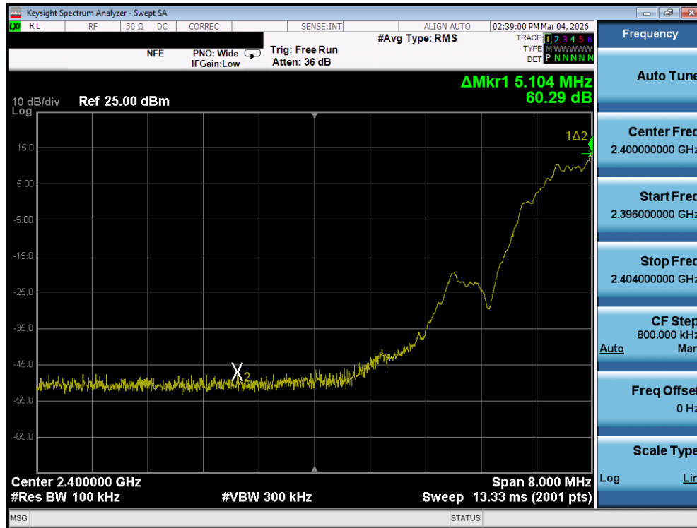
Plot 7-143. Band Edge Plot (Bluetooth (LE), 2Mbps - Ch. 0) - DUAL ANT2
