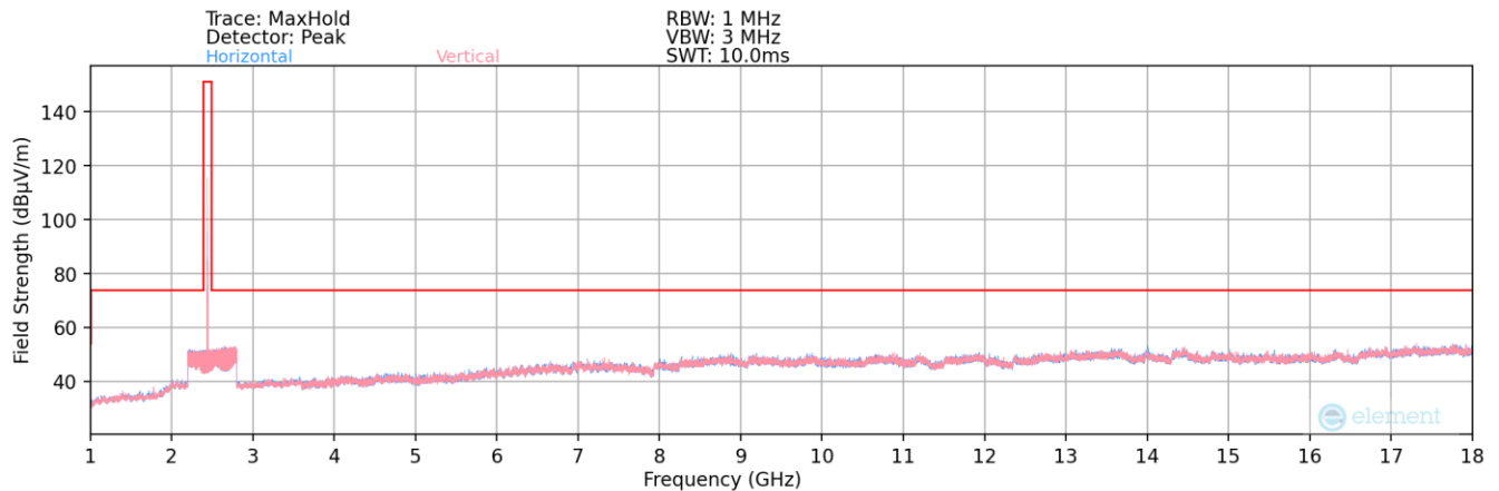
Plot 7-176. Radiated Spurious Plot above 1GHz (Bluetooth (LE) – Ch. 17) – DUAL
