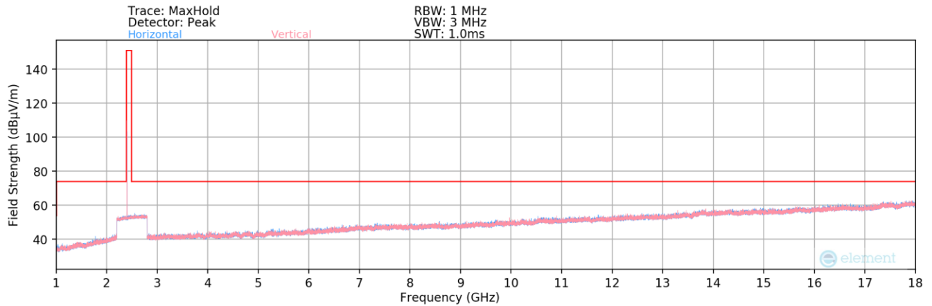
Plot 7-172. Radiated Spurious Plot above 1GHz (Bluetooth (LE) – Ch. 37) – Ant 2
