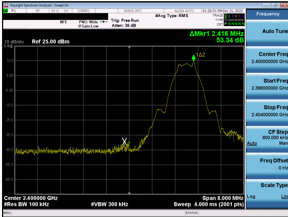
Plot 7-137. Band Edge Plot (Bluetooth (LE), 1Mbps – Ch. 37) – DUAL ANT1
