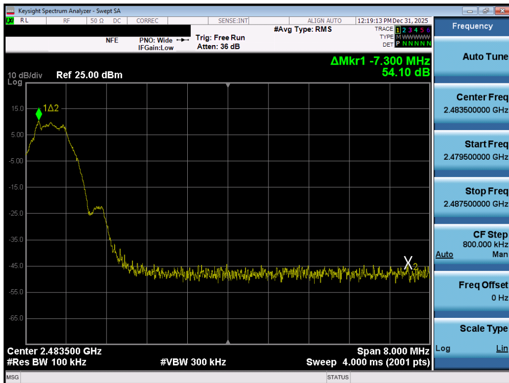
Plot 7-124. Band Edge Plot (Bluetooth (LE), 500kbps – Ch. 39) – SISO ANT1
