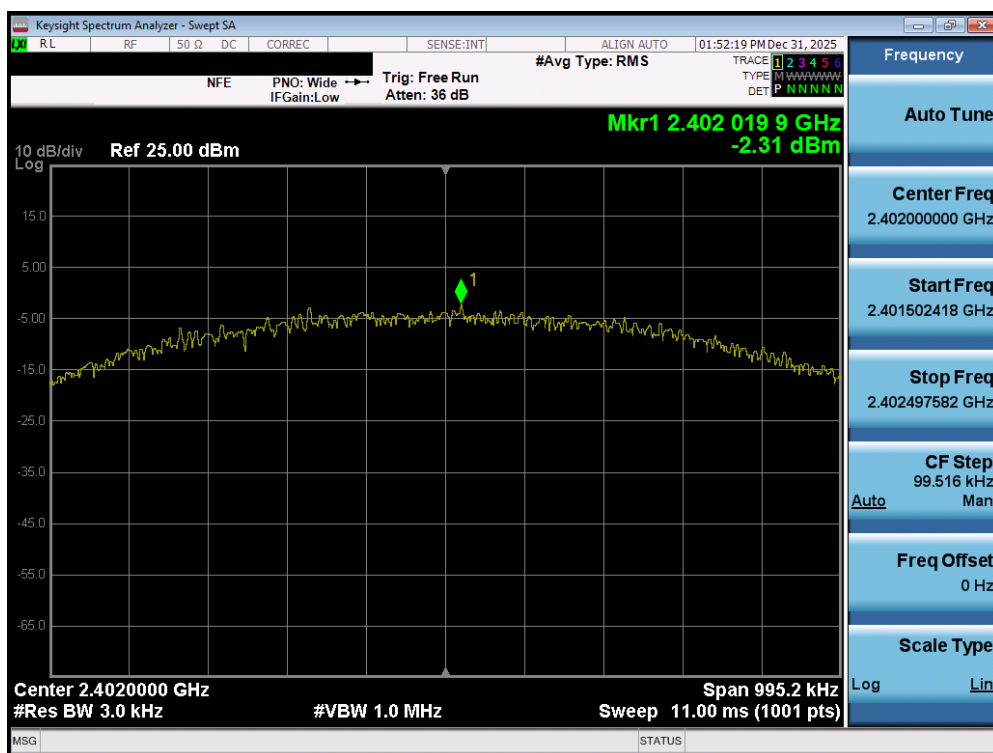
Plot 7-115. Power Spectral Density Plot (Bluetooth (LE), 1Mbps – Ch. 37) – DUAL ANT2
