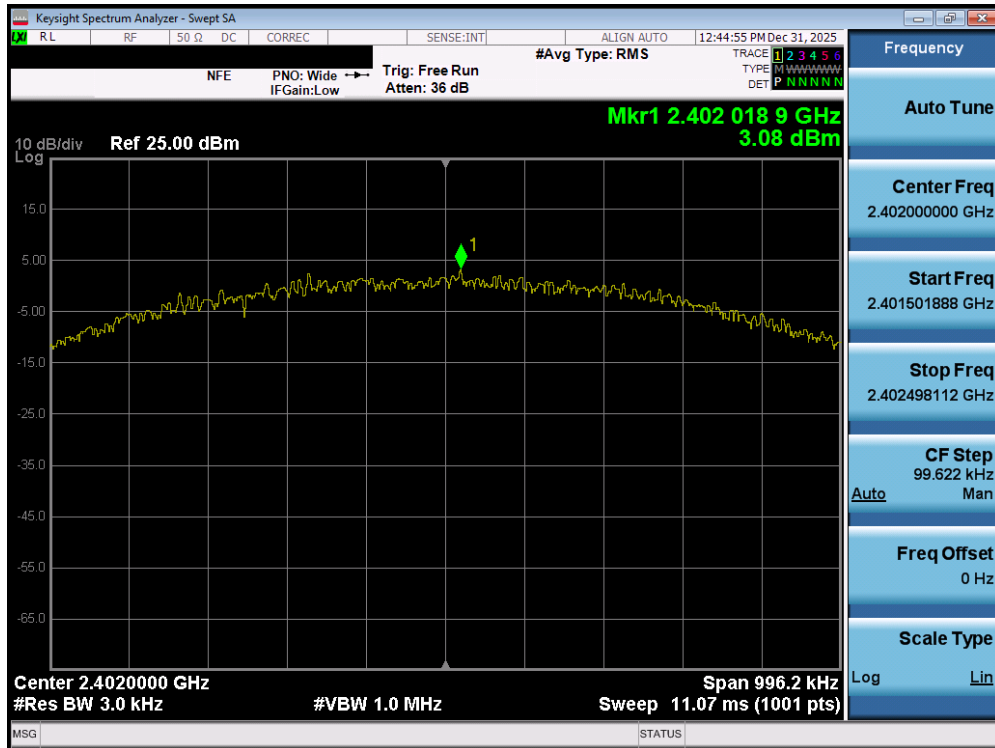
Plot 7-103. Power Spectral Density Plot (Bluetooth (LE), 1Mbps – Ch. 37) – SISO ANT2
