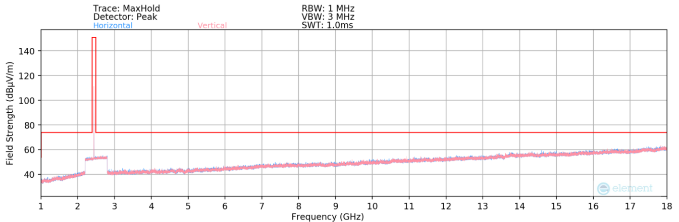
Plot 7-173. Radiated Spurious Plot above 1GHz (Bluetooth (LE) – Ch. 17) – Ant 2
