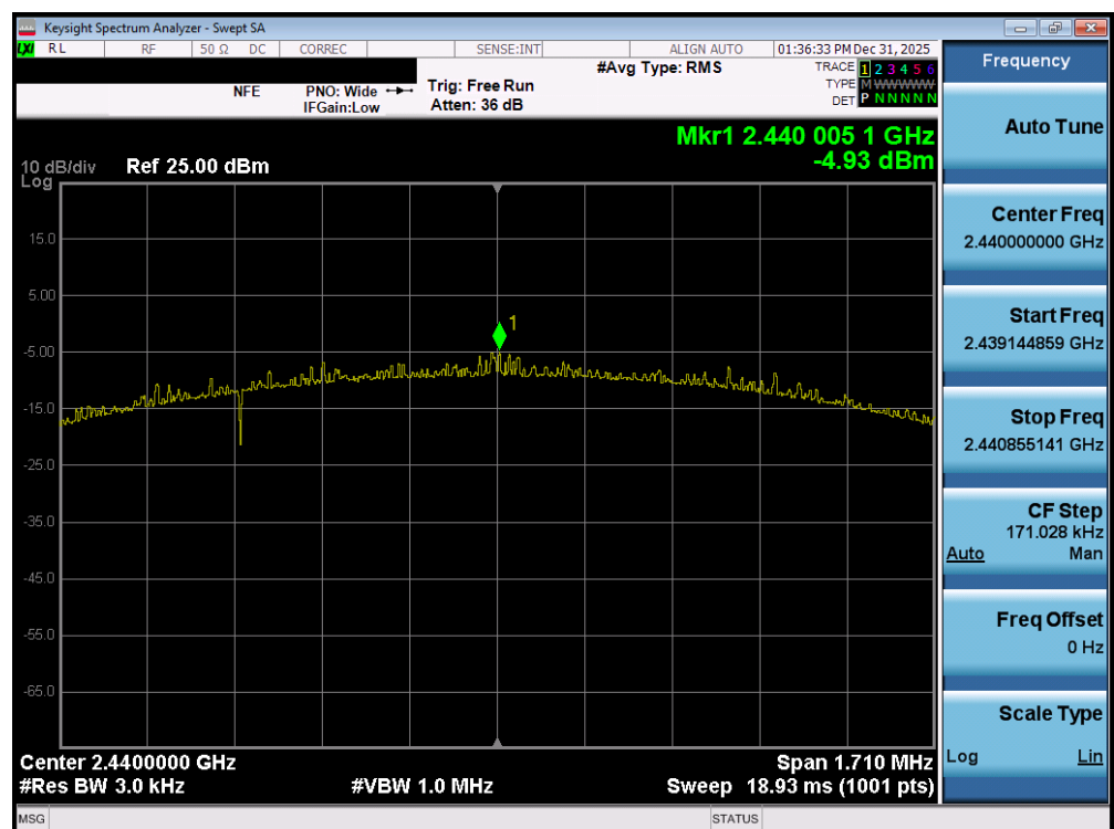
Plot 7-113. Power Spectral Density Plot (Bluetooth (LE), 2Mbps – Ch. 17) – DUAL ANT1
