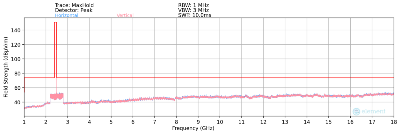
Plot 7-177. Radiated Spurious Plot above 1GHz (Bluetooth (LE) – Ch. 39) – DUAL
