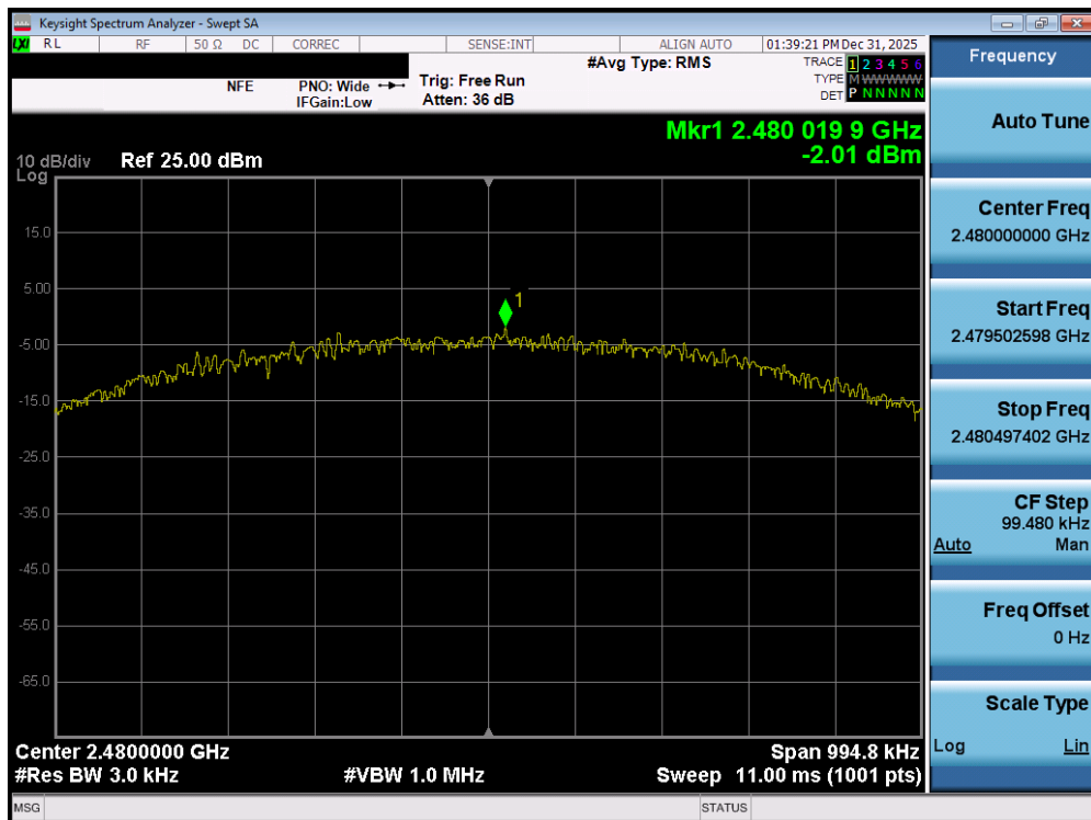
Plot 7-111. Power Spectral Density Plot (Bluetooth (LE), 1Mbps – Ch. 39) – DUAL ANT1
