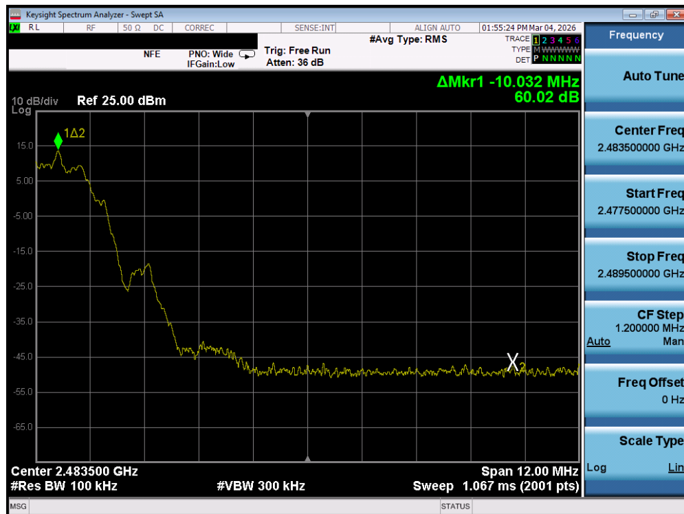
Plot 7-140. Band Edge Plot (Bluetooth (LE), 2Mbps - Ch. 36) - DUAL ANT1
