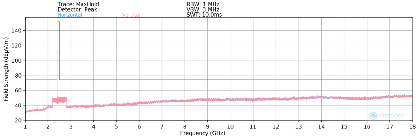
Plot 7-169. Radiated Spurious Plot above 1GHz (Bluetooth (LE) – Ch. 37) – Ant 1
