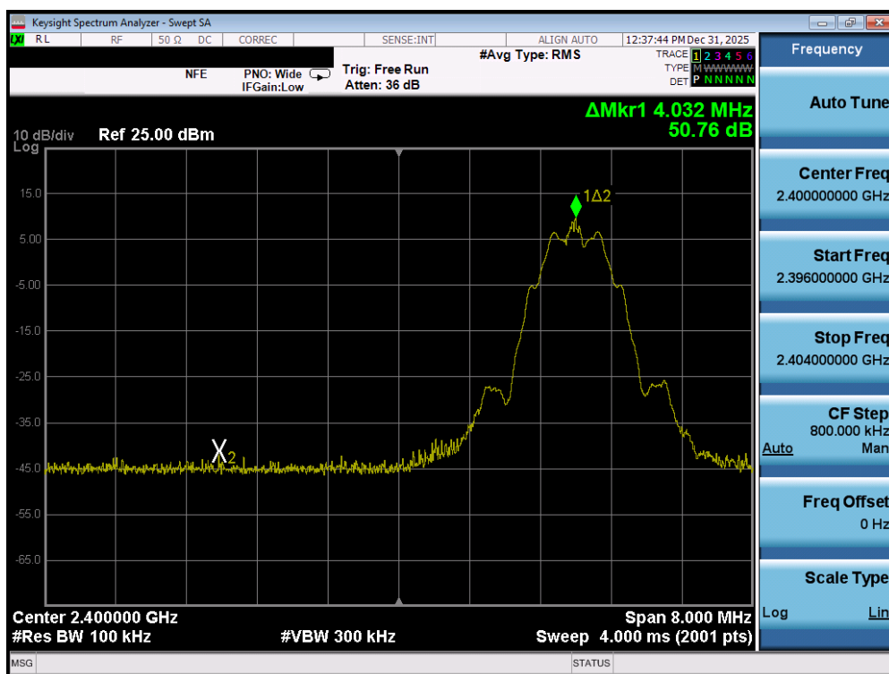
Plot 7-129. Band Edge Plot (Bluetooth (LE), 125kbps – Ch. 37) – SISO ANT2
