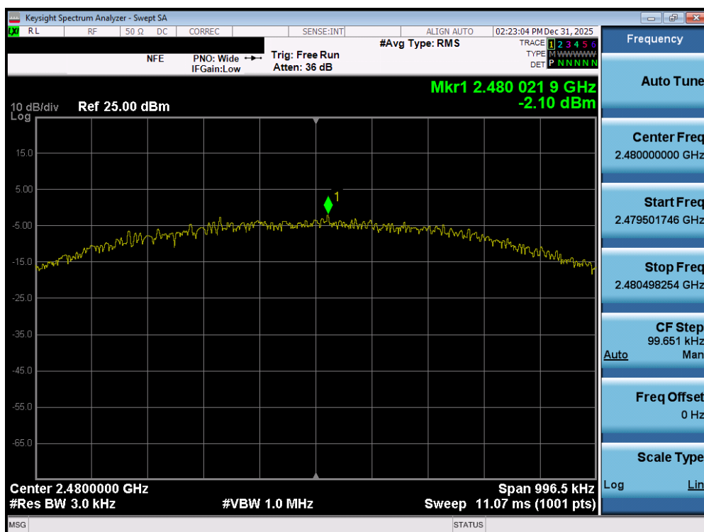
Plot 7-117. Power Spectral Density Plot (Bluetooth (LE), 1Mbps – Ch. 39) – DUAL ANT2
