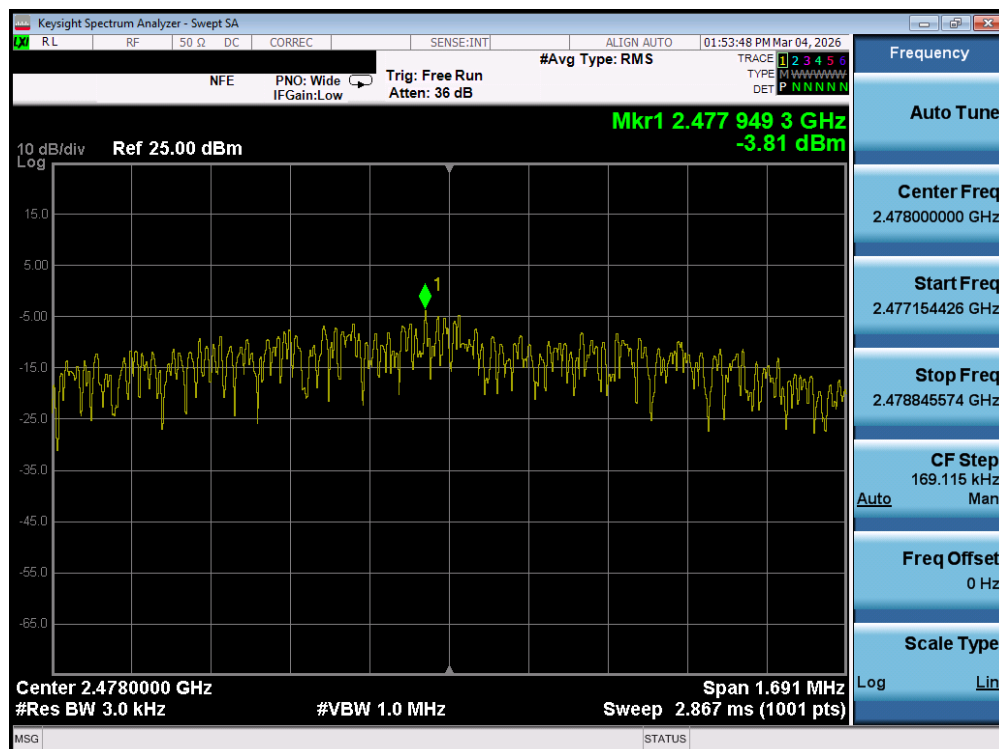
Plot 7-114. Power Spectral Density Plot (Bluetooth (LE), 2Mbps – Ch. 36) – DUAL ANT1
