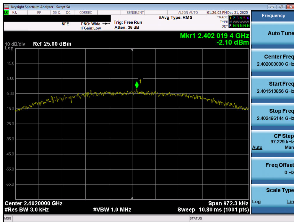
Plot 7-109. Power Spectral Density Plot (Bluetooth (LE), 1Mbps – Ch. 37) – DUAL ANT1
