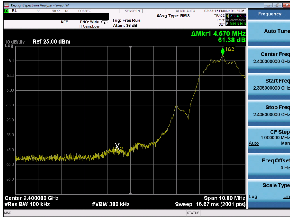
Plot 7-135. Band Edge Plot (Bluetooth (LE), 2Mbps – Ch. 0) – SISO ANT2
