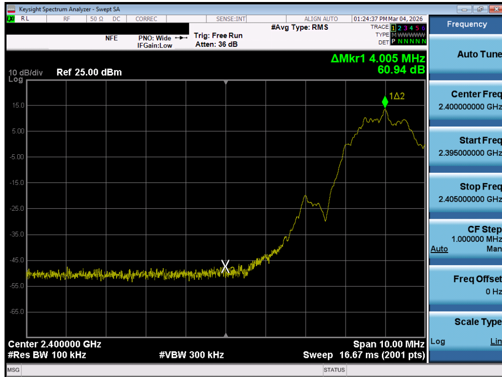
Plot 7-139. Band Edge Plot (Bluetooth (LE), 2Mbps - Ch. 0) - DUAL ANT1
