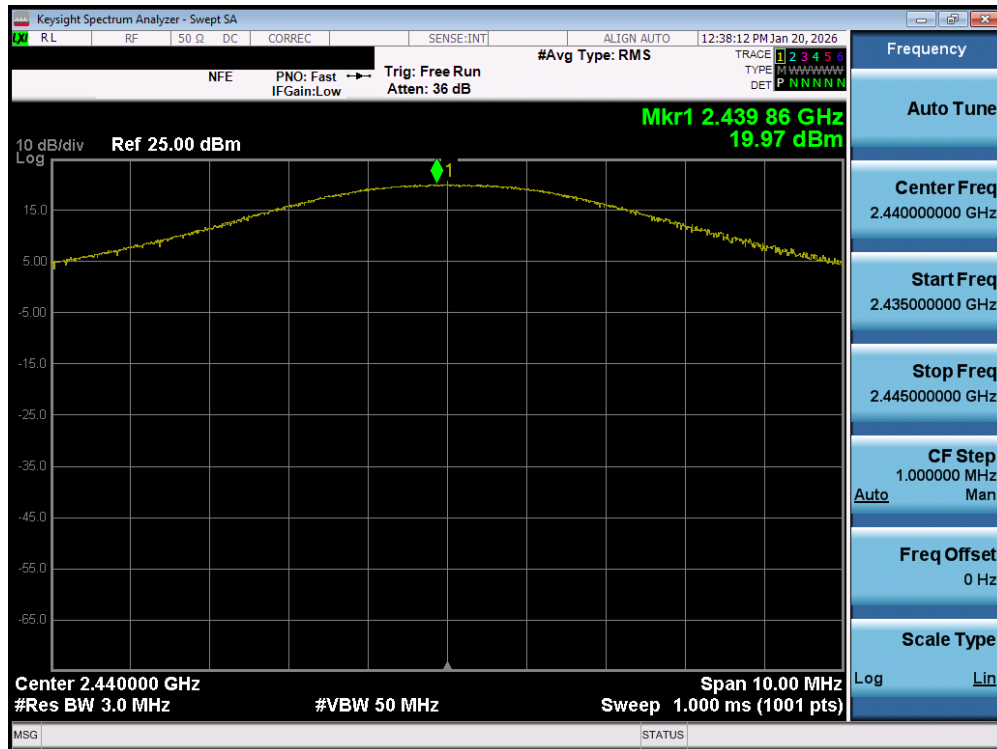
Plot 9-1. Conducted Output Power Measurements SISO ANT1 (Spot-check)
