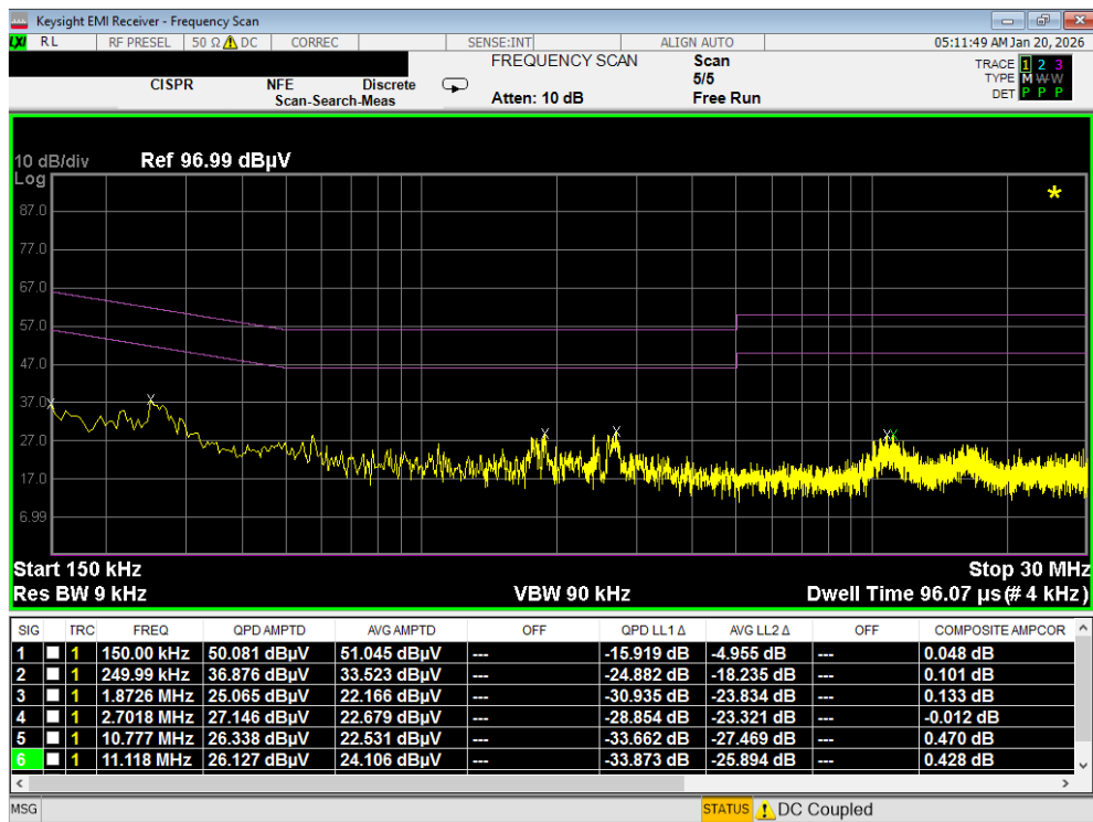
Plot 7-186. Line Conducted Plot with Bluetooth LE (N)
