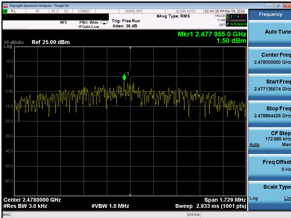
Plot 7-108. Power Spectral Density Plot (Bluetooth (LE), 2Mbps – Ch. 36) – SISO ANT2
