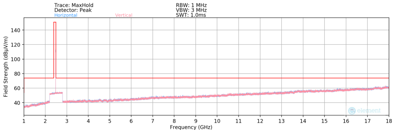
Plot 7-174. Radiated Spurious Plot above 1GHz (Bluetooth (LE) – Ch. 39) – Ant 2
