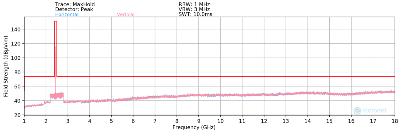
Plot 7-170. Radiated Spurious Plot above 1GHz (Bluetooth (LE) – Ch. 17) – Ant 1
