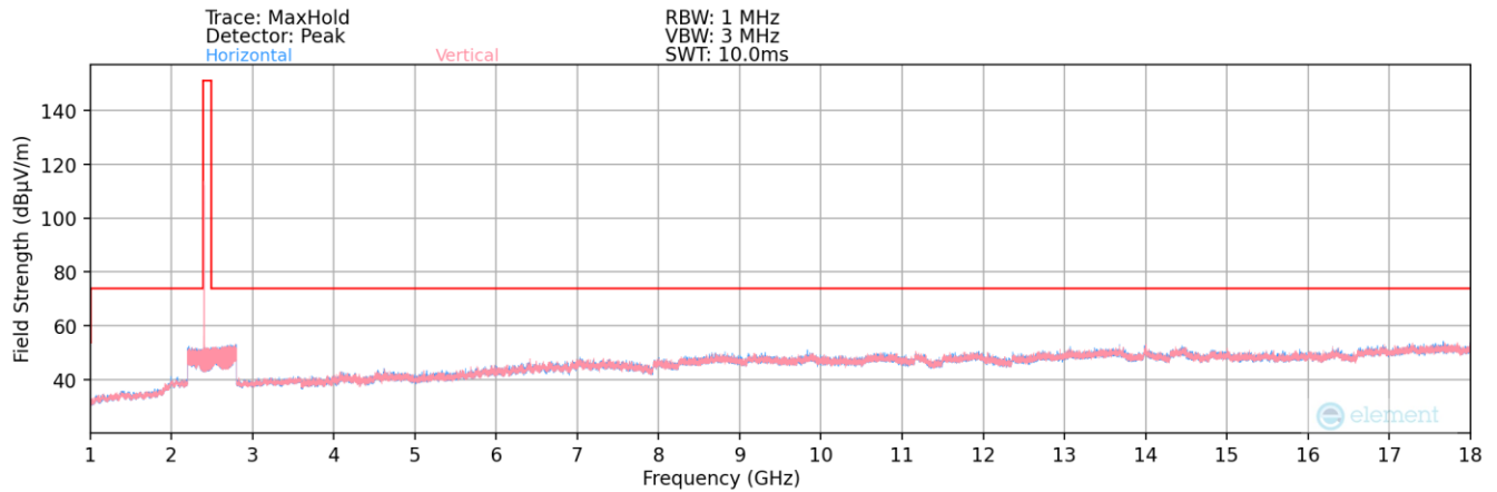
Plot 7-175. Radiated Spurious Plot above 1GHz (Bluetooth (LE) – Ch. 37) – DUAL
