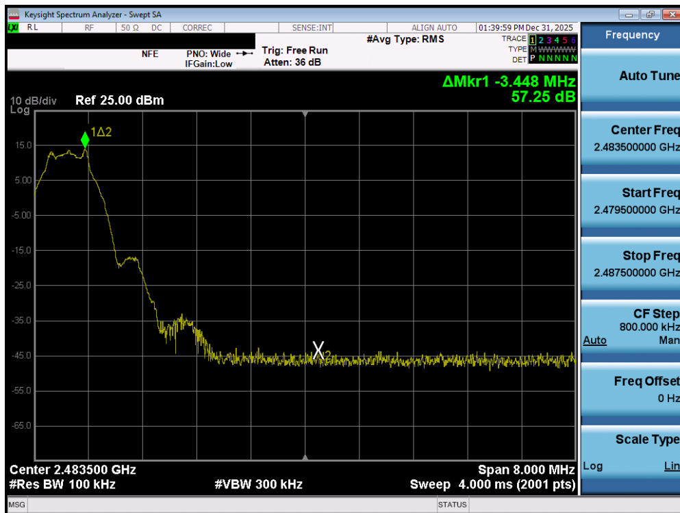
Plot 7-138. Band Edge Plot (Bluetooth (LE), 1Mbps – Ch. 39) – DUAL ANT1
