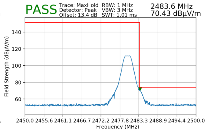
Plot 7-182. Radiated Restricted Upper Band Edge Measurement (Peak) – SISO ANT2 – 2M
