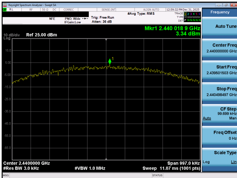
Plot 7-104. Power Spectral Density Plot (Bluetooth (LE), 1Mbps – Ch. 17) – SISO ANT2
