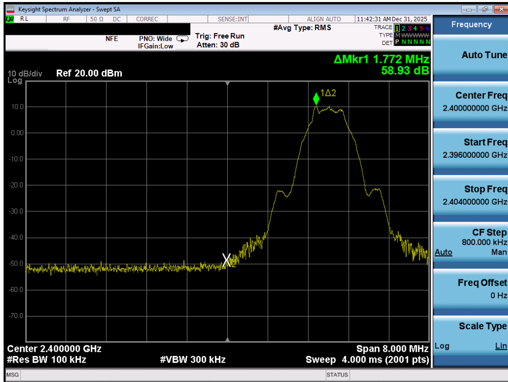
Plot 7-123. Band Edge Plot (Bluetooth (LE), 500kbps – Ch. 37) – SISO ANT1
