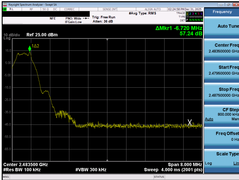
Plot 7-142. Band Edge Plot (Bluetooth (LE), 1Mbps - Ch. 39) - DUAL ANT2
