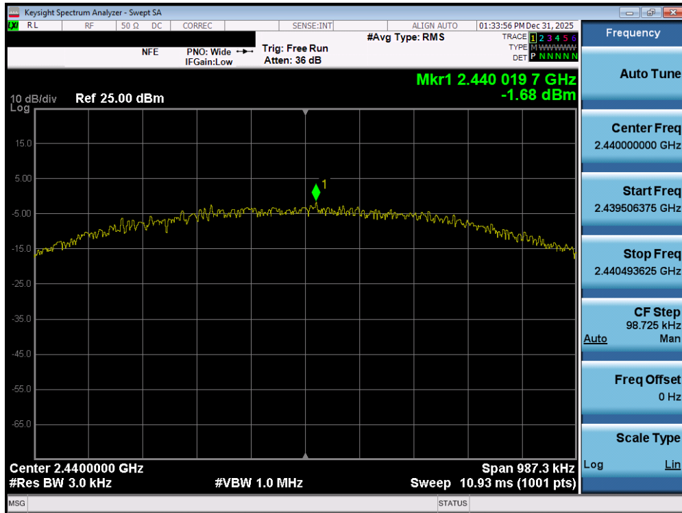
Plot 7-110. Power Spectral Density Plot (Bluetooth (LE), 1Mbps – Ch. 17) – DUAL ANT1
