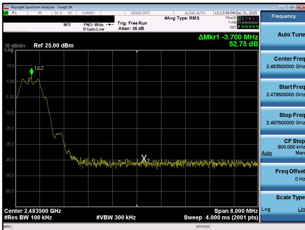
Plot 7-122. Band Edge Plot (Bluetooth (LE), 125kbps – Ch. 39) – SISO ANT1
