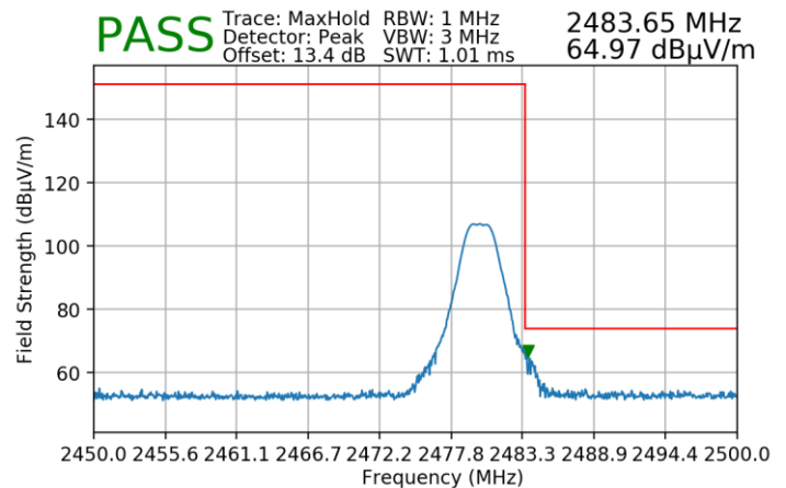
Plot 7-180. Radiated Restricted Upper Band Edge Measurement (Peak) – SISO ANT1 – 2M
