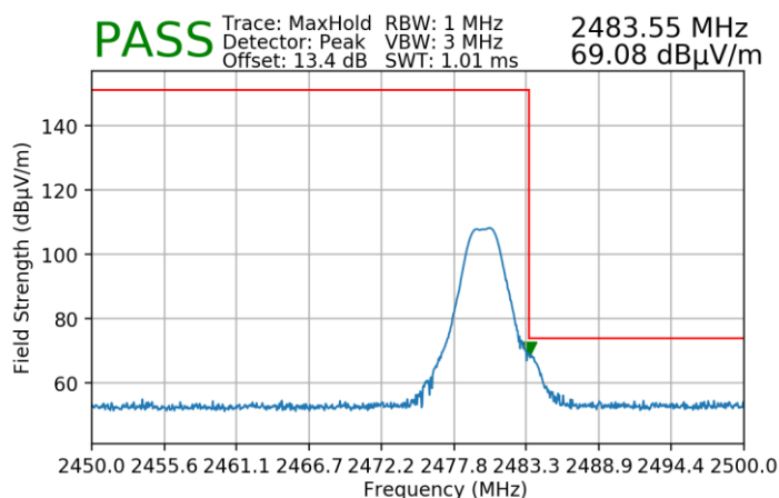
Plot 7-184. Radiated Restricted Upper Band Edge Measurement (Peak) – DUAL – 2M
