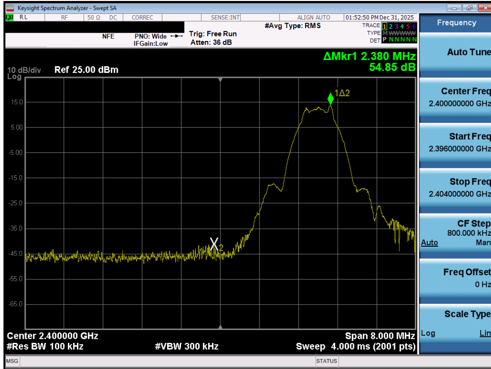
Plot 7-141. Band Edge Plot (Bluetooth (LE), 1Mbps - Ch. 37) - DUAL ANT2
