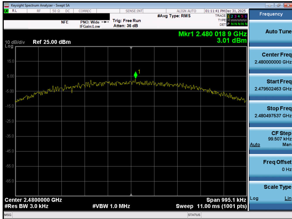
Plot 7-105. Power Spectral Density Plot (Bluetooth (LE), 1Mbps – Ch. 39) – SISO ANT2
