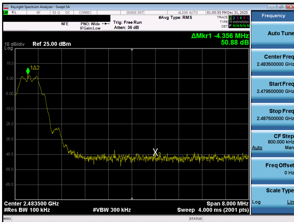
Plot 7-130. Band Edge Plot (Bluetooth (LE), 125kbps – Ch. 39) – SISO ANT2
