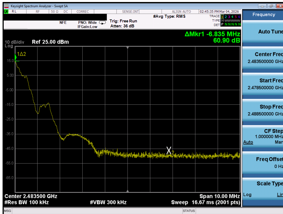
Plot 7-136. Band Edge Plot (Bluetooth (LE), 2Mbps – Ch. 36) – SISO ANT2
