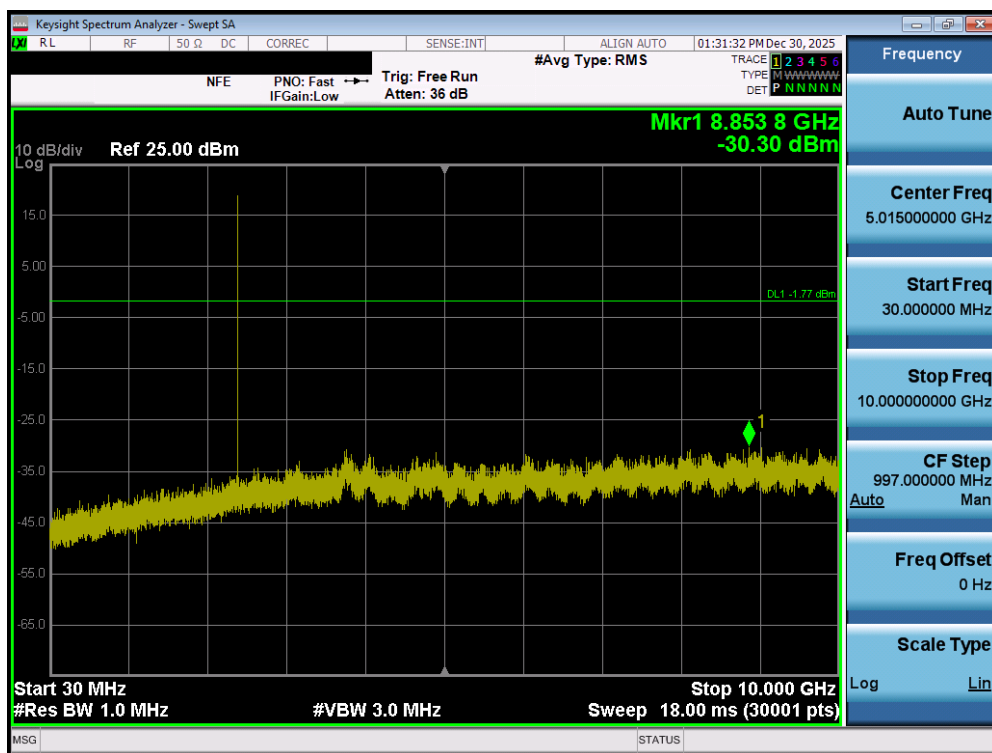
Plot 7-145. Conducted Spurious Plot (Bluetooth, 1Mbps – Ch. 0) - SISO ANT2
