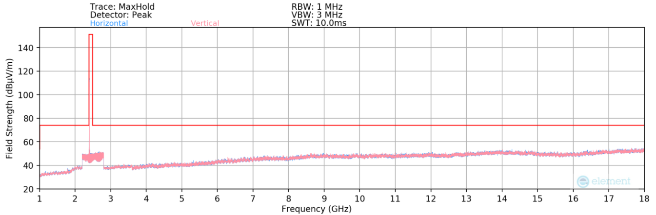
Plot 7-166. Radiated Spurious Plot above 1GHz (BT – Ch. 0)
