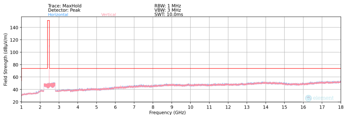
Plot 7-165. Radiated Spurious Plot above 1GHz (BT – Ch. 78)
