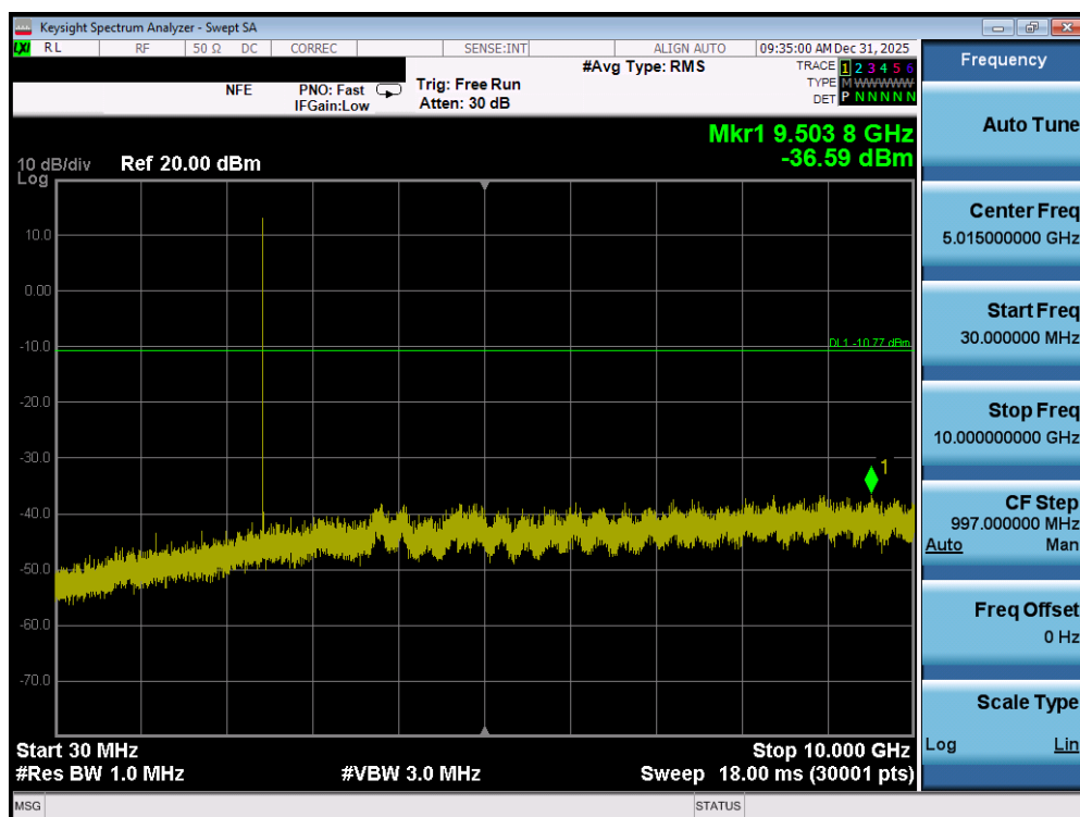
Plot 7-159. Conducted Spurious Plot (Bluetooth, 1Mbps – Ch. 39) – DUAL ANT2
