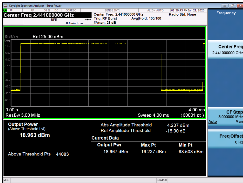
Plot 9-2. Conducted Output Power Measurements SISO ANT 2 (Spot-check)
