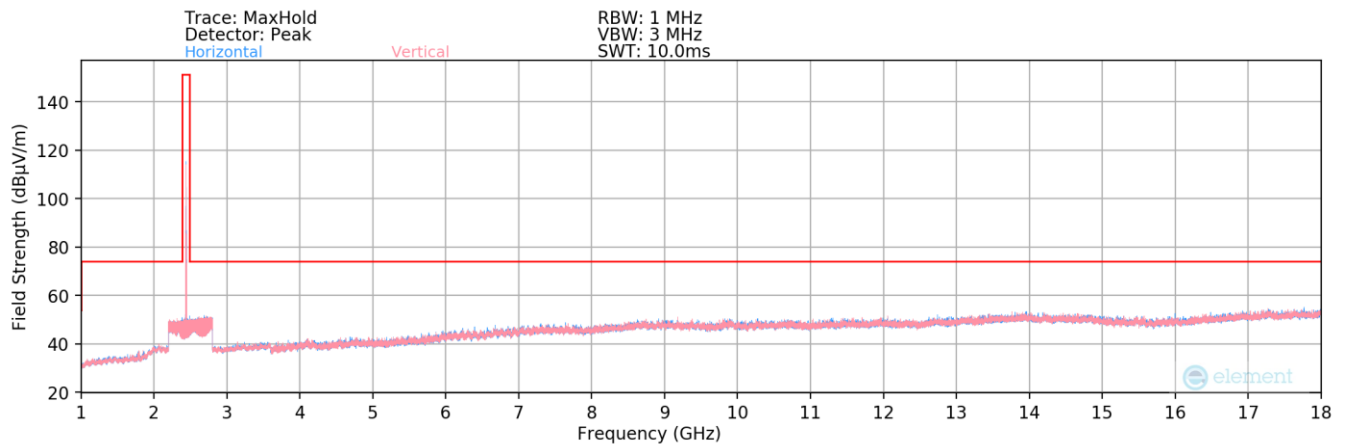
Plot 7-167. Radiated Spurious Plot above 1GHz (BT – Ch. 39)
