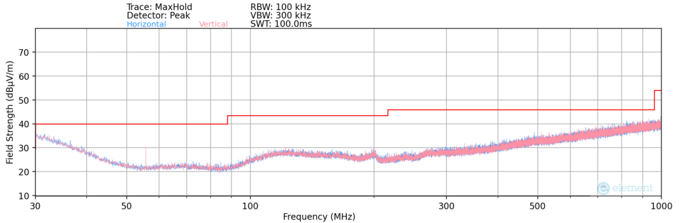
Plot 7-183. Radiated Spurious Plot below 1GHz – DUAL
