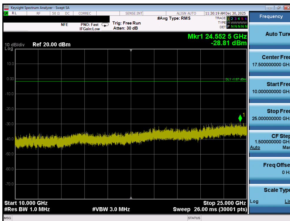
Plot 7-140. Conducted Spurious Plot (Bluetooth, 1Mbps – Ch. 0) - SISO ANT1
