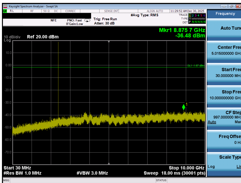
Plot 7-139. Conducted Spurious Plot (Bluetooth, 1Mbps – Ch. 0) - SISO ANT1
