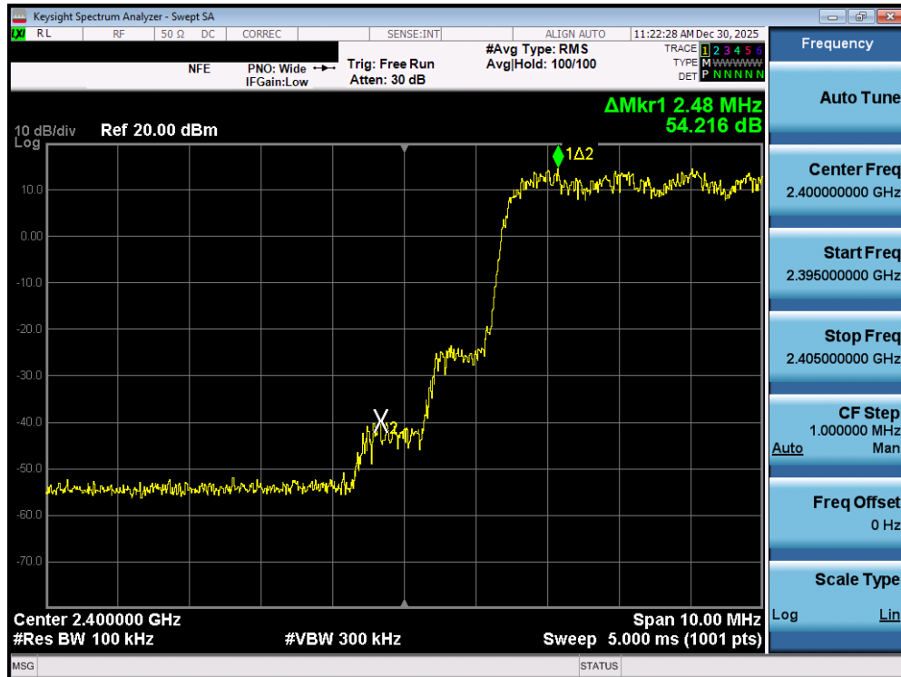
Plot 7-111. Band Edge Plot (Bluetooth with Hopping Enabled, 3 Mbps) – SISO ANT1
