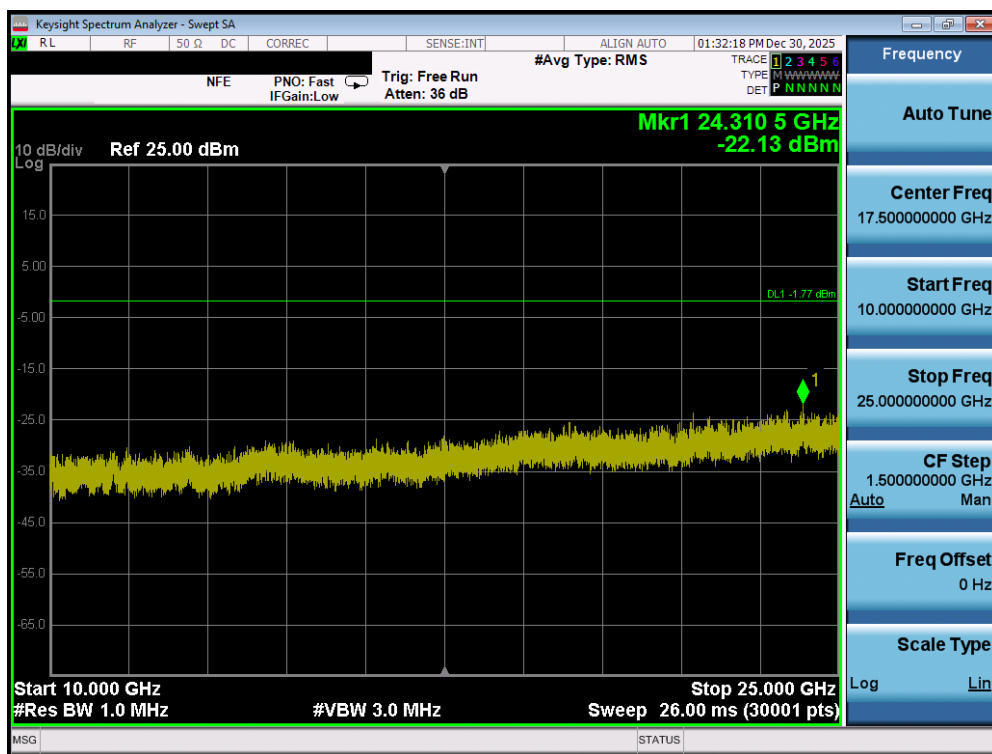
Plot 7-146. Conducted Spurious Plot (Bluetooth, 1Mbps – Ch. 0) - SISO ANT2
