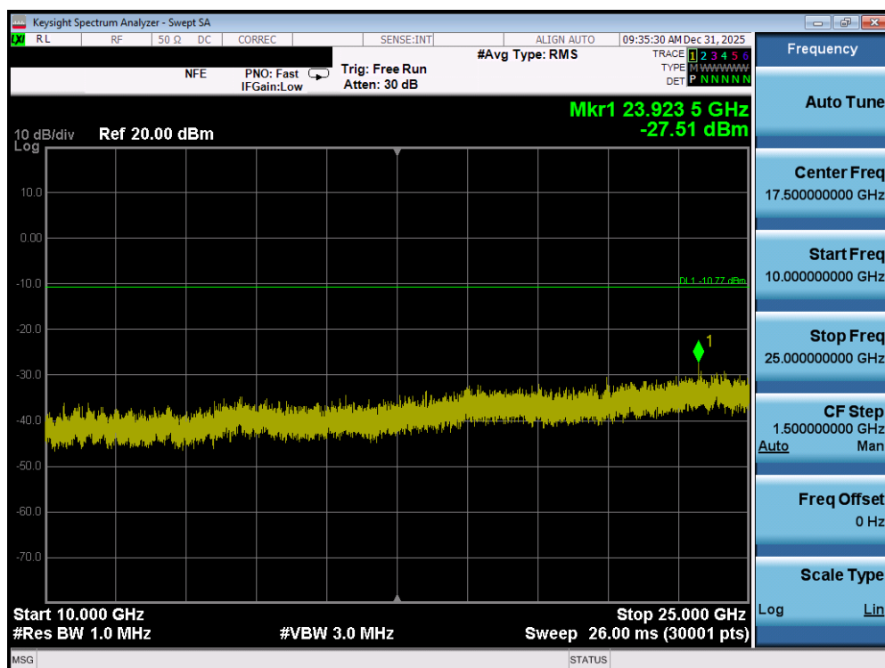
Plot 7-160. Conducted Spurious Plot (Bluetooth, 1Mbps – Ch. 39) – DUAL ANT2
