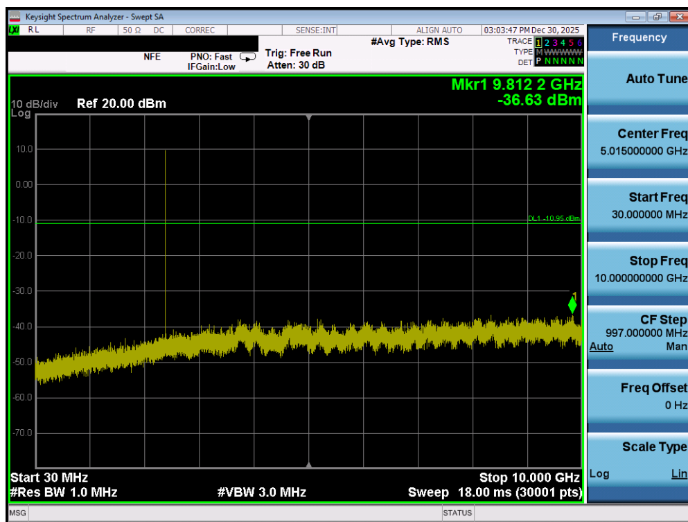
Plot 7-151. Conducted Spurious Plot (Bluetooth, 1Mbps – Ch. 0) – DUAL ANT1
