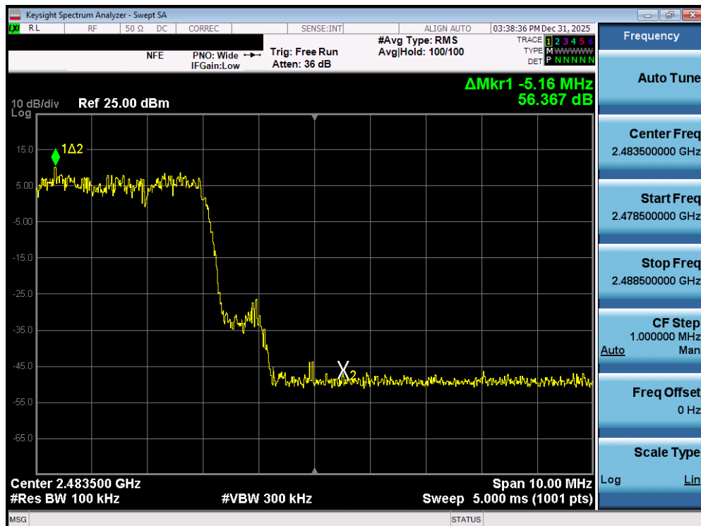
Plot 7-120. Band Edge Plot (Bluetooth with Hopping Enabled, 3 Mbps) – DUAL ANT1
