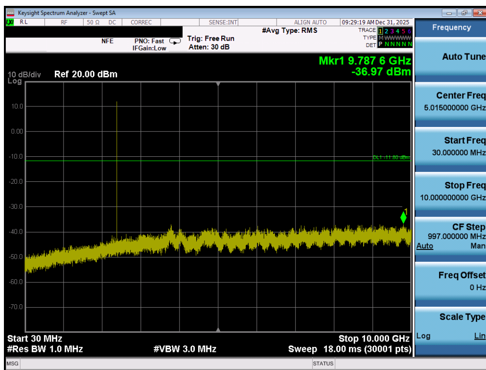
Plot 7-157. Conducted Spurious Plot (Bluetooth, 1Mbps – Ch. 0) – DUAL ANT2
