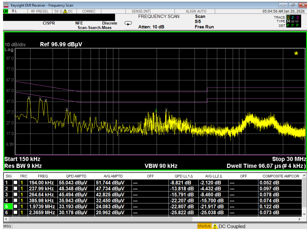
Plot 7-185. Line-Conducted Test Plot (N)
