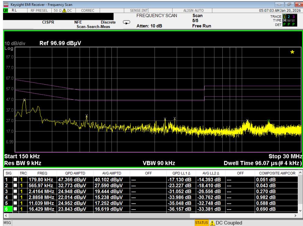
Plot 7-184. Line-Conducted Test Plot (L1)
