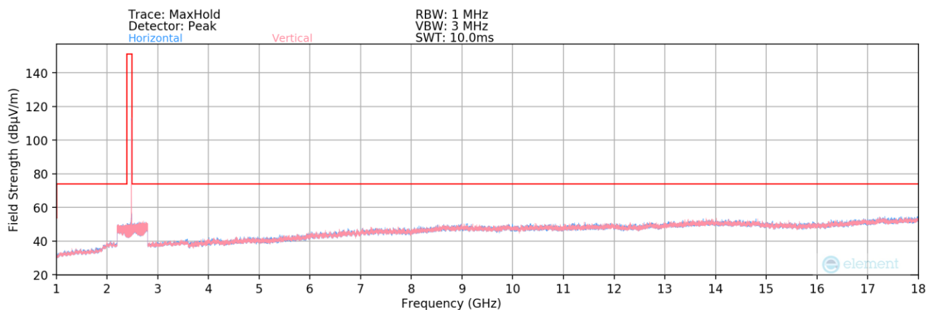
Plot 7-168. Radiated Spurious Plot above 1GHz (BT – Ch. 78)
