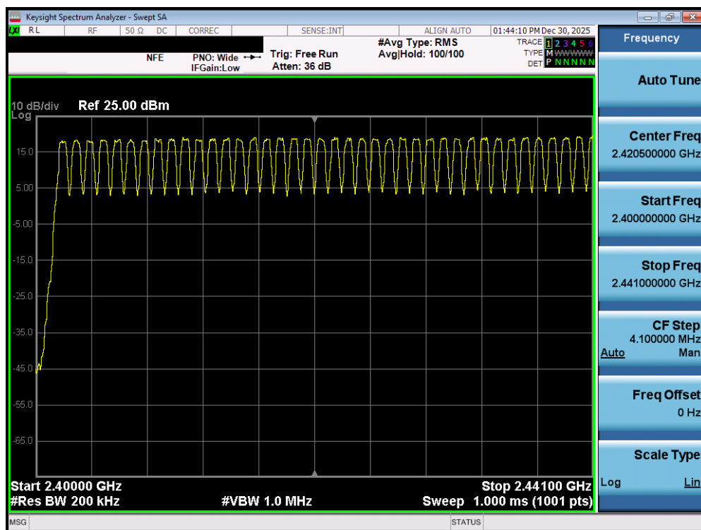
Plot 7-133. Low End Spectrum Channel Hopping Plot (Bluetooth) – SISO ANT2
