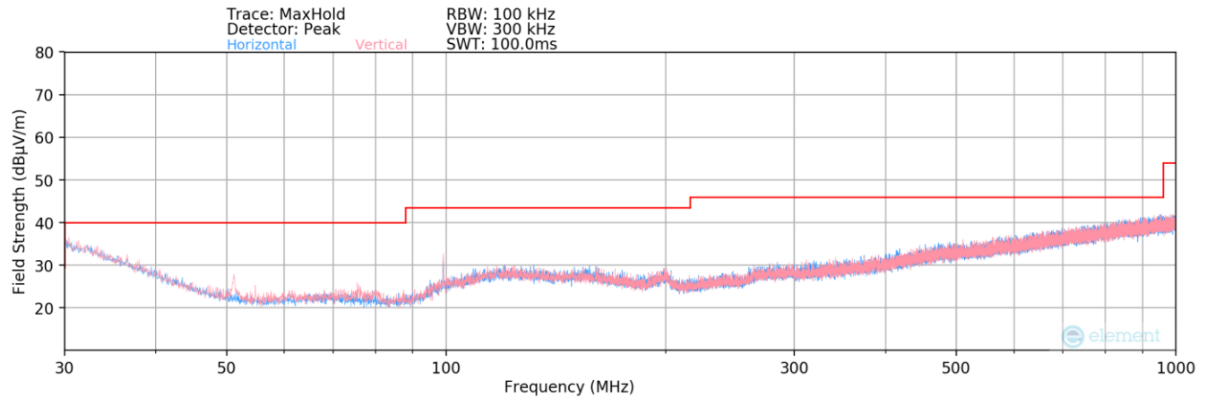
Plot 7-182. Radiated Spurious Plot below 1GHz – SISO ANT2
