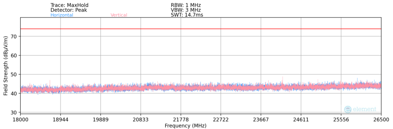
Plot 7-173. Radiated Spurious Plot above 18GHz
