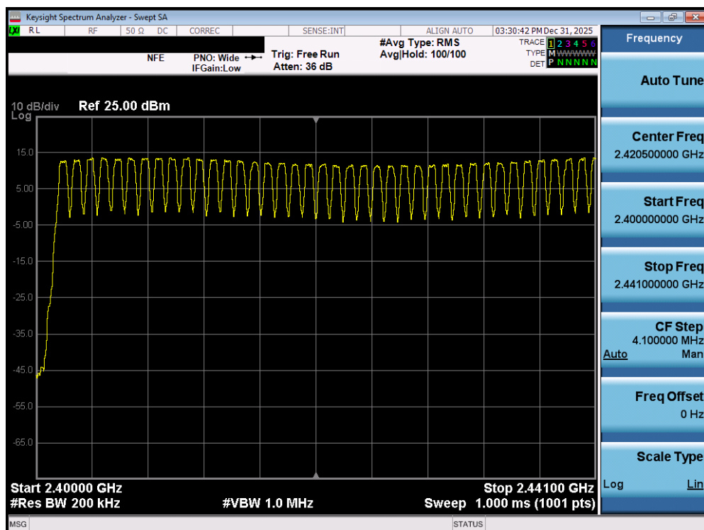
Plot 7-135. Low End Spectrum Channel Hopping Plot (Bluetooth) – DUAL ANT1
