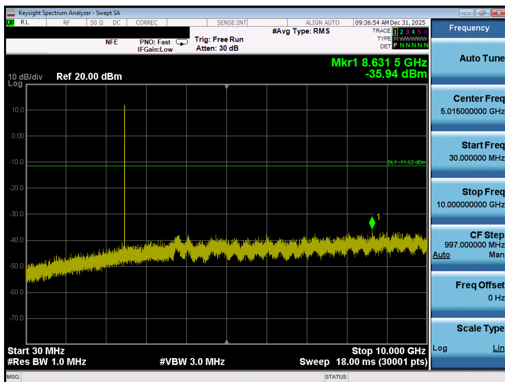
Plot 7-161. Conducted Spurious Plot (Bluetooth, 1Mbps – Ch. 78) – DUAL ANT2
