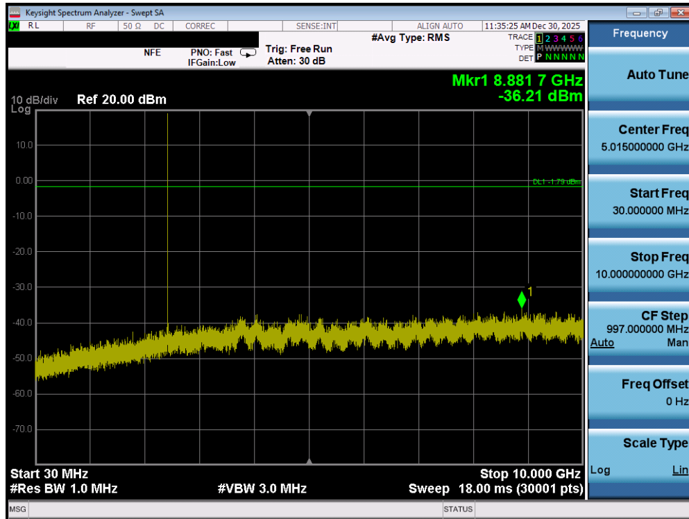
Plot 7-141. Conducted Spurious Plot (Bluetooth, 1Mbps – Ch. 39) - SISO ANT1
