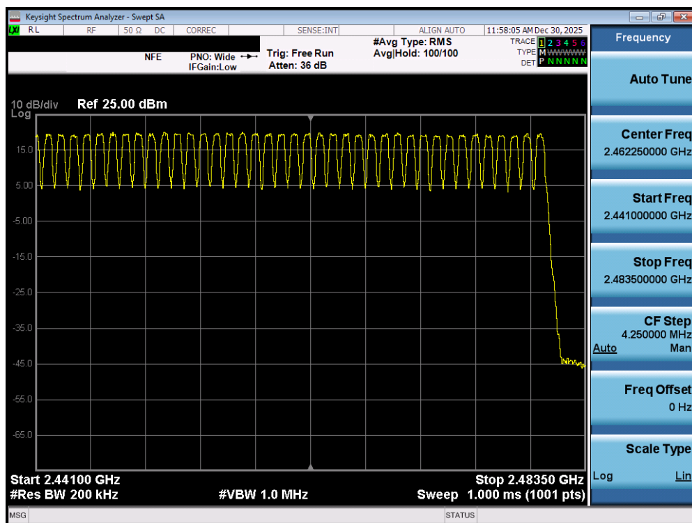
Plot 7-132. High End Spectrum Channel Hopping Plot (Bluetooth) – SISO ANT1
