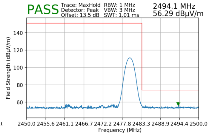
Plot 7-178. Radiated Restricted Upper Band Edge Measurement (Peak) – SISO ANT2
