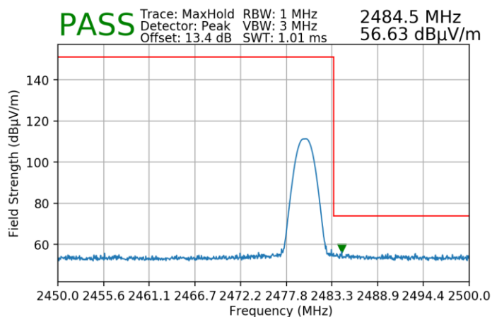
Plot 7-180. Radiated Restricted Upper Band Edge Measurement (Peak) – DUAL
