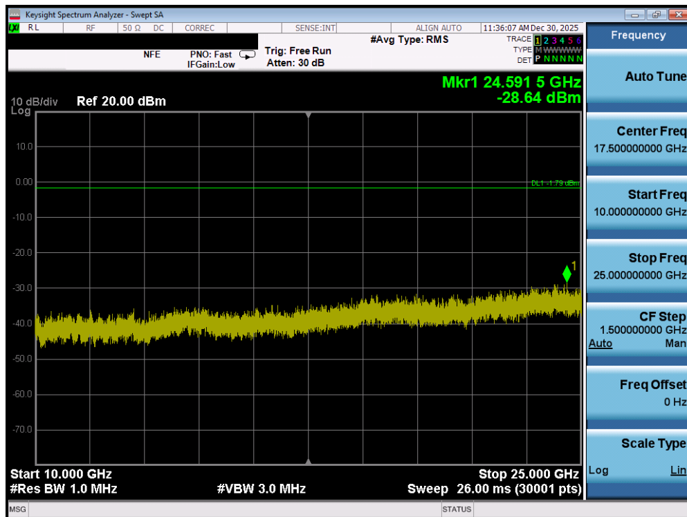
Plot 7-142. Conducted Spurious Plot (Bluetooth, 1Mbps – Ch. 39) - SISO ANT1
