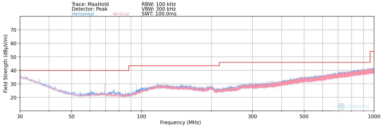
Plot 7-181. Radiated Spurious Plot below 1GHz – SISO ANT1
