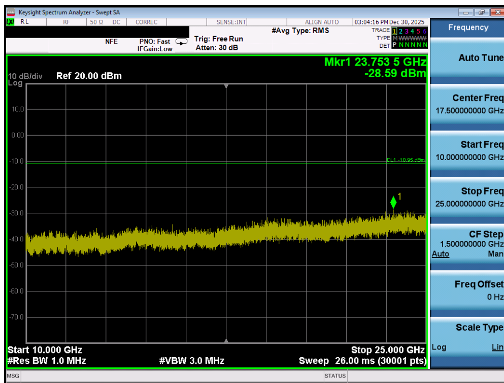
Plot 7-152. Conducted Spurious Plot (Bluetooth, 1Mbps – Ch. 0) – DUAL ANT1
