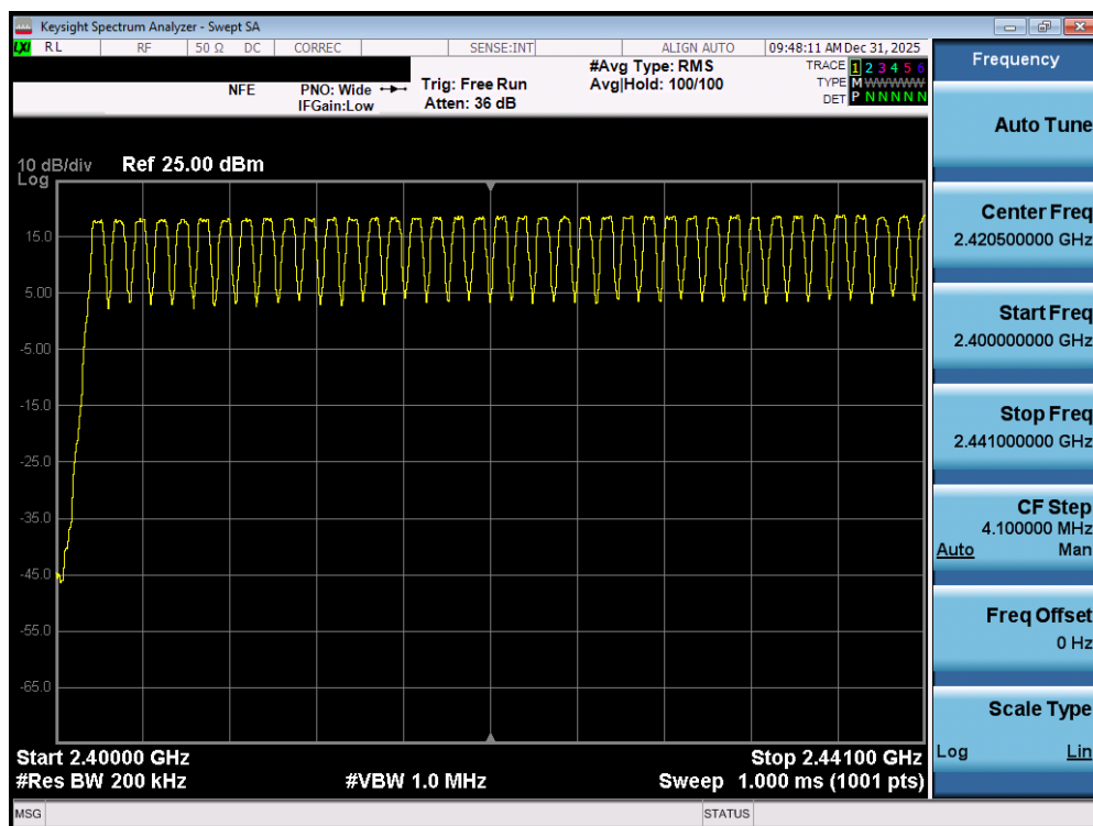
Plot 7-137. Low End Spectrum Channel Hopping Plot (Bluetooth) – DUAL ANT2
