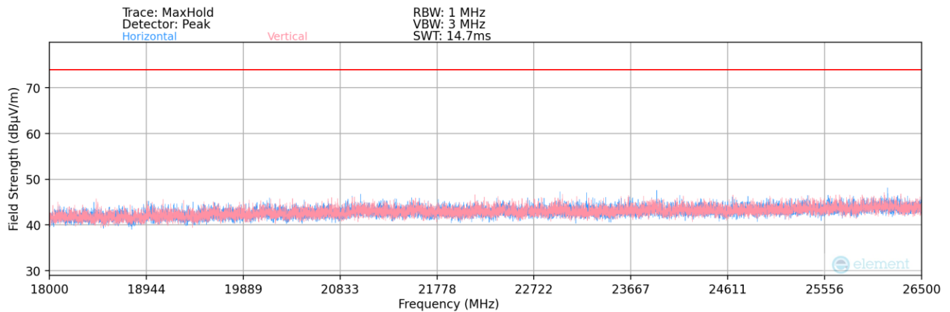
Plot 7-174. Radiated Spurious Plot above 18GHz
