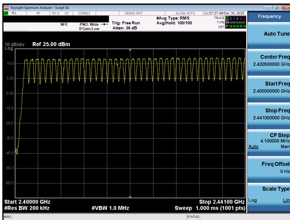
Plot 7-131. Low End Spectrum Channel Hopping Plot (Bluetooth) – SISO ANT1
