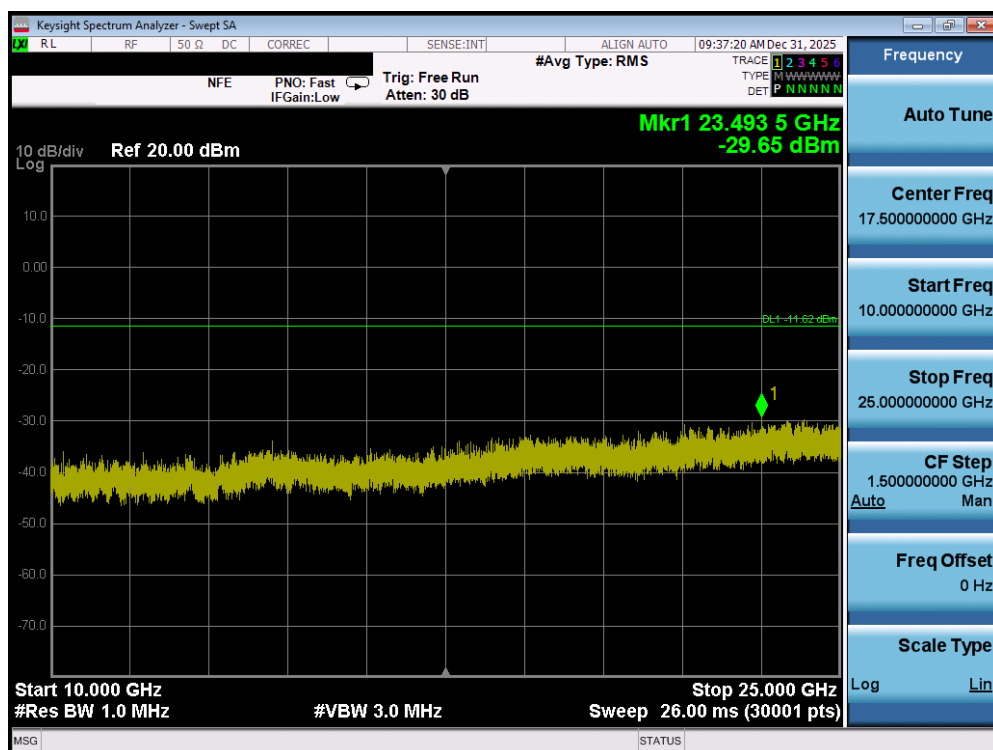
Plot 7-162. Conducted Spurious Plot (Bluetooth, 1Mbps – Ch. 78) – DUAL ANT2
