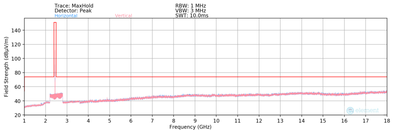
Plot 7-164. Radiated Spurious Plot above 1GHz (BT – Ch. 39)
