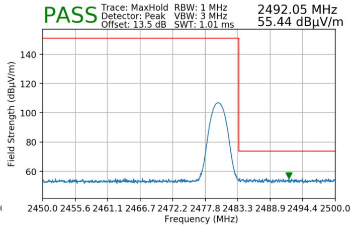
Plot 7-176. Radiated Restricted Upper Band Edge Measurement (Peak) – SISO ANT1
