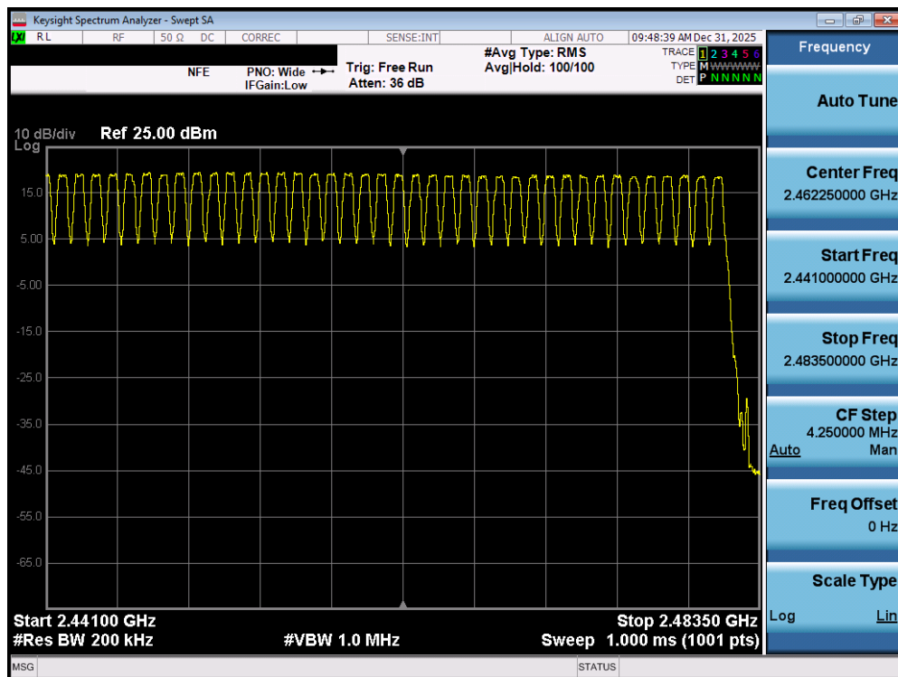
Plot 7-138. High End Spectrum Channel Hopping Plot (Bluetooth) – DUAL ANT2
