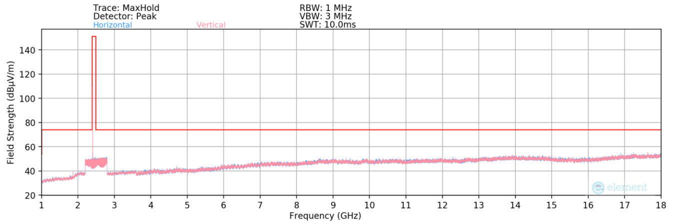
Plot 7-163. Radiated Spurious Plot above 1GHz (BT – Ch. 0)
