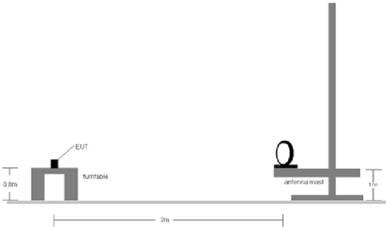
Figure 7-11. Radiated Test Setup <30M
