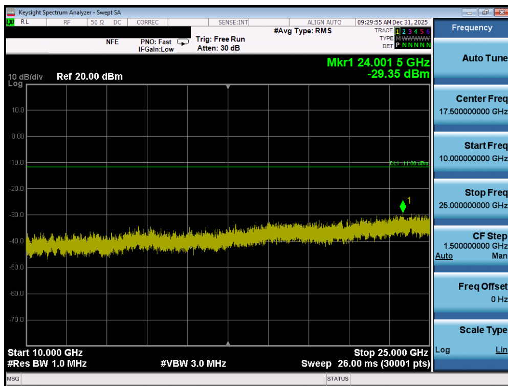
Plot 7-158. Conducted Spurious Plot (Bluetooth, 1Mbps – Ch. 0) – DUAL ANT2
