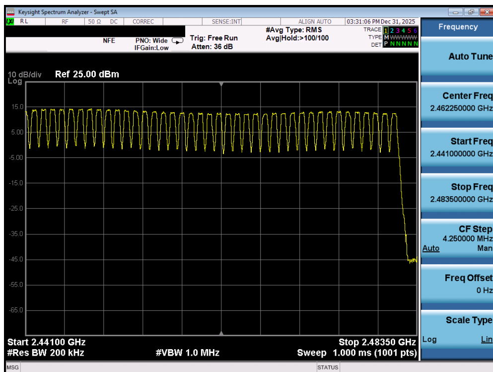
Plot 7-136. High End Spectrum Channel Hopping Plot (Bluetooth) – DUAL ANT1
