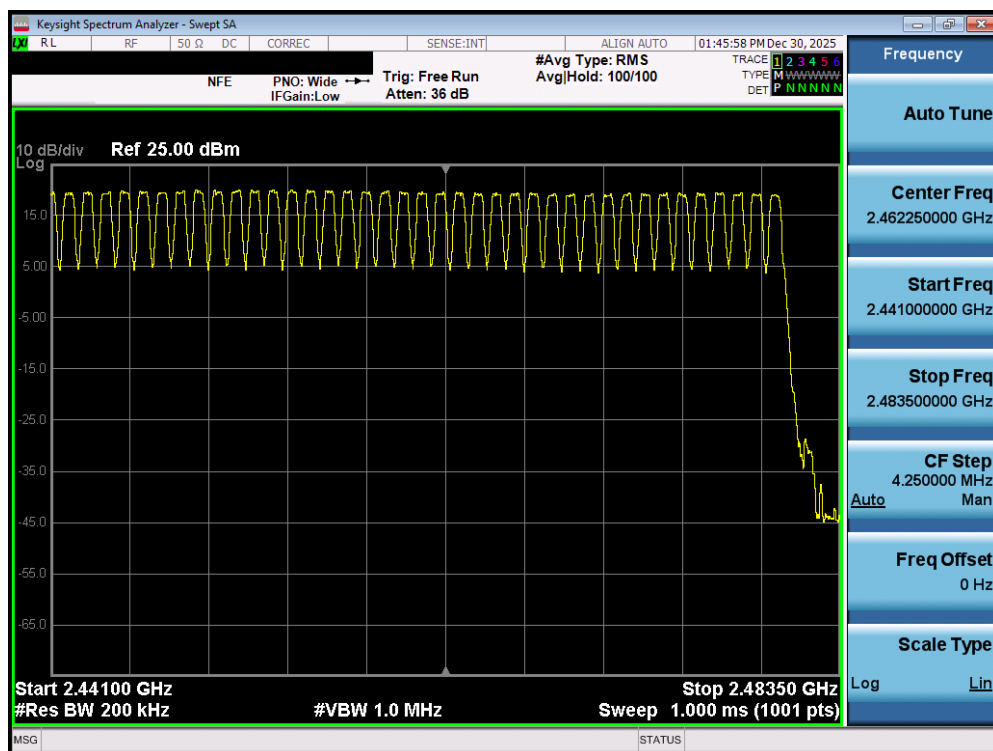
Plot 7-134. High End Spectrum Channel Hopping Plot (Bluetooth) – SISO ANT2
