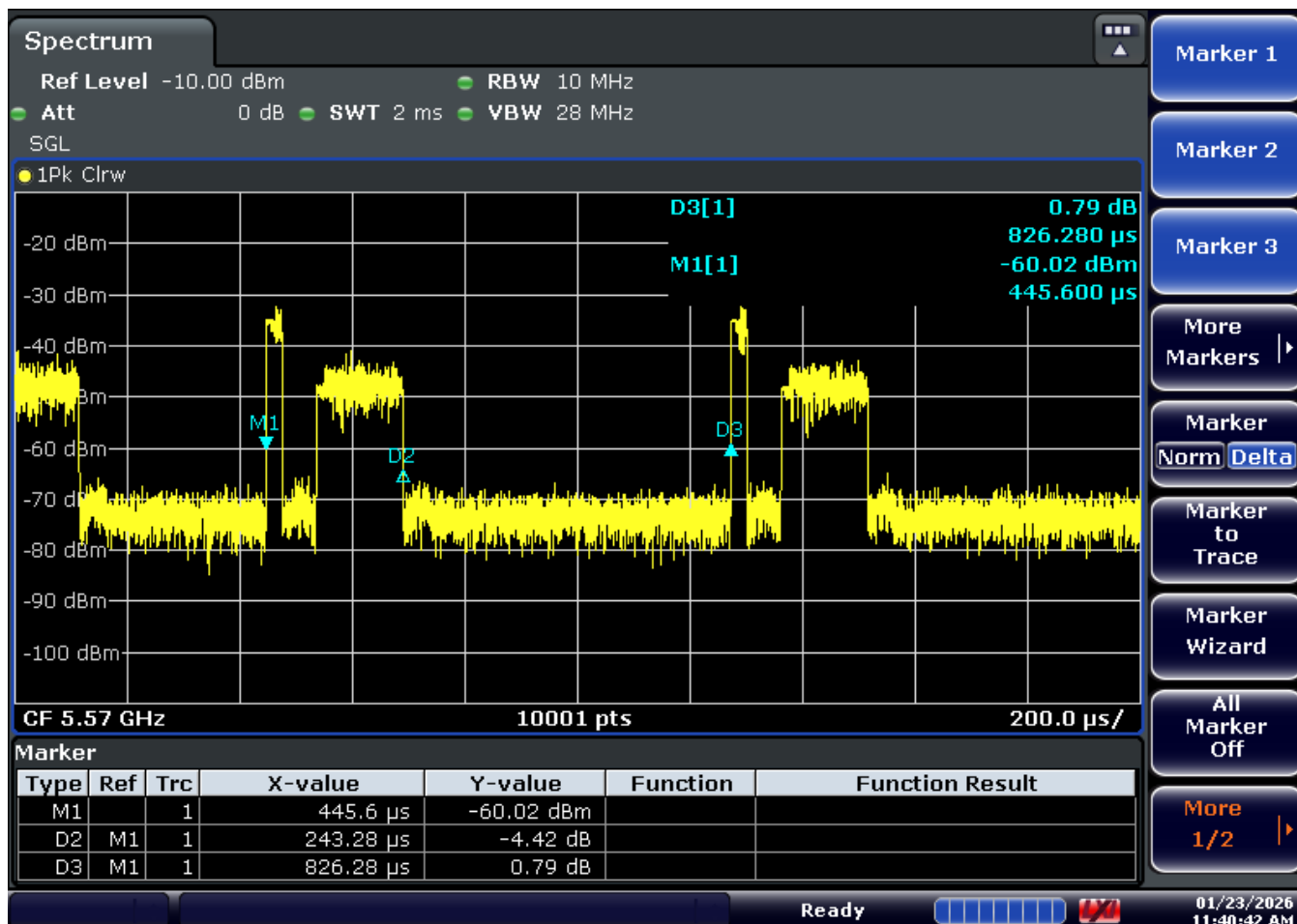
Figure 9-1. Band 2C Pulse Width + Period
