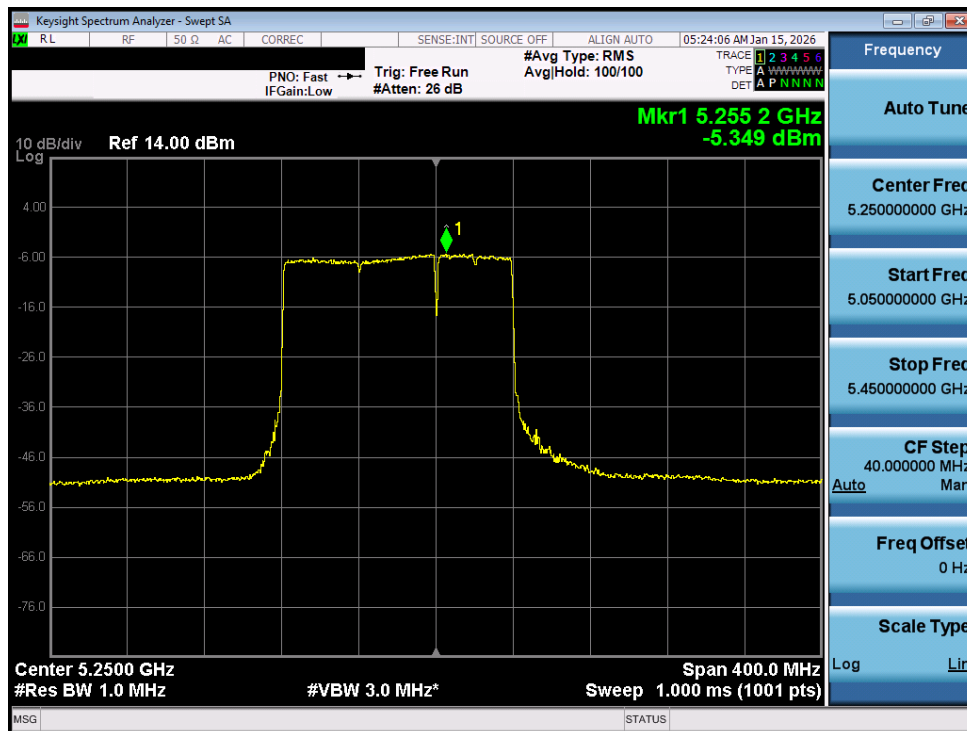
Plot 7-197. Power Spectral Density Plot MIMO ANT1 (160MHz BW 802.11be (UNII Band 1/2A) – Ch. 50)
