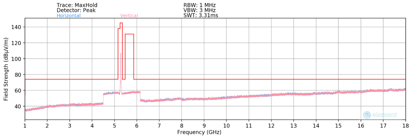
Plot 7-212. Radiated Spurious Plot above 1GHz MIMO (802.11a – UNII Band 2A Ch. 56)
