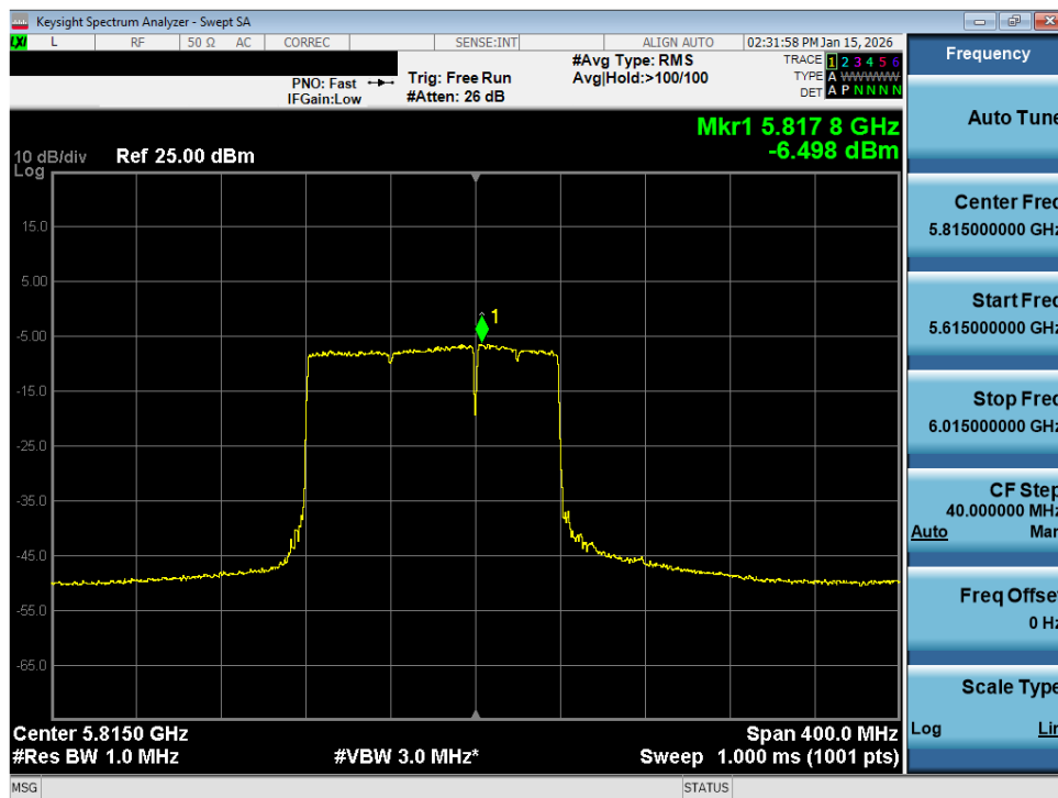
Plot 7-209. Power Spectral Density Plot MIMO ANT2 (160MHz BW 802.11be (UNII Band 3/4) – Ch. 163)
