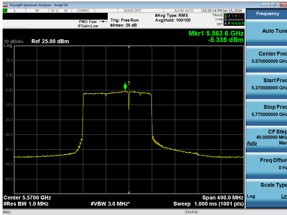
Plot 7-206. Power Spectral Density Plot MIMO ANT2 (160MHz BW 802.11be (UNII Band 2C) – Ch. 114)
