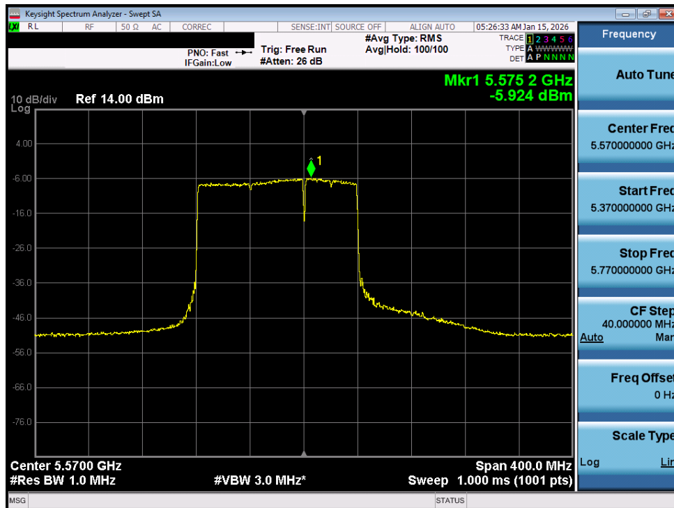
Plot 7-199. Power Spectral Density Plot MIMO ANT1 (160MHz BW 802.11be (UNII Band 2C) – Ch. 114)
