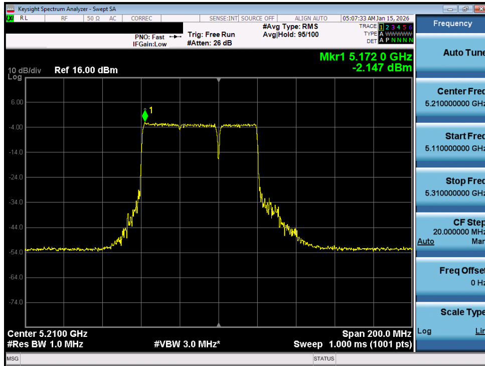
Plot 7-196. Power Spectral Density Plot MIMO ANT1 (80MHz BW 802.11be (UNII Band 1) – Ch. 42)
