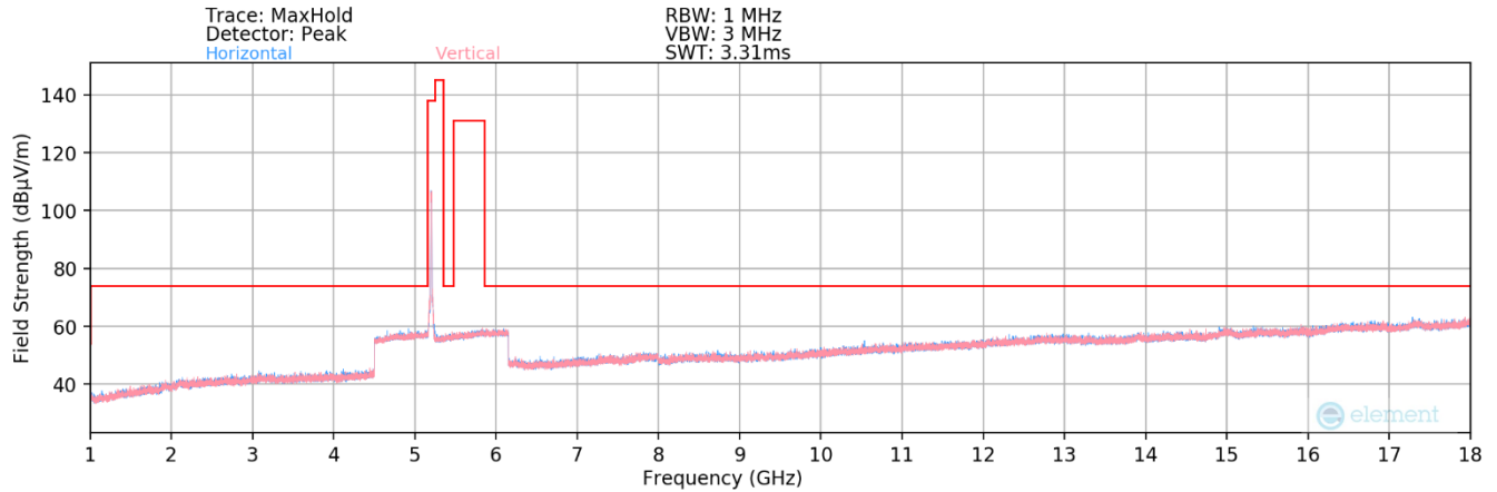
Plot 7-211. Radiated Spurious Plot above 1GHz MIMO (802.11a – UNII Band 1 Ch. 40)
