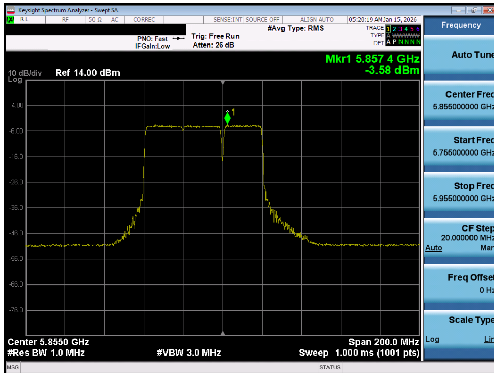
Plot 7-201. Power Spectral Density Plot MIMO ANT1 (80MHz BW 802.11be (UNII Band 3/4) – Ch. 171)
