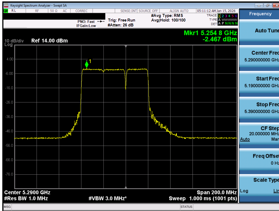
Plot 7-198. Power Spectral Density Plot MIMO ANT1 (80MHz BW 802.11be (UNII Band 2A) – Ch. 58)
