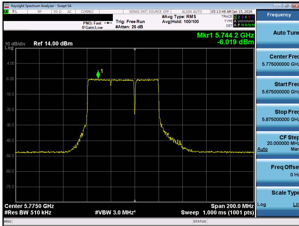
Plot 7-200. Power Spectral Density Plot MIMO ANT1 (80MHz BW 802.11be (UNII Band 3) – Ch. 155)
