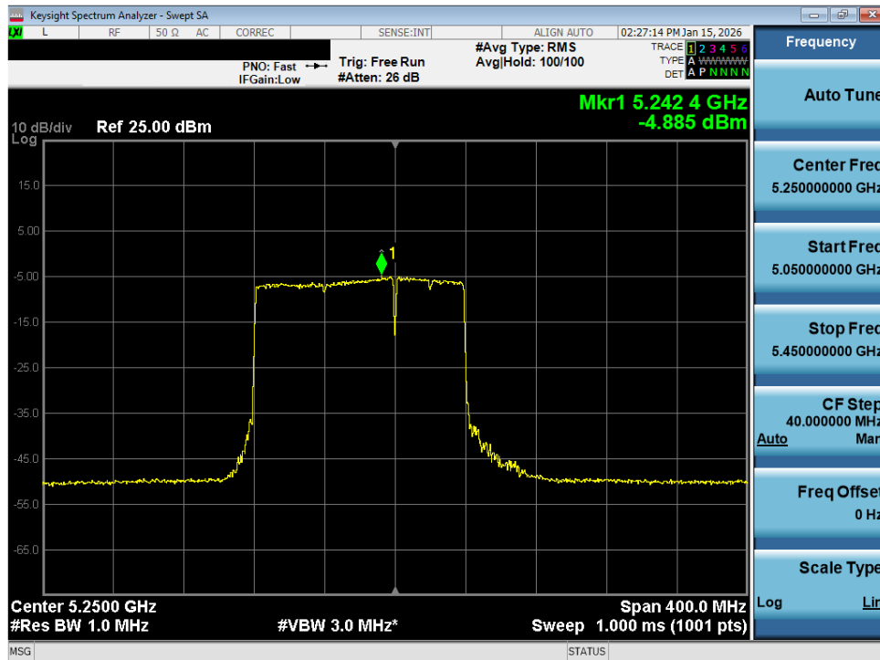
Plot 7-204. Power Spectral Density Plot MIMO ANT2 (160MHz BW 802.11be (UNII Band 1/2A) – Ch. 50)
