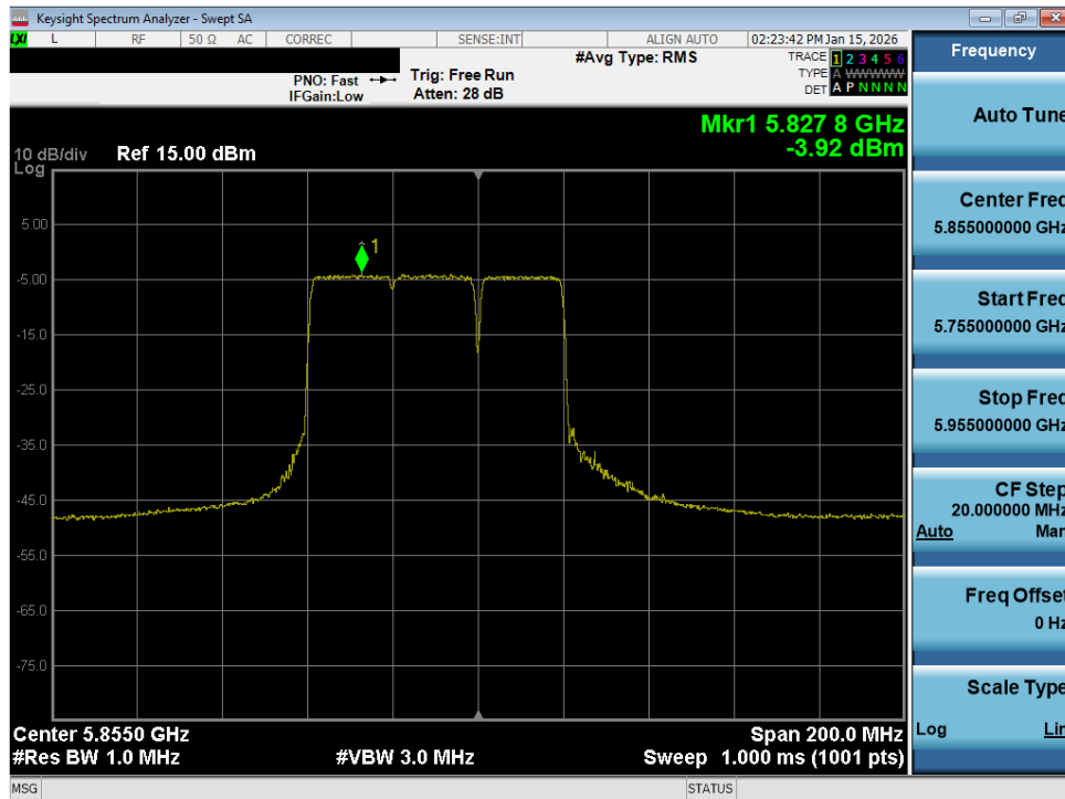
Plot 7-208. Power Spectral Density Plot MIMO ANT2 (80MHz BW 802.11be (UNII Band 3/4) – Ch. 171)
