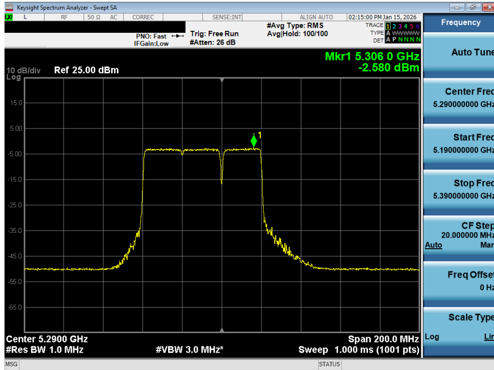
Plot 7-205. Power Spectral Density Plot MIMO ANT2 (80MHz BW 802.11be (UNII Band 2A) – Ch. 58)
