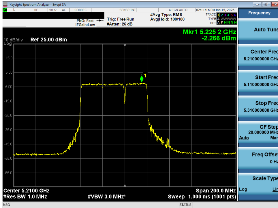
Plot 7-203. Power Spectral Density Plot MIMO ANT2 (80MHz BW 802.11be (UNII Band 1) – Ch. 42)
