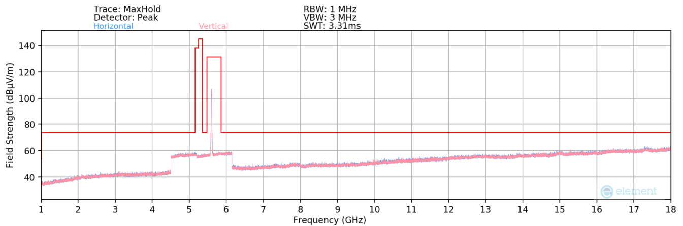
Plot 7-213. Radiated Spurious Plot above 1GHz MIMO (802.11a – UNII Band 2C Ch. 120)
