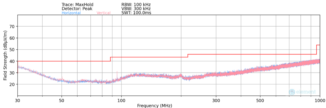
Plot 7-210. Radiated Spurious Plot below 1GHz MIMO (802.11a)
