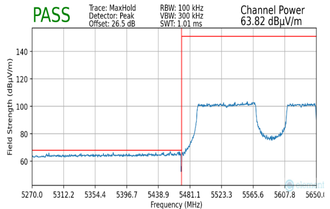
Plot 7-267. Radiated Lower Band Edge Plot MIMO (Peak – UNII Band 2C)
