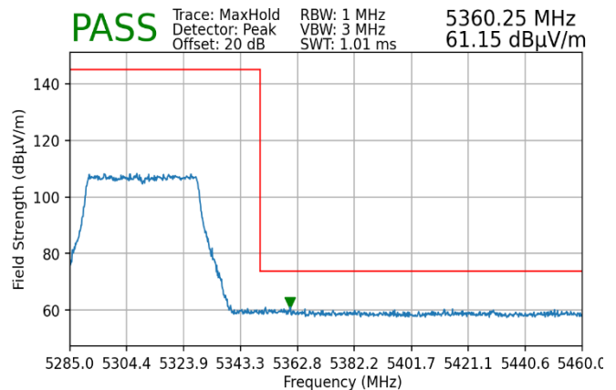
Plot 7-231. Radiated Upper Band Edge Plot MIMO (Peak – UNII Band 2A)
