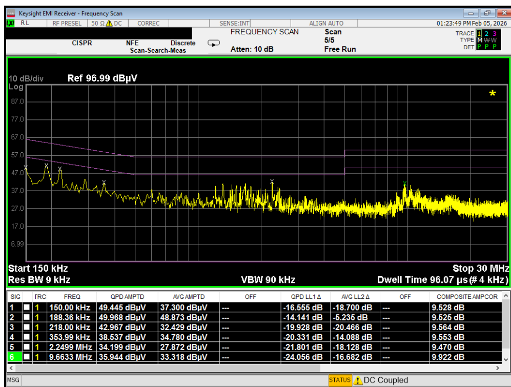
Plot 7-274. Line Conducted Plot with 802.11a UNII Band 2A (N)
