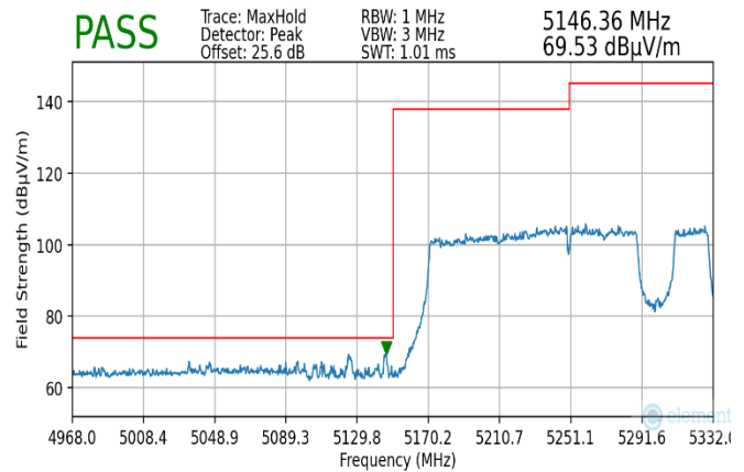
Plot 7-265. Radiated Lower Band Edge Plot MIMO (Peak – UNII Band 1)
