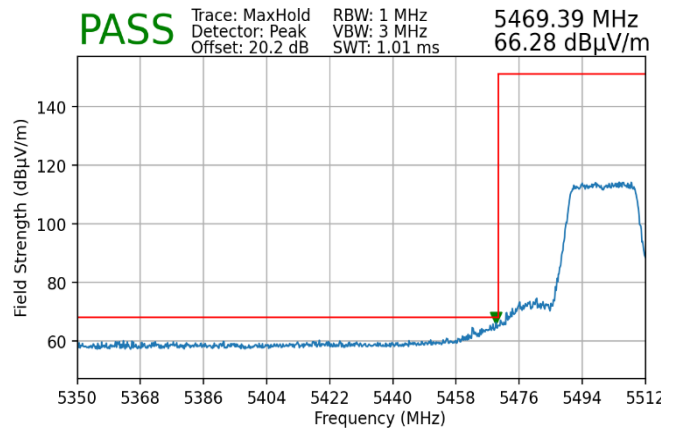
Plot 7-223. Radiated Lower Band Edge Plot MIMO (Peak – UNII Band 2C)
