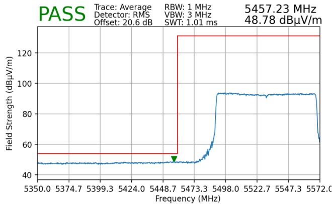
Plot 7-242. Radiated Lower Band Edge Plot MIMO (Average – UNII Band 2C)
