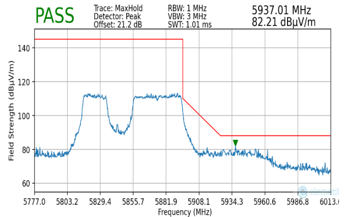
Plot 7-256. Radiated Upper Band Edge Plot MIMO (Peak – UNII Band 4)
