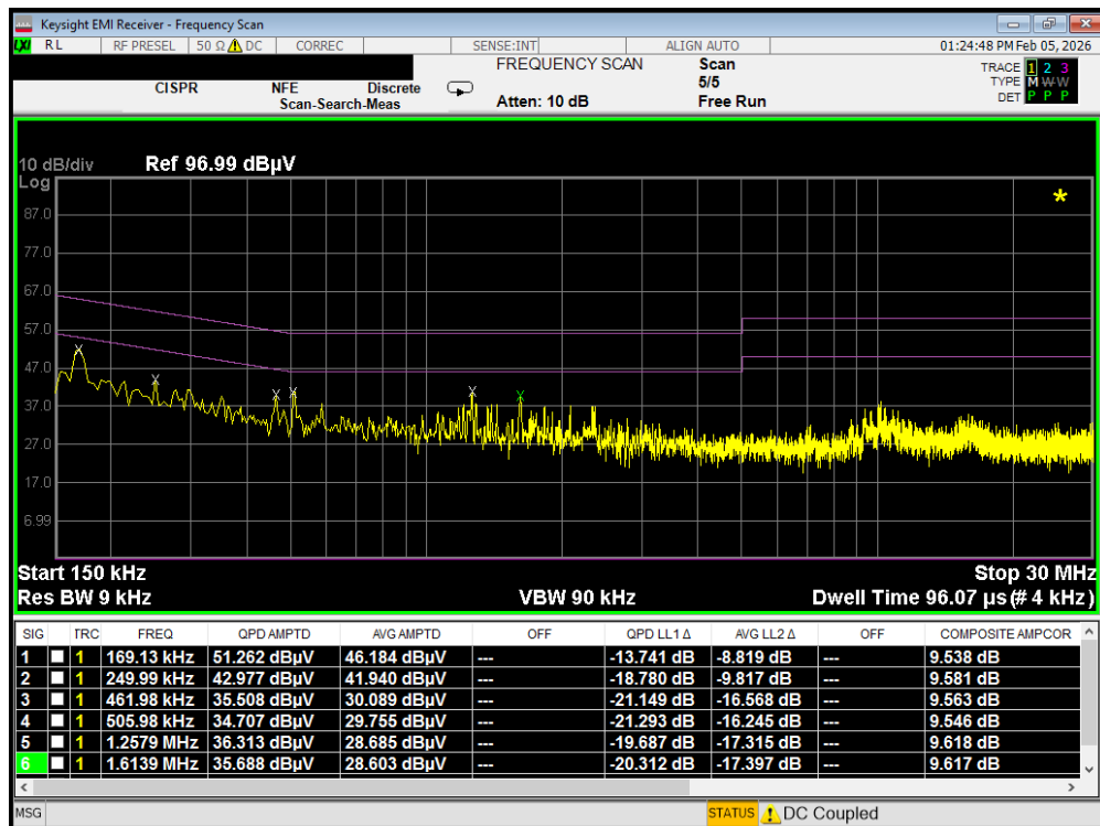
Plot 7-276. Line Conducted Plot with 802.11a UNII Band 2C (N)
