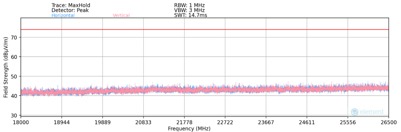
Plot 7-216. Radiated Spurious Plot 18GHz – 26.5GHz MIMO (802.11a)
