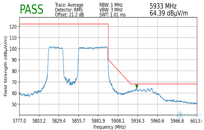
Plot 7-255. Radiated Upper Band Edge Plot MIMO (Average – UNII Band 4)
