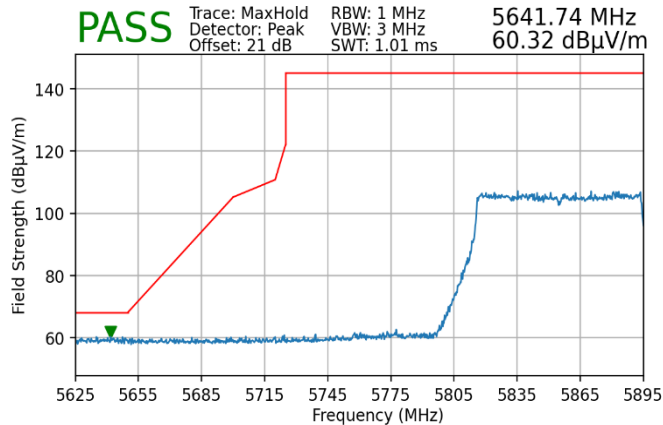
Plot 7-245. Radiated Lower Band Edge Plot MIMO (Peak – UNII Band 4)
