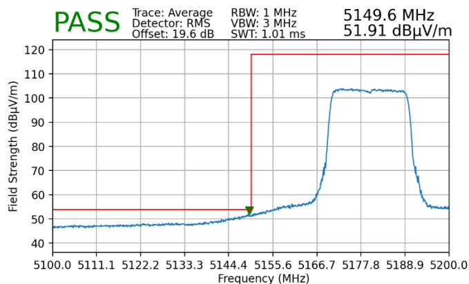
Plot 9-1. Radiated Lower Band Edge Plot MIMO (Average – UNII Band 1)
