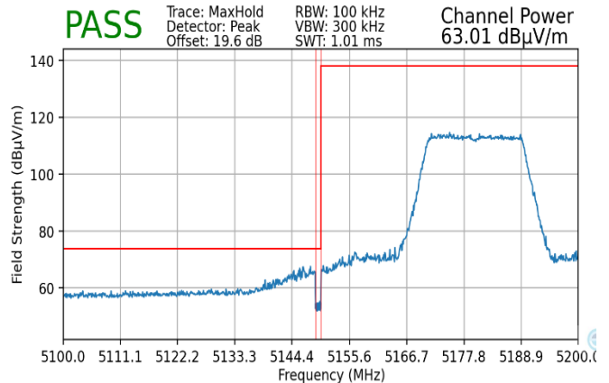
Plot 7-219. Radiated Lower Band Edge Plot MIMO (Peak – UNII Band 1)
