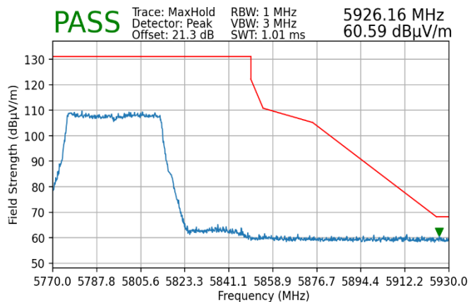
Plot 7-234. Radiated Upper Band Edge Plot MIMO (Peak – UNII Band 3)
