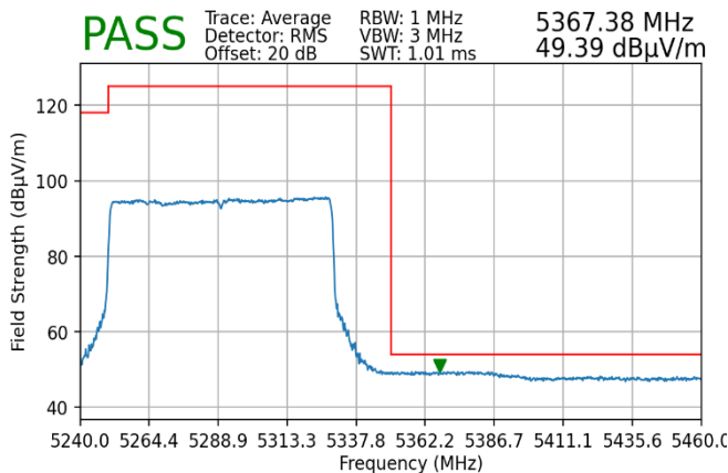
Plot 7-240. Radiated Upper Band Edge Plot MIMO (Average – UNII Band 2A)
