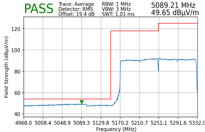
Plot 7-257. Radiated Lower Band Edge Plot MIMO (Average – UNII Band 1)
