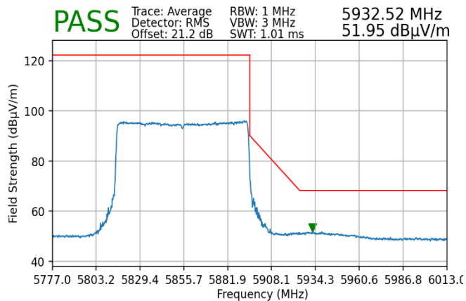
Plot 7-246. Radiated Upper Band Edge Plot MIMO (Average – UNII Band 4)
