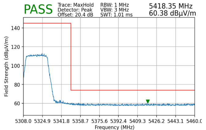
Plot 7-221. Radiated Upper Band Edge Plot MIMO (Peak – UNII Band 2A)
