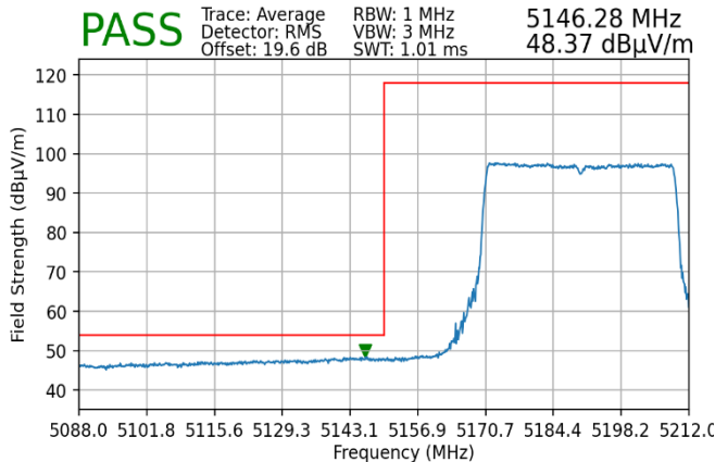
Plot 7-228. Radiated Lower Band Edge Plot MIMO (Average – UNII Band 1)
