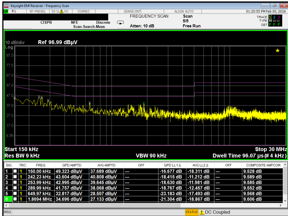
Plot 7-275. Line Conducted Plot with 802.11a UNII Band 2C (L1)
