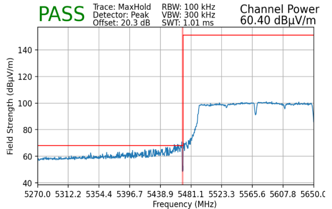
Plot 7-260. Radiated Lower Band Edge Plot MIMO (Peak – UNII Band 2C)
