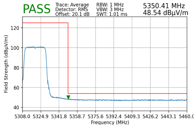
Plot 7-220. Radiated Upper Band Edge Plot MIMO (Average – UNII Band 2A)
