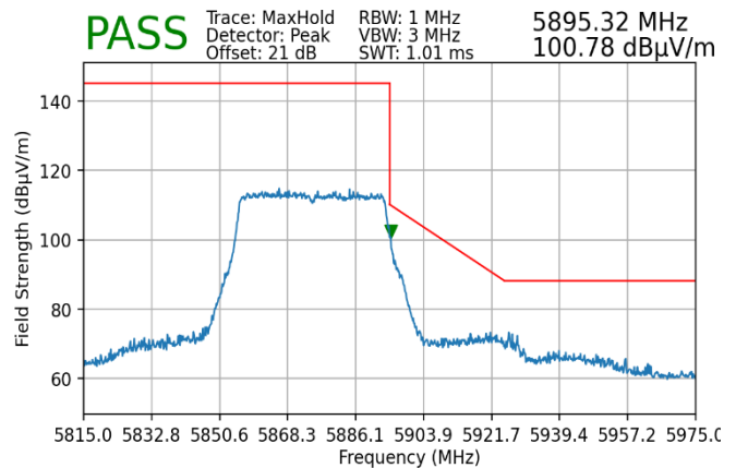
Plot 7-237. Radiated Upper Band Edge Plot MIMO (Peak – UNII Band 4)
