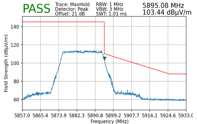
Plot 7-227. Radiated Upper Band Edge Plot MIMO (Peak – UNII Band 4)
