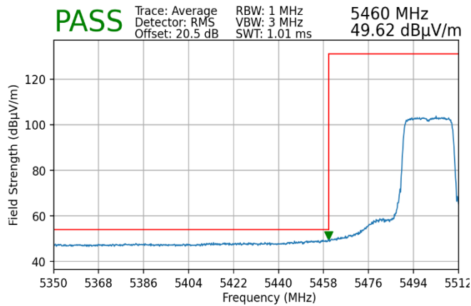
Plot 7-222. Radiated Lower Band Edge Plot MIMO (Average – UNII Band 2C)
