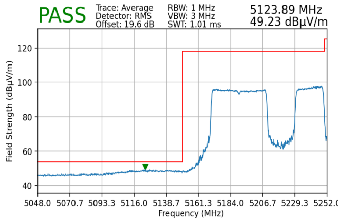
Plot 7-248. Radiated Lower Band Edge Plot MIMO (Average – UNII Band 1)
