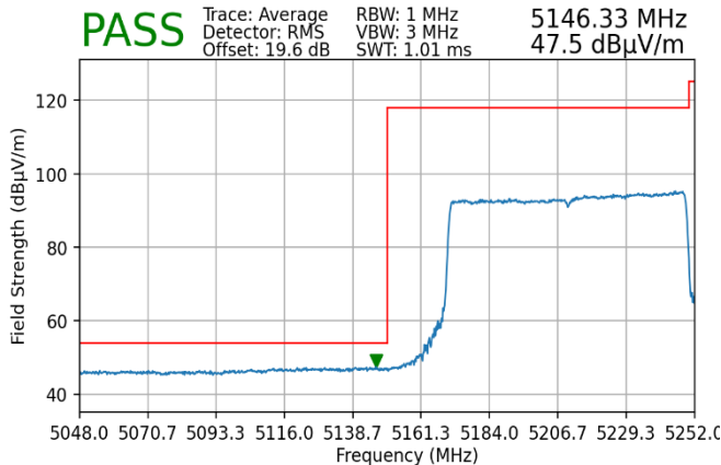
Plot 7-238. Radiated Lower Band Edge Plot MIMO (Average – UNII Band 1)
