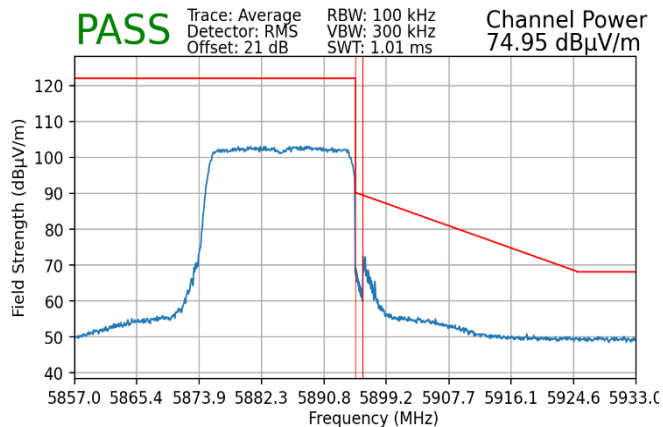
Plot 7-226. Radiated Upper Band Edge Plot MIMO (Average – UNII Band 4)
