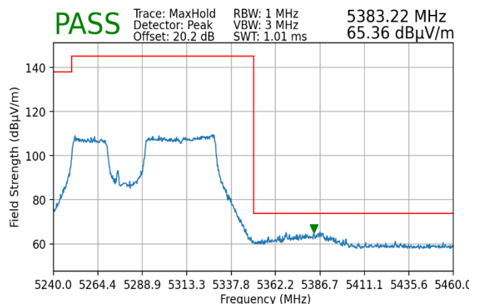
Plot 7-251. Radiated Upper Band Edge Plot MIMO (Peak – UNII Band 2A)
