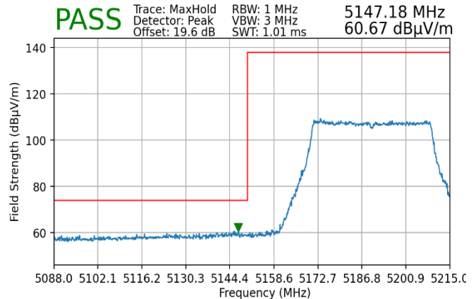
Plot 7-229. Radiated Lower Band Edge Plot MIMO (Peak – UNII Band 1)
