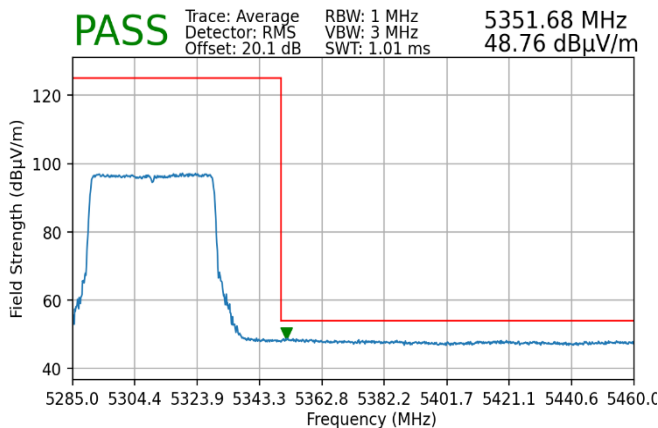
Plot 7-230. Radiated Upper Band Edge Plot MIMO (Average – UNII Band 2A)
