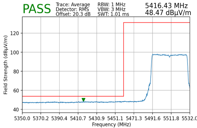
Plot 7-232. Radiated Lower Band Edge Plot MIMO (Average – UNII Band 2C)
