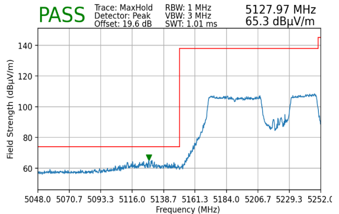
Plot 7-249. Radiated Lower Band Edge Plot MIMO (Peak – UNII Band 1)
