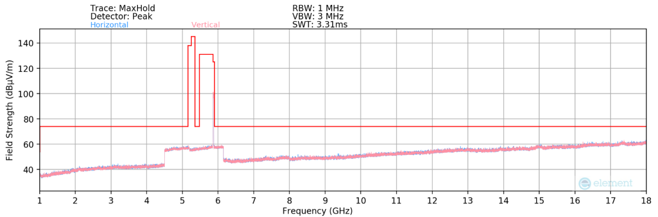
Plot 7-215. Radiated Spurious Plot above 1GHz MIMO (802.11a – UNII Band 4 Ch. 173)
