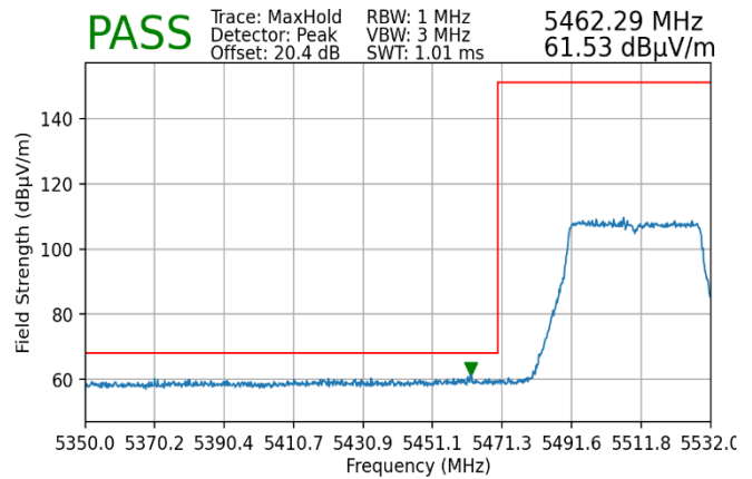
Plot 7-233. Radiated Lower Band Edge Plot MIMO (Peak – UNII Band 2C)
