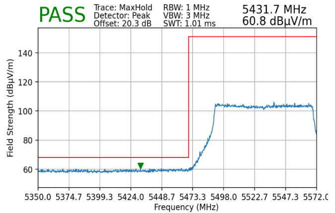
Plot 7-243. Radiated Lower Band Edge Plot MIMO (Peak – UNII Band 2C)
