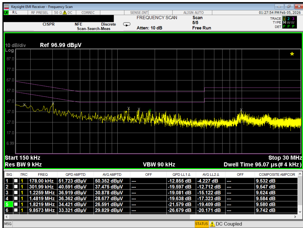
Plot 7-278. Line Conducted Plot with 802.11a UNII Band 3 (N)
