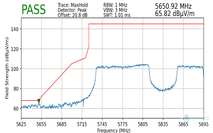
Plot 7-270. Radiated Lower Band Edge Plot MIMO (Peak – UNII Band 4)
