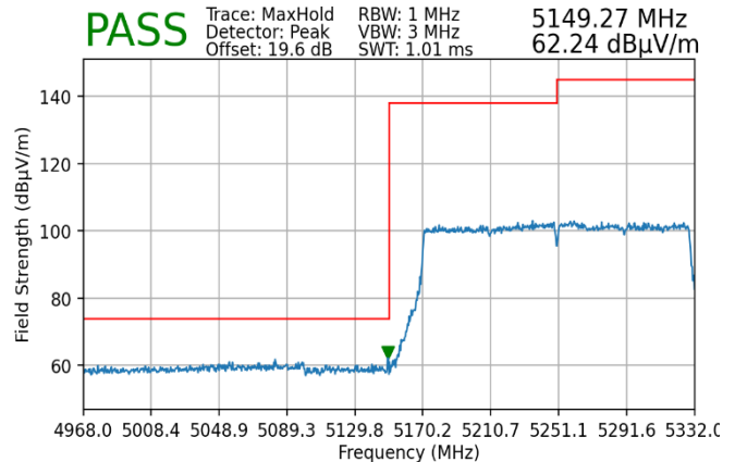
Plot 7-258. Radiated Lower Band Edge Plot MIMO (Peak – UNII Band 1)
