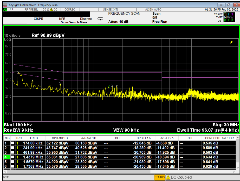
Plot 7-279. Line Conducted Plot with 802.11a UNII Band 4 (L1)
