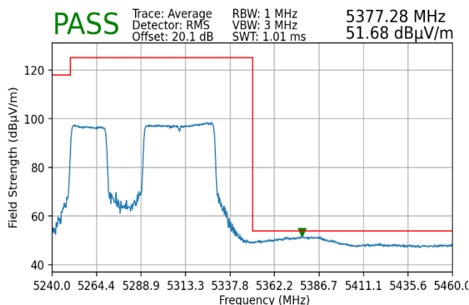
Plot 7-250. Radiated Upper Band Edge Plot MIMO (Average – UNII Band 2A)
