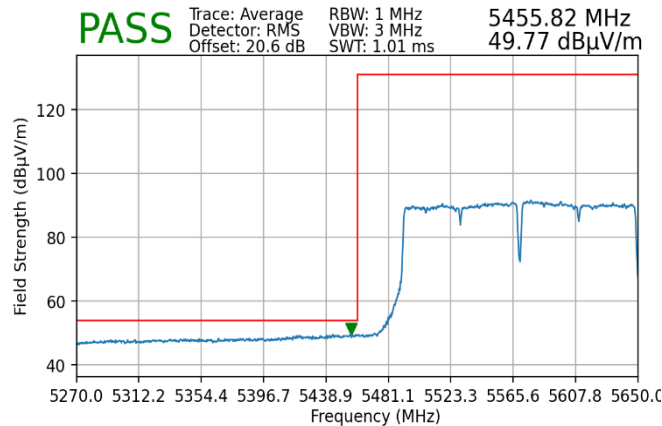
Plot 7-259. Radiated Lower Band Edge Plot MIMO (Average – UNII Band 2C)
