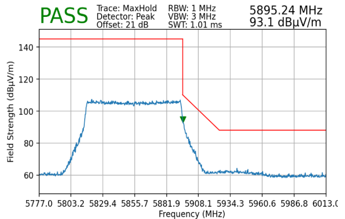
Plot 7-247. Radiated Upper Band Edge Plot MIMO (Peak – UNII Band 4)
