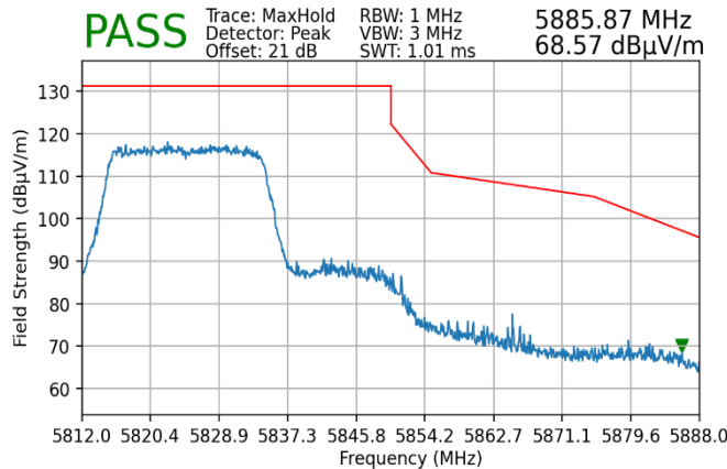
Plot 7-224. Radiated Upper Band Edge Plot MIMO (Peak – UNII Band 3)
