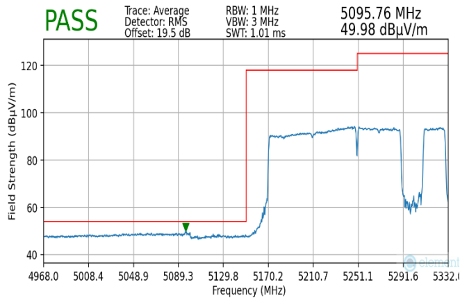
Plot 7-264. Radiated Lower Band Edge Plot MIMO (Average – UNII Band 1)
