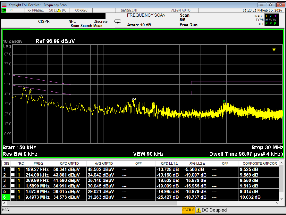
Plot 7-271. Line Conducted Plot with 802.11a UNII Band 1 (L1)
