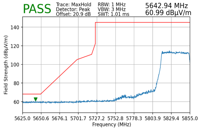
Plot 7-235. Radiated Lower Band Edge Plot MIMO (Peak – UNII Band 4)
