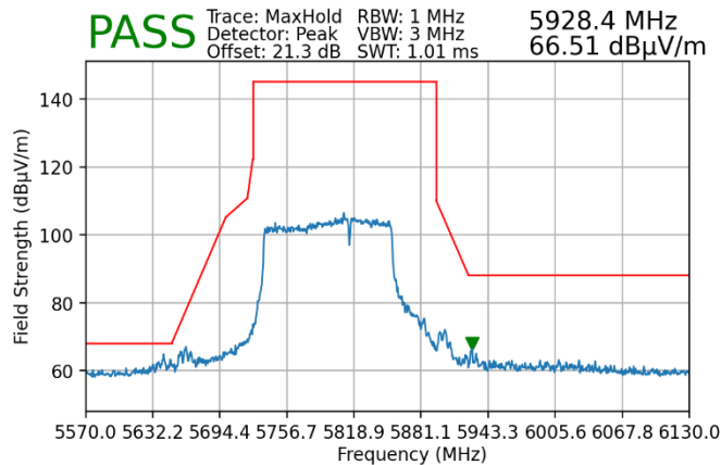
Plot 7-268. Radiated Lower Band Edge Plot MIMO (Peak – UNII Band 4)
