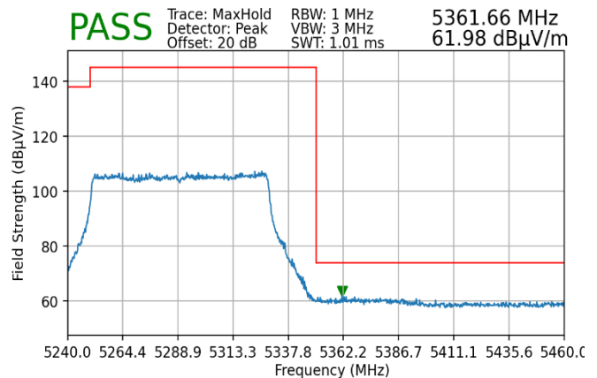
Plot 7-241. Radiated Upper Band Edge Plot MIMO (Peak – UNII Band 2A)
