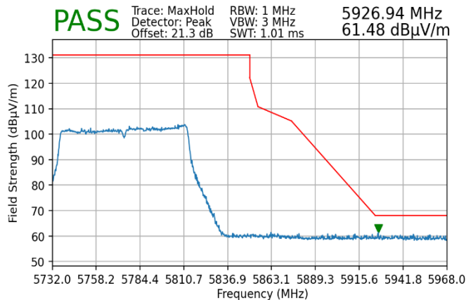
Plot 7-244. Radiated Upper Band Edge Plot MIMO (Peak – UNII Band 3)
