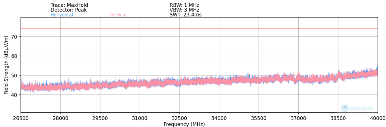
Plot 7-217. Radiated Spurious Plot 26.5GHz – 40GHz MIMO (802.11a)
