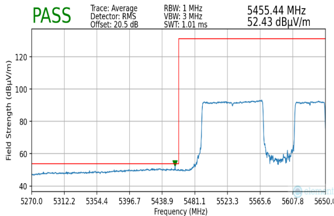
Plot 7-266. Radiated Lower Band Edge Plot MIMO (Average – UNII Band 2C)
