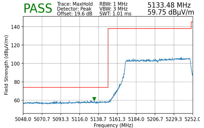
Plot 7-239. Radiated Lower Band Edge Plot MIMO (Peak – UNII Band 1)
