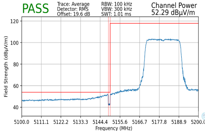
Plot 7-218. Radiated Lower Band Edge Plot MIMO (Average – UNII Band 1)
