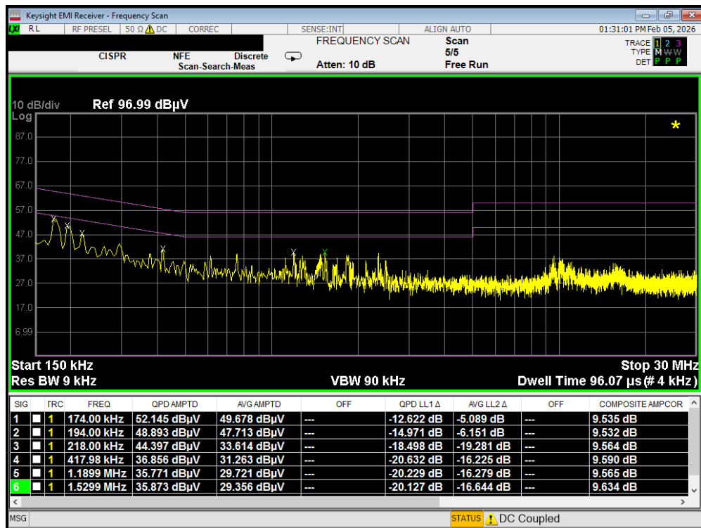
Plot 7-280. Line Conducted Plot with 802.11a UNII Band 4 (N)
