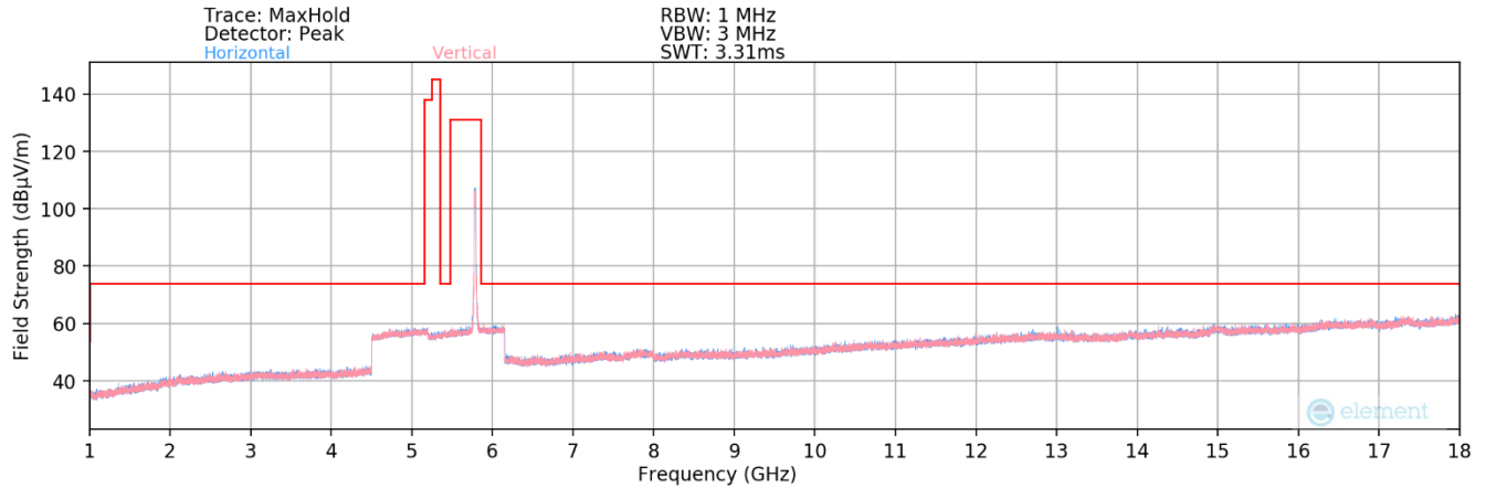
Plot 7-214. Radiated Spurious Plot above 1GHz MIMO (802.11a – UNII Band 3 Ch. 157)
