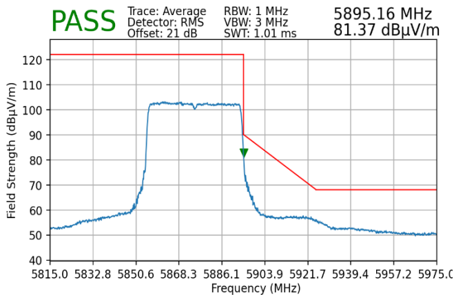
Plot 7-236. Radiated Upper Band Edge Plot MIMO (Average – UNII Band 4)
