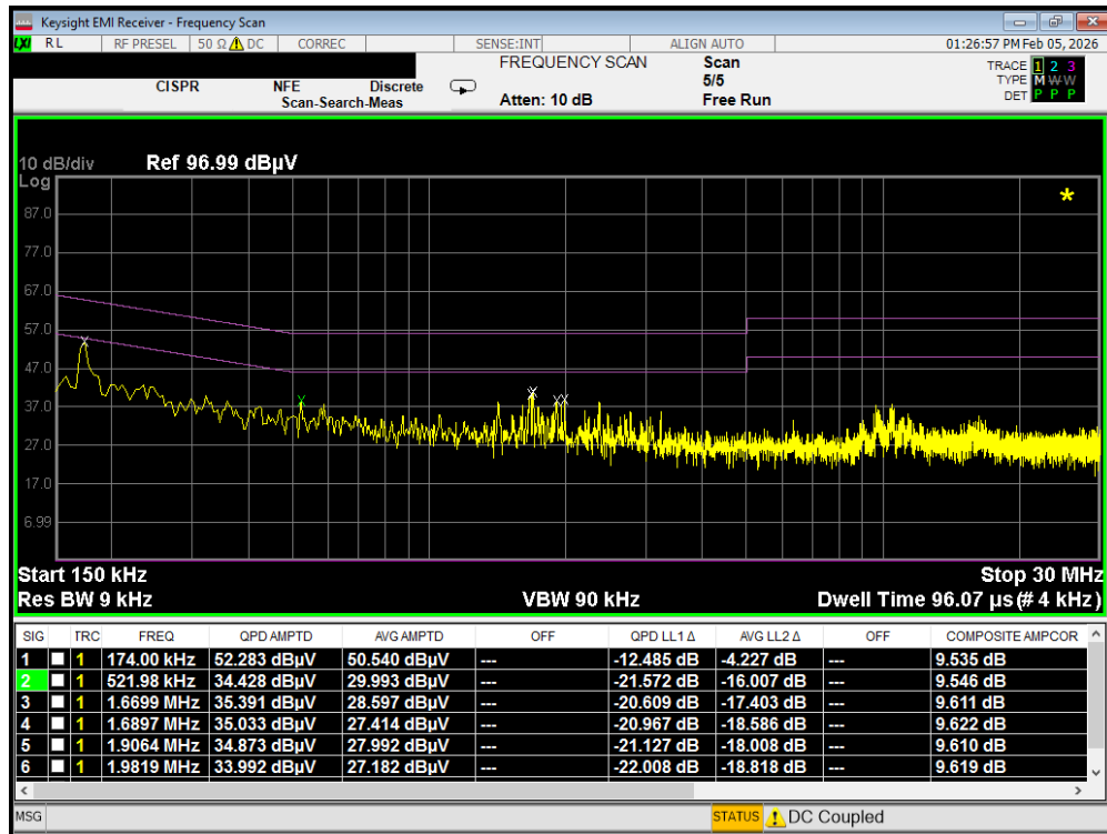
Plot 7-277. Line Conducted Plot with 802.11a UNII Band 3 (L1)
