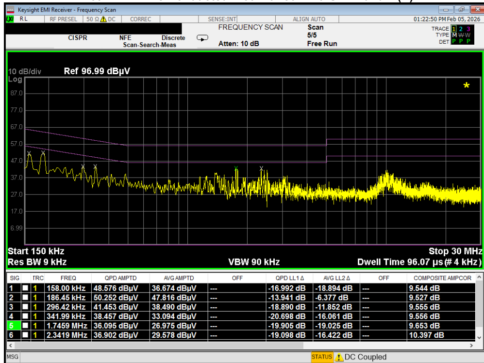
Plot 7-273. Line Conducted Plot with 802.11a UNII Band 2A (L1)
