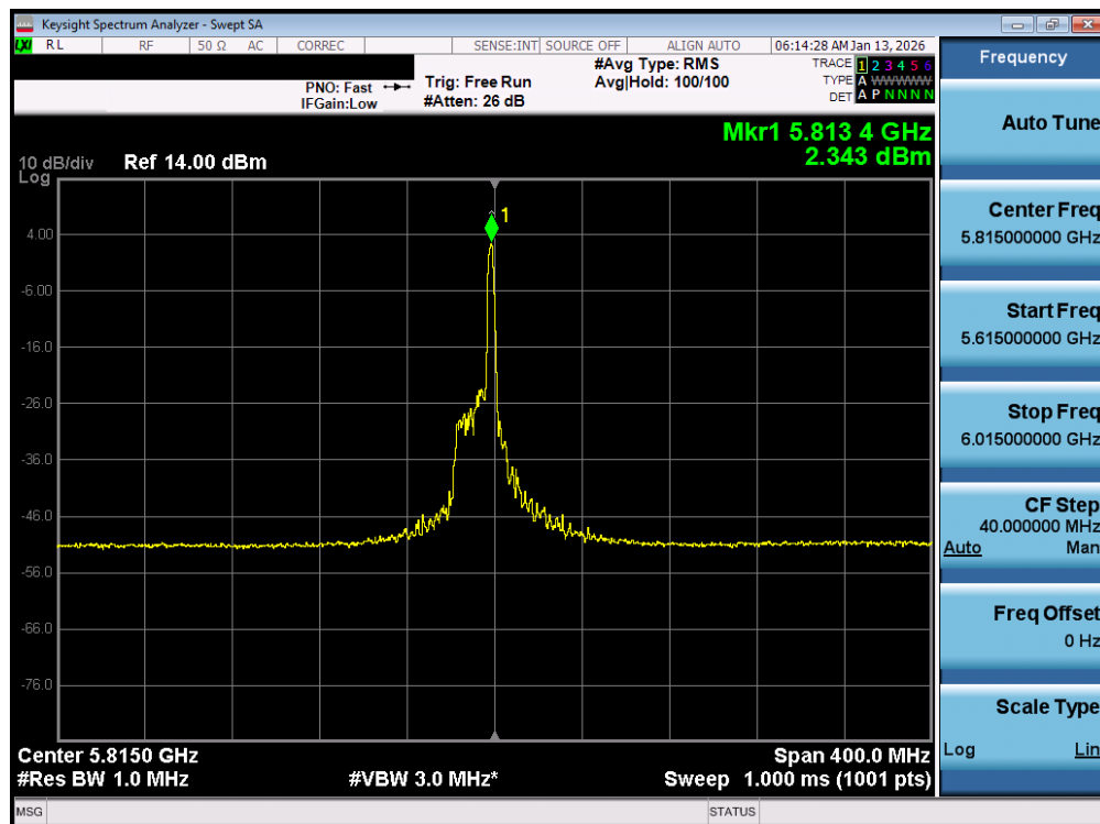
Plot 7-97. Power Spectral Density Plot MIMO ANT1 (160MHz(U) BW 802.11be – 26 Tones (UNII Band 3/4) – Ch. 163)
