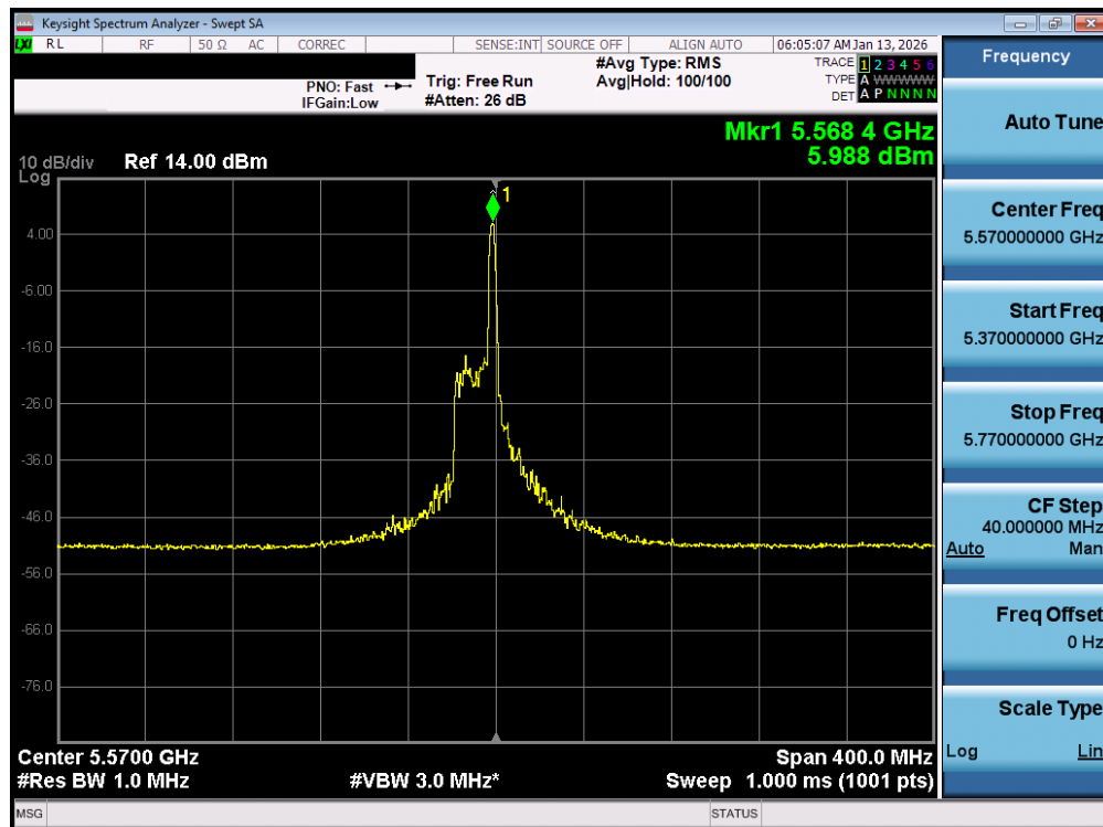
Plot 7-90. Power Spectral Density Plot MIMO ANT1 (160MHz BW 802.11be – 26 Tones (UNII Band 2C) – Ch. 114)
