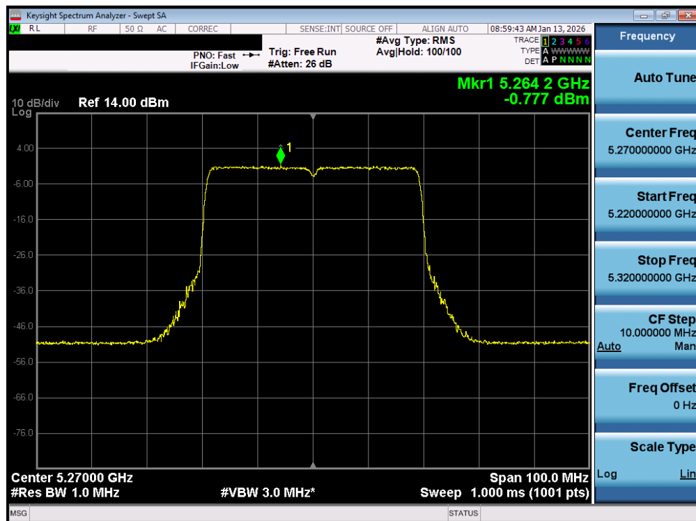
Plot 7-103. Power Spectral Density Plot MIMO ANT1 (40MHz BW 802.11be – 484 Tones (UNII Band 2A) – Ch. 54)
