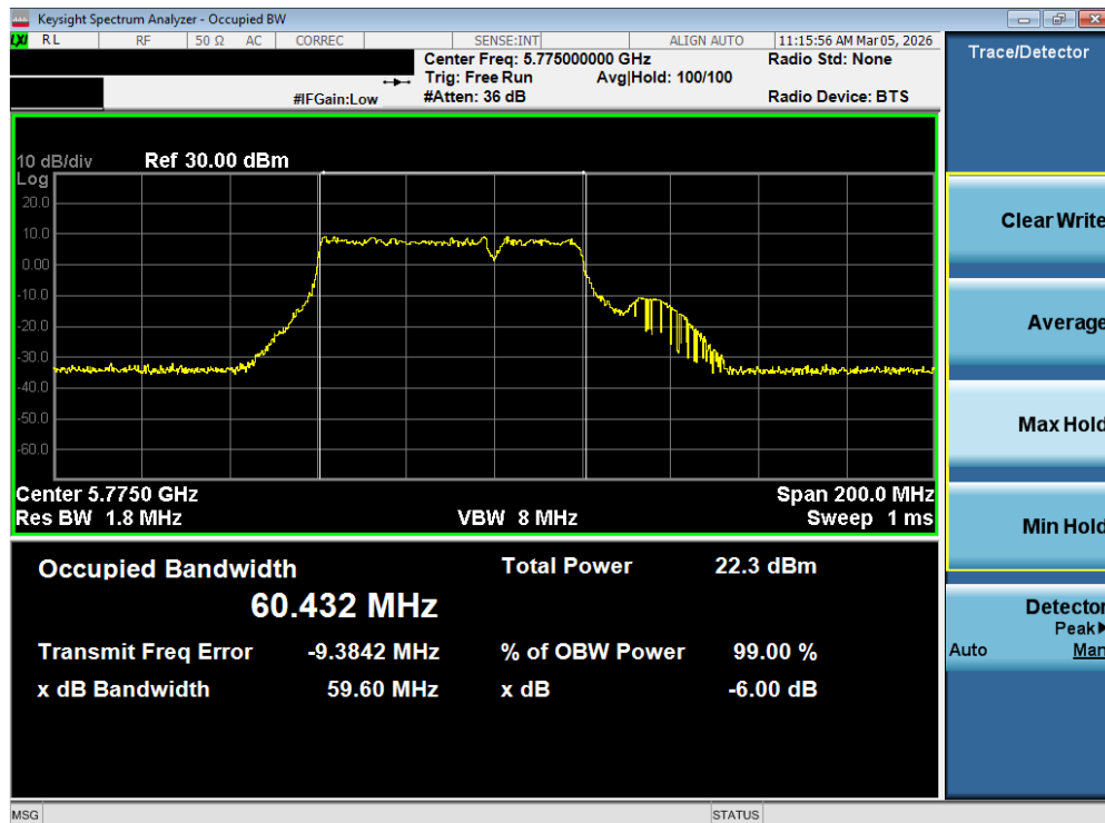
Plot 7-79. 6dB Bandwidth Plot MIMO ANT2 (80MHz BW 802.11be – 484 + 242 Tones (UNII Band 3) – Ch. 155)
