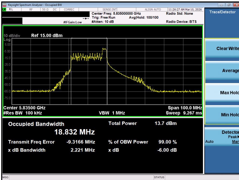
Plot 7-67. 6dB Bandwidth Plot MIMO ANT2 (40MHz BW 802.11be – 26 Tones (UNII Band 3/4) – Ch. 167)
