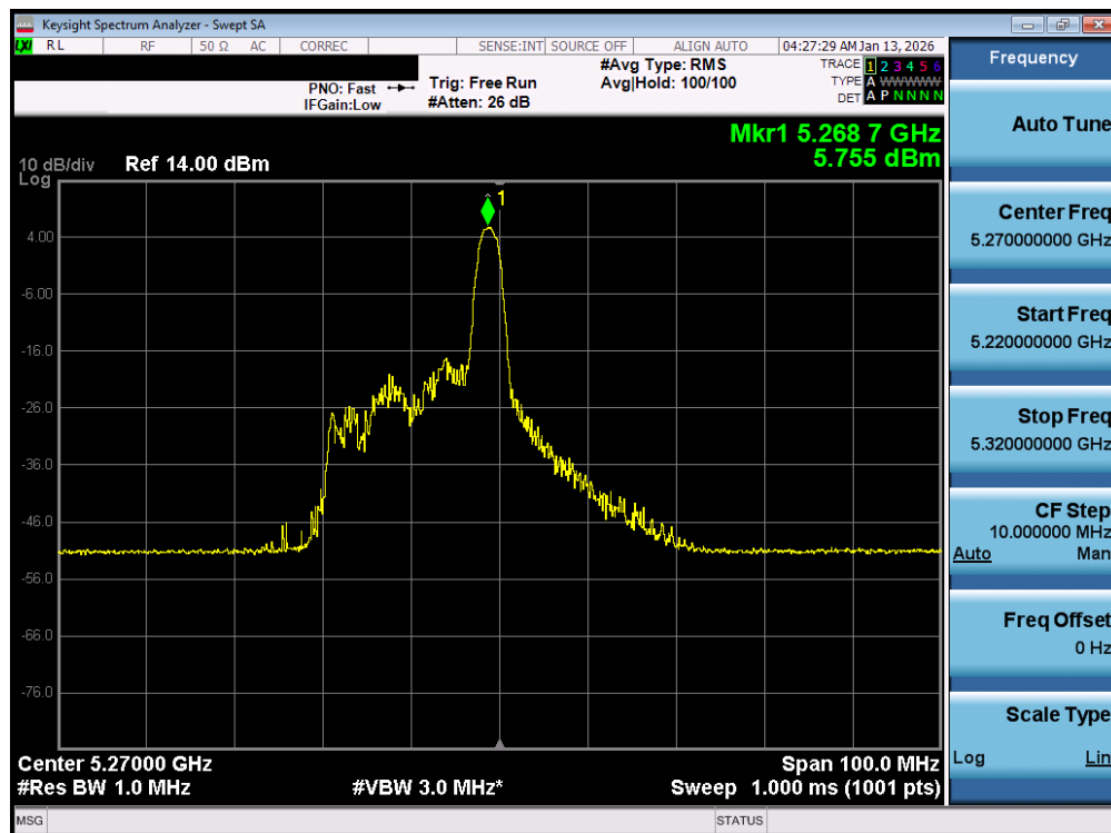
Plot 7-85. Power Spectral Density Plot MIMO ANT1 (40MHz BW 802.11be – 26 Tones (UNII Band 2A) – Ch. 54)
