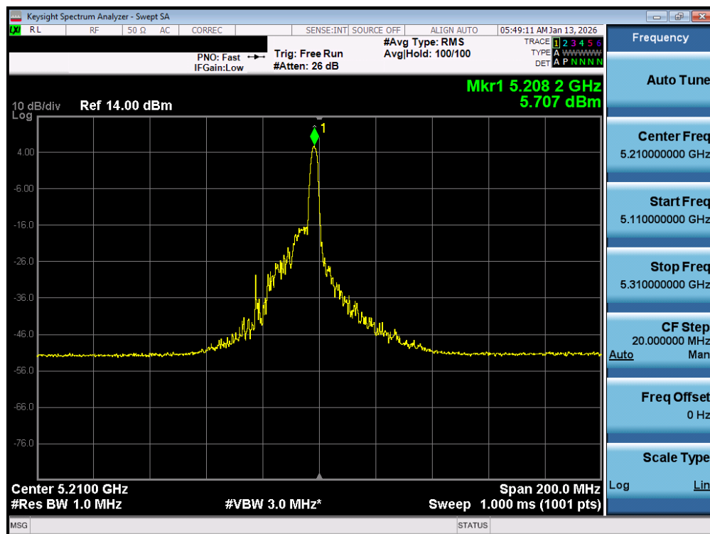
Plot 7-82. Power Spectral Density Plot MIMO ANT1 (80MHz BW 802.11be – 26 Tones (UNII Band 1) – Ch. 42)
