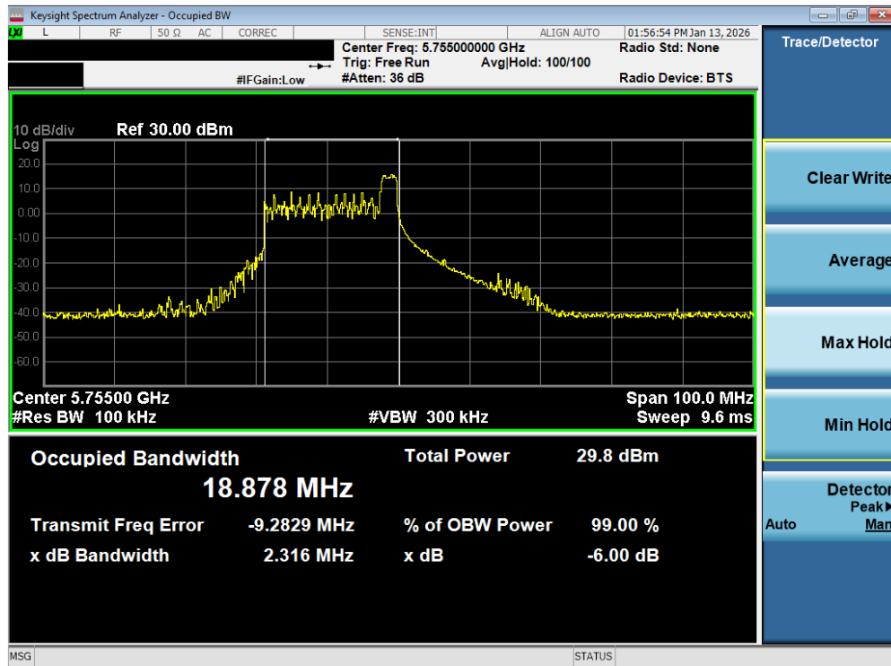
Plot 7-63. 6dB Bandwidth Plot MIMO ANT2 (40MHz BW 802.11be – 26 Tones (UNII Band 3) – Ch. 151)
