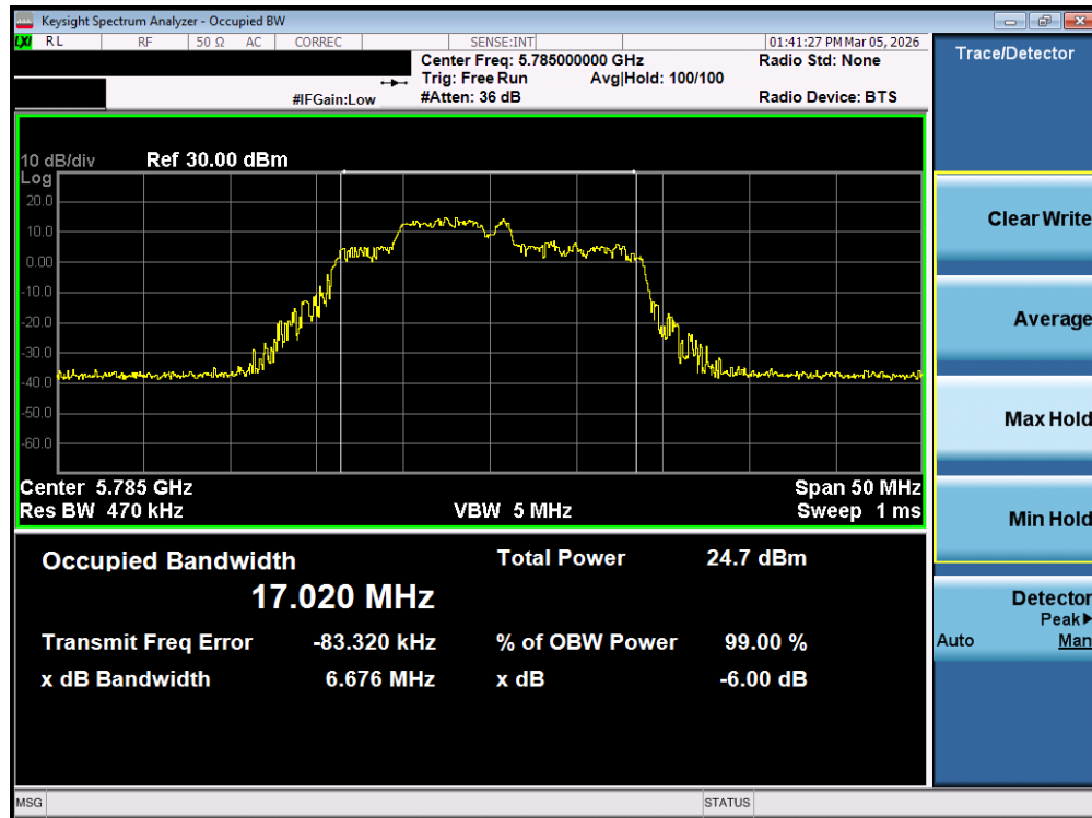
Plot 7-59. 6dB Bandwidth Plot MIMO ANT1 (20MHz BW 802.11be – 52 + 26 Tones (UNII Band 3) – Ch. 157)
