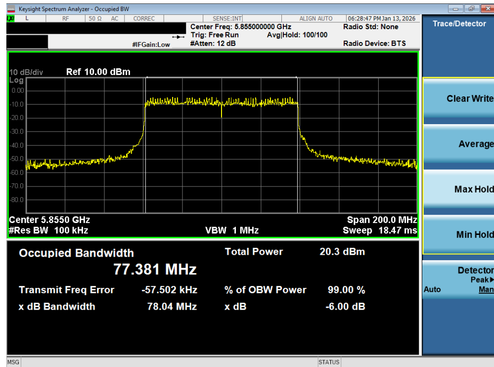
Plot 7-75. 6dB Bandwidth Plot MIMO ANT2 (80MHz BW 802.11be – 996 Tones (UNII Band 3/4) – Ch. 171)
