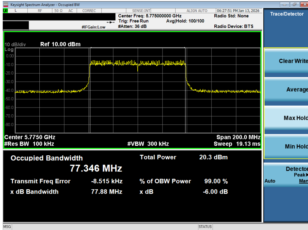
Plot 7-72. 6dB Bandwidth Plot MIMO ANT2 (80MHz BW 802.11be – 996 Tones (UNII Band 3) – Ch. 155)
