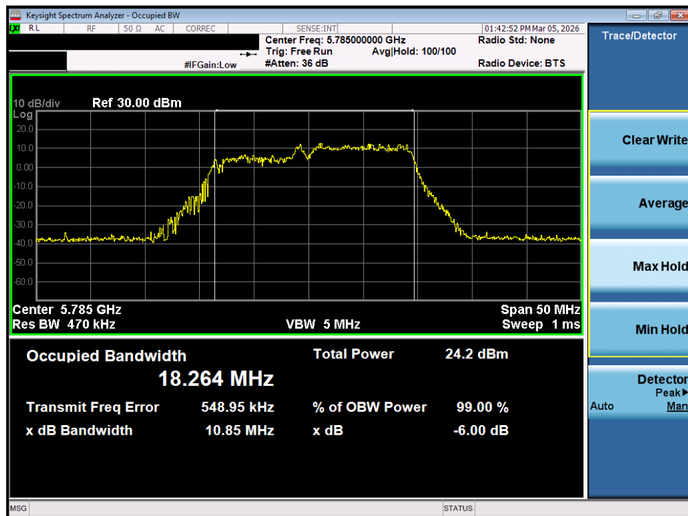
Plot 7-60. 6dB Bandwidth Plot MIMO ANT1 (20MHz BW 802.11be – 106 + 26 Tones (UNII Band 3) – Ch. 157)
