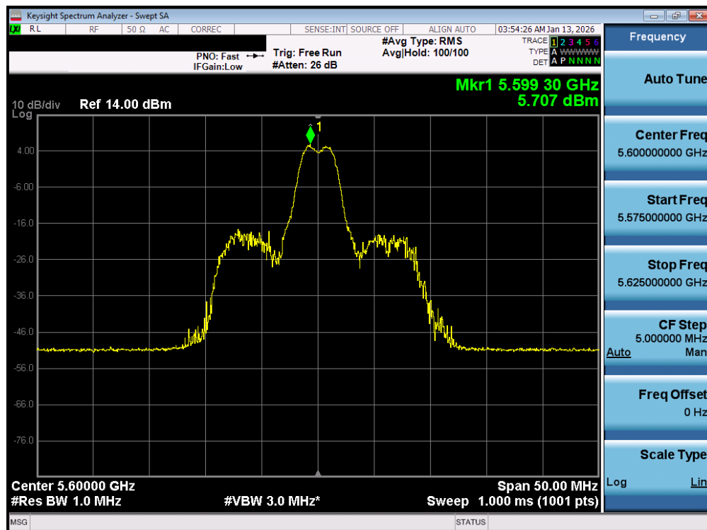
Plot 7-87. Power Spectral Density Plot MIMO ANT1 (20MHz BW 802.11be – 26 Tones (UNII Band 2C) – Ch. 120)
