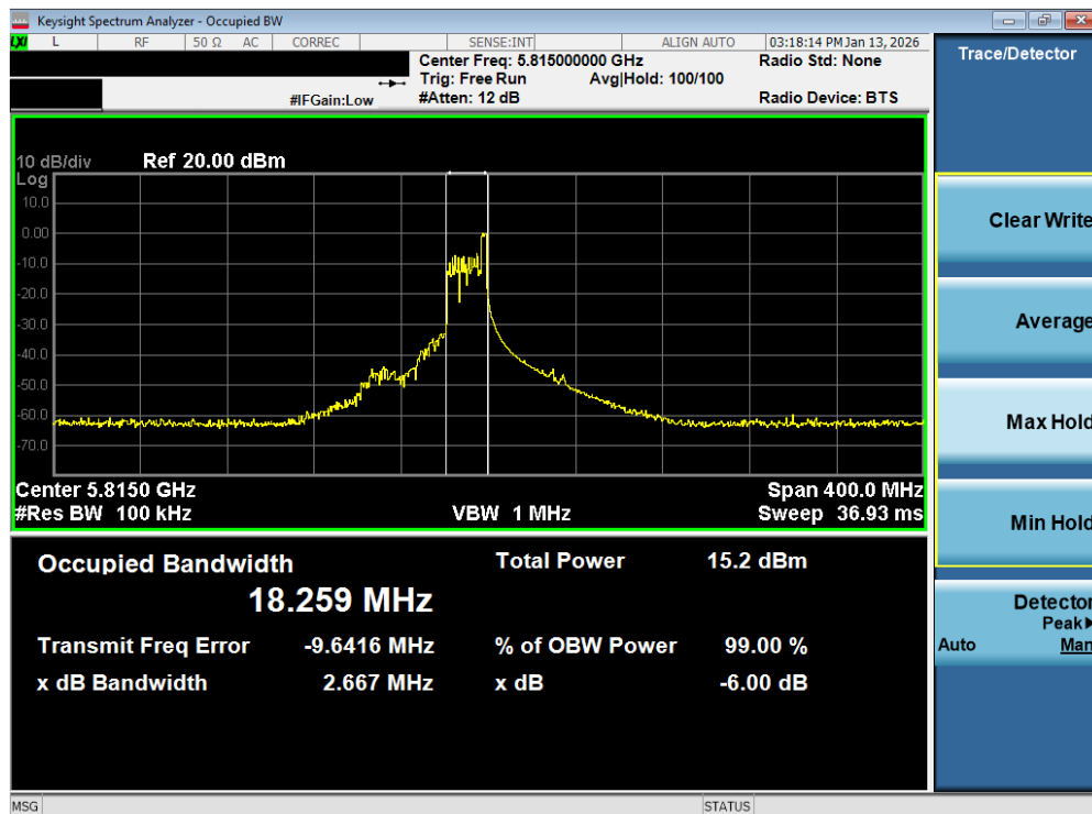
Plot 7-69. 6dB Bandwidth Plot MIMO ANT2 (160MHz(U) BW 802.11be – 26 Tones (UNII Band 3/4) – Ch. 163)
