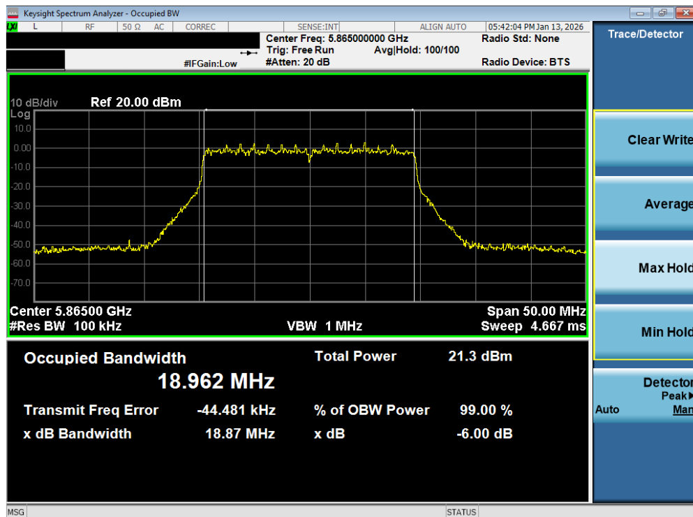
Plot 7-73. 6dB Bandwidth Plot MIMO ANT2 (20MHz BW 802.11be – 242 Tones (UNII Band 4) – Ch. 173)
