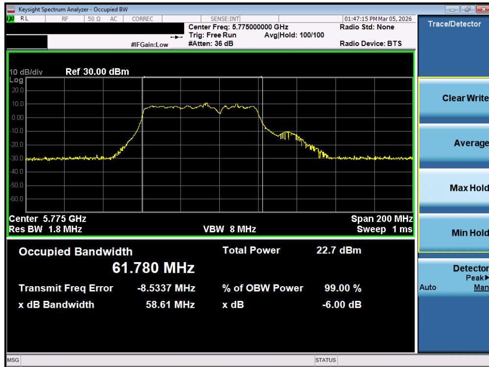
Plot 7-61. 6dB Bandwidth Plot MIMO ANT1 (80MHz BW 802.11be – 484 + 242 Tones (UNII Band 3) – Ch. 155)
