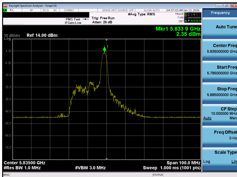
Plot 7-95. Power Spectral Density Plot MIMO ANT1 (40MHz BW 802.11be – 26 Tones (UNII Band 3/4) – Ch. 167)
