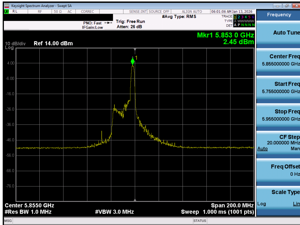
Plot 7-96. Power Spectral Density Plot MIMO ANT1 (80MHz BW 802.11be – 26 Tones (UNII Band 3/4) – Ch. 171)
