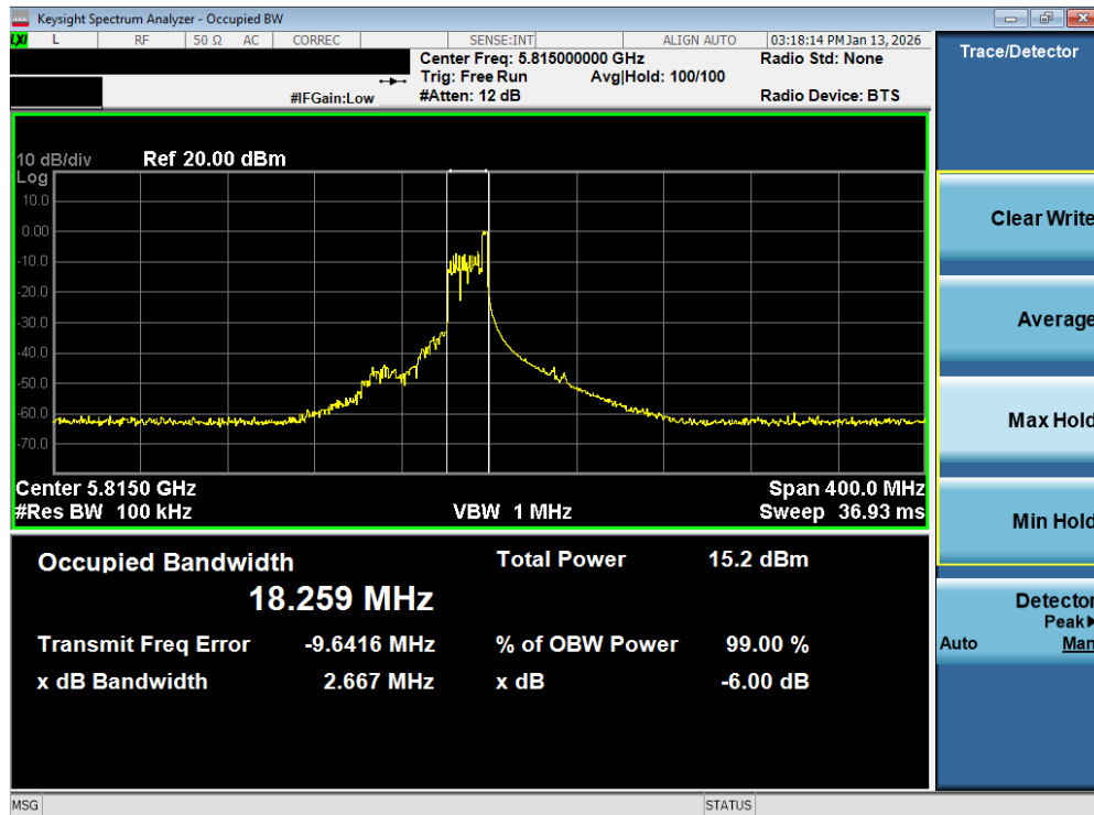
Plot 7-65. 6dB Bandwidth Plot MIMO ANT2 (160MHz BW 802.11be – 26 Tones (UNII Band 3/4) – Ch. 163)
