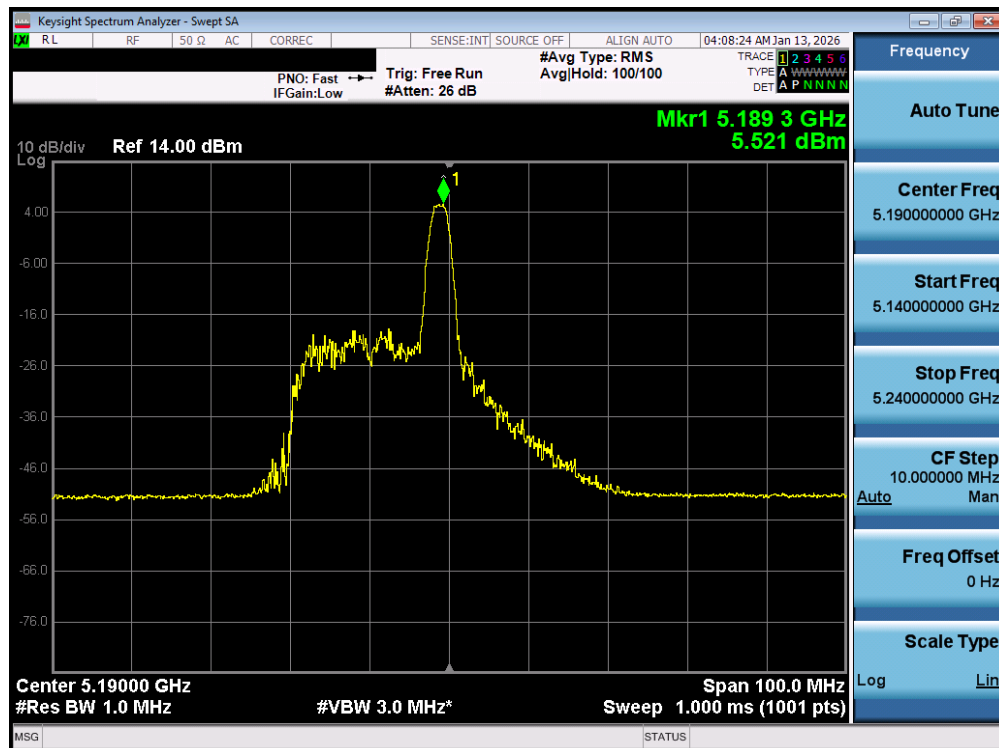
Plot 7-81. Power Spectral Density Plot MIMO ANT1 (40MHz BW 802.11be – 26 Tones (UNII Band 1) – Ch. 38)
