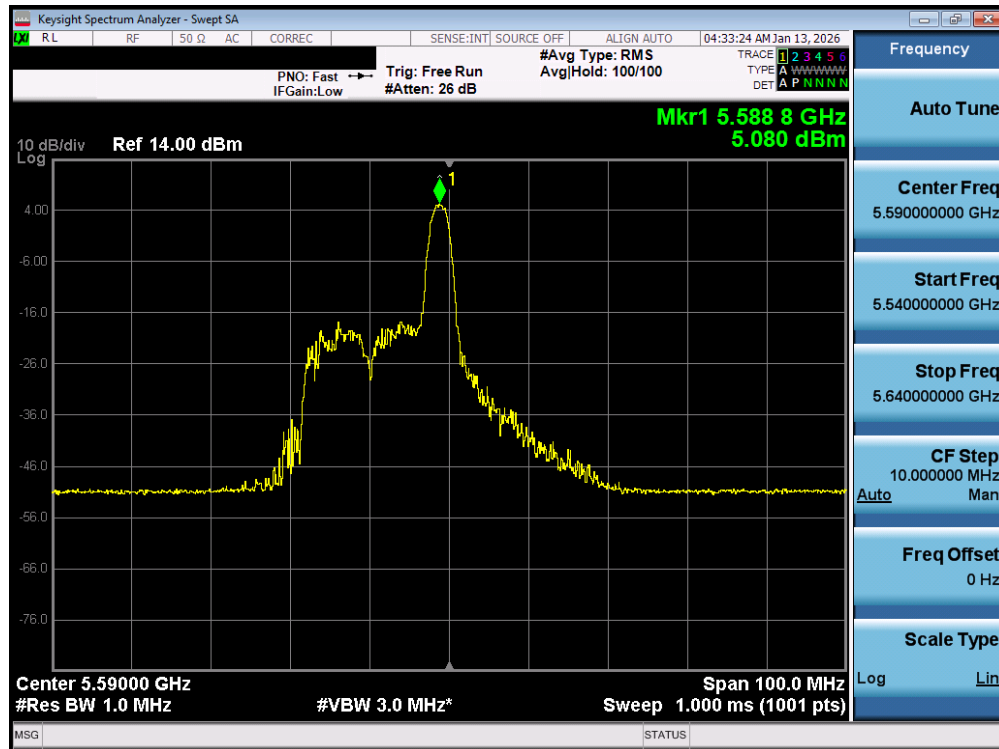
Plot 7-88. Power Spectral Density Plot MIMO ANT1 (40MHz BW 802.11be – 26 Tones (UNII Band 2C) – Ch. 118)
