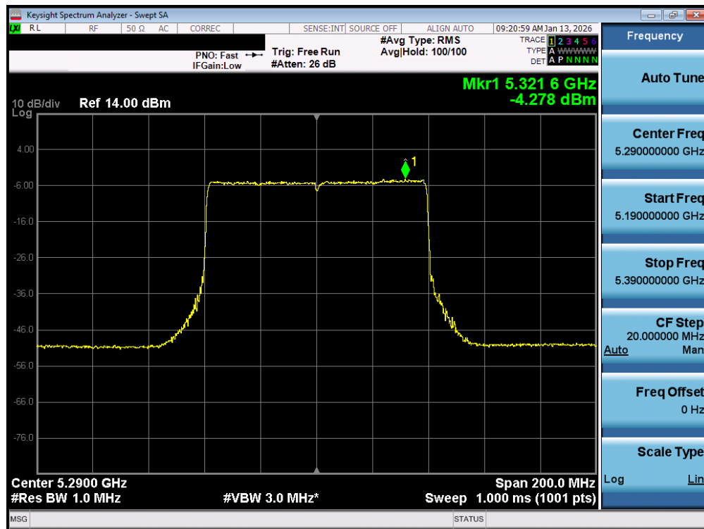
Plot 7-104. Power Spectral Density Plot MIMO ANT1 (80MHz BW 802.11be – 996 Tones (UNII Band 2A) – Ch. 58)
