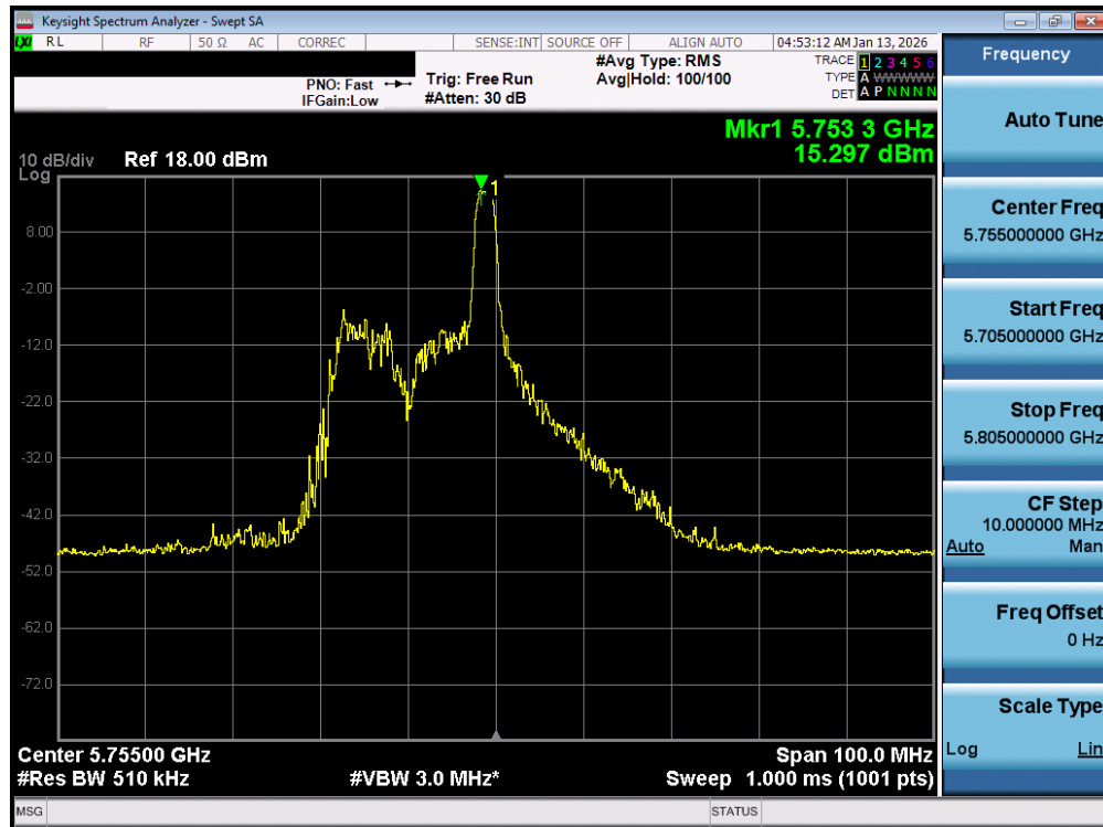
Plot 7-92. Power Spectral Density Plot MIMO ANT1 (40MHz BW 802.11be – 26 Tones (UNII Band 3) – Ch. 151)
