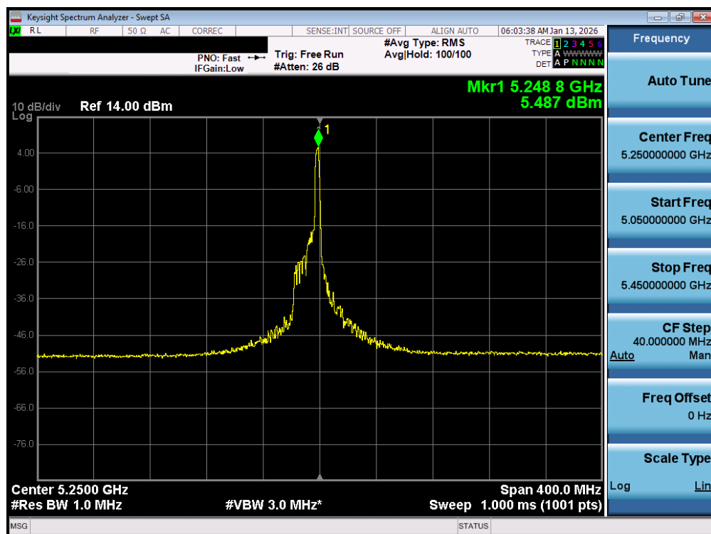
Plot 7-83. Power Spectral Density Plot MIMO ANT1 (160MHz BW 802.11be – 26 Tones (UNII Band 1/2A) – Ch. 50)
