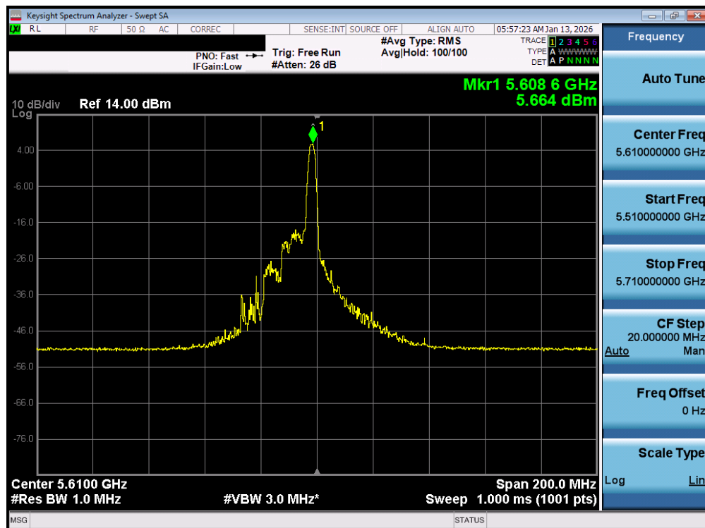
Plot 7-89. Power Spectral Density Plot MIMO ANT1 (80MHz BW 802.11be – 26 Tones (UNII Band 2C) – Ch. 122)
