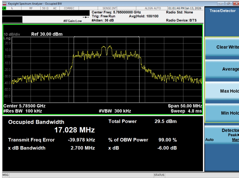
Plot 7-62. 6dB Bandwidth Plot MIMO ANT2 (20MHz BW 802.11be – 26 Tones (UNII Band 3) – Ch. 157)
