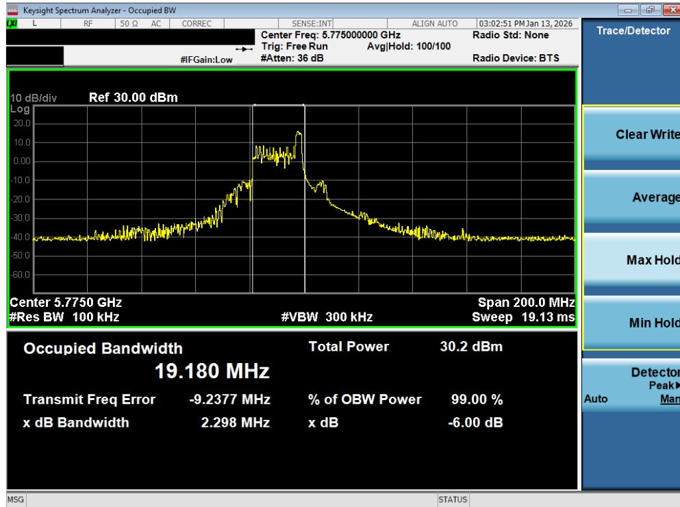
Plot 7-64. 6dB Bandwidth Plot MIMO ANT2 (80MHz BW 802.11be – 26 Tones (UNII Band 3) – Ch. 155)
