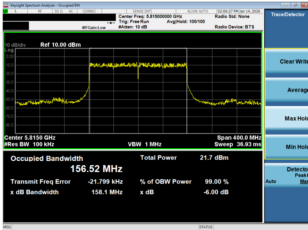
Plot 7-76. 6dB Bandwidth Plot MIMO ANT2 (160MHz BW 802.11be – 996*2 Tones (UNII Band 3/4) – Ch. 163)
