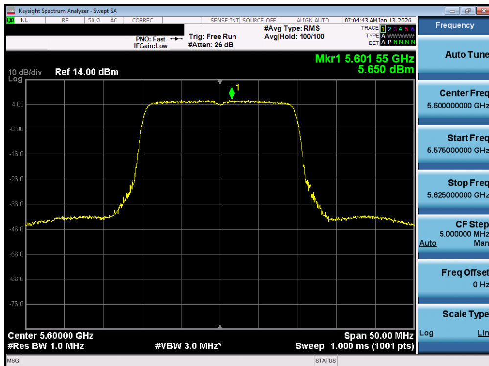
Plot 7-105. Power Spectral Density Plot MIMO ANT1 (20MHz BW 802.11be – 242 Tones (UNII Band 2C) – Ch. 120)
