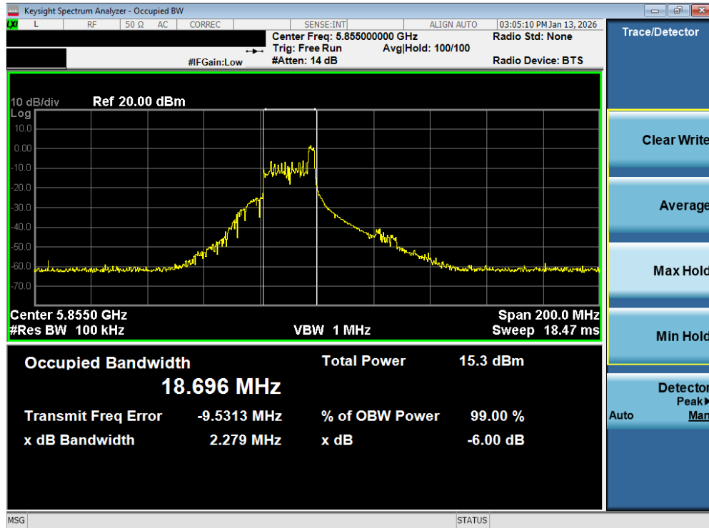
Plot 7-68. 6dB Bandwidth Plot MIMO ANT2 (80MHz BW 802.11be – 26 Tones (UNII Band 3/4) – Ch. 171)
