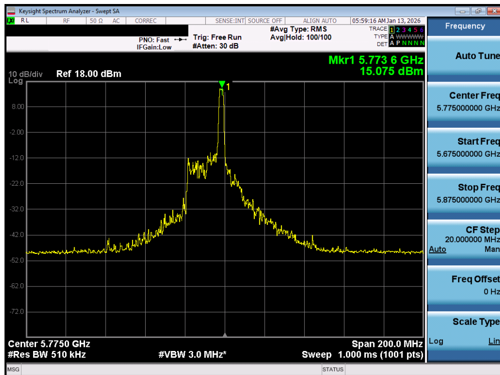
Plot 7-93. Power Spectral Density Plot MIMO ANT1 (80MHz BW 802.11be – 26 Tones (UNII Band 3) – Ch. 155)
