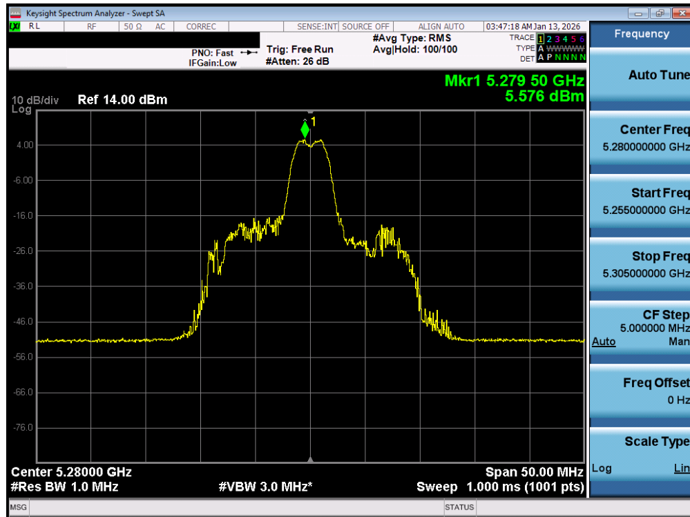
Plot 7-84. Power Spectral Density Plot MIMO ANT1 (20MHz BW 802.11be – 26 Tones (UNII Band 2A) – Ch. 56)
