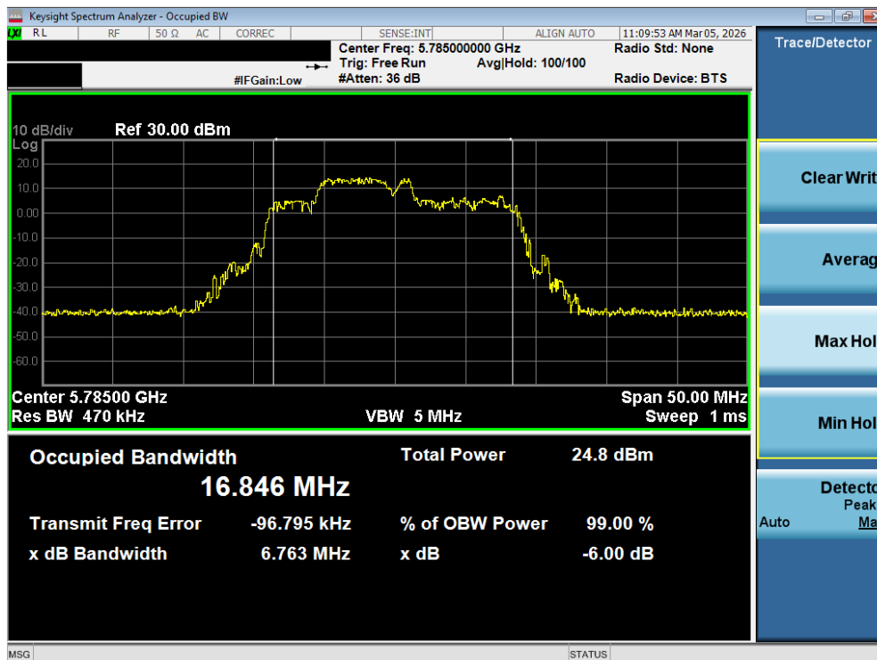
Plot 7-77. 6dB Bandwidth Plot MIMO ANT2 (20MHz BW 802.11be – 52 +26 Tones (UNII Band 3) – Ch. 157)
