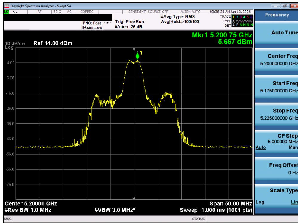
Plot 7-80. Power Spectral Density Plot MIMO ANT1 (20MHz BW 802.11be – 26 Tones (UNII Band 1) – Ch. 40)
