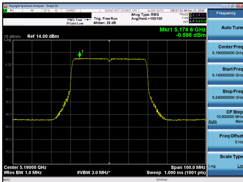
Plot 7-99. Power Spectral Density Plot MIMO ANT1 (40MHz BW 802.11be – 484 Tones (UNII Band 1) – Ch. 38)
