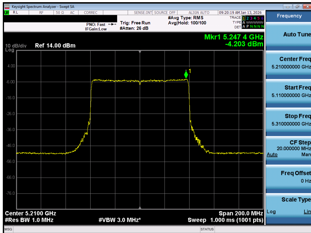
Plot 7-100. Power Spectral Density Plot MIMO ANT1 (80MHz BW 802.11be – 996 Tones (UNII Band 1) – Ch. 42)
