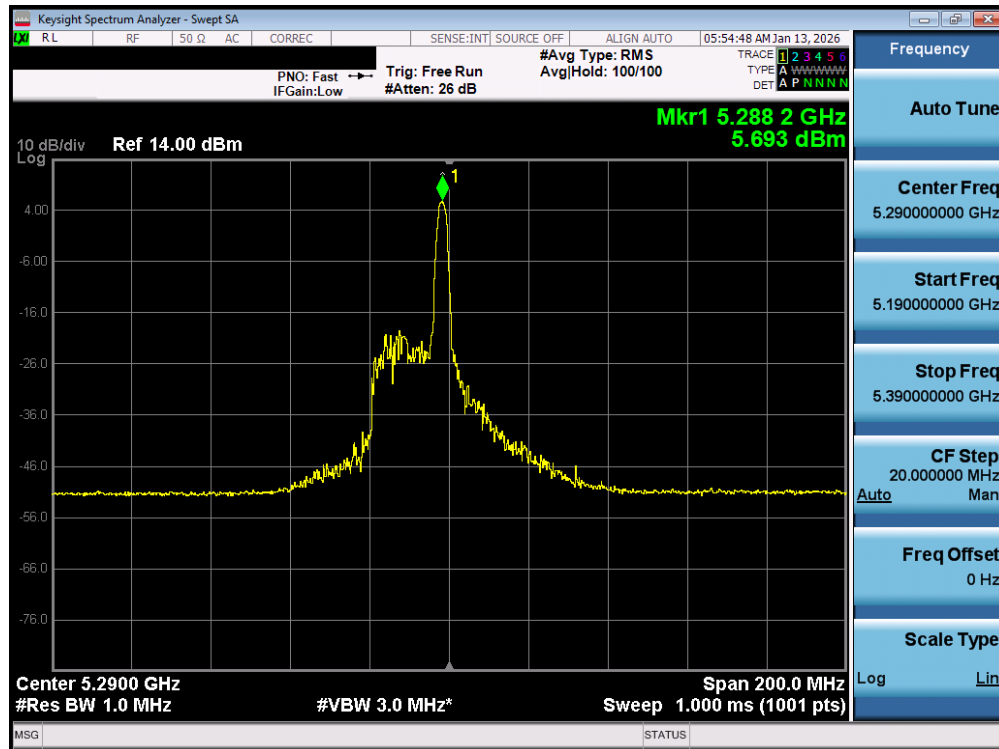
Plot 7-86. Power Spectral Density Plot MIMO ANT1 (80MHz BW 802.11be – 26 Tones (UNII Band 2A) – Ch. 58)
