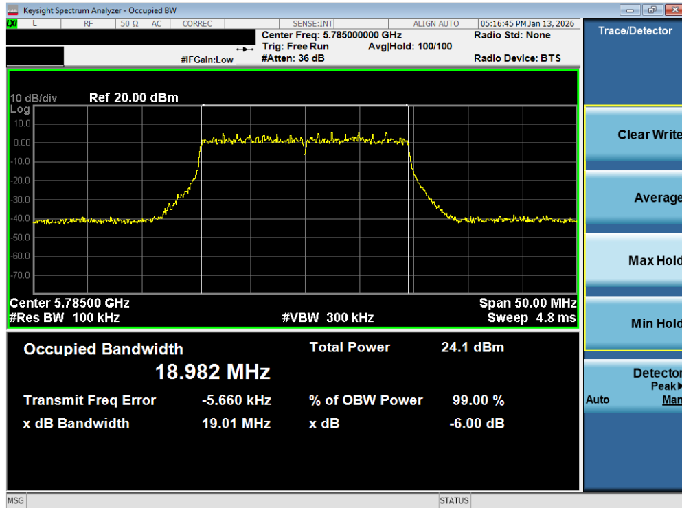
Plot 7-70. 6dB Bandwidth Plot MIMO ANT2 (20MHz BW 802.11be – 242 Tones (UNII Band 3) – Ch. 157)
