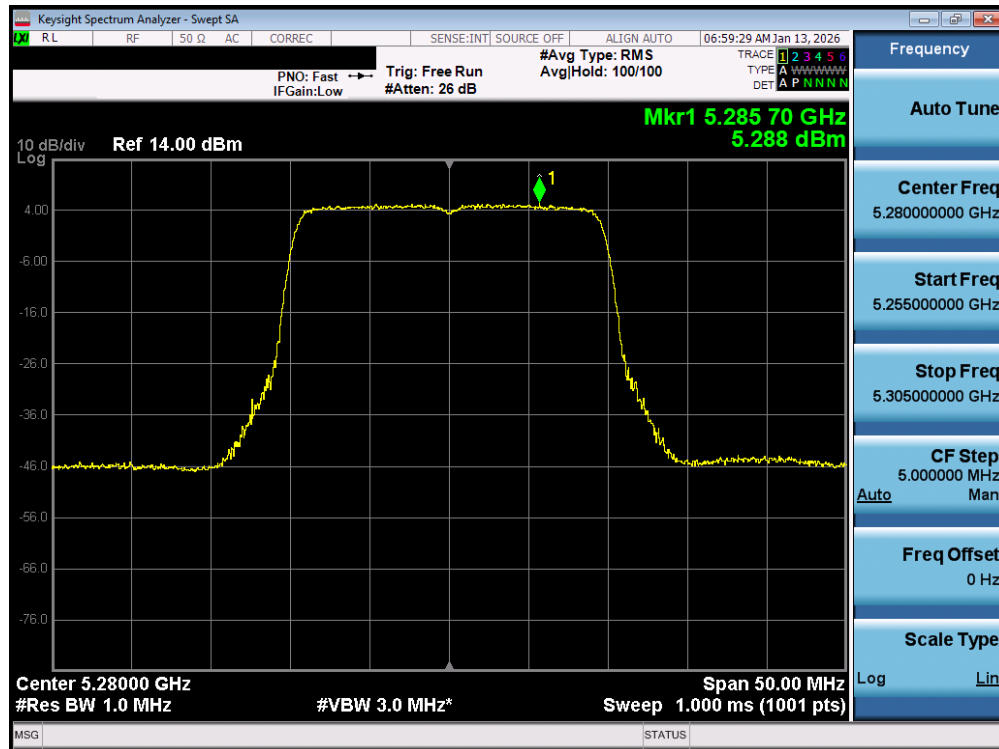
Plot 7-102. Power Spectral Density Plot MIMO ANT1 (20MHz BW 802.11be – 242 Tones (UNII Band 2A) – Ch. 56)
