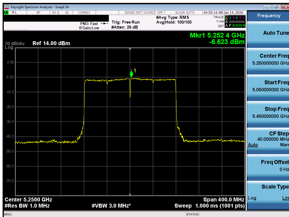
Plot 7-101. Power Spectral Density Plot MIMO ANT1 (160MHz BW 802.11be – 2x996 Tones (UNII Band 1/2A) – Ch. 50)
