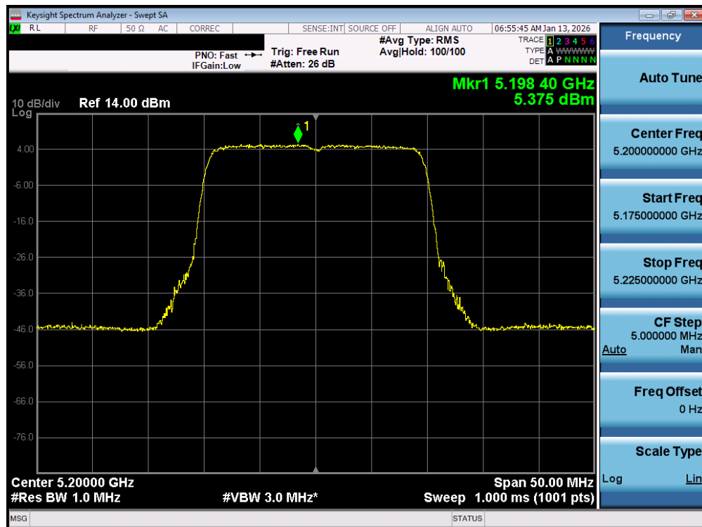
Plot 7-98. Power Spectral Density Plot MIMO ANT1 (20MHz BW 802.11be – 242 Tones (UNII Band 1) – Ch. 40)
