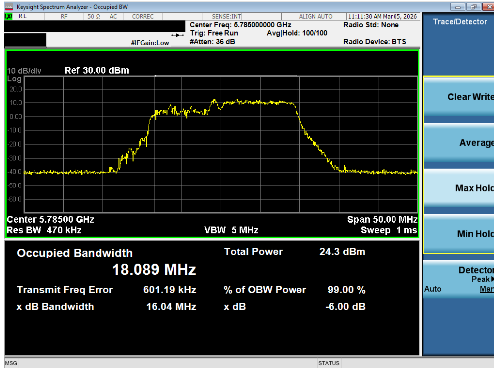
Plot 7-78. 6dB Bandwidth Plot MIMO ANT2 (20MHz BW 802.11be – 106 + 26 Tones (UNII Band 3) – Ch. 157)
