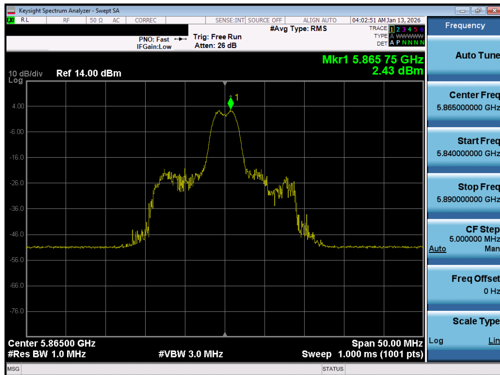
Plot 7-94. Power Spectral Density Plot MIMO ANT1 (20MHz BW 802.11be – 26 Tones (UNII Band 4) – Ch. 173)
