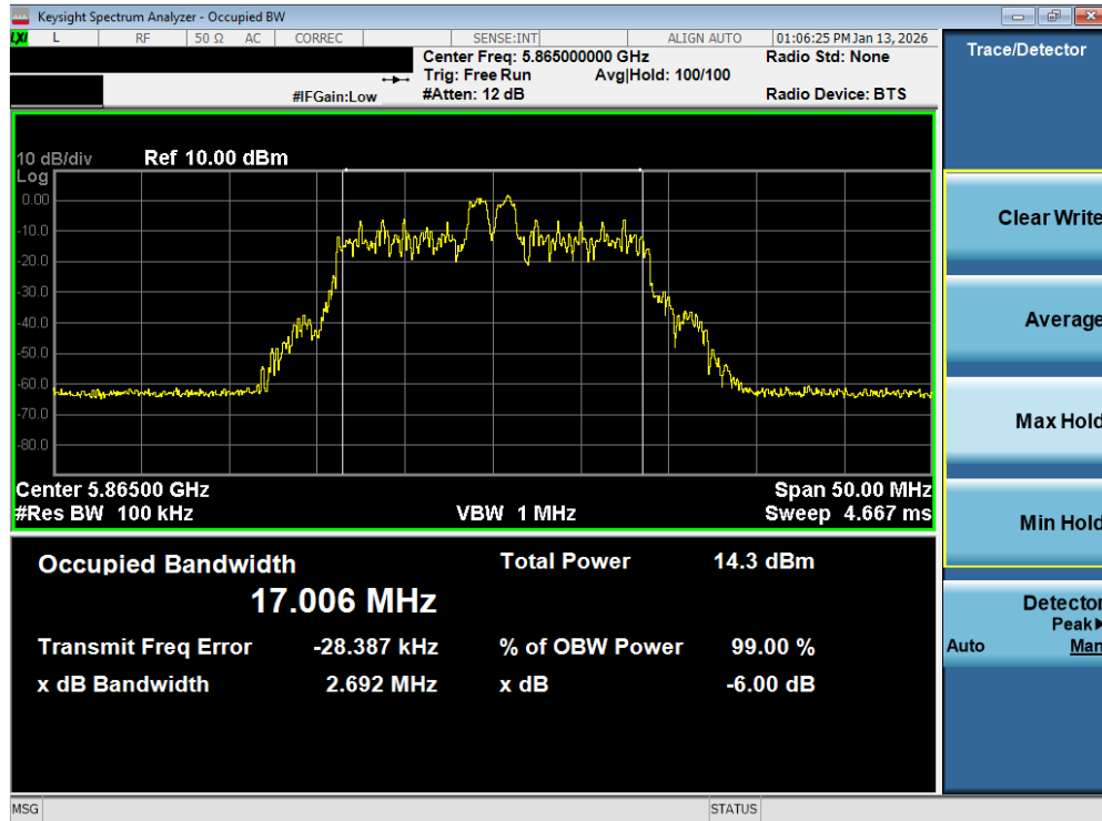
Plot 7-66. 6dB Bandwidth Plot MIMO ANT2 (20MHz BW 802.11be – 26 Tones (UNII Band 4) – Ch. 173)
