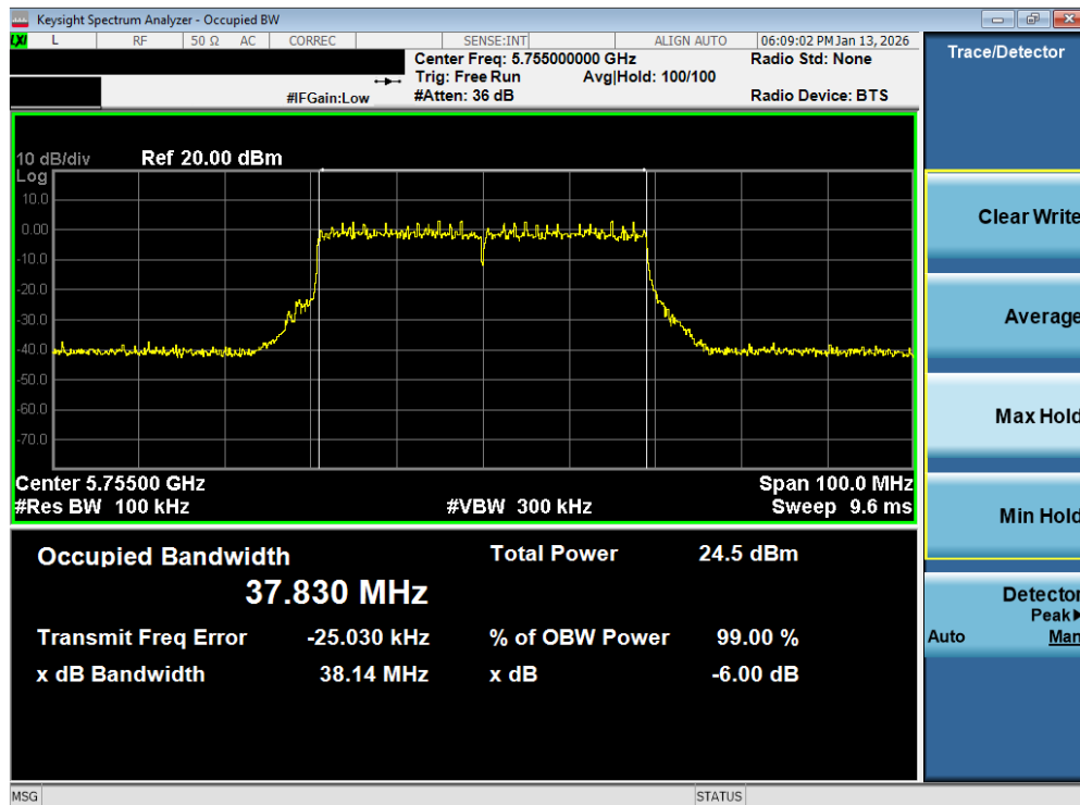
Plot 7-71. 6dB Bandwidth Plot MIMO ANT2 (40MHz BW 802.11be – 484 Tones (UNII Band 3) – Ch. 151)
