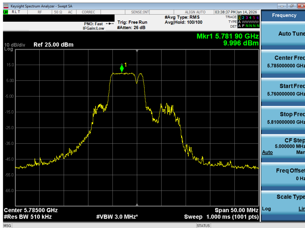
Plot 7-181. Power Spectral Density Plot MIMO ANT2 (20MHz BW 802.11be – 52+26 Tones (UNII Band 3) – Ch. 157)
