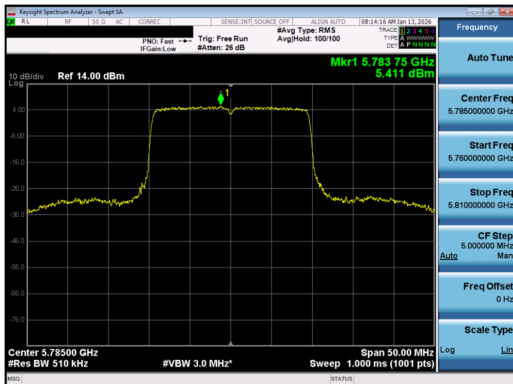
Plot 7-109. Power Spectral Density Plot MIMO ANT1 (20MHz BW 802.11be – 242 Tones (UNII Band 3) – Ch. 157)
