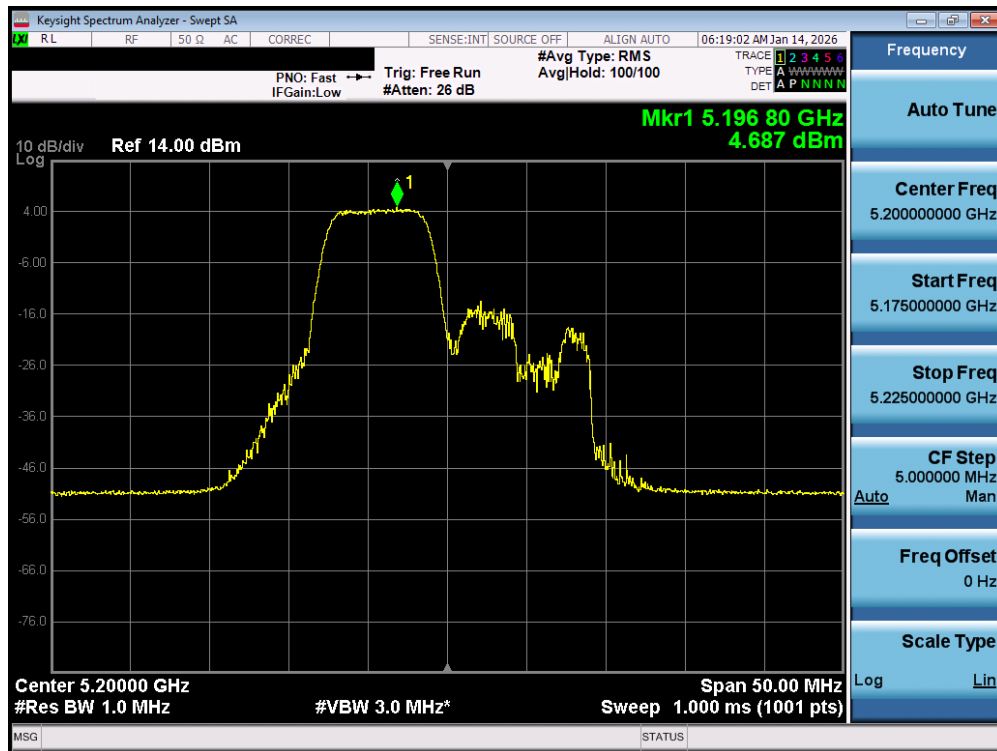
Plot 7-116. Power Spectral Density Plot MIMO ANT1 (20MHz BW 802.11be – 52+26 Tones (UNII Band 1) – Ch. 40)
