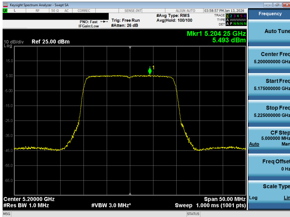
Plot 7-152. Power Spectral Density Plot MIMO ANT2 (20MHz BW 802.11be – 242 Tones (UNII Band 1) – Ch. 40)
