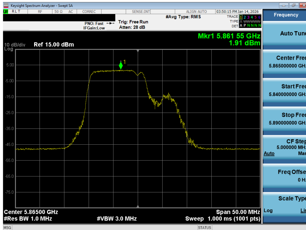
Plot 7-185. Power Spectral Density Plot MIMO ANT2 (20MHz BW 802.11be – 106+26 Tones (UNII Band 4) – Ch. 173)
