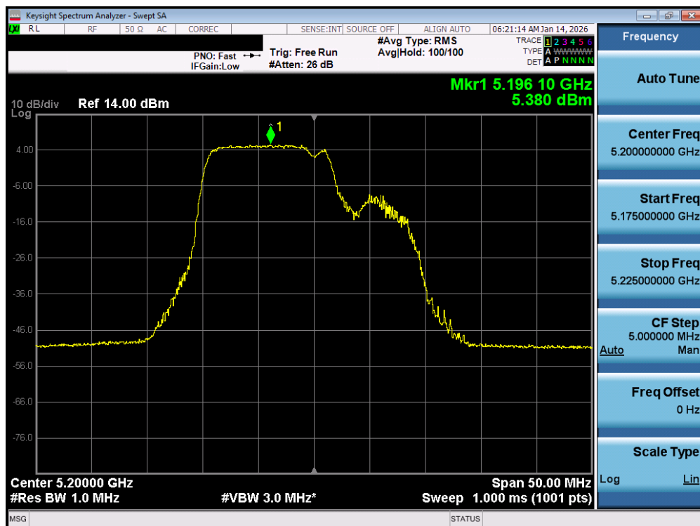
Plot 7-117. Power Spectral Density Plot MIMO ANT1 (20MHz BW 802.11be – 106+26 Tones (UNII Band 1) – Ch. 40)
