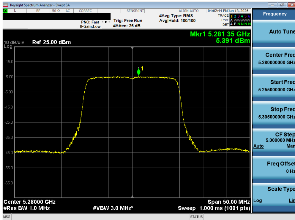
Plot 7-156. Power Spectral Density Plot MIMO ANT2 (20MHz BW 802.11be – 242 Tones (UNII Band 2A) – Ch. 56)
