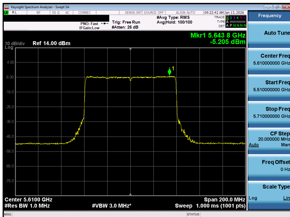
Plot 7-107. Power Spectral Density Plot MIMO ANT1 (80MHz BW 802.11be – 996 Tones (UNII Band 2C) – Ch. 122)
