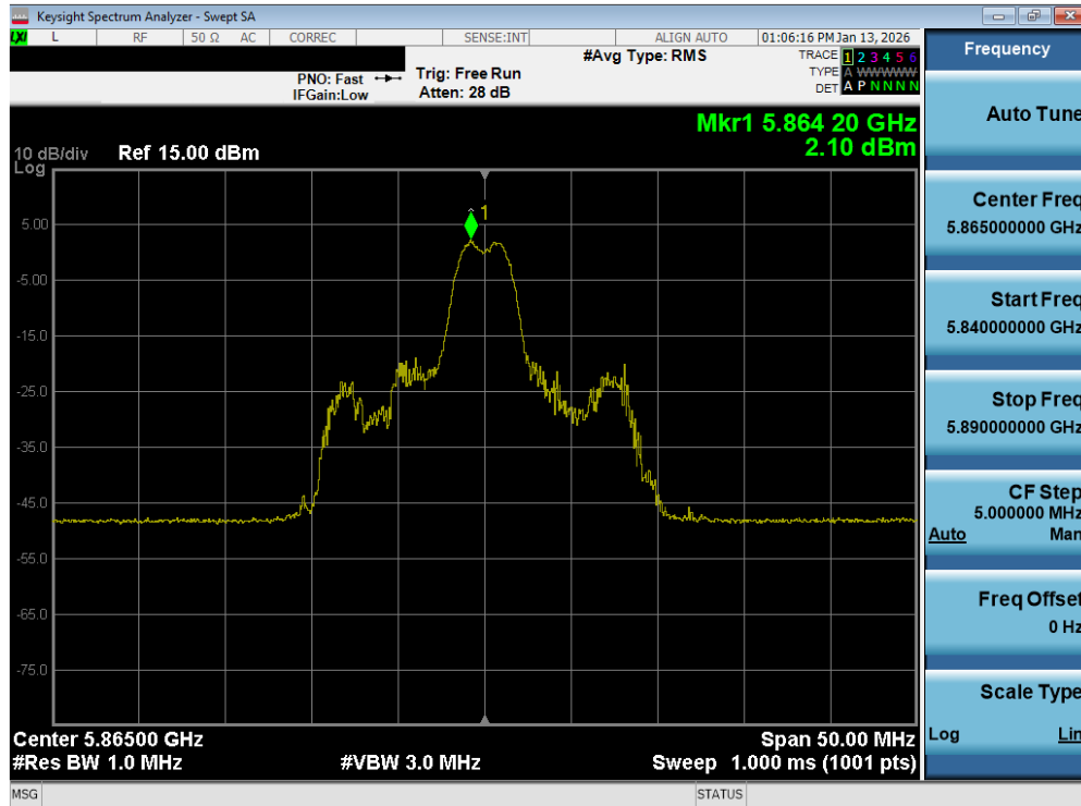
Plot 7-148. Power Spectral Density Plot MIMO ANT2 (20MHz BW 802.11be – 26 Tones (UNII Band 4) – Ch. 173)
