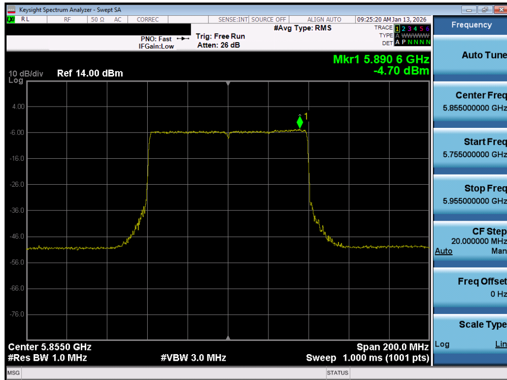
Plot 7-114. Power Spectral Density Plot MIMO ANT1 (80MHz BW 802.11be – 996 Tones (UNII Band 3/4) – Ch. 171)
