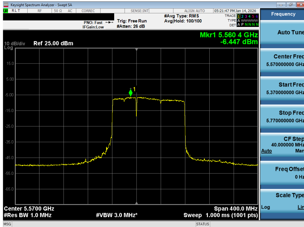
Plot 7-180. Power Spectral Density Plot MIMO ANT2 (160MHz BW 802.11be – 996+484 Tones (UNII Band 2C) – Ch. 114)
