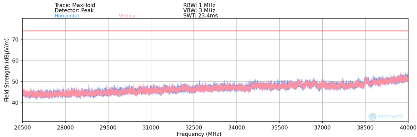
Plot 7-201. Radiated Spurious Plot 26.5GHz - 40GHz (802.11be)
