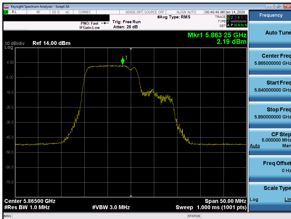
Plot 7-131. Power Spectral Density Plot MIMO ANT1 (20MHz BW 802.11be – 106+26 Tones (UNII Band 4) – Ch. 173)
