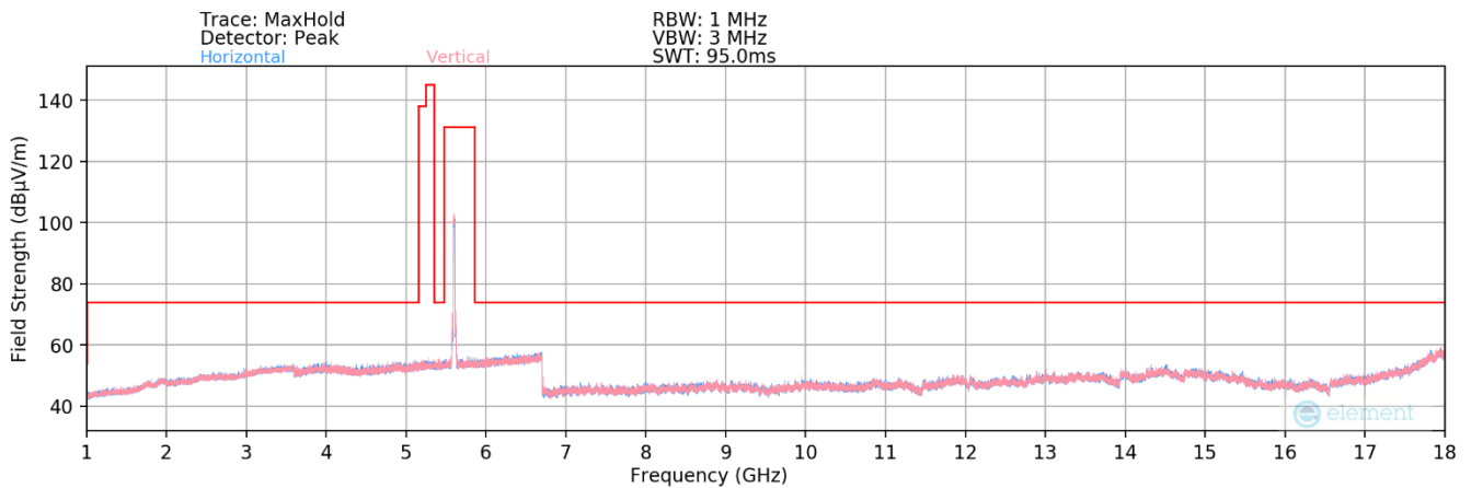
Plot 7-197. Radiated Spurious Plot above 1GHz MIMO (802.11be – UNII 2C Ch. 120)
