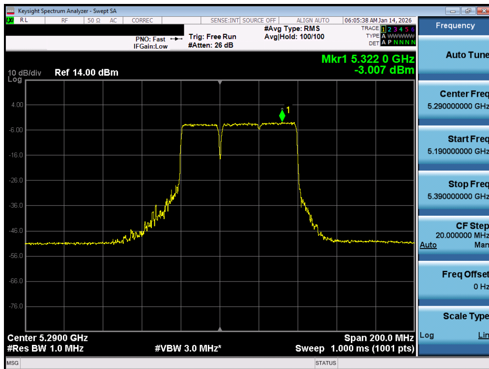
Plot 7-122. Power Spectral Density Plot MIMO ANT1 (80MHz BW 802.11be – 484+242Tones (UNII Band 2A) – Ch. 58)
