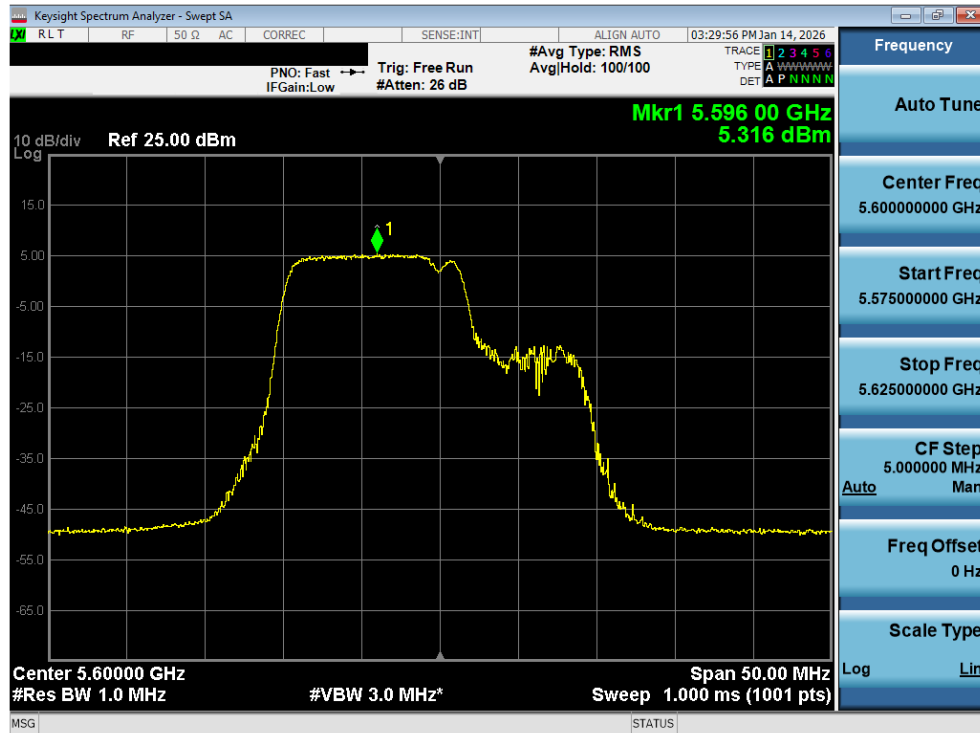
Plot 7-178. Power Spectral Density Plot MIMO ANT2 (20MHz BW 802.11be – 106+26 Tones (UNII Band 2C) – Ch. 120)
