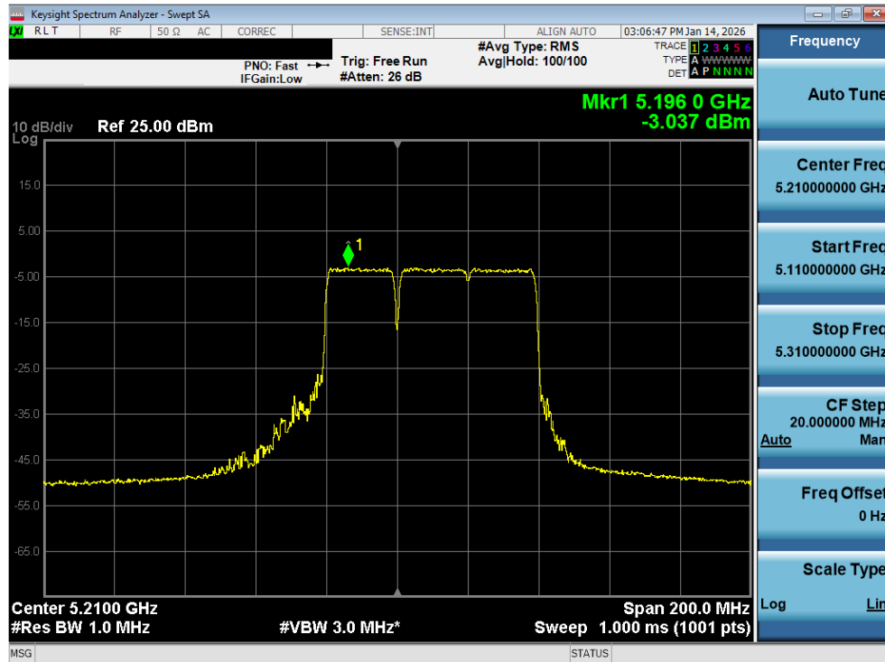
Plot 7-172. Power Spectral Density Plot MIMO ANT2 (80MHz BW 802.11be – 484+242Tones (UNII Band 1) – Ch. 42)
