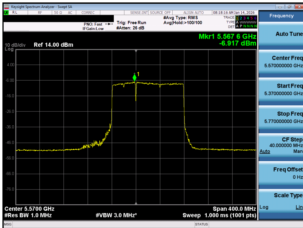
Plot 7-126. Power Spectral Density Plot MIMO ANT1 (160MHz BW 802.11be – 996+484 Tones (UNII Band 2C) – Ch. 114)
