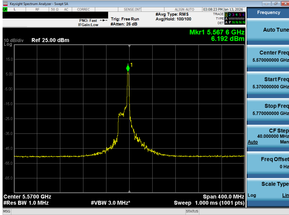
Plot 7-144. Power Spectral Density Plot MIMO ANT2 (160MHz BW 802.11be – 26 Tones (UNII Band 2C) – Ch. 114)
