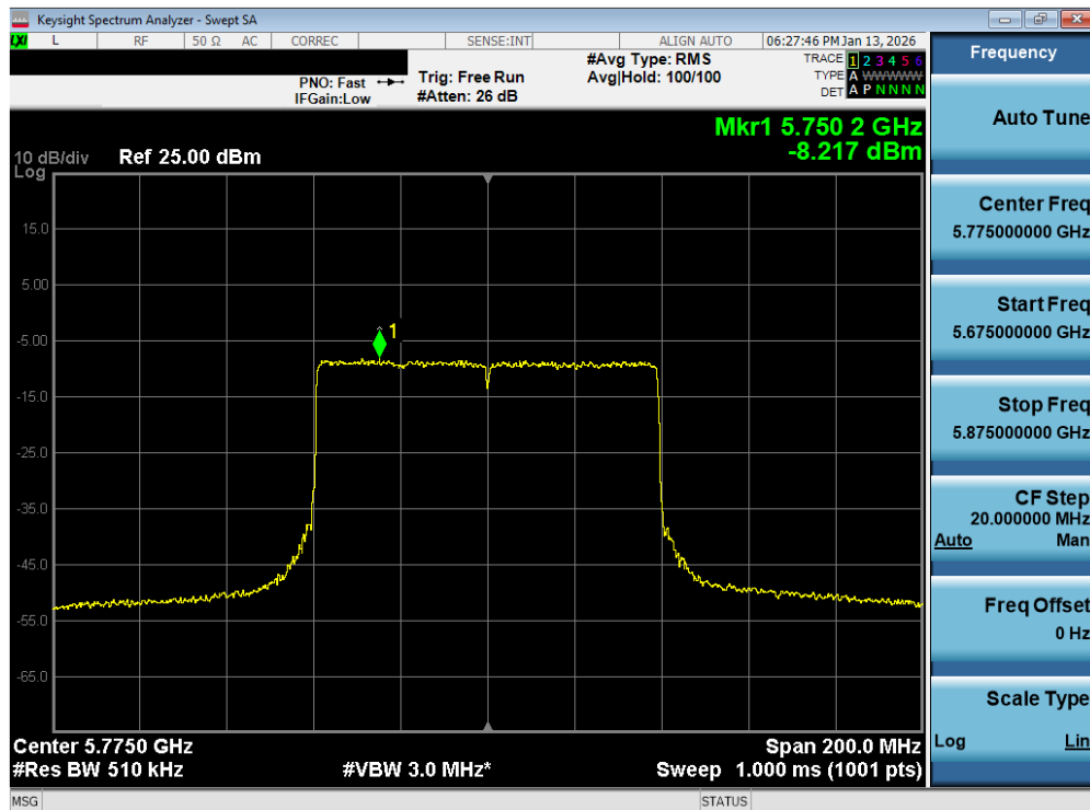
Plot 7-165. Power Spectral Density Plot MIMO ANT2 (80MHz BW 802.11be – 996 Tones (UNII Band 3) – Ch. 155)
