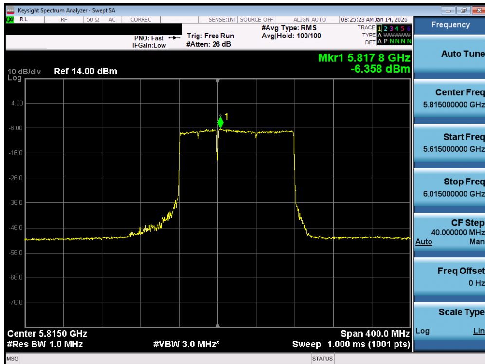
Plot 7-133. Power Spectral Density Plot MIMO ANT1 (160MHz BW 802.11be – 996+484 Tones (UNII Band 3/4) – Ch. 163)
