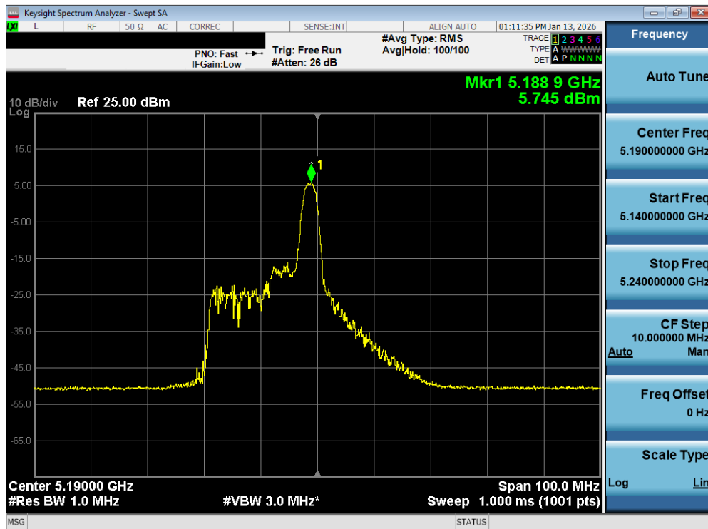
Plot 7-135. Power Spectral Density Plot MIMO ANT2 (40MHz BW 802.11be – 26 Tones (UNII Band 1) – Ch. 38)
