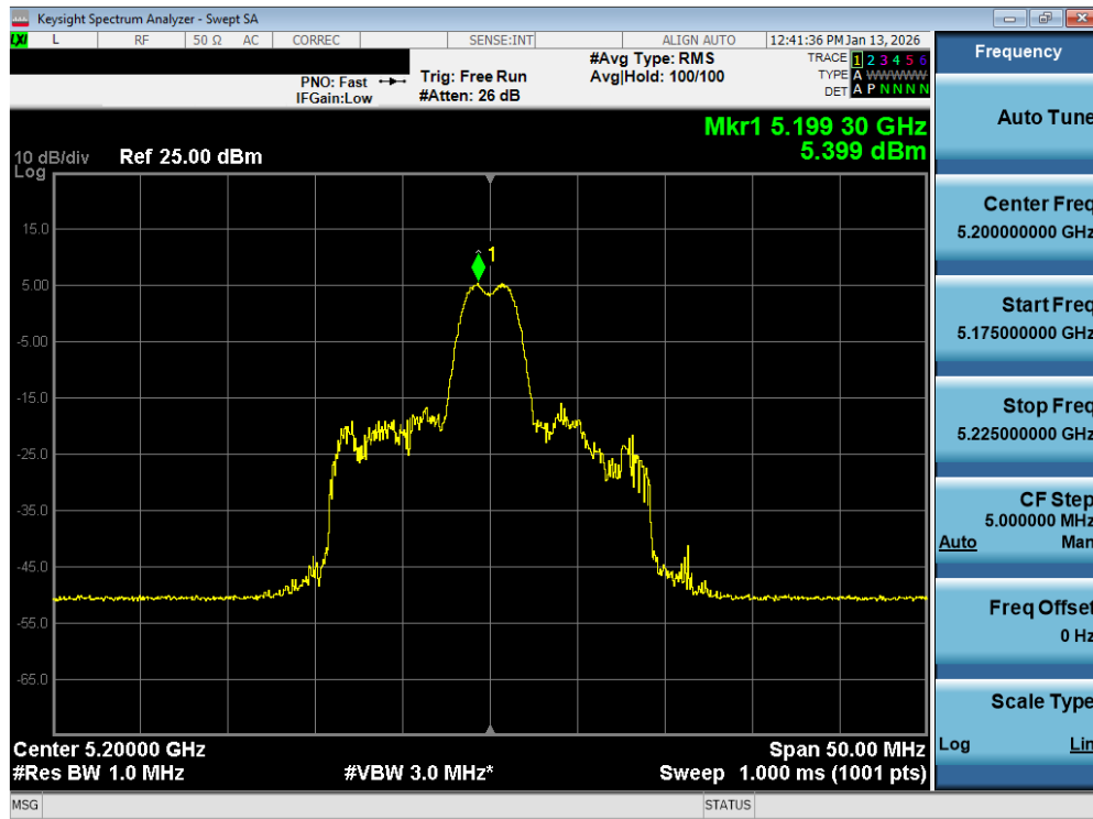
Plot 7-134. Power Spectral Density Plot MIMO ANT2 (20MHz BW 802.11be – 26 Tones (UNII Band 1) – Ch. 40)
