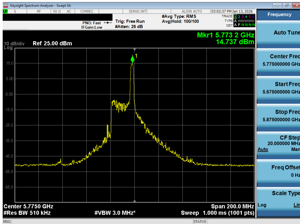
Plot 7-147. Power Spectral Density Plot MIMO ANT2 (80MHz BW 802.11be – 26 Tones (UNII Band 3) – Ch. 155)
