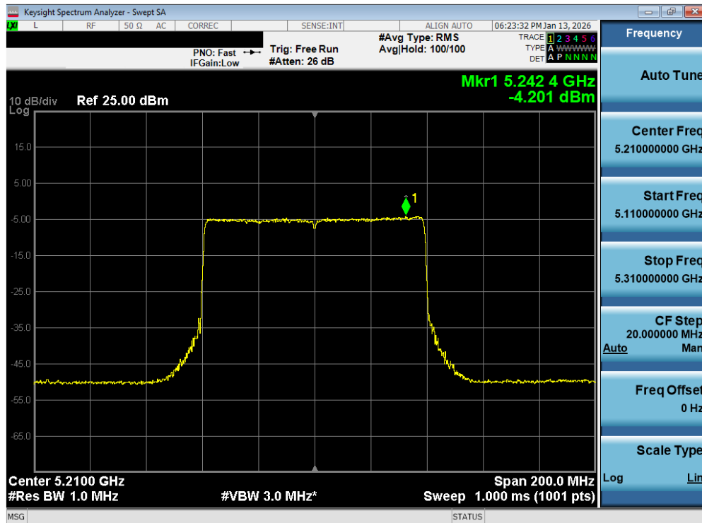
Plot 7-154. Power Spectral Density Plot MIMO ANT2 (80MHz BW 802.11be – 996 Tones (UNII Band 1) – Ch. 42)
