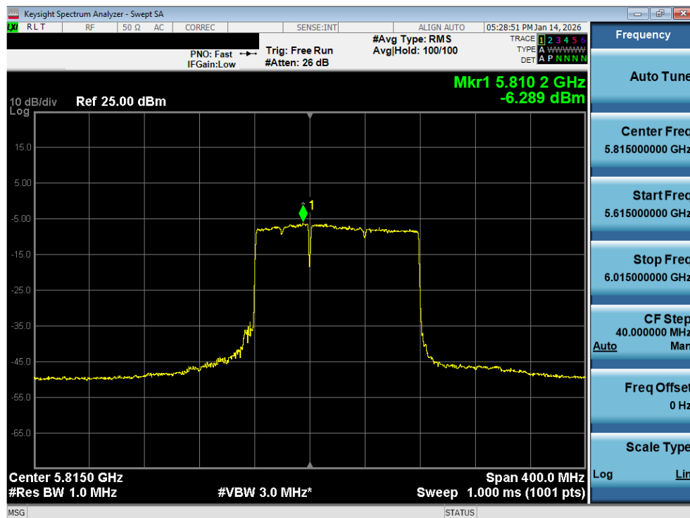
Plot 7-187. Power Spectral Density Plot MIMO ANT2 (160MHz BW 802.11be – 996+484 Tones (UNII Band 3/4) – Ch. 163)
