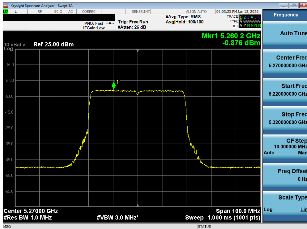
Plot 7-157. Power Spectral Density Plot MIMO ANT2 (40MHz BW 802.11be – 484 Tones (UNII Band 2A) – Ch. 54)
