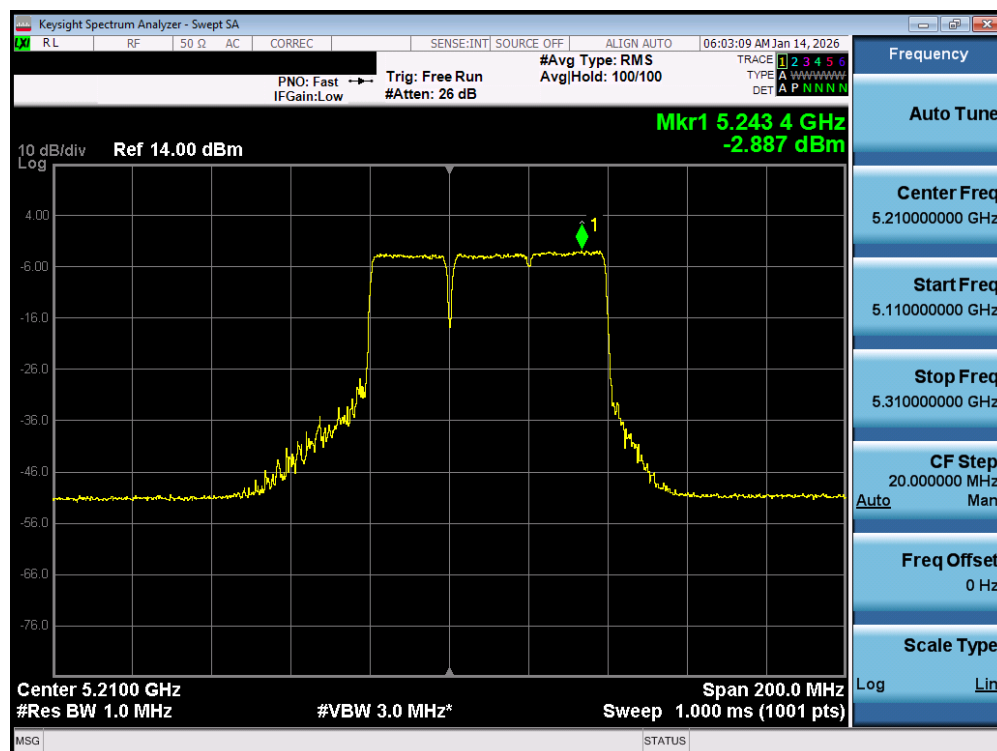
Plot 7-118. Power Spectral Density Plot MIMO ANT1 (80MHz BW 802.11be – 484+242Tones (UNII Band 1) – Ch. 42)
