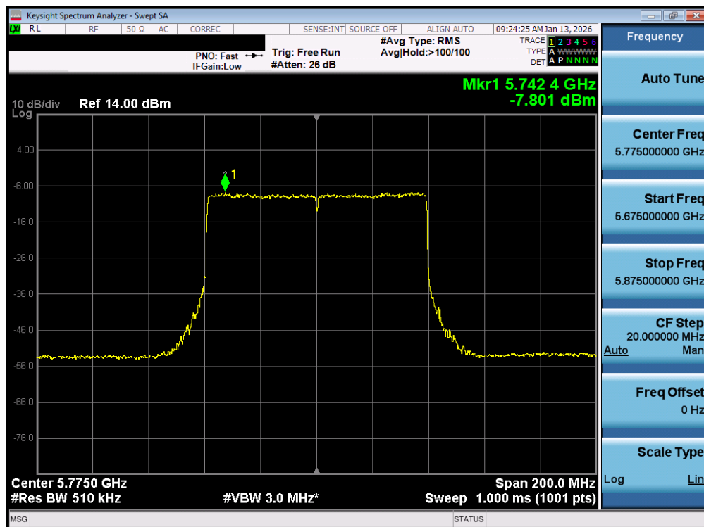
Plot 7-111. Power Spectral Density Plot MIMO ANT1 (80MHz BW 802.11be – 996 Tones (UNII Band 3) – Ch. 155)
