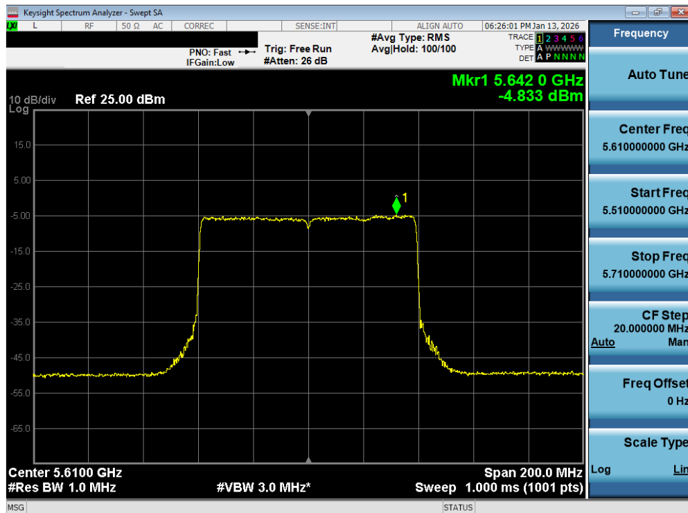
Plot 7-161. Power Spectral Density Plot MIMO ANT2 (80MHz BW 802.11be – 996 Tones (UNII Band 2C) – Ch. 122)
