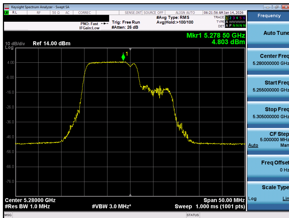
Plot 7-121. Power Spectral Density Plot MIMO ANT1 (20MHz BW 802.11be – 106+26 Tones (UNII Band 2A) – Ch. 56)
