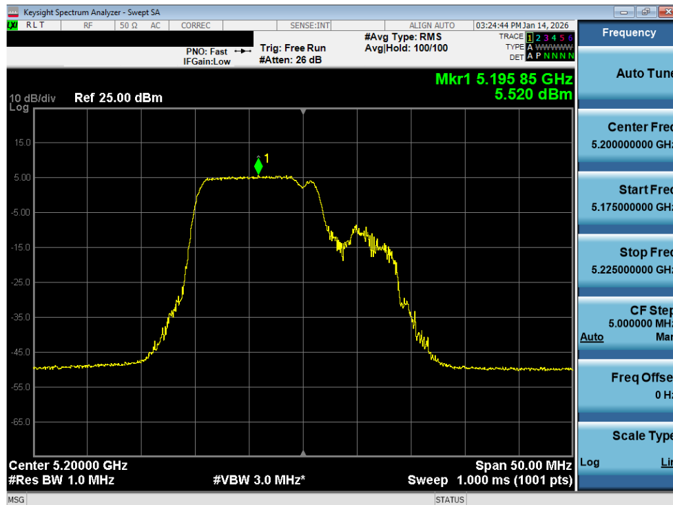
Plot 7-171. Power Spectral Density Plot MIMO ANT2 (20MHz BW 802.11be – 106+26 Tones (UNII Band 1) – Ch. 40)
