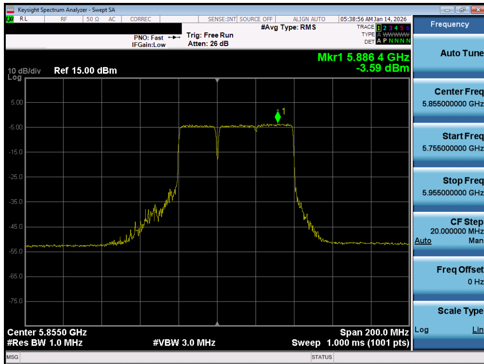
Plot 7-132. Power Spectral Density Plot MIMO ANT1 (80MHz BW 802.11be – 484+242Tones (UNII Band 3/4) – Ch. 171)
