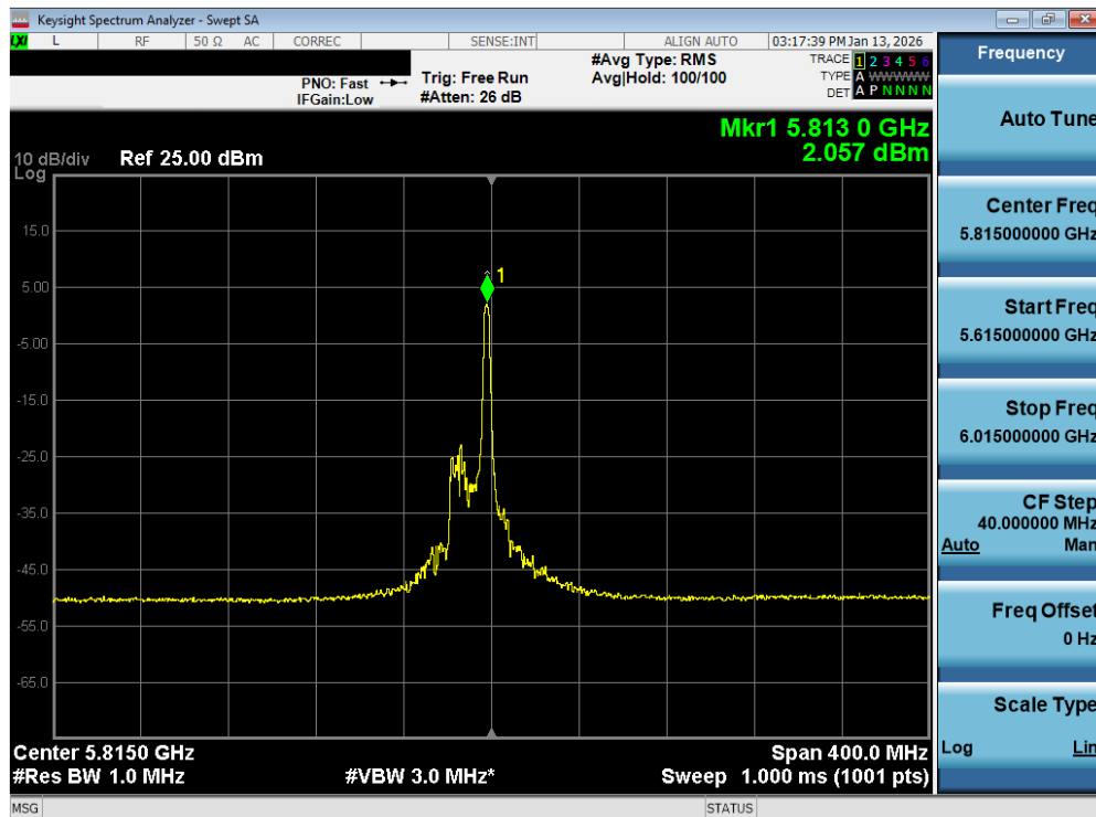
Plot 7-151. Power Spectral Density Plot MIMO ANT2 (160MHz(U) BW 802.11be – 26 Tones (UNII Band 3/4) – Ch. 163)
