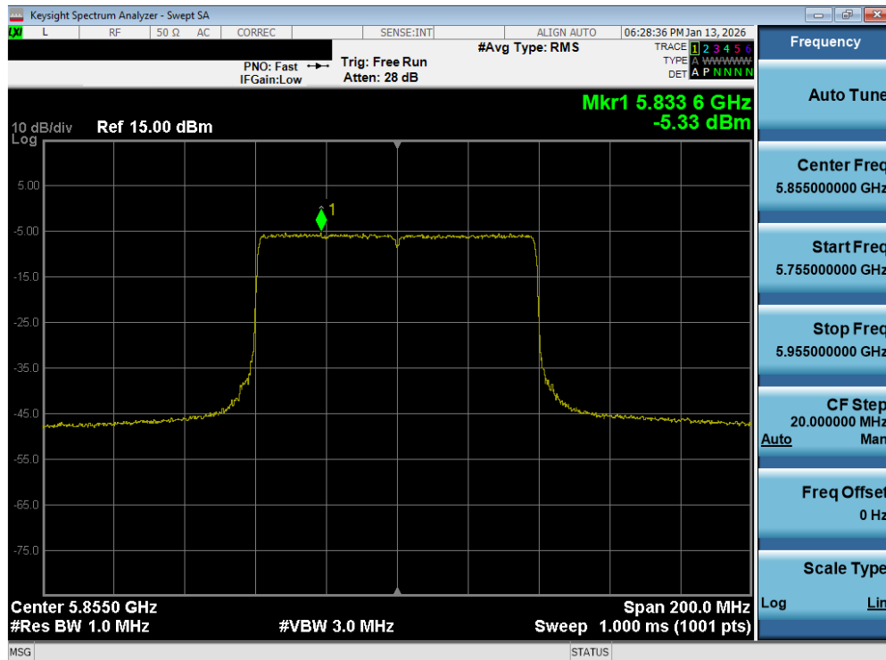
Plot 7-168. Power Spectral Density Plot MIMO ANT2 (80MHz BW 802.11be – 996 Tones (UNII Band 3/4) – Ch. 171)
