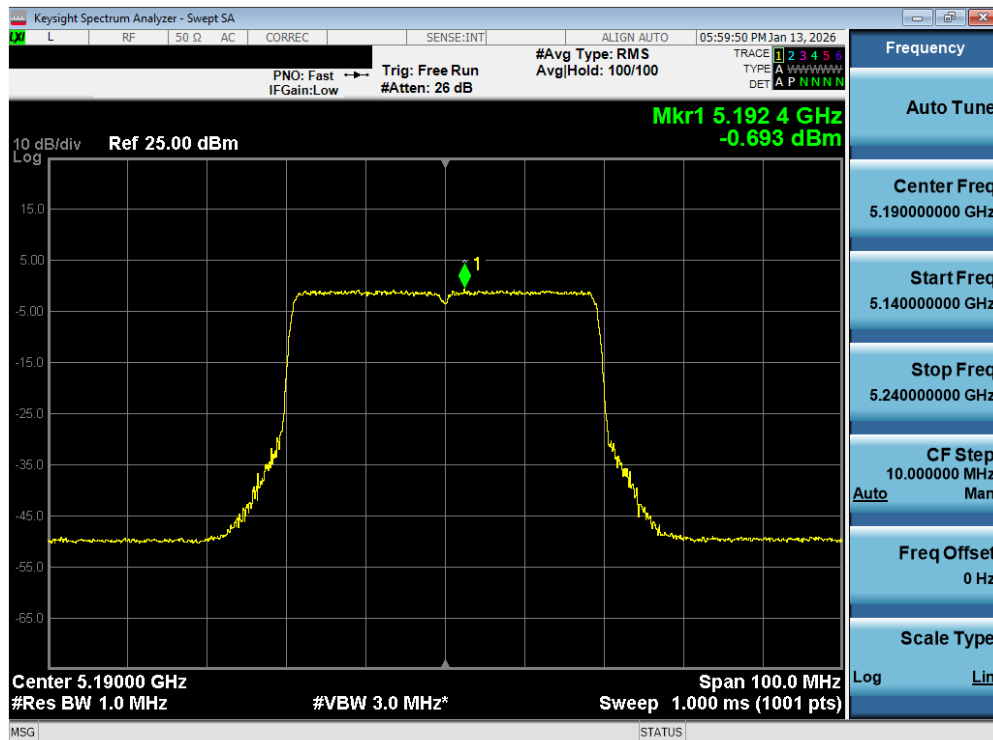
Plot 7-153. Power Spectral Density Plot MIMO ANT2 (40MHz BW 802.11be – 484 Tones (UNII Band 1) – Ch. 38)
