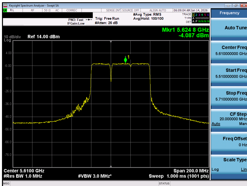
Plot 7-125. Power Spectral Density Plot MIMO ANT1 (80MHz BW 802.11be – 484+242Tones (UNII Band 2C) – Ch. 122)
