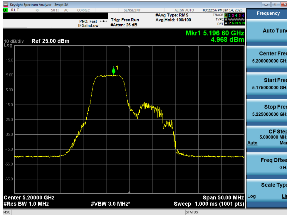
Plot 7-170. Power Spectral Density Plot MIMO ANT2 (20MHz BW 802.11be – 52+26 Tones (UNII Band 1) – Ch. 40)
