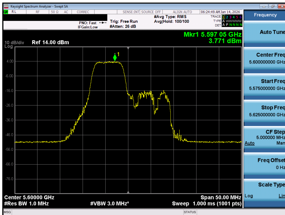
Plot 7-123. Power Spectral Density Plot MIMO ANT1 (20MHz BW 802.11be – 52+26 Tones (UNII Band 2C) – Ch. 120)
