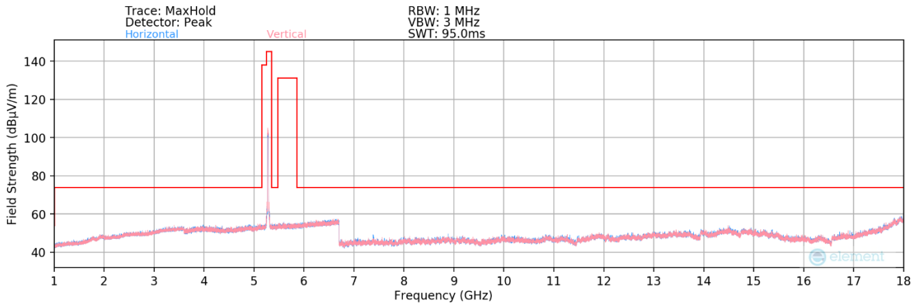
Plot 7-196. Radiated Spurious Plot above 1GHz MIMO (802.11be – UNII 2A Ch. 56)
