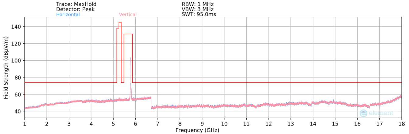
Plot 7-198. Radiated Spurious Plot above 1GHz MIMO (802.11be – UNII 3 Ch. 157)
