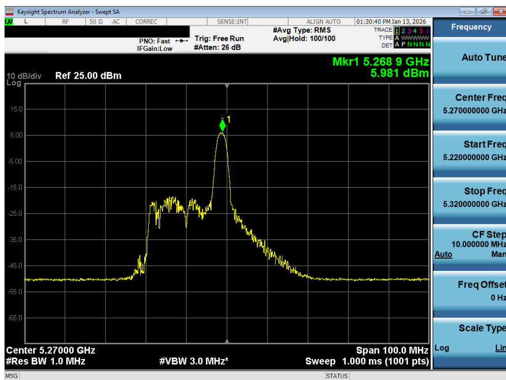
Plot 7-139. Power Spectral Density Plot MIMO ANT2 (40MHz BW 802.11be – 26 Tones (UNII Band 2A) – Ch. 54)
