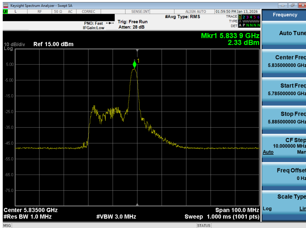
Plot 7-149. Power Spectral Density Plot MIMO ANT2 (40MHz BW 802.11be – 26 Tones (UNII Band 3/4) – Ch. 167)
