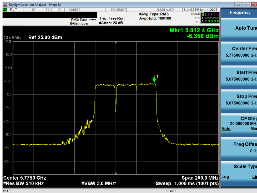
Plot 7-183. Power Spectral Density Plot MIMO ANT2 (80MHz BW 802.11be – 484+242Tones (UNII Band 3) – Ch. 155)
