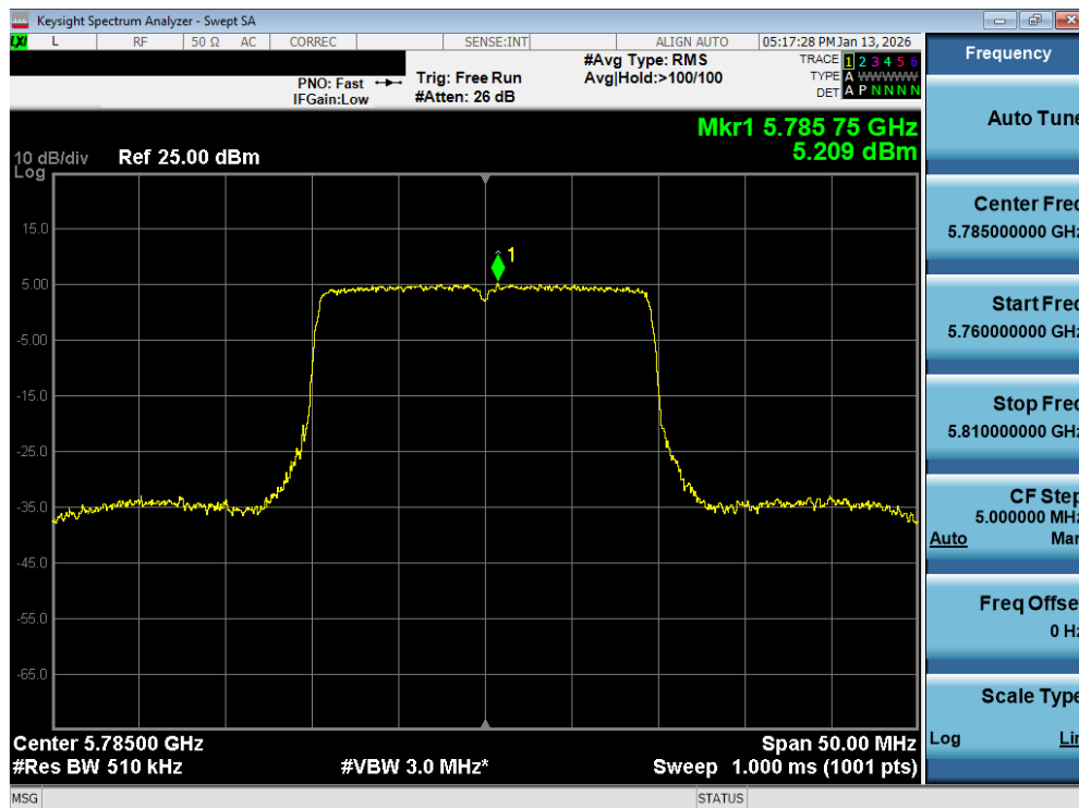
Plot 7-163. Power Spectral Density Plot MIMO ANT2 (20MHz BW 802.11be – 242 Tones (UNII Band 3) – Ch. 157)
