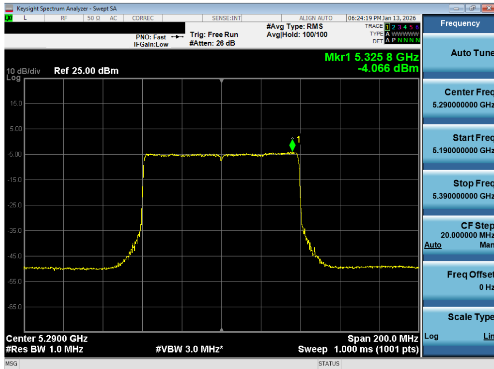
Plot 7-158. Power Spectral Density Plot MIMO ANT2 (80MHz BW 802.11be – 996 Tones (UNII Band 2A) – Ch. 58)
