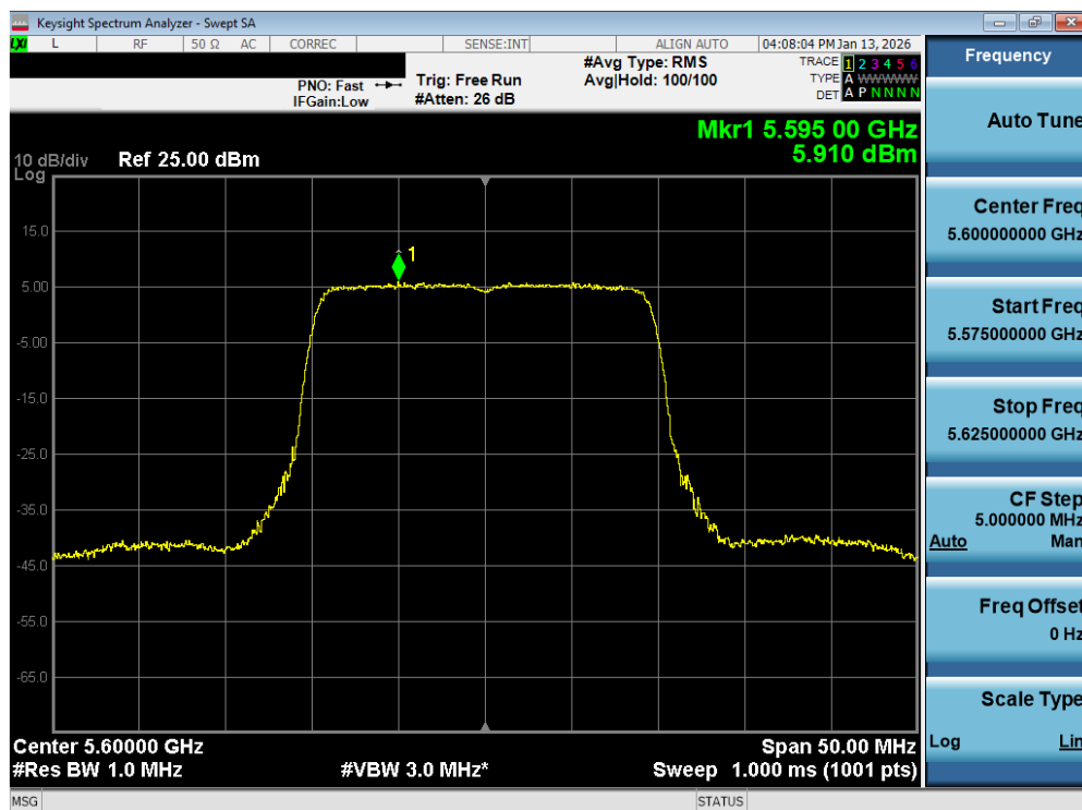
Plot 7-159. Power Spectral Density Plot MIMO ANT2 (20MHz BW 802.11be – 242 Tones (UNII Band 2C) – Ch. 120)
