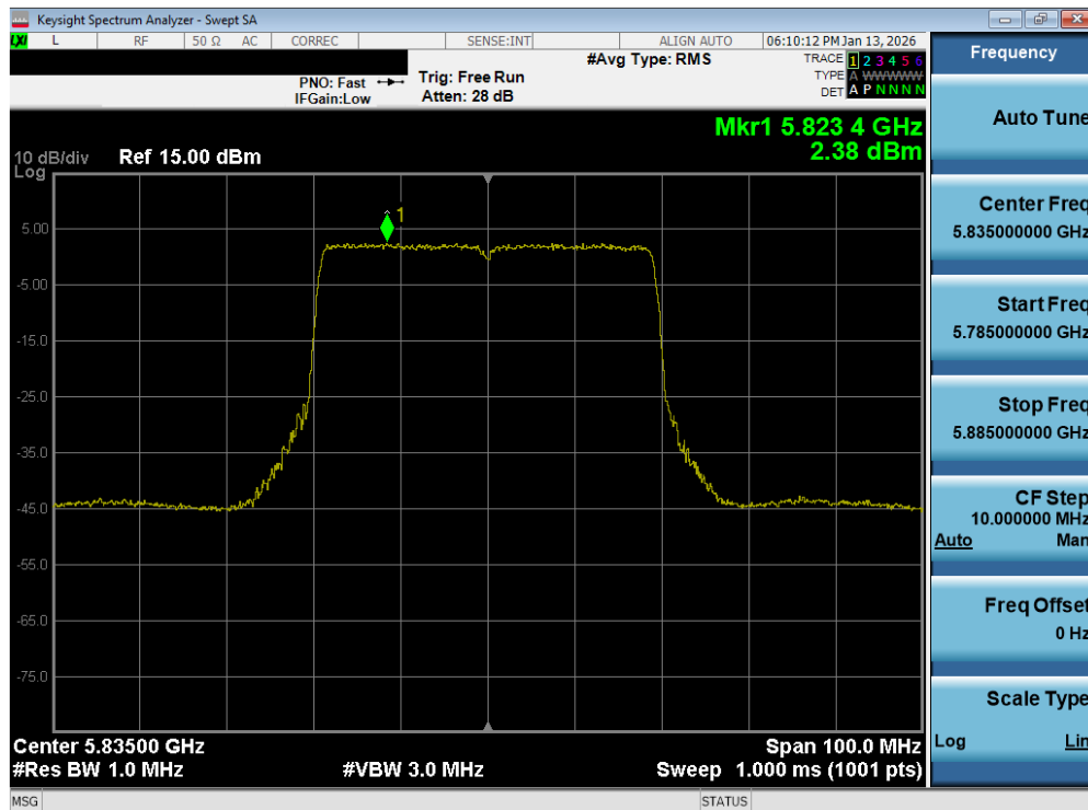
Plot 7-167. Power Spectral Density Plot MIMO ANT2 (40MHz BW 802.11be – 484 Tones (UNII Band 3/4) – Ch. 167)
