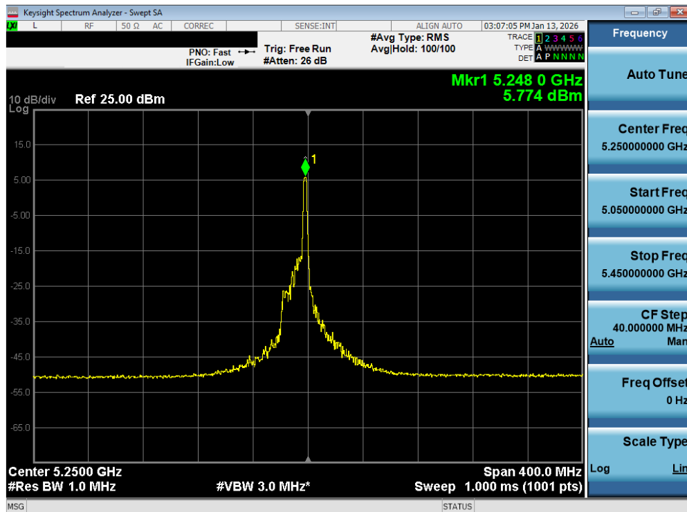
Plot 7-137. Power Spectral Density Plot MIMO ANT2 (160MHz BW 802.11be – 26 Tones (UNII Band 1/2A) – Ch. 50)
