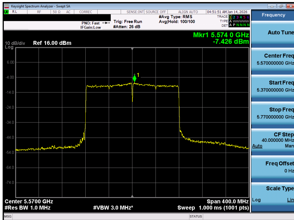
Plot 7-108. Power Spectral Density Plot MIMO ANT1 (160MHz BW 802.11be – 2x996 Tones (UNII Band 2C) – Ch. 114)
