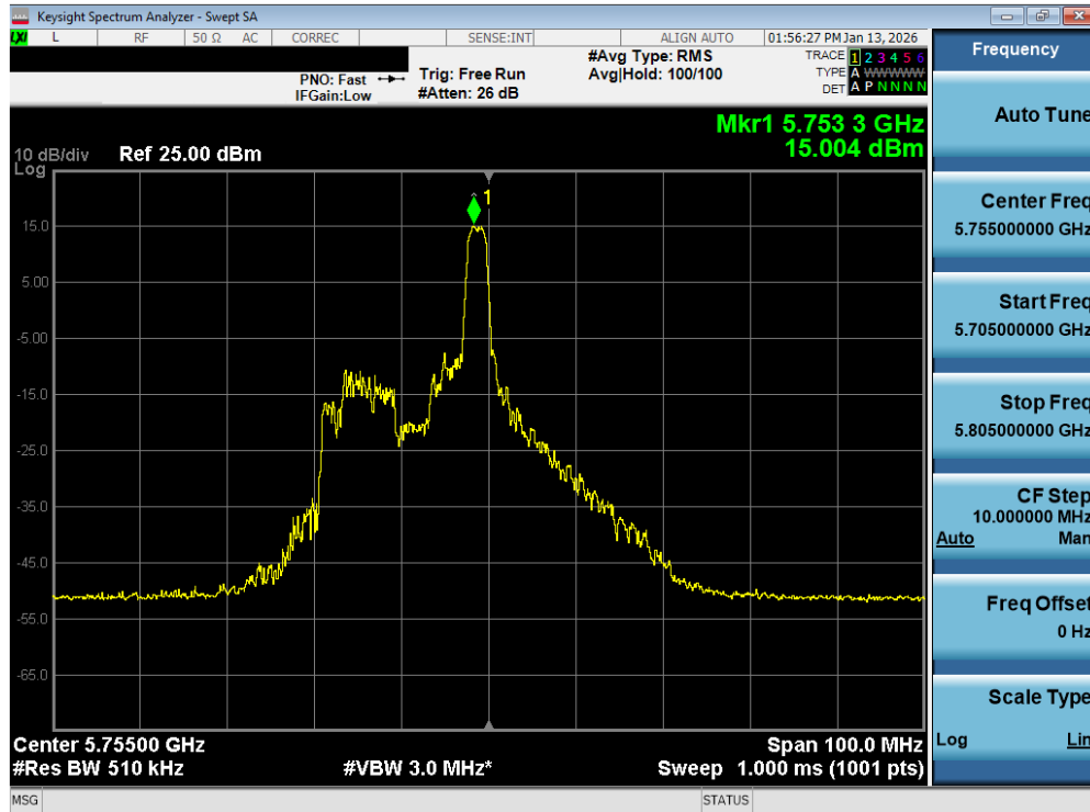
Plot 7-146. Power Spectral Density Plot MIMO ANT2 (40MHz BW 802.11be – 26 Tones (UNII Band 3) – Ch. 151)
