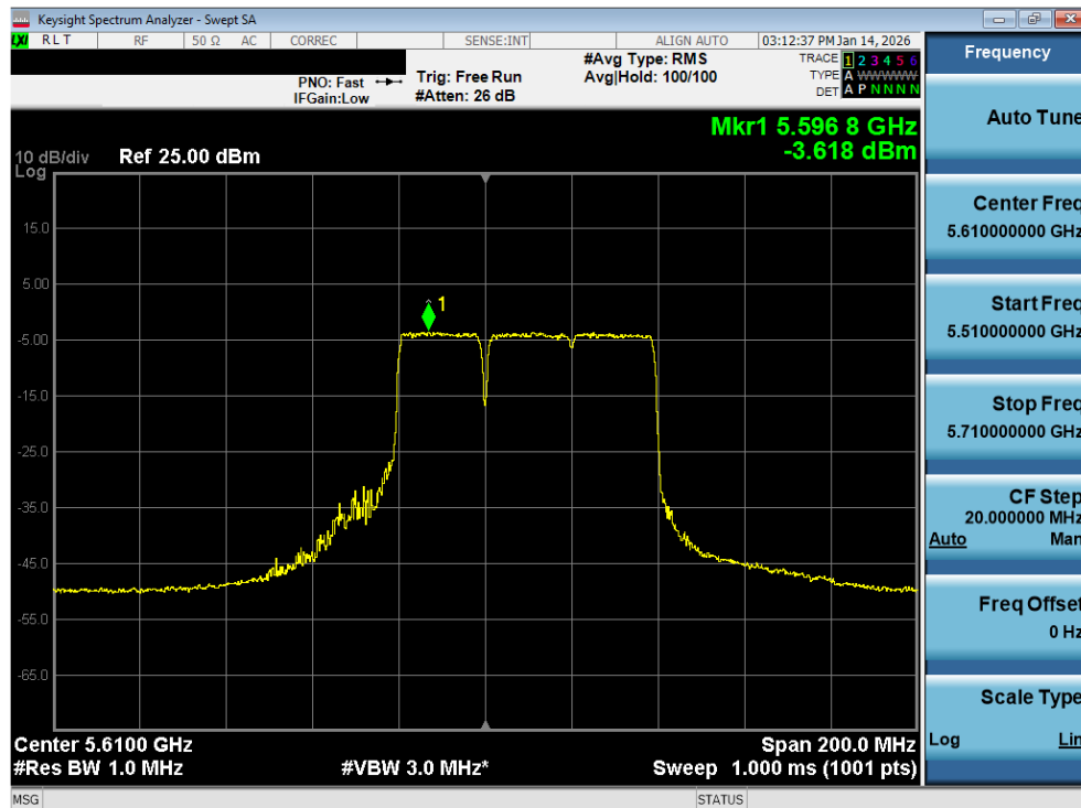
Plot 7-179. Power Spectral Density Plot MIMO ANT2 (80MHz BW 802.11be – 484+242Tones (UNII Band 2C) – Ch. 122)
