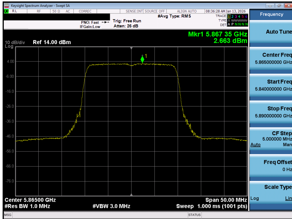
Plot 7-112. Power Spectral Density Plot MIMO ANT1 (20MHz BW 802.11be – 242 Tones (UNII Band 4) – Ch. 173)
