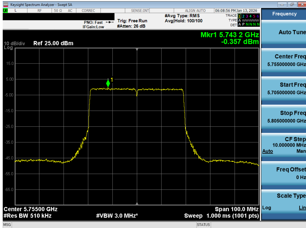
Plot 7-164. Power Spectral Density Plot MIMO ANT2 (40MHz BW 802.11be – 484 Tones (UNII Band 3) – Ch. 151)
