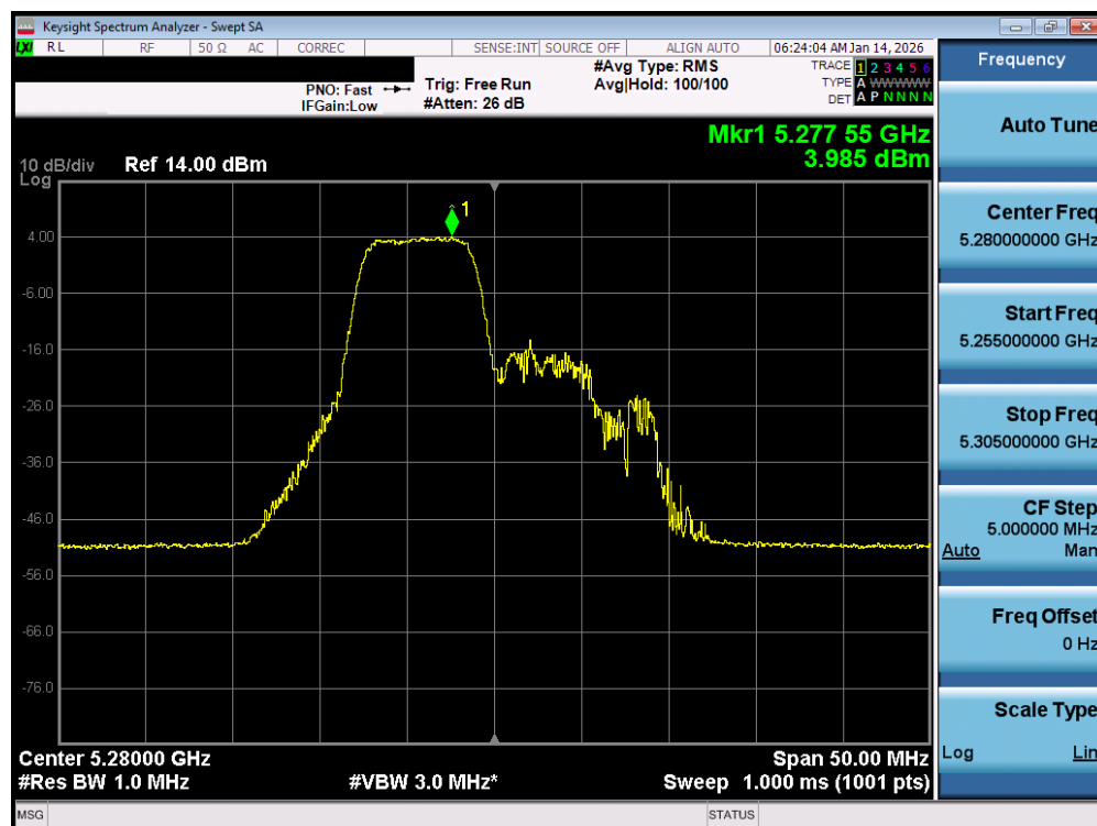
Plot 7-120. Power Spectral Density Plot MIMO ANT1 (20MHz BW 802.11be – 52+26 Tones (UNII Band 2A) – Ch. 56)
