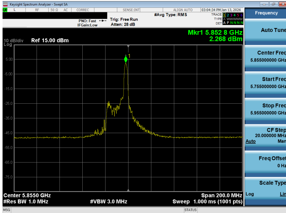
Plot 7-150. Power Spectral Density Plot MIMO ANT2 (80MHz BW 802.11be – 26 Tones (UNII Band 3/4) – Ch. 171)
