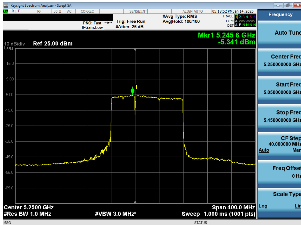
Plot 7-173. Power Spectral Density Plot MIMO ANT2 (160MHz BW 802.11be – 996+484 Tones (UNII Band 1/2A) – Ch. 50)
