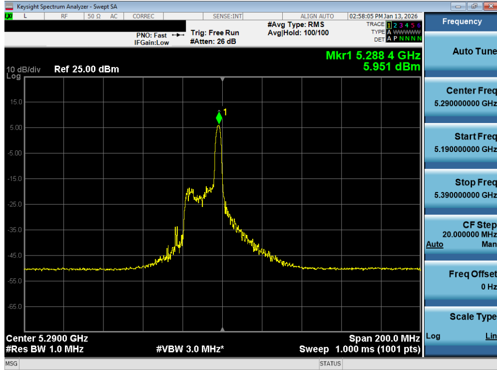
Plot 7-140. Power Spectral Density Plot MIMO ANT2 (80MHz BW 802.11be – 26 Tones (UNII Band 2A) – Ch. 58)
