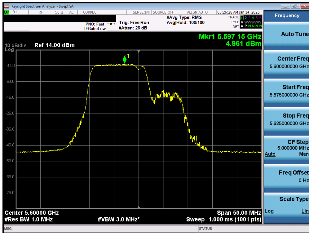
Plot 7-124. Power Spectral Density Plot MIMO ANT1 (20MHz BW 802.11be – 106+26 Tones (UNII Band 2C) – Ch. 120)
