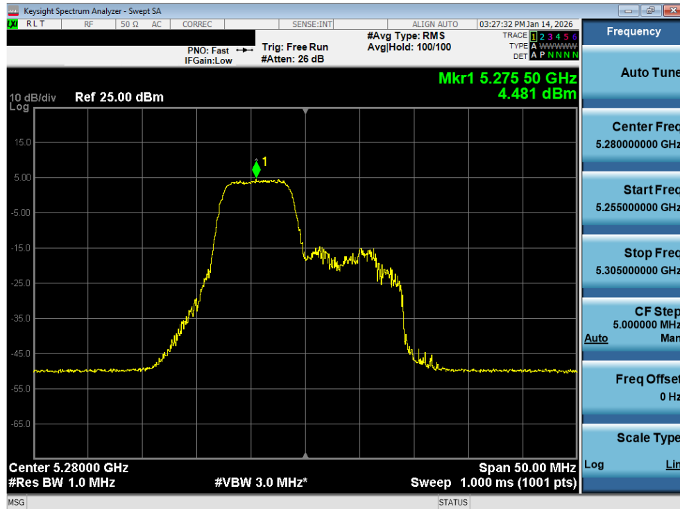
Plot 7-174. Power Spectral Density Plot MIMO ANT2 (20MHz BW 802.11be – 52+26 Tones (UNII Band 2A) – Ch. 56)
