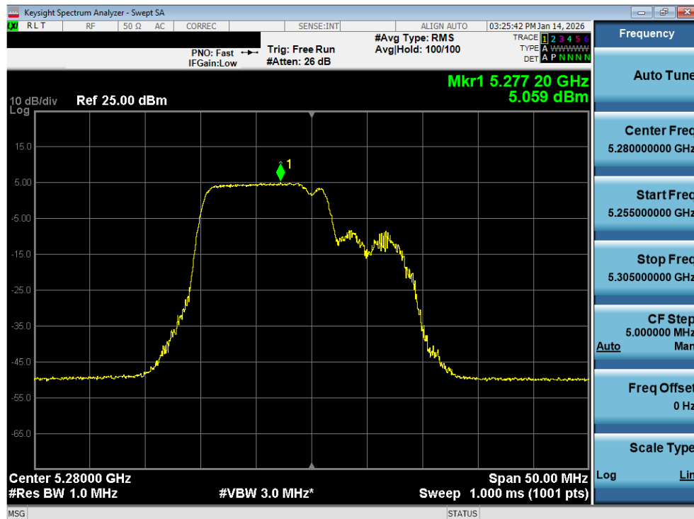
Plot 7-175. Power Spectral Density Plot MIMO ANT2 (20MHz BW 802.11be – 106+26 Tones (UNII Band 2A) – Ch. 56)
