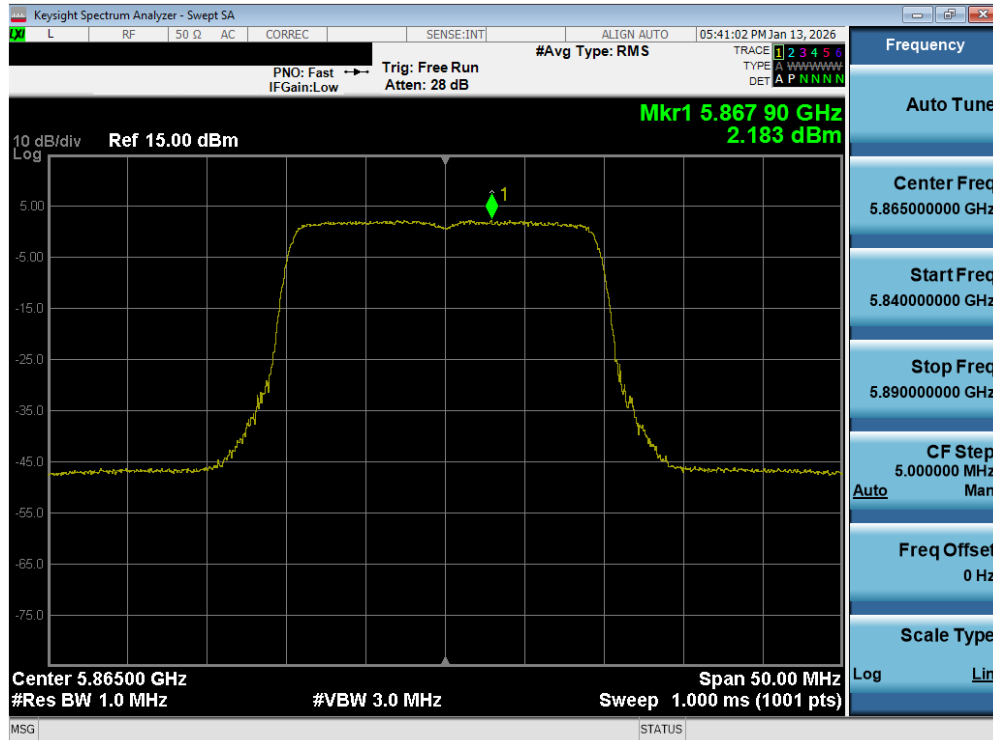
Plot 7-166. Power Spectral Density Plot MIMO ANT2 (20MHz BW 802.11be – 242 Tones (UNII Band 4) – Ch. 173)
