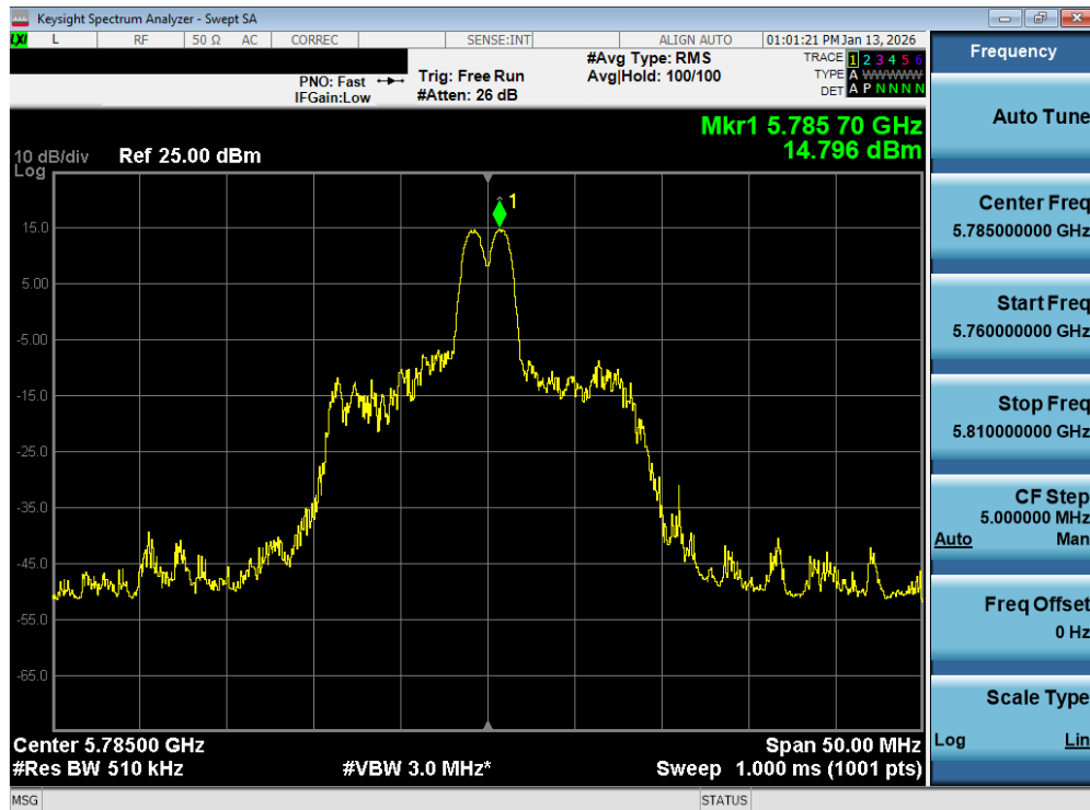
Plot 7-145. Power Spectral Density Plot MIMO ANT2 (20MHz BW 802.11be – 26 Tones (UNII Band 3) – Ch. 157)
