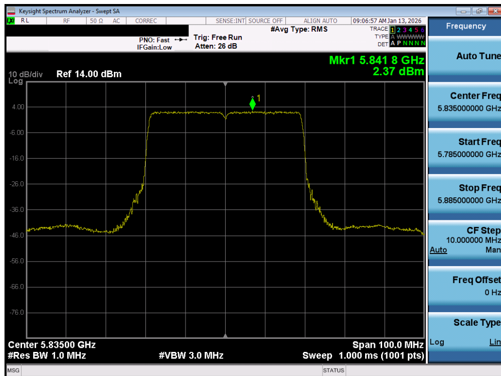
Plot 7-113. Power Spectral Density Plot MIMO ANT1 (40MHz BW 802.11be – 484 Tones (UNII Band 3/4) – Ch. 167)
