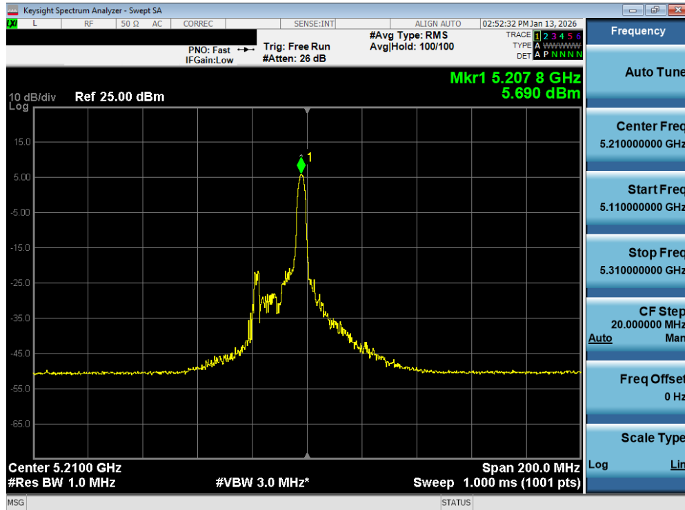
Plot 7-136. Power Spectral Density Plot MIMO ANT2 (80MHz BW 802.11be – 26 Tones (UNII Band 1) – Ch. 42)
