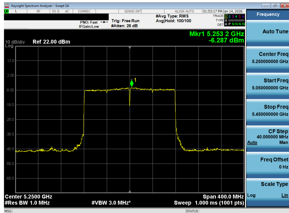
Plot 7-155. Power Spectral Density Plot MIMO ANT2 (160MHz BW 802.11be – 2x996 Tones (UNII Band 1/2A) – Ch. 50)
