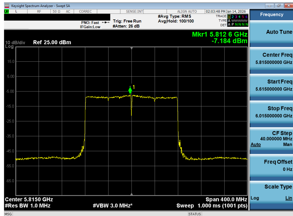
Plot 7-169. Power Spectral Density Plot MIMO ANT2 (160MHz BW 802.11be – 996*2 Tones (UNII Band 3/4) – Ch. 163)
