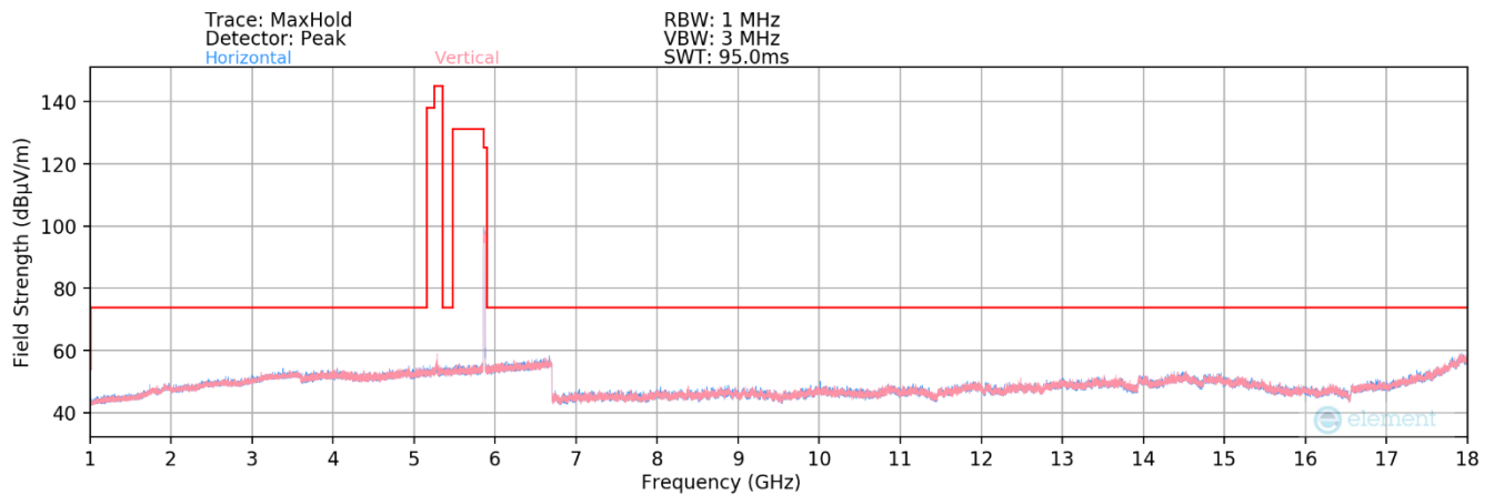
Plot 7-199. Radiated Spurious Plot above 1GHz MIMO (802.11be – UNII 4 Ch. 173)
