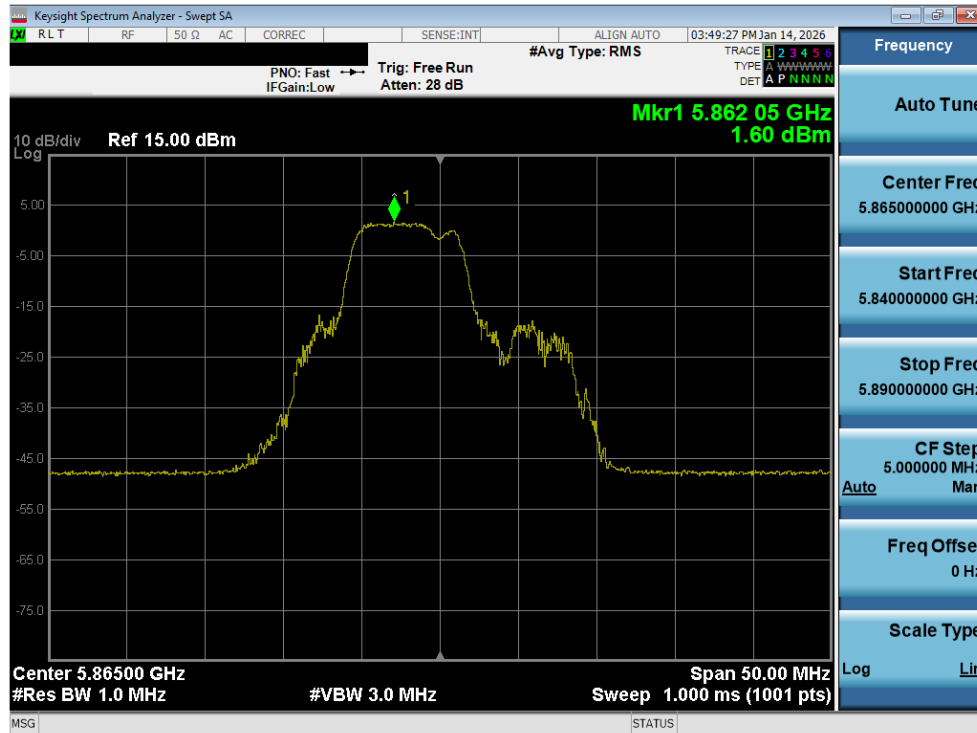
Plot 7-184. Power Spectral Density Plot MIMO ANT2 (20MHz BW 802.11be – 52+26 Tones (UNII Band 4) – Ch. 173)
