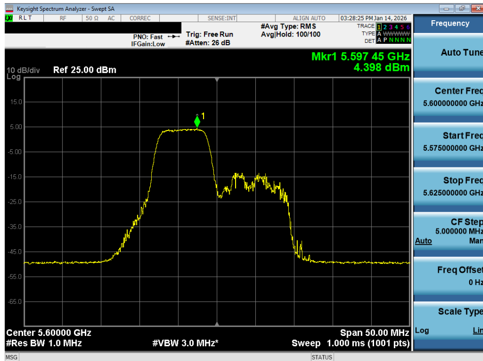
Plot 7-177. Power Spectral Density Plot MIMO ANT2 (20MHz BW 802.11be – 52+26 Tones (UNII Band 2C) – Ch. 120)
