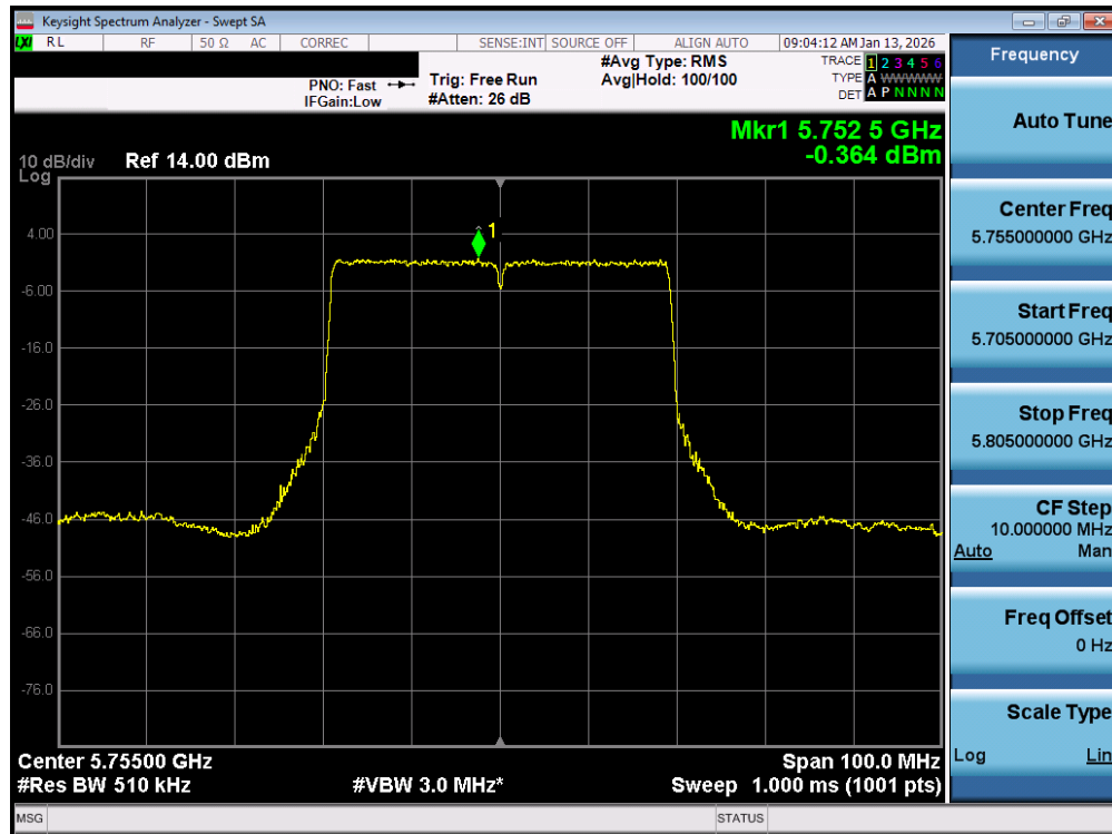
Plot 7-110. Power Spectral Density Plot MIMO ANT1 (40MHz BW 802.11be – 484 Tones (UNII Band 3) – Ch. 151)
