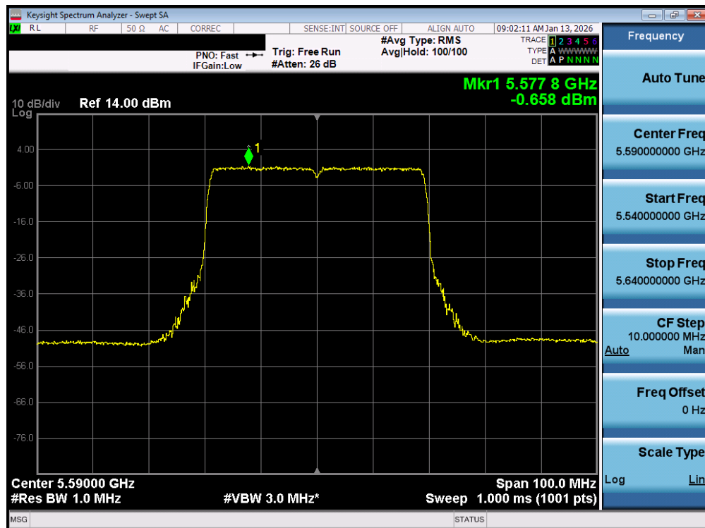
Plot 7-106. Power Spectral Density Plot MIMO ANT1 (40MHz BW 802.11be – 484 Tones (UNII Band 2C) – Ch. 118)
