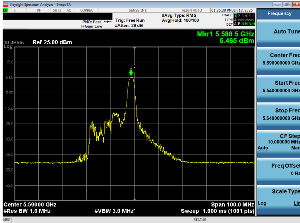
Plot 7-142. Power Spectral Density Plot MIMO ANT2 (40MHz BW 802.11be – 26 Tones (UNII Band 2C) – Ch. 118)
