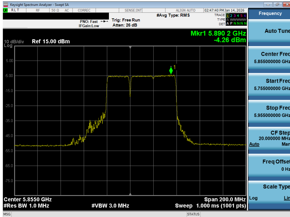
Plot 7-186. Power Spectral Density Plot MIMO ANT2 (80MHz BW 802.11be – 484+242Tones (UNII Band 3/4) – Ch. 171)
