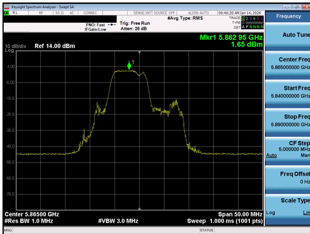
Plot 7-130. Power Spectral Density Plot MIMO ANT1 (20MHz BW 802.11be – 52+26 Tones (UNII Band 4) – Ch. 173)
