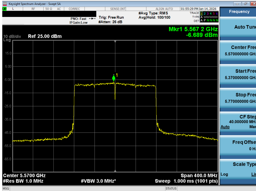
Plot 7-162. Power Spectral Density Plot MIMO ANT2 (160MHz BW 802.11be – 2x996 Tones (UNII Band 2C) – Ch. 114)
