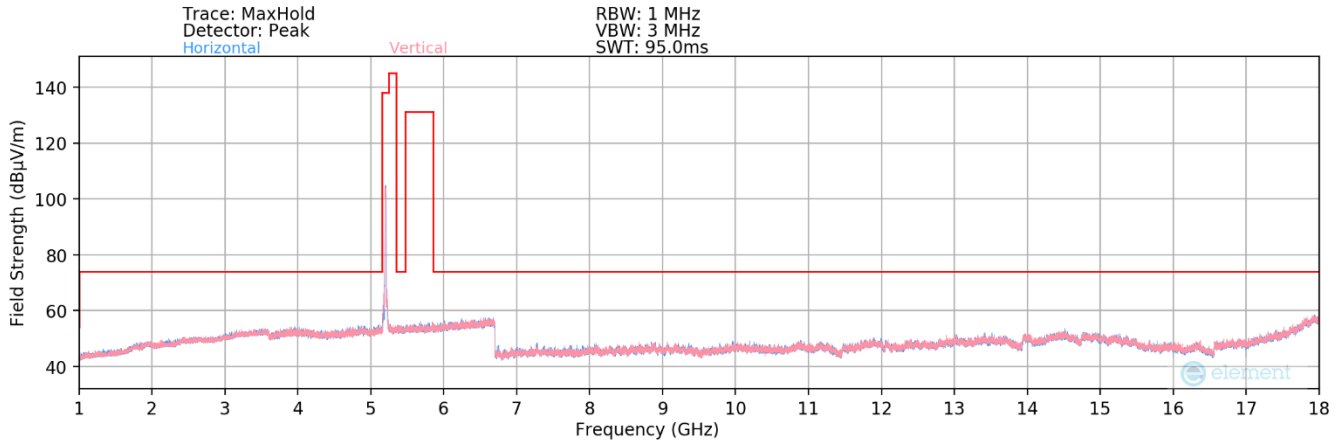
Plot 7-195. Radiated Spurious Plot above 1GHz MIMO (802.11be – UNII 1 Ch. 40)
