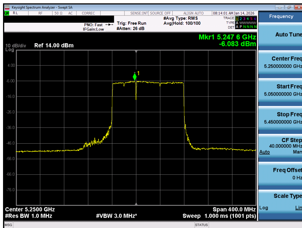
Plot 7-119. Power Spectral Density Plot MIMO ANT1 (160MHz BW 802.11be – 996+484 Tones (UNII Band 1/2A) – Ch. 50)
