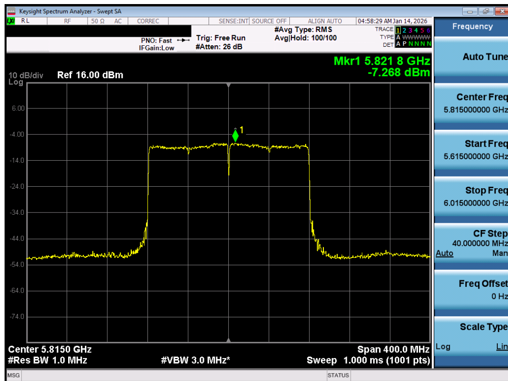
Plot 7-115. Power Spectral Density Plot MIMO ANT1 (160MHz BW 802.11be – 2x996 Tones (UNII Band 3/4) – Ch. 163)
