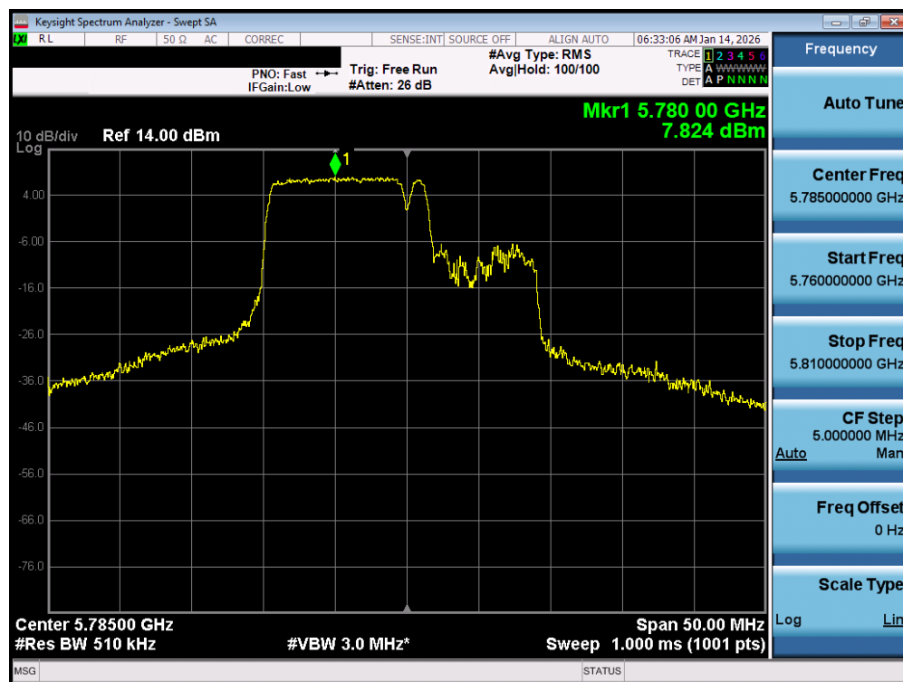
Plot 7-128. Power Spectral Density Plot MIMO ANT1 (20MHz BW 802.11be – 106+26 Tones (UNII Band 3) – Ch. 157)
