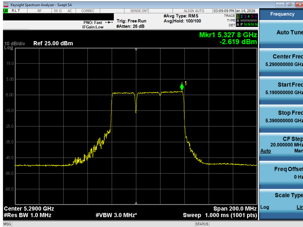
Plot 7-176. Power Spectral Density Plot MIMO ANT2 (80MHz BW 802.11be – 484+242Tones (UNII Band 2A) – Ch. 58)
