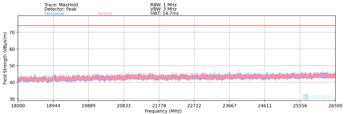
Plot 7-200. Radiated Spurious Plot 18GHz - 26.5GHz (802.11be)
