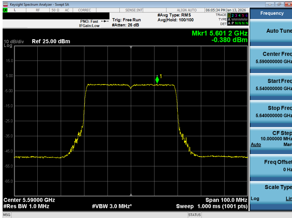
Plot 7-160. Power Spectral Density Plot MIMO ANT2 (40MHz BW 802.11be – 484 Tones (UNII Band 2C) – Ch. 118)
