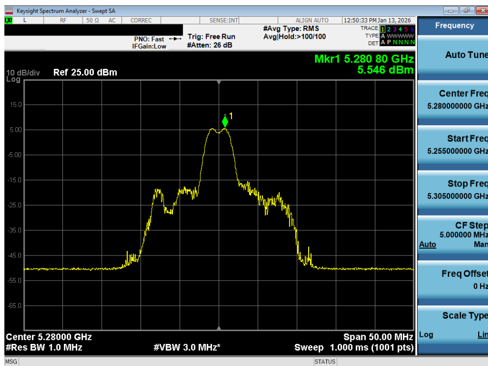
Plot 7-138. Power Spectral Density Plot MIMO ANT2 (20MHz BW 802.11be – 26 Tones (UNII Band 2A) – Ch. 56)
