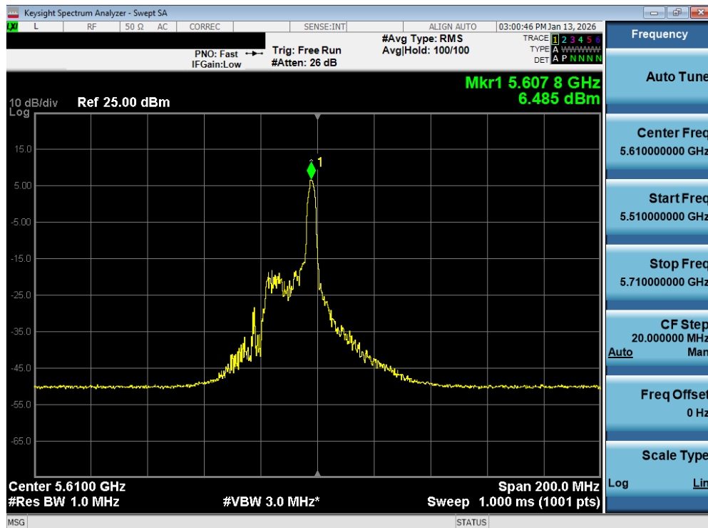
Plot 7-143. Power Spectral Density Plot MIMO ANT2 (80MHz BW 802.11be – 26 Tones (UNII Band 2C) – Ch. 122)
