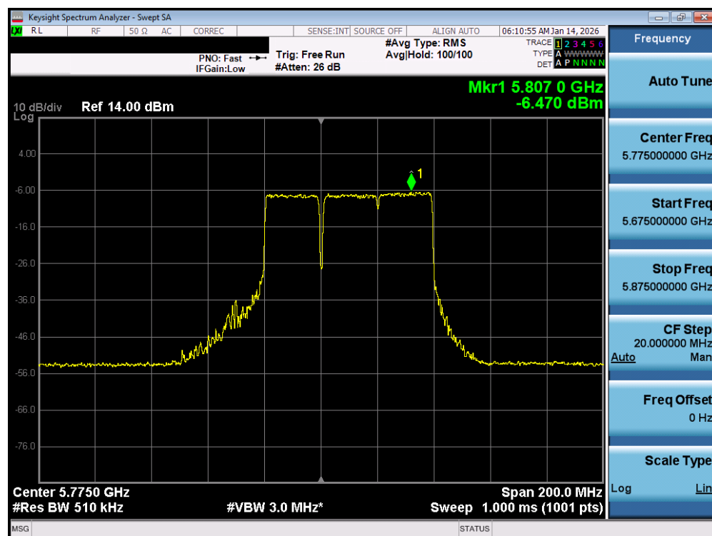
Plot 7-129. Power Spectral Density Plot MIMO ANT1 (80MHz BW 802.11be – 484+242Tones (UNII Band 3) – Ch. 155)
