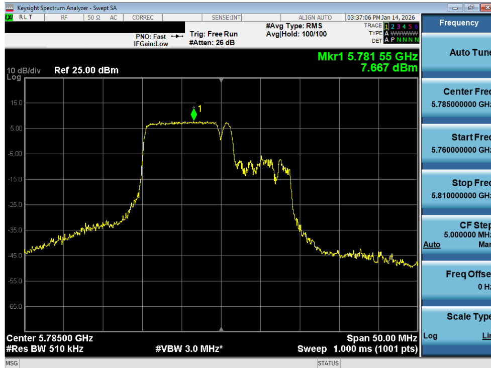
Plot 7-182. Power Spectral Density Plot MIMO ANT2 (20MHz BW 802.11be – 106+26 Tones (UNII Band 3) – Ch. 157)
