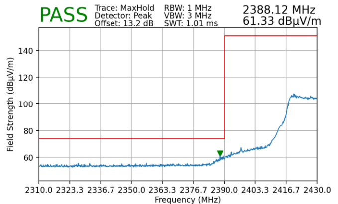
Plot 7-260. Radiated Restricted Lower Band Edge Measurement MIMO (Peak)
