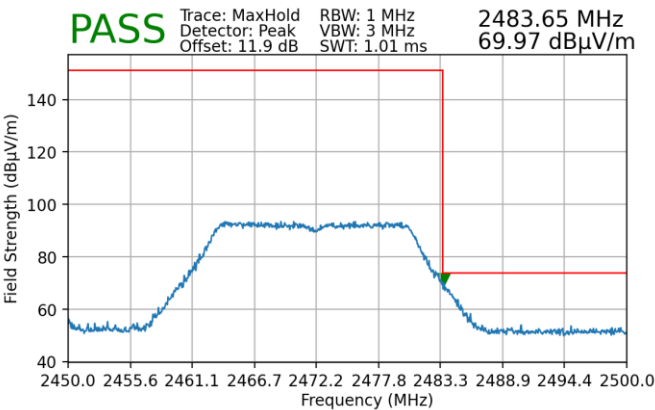
Plot 7-252. Radiated Restricted Upper Band Edge Measurement MIMO (Peak)
