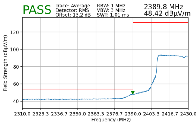
Plot 7-255. Radiated Restricted Lower Band Edge Measurement MIMO (Average)
