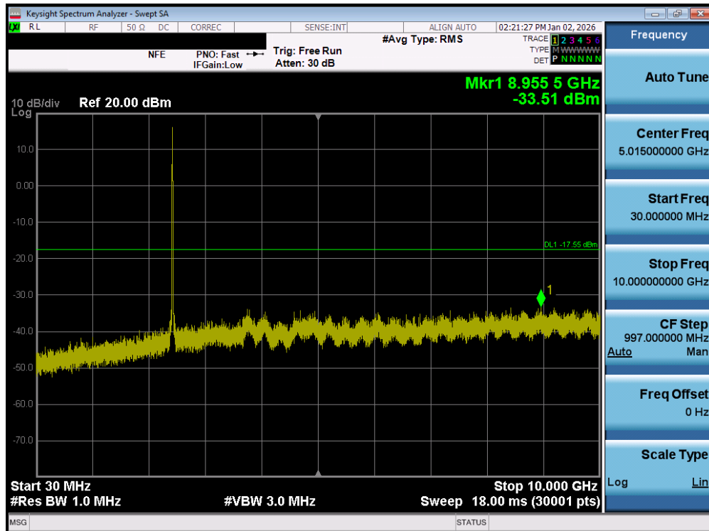
Plot 7-206. Conducted Spurious Plot MIMO ANT2 (802.11b – Ch. 6) – MIMO ANT2
