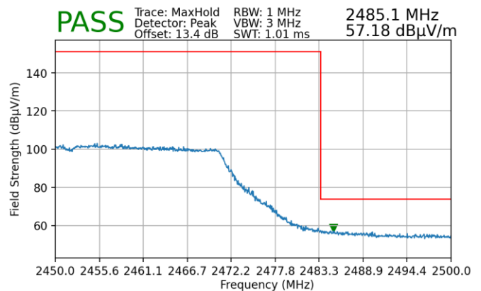
Plot 7-268. Radiated Restricted Upper Band Edge Measurement MIMO (Peak)
