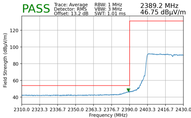
Plot 7-253. Radiated Restricted Lower Band Edge Measurement MIMO (Average)
