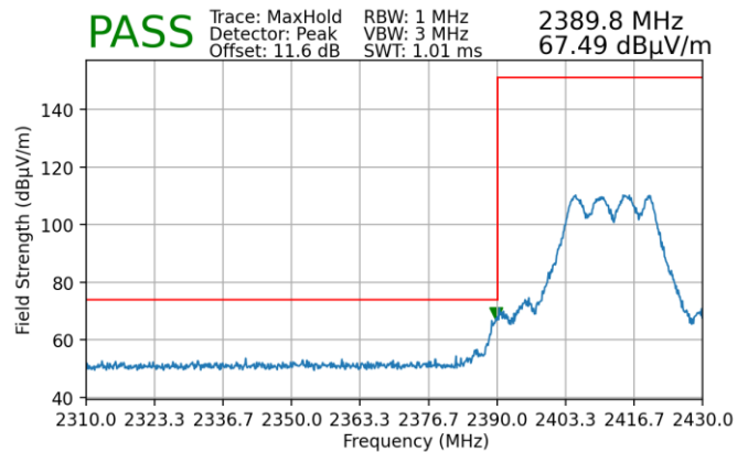
Plot 7-236. Radiated Restricted Lower Band Edge Measurement MIMO (Peak)
