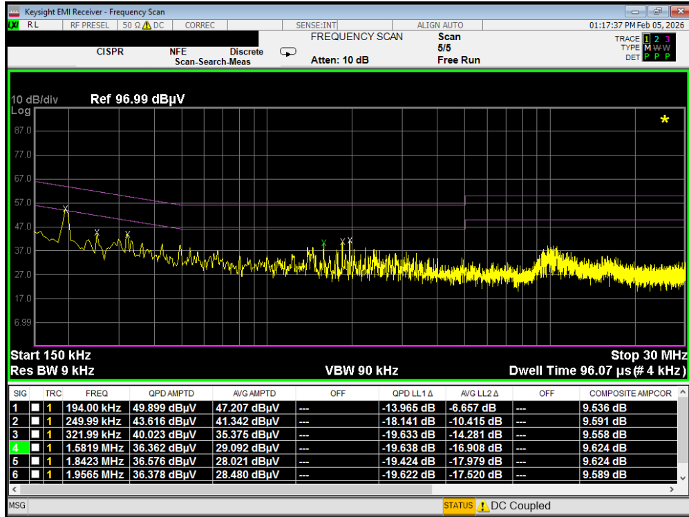
Plot 7-273. Line Conducted Plot with 802.11b (L1)
