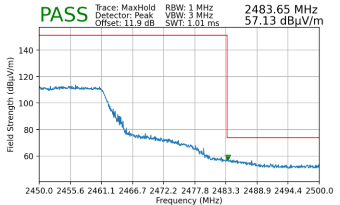
Plot 7-244. Radiated Restricted Upper Band Edge Measurement MIMO (Peak)
