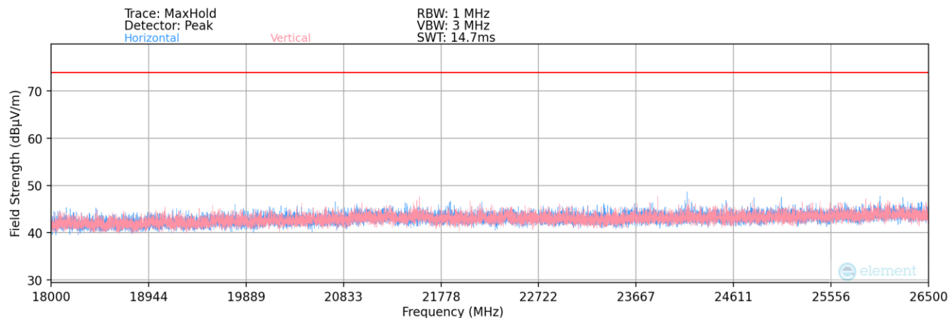
Plot 7-233. Radiated Spurious Plot 18GHz – 26.5GHz (2.4GHz – 6GHz)
