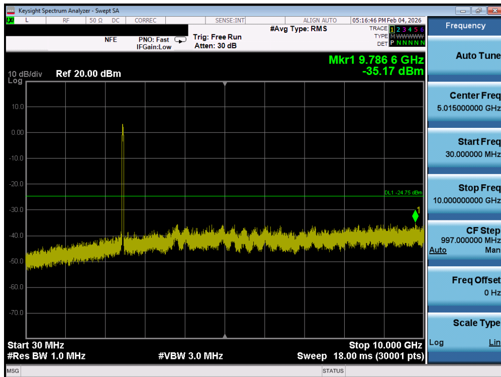
Plot 7-214. Conducted Spurious Plot MIMO ANT1 (802.11n 40MHz – Ch. 11) – MIMO ANT1
