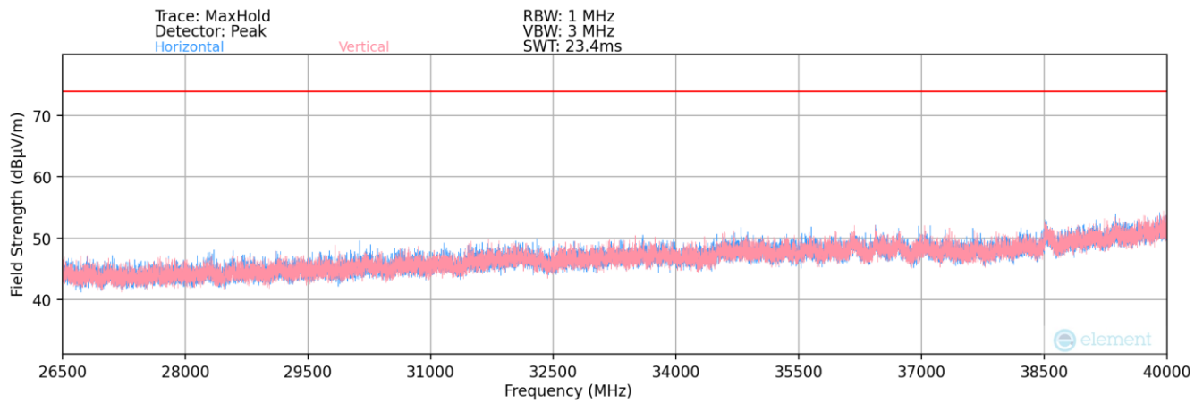
Plot 7-230. Radiated Spurious Plot above 26.5GHz (2.4GHz – 5GHz)
