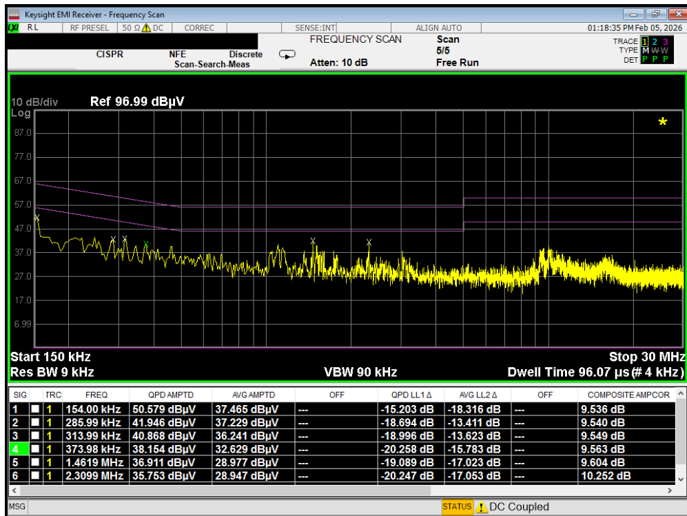
Plot 7-274. Line Conducted Plot with 802.11b (N)
