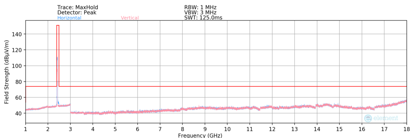
Plot 7-223. Radiated Spurious Plot above 1GHz MIMO (802.11b – Ch. 1)
