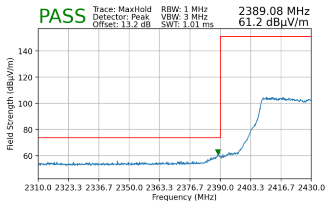
Plot 7-256. Radiated Restricted Lower Band Edge Measurement MIMO (Peak)
