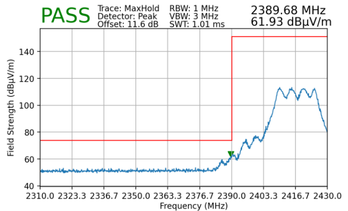
Plot 7-238. Radiated Restricted Lower Band Edge Measurement MIMO (Peak)
