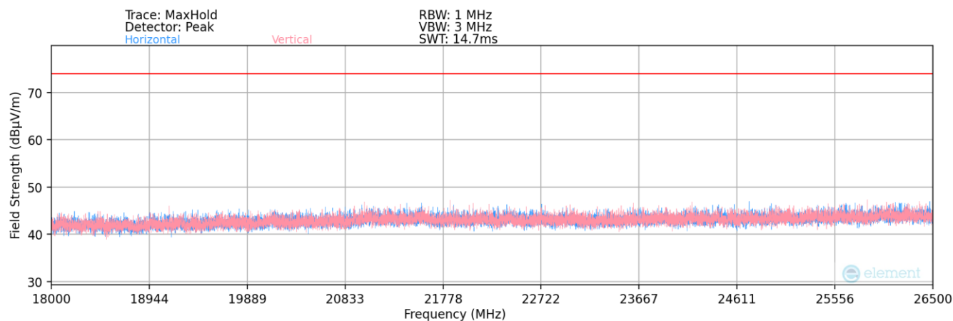
Plot 7-226. Radiated Spurious Plot above 18GHz MIMO
