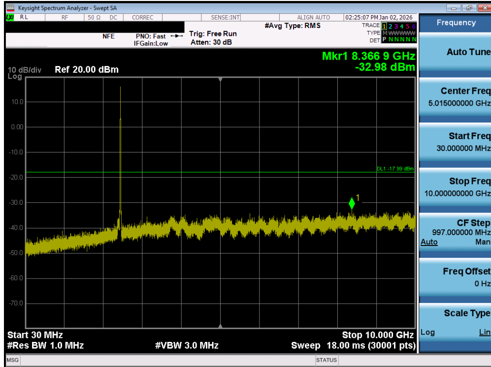
Plot 7-208. Conducted Spurious Plot MIMO ANT2 (802.11b – Ch. 11) – MIMO ANT2
