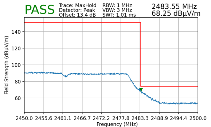
Plot 7-272. Radiated Restricted Upper Band Edge Measurement MIMO (Peak)
