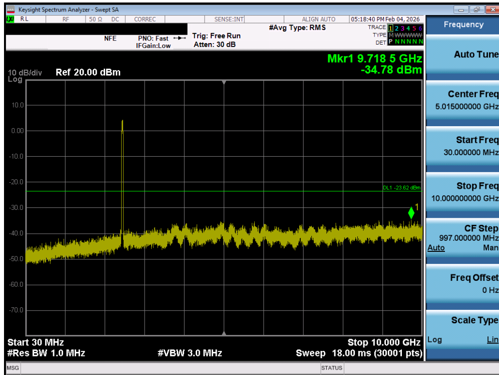
Plot 7-220. Conducted Spurious Plot MIMO ANT2 (802.11n 40MHz – Ch. 11) – MIMO ANT2
