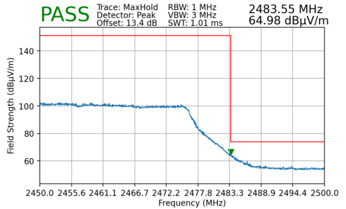
Plot 7-270. Radiated Restricted Upper Band Edge Measurement MIMO (Peak)
