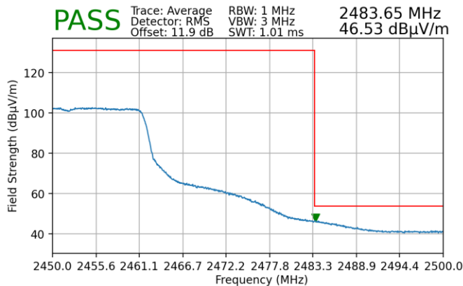
Plot 7-243. Radiated Restricted Upper Band Edge Measurement MIMO (Average)
