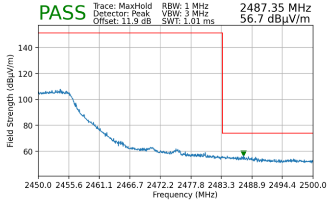
Plot 7-262. Radiated Restricted Upper Band Edge Measurement MIMO (Peak)
