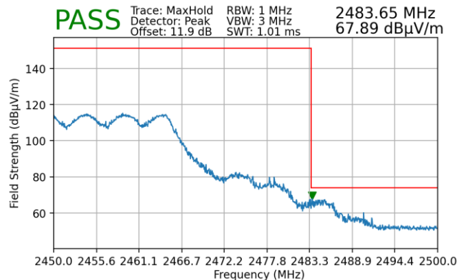
Plot 7-246. Radiated Restricted Upper Band Edge Measurement MIMO (Peak)
