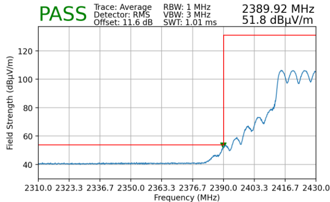
Plot 7-239. Radiated Restricted Lower Band Edge Measurement MIMO (Average)
