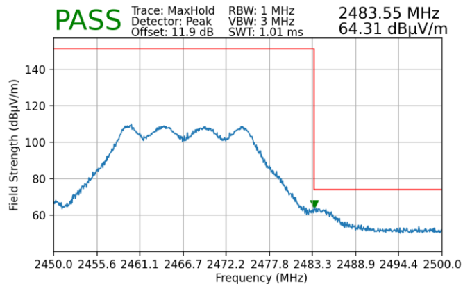
Plot 7-250. Radiated Restricted Upper Band Edge Measurement MIMO (Peak)
