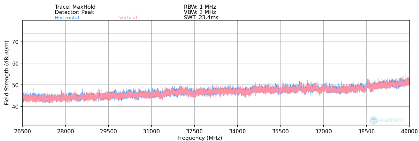
Plot 7-234. Radiated Spurious Plot above 26.5GHz (2.4GHz – 6GHz)
