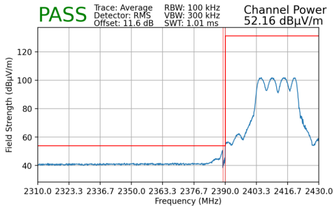
Plot 7-235. Radiated Restricted Lower Band Edge Measurement MIMO (Average)
