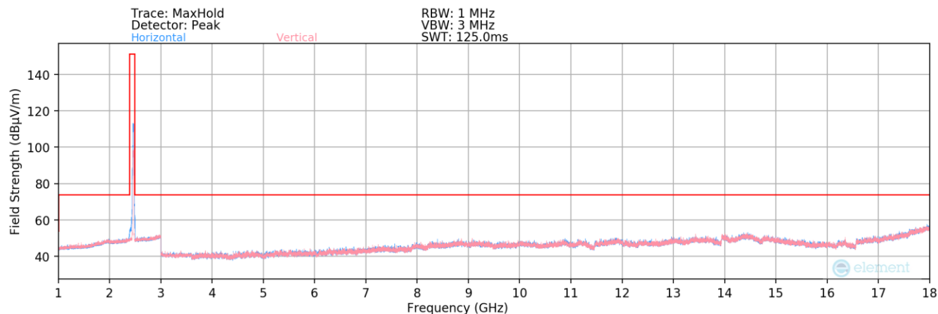
Plot 7-225. Radiated Spurious Plot above 1GHz MIMO (802.11b – Ch. 11)
