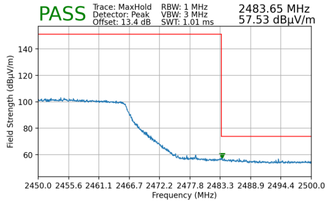
Plot 7-266. Radiated Restricted Upper Band Edge Measurement MIMO (Peak)
