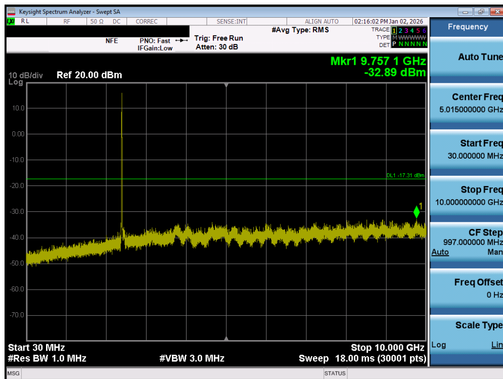
Plot 7-204. Conducted Spurious Plot MIMO ANT2 (802.11b – Ch. 1) – MIMO ANT2
