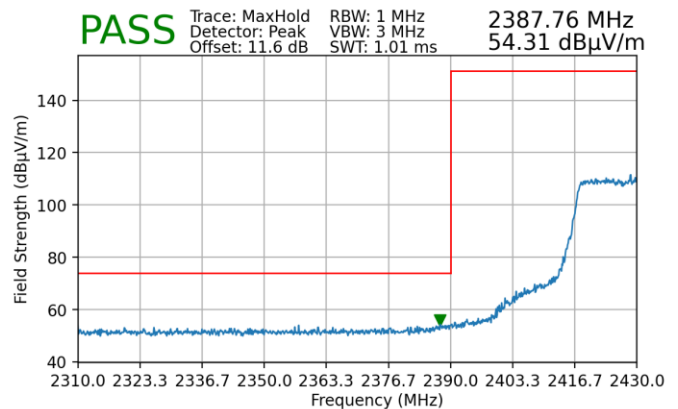
Plot 7-242. Radiated Restricted Lower Band Edge Measurement MIMO (Peak)
