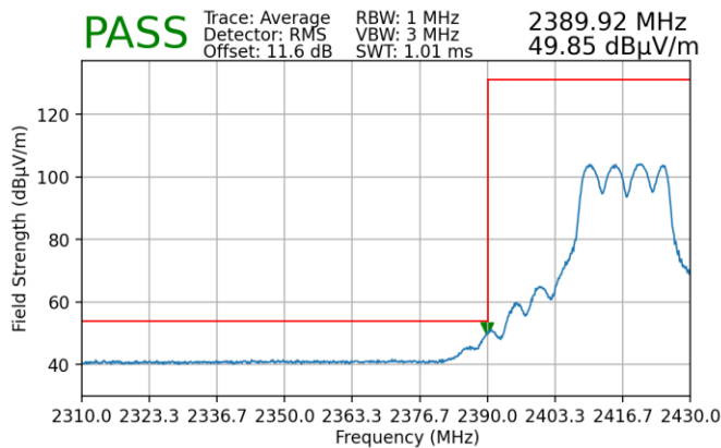
Plot 7-237. Radiated Restricted Lower Band Edge Measurement MIMO (Average)
