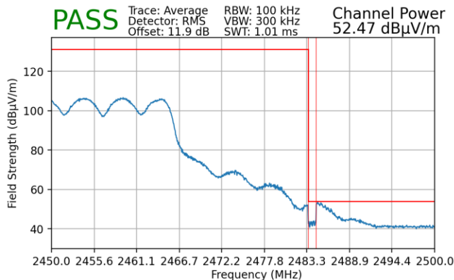
Plot 7-245. Radiated Restricted Upper Band Edge Measurement MIMO (Average)
