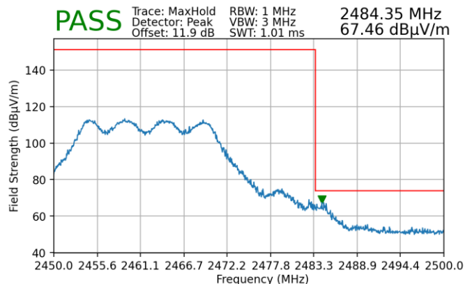
Plot 7-248. Radiated Restricted Upper Band Edge Measurement MIMO (Peak)
