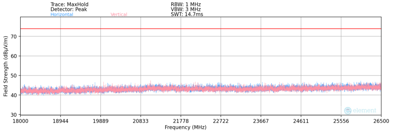
Plot 7-229. Radiated Spurious Plot 18GHz – 26.5GHz (2.4GHz – 5GHz)
