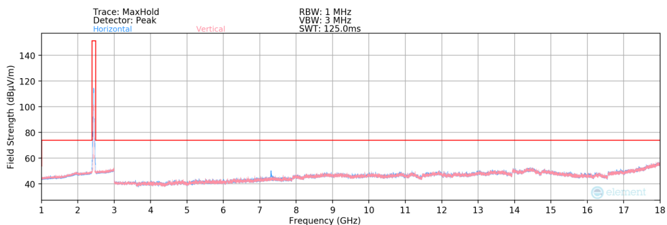
Plot 7-224. Radiated Spurious Plot above 1GHz MIMO (802.11b – Ch. 6)
