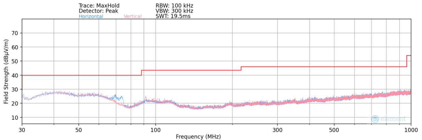
Plot 7-231. Radiated Spurious Plot below 1GHz (2.4GHz – 6GHz)
