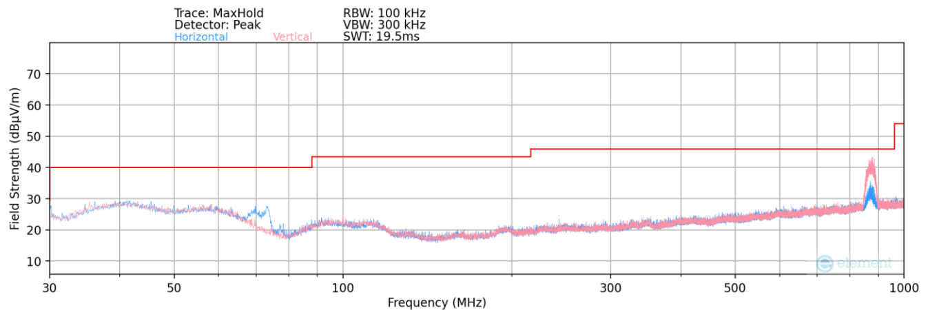
Plot 7-227. Radiated Spurious Plot below 1GHz (2.4GHz – 5GHz)
