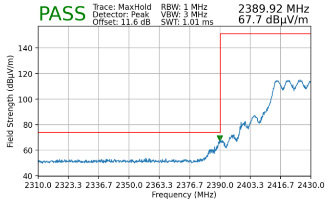
Plot 7-240. Radiated Restricted Lower Band Edge Measurement MIMO (Peak)
