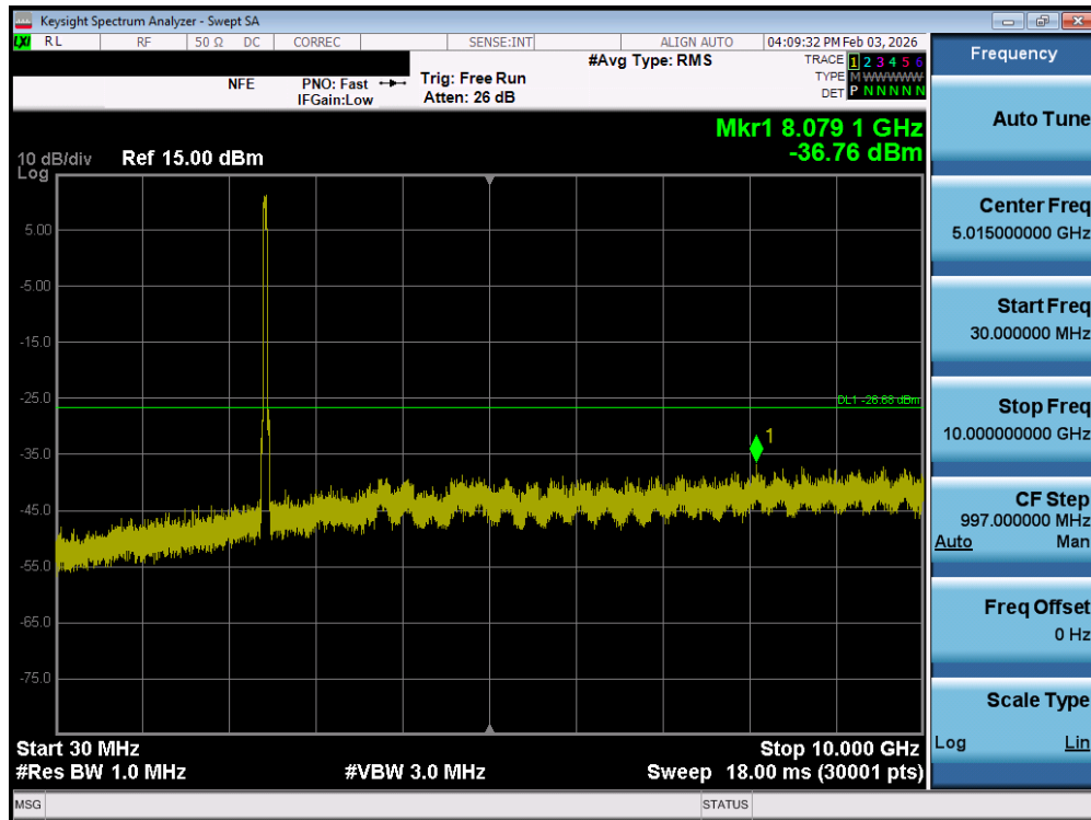
Plot 7-212. Conducted Spurious Plot MIMO ANT1 (802.11n 40MHz – Ch. 6) – MIMO ANT1
