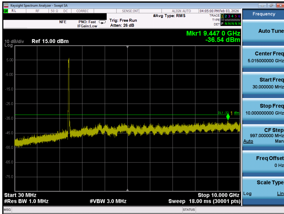
Plot 7-210. Conducted Spurious Plot MIMO ANT1 (802.11n 40MHz – Ch. 3) – MIMO ANT1
