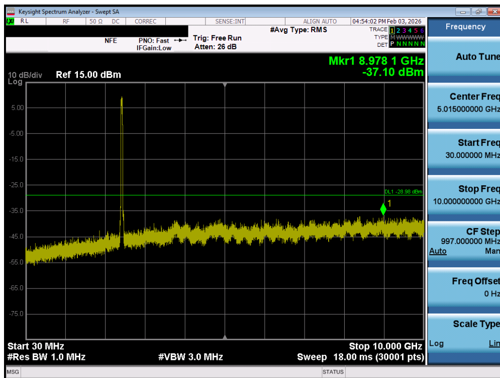
Plot 7-218. Conducted Spurious Plot MIMO ANT2 (802.11n 40MHz – Ch. 6) – MIMO ANT2
