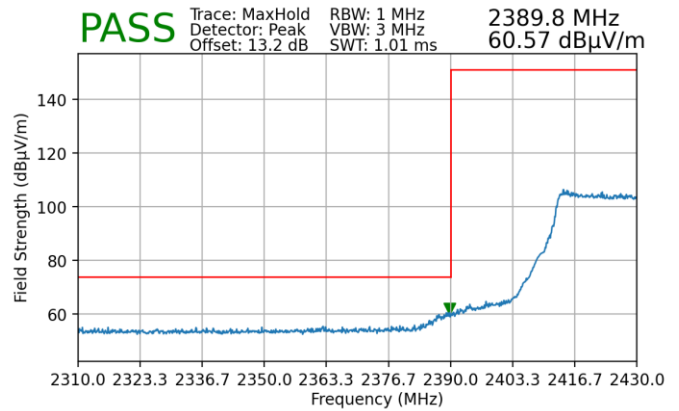
Plot 7-258. Radiated Restricted Lower Band Edge Measurement MIMO (Peak)
