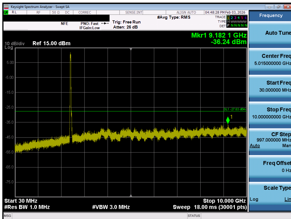
Plot 7-216. Conducted Spurious Plot MIMO ANT2 (802.11n 40MHz – Ch. 3) – MIMO ANT2
