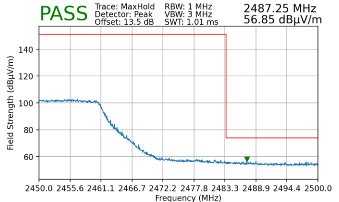
Plot 7-264. Radiated Restricted Upper Band Edge Measurement MIMO (Peak)
