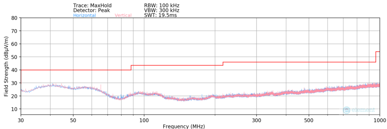
Plot 7-222. Radiated Spurious Plot below 1GHz MIMO
