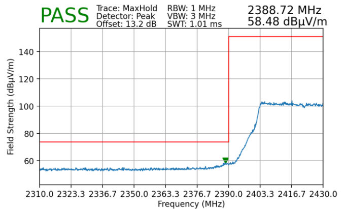
Plot 7-254. Radiated Restricted Lower Band Edge Measurement MIMO (Peak)
