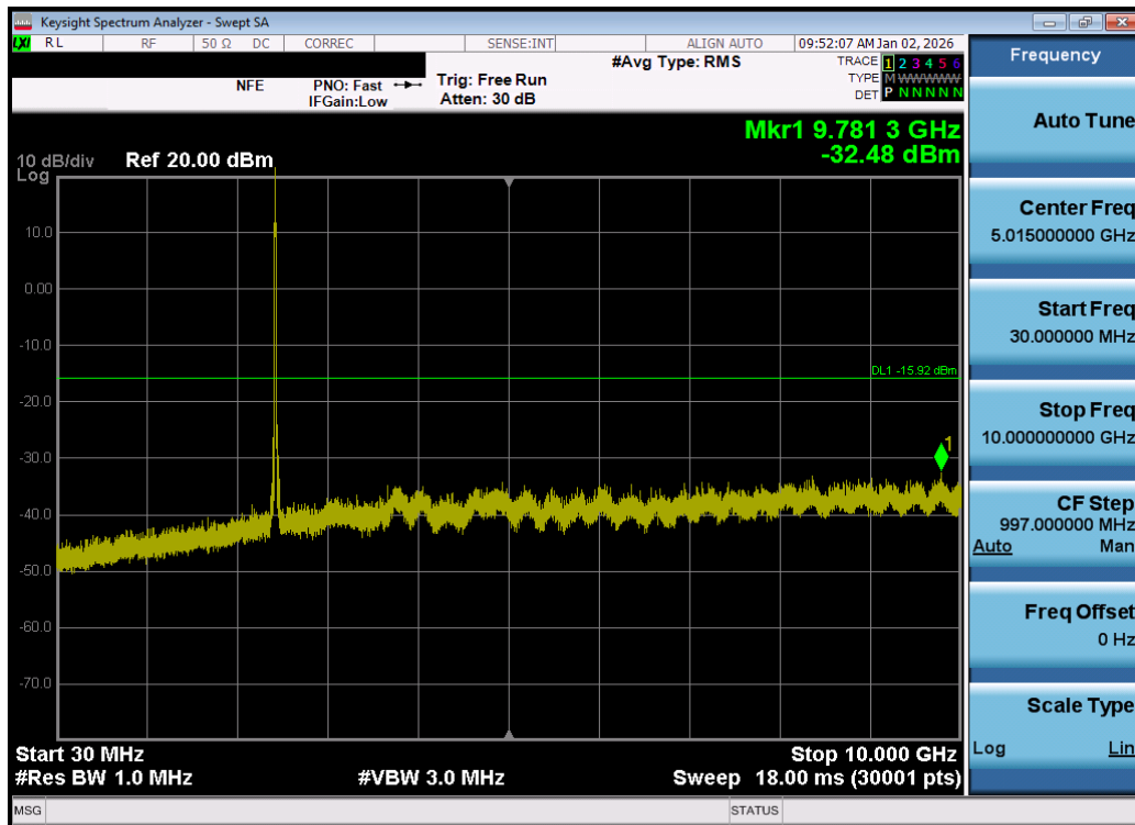
Plot 7-117. Conducted Spurious Plot MIMO ANT1 (802.11be OFDMA – 26 Tones – Ch. 6) – DUAL ANT 1
