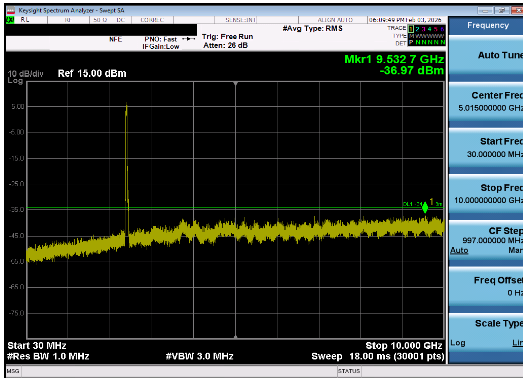
Plot 7-127. Conducted Spurious Plot MIMO ANT1 (802.11be OFDMA – 484 Tones – Ch. 3) – DUAL ANT 1
