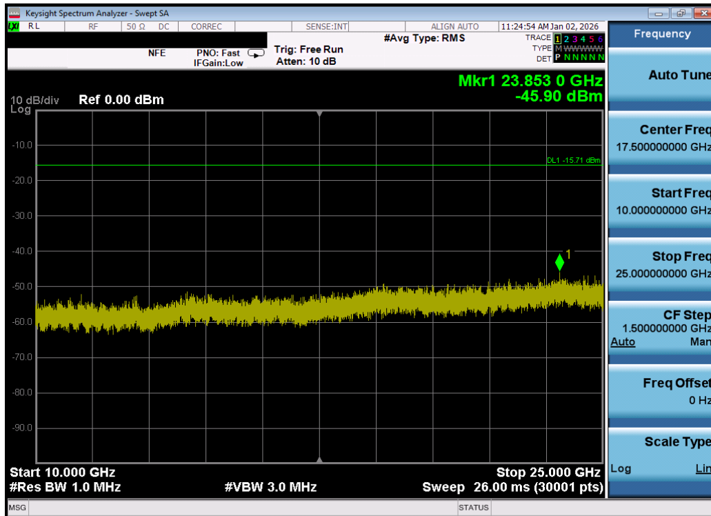
Plot 7-136. Conducted Spurious Plot MIMO ANT2 (802.11be OFDMA – 26 Tones – Ch. 6) – DUAL ANT 2
