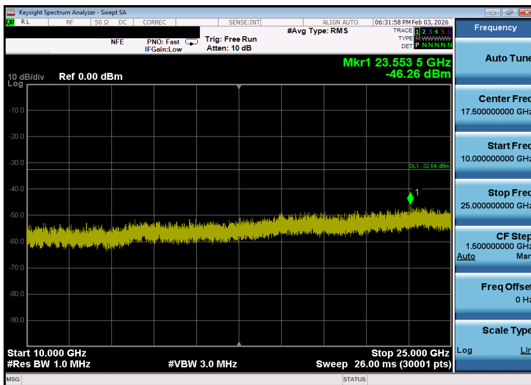
Plot 7-146. Conducted Spurious Plot MIMO ANT2 (802.11be OFDMA – 484 Tones – Ch. 3) – DUAL ANT 2
