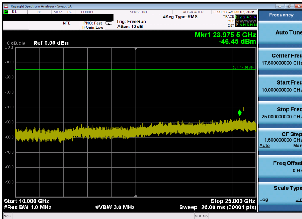
Plot 7-138. Conducted Spurious Plot MIMO ANT2 (802.11be OFDMA – 26 Tones – Ch. 11) – DUAL ANT 2
