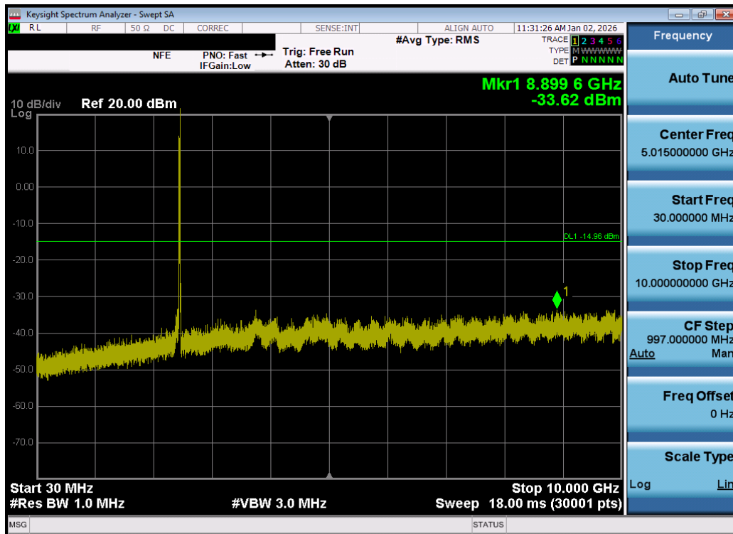
Plot 7-137. Conducted Spurious Plot MIMO ANT2 (802.11be OFDMA – 26 Tones – Ch. 11) – DUAL ANT 2
