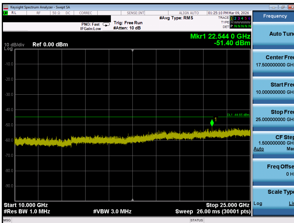
Plot 7-150. Conducted Spurious Plot MIMO ANT2 (802.11be OFDMA – 484 Tones – Ch. 11) – DUAL ANT 2
