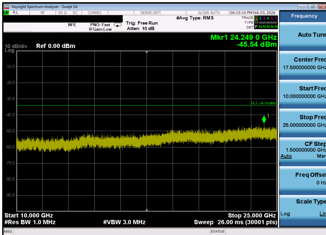
Plot 7-128. Conducted Spurious Plot MIMO ANT1 (802.11be OFDMA – 484 Tones – Ch. 3) – DUAL ANT 1
