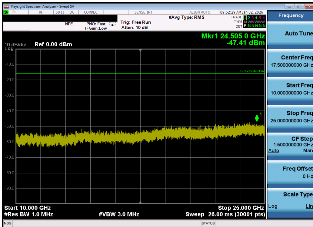
Plot 7-118. Conducted Spurious Plot MIMO ANT1 (802.11be OFDMA – 26 Tones – Ch. 6) – DUAL ANT 1
