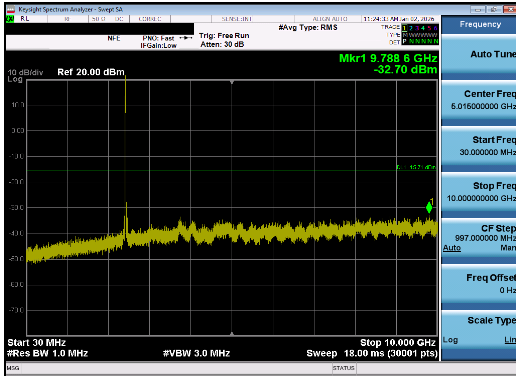
Plot 7-135. Conducted Spurious Plot MIMO ANT2 (802.11be OFDMA – 26 Tones – Ch. 6) – DUAL ANT 2
