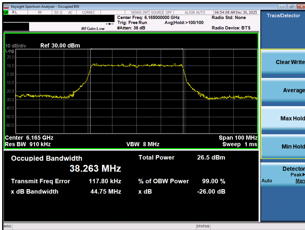
Plot 7-26. 26dB Bandwidth Plot MIMO ANT1 (40MHz 802.11ax/be (Full Tones) (UNII Band 5) – Ch. 43) – SP
