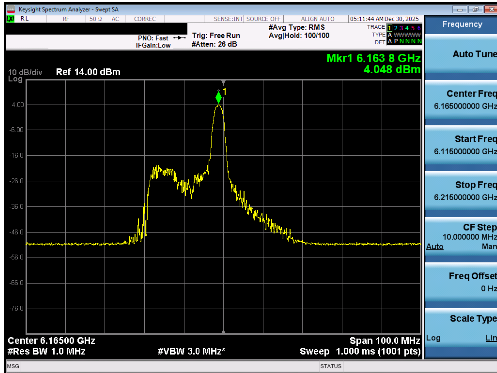
Plot 7-59. Power Spectral Density Plot MIMO ANT1 (40MHz 802.11ax/be (26 Tones) (UNII Band 5) – Ch. 43) - SP
