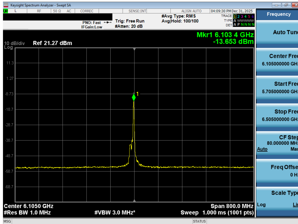
Plot 7-79. Power Spectral Density Plot MIMO ANT2 (320MHz 802.11be (26 Tones) (UNII Band 5) – Ch. 31) - LPI
