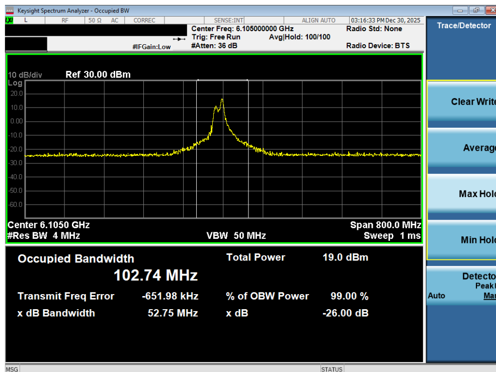
Plot 7-41. 26dB Bandwidth Plot MIMO ANT2 (320MHz 802.11be (26 Tones) (UNII Band 5) – Ch. 31) - SP
