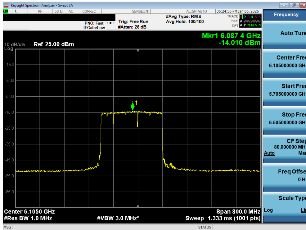
Plot 7-83. Power Spectral Density Plot MIMO ANT2 (320MHz 802.11be (UNII Band 5) – Ch. 31) LPI
