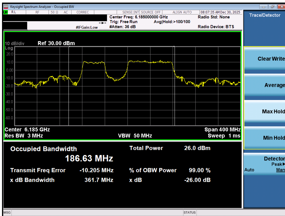
Plot 7-19. 26dB Bandwidth Plot MIMO ANT1 (160MHz 802.11be (996+484 Tones) (UNII Band 5) – Ch. 47) - SP
