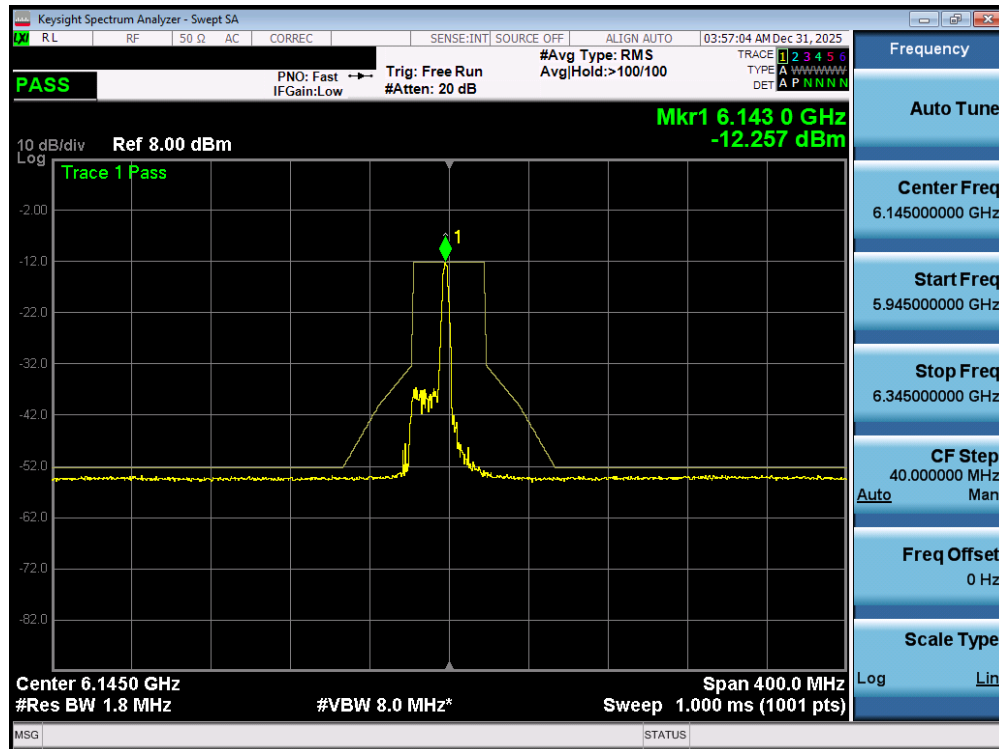
Plot 7-103. In Band Emissions Plot MIMO ANT1 (80MHz 802.11ax/be (26 Tones) (UNII Band 5) – Ch. 39) - LPI
