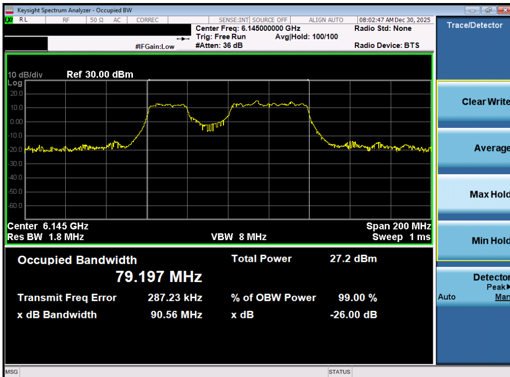
Plot 7-18. 26dB Bandwidth Plot MIMO ANT1 (80MHz 802.11be (484+242 Tones) (UNII Band 5) – Ch. 39) - SP
