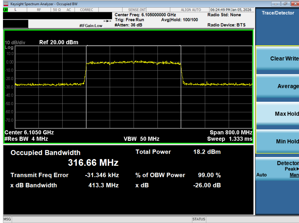
Plot 7-49. 26dB Bandwidth Plot MIMO ANT2 (320MHz 802.11be (Full Tones) (UNII Band 5) – Ch. 31) - LPI
