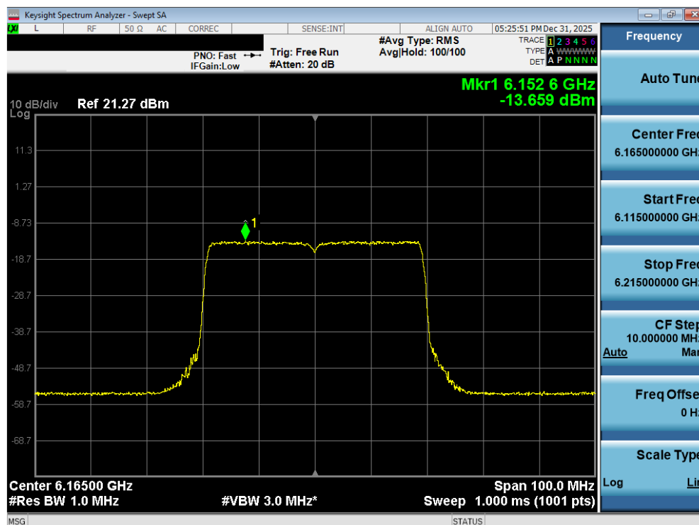
Plot 7-94. Power Spectral Density Plot MIMO ANT2 (40MHz 802.11ax/be (Full Tones) (UNII Band 5) – Ch. 43) - LPI
