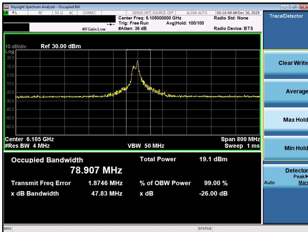
Plot 7-14. 26dB Bandwidth Plot MIMO ANT1 (320MHz 802.11be (26 Tones) (UNII Band 5) – Ch. 31) - SP
