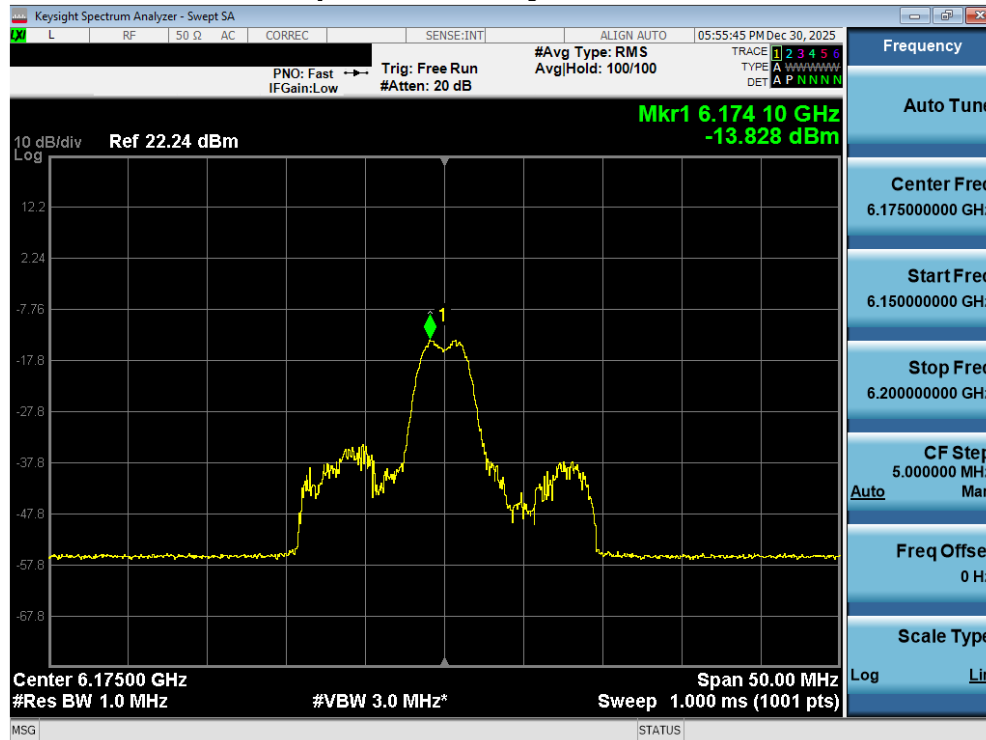
Plot 7-75. Power Spectral Density Plot MIMO ANT2 (20MHz 802.11ax/be (26 Tones) (UNII Band 5) – Ch. 45) - LPI
