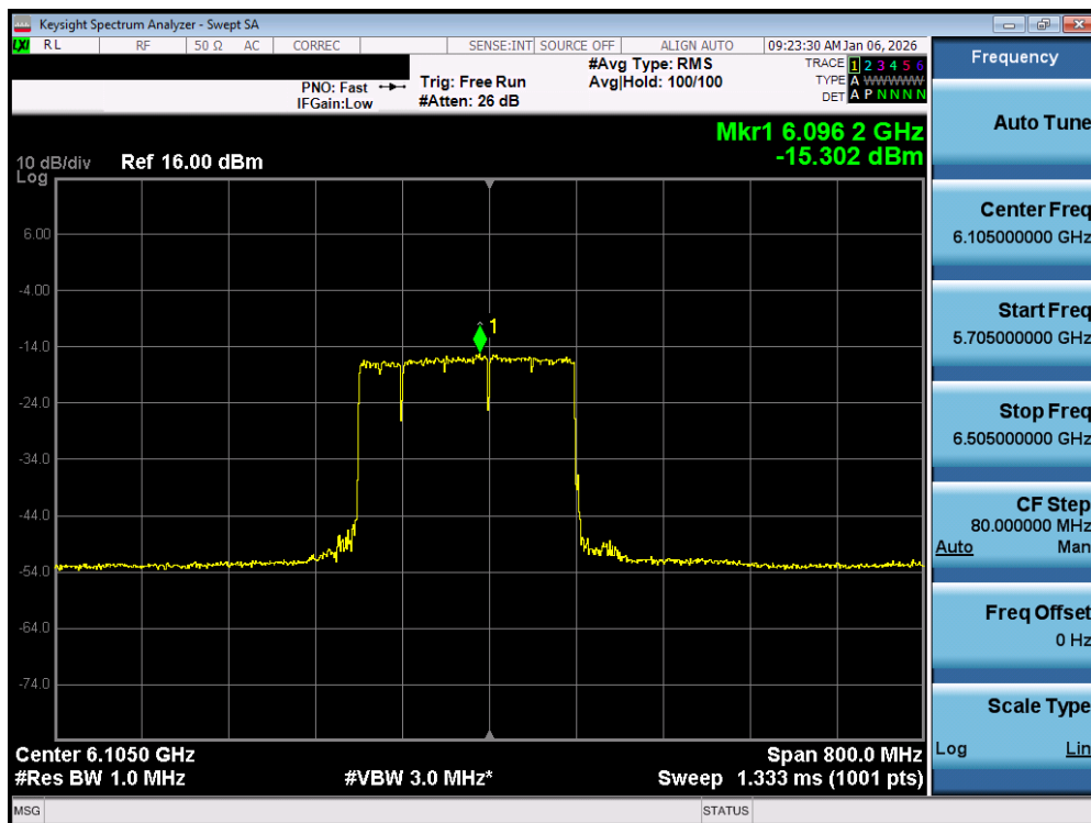
Plot 7-66. Power Spectral Density Plot MIMO ANT1 (320MHz 802.11be (UNII Band 5) – Ch. 31) - LPI
