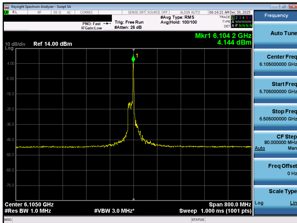
Plot 7-62. Power Spectral Density Plot MIMO ANT1 (320MHz 802.11be (26 Tones) (UNII Band 5) – Ch. 31) - SP
