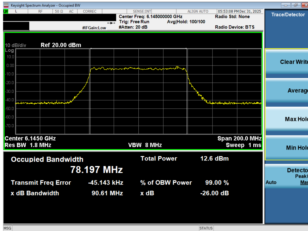
Plot 7-47. 26dB Bandwidth Plot MIMO ANT2 (80MHz 802.11ax/be (Full Tones) (UNII Band 5) – Ch. 39) - LPI
