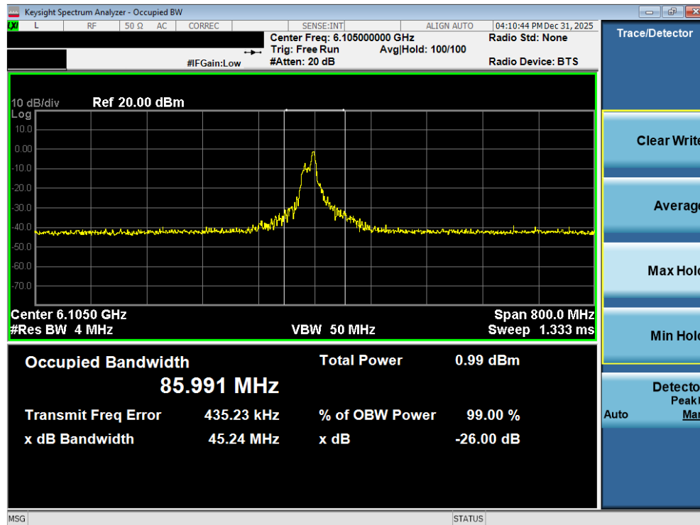
Plot 7-32. 26dB Bandwidth Plot MIMO ANT2 (320MHz 802.11be (26 Tones) (UNII Band 5) – Ch. 31) - LPI
