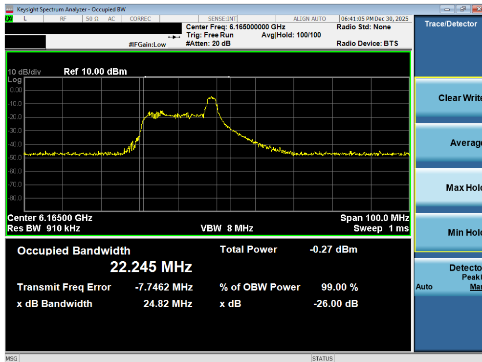
Plot 7-29. 26dB Bandwidth Plot MIMO ANT2 (40MHz 802.11ax/be (26 Tones) (UNII Band 5) – Ch. 43) - LPI
