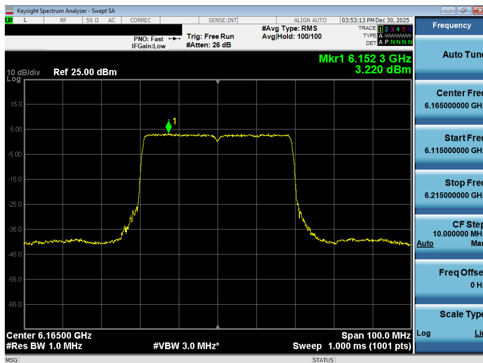
Plot 7-99. Power Spectral Density Plot MIMO ANT2 (40MHz 802.11ax/be (Full Tones) (UNII Band 5) – Ch. 43) - SP
