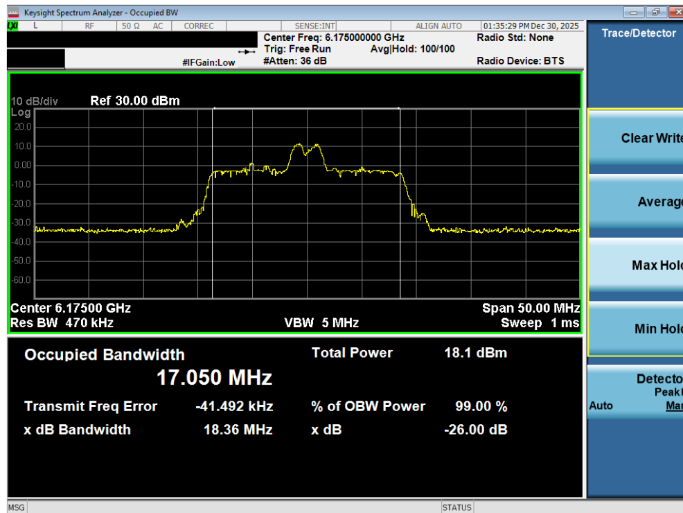
Plot 7-37. 26dB Bandwidth Plot MIMO ANT2 (20MHz 802.11ax/be (26 Tones) (UNII Band 5) – Ch. 45) - SP
