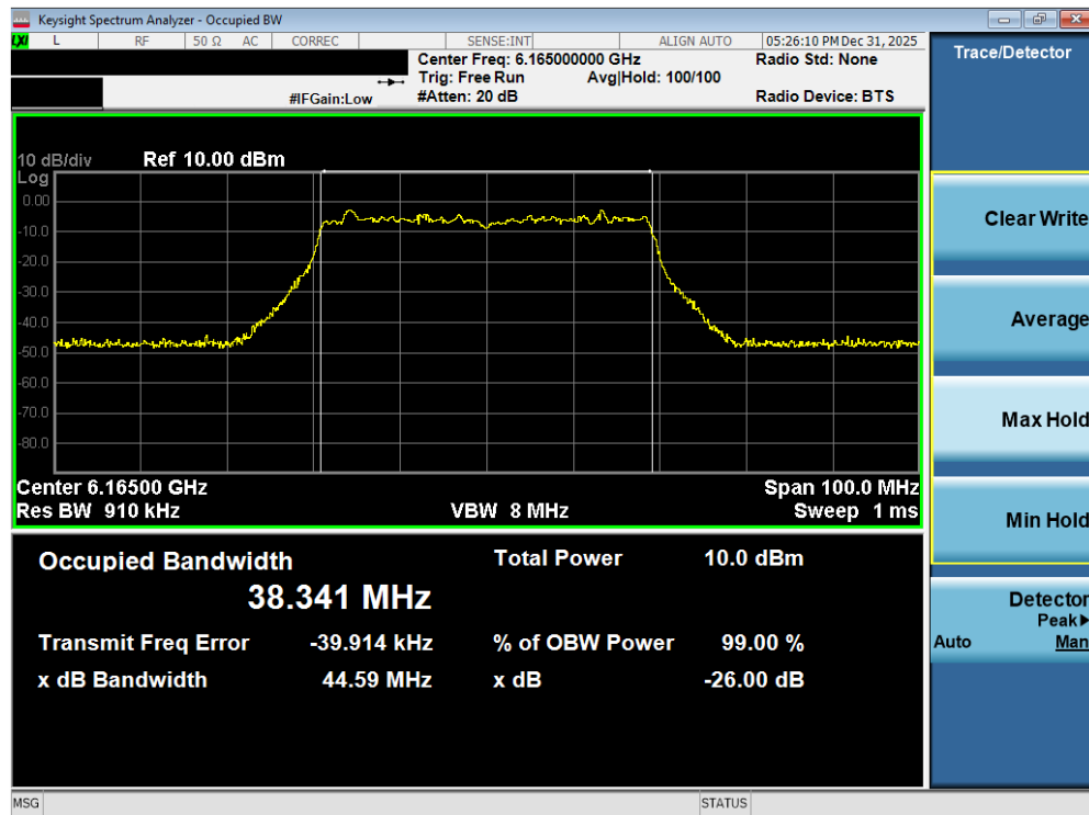
Plot 7-46. 26dB Bandwidth Plot MIMO ANT2 (40MHz 802.11ax/be (Full Tones) (UNII Band 5) – Ch. 43) - LPI
