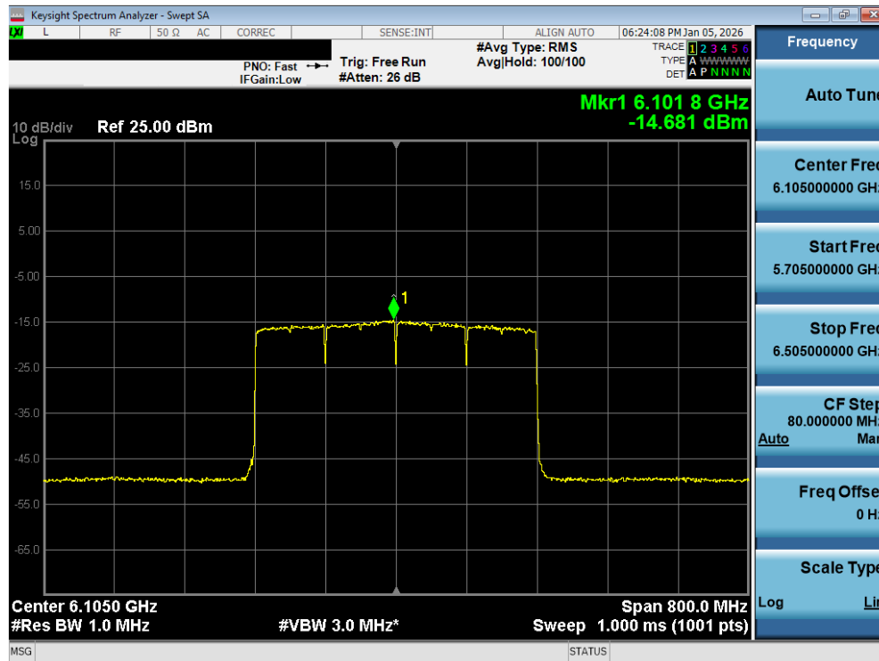
Plot 7-97. Power Spectral Density Plot MIMO ANT2 (320MHz 802.11be (Full Tones) (UNII Band 5) – Ch. 31) - LPI
