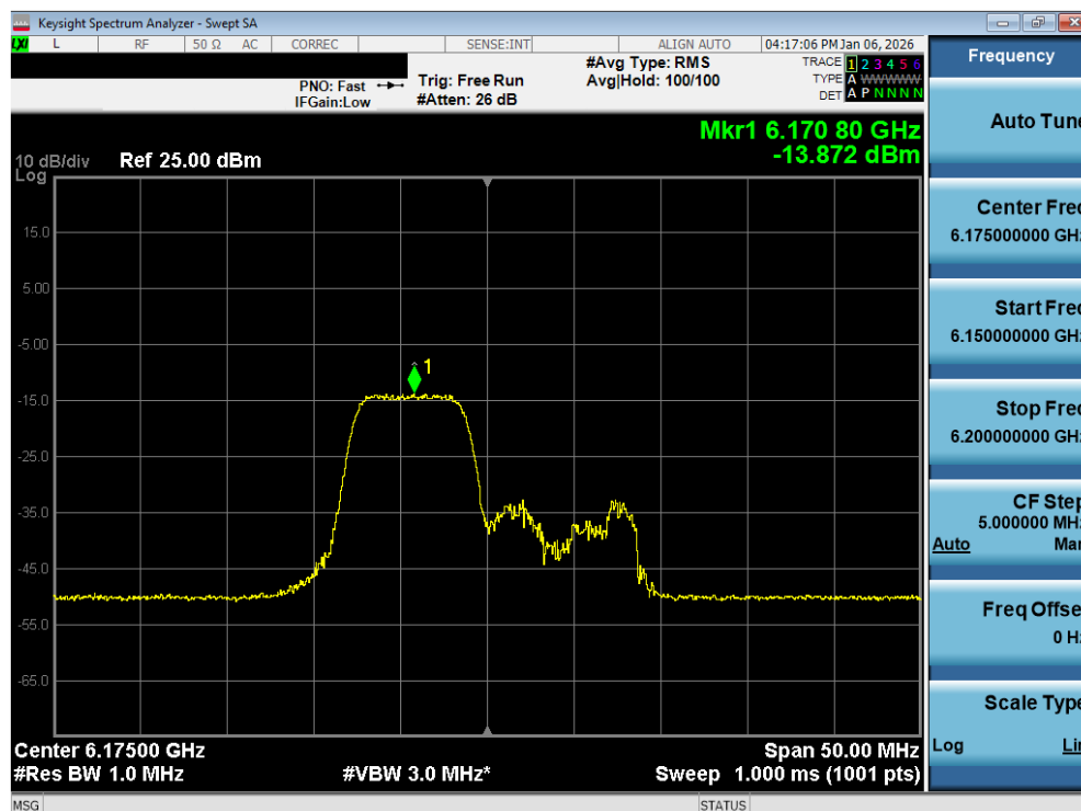
Plot 7-80. Power Spectral Density Plot MIMO ANT2 (20MHz 802.11be (52+26 Tones) (UNII Band 5) – Ch. 45) - LPI
