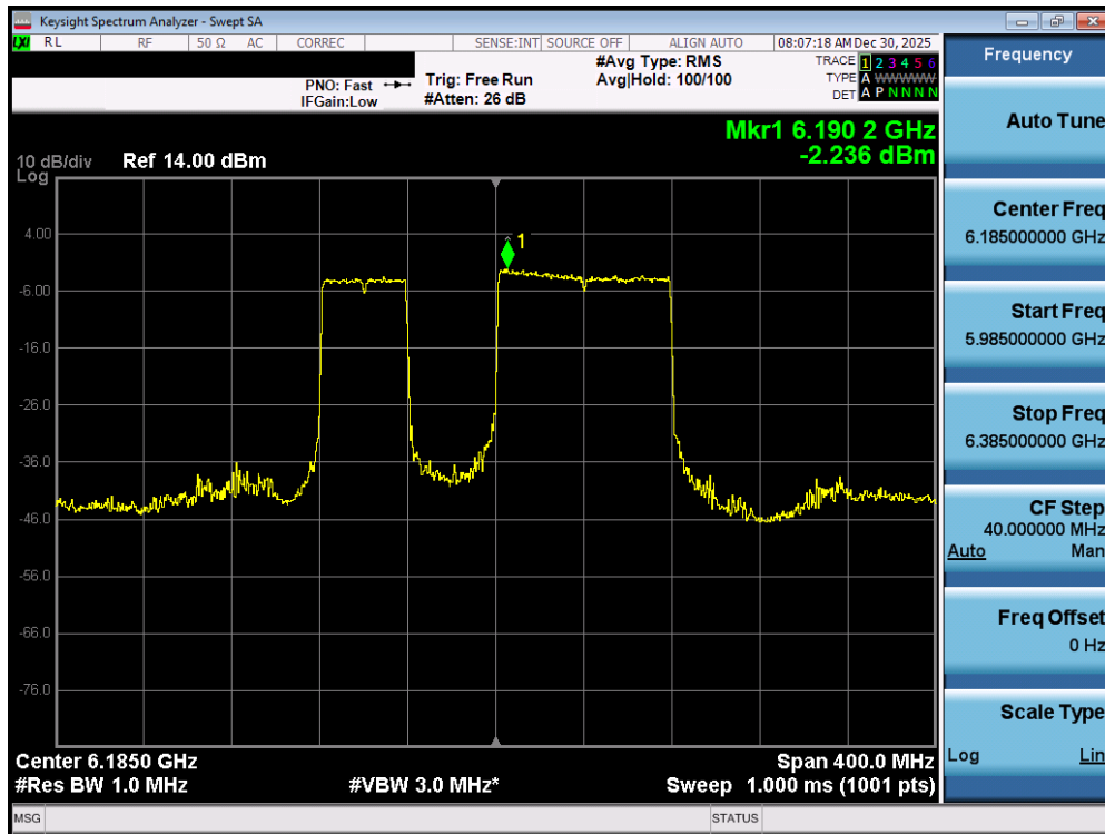
Plot 7-65. Power Spectral Density Plot MIMO ANT1 (160MHz 802.11be (996+484 Tones) (UNII Band 5) – Ch. 47) - SP
