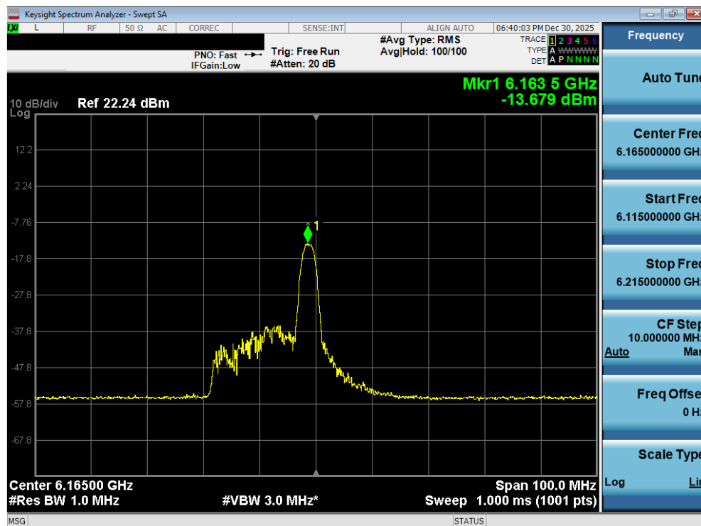
Plot 7-76. Power Spectral Density Plot MIMO ANT2 (40MHz 802.11ax/be (26 Tones) (UNII Band 5) – Ch. 43) - LPI
