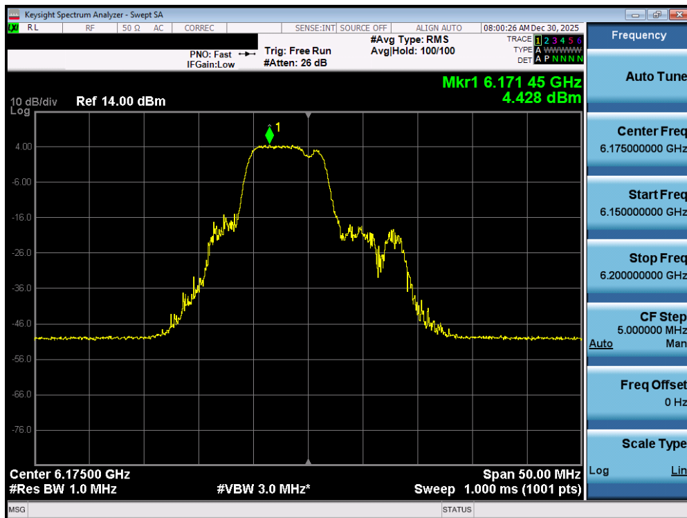
Plot 7-63. Power Spectral Density Plot MIMO ANT1 (20MHz 802.11be (52+26 Tones) (UNII Band 5) – Ch. 45) – SP
