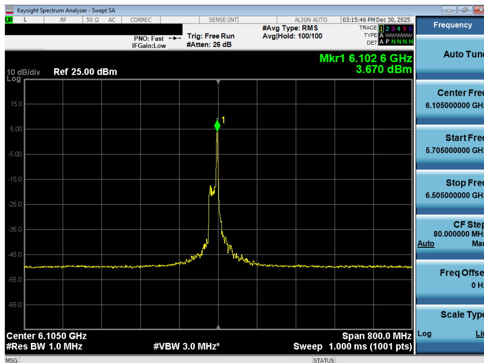
Plot 7-88. Power Spectral Density Plot MIMO ANT2 (320MHz 802.11be (26 Tones) (UNII Band 5) – Ch. 31) - SP
