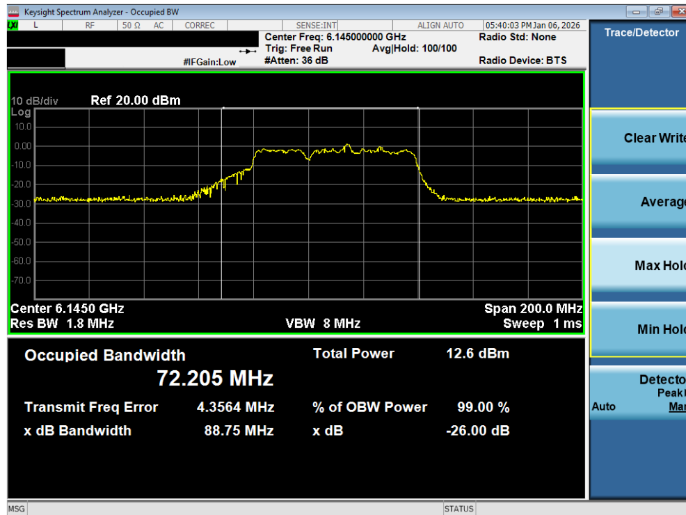
Plot 7-34. 26dB Bandwidth Plot MIMO ANT2 (80MHz 802.11be (484+242 Tones) (UNII Band 5) – Ch. 39) - LPI
