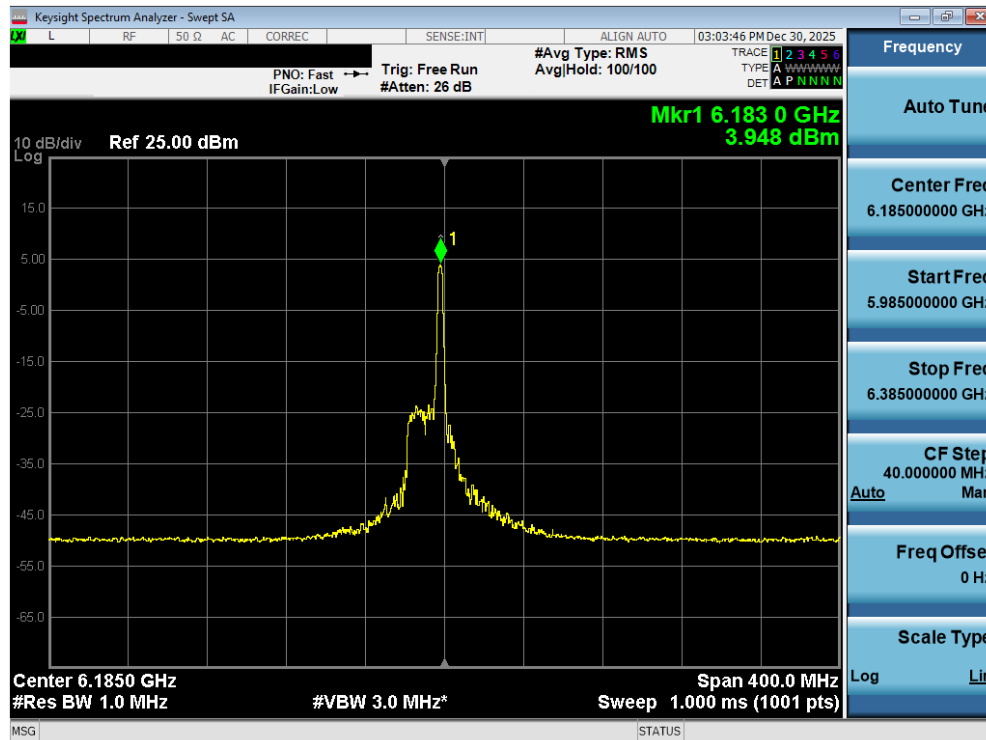
Plot 7-87. Power Spectral Density Plot MIMO ANT2 (160MHz 802.11ax/be (26 Tones) (UNII Band 5) – Ch. 47) - SP
