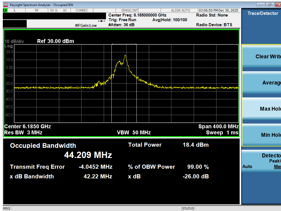
Plot 7-40. 26dB Bandwidth Plot MIMO ANT2 (160MHz 802.11ax/be (26 Tones) (UNII Band 5) – Ch. 47) - SP
