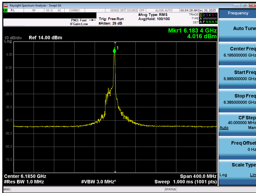
Plot 7-61. Power Spectral Density Plot MIMO ANT1 (160MHz 802.11ax/be (26 Tones) (UNII Band 5) – Ch. 47) - SP
