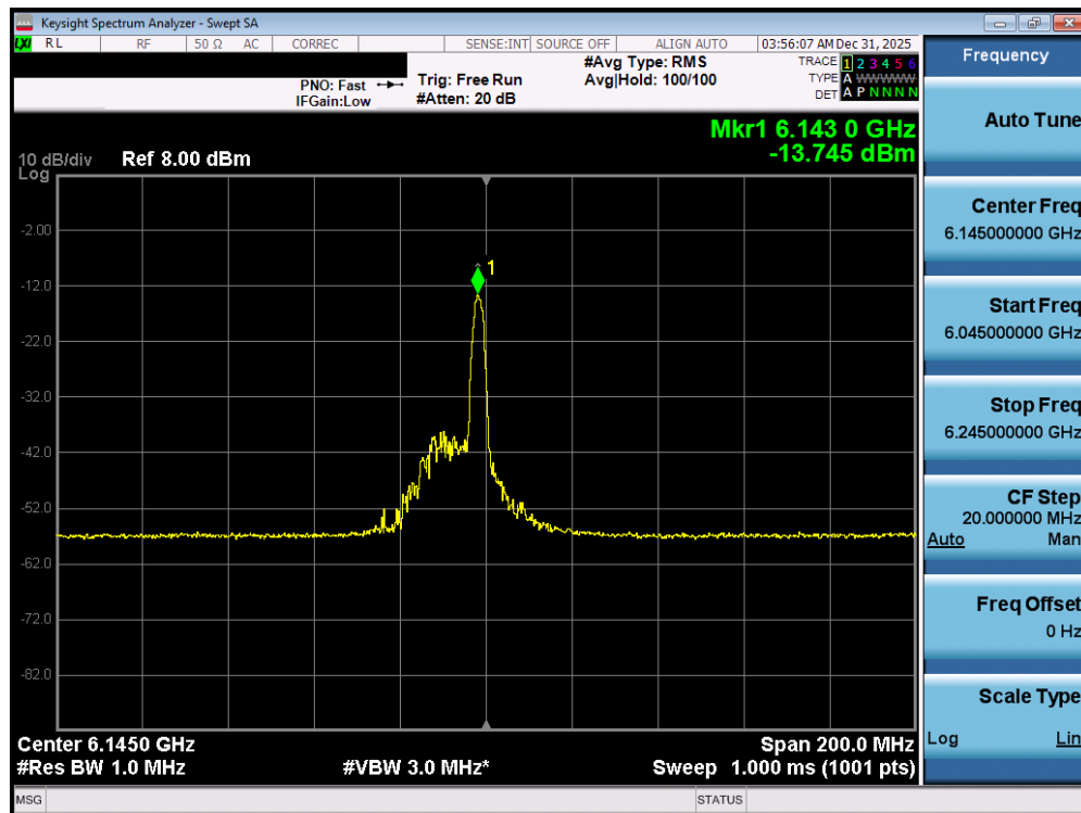
Plot 7-55. Power Spectral Density Plot MIMO ANT1 (80MHz 802.11ax/be (26 Tones) (UNII Band 5) – Ch. 39) - LPI
