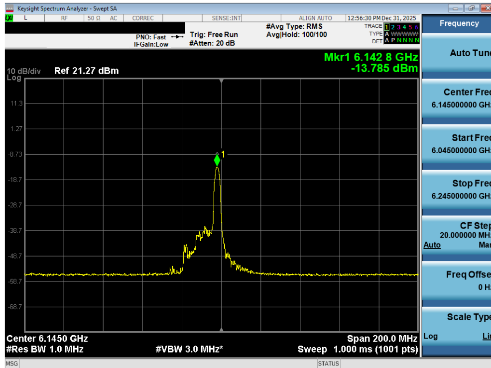
Plot 7-77. Power Spectral Density Plot MIMO ANT2 (80MHz 802.11ax/be (26 Tones) (UNII Band 5) – Ch. 39) - LPI
