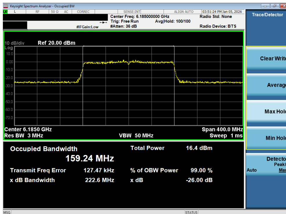
Plot 7-48. 26dB Bandwidth Plot MIMO ANT2 (160MHz 802.11ax/be (Full Tones) (UNII Band 5) – Ch. 47) - LPI
