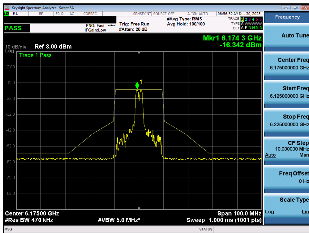
Plot 7-101. In Band Emissions Plot MIMO ANT1 (20MHz 802.11ax/be (26 Tones) (UNII Band 5) – Ch. 45) - LPI
