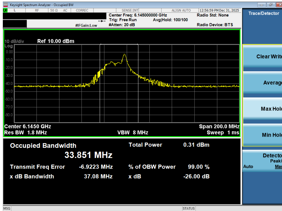
Plot 7-30. 26dB Bandwidth Plot MIMO ANT2 (80MHz 802.11ax/be (26 Tones) (UNII Band 5) – Ch. 39) - LPI
