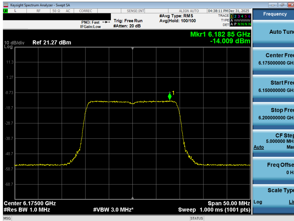
Plot 7-93. Power Spectral Density Plot MIMO ANT2 (20MHz 802.11ax/be (Full Tones) (UNII Band 5) – Ch. 45) - LPI
