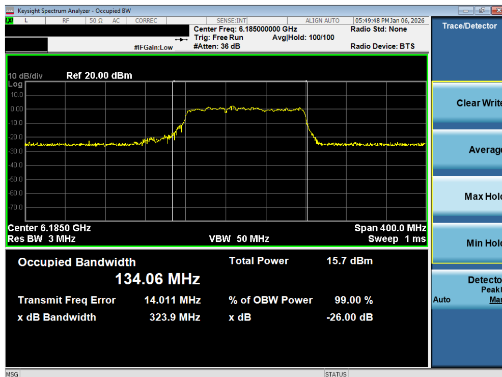
Plot 7-35. 26dB Bandwidth Plot MIMO ANT2 (160MHz 802.11be (996+484 Tones) (UNII Band 5) – Ch. 47) - LPI
