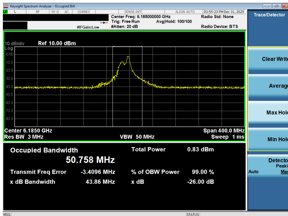
Plot 7-31. 26dB Bandwidth Plot MIMO ANT2 (160MHz 802.11ax/be (26 Tones) (UNII Band 5) – Ch. 47) - LPI
