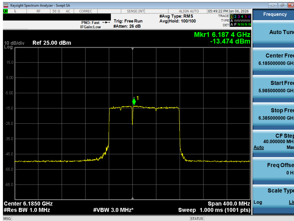
Plot 7-82. Power Spectral Density Plot MIMO ANT2 (160MHz 802.11be (996+484 Tones) (UNII Band 5) – Ch. 47) - LPI
