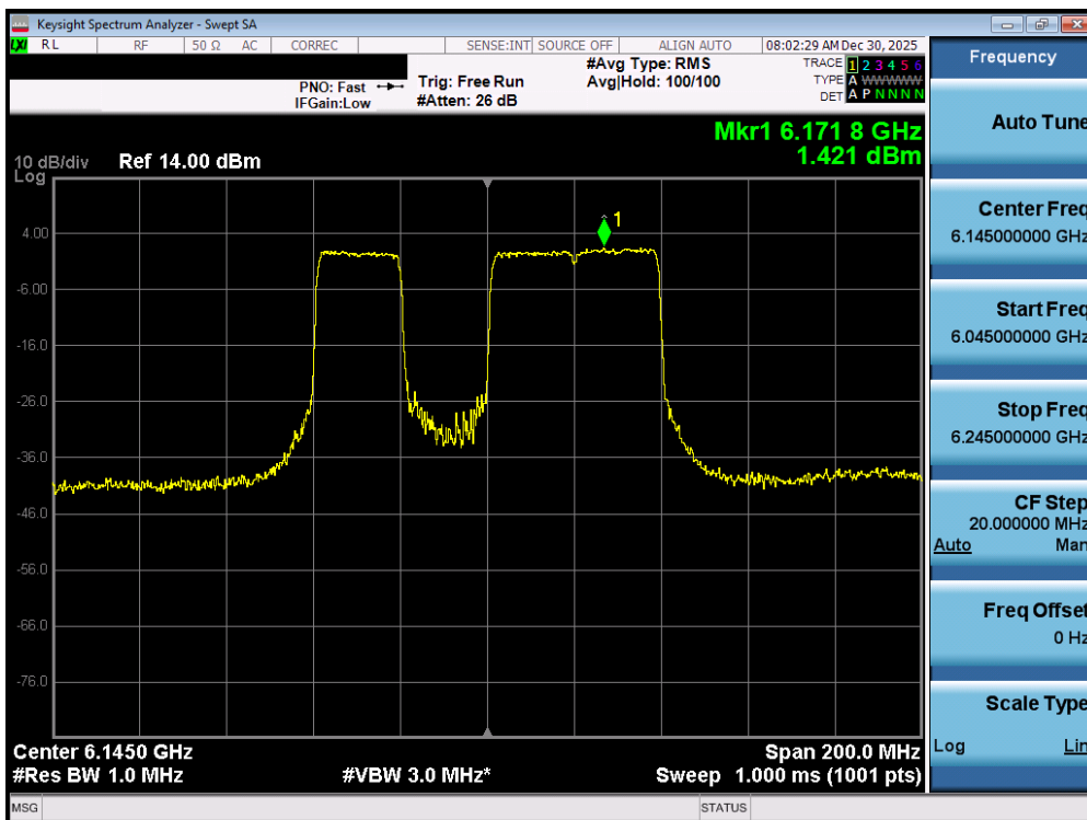
Plot 7-64. Power Spectral Density Plot MIMO ANT1 (80MHz 802.11be (484+242 Tones) (UNII Band 5) – Ch. 39) - SP
