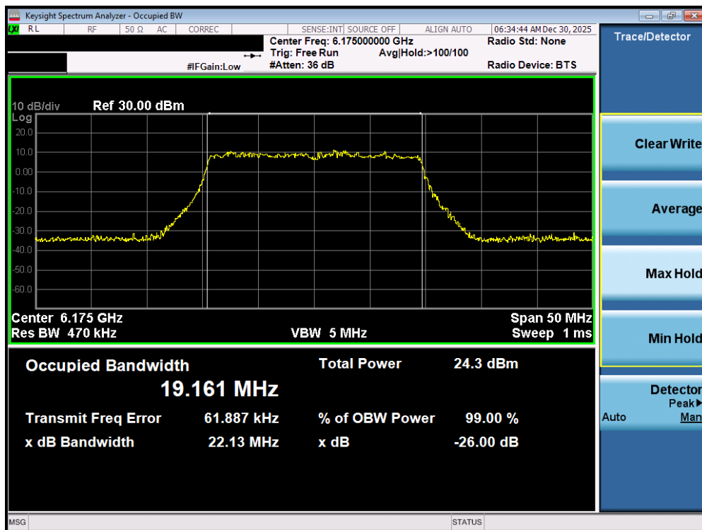
Plot 7-25. 26dB Bandwidth Plot MIMO ANT1 (20MHz 802.11ax/be (Full Tones) (UNII Band 5) – Ch. 45) - SP
