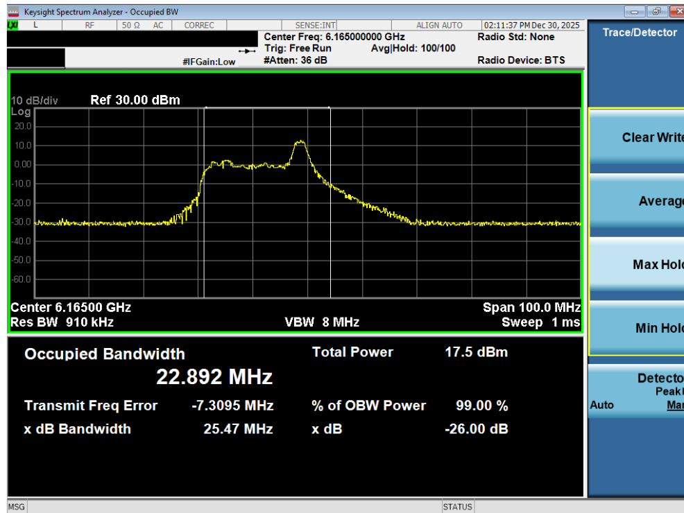
Plot 7-38. 26dB Bandwidth Plot MIMO ANT2 (40MHz 802.11ax/be (26 Tones) (UNII Band 5) – Ch. 43) - SP
