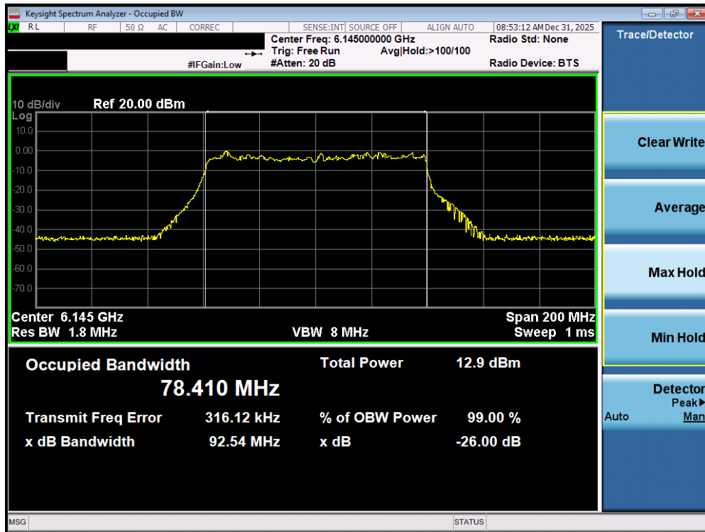
Plot 7-22. 26dB Bandwidth Plot MIMO ANT1 (80MHz 802.11ax/be (Full Tones) (UNII Band 5) – Ch. 39) - LPI
