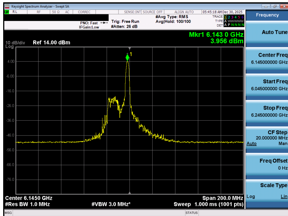
Plot 7-60. Power Spectral Density Plot MIMO ANT1 (80MHz 802.11ax/be (26 Tones) (UNII Band 5) – Ch. 39) - SP
