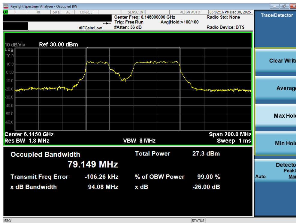
Plot 7-43. 26dB Bandwidth Plot MIMO ANT2 (80MHz 802.11be (484+242 Tones) (UNII Band 5) – Ch. 39) - SP
