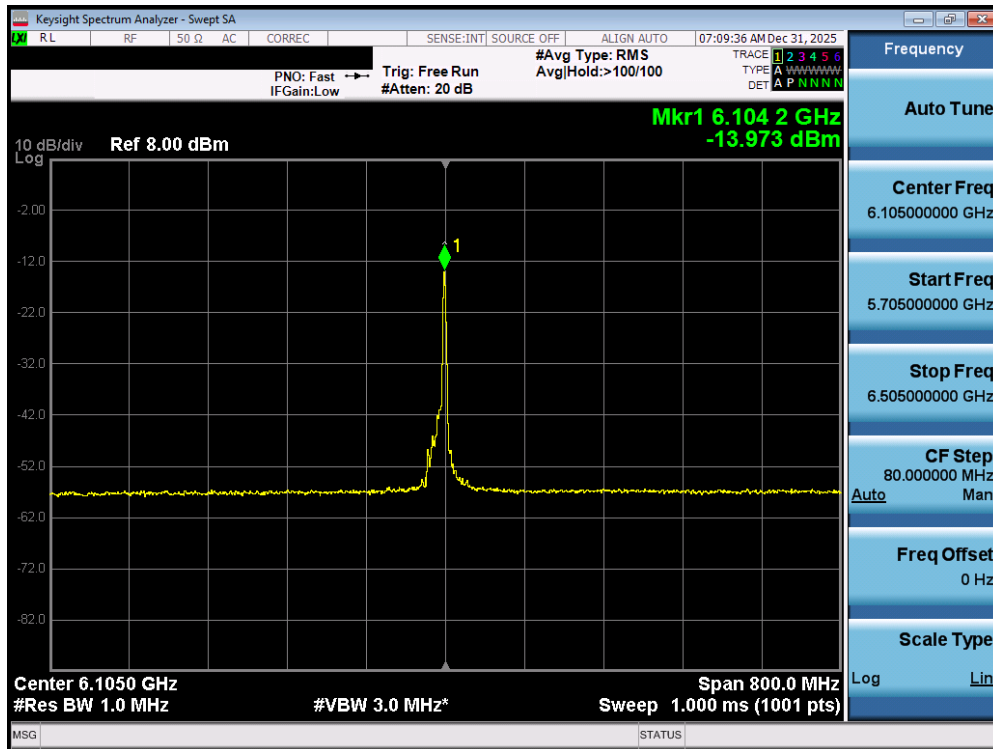
Plot 7-57. Power Spectral Density Plot MIMO ANT1 (320MHz 802.11be (26 Tones) (UNII Band 5) – Ch. 31) - LPI
