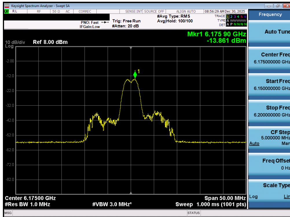
Plot 7-53. Power Spectral Density Plot MIMO ANT1 (20MHz 802.11ax/be (26 Tones) (UNII Band 5) – Ch. 45) - LPI
