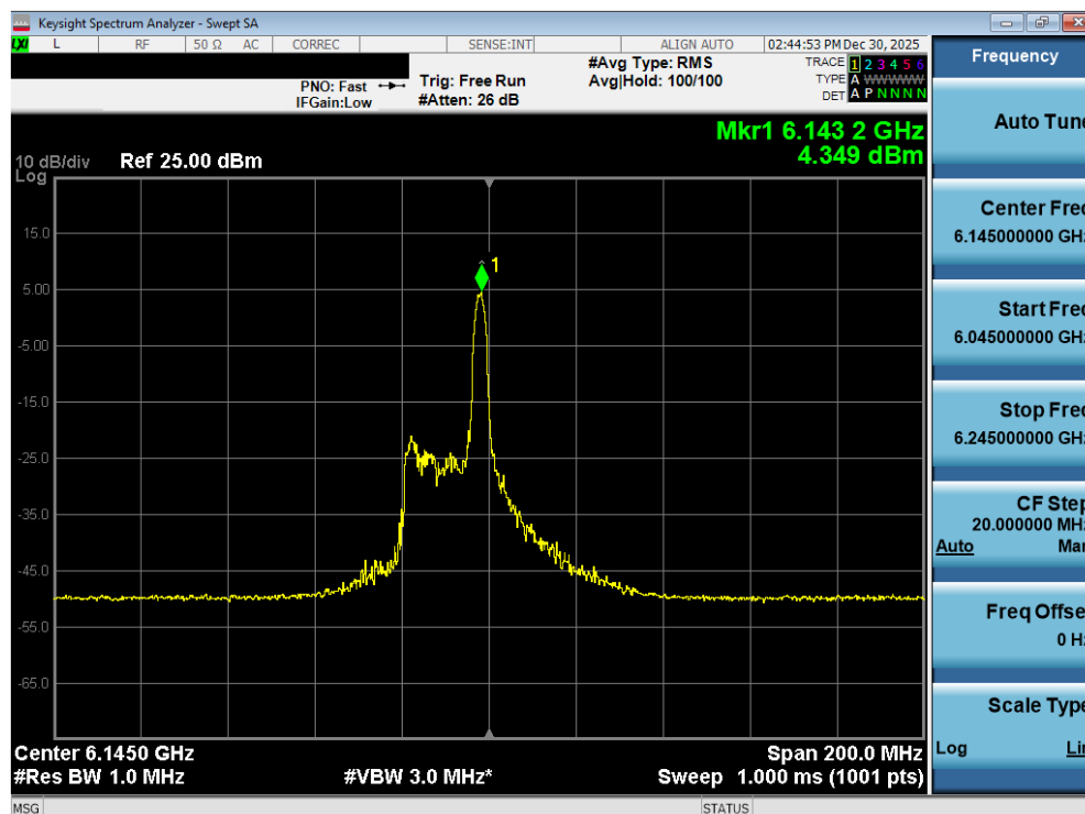
Plot 7-86. Power Spectral Density Plot MIMO ANT2 (80MHz 802.11ax/be (26 Tones) (UNII Band 5) – Ch. 39) - SP
