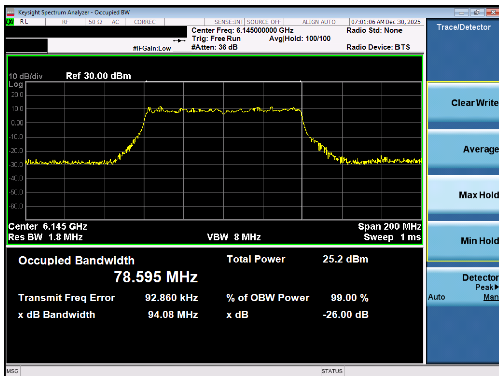
Plot 7-27. 26dB Bandwidth Plot MIMO ANT1 (80MHz 802.11ax/be (Full Tones) (UNII Band 5) – Ch. 39) – SP
