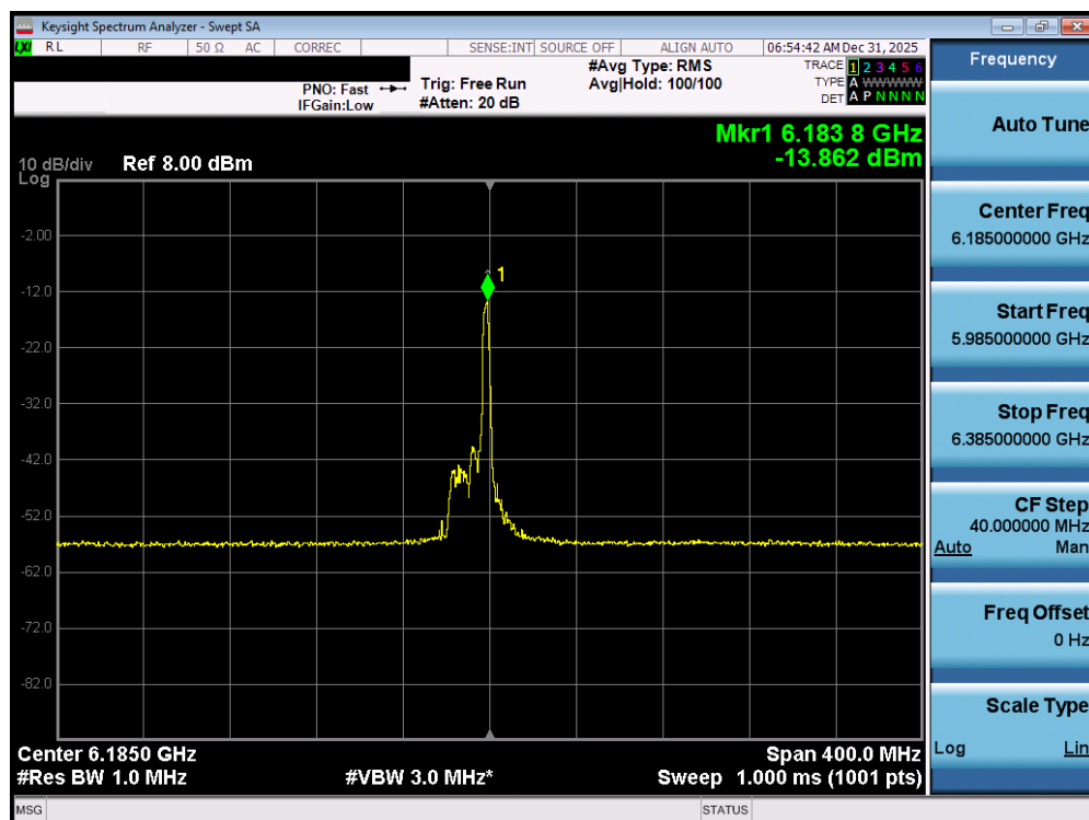
Plot 7-56. Power Spectral Density Plot MIMO ANT1 (160MHz 802.11ax/be (26 Tones) (UNII Band 5) – Ch. 47) - LPI
