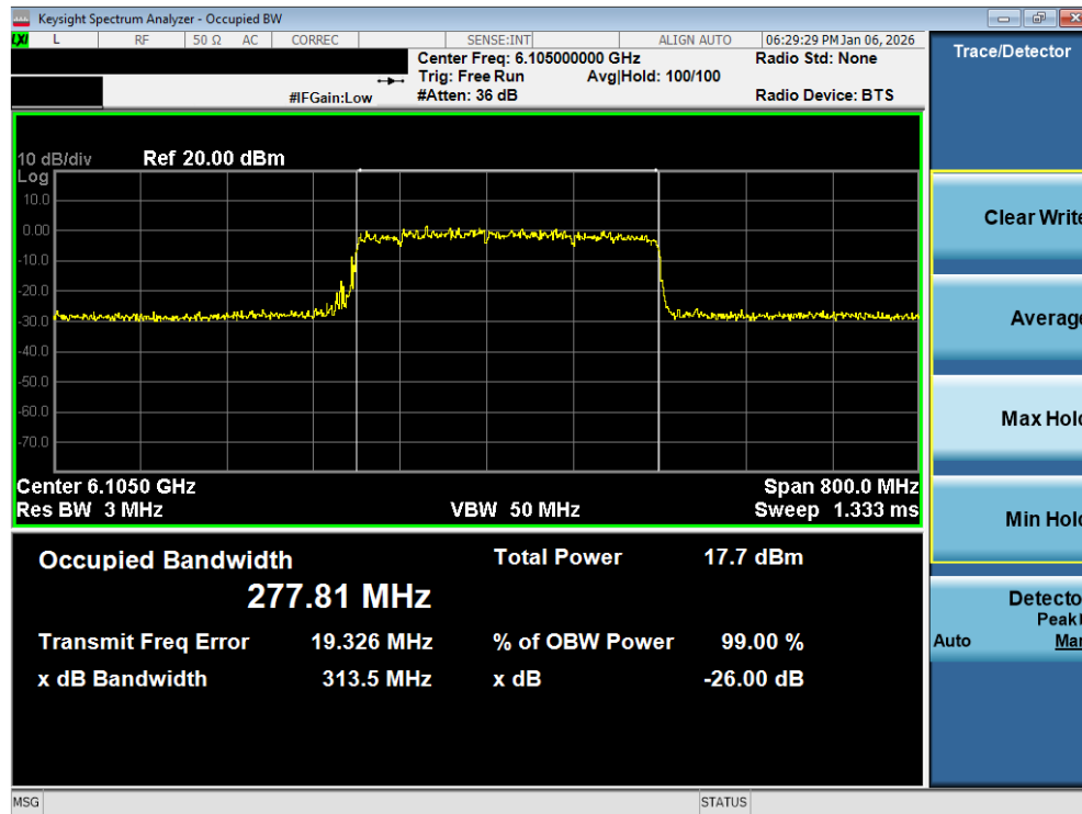
Plot 7-36. 26dB Bandwidth Plot MIMO ANT2 (320MHz 802.11be (3*996+484 Tones) (UNII Band 5) – Ch. 31) LPI
