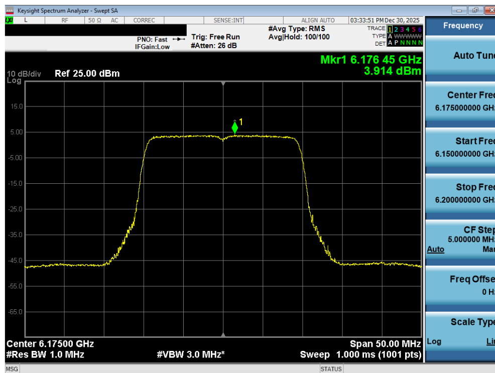
Plot 7-98. Power Spectral Density Plot MIMO ANT2 (20MHz 802.11ax/be (Full Tones) (UNII Band 5) – Ch. 45) - SP
