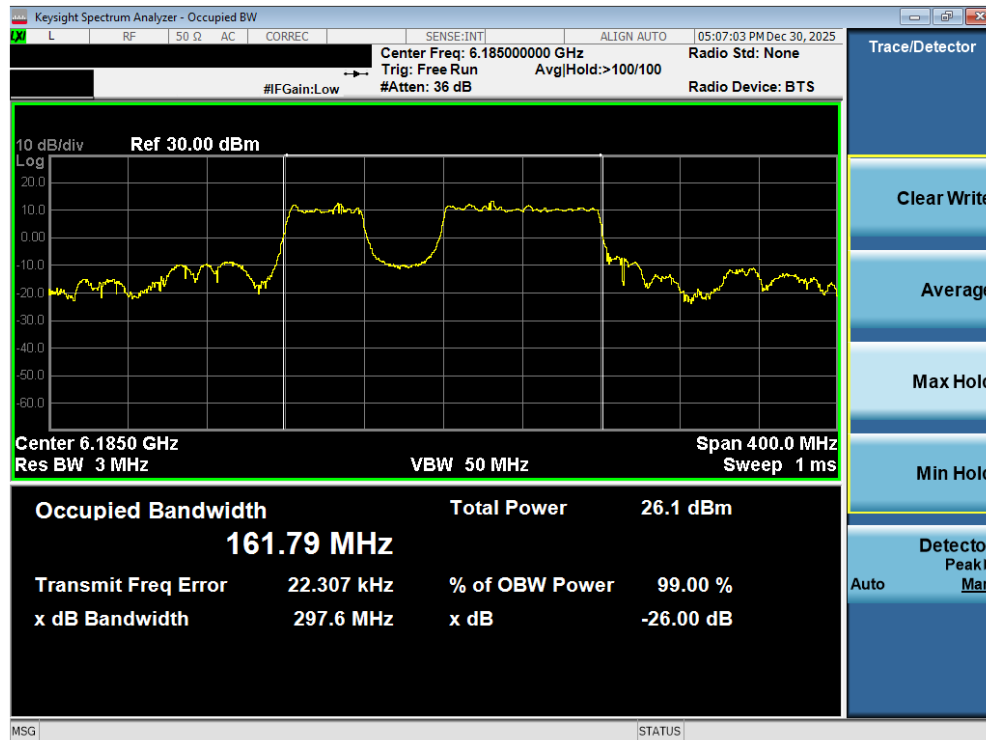
Plot 7-44. 26dB Bandwidth Plot MIMO ANT2 (160MHz 802.11be (996+484 Tones) (UNII Band 5) – Ch. 47) - SP
