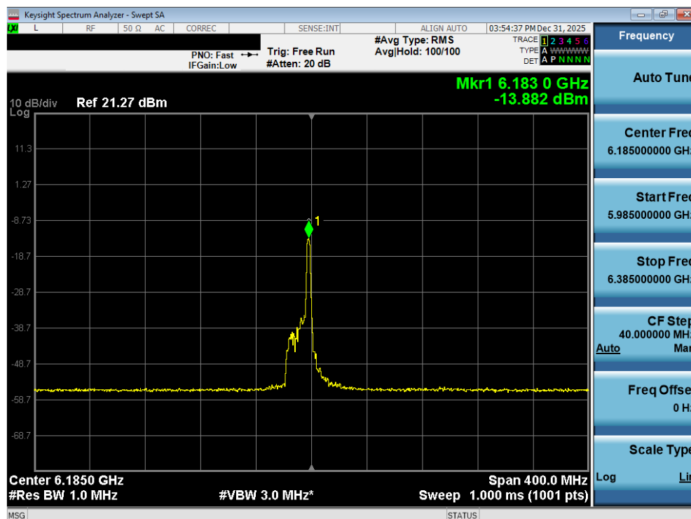
Plot 7-78. Power Spectral Density Plot MIMO ANT2 (160MHz 802.11ax/be (26 Tones) (UNII Band 5) – Ch. 47) - LPI
