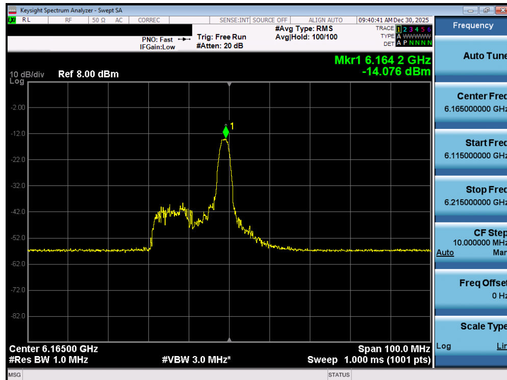
Plot 7-54. Power Spectral Density Plot MIMO ANT1 (40MHz 802.11ax/be (26 Tones) (UNII Band 5) – Ch. 43) - LPI
