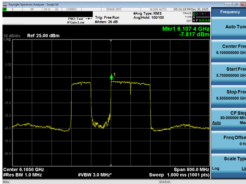
Plot 7-92. Power Spectral Density Plot MIMO ANT2 (320MHz 802.11be (996x3 Tones) (UNII Band 5) – Ch. 31) – SP
