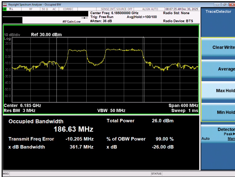
Plot 7-17. 26dB Bandwidth Plot MIMO ANT1 (160MHz 802.11be (996+484 Tones)) (UNII Band 5) – Ch. 47) - SP
