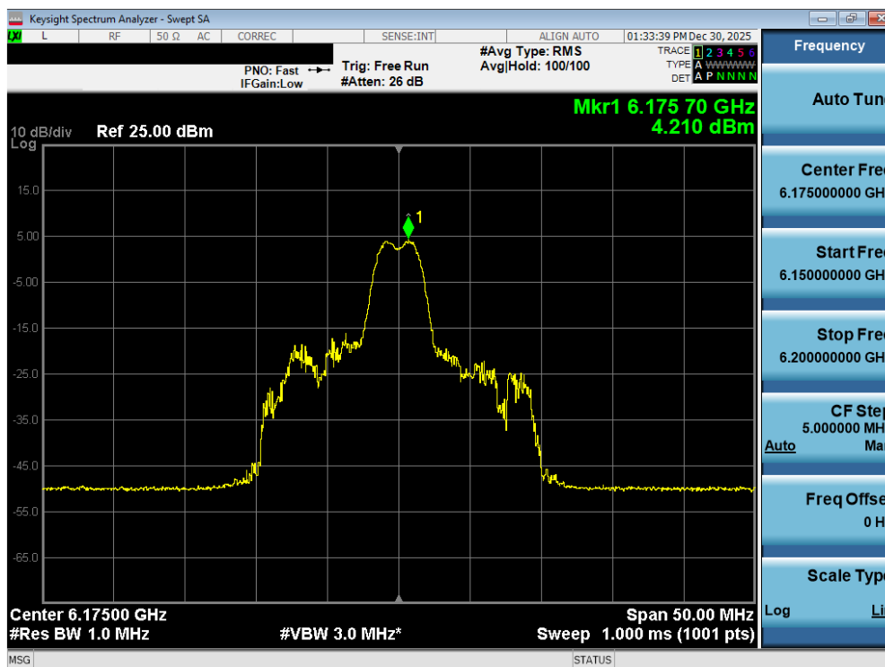
Plot 7-84. Power Spectral Density Plot MIMO ANT2 (20MHz 802.11ax/be (26 Tones) (UNII Band 5) – Ch. 45) - SP
