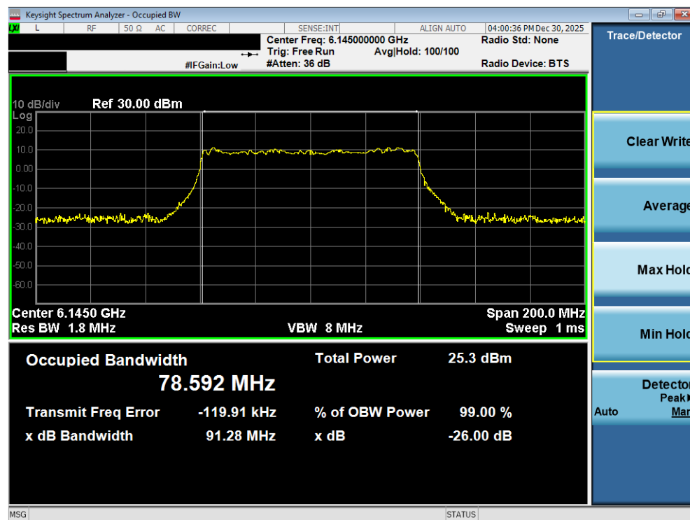
Plot 7-52. 26dB Bandwidth Plot MIMO ANT2 (80MHz 802.11ax/be (Full Tones) (UNII Band 5) – Ch. 39) - SP
