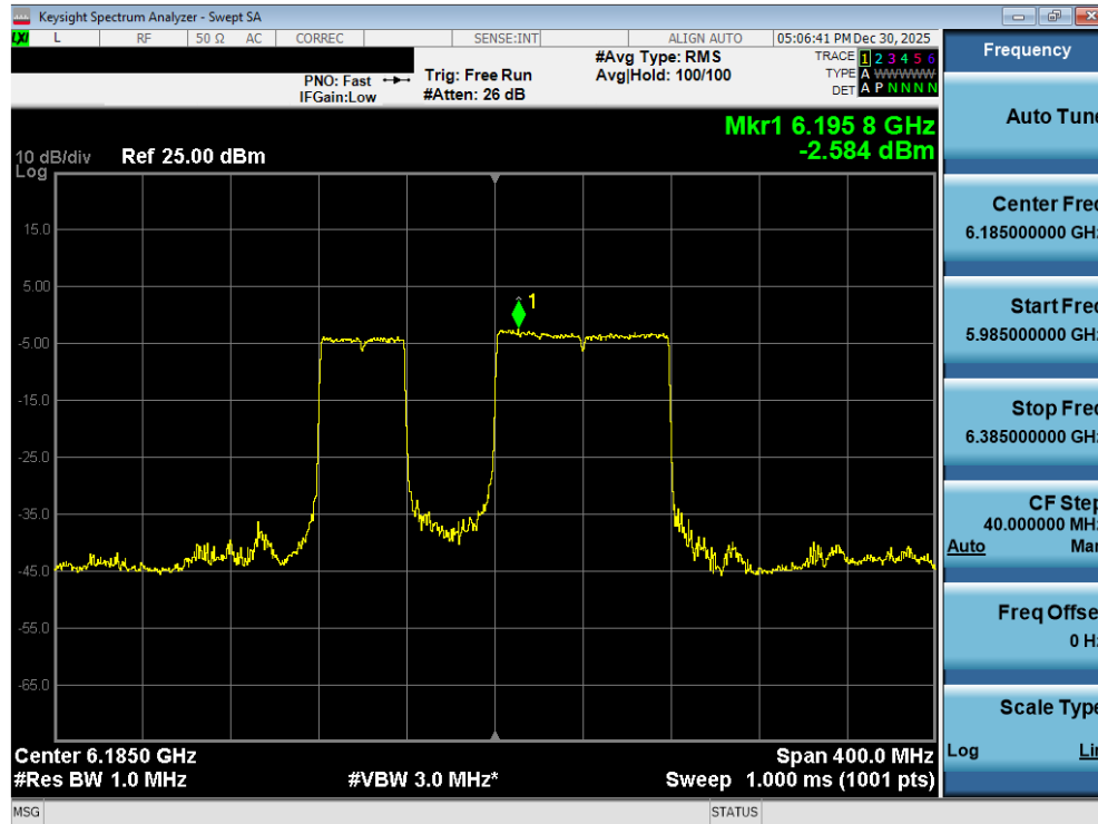
Plot 7-91. Power Spectral Density Plot MIMO ANT2 (160MHz 802.11be (996+484 Tones) (UNII Band 5) – Ch. 47) – SP
