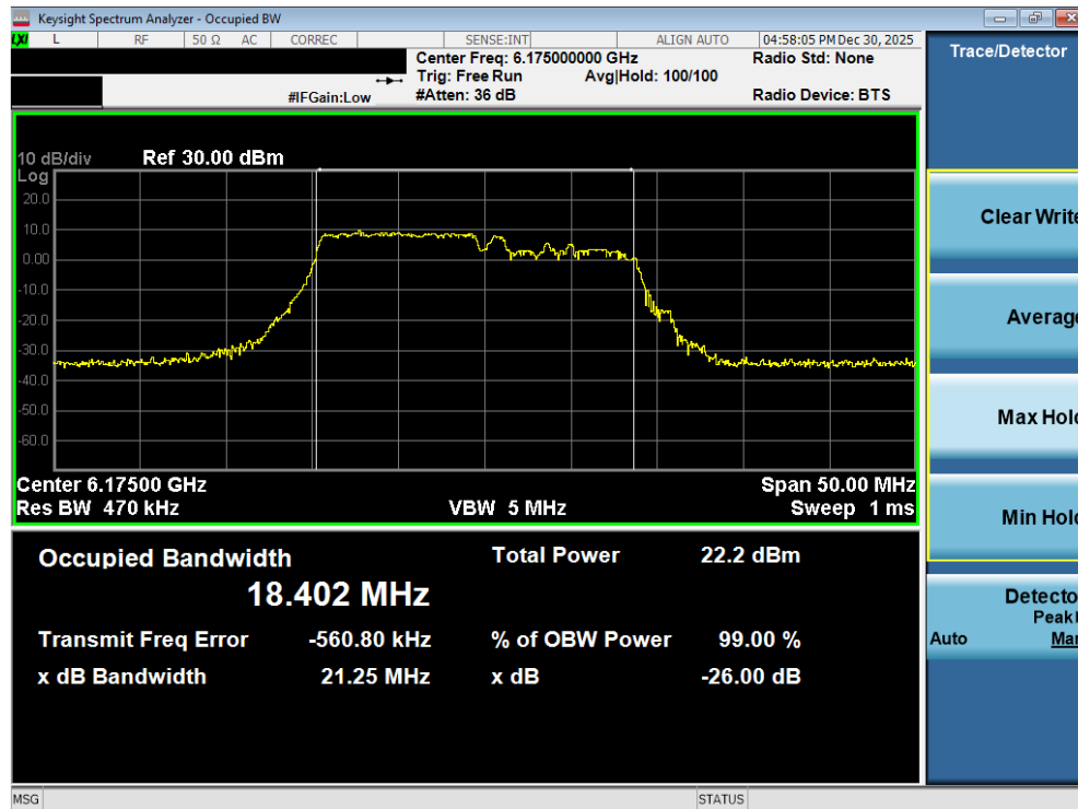
Plot 7-42. 26dB Bandwidth Plot MIMO ANT2 (20MHz 802.11be (106+26 Tones) (UNII Band 5) – Ch. 45) – SP
