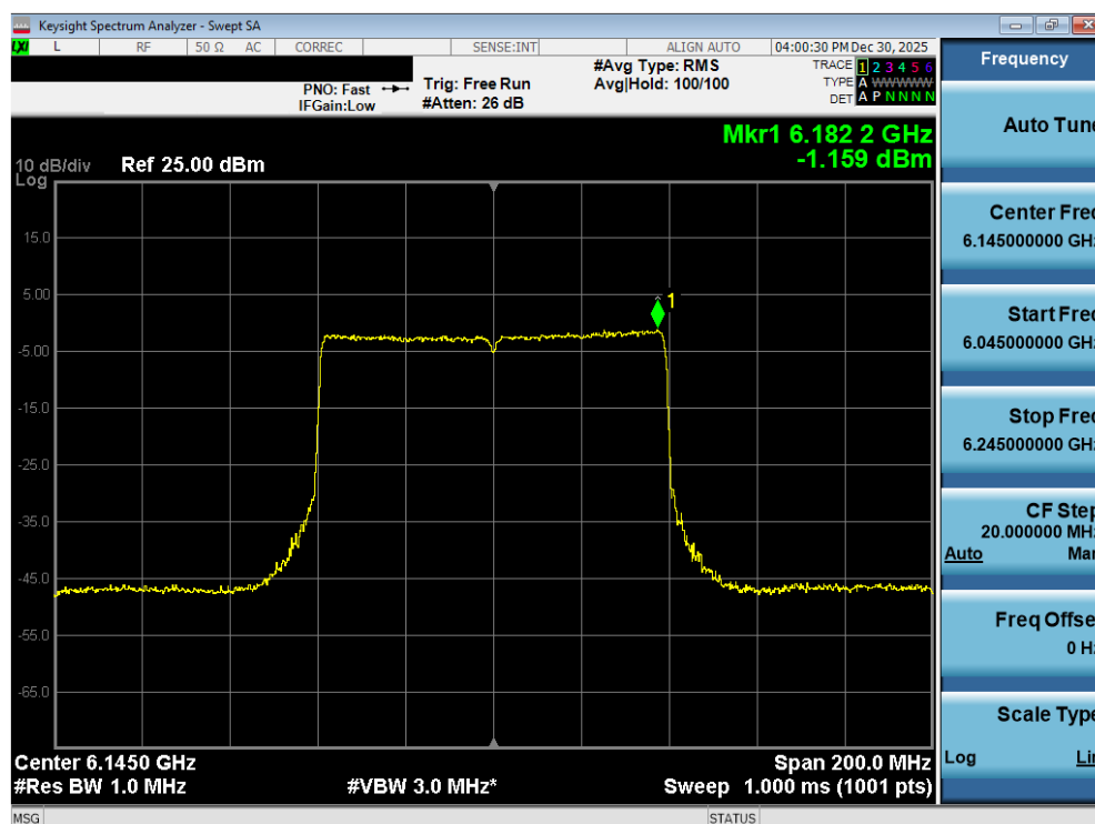
Plot 7-100. Power Spectral Density Plot MIMO ANT2 (80MHz 802.11ax/be (Full Tones) (UNII Band 5) – Ch. 39) - SP
