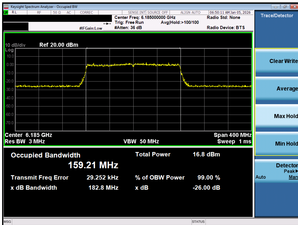
Plot 7-23. 26dB Bandwidth Plot MIMO ANT1 (160MHz 802.11ax/be (Full Tones) (UNII Band 5) – Ch. 47) - LPI
