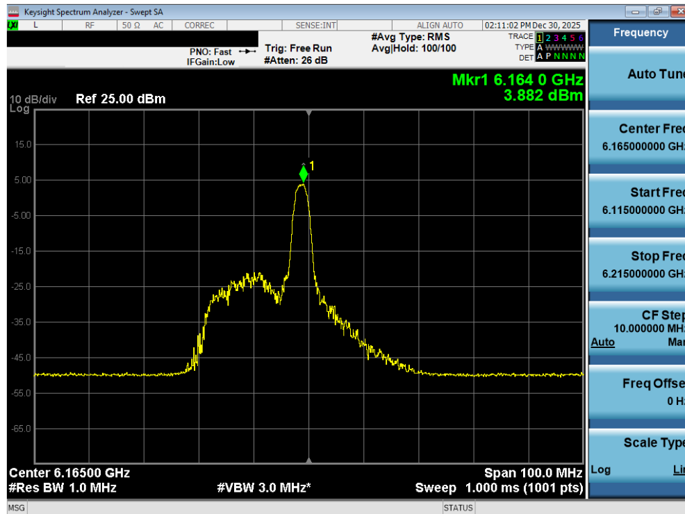
Plot 7-85. Power Spectral Density Plot MIMO ANT2 (40MHz 802.11ax/be (26 Tones) (UNII Band 5) – Ch. 43) - SP
