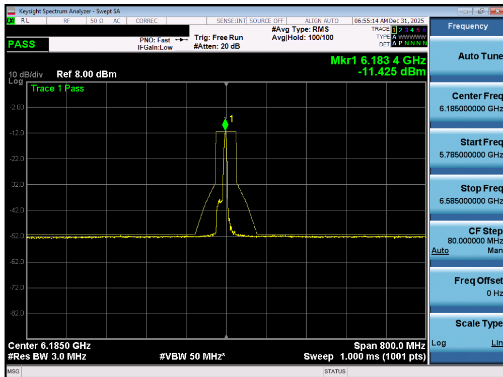
Plot 7-104. In Band Emissions Plot MIMO ANT1 (160MHz 802.11ax/be (26 Tones) (UNII Band 5) – Ch. 47) - LPI
