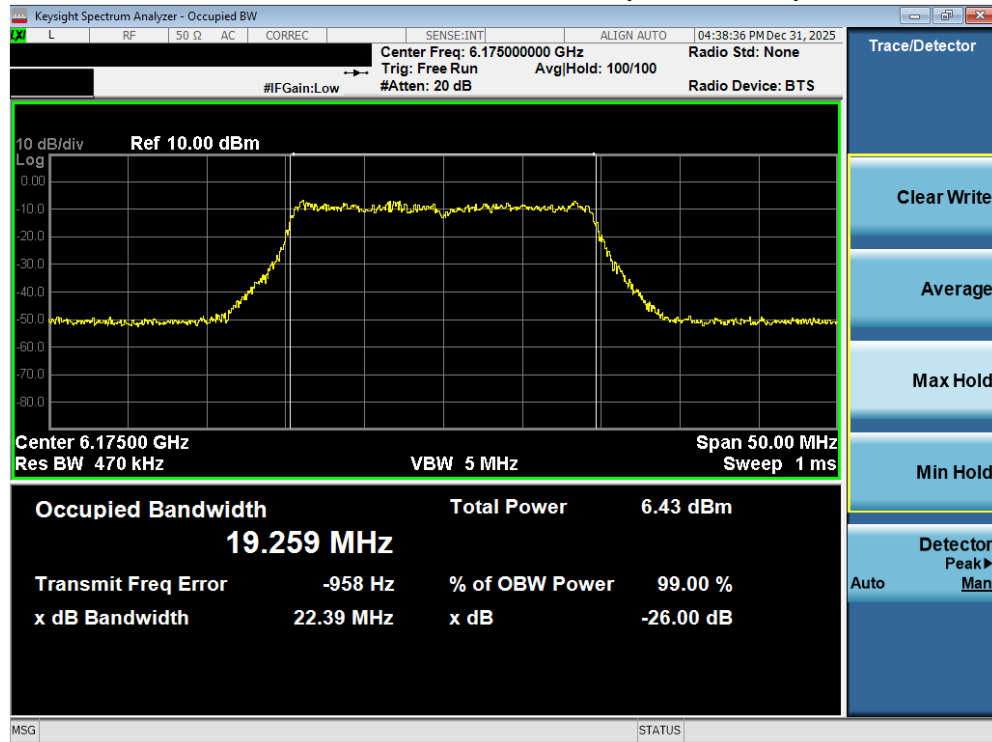
Plot 7-45. 26dB Bandwidth Plot MIMO ANT2 (20MHz 802.11ax/be (Full Tones) (UNII Band 5) – Ch. 45) - LPI
