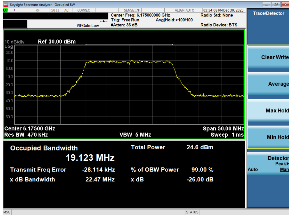
Plot 7-50. 26dB Bandwidth Plot MIMO ANT2 (20MHz 802.11ax/be (Full Tones) (UNII Band 5) – Ch. 45) - SP
