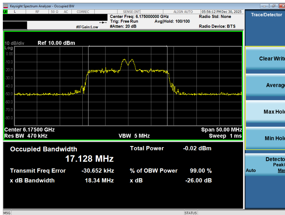
Plot 7-28. 26dB Bandwidth Plot MIMO ANT2 (20MHz 802.11ax/be (26 Tones) (UNII Band 5) – Ch. 45) - LPI
