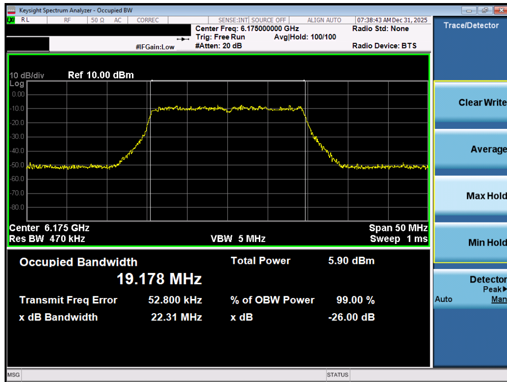
Plot 7-20. 26dB Bandwidth Plot MIMO ANT1 (20MHz 802.11ax/be (Full Tones) (UNII Band 5) – Ch. 45) – LPI
