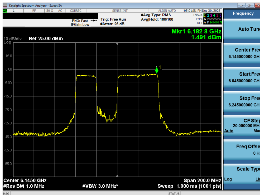
Plot 7-90. Power Spectral Density Plot MIMO ANT2 (80MHz 802.11be (484+242 Tones) (UNII Band 5) – Ch. 39) - SP
