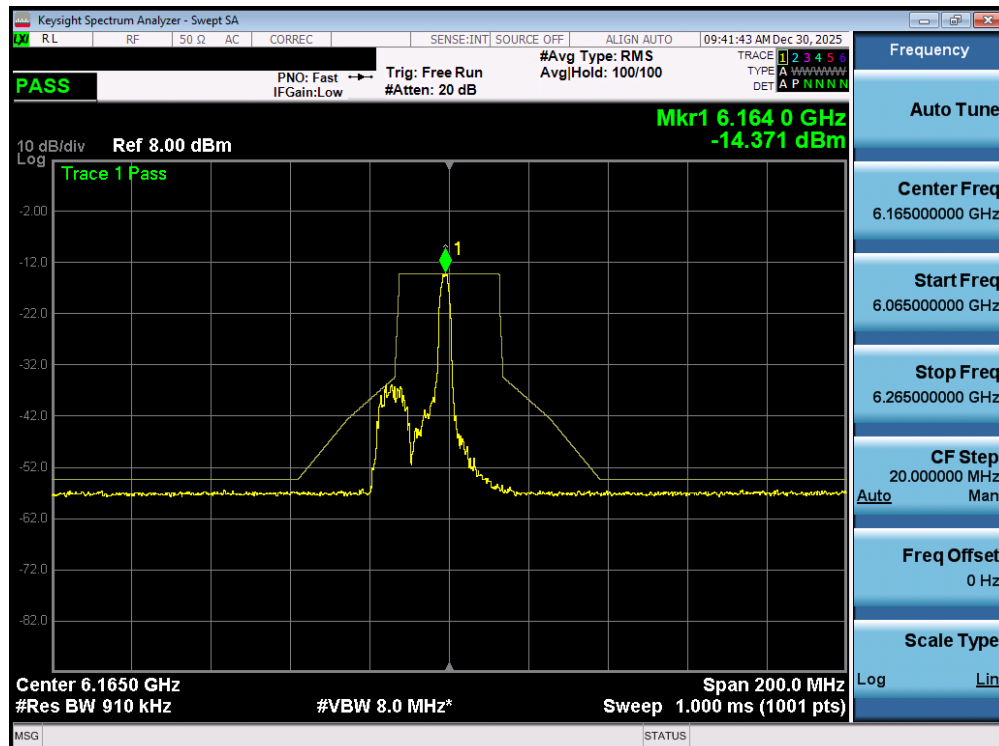
Plot 7-102. In Band Emissions Plot MIMO ANT1 (40MHz 802.11ax/be (26 Tones) (UNII Band 5) – Ch. 43) - LPI
