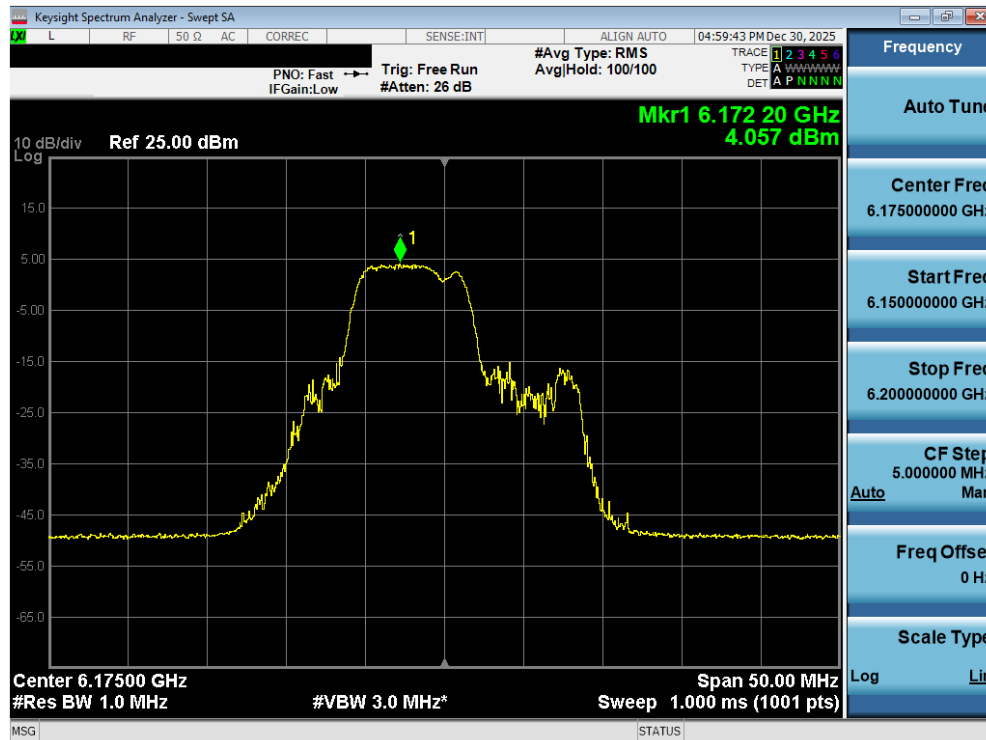
Plot 7-89. Power Spectral Density Plot MIMO ANT2 (20MHz 802.11be (52+26 Tones) (UNII Band 5) – Ch. 45) – SP
