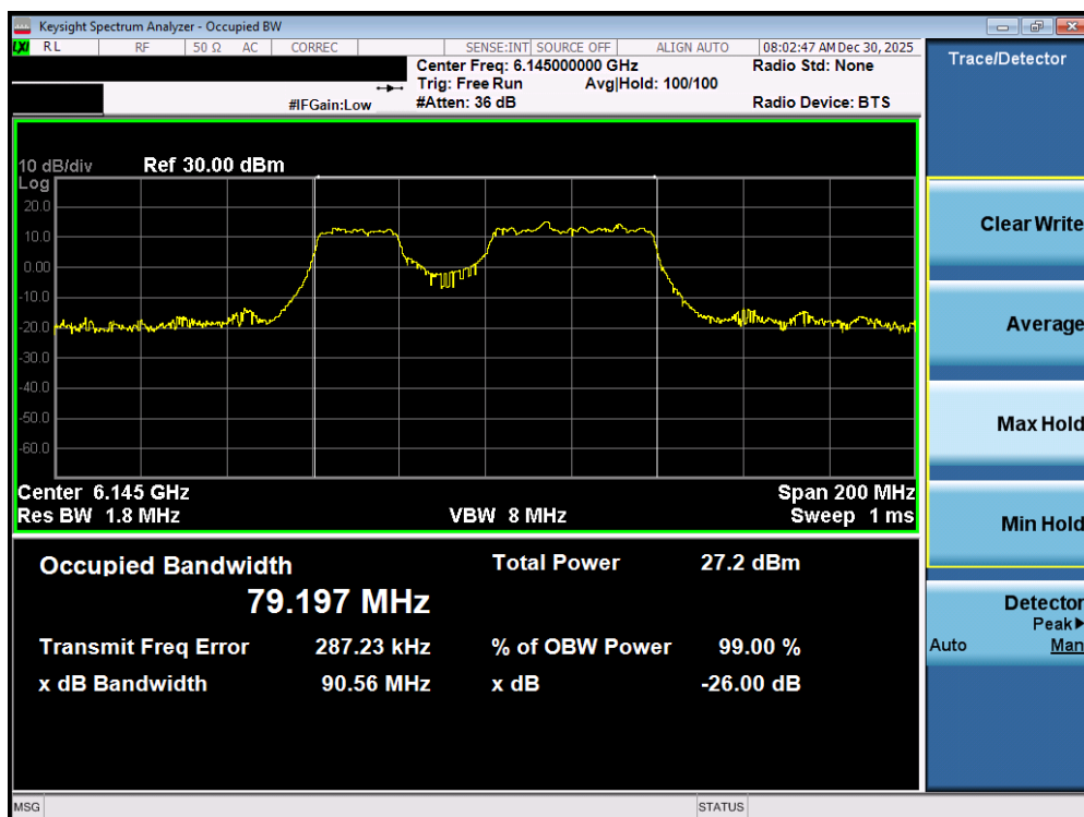
Plot 7-16. 26dB Bandwidth Plot MIMO ANT1 (80MHz 802.11be (484+242 Tones) (UNII Band 5) – Ch. 39) - SP
