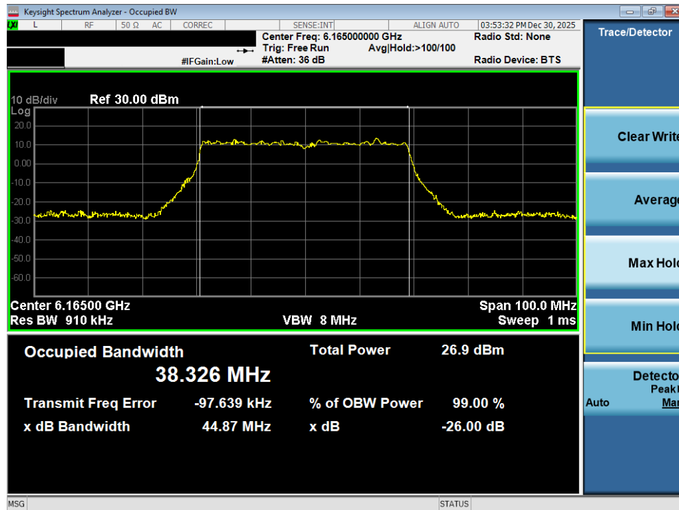
Plot 7-51. 26dB Bandwidth Plot MIMO ANT2 (40MHz 802.11ax/be (Full Tones) (UNII Band 5) – Ch. 43) – SP
