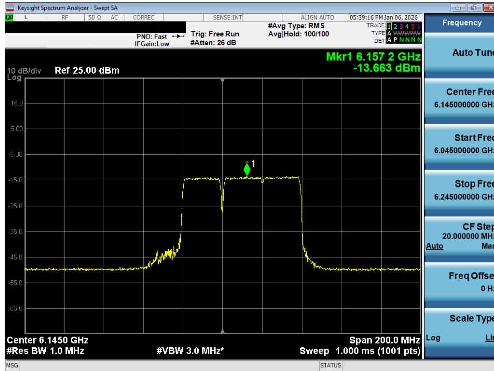
Plot 7-81. Power Spectral Density Plot MIMO ANT2 (80MHz 802.11be (484+242 Tones) (UNII Band 5) – Ch. 39) - LPI
