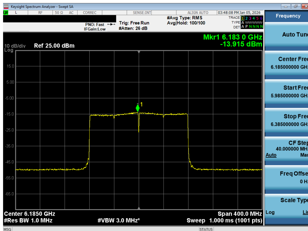
Plot 7-96. Power Spectral Density Plot MIMO ANT2 (160MHz 802.11ax/be (Full Tones) (UNII Band 5) – Ch. 47) - LPI
