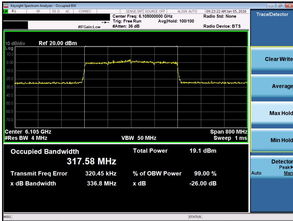
Plot 7-24. 26dB Bandwidth Plot MIMO ANT1 (320MHz 802.11be (Full Tones) (UNII Band 5) – Ch. 31) - LPI
