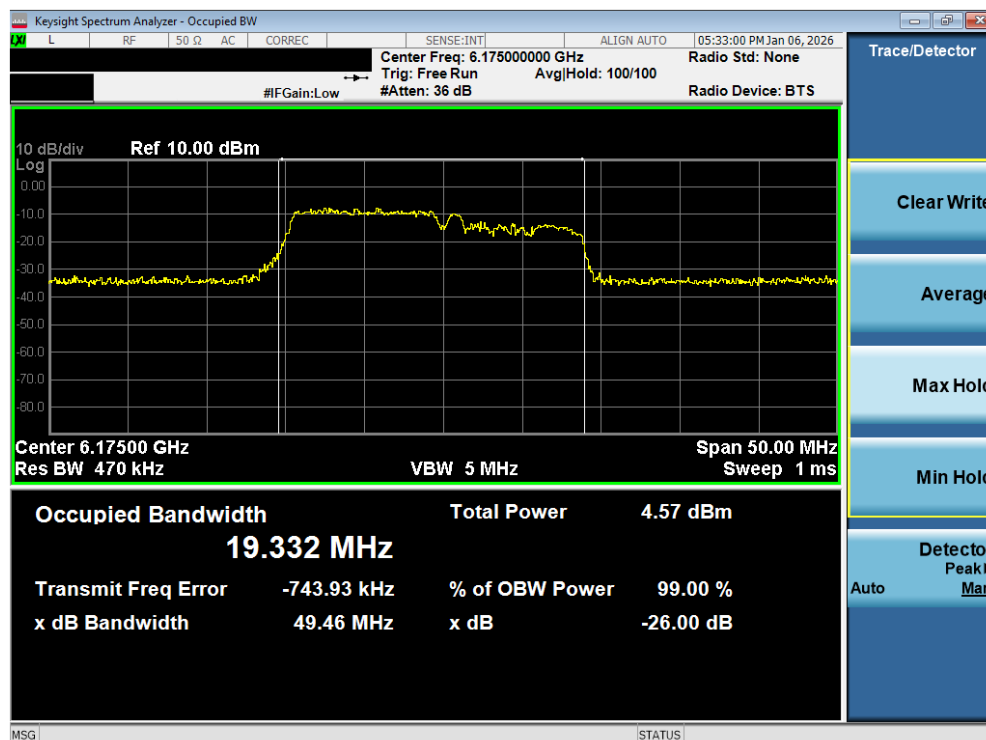
Plot 7-33. 26dB Bandwidth Plot MIMO ANT2 (20MHz 802.11be (106+26 Tones) (UNII Band 5) – Ch. 45) - LPI
