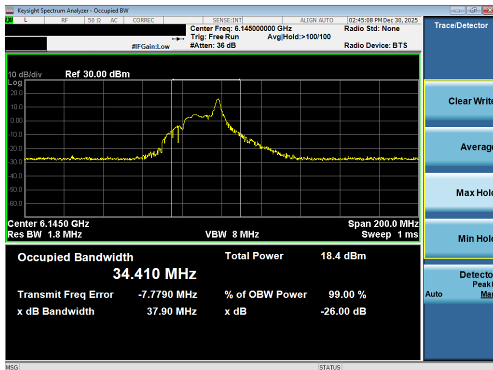
Plot 7-39. 26dB Bandwidth Plot MIMO ANT2 (80MHz 802.11ax/be (26 Tones) (UNII Band 5) – Ch. 39) - SP
