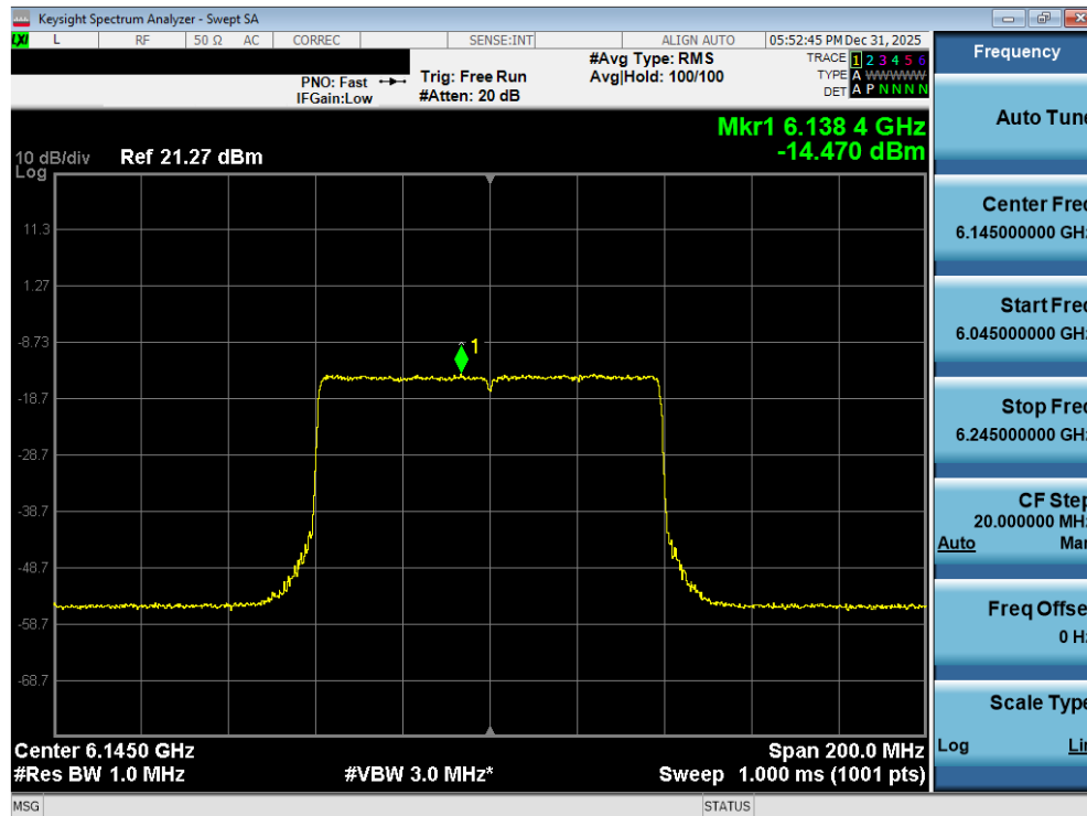
Plot 7-95. Power Spectral Density Plot MIMO ANT2 (80MHz 802.11ax/be (Full Tones) (UNII Band 5) – Ch. 39) - LPI
