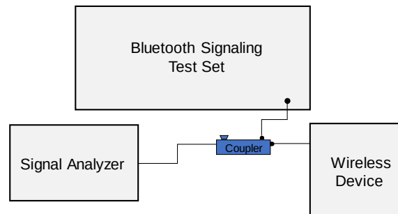
Figure 8-10 Power Measurement Setup
