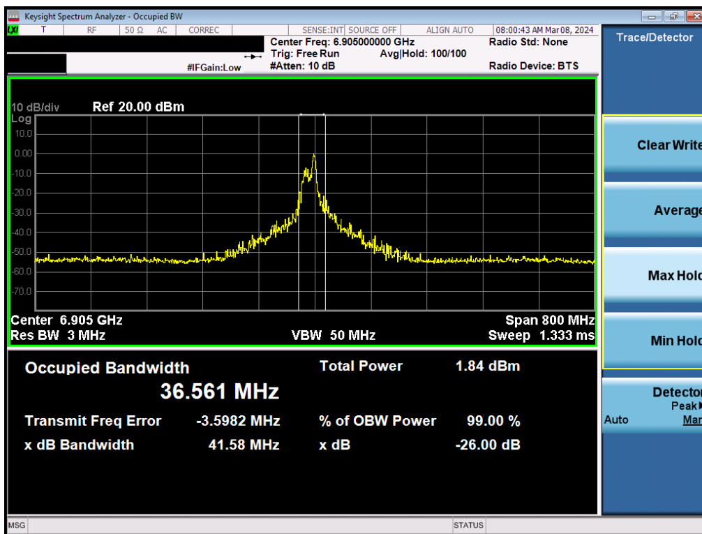
Plot 7-20. Occupied Bandwidth Plot MIMO ANT1 (320MHz BW 802. 11be (26 Tones) (UNII Band 8) – Ch. 191)
