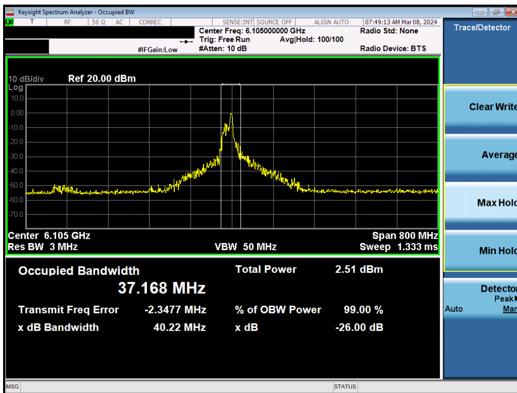
Plot 7-5. Occupied Bandwidth Plot MIMO ANT1 (320MHz BW 802. 11be (26 Tones) (UNII Band 5) – Ch. 31)
