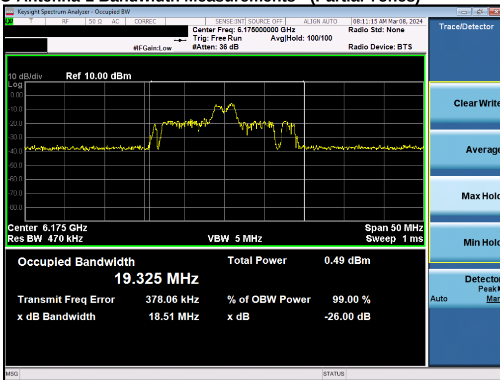
Plot 7-1. Occupied Bandwidth Plot MIMO ANT1 (20MHz BW 802.11be (26 Tones) (UNII Band 5) – Ch. 45)
