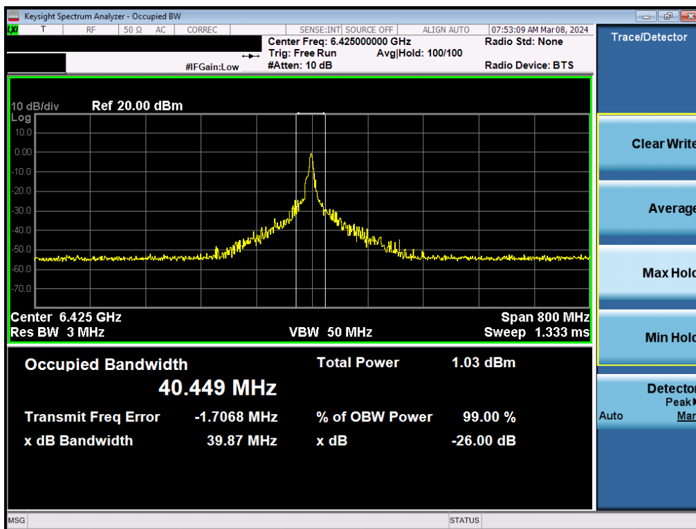
Plot 7-10. Occupied Bandwidth Plot MIMO ANT1 (320MHz BW 802. 11be (26 Tones) (UNII Band 6) – Ch. 95)
