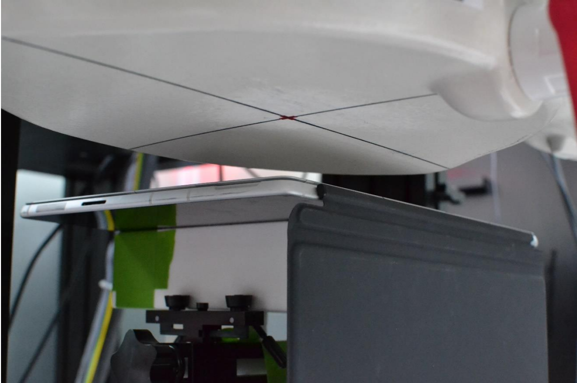
SAR Test Setup Photo 13 – Laptop, Back Side at 25mm – Antenna 8
