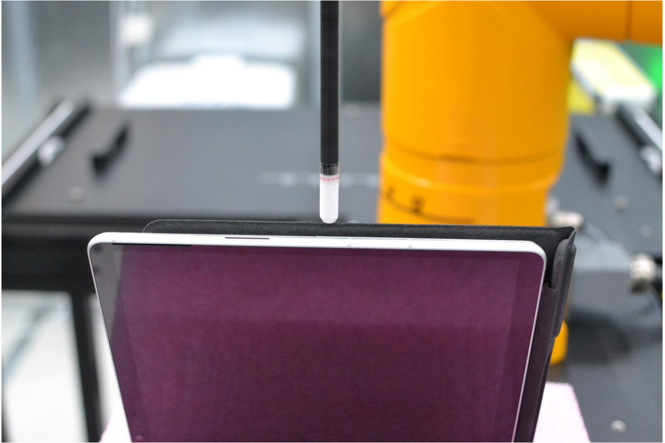
Near Field Power Density Test Setup Photo 41 – Right Edge with keyboard accessory at 2 mm
