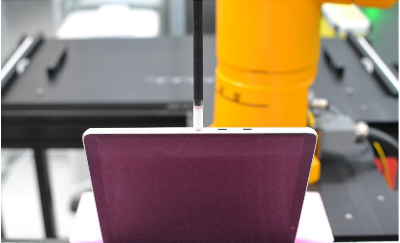
Near Field Power Density Test Setup Photo 44 – Left Edge at 2 mm
