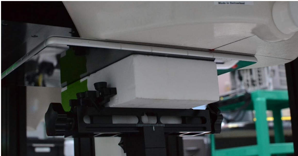
SAR Test Setup Photo 1 – Tablet, Back Side at 0 mm – Antenna 1 & 2
