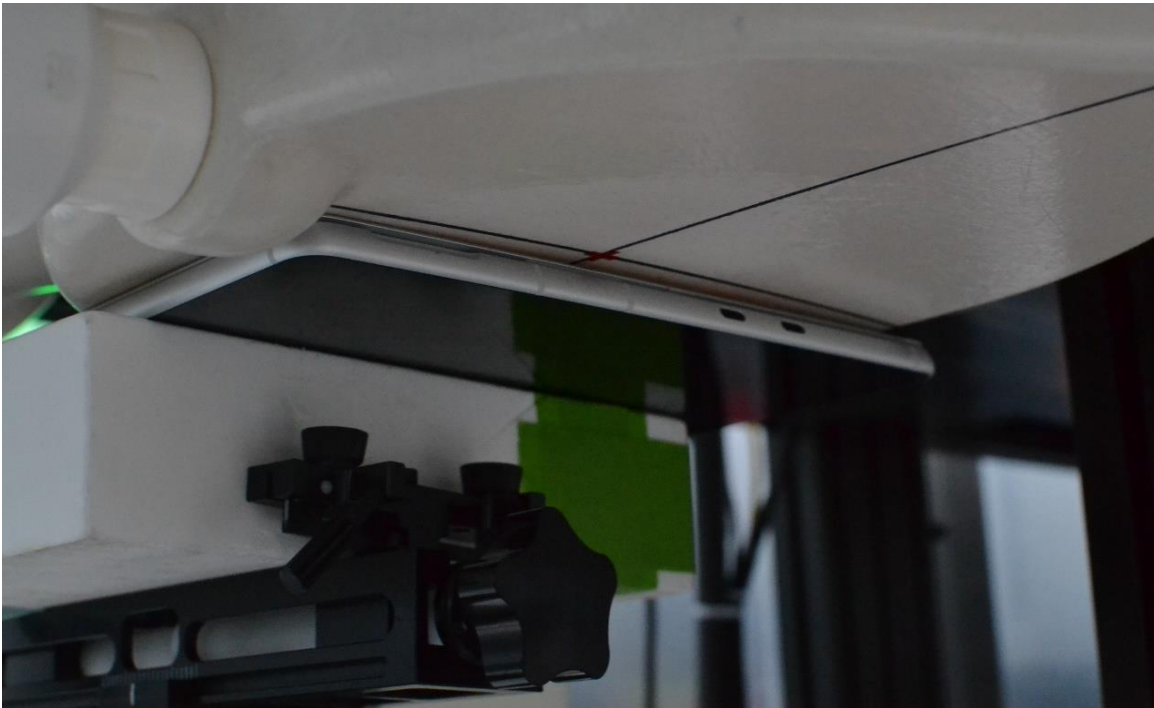
SAR Test Setup Photo 8 – Tablet, Back Side at 0mm – Antenna 6
