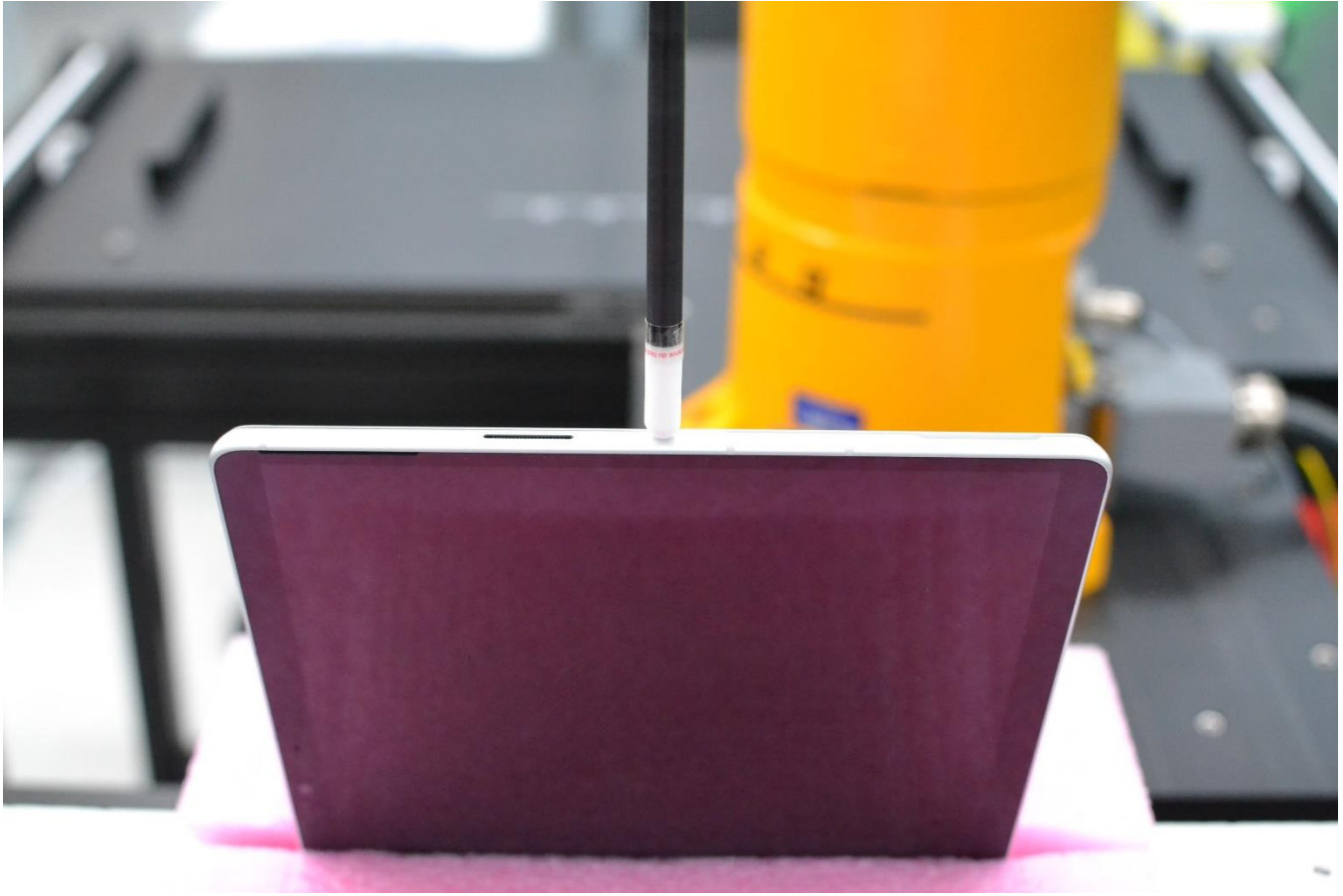
Near Field Power Density Test Setup Photo 40 – Right Edge at 2 mm
