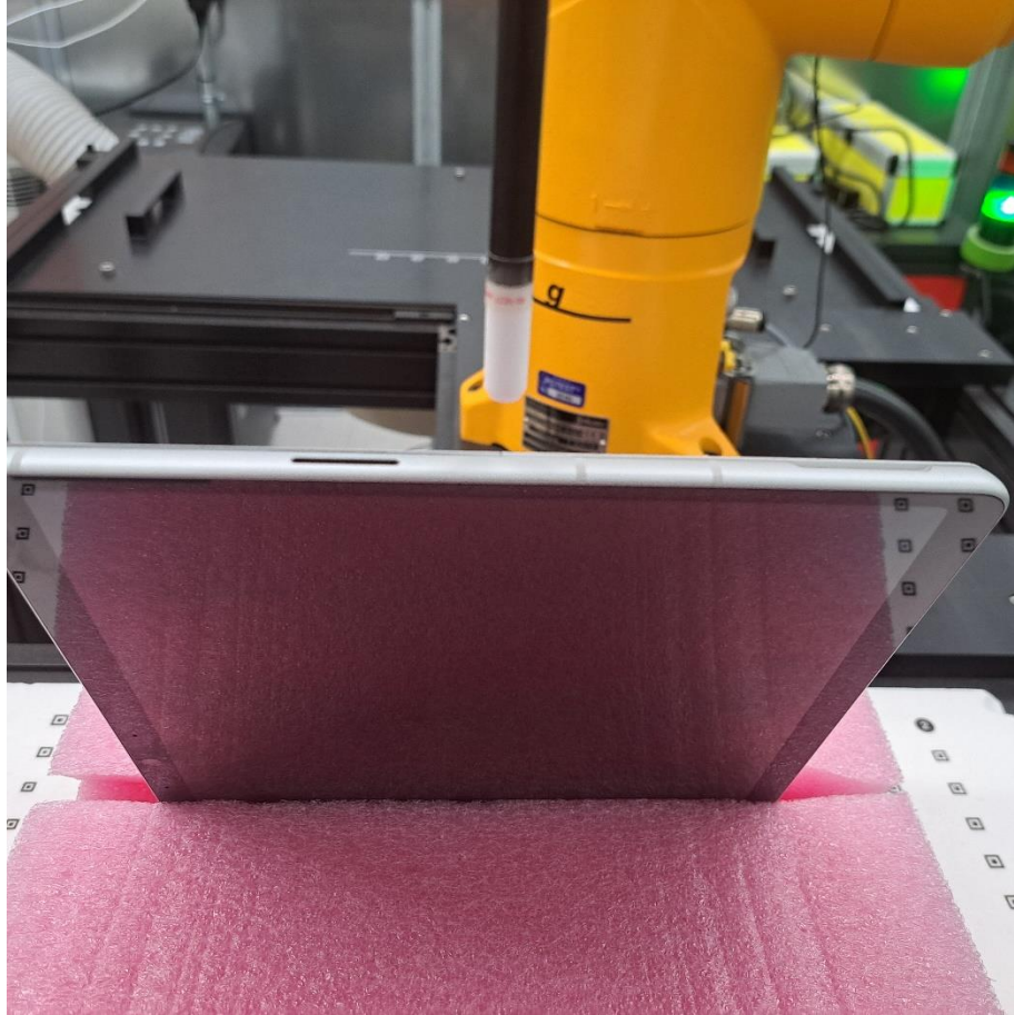
Near Field Power Density Test Setup Photo 42 – Right Edge at 9.27 mm
