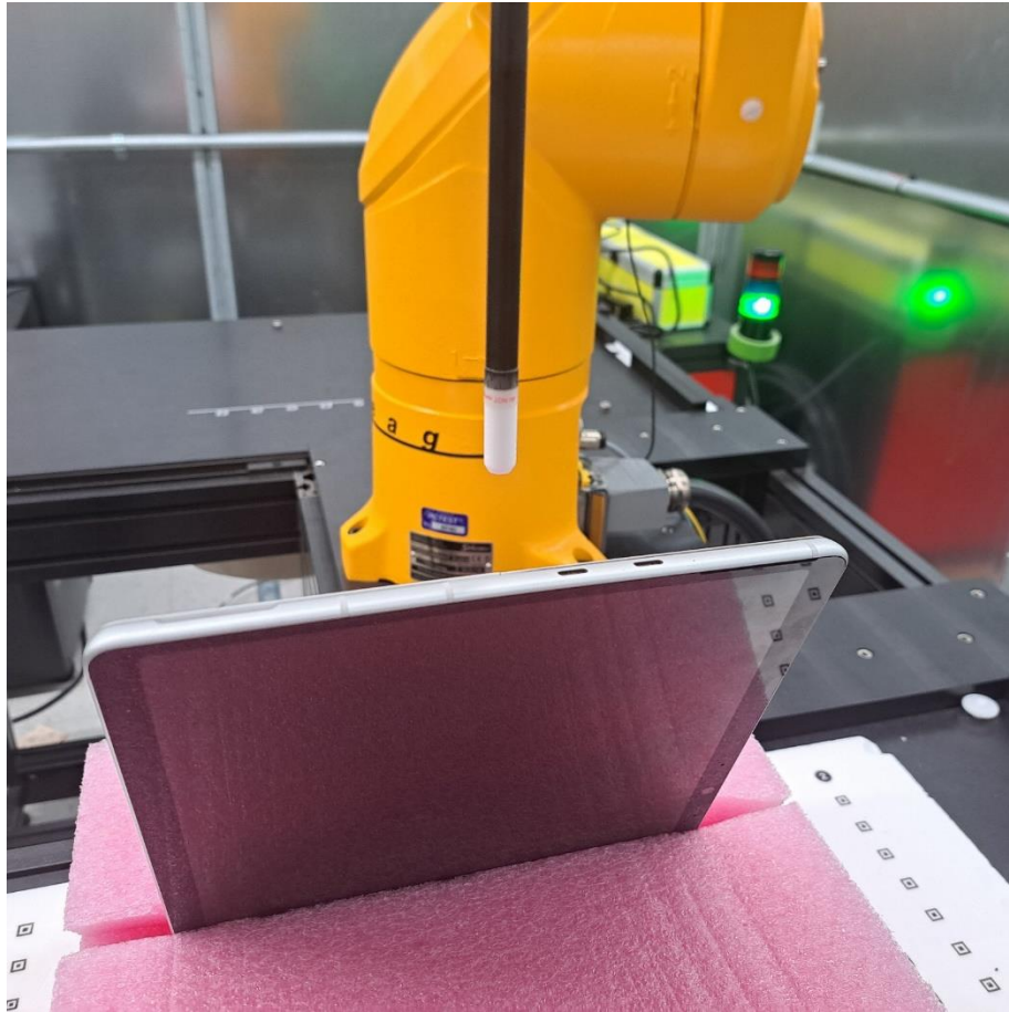
Near Field Power Density Test Setup Photo 47– Left Edge at 25 mm
