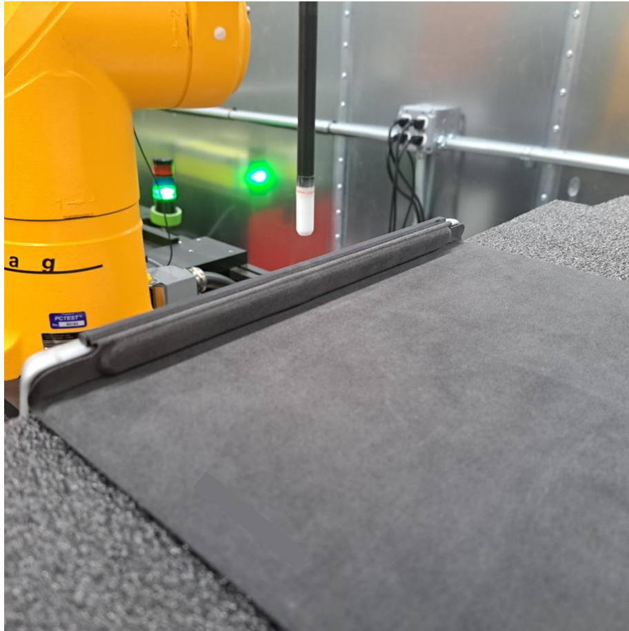
Near Field Power Density Test Setup Photo 49 – Laptop Bottom Edge at 8.94 mm
