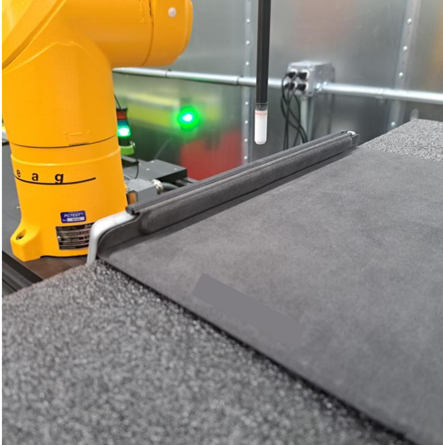
Near Field Power Density Test Setup Photo 50 – Laptop Bottom Edge at 10.02 mm
