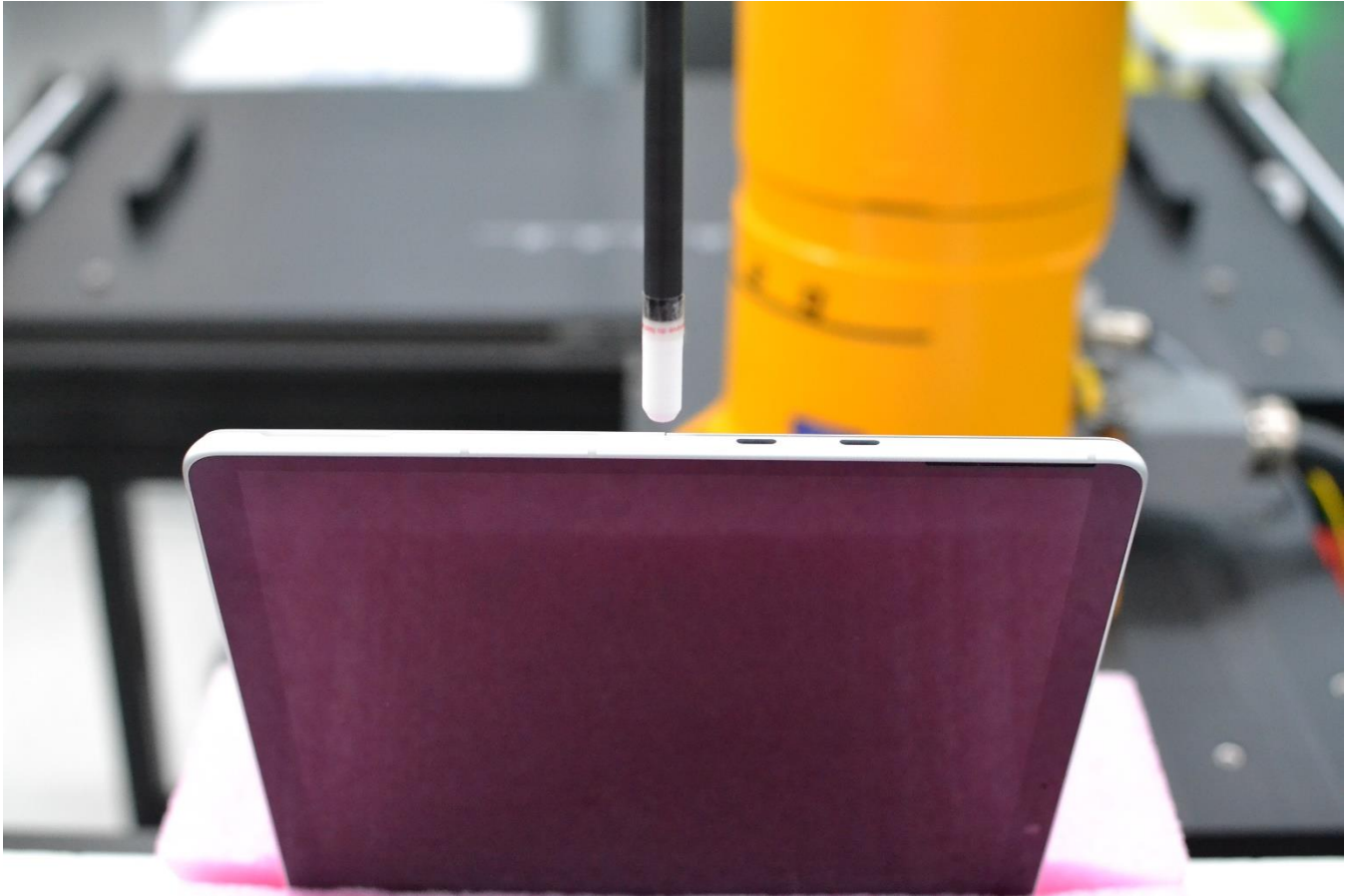
Near Field Power Density Test Setup Photo 46 – Left Edge at 8.54 mm
