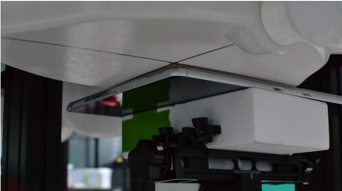
SAR Test Setup Photo 12 – Tablet, Back Side at 0mm – Antenna 8
