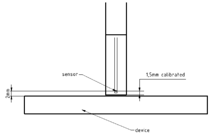
Figure K-3 EUmWVx Probe
