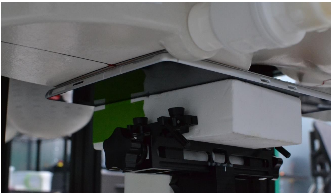
SAR Test Setup Photo 10 – Tablet, Back Side at 0mm – Antenna 7
