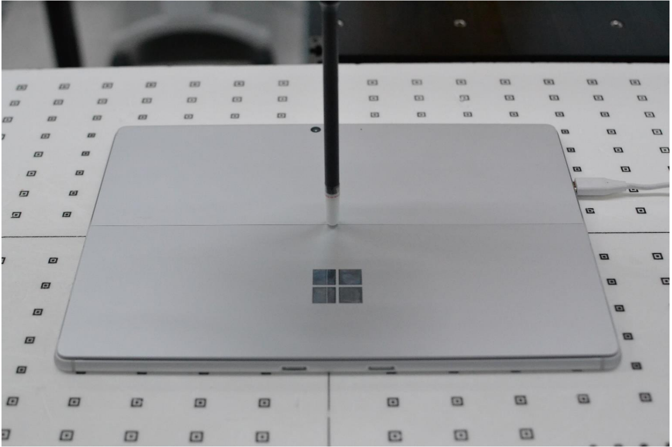
Near Field Power Density Test Setup Photo 38 – Back Side at 2 mm
