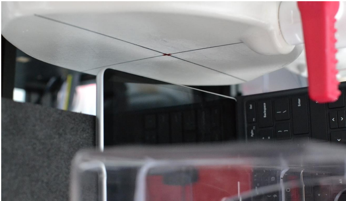
SAR Test Setup Photo 34 – Laptop, Right Edge at 25 mm – All Antennas
