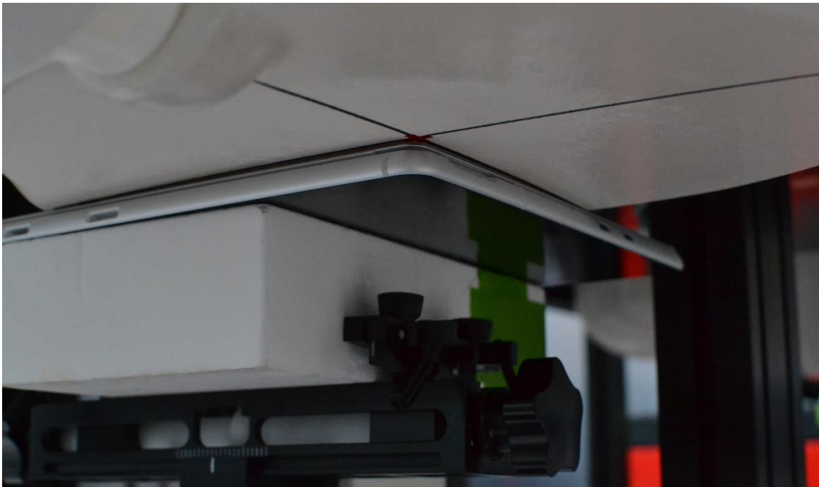
SAR Test Setup Photo 6 – Tablet, Back Side at 0mm – Antenna 5
