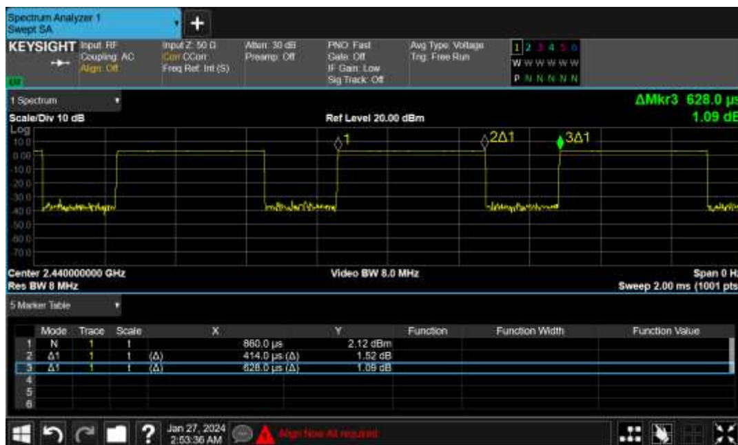
Figure 8.1 Duty Cycle 1 Mbps 2440MHz (Ch.0)
