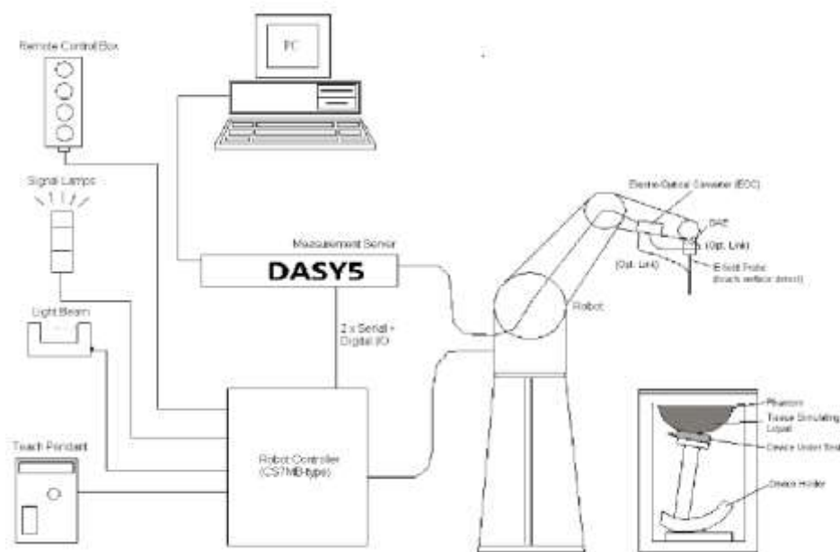
DASY5 System Setup
