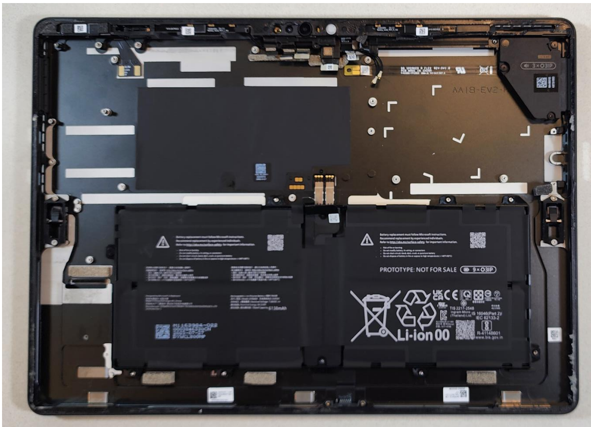
Model 2085 Internal Photographs
