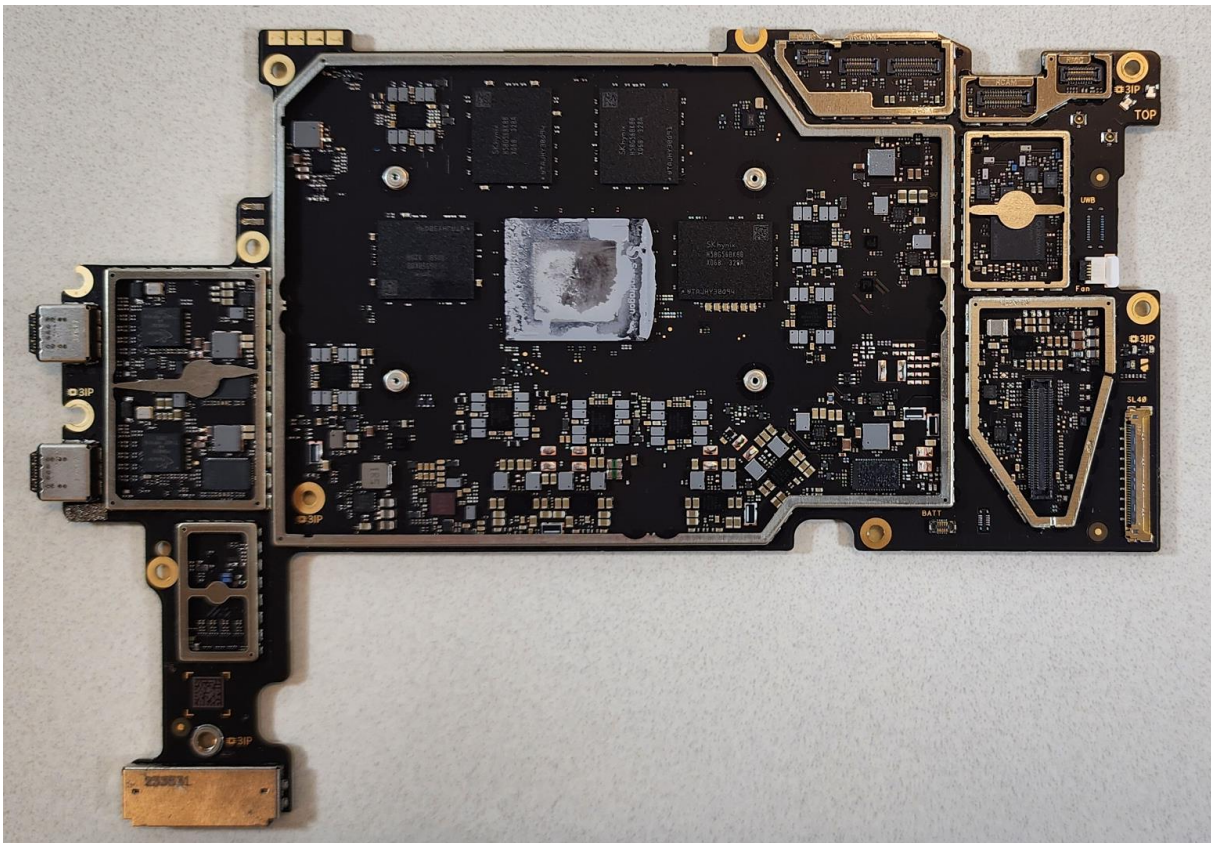
Model 2085 Internal Photographs
