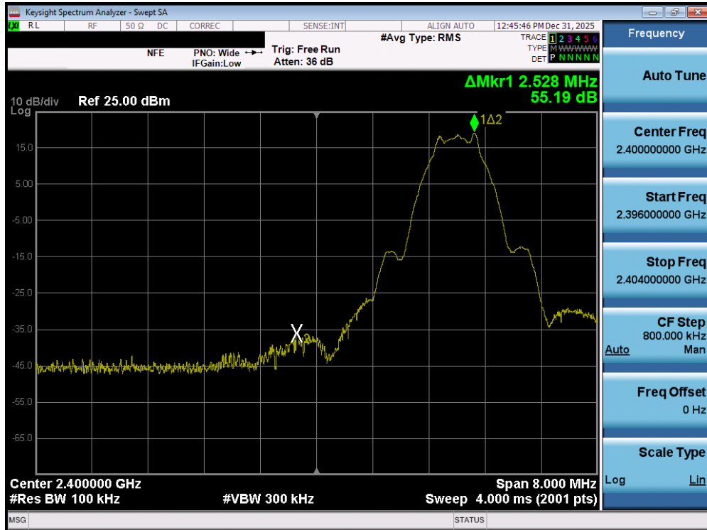
Plot 7-133. Band Edge Plot (Bluetooth (LE), 1Mbps – Ch. 37) – SISO ANT2
