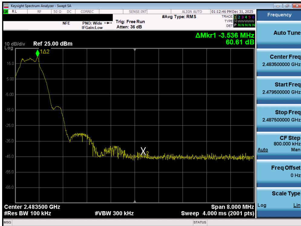
Plot 7-134. Band Edge Plot (Bluetooth (LE), 1Mbps – Ch. 39) – SISO ANT2
