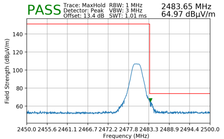
Plot 7-180. Radiated Restricted Upper Band Edge Measurement (Peak) – SISO ANT1 – 2M
