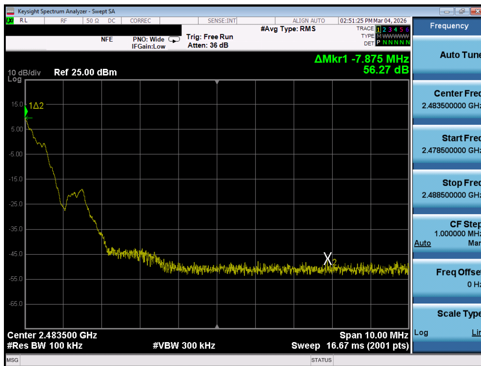
Plot 7-144. Band Edge Plot (Bluetooth (LE), 2Mbps - Ch. 36) - DUAL ANT2
