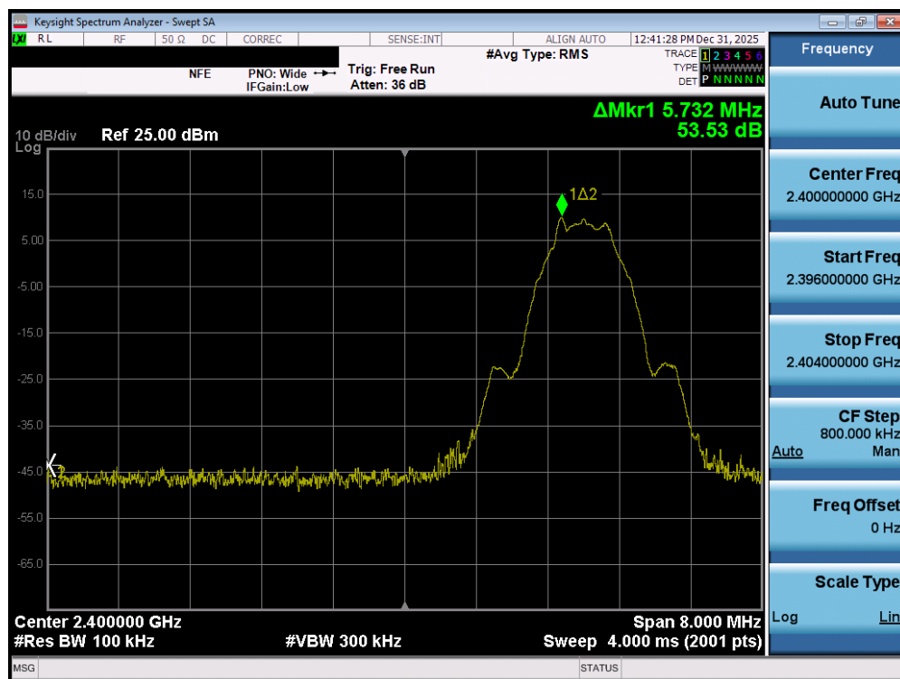
Plot 7-131. Band Edge Plot (Bluetooth (LE), 500kbps – Ch. 37) – SISO ANT2
