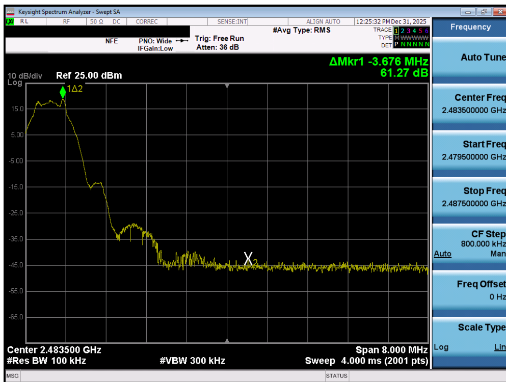
Plot 7-126. Band Edge Plot (Bluetooth (LE), 1Mbps – Ch. 39) – SISO ANT1
