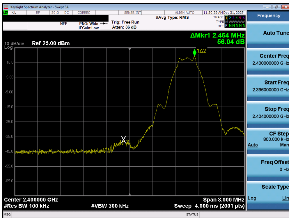
Plot 7-125. Band Edge Plot (Bluetooth (LE), 1Mbps – Ch. 37) – SISO ANT1
