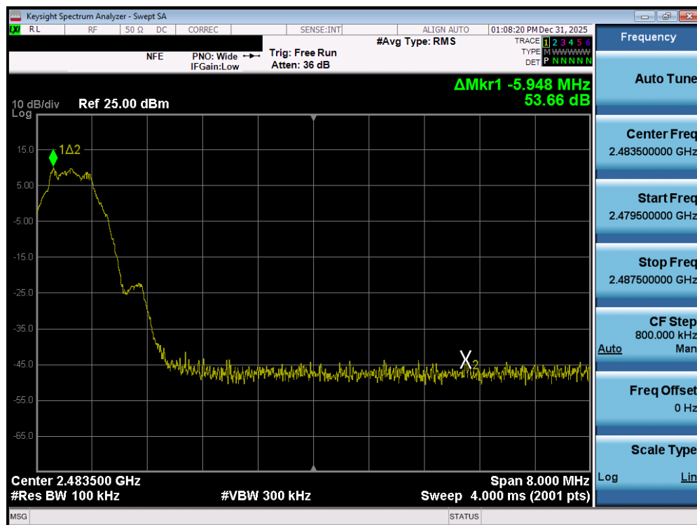
Plot 7-132. Band Edge Plot (Bluetooth (LE), 500kbps – Ch. 39) – SISO ANT2
