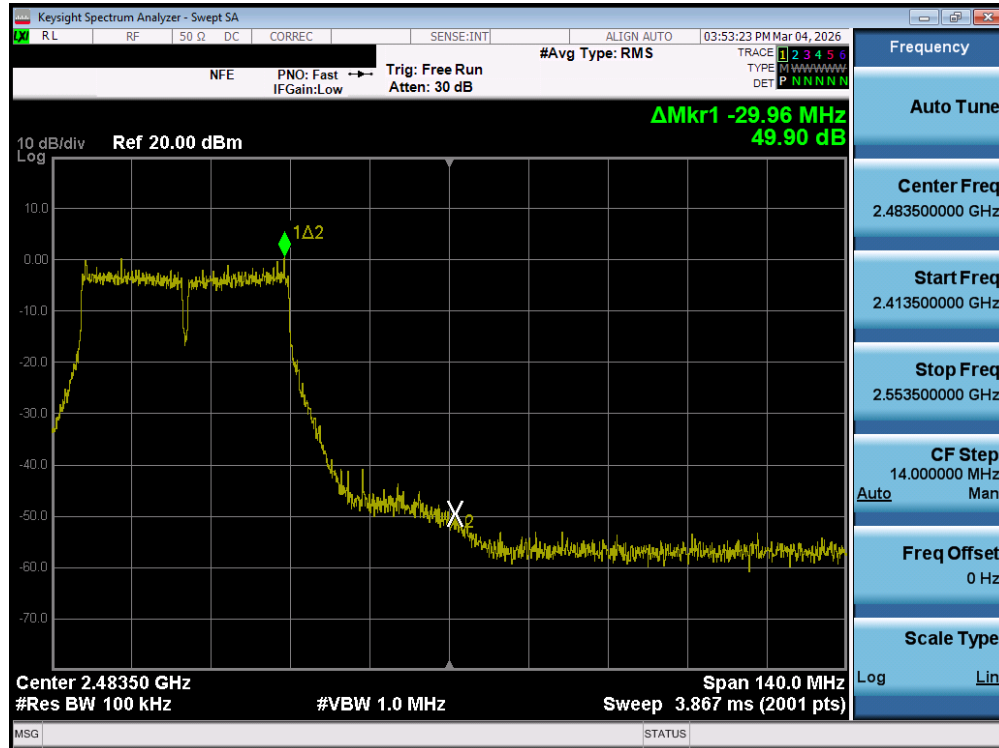
Plot 7-187. Band Edge Plot MIMO ANT2 (802.11n 40MHz (2.4GHz) – Ch. 6) – MIMO ANT2
