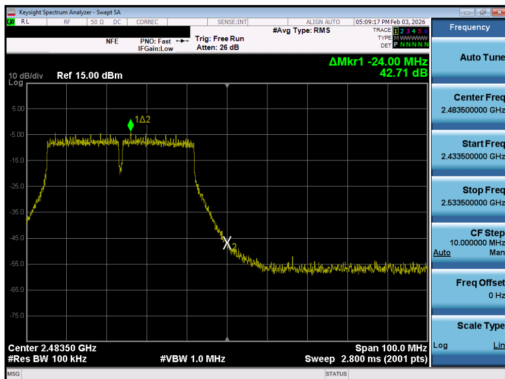
Plot 7-191. Band Edge Plot MIMO ANT2 (802.11n 40MHz (2.4GHz) - Ch. 10) - MIMO ANT2
