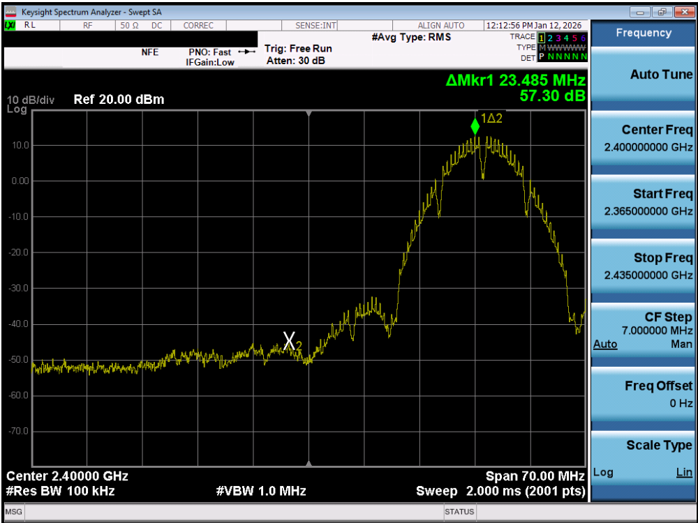
Plot 7-99. Band Edge Plot MIMO ANT1 (802.11b – Ch. 3) – MIMO ANT1
