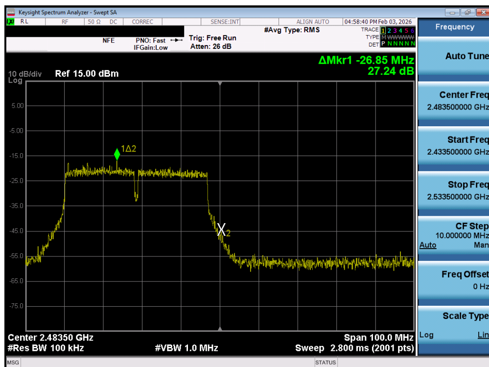
Plot 7-192. Band Edge Plot MIMO ANT2 (802.11n 40MHz (2.4GHz) - Ch. 11) - MIMO ANT2
