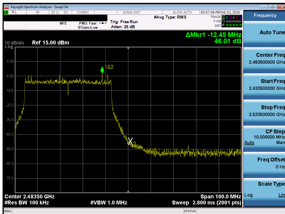
Plot 7-197. Band Edge Plot MIMO ANT2 (802.11be 40MHz (2.4GHz) – Ch. 10) – MIMO ANT2
