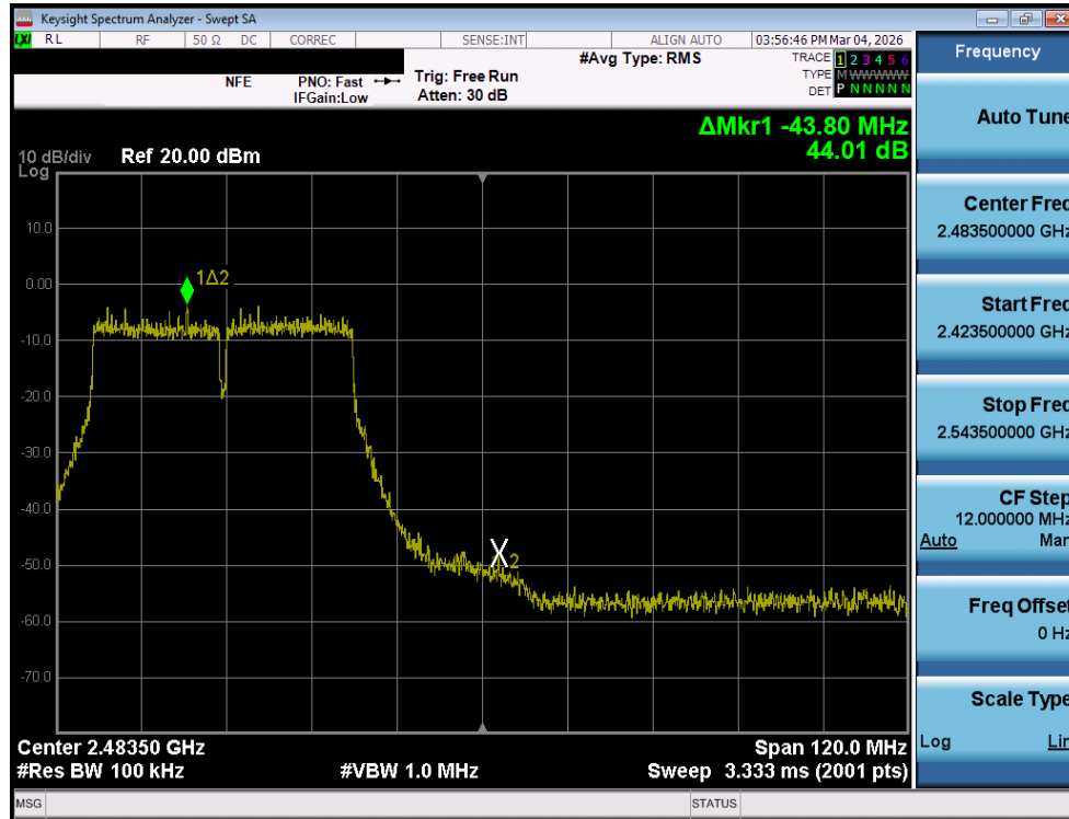
Plot 7-189. Band Edge Plot MIMO ANT2 (802.11n 40MHz (2.4GHz) – Ch. 8) – MIMO ANT2
