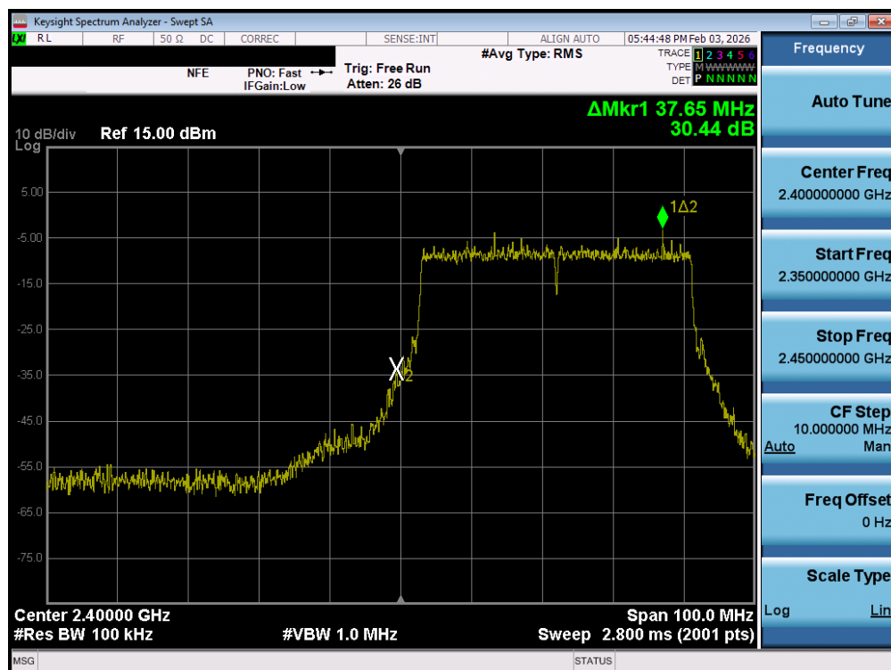
Plot 7-193. Band Edge Plot MIMO ANT2 (802.11be 40MHz (2.4GHz) – Ch. 3) – MIMO ANT2
