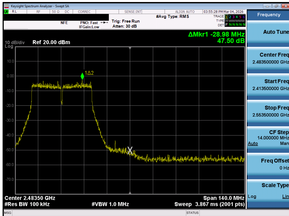
Plot 7-188. Band Edge Plot MIMO ANT2 (802.11n 40MHz (2.4GHz) – Ch. 7) – MIMO ANT2
