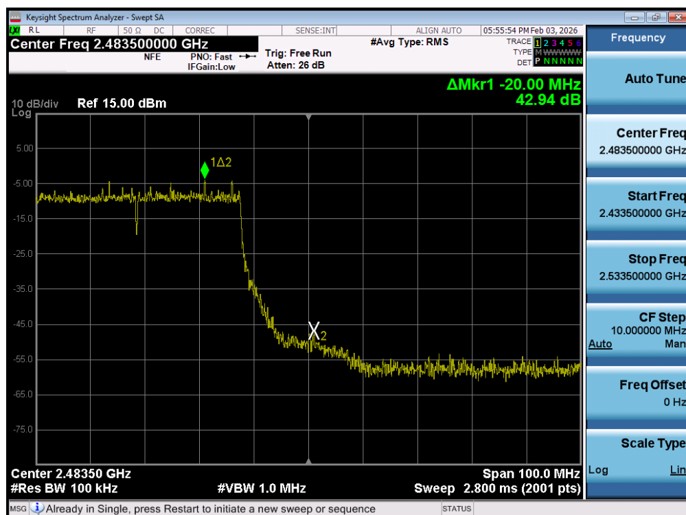
Plot 7-196. Band Edge Plot MIMO ANT2 (802.11be 40MHz (2.4GHz) – Ch. 9) – MIMO ANT2
