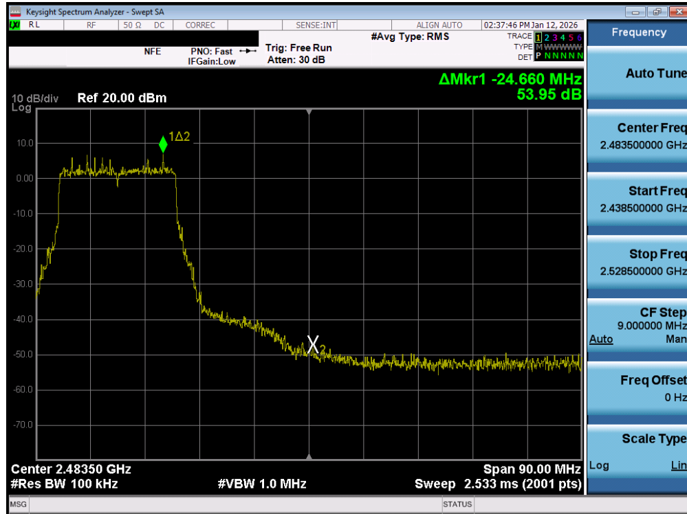
Plot 7-158. Band Edge Plot MIMO ANT2 (802.11be 20MHz (2.4GHz) – Ch. 9) – MIMO ANT2
