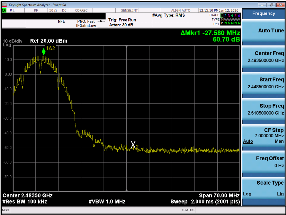
Plot 7-100. Band Edge Plot MIMO ANT1 (802.11b – Ch. 10) – MIMO ANT1
