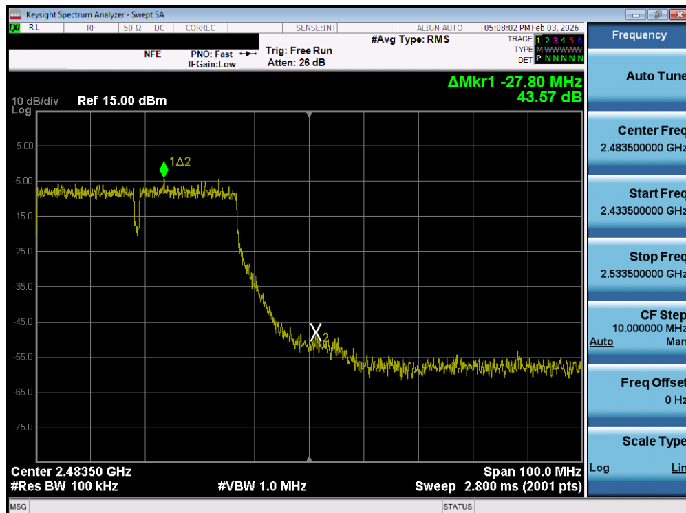
Plot 7-190. Band Edge Plot MIMO ANT2 (802.11n 40MHz (2.4GHz) – Ch. 9) – MIMO ANT2
