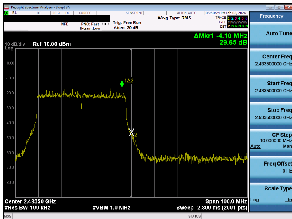
Plot 7-198. Band Edge Plot MIMO ANT2 (802.11be 40MHz (2.4GHz) – Ch. 11) – MIMO ANT2
