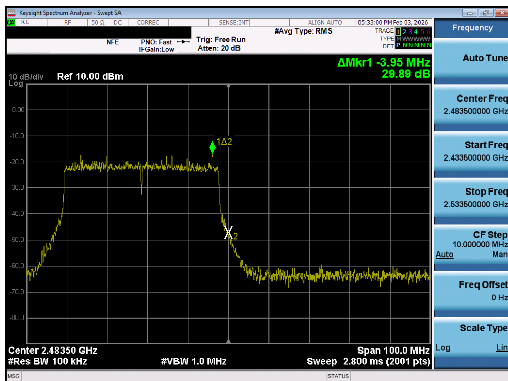
Plot 7-182. Band Edge Plot MIMO ANT1 (802.11be 40MHz (2.4GHz) – Ch. 11) – MIMO ANT
