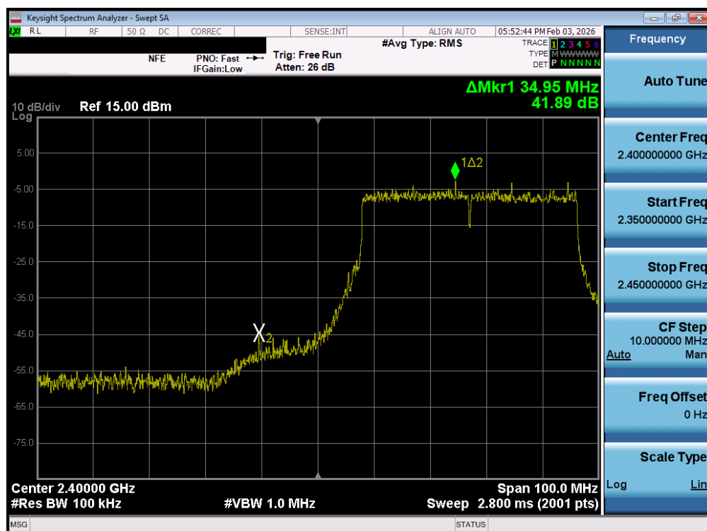
Plot 7-194. Band Edge Plot MIMO ANT2 (802.11be 40MHz (2.4GHz) – Ch. 4) – MIMO ANT2
