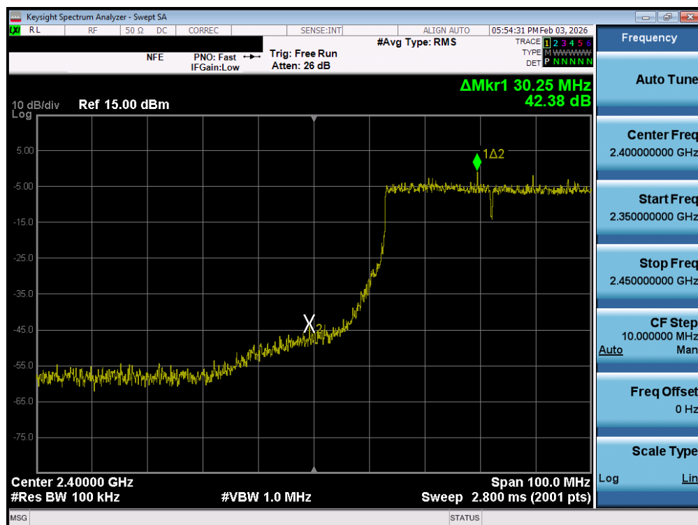
Plot 7-195. Band Edge Plot MIMO ANT2 (802.11be 40MHz (2.4GHz) – Ch. 5) – MIMO ANT2
