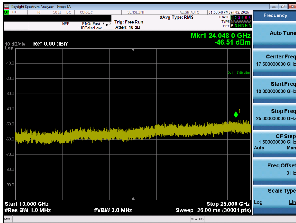
Plot 7-200. Conducted Spurious Plot MIMO ANT1 (802.11b – Ch. 1) – MIMO ANT1
