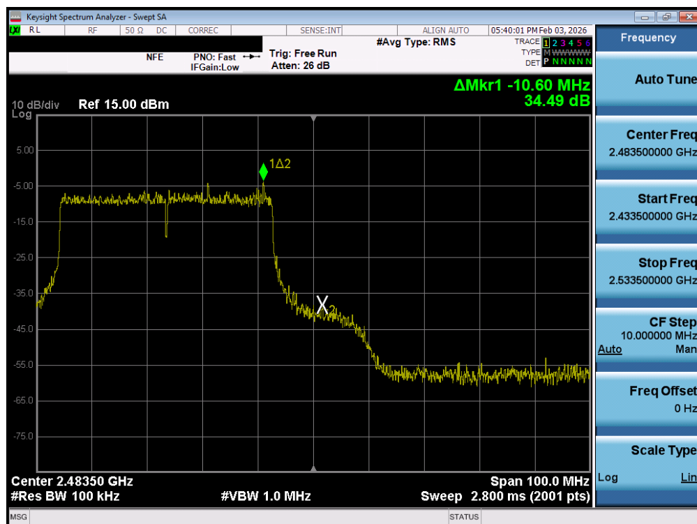
Plot 7-181. Band Edge Plot MIMO ANT1 (802.11be 40MHz (2.4GHz) – Ch. 10) – MIMO ANT1
