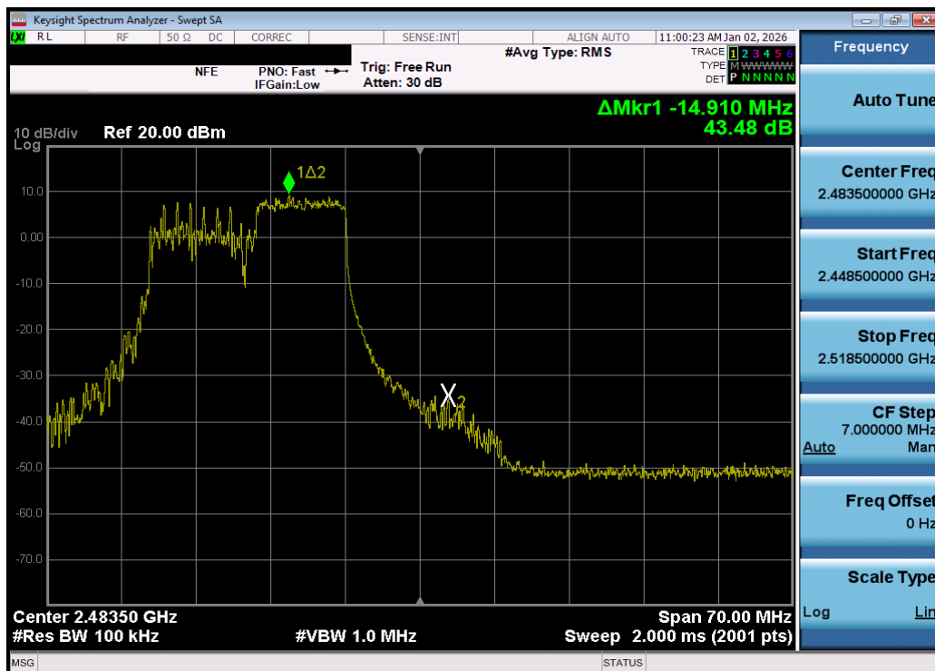
Plot 7-66. Band Edge Plot MIMO ANT1 (802.11be OFDMA – 106 Tones – Ch. 12) – DUAL ANT 1
