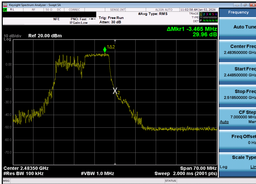
Plot 7-67. Band Edge Plot MIMO ANT1 (802.11be OFDMA – 106 Tones – Ch. 13) – DUAL ANT 1
