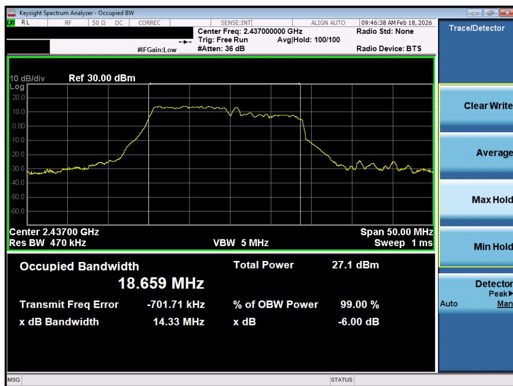
Plot 7-35. OBW Plot MIMO ANT1 (802.11ax OFDMA – 106 + 26 Tones – Ch. 6)
