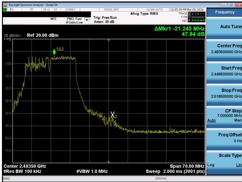
Plot 7-71. Band Edge Plot MIMO ANT1 (802.11be OFDMA – 106 + 26 Tones – Ch. 11) – DUAL ANT 1
