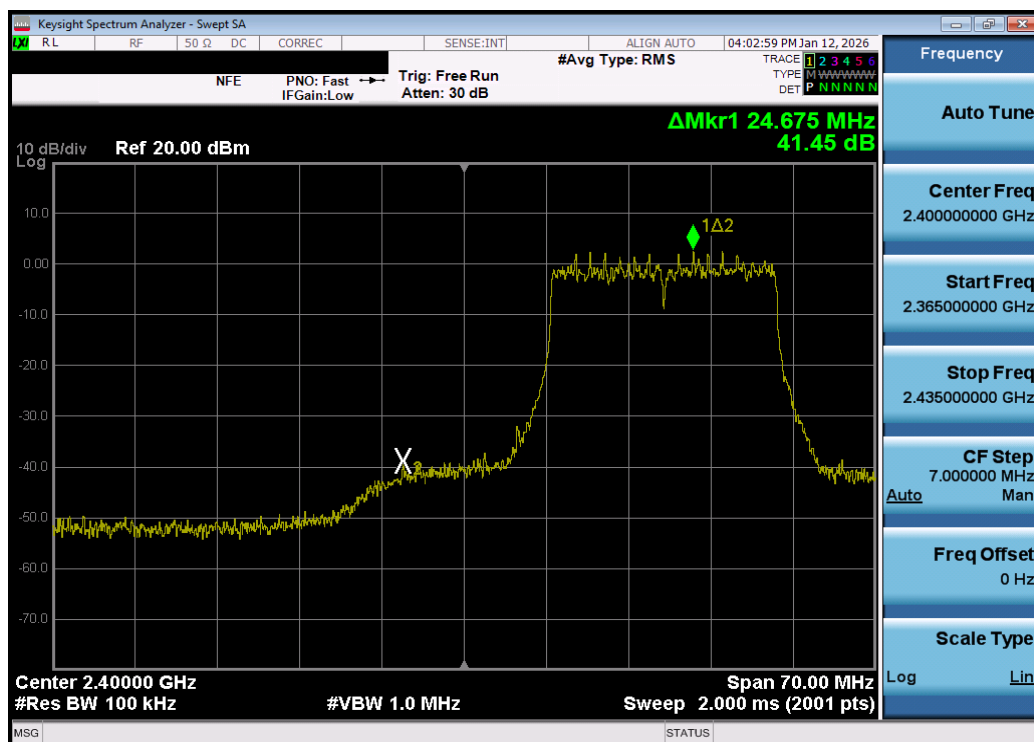
Plot 7-75. Band Edge Plot MIMO ANT1 (802.11be OFDMA – 242 Tones – Ch. 2) – DUAL ANT 1
