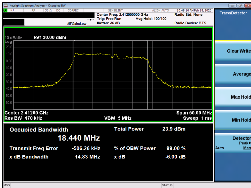
Plot 7-40. OBW Plot MIMO ANT2 (802.11ax OFDMA – 106 + 26 Tones – Ch. 1)
