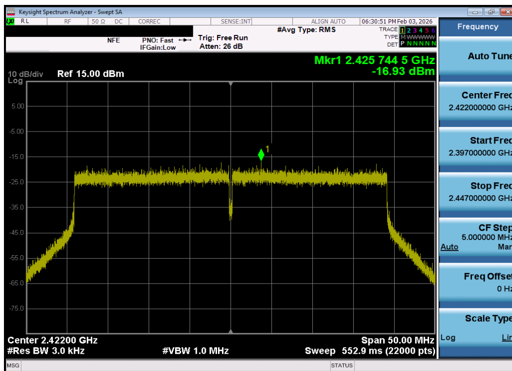
Plot 7-58. Power Spectral Density Plot MIMO ANT2 (802.11be OFDMA – 484 Tones – Ch. 3) – DUAL ANT 2
