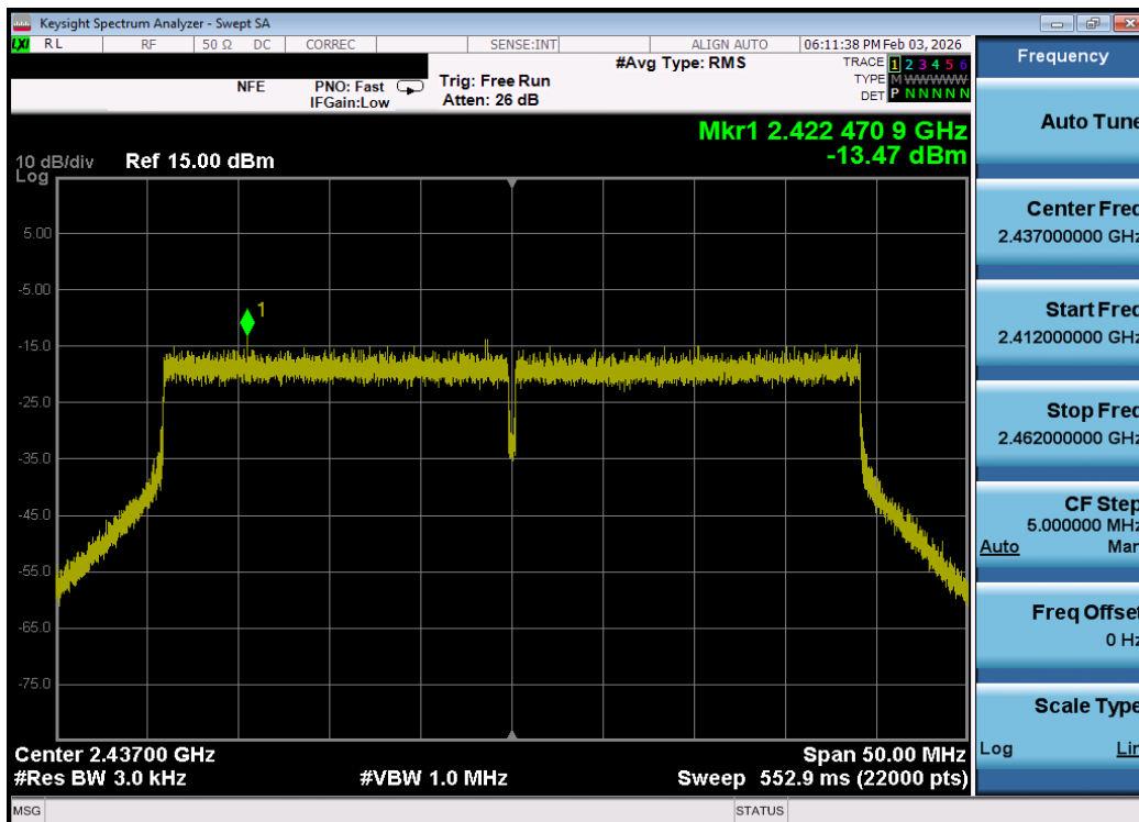
Plot 7-50. Power Spectral Density Plot MIMO ANT1 (802.11be OFDMA – 484 Tones – Ch. 6) – DUAL ANT 1
