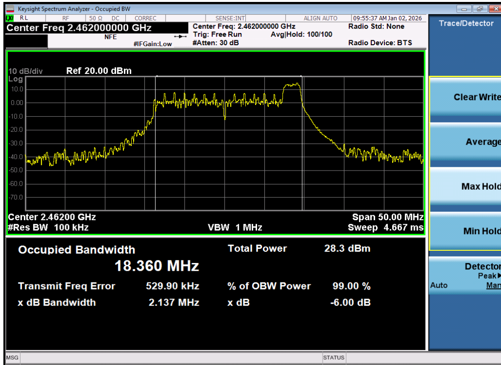
Plot 7-3. 6dB Bandwidth Plot MIMO ANT1 (802.11be OFDMA – 26 Tones – Ch. 11) – DUAL ANT 1
