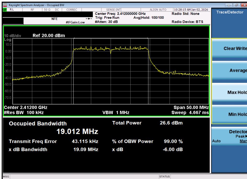
Plot 7-4. 6dB Bandwidth Plot MIMO ANT1 (802.11be OFDMA – 242 Tones – Ch. 1) – DUAL ANT 1
