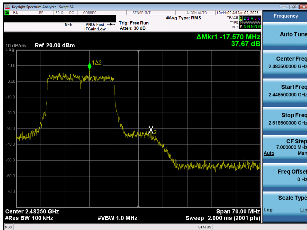
Plot 7-80. Band Edge Plot MIMO ANT1 (802.11be OFDMA – 242 Tones – Ch. 12) – DUAL ANT 1
