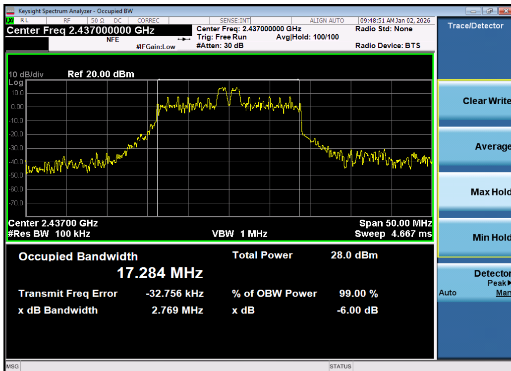
Plot 7-2. 6dB Bandwidth Plot MIMO ANT1 (802.11be OFDMA – 26 Tones – Ch. 6) – DUAL ANT 1
