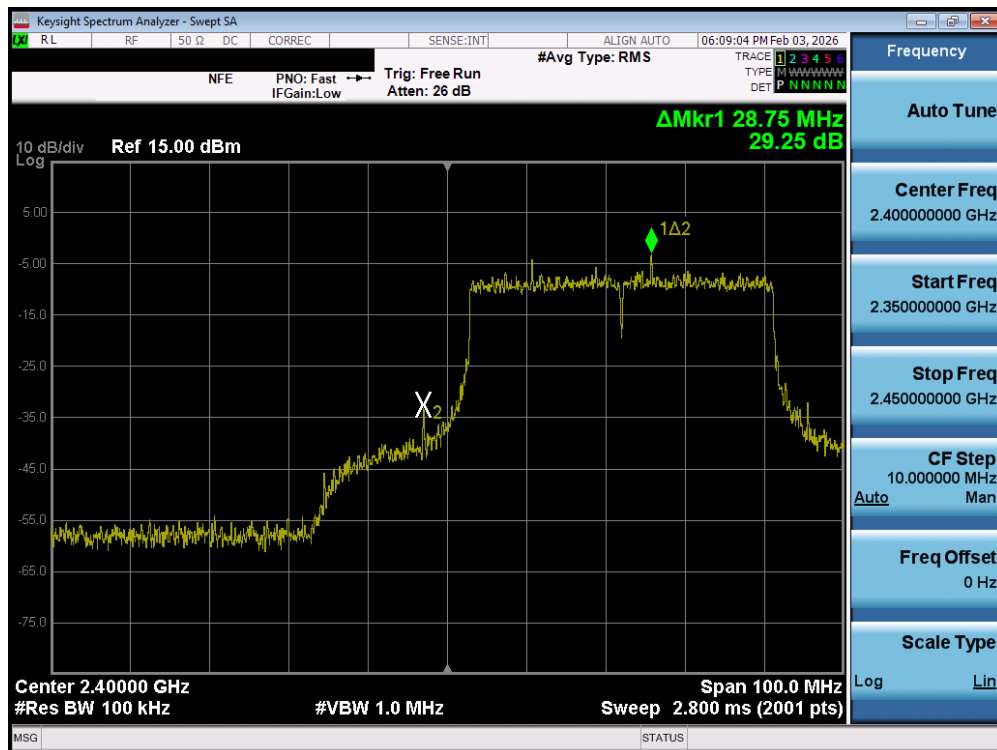
Plot 7-82. Band Edge Plot MIMO ANT1 (802.11be OFDMA – 484 Tones – Ch. 3) – DUAL ANT 1
