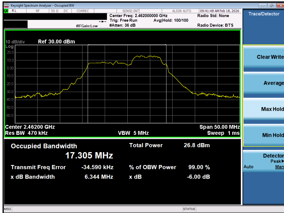
Plot 7-33. OBW Plot MIMO ANT1 (802.11ax OFDMA – 52 + 26 Tones – Ch. 11)
