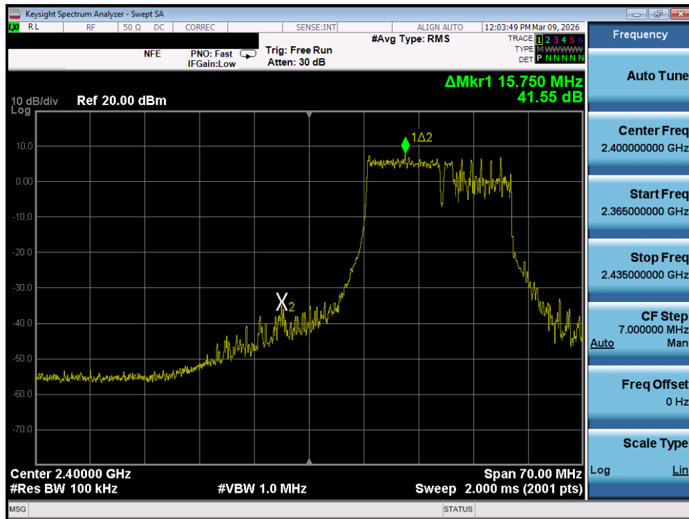
Plot 7-69. Band Edge Plot MIMO ANT1 (802.11be OFDMA – 106 + 26 Tones – Ch. 2) – DUAL ANT 1
