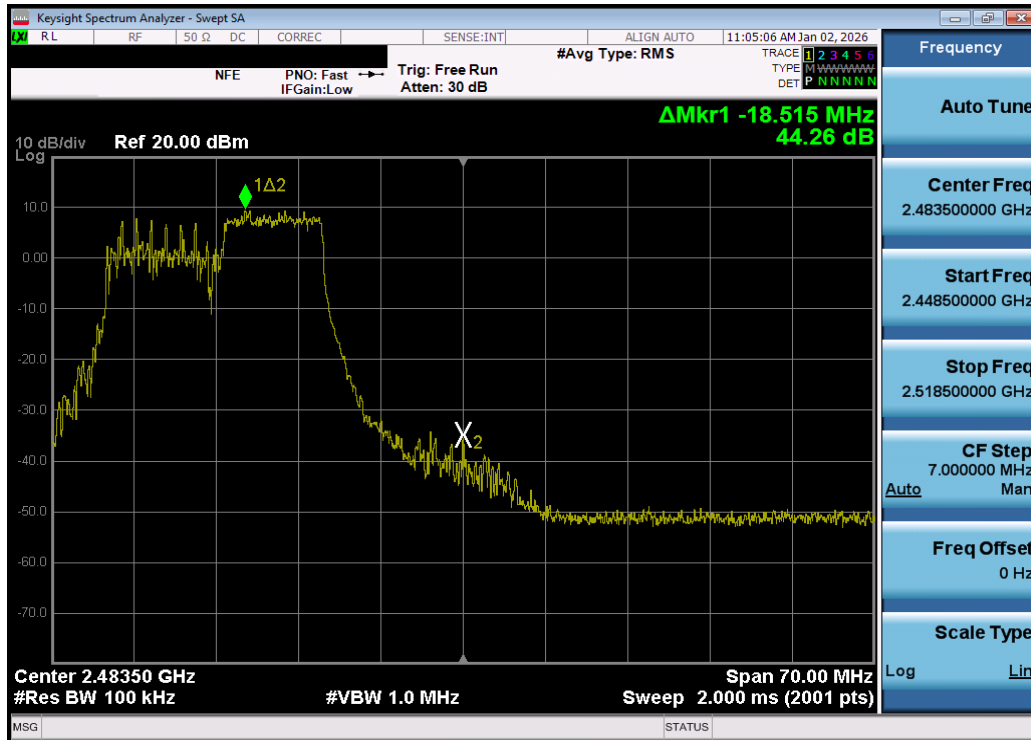
Plot 7-65. Band Edge Plot MIMO ANT1 (802.11be OFDMA – 106 Tones – Ch. 11) – DUAL ANT 1
