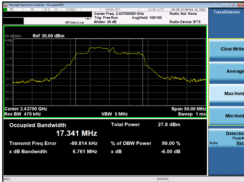
Plot 7-32. OBW Plot MIMO ANT1 (802.11ax OFDMA – 52 + 26 Tones – Ch. 6)
