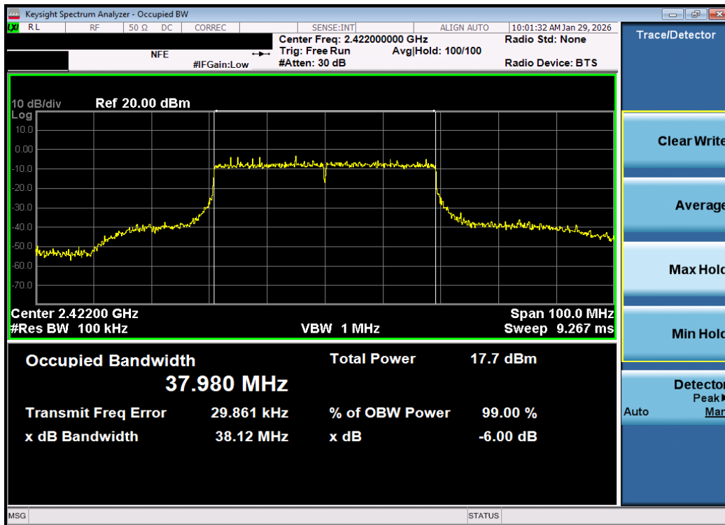
Plot 7-7. 6dB Bandwidth Plot MIMO ANT1 (802.11be OFDMA – 484 Tones – Ch. 3) – DUAL ANT 1
