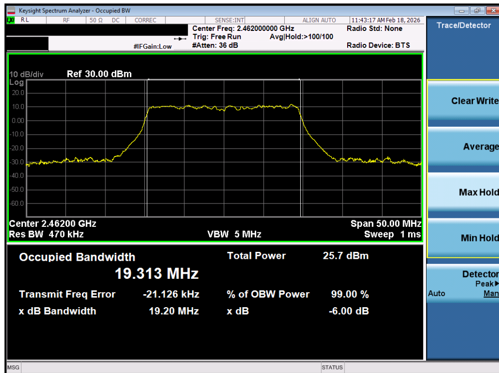
Plot 7-24. OBW Plot MIMO ANT1 (802.11ax OFDMA – 242 Tones – Ch. 11)
