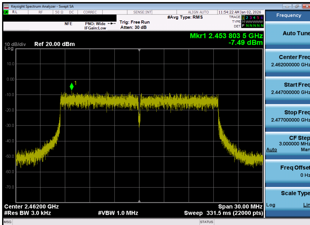
Plot 7-57. Power Spectral Density Plot MIMO ANT2 (802.11be OFDMA – 242 Tones – Ch. 11) – DUAL ANT 2
