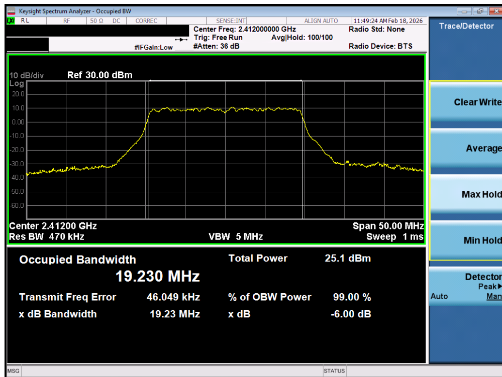
Plot 7-28. OBW Plot MIMO ANT2 (802.11ax OFDMA – 242 Tones – Ch. 1)
