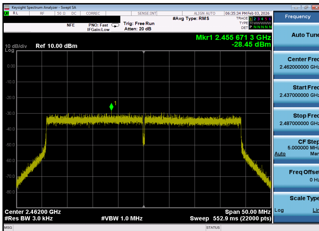
Plot 7-60. Power Spectral Density Plot MIMO ANT2 (802.11be OFDMA – 484 Tones – Ch. 11) – DUAL ANT 2
