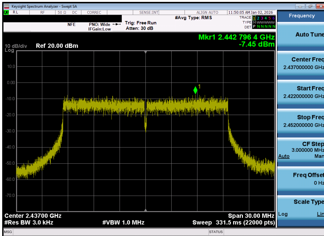
Plot 7-56. Power Spectral Density Plot MIMO ANT2 (802.11be OFDMA – 242 Tones – Ch. 6) – DUAL ANT 2
