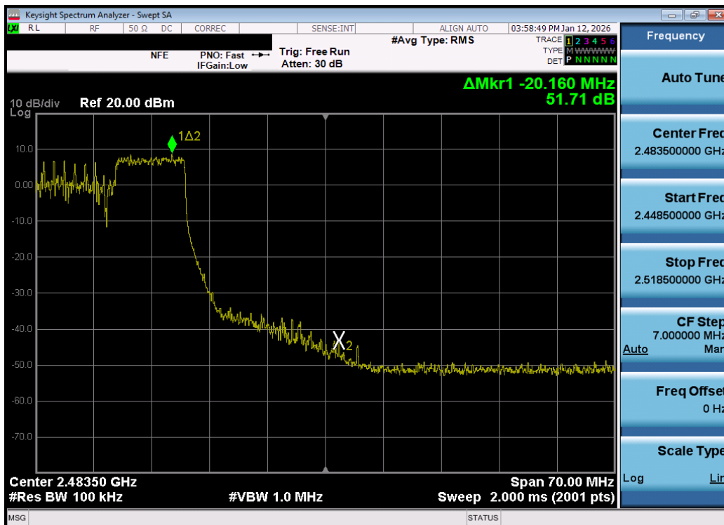
Plot 7-64. Band Edge Plot MIMO ANT1 (802.11be OFDMA – 106 Tones – Ch. 10) – DUAL ANT 1
