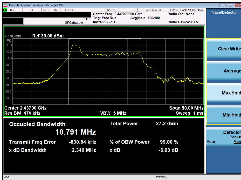
Plot 7-26. OBW Plot MIMO ANT2 (802.11ax OFDMA – 26 Tones – Ch. 6)
