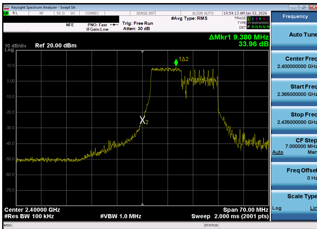
Plot 7-61. Band Edge Plot MIMO ANT1 (802.11be OFDMA – 106 Tones – Ch. 1) – DUAL ANT 1
