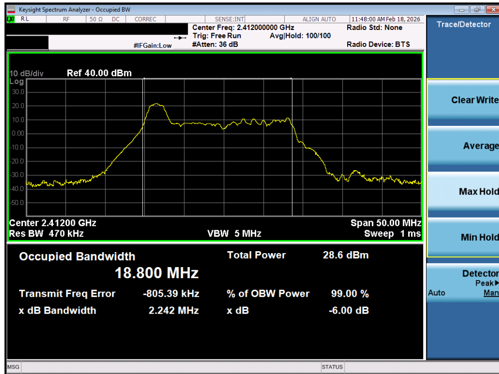
Plot 7-25. OBW Plot MIMO ANT2 (802.11ax OFDMA – 26 Tones – Ch. 1)
