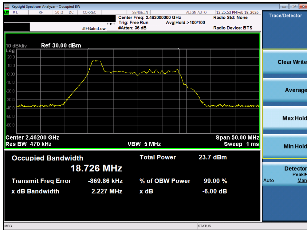
Plot 7-27. OBW Plot MIMO ANT2 (802.11ax OFDMA – 26 Tones – Ch. 11)
