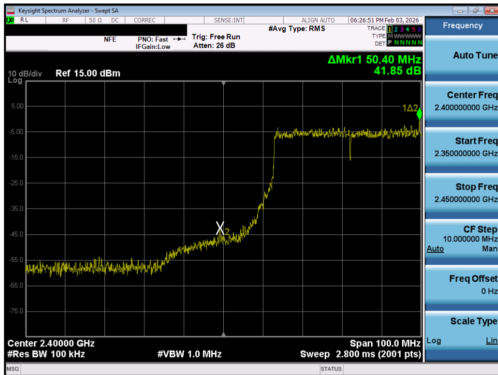
Plot 7-84. Band Edge Plot MIMO ANT1 (802.11be OFDMA - 484 Tones - Ch. 5) - DUAL ANT 1
