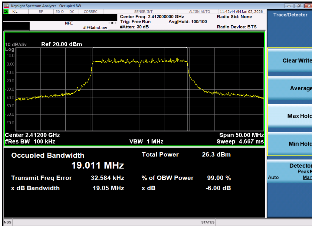
Plot 7-13. 6dB Bandwidth Plot MIMO ANT2 (802.11be OFDMA – 242 Tones – Ch. 1) – DUAL ANT 2
