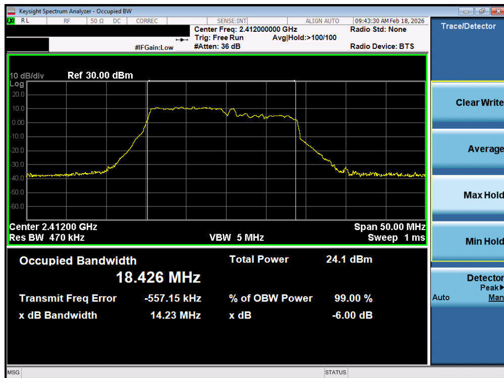
Plot 7-34. OBW Plot MIMO ANT1 (802.11ax OFDMA – 106 + 26 Tones – Ch. 1)
