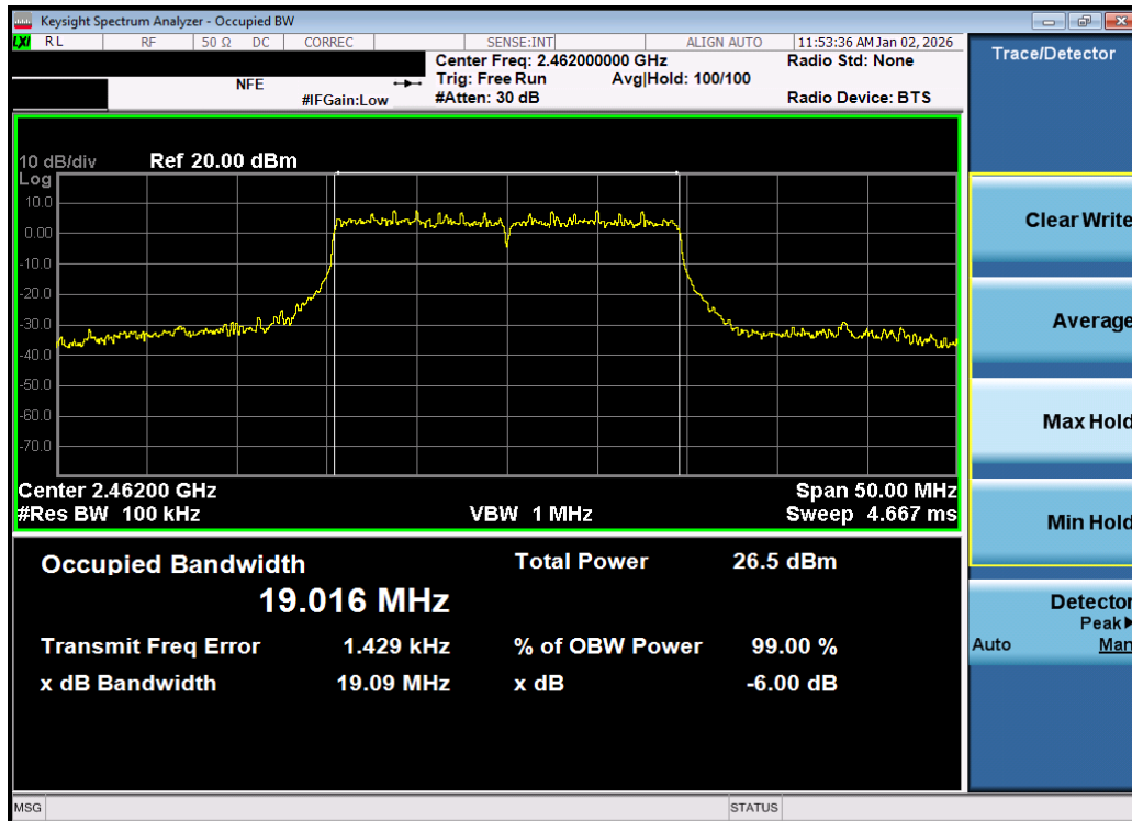
Plot 7-15. 6dB Bandwidth Plot MIMO ANT2 (802.11be OFDMA – 242 Tones – Ch. 11) – DUAL ANT 2
