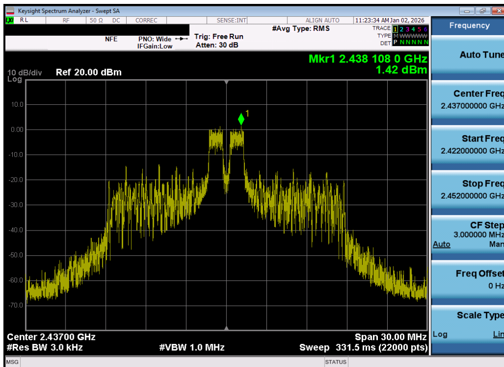
Plot 7-53. Power Spectral Density Plot MIMO ANT2 (802.11be OFDMA – 26 Tones – Ch. 6) – DUAL ANT 2
