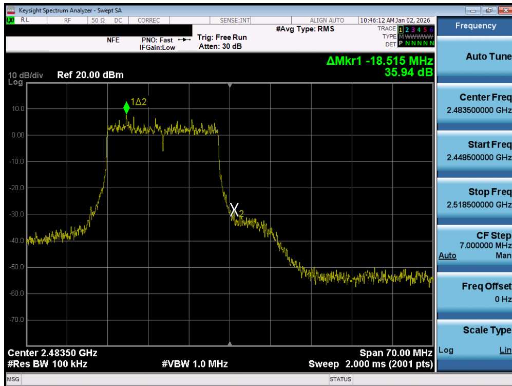
Plot 7-81. Band Edge Plot MIMO ANT1 (802.11be OFDMA – 242 Tones – Ch. 13) – DUAL ANT 1
