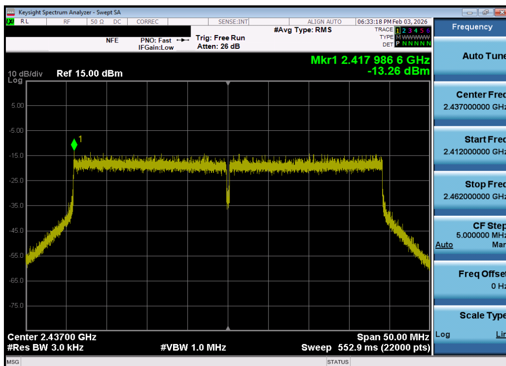
Plot 7-59. Power Spectral Density Plot MIMO ANT2 (802.11be OFDMA – 484 Tones – Ch. 6) – DUAL ANT 2
