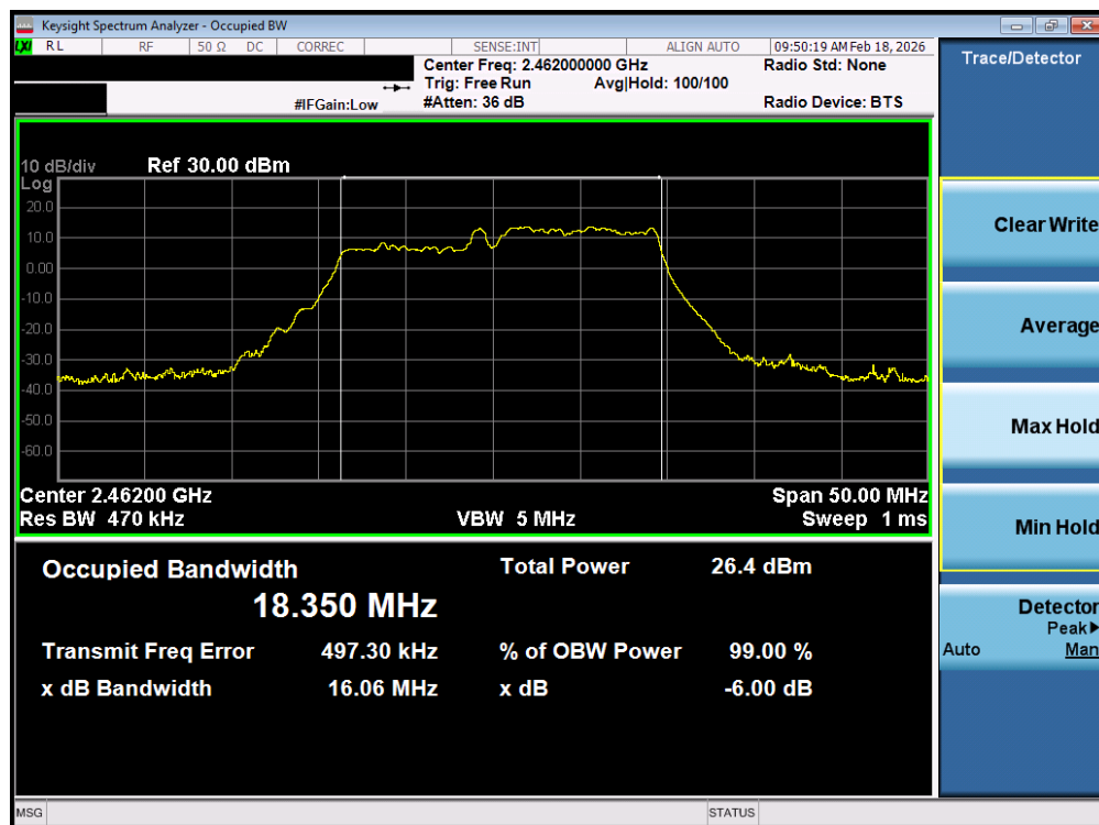
Plot 7-36. OBW Plot MIMO ANT1 (802.11ax OFDMA – 106 + 26 Tones – Ch. 11)
