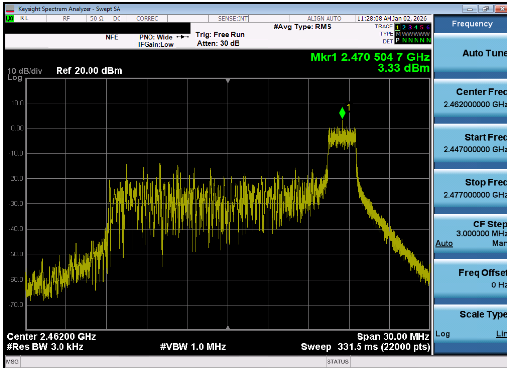
Plot 7-54. Power Spectral Density Plot MIMO ANT2 (802.11be OFDMA – 26 Tones – Ch. 11) – DUAL ANT 2
