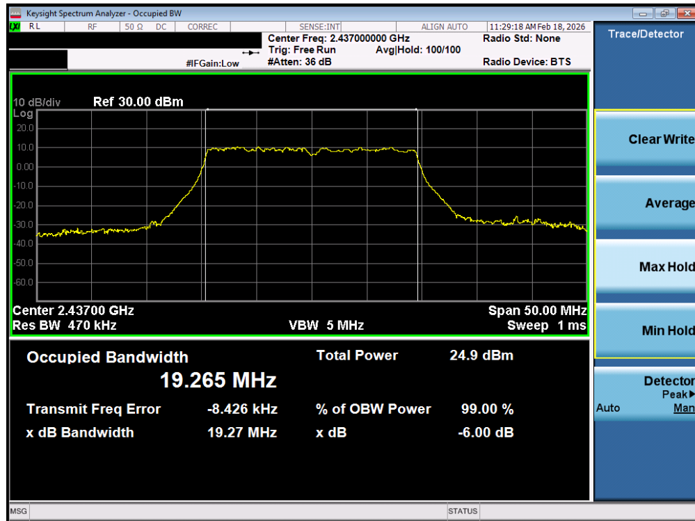
Plot 7-23. OBW Plot MIMO ANT1 (802.11ax OFDMA – 242 Tones – Ch. 6)
