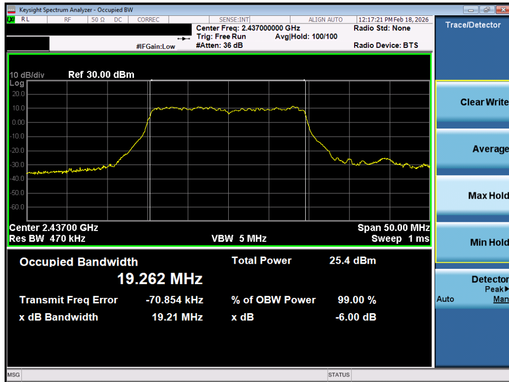
Plot 7-29. OBW Plot MIMO ANT2 (802.11ax OFDMA – 242 Tones – Ch. 6)
