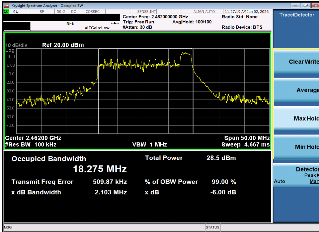
Plot 7-12. 6dB Bandwidth Plot MIMO ANT2 (802.11be OFDMA – 26 Tones – Ch. 11) – DUAL ANT 2
