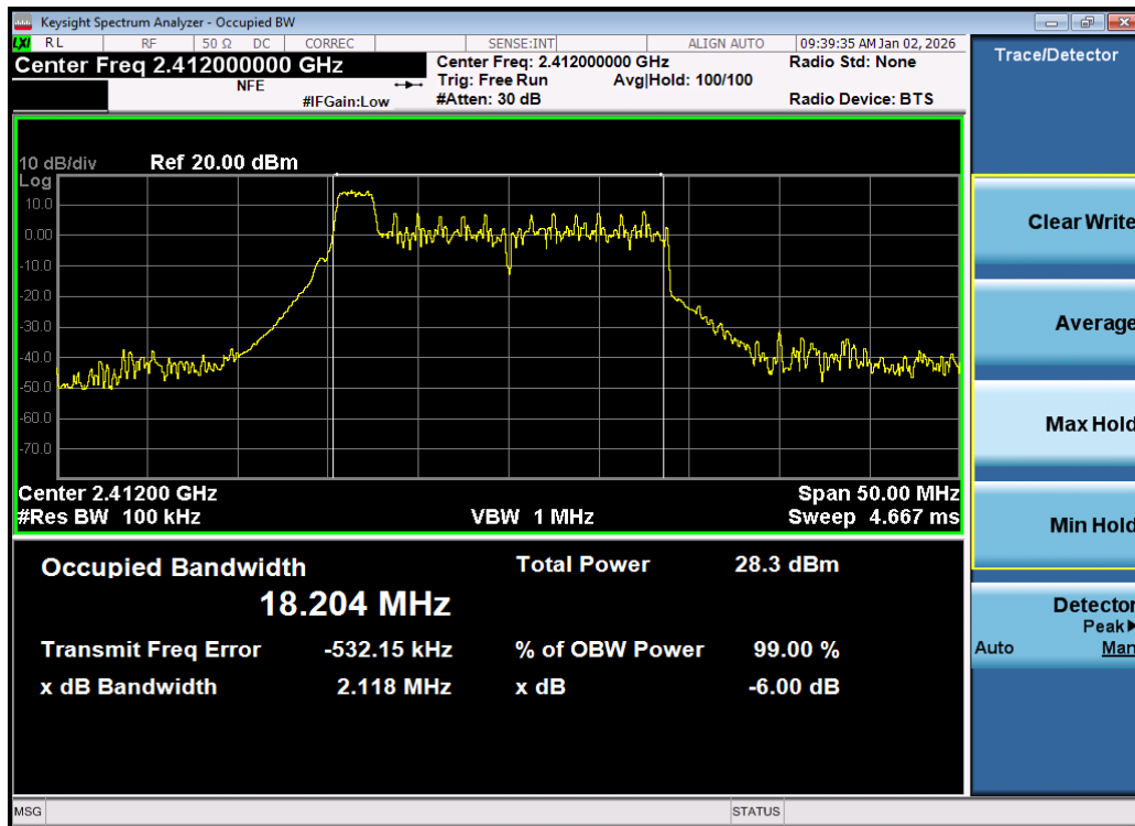
Plot 7-1. 6dB Bandwidth Plot MIMO ANT1 (802.11be OFDMA – 26 Tones – Ch. 1) – DUAL ANT 1
