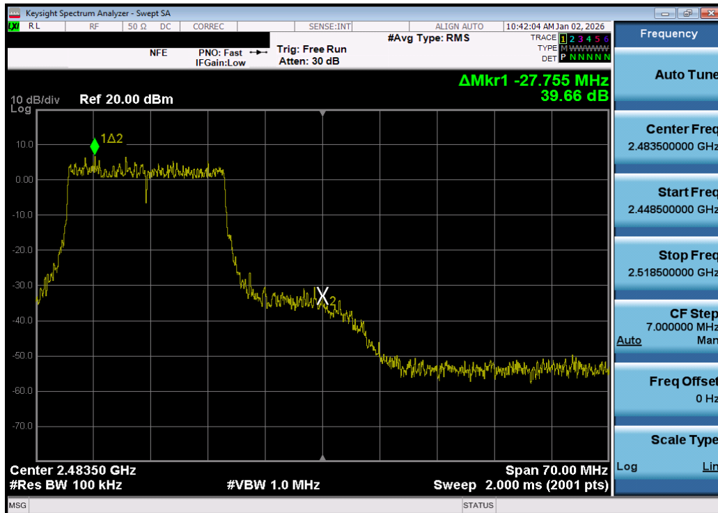
Plot 7-79. Band Edge Plot MIMO ANT1 (802.11be OFDMA – 242 Tones – Ch. 11) – DUAL ANT 1
