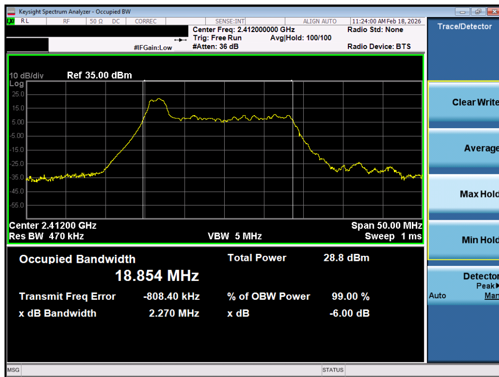
Plot 7-19. OBW Plot MIMO ANT1 (802.11ax OFDMA – 26 Tones – Ch. 1)
