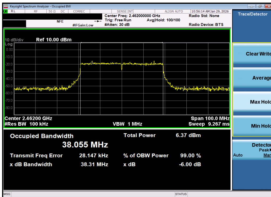
Plot 7-18. 6dB Bandwidth Plot MIMO ANT2 (802.11be OFDMA – 484 Tones – Ch. 11) – DUAL ANT 2
