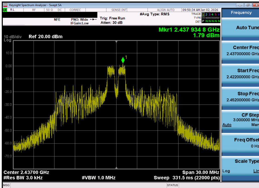
Plot 7-44. Power Spectral Density Plot MIMO ANT1 (802.11be OFDMA – 26 Tones – Ch. 6) – DUAL ANT 1
