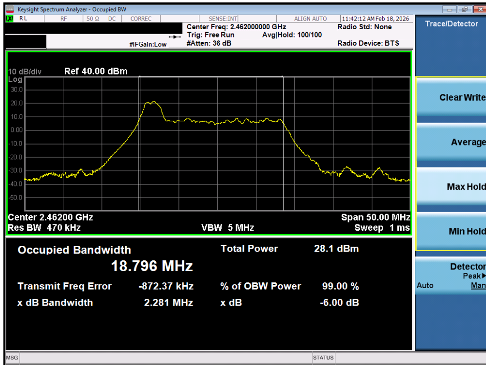
Plot 7-21. OBW Plot MIMO ANT1 (802.11ax OFDMA – 26 Tones – Ch. 11)
