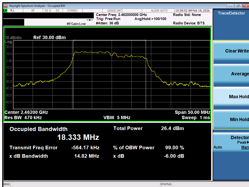
Plot 7-42. OBW Plot MIMO ANT2 (802.11ax OFDMA - 106 + 26 Tones - Ch. 11)
