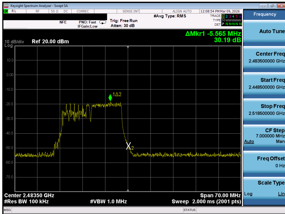
Plot 7-73. Band Edge Plot MIMO ANT1 (802.11be OFDMA – 106 + 26 Tones – Ch. 13) – DUAL ANT 1
