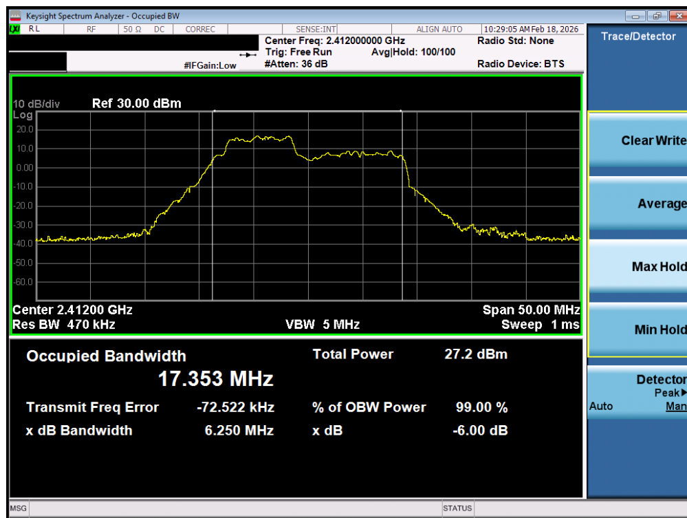
Plot 7-31. OBW Plot MIMO ANT1 (802.11ax OFDMA – 52 + 26 Tones – Ch. 1)
