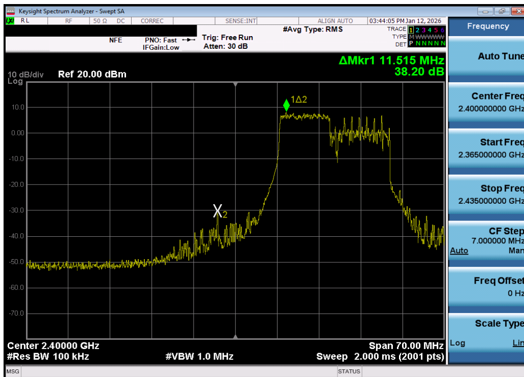
Plot 7-62. Band Edge Plot MIMO ANT1 (802.11be OFDMA – 106 Tones – Ch. 2) – DUAL ANT 1
