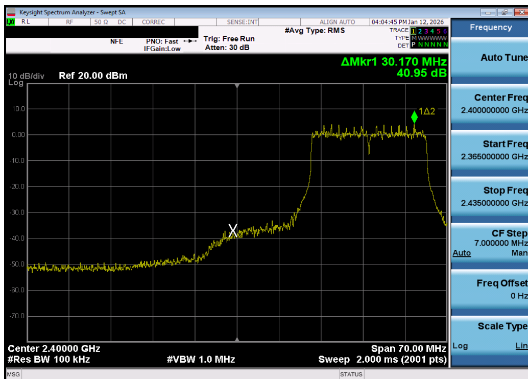
Plot 7-76. Band Edge Plot MIMO ANT1 (802.11be OFDMA – 242 Tones – Ch. 3) – DUAL ANT 1
