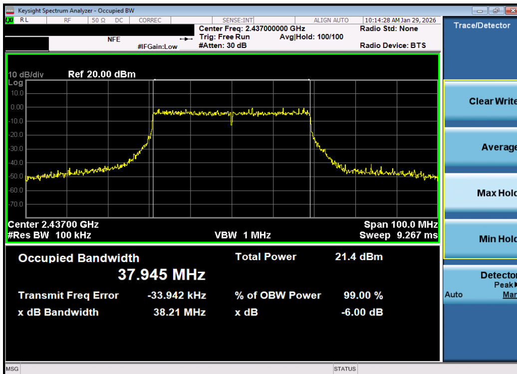
Plot 7-8. 6dB Bandwidth Plot MIMO ANT1 (802.11be OFDMA – 484 Tones – Ch. 6) – DUAL ANT 1
