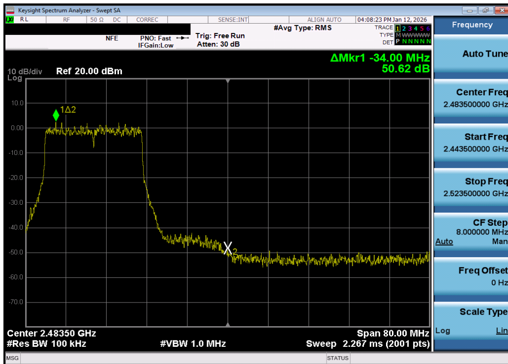
Plot 7-78. Band Edge Plot MIMO ANT1 (802.11be OFDMA – 242 Tones – Ch. 10) – DUAL ANT 1
