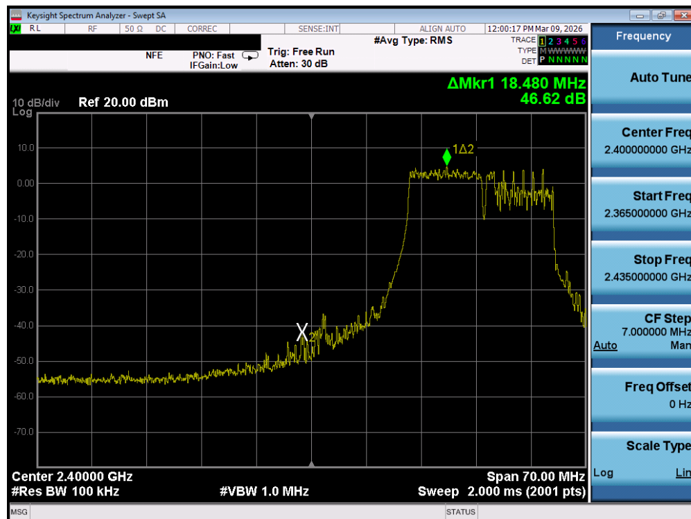
Plot 7-68. Band Edge Plot MIMO ANT1 (802.11be OFDMA – 106 + 26 Tones – Ch. 1) – DUAL ANT 1
