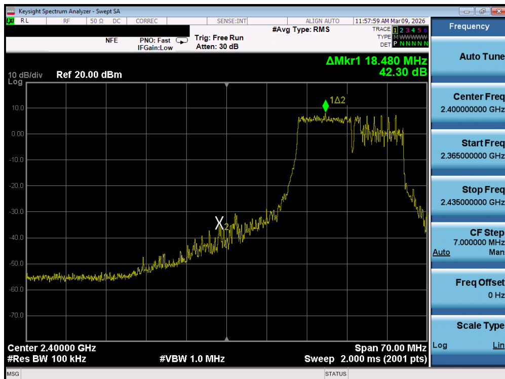
Plot 7-70. Band Edge Plot MIMO ANT1 (802.11be OFDMA – 106 + 26 Tones – Ch. 3) – DUAL ANT 1
