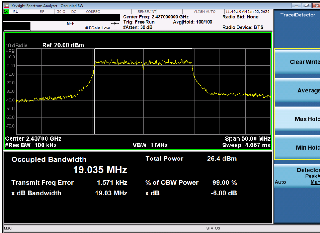
Plot 7-14. 6dB Bandwidth Plot MIMO ANT2 (802.11be OFDMA – 242 Tones – Ch. 6) – DUAL ANT 2
