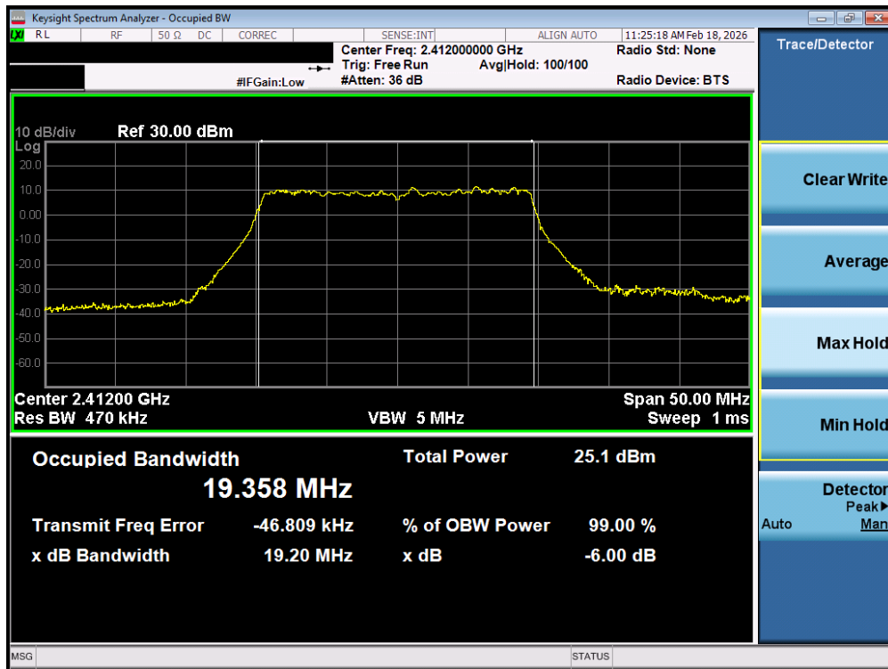
Plot 7-22. OBW Plot MIMO ANT1 (802.11ax OFDMA – 242 Tones – Ch. 1)
