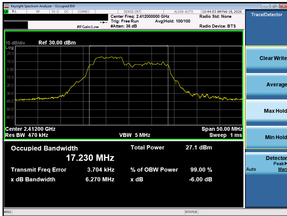
Plot 7-37. OBW Plot MIMO ANT2 (802.11ax OFDMA – 52 + 26 Tones – Ch. 1)
