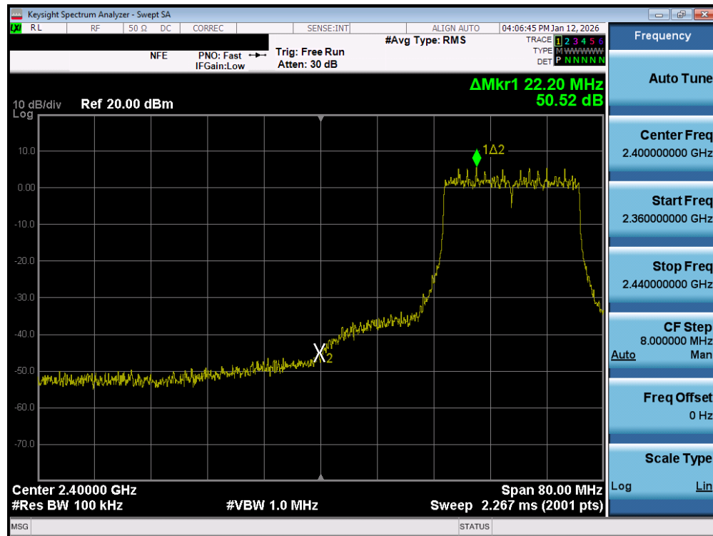
Plot 7-77. Band Edge Plot MIMO ANT1 (802.11be OFDMA – 242 Tones – Ch. 4) – DUAL ANT 1
