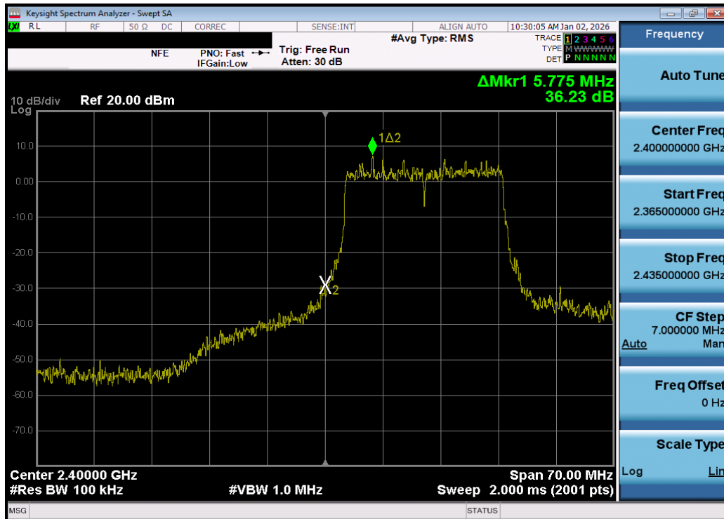
Plot 7-74. Band Edge Plot MIMO ANT1 (802.11be OFDMA – 242 Tones – Ch. 1) – DUAL ANT 1
