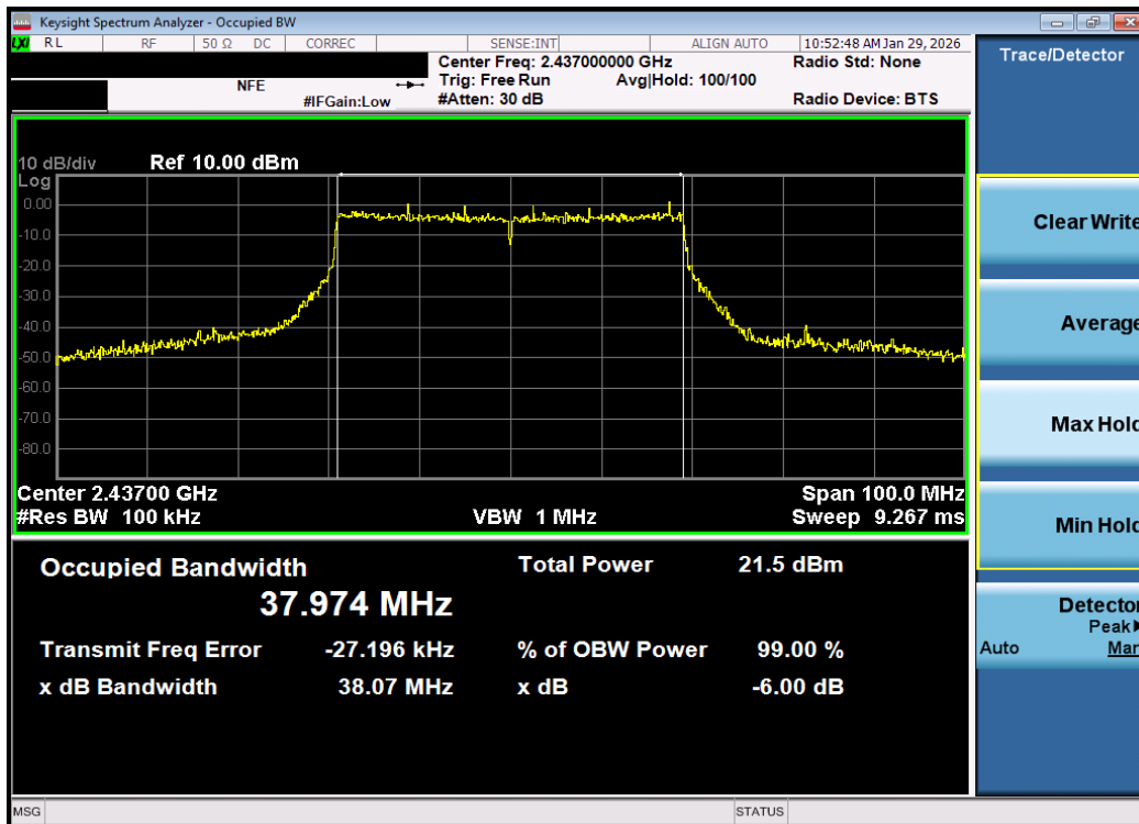
Plot 7-17. 6dB Bandwidth Plot MIMO ANT2 (802.11be OFDMA – 484 Tones – Ch. 6) – DUAL ANT 2
