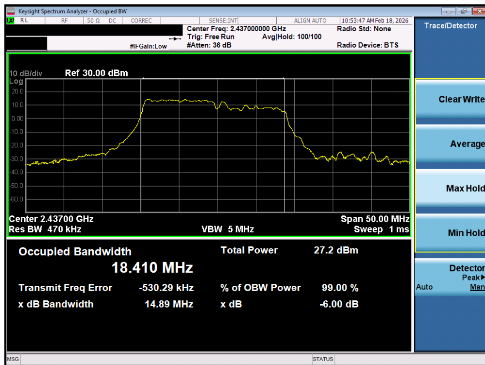
Plot 7-41. OBW Plot MIMO ANT2 (802.11ax OFDMA - 106 + 26 Tones - Ch. 6)
