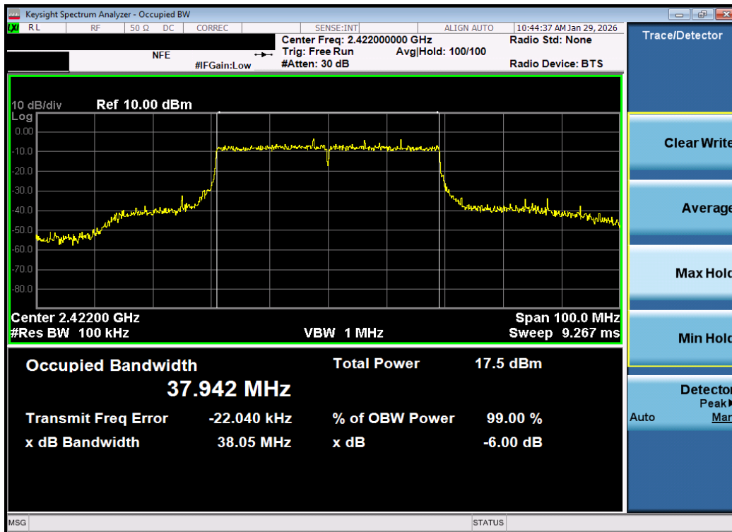
Plot 7-16. 6dB Bandwidth Plot MIMO ANT2 (802.11be OFDMA – 484 Tones – Ch. 3) – DUAL ANT 2
