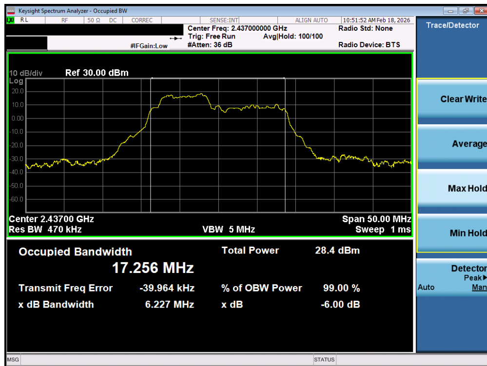
Plot 7-38. OBW Plot MIMO ANT2 (802.11ax OFDMA – 52 + 26 Tones – Ch. 6)
