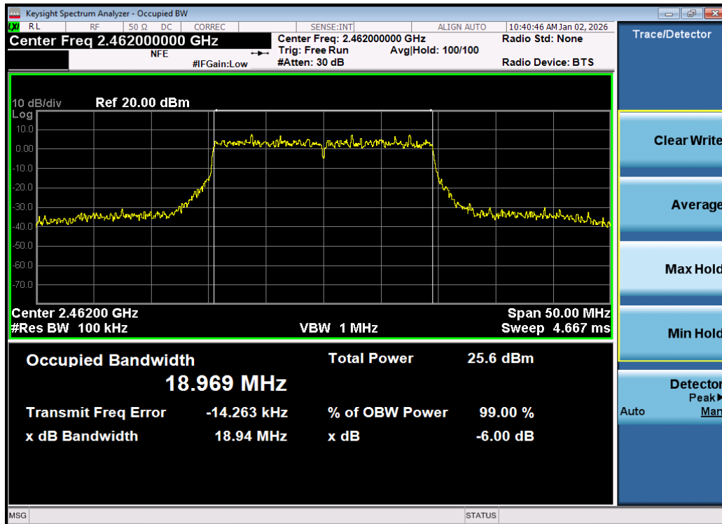
Plot 7-6. 6dB Bandwidth Plot MIMO ANT1 (802.11be OFDMA – 242 Tones – Ch. 11) – DUAL ANT 1
