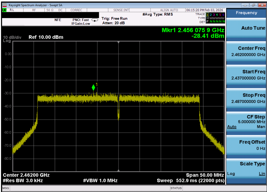
Plot 7-51. Power Spectral Density Plot MIMO ANT1 (802.11be OFDMA – 484 Tones – Ch. 11) – DUAL ANT 1
