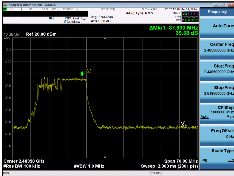
Plot 7-72. Band Edge Plot MIMO ANT1 (802.11be OFDMA – 106 + 26 Tones – Ch. 12) – DUAL ANT 1
