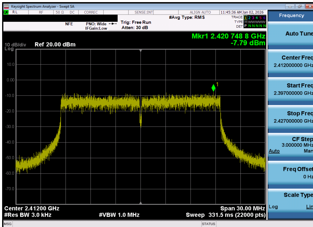
Plot 7-55. Power Spectral Density Plot MIMO ANT2 (802.11be OFDMA – 242 Tones – Ch. 1) – DUAL ANT 2
