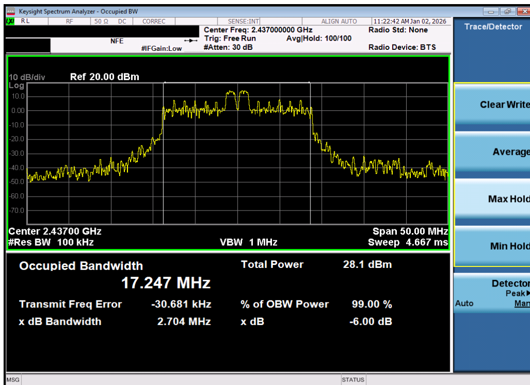
Plot 7-11. 6dB Bandwidth Plot MIMO ANT2 (802.11be OFDMA – 26 Tones – Ch. 6) – DUAL ANT 2
