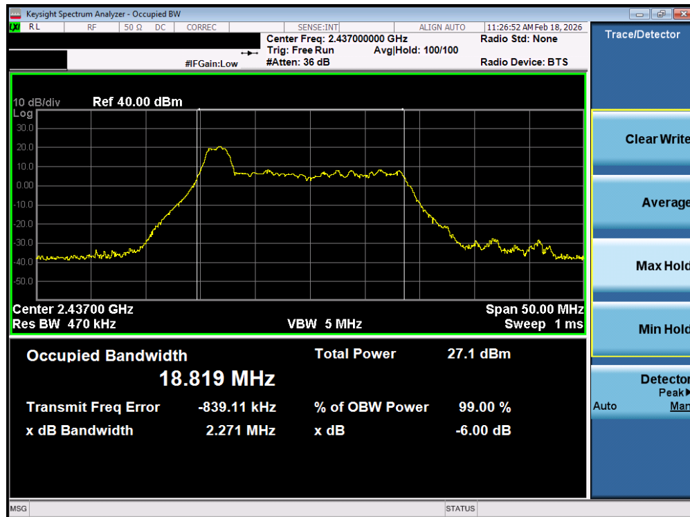
Plot 7-20. OBW Plot MIMO ANT1 (802.11ax OFDMA – 26 Tones – Ch. 6)
