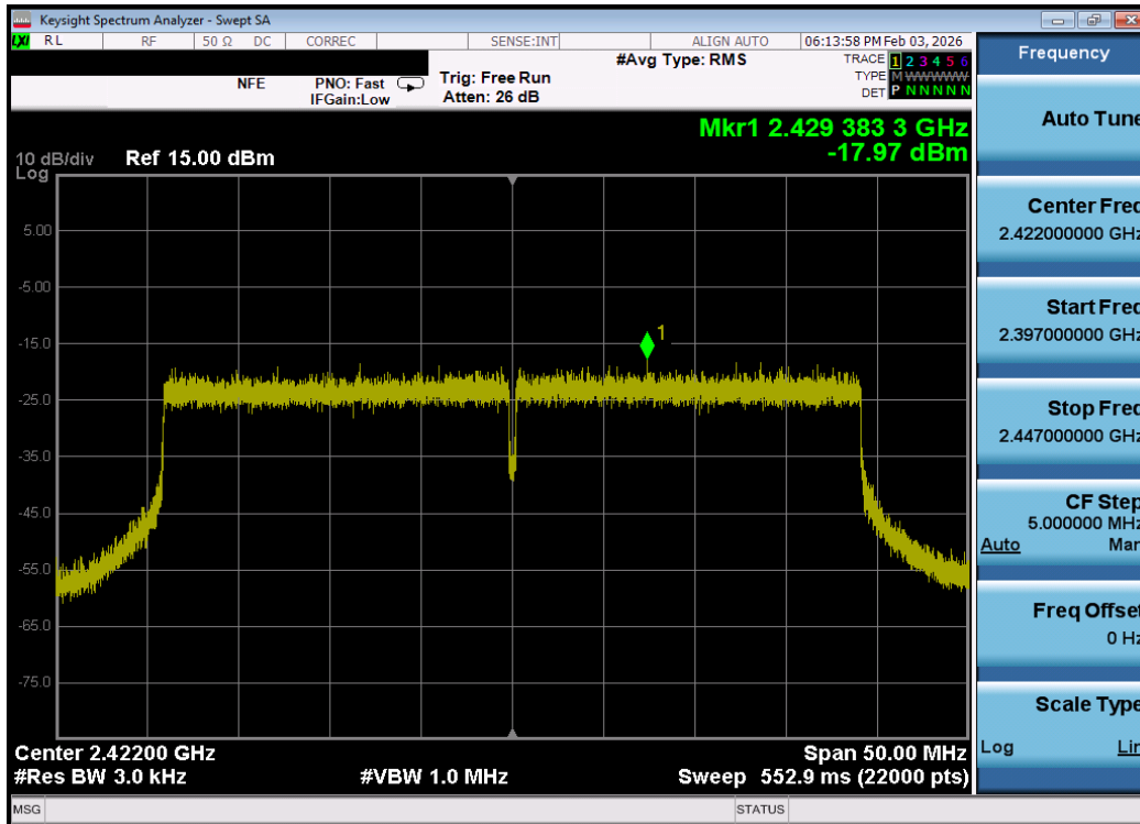
Plot 7-49. Power Spectral Density Plot MIMO ANT1 (802.11be OFDMA – 484 Tones – Ch. 3) – DUAL ANT 1
