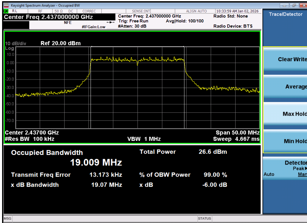
Plot 7-5. 6dB Bandwidth Plot MIMO ANT1 (802.11be OFDMA – 242 Tones – Ch. 6) – DUAL ANT 1
