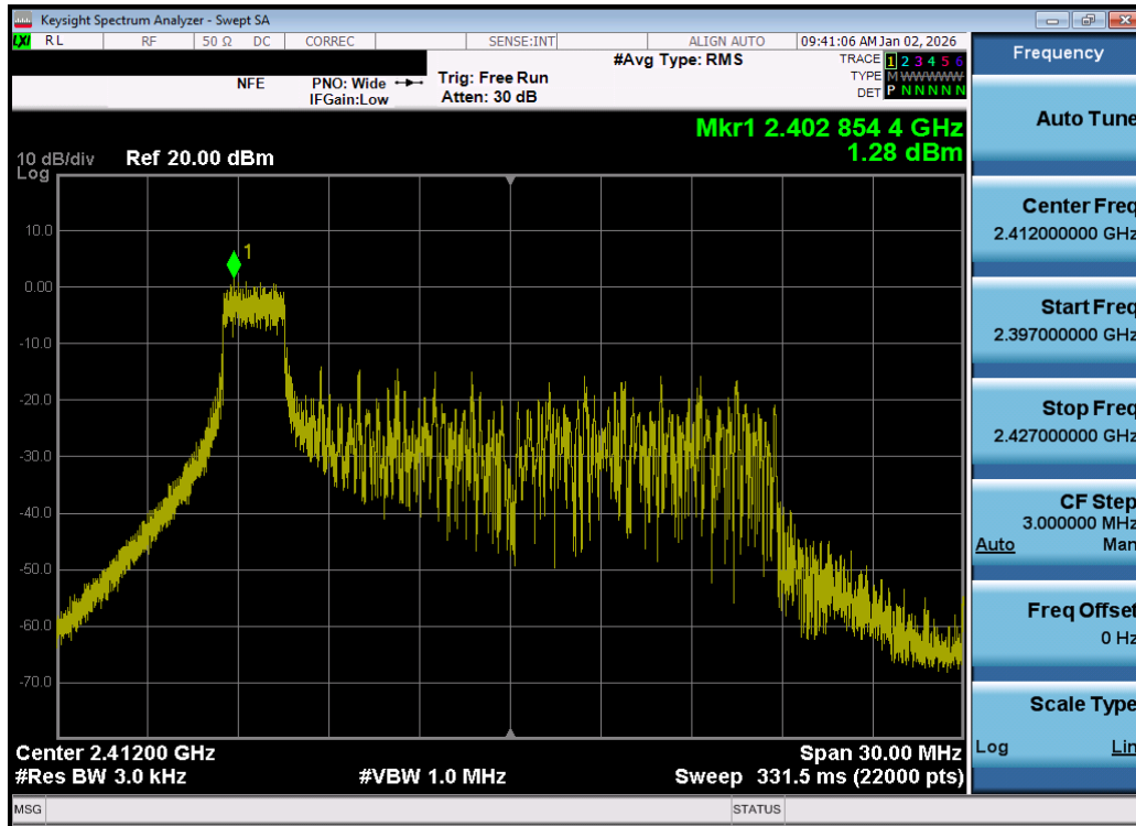
Plot 7-43. Power Spectral Density Plot MIMO ANT1 (802.11be OFDMA – 26 Tones – Ch. 1) – DUAL ANT 1
