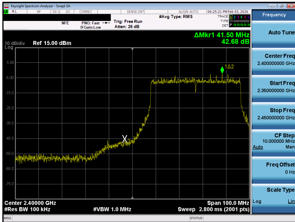
Plot 7-83. Band Edge Plot MIMO ANT1 (802.11be OFDMA - 484 Tones - Ch. 4) - DUAL ANT 1
