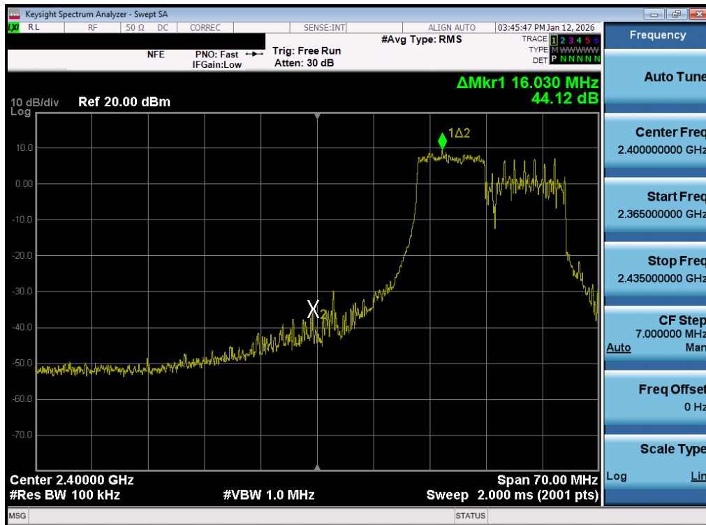
Plot 7-63. Band Edge Plot MIMO ANT1 (802.11be OFDMA – 106 Tones – Ch. 3) – DUAL ANT 1
