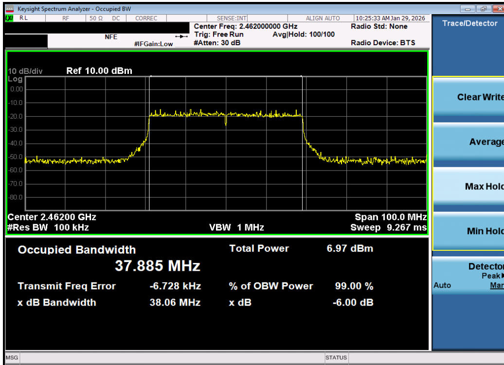
Plot 7-9. 6dB Bandwidth Plot MIMO ANT1 (802.11be OFDMA – 484 Tones – Ch. 11) – DUAL ANT 1
