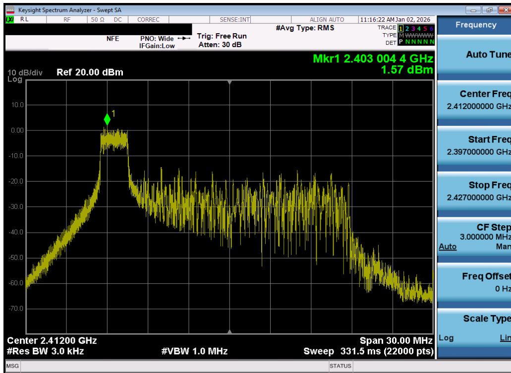
Plot 7-52. Power Spectral Density Plot MIMO ANT2 (802.11be OFDMA – 26 Tones – Ch. 1) – DUAL ANT 2
