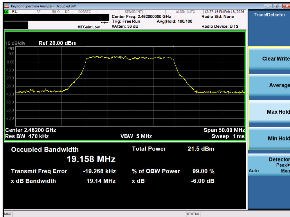
Plot 7-30. OBW Plot MIMO ANT2 (802.11ax OFDMA – 242 Tones – Ch. 11)
