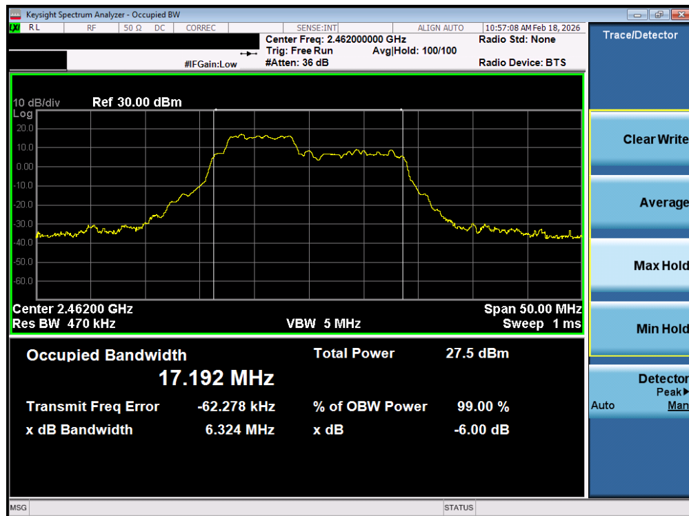
Plot 7-39. OBW Plot MIMO ANT2 (802.11ax OFDMA – 52 + 26 Tones – Ch. 11)
