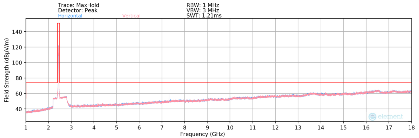
Plot 7-152. Radiated Spurious Plot above 1GHz MIMO (802.11be OFDMA – 26 Tones – Ch. 6)
