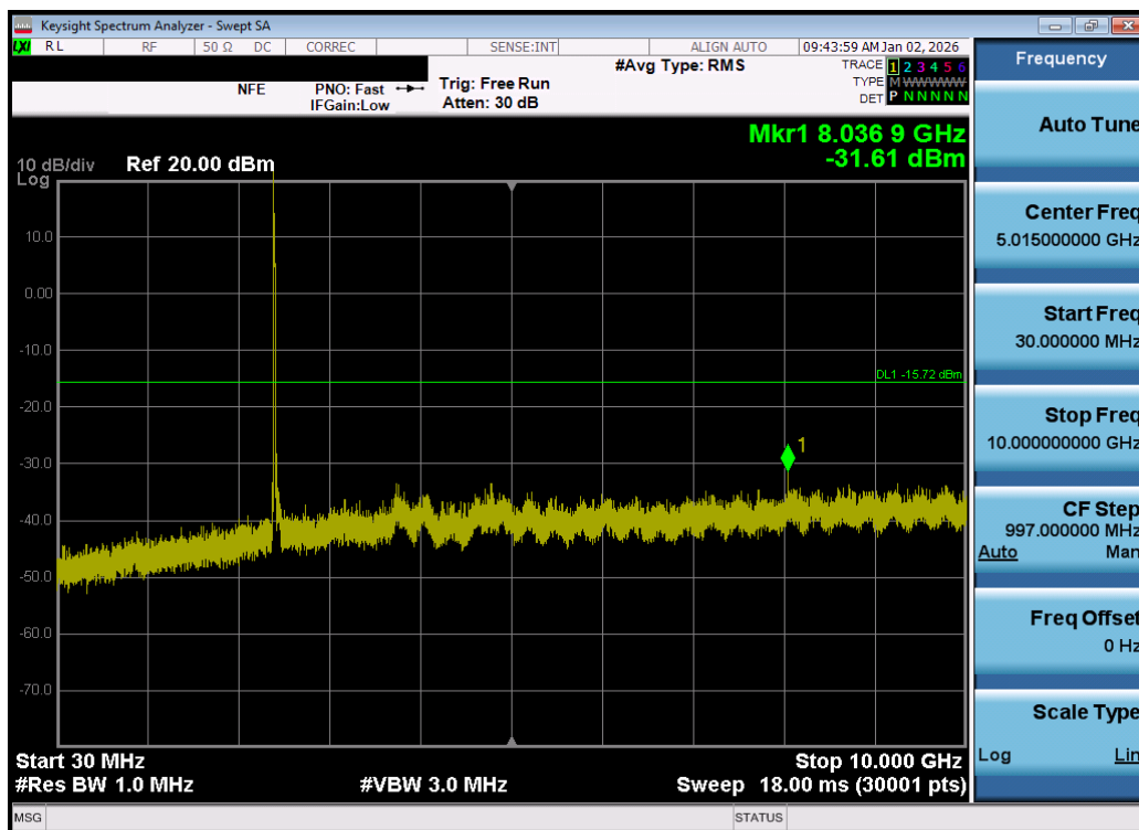
Plot 7-115. Conducted Spurious Plot MIMO ANT1 (802.11be OFDMA – 26 Tones – Ch. 1) – DUAL ANT 1
