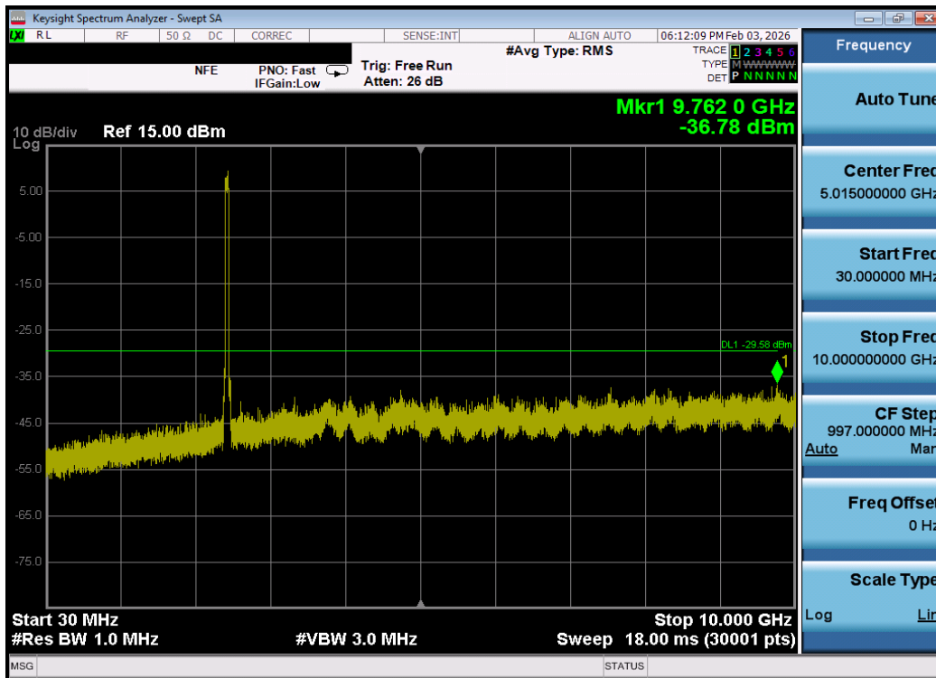
Plot 7-129. Conducted Spurious Plot MIMO ANT1 (802.11be OFDMA – 484 Tones – Ch. 6) – DUAL ANT 1
