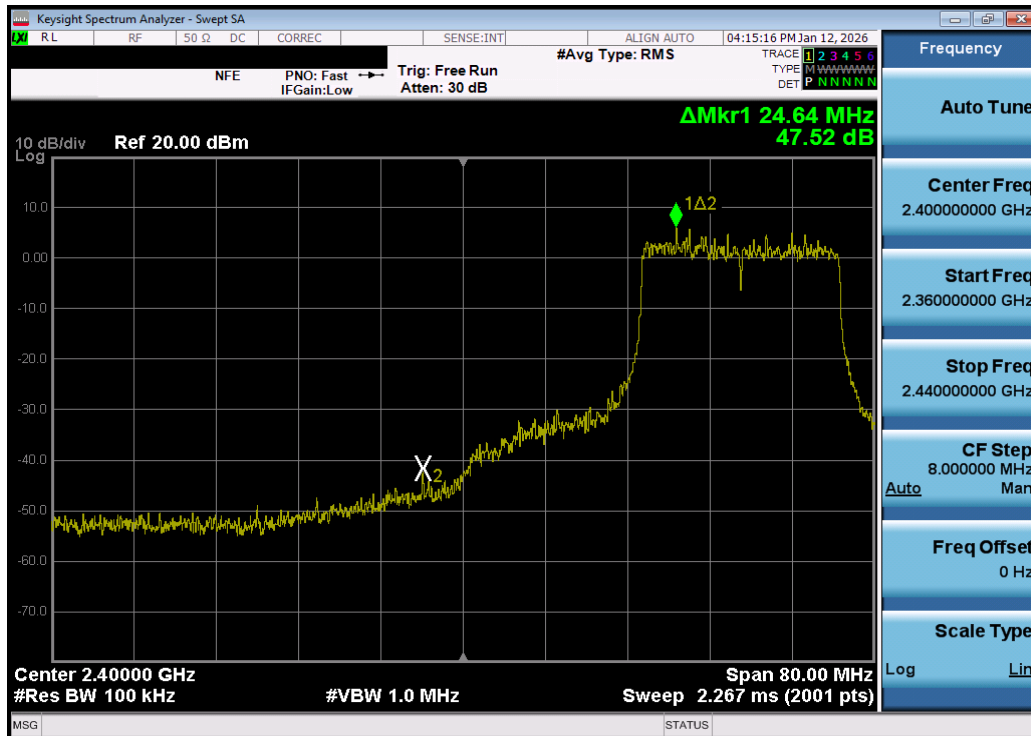
Plot 7-104. Band Edge Plot MIMO ANT2 (802.11be OFDMA – 242 Tones – Ch. 4) – DUAL ANT 2
