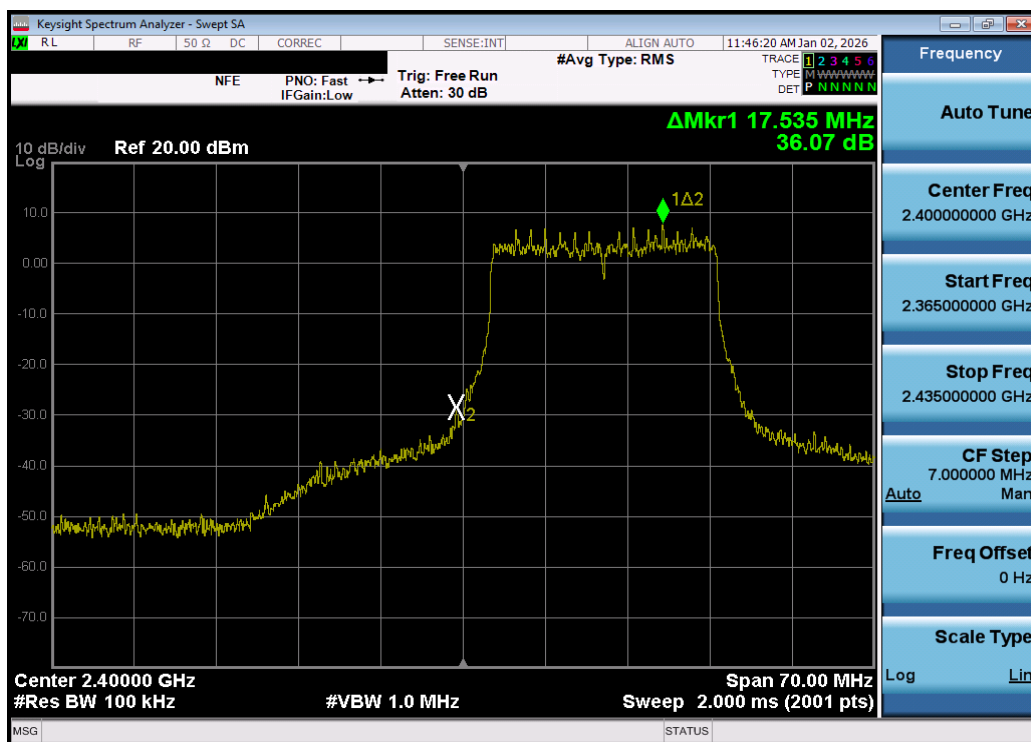
Plot 7-101. Band Edge Plot MIMO ANT2 (802.11be OFDMA – 242 Tones – Ch. 1) – DUAL ANT 2
