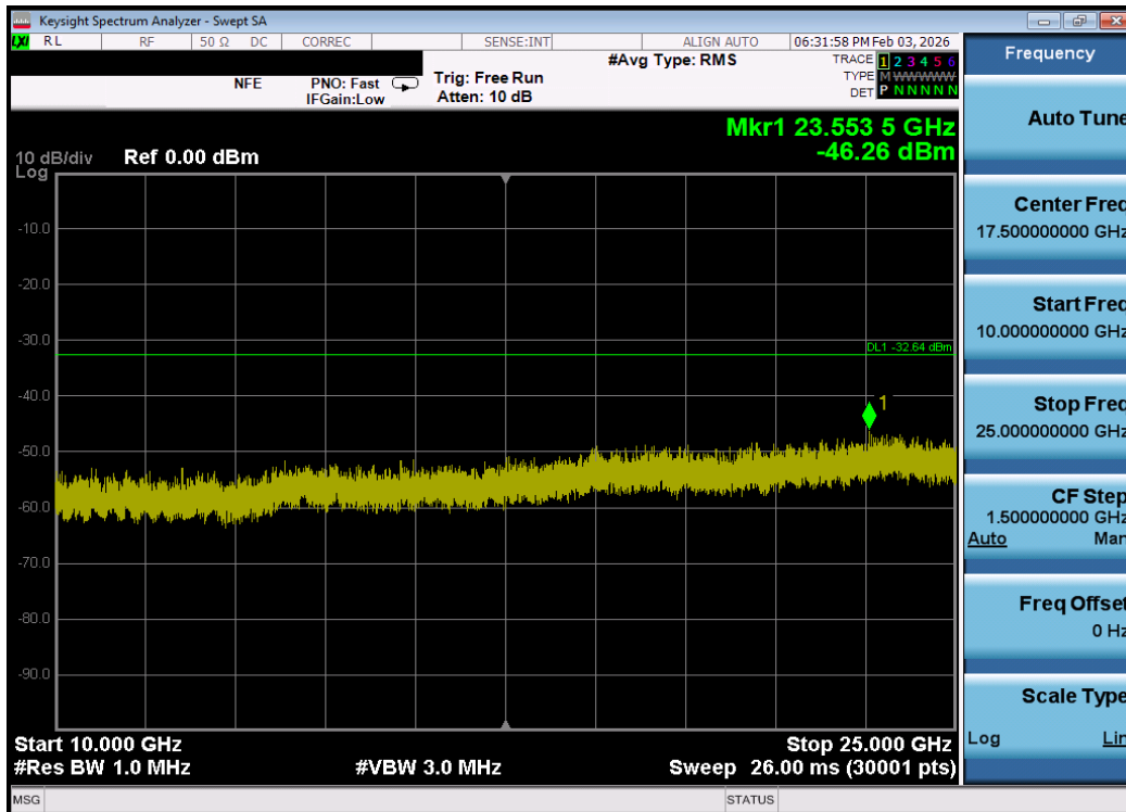
Plot 7-146. Conducted Spurious Plot MIMO ANT2 (802.11be OFDMA – 484 Tones – Ch. 3) – DUAL ANT 2
