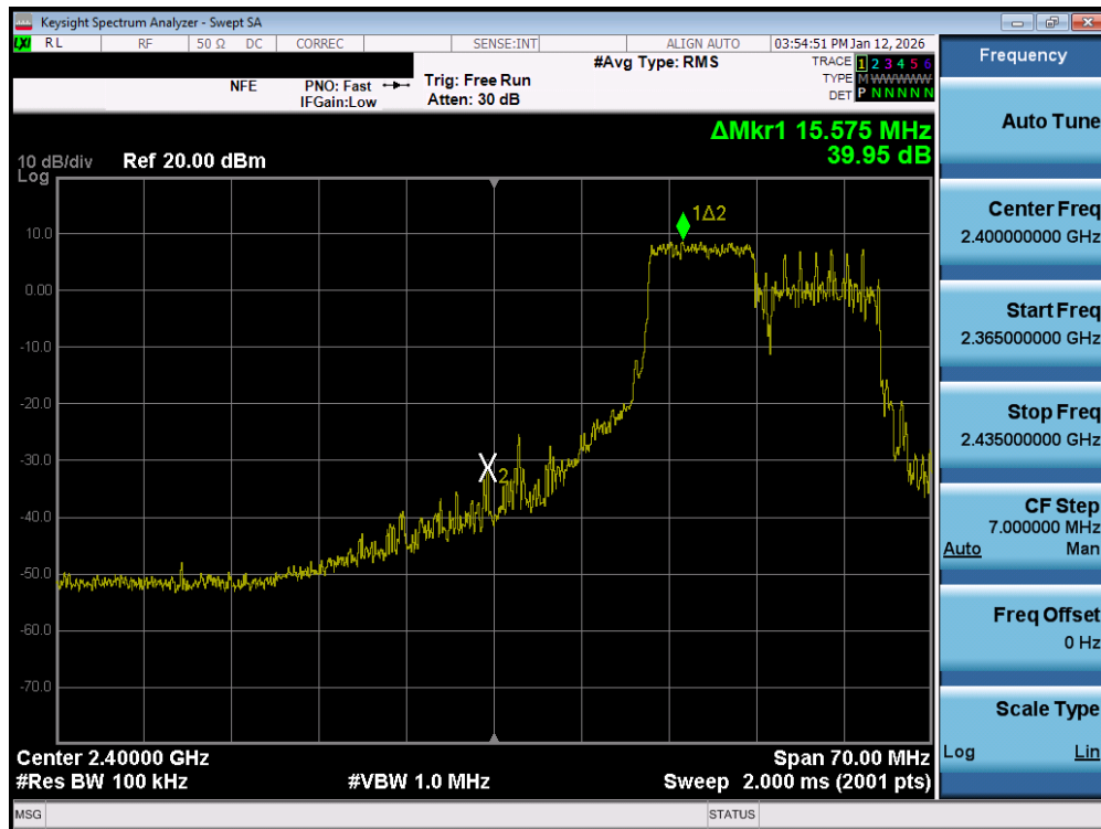
Plot 7-90. Band Edge Plot MIMO ANT2 (802.11be OFDMA – 106 Tones – Ch. 3) – DUAL ANT 2
