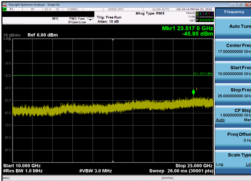
Plot 7-148. Conducted Spurious Plot MIMO ANT2 (802.11be OFDMA – 484 Tones – Ch. 6) – DUAL ANT 2
