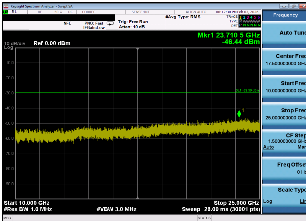
Plot 7-130. Conducted Spurious Plot MIMO ANT1 (802.11be OFDMA – 484 Tones – Ch. 6) – DUAL ANT 1
