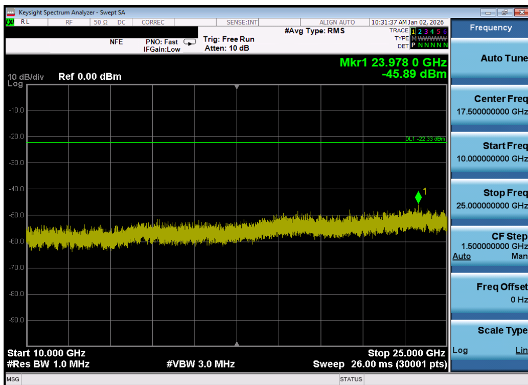
Plot 7-122. Conducted Spurious Plot MIMO ANT1 (802.11be OFDMA – 242 Tones – Ch. 1) – DUAL ANT 1
