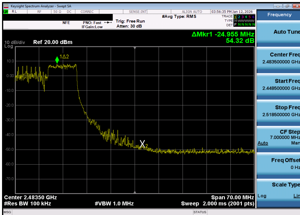
Plot 7-91. Band Edge Plot MIMO ANT2 (802.11be OFDMA – 106 Tones – Ch. 10) – DUAL ANT 2
