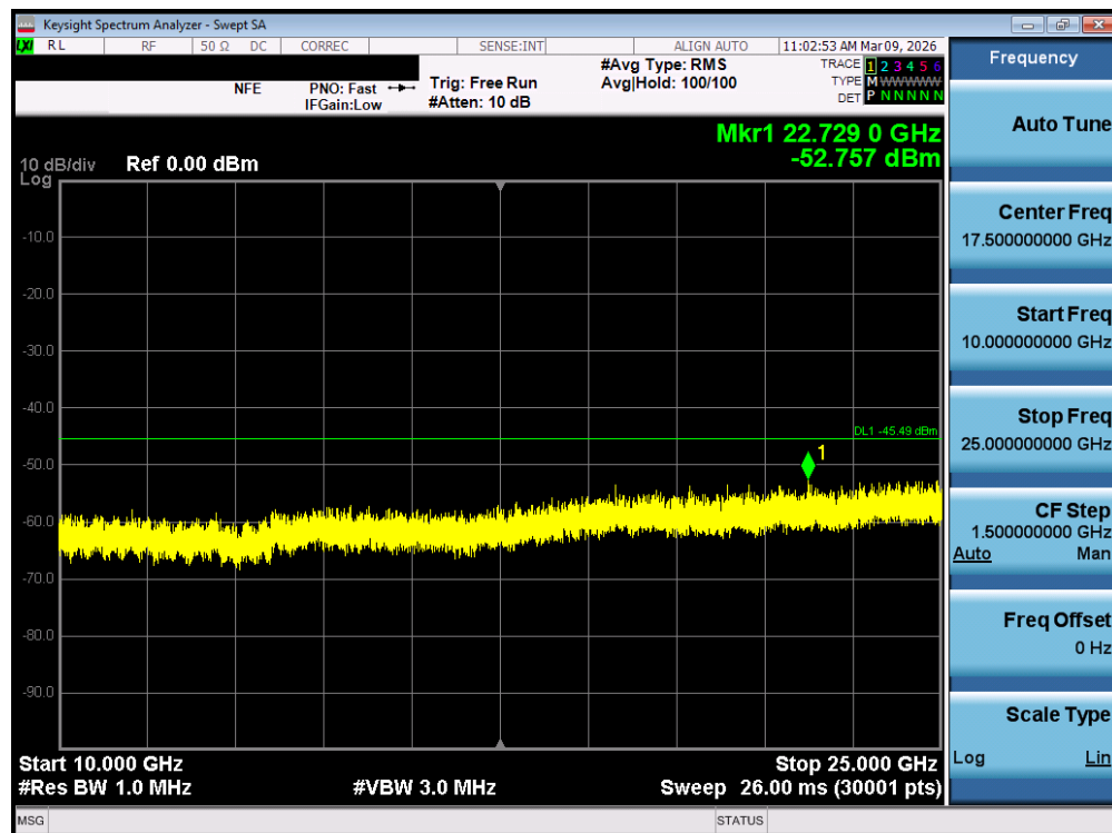
Plot 7-132. Conducted Spurious Plot MIMO ANT1 (802.11be OFDMA – 484 Tones – Ch. 11) – DUAL ANT 1
