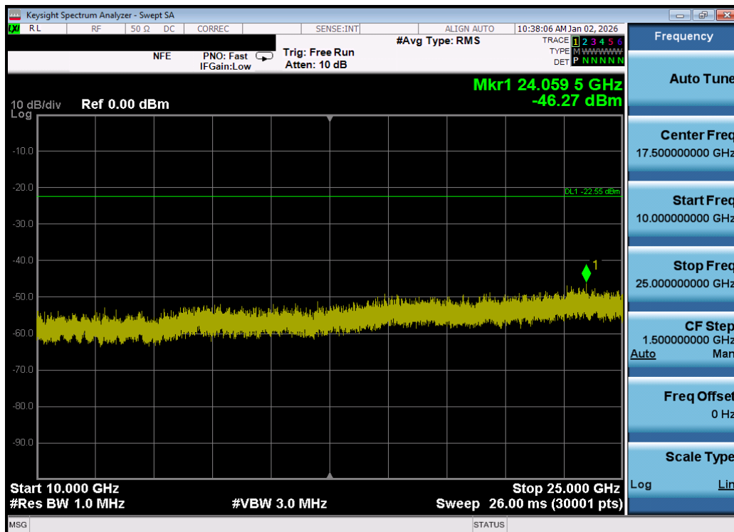
Plot 7-124. Conducted Spurious Plot MIMO ANT1 (802.11be OFDMA – 242 Tones – Ch. 6) – DUAL ANT 1
