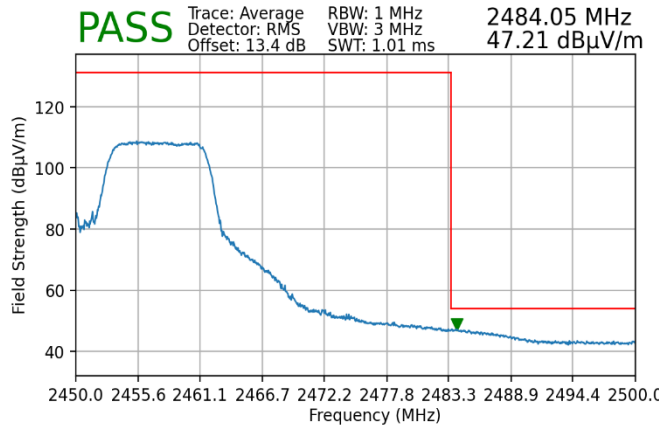
Plot 7-163. Radiated Restricted Upper Band Edge Measurement MIMO (Average – 106 Tones)
