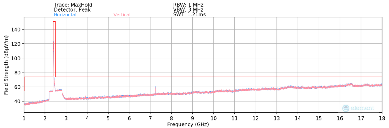
Plot 7-151. Radiated Spurious Plot above 1GHz MIMO (802.11be OFDMA – 26 Tones – Ch. 1)
