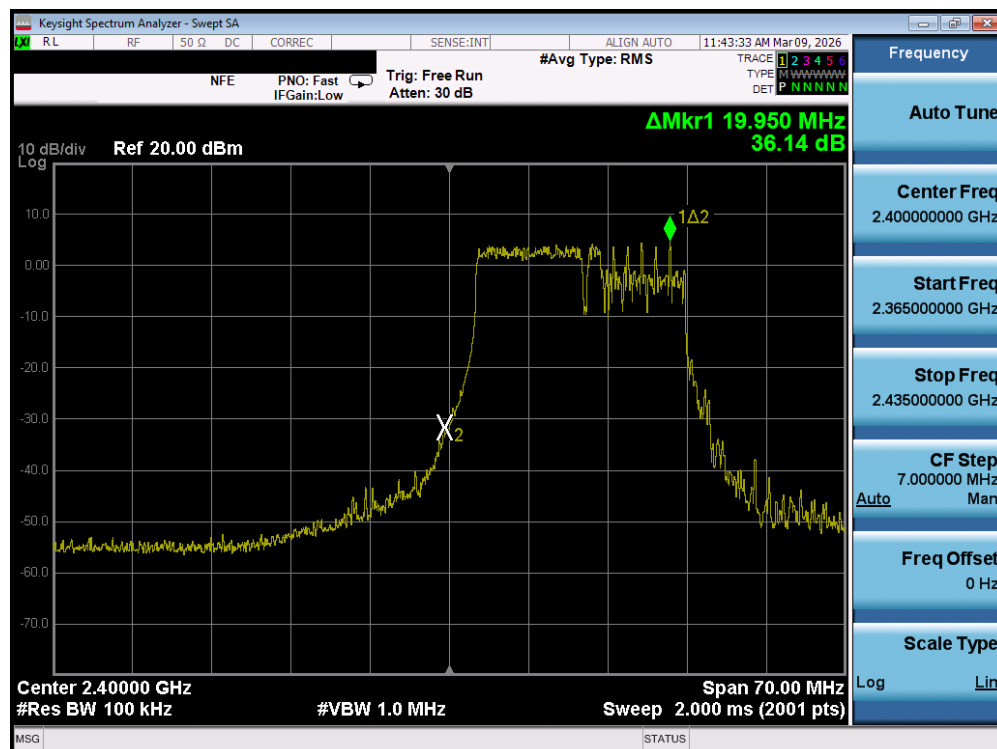
Plot 7-95. Band Edge Plot MIMO ANT1 (802.11be OFDMA – 106 + 26 Tones – Ch. 1) – DUAL ANT 2
