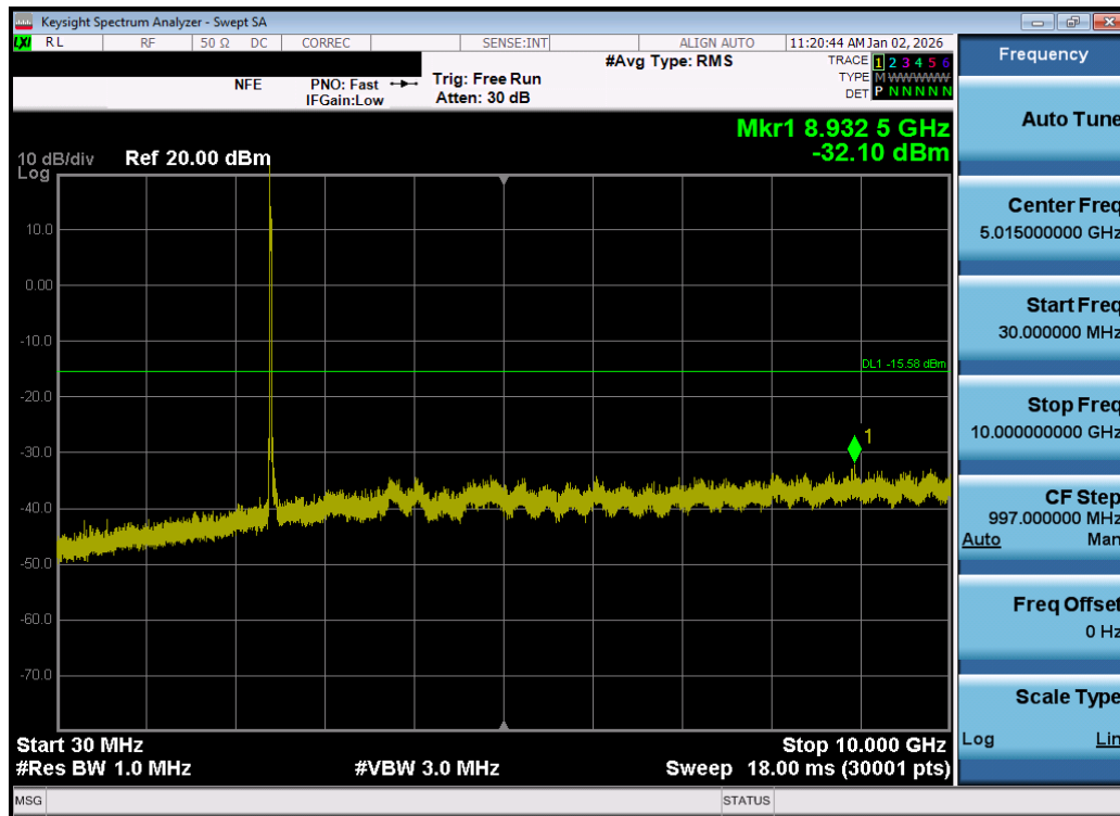
Plot 7-133. Conducted Spurious Plot MIMO ANT2 (802.11be OFDMA – 26 Tones – Ch. 1) – DUAL ANT 2
