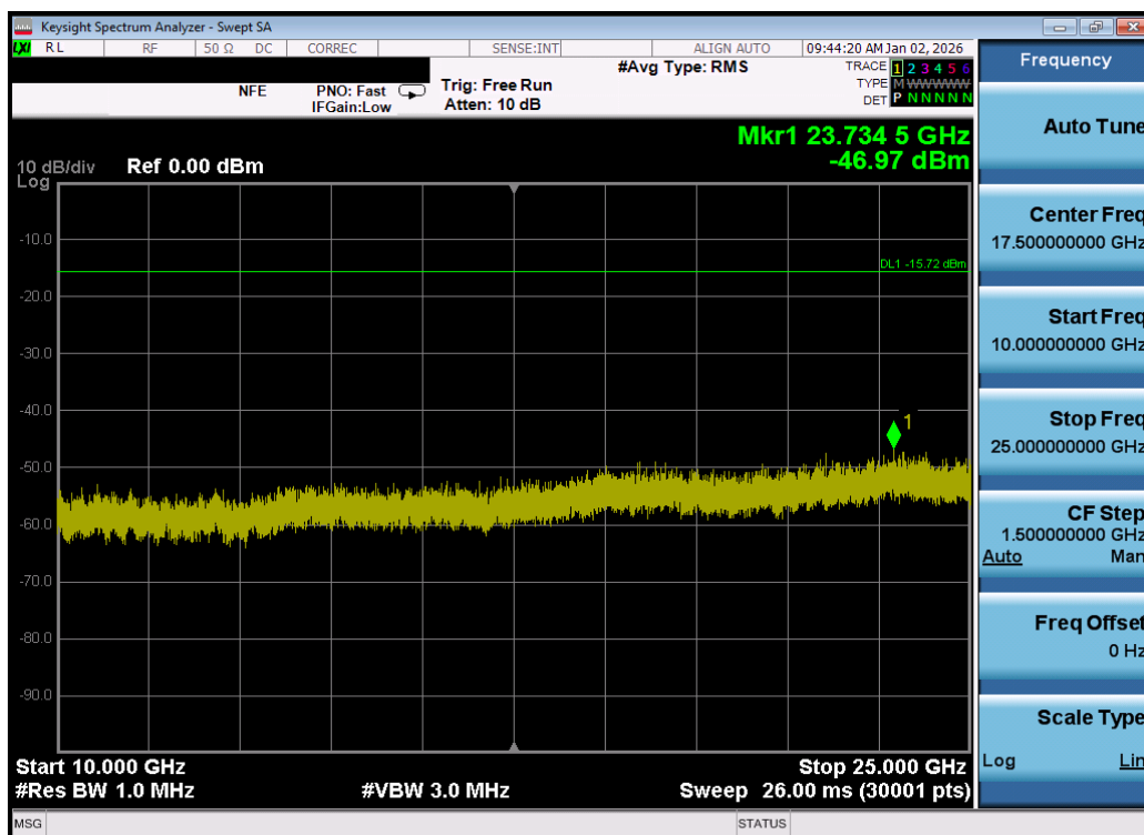
Plot 7-116. Conducted Spurious Plot MIMO ANT1 (802.11be OFDMA – 26 Tones – Ch. 1) – DUAL ANT 1
