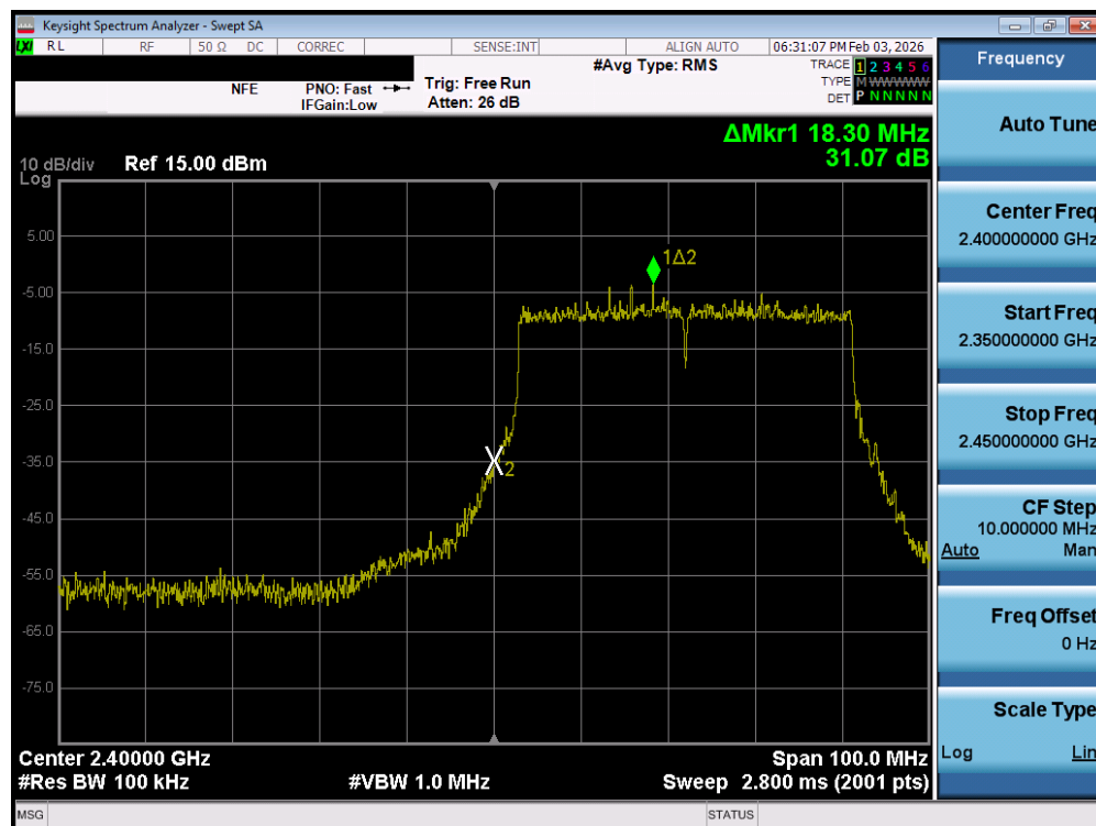
Plot 7-109. Band Edge Plot MIMO ANT2 (802.11be OFDMA – 484 Tones – Ch. 3) – DUAL ANT 2
