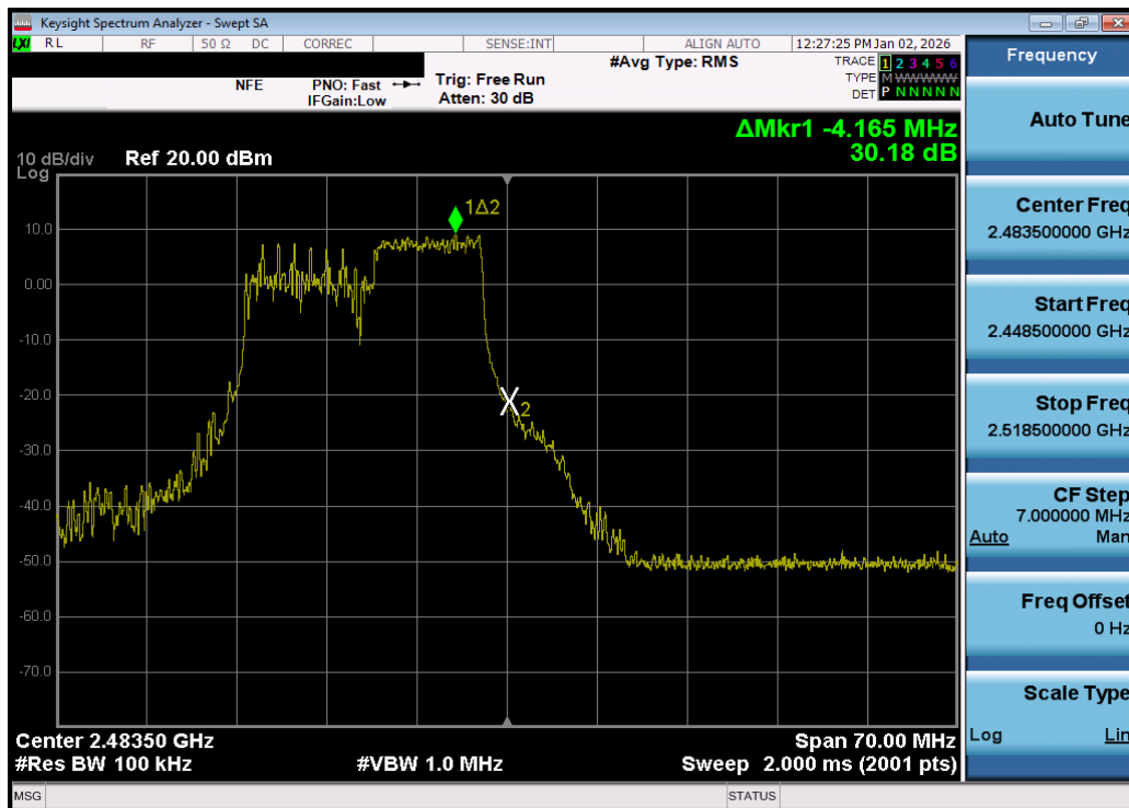
Plot 7-94. Band Edge Plot MIMO ANT2 (802.11be OFDMA – 106 Tones – Ch. 13) – DUAL ANT 2
