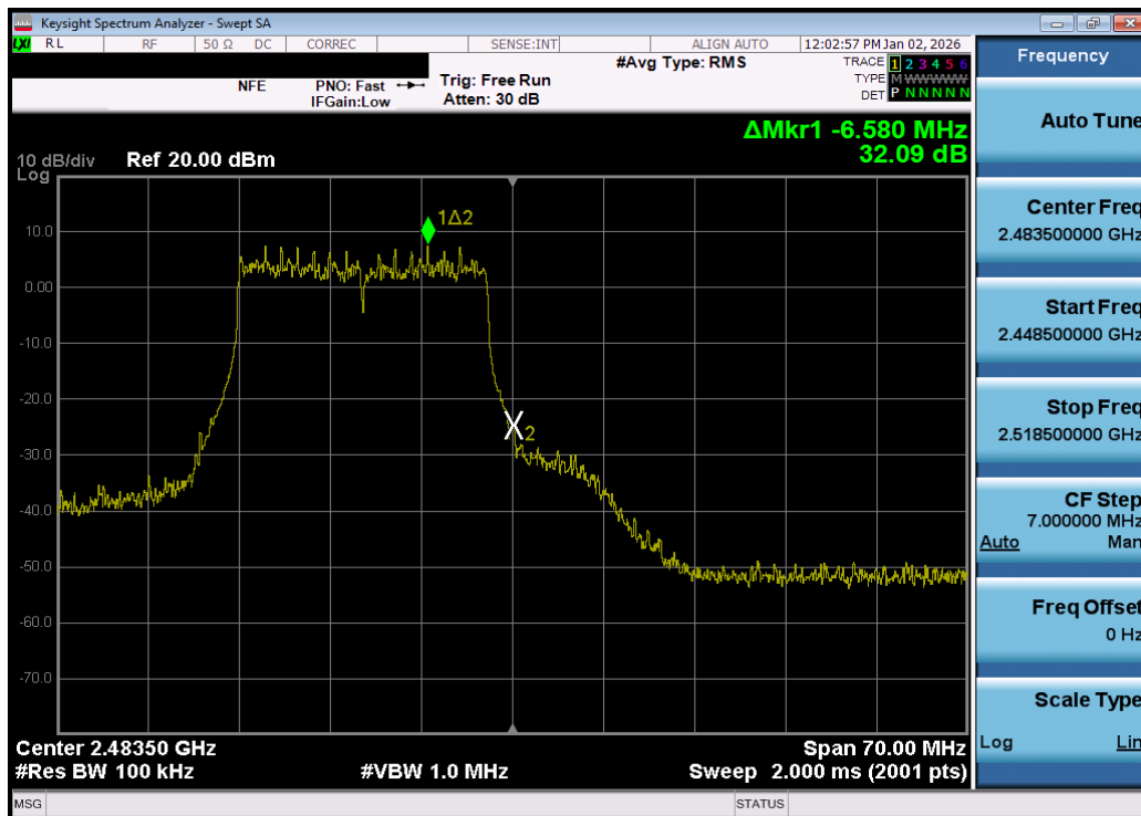
Plot 7-108. Band Edge Plot MIMO ANT2 (802.11be OFDMA – 242 Tones – Ch. 13) – DUAL ANT 2
