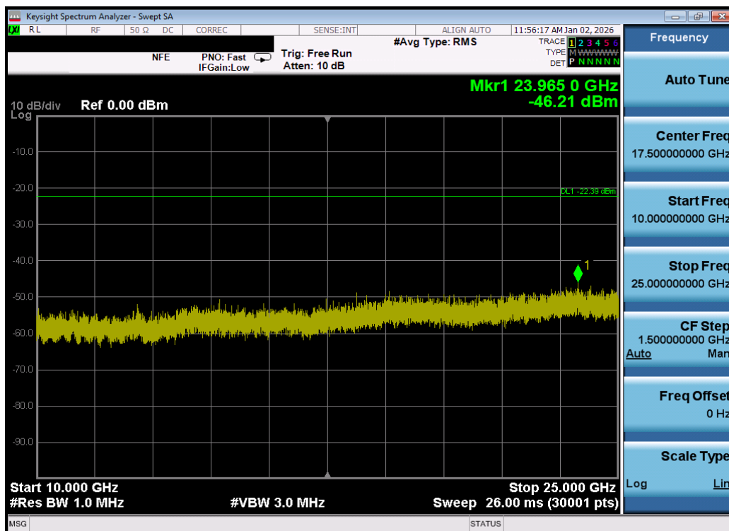
Plot 7-144. Conducted Spurious Plot MIMO ANT2 (802.11be OFDMA – 242 Tones – Ch. 11) – DUAL ANT 2
