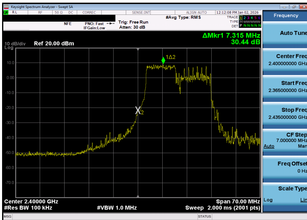
Plot 7-88. Band Edge Plot MIMO ANT2 (802.11be OFDMA – 106 Tones – Ch. 1) – DUAL ANT 2
