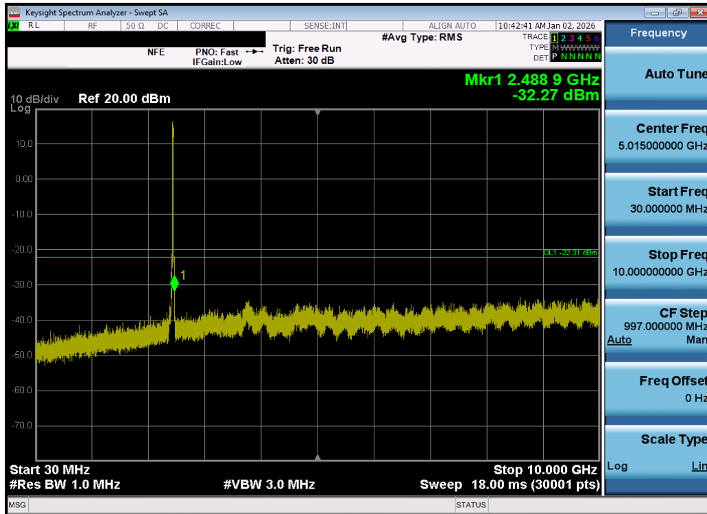
Plot 7-125. Conducted Spurious Plot MIMO ANT1 (802.11be OFDMA – 242 Tones – Ch. 11) – DUAL ANT 1
