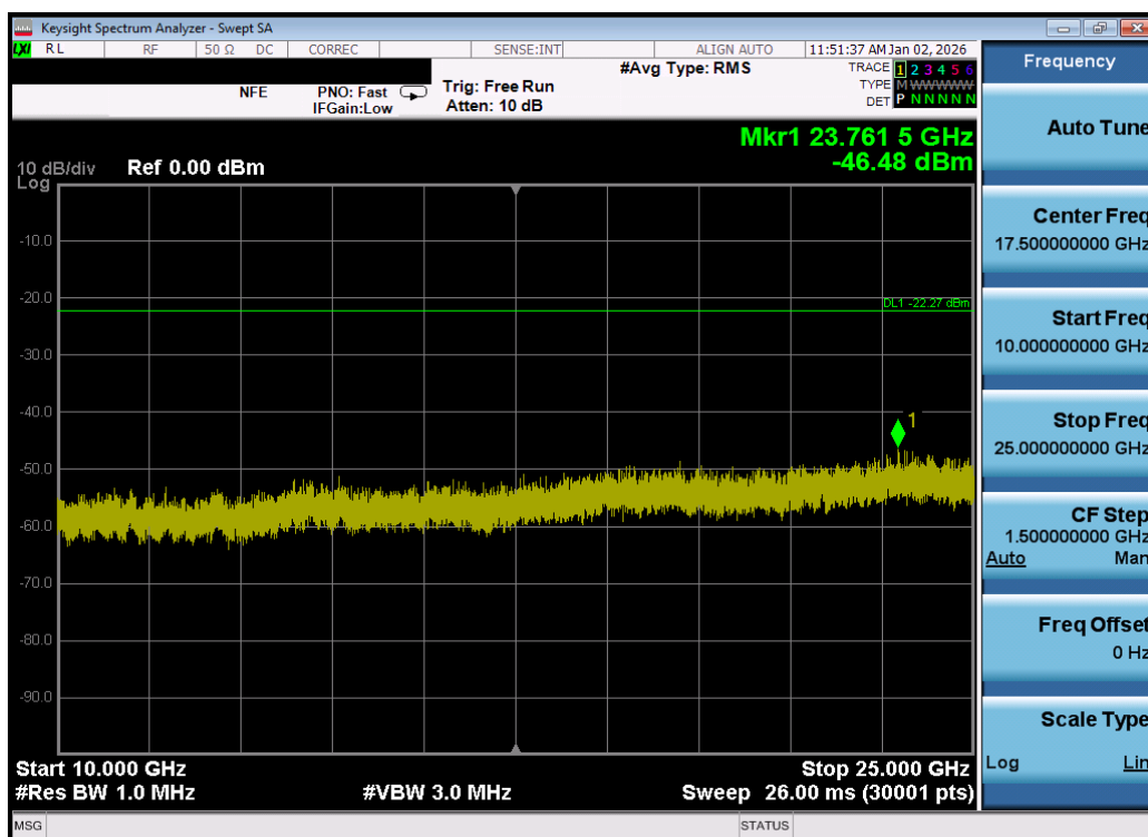
Plot 7-142. Conducted Spurious Plot MIMO ANT2 (802.11be OFDMA – 242 Tones – Ch. 6) – DUAL ANT 2
