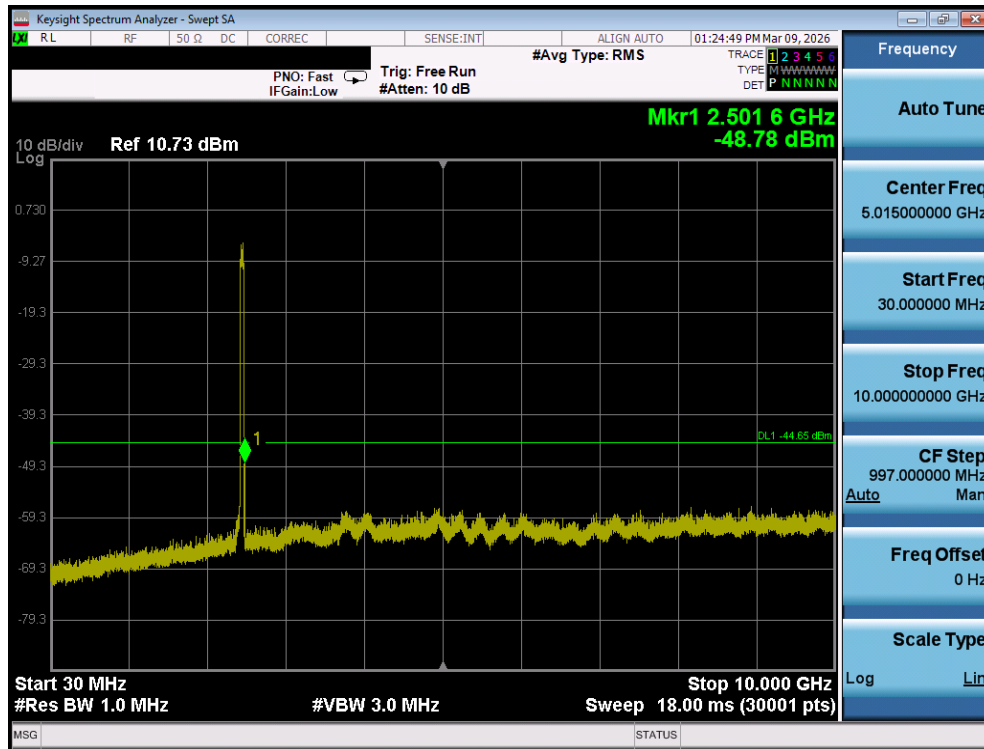
Plot 7-149. Conducted Spurious Plot MIMO ANT2 (802.11be OFDMA – 484 Tones – Ch. 11) – DUAL ANT 2
