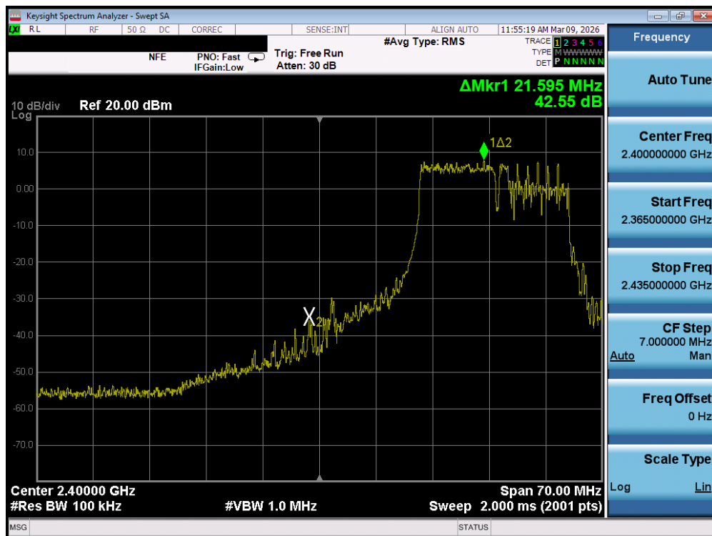
Plot 7-97. Band Edge Plot MIMO ANT1 (802.11be OFDMA – 106 + 26 Tones – Ch. 3) – DUAL ANT 2
