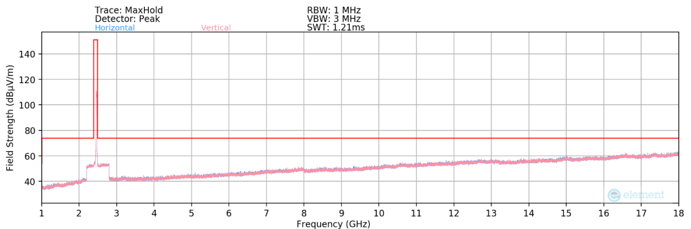
Plot 7-156. Radiated Spurious Plot above 1GHz MIMO (802.11be OFDMA – 242 Tones – Ch. 11)
