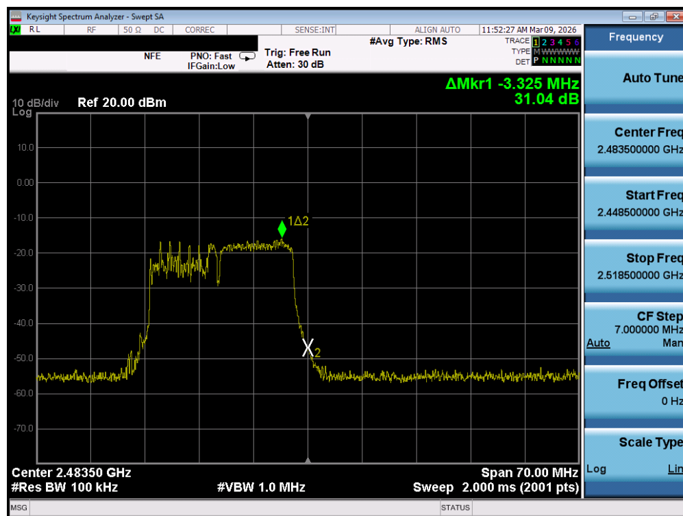
Plot 7-100. Band Edge Plot MIMO ANT1 (802.11be OFDMA – 106 + 26 Tones – Ch. 13) – DUAL ANT 2
