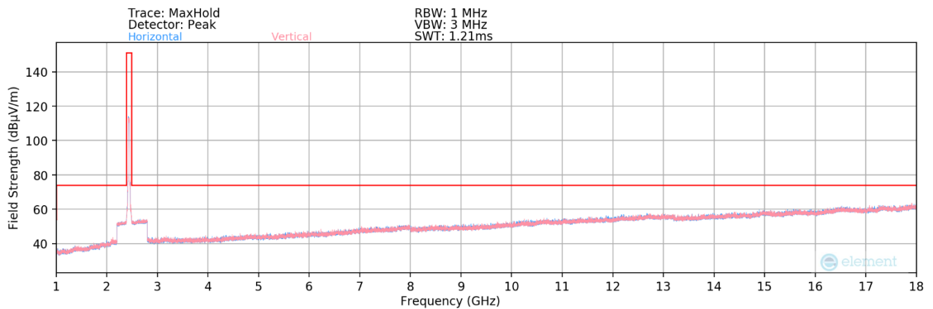
Plot 7-155. Radiated Spurious Plot above 1GHz MIMO (802.11be OFDMA – 242 Tones – Ch. 6)
