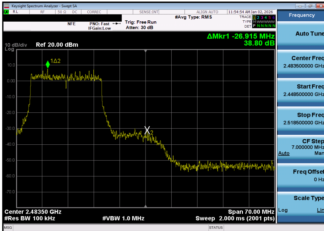
Plot 7-106. Band Edge Plot MIMO ANT2 (802.11be OFDMA – 242 Tones – Ch. 11) – DUAL ANT 2
