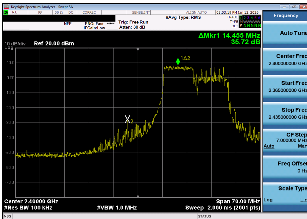
Plot 7-89. Band Edge Plot MIMO ANT2 (802.11be OFDMA – 106 Tones – Ch. 2) – DUAL ANT 2
