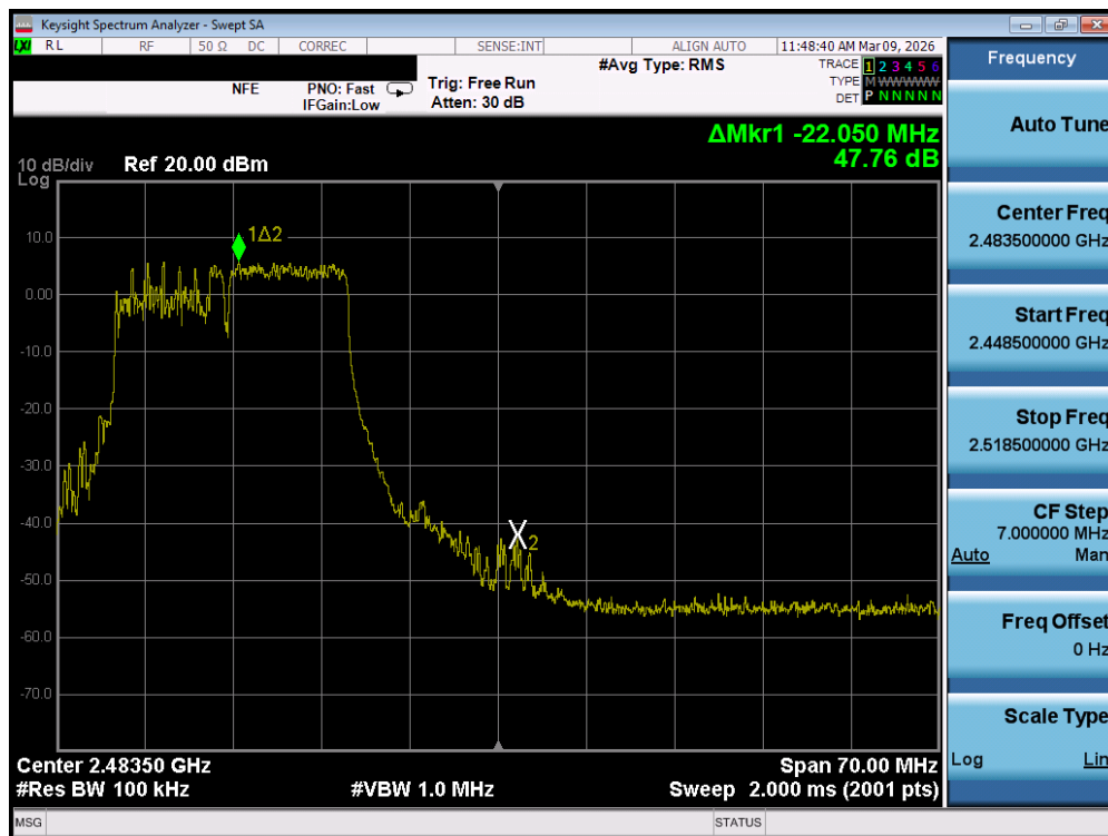
Plot 7-98. Band Edge Plot MIMO ANT1 (802.11be OFDMA – 106 + 26 Tones – Ch. 11) – DUAL ANT 2
