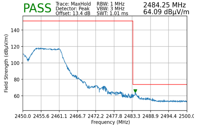
Plot 7-164. Radiated Restricted Upper Band Edge Measurement MIMO (Peak – 106 Tones)
