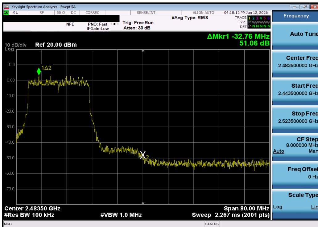
Plot 7-105. Band Edge Plot MIMO ANT2 (802.11be OFDMA – 242 Tones – Ch. 10) – DUAL ANT 2
