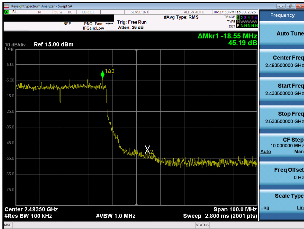
Plot 7-85. Band Edge Plot MIMO ANT1 (802.11be OFDMA – 484 Tones – Ch. 9) – DUAL ANT 1
