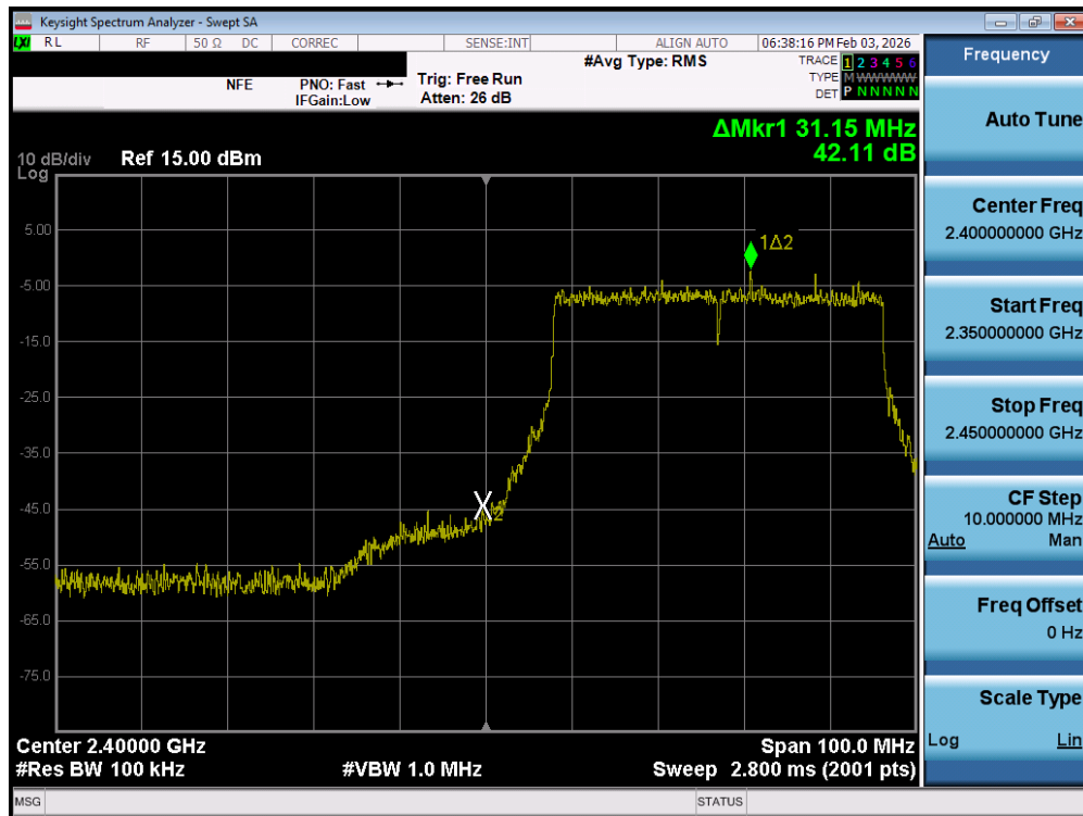
Plot 7-110. Band Edge Plot MIMO ANT2 (802.11be OFDMA – 484 Tones – Ch. 4) – DUAL ANT 2
