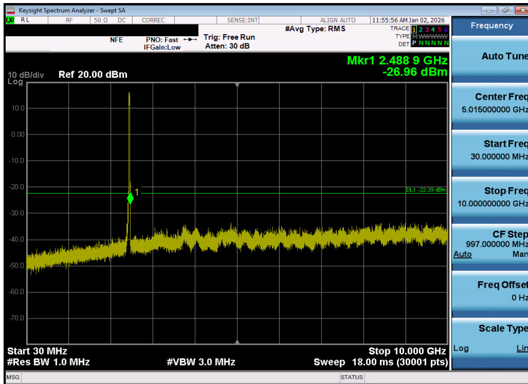
Plot 7-143. Conducted Spurious Plot MIMO ANT2 (802.11be OFDMA – 242 Tones – Ch. 11) – DUAL ANT 2
