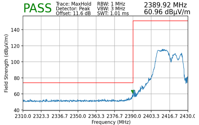
Plot 7-160. Radiated Restricted Lower Band Edge Measurement MIMO (Peak – 106 Tones)
