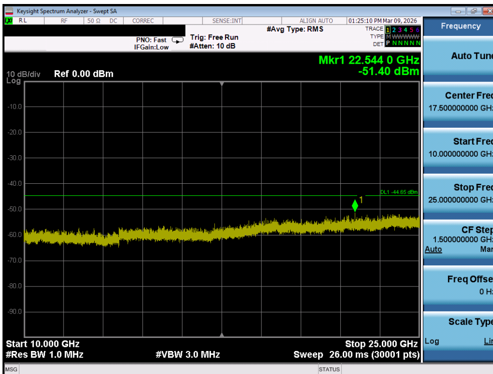
Plot 7-150. Conducted Spurious Plot MIMO ANT2 (802.11be OFDMA – 484 Tones – Ch. 11) – DUAL ANT 2
