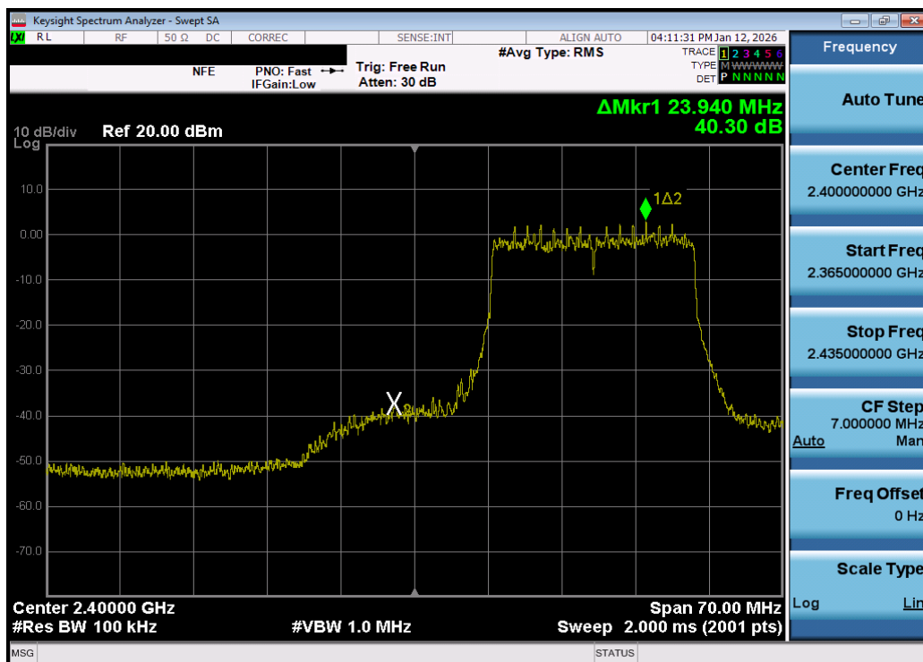
Plot 7-102. Band Edge Plot MIMO ANT2 (802.11be OFDMA – 242 Tones – Ch. 2) – DUAL ANT 2
