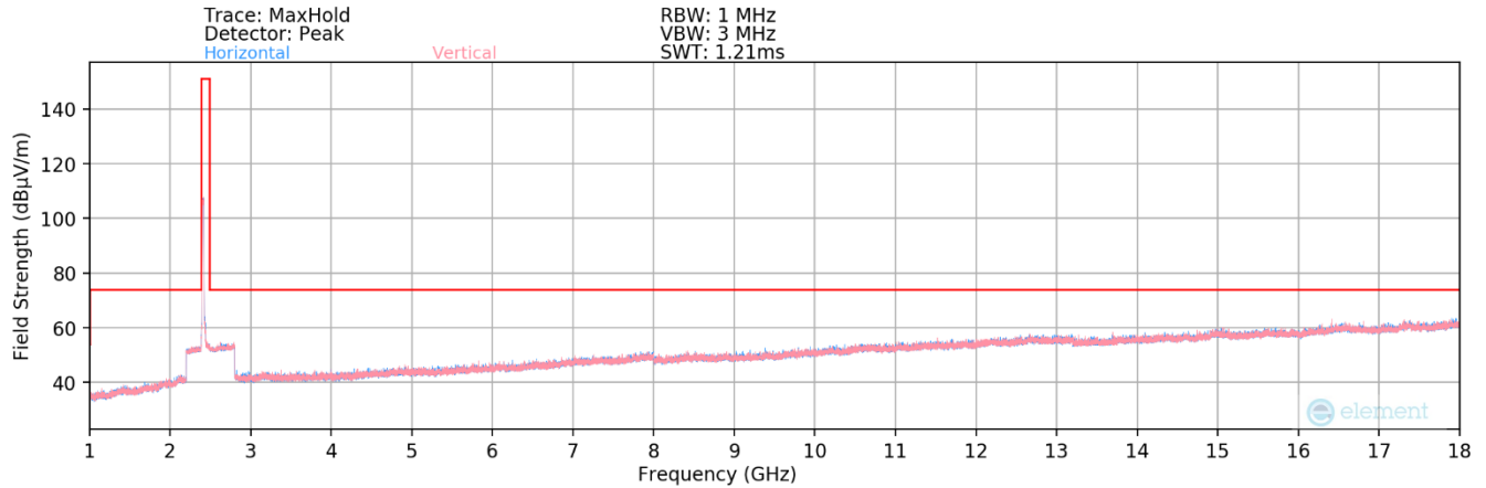
Plot 7-154. Radiated Spurious Plot above 1GHz MIMO (802.11be OFDMA – 242 Tones – Ch. 1)
