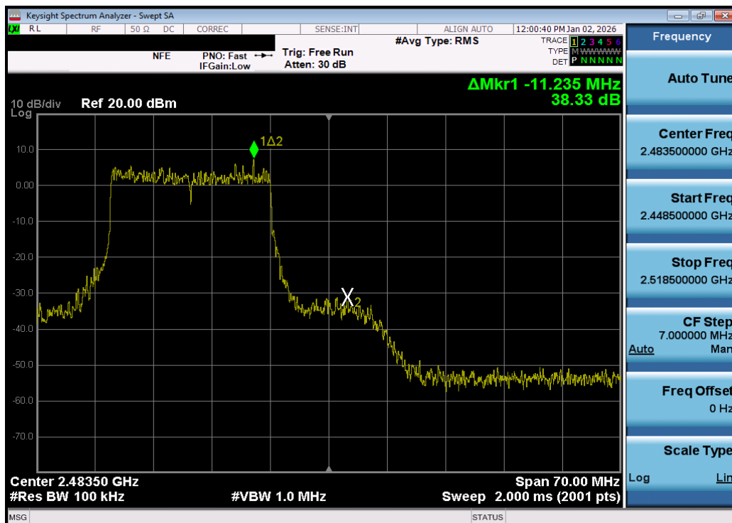
Plot 7-107. Band Edge Plot MIMO ANT2 (802.11be OFDMA – 242 Tones – Ch. 12) – DUAL ANT 2
