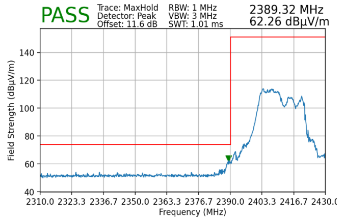
Plot 7-158. Radiated Restricted Lower Band Edge Measurement MIMO (Peak – 106 Tones)
