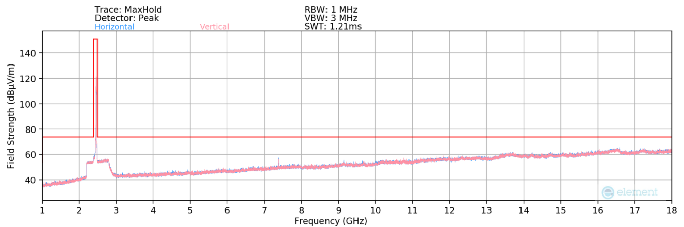
Plot 7-153. Radiated Spurious Plot above 1GHz MIMO (802.11be OFDMA – 26 Tones – Ch. 11)
