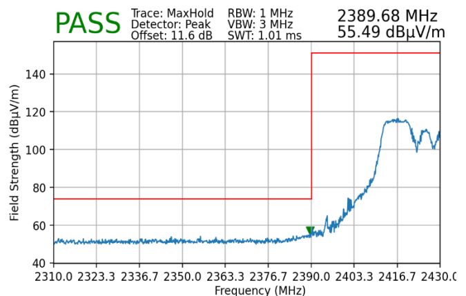
Plot 7-162. Radiated Restricted Lower Band Edge Measurement MIMO (Peak – 106 Tones)
