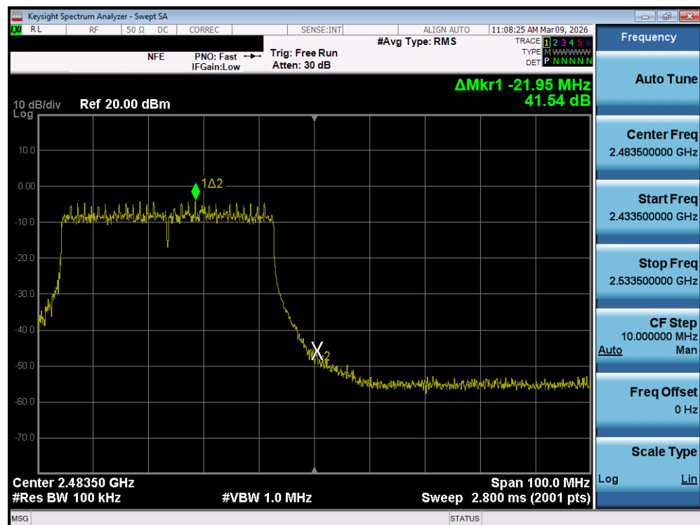
Plot 7-86. Band Edge Plot MIMO ANT1 (802.11be OFDMA – 484 Tones – Ch. 10) – DUAL ANT 1
