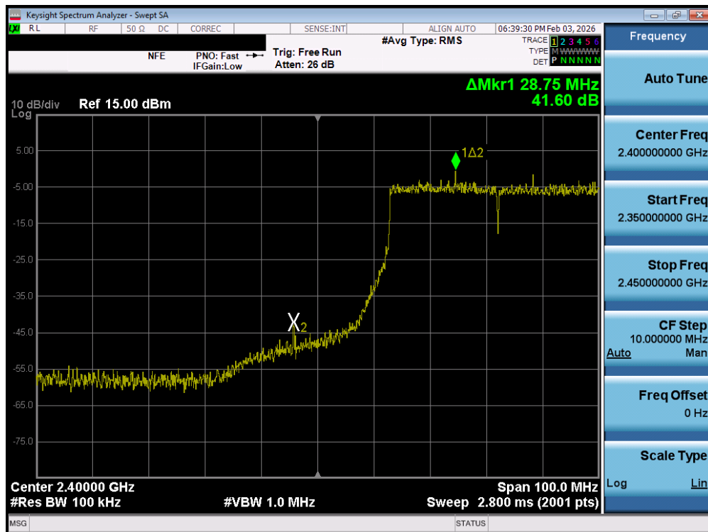
Plot 7-111. Band Edge Plot MIMO ANT2 (802.11be OFDMA – 484 Tones – Ch. 5) – DUAL ANT 2
