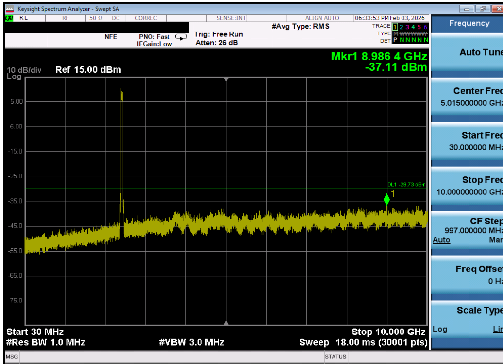
Plot 7-147. Conducted Spurious Plot MIMO ANT2 (802.11be OFDMA – 484 Tones – Ch. 6) – DUAL ANT 2
