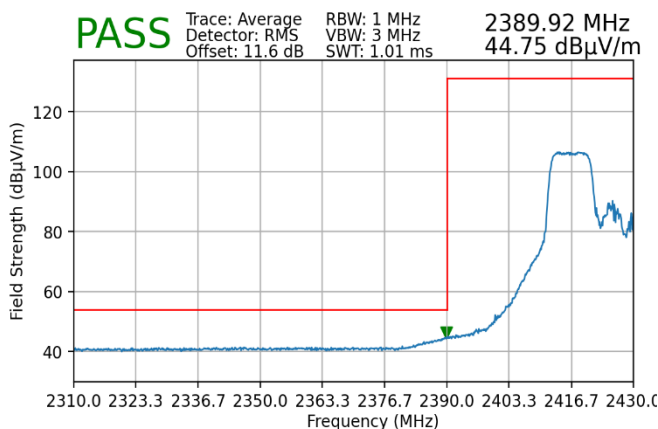
Plot 7-161. Radiated Restricted Lower Band Edge Measurement MIMO (Average – 106 Tones)
