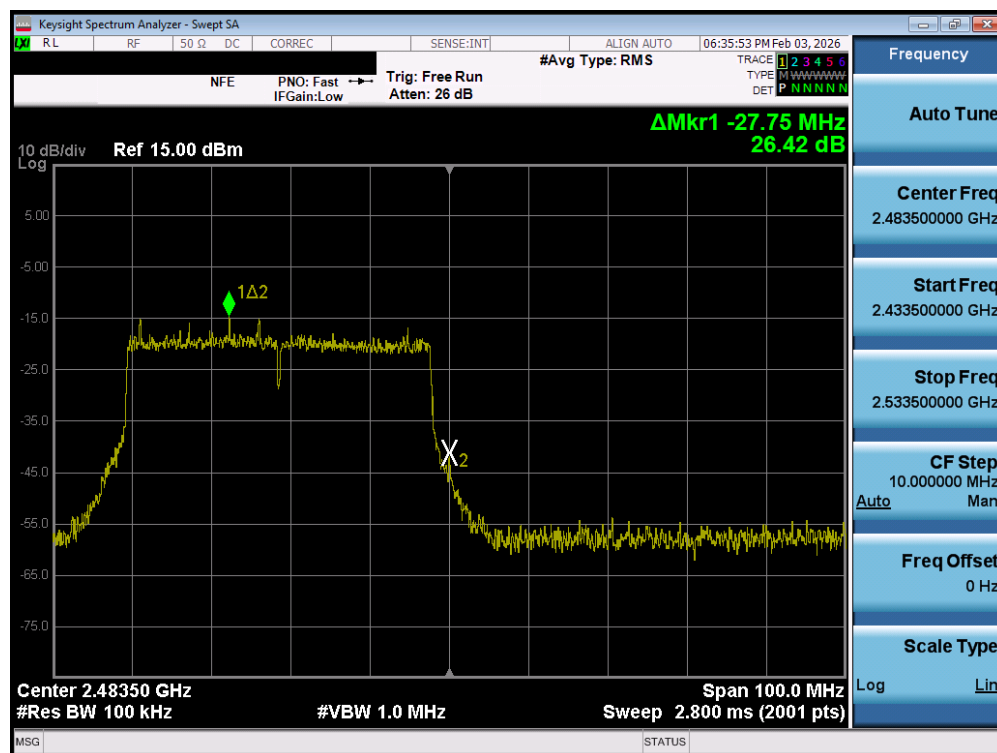
Plot 7-114. Band Edge Plot MIMO ANT2 (802.11be OFDMA – 484 Tones – Ch. 11) – DUAL ANT 2
