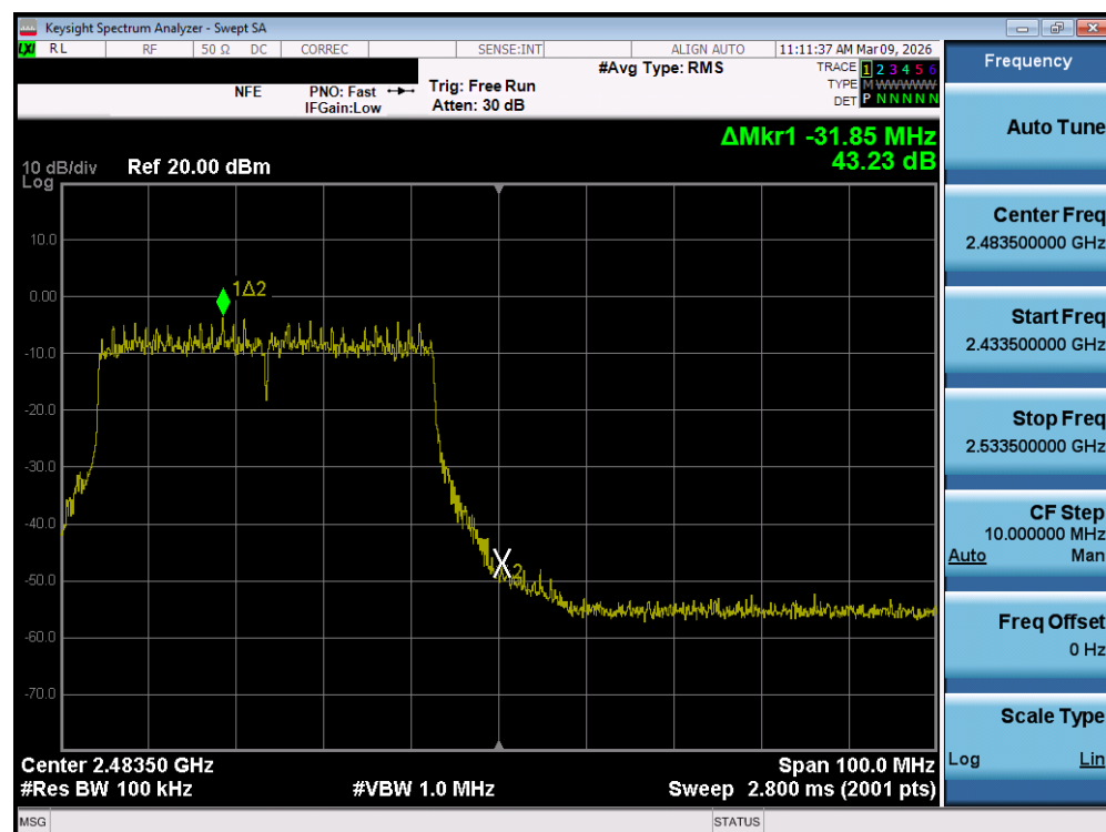
Plot 7-113. Band Edge Plot MIMO ANT2 (802.11be OFDMA – 484 Tones – Ch. 10) – DUAL ANT 2
