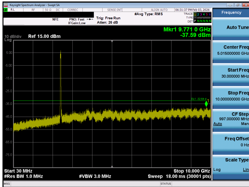
Plot 7-145. Conducted Spurious Plot MIMO ANT2 (802.11be OFDMA – 484 Tones – Ch. 3) – DUAL ANT 2
