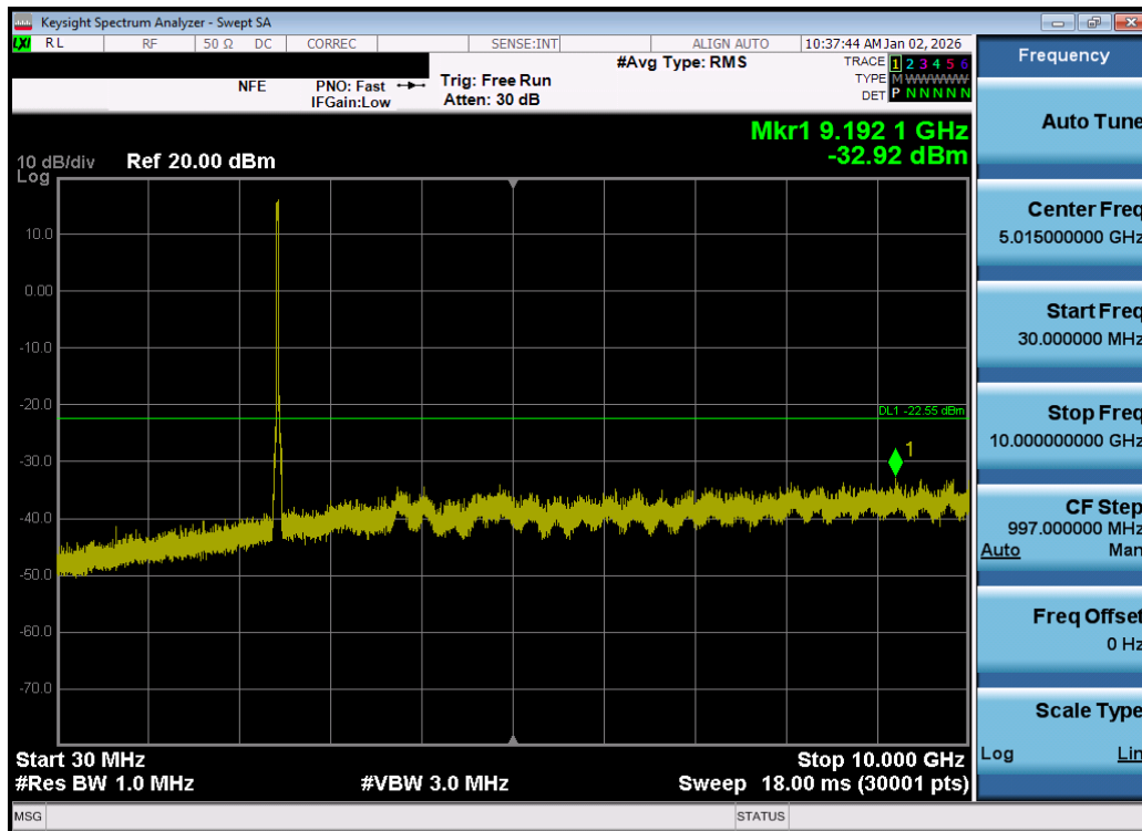
Plot 7-123. Conducted Spurious Plot MIMO ANT1 (802.11be OFDMA – 242 Tones – Ch. 6) – DUAL ANT 1
