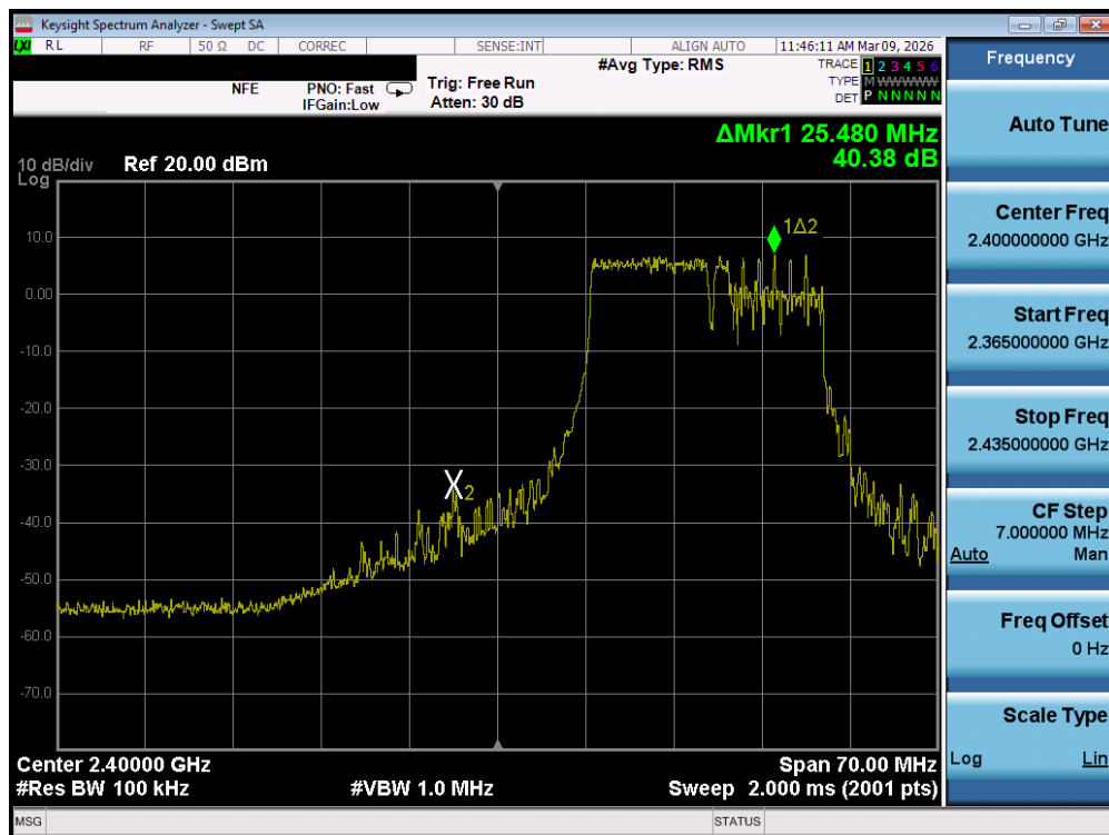
Plot 7-96. Band Edge Plot MIMO ANT1 (802.11be OFDMA – 106 + 26 Tones – Ch. 2) – DUAL ANT 2
