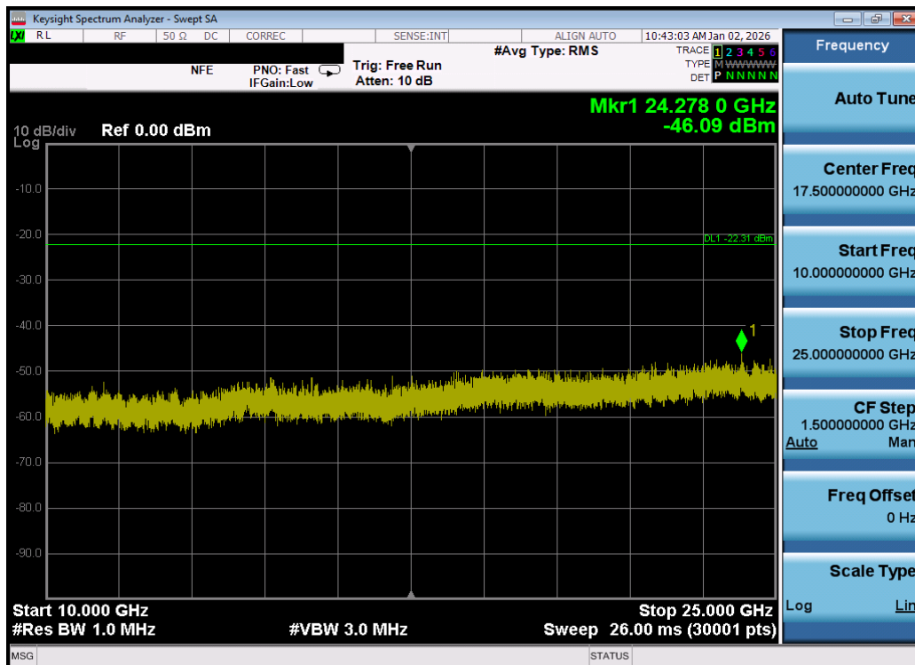
Plot 7-126. Conducted Spurious Plot MIMO ANT1 (802.11be OFDMA – 242 Tones – Ch. 11) – DUAL ANT 1
