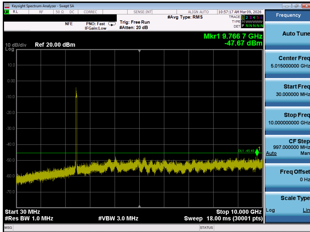
Plot 7-131. Conducted Spurious Plot MIMO ANT1 (802.11be OFDMA – 484 Tones – Ch. 11) – DUAL ANT 1
