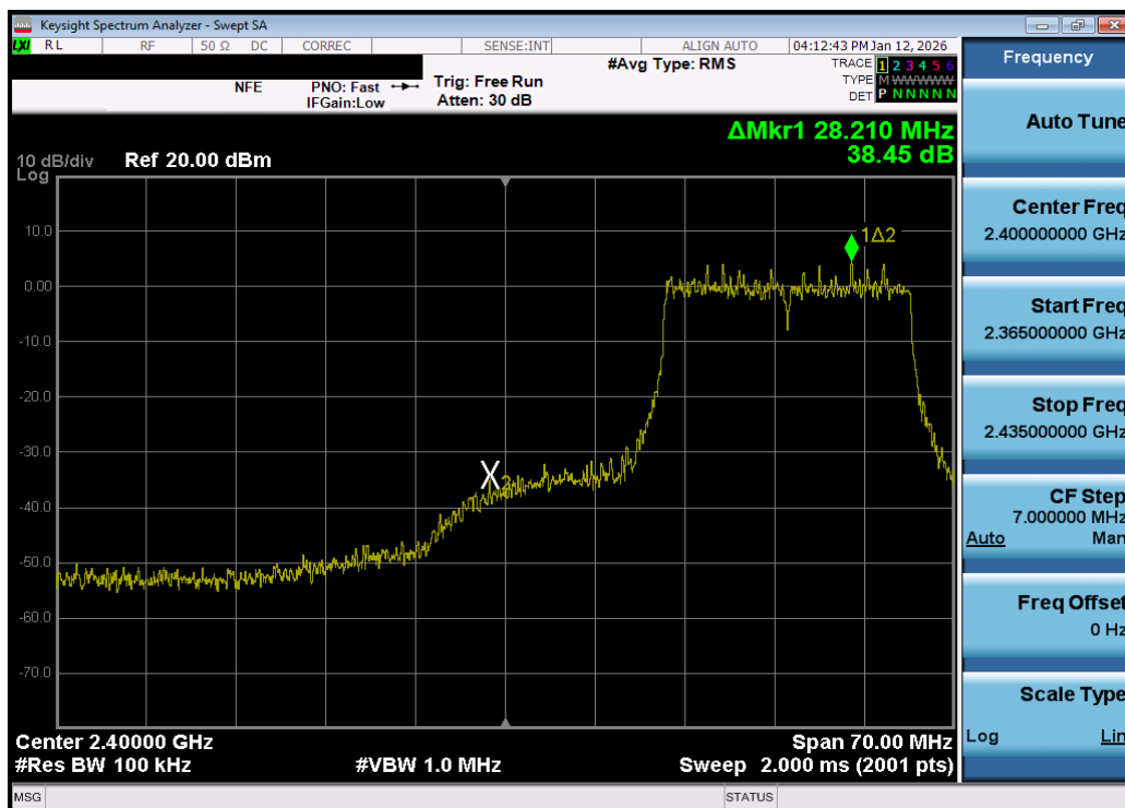
Plot 7-103. Band Edge Plot MIMO ANT2 (802.11be OFDMA – 242 Tones – Ch. 3) – DUAL ANT 2
