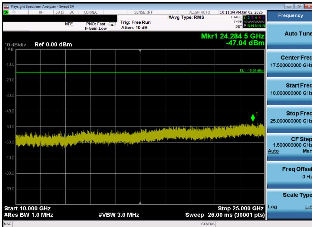
Plot 7-120. Conducted Spurious Plot MIMO ANT1 (802.11be OFDMA – 26 Tones – Ch. 11) – DUAL ANT 1
