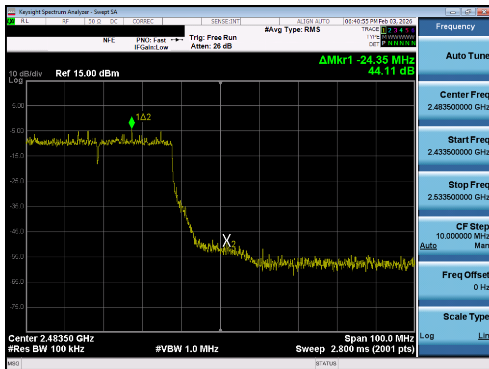
Plot 7-112. Band Edge Plot MIMO ANT2 (802.11be OFDMA – 484 Tones – Ch. 9) – DUAL ANT 2
