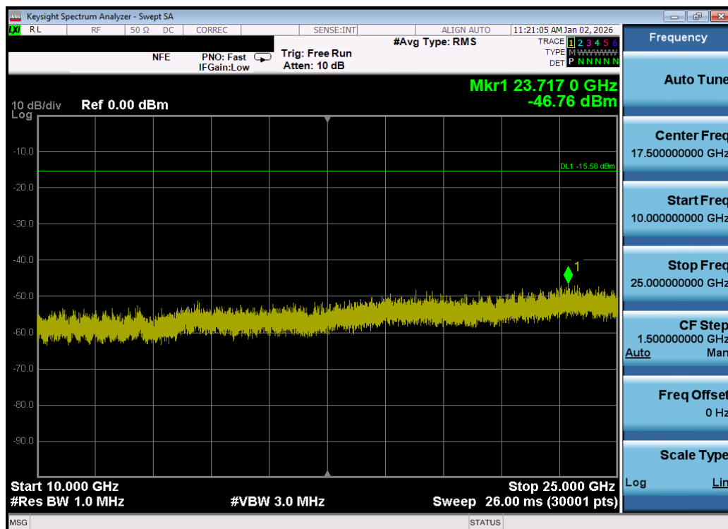
Plot 7-134. Conducted Spurious Plot MIMO ANT2 (802.11be OFDMA – 26 Tones – Ch. 1) – DUAL ANT 2
