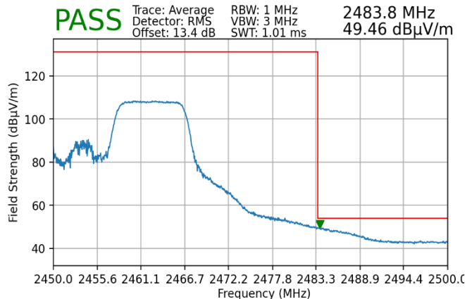
Plot 7-165. Radiated Restricted Upper Band Edge Measurement MIMO (Average – 106 Tones)
