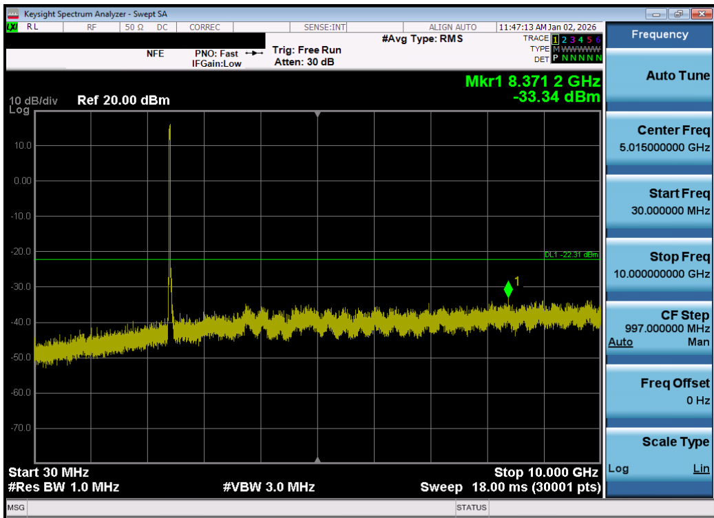
Plot 7-139. Conducted Spurious Plot MIMO ANT2 (802.11be OFDMA – 242 Tones – Ch. 1) – DUAL ANT 2
