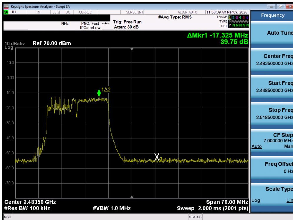
Plot 7-99. Band Edge Plot MIMO ANT1 (802.11be OFDMA – 106 + 26 Tones – Ch. 12) – DUAL ANT 2
