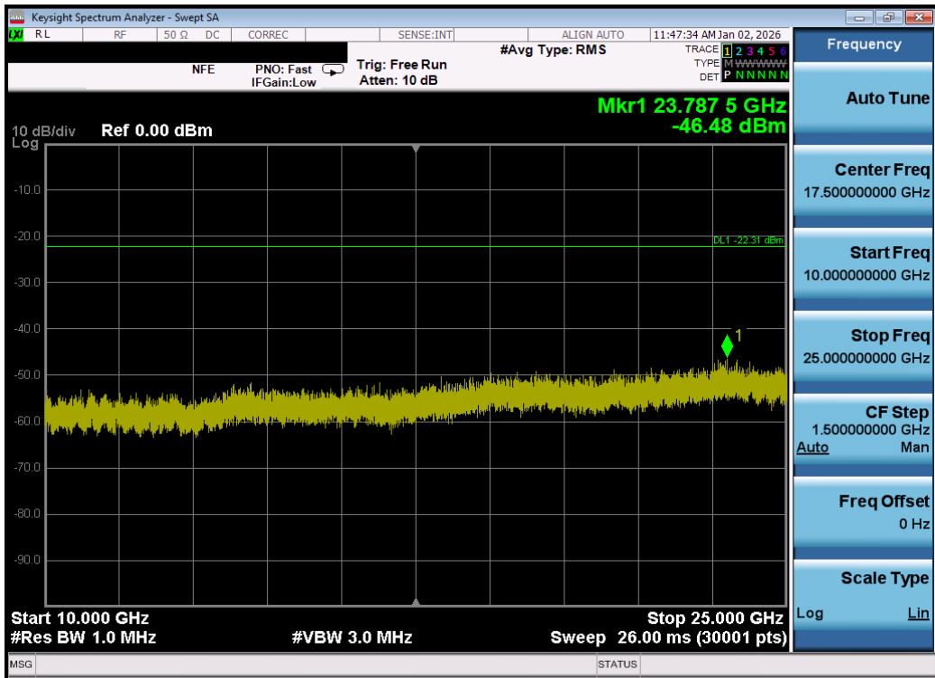
Plot 7-140. Conducted Spurious Plot MIMO ANT2 (802.11be OFDMA – 242 Tones – Ch. 1) – DUAL ANT 2
