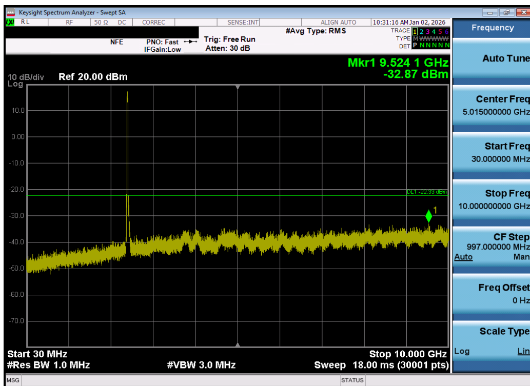
Plot 7-121. Conducted Spurious Plot MIMO ANT1 (802.11be OFDMA – 242 Tones – Ch. 1) – DUAL ANT 1
