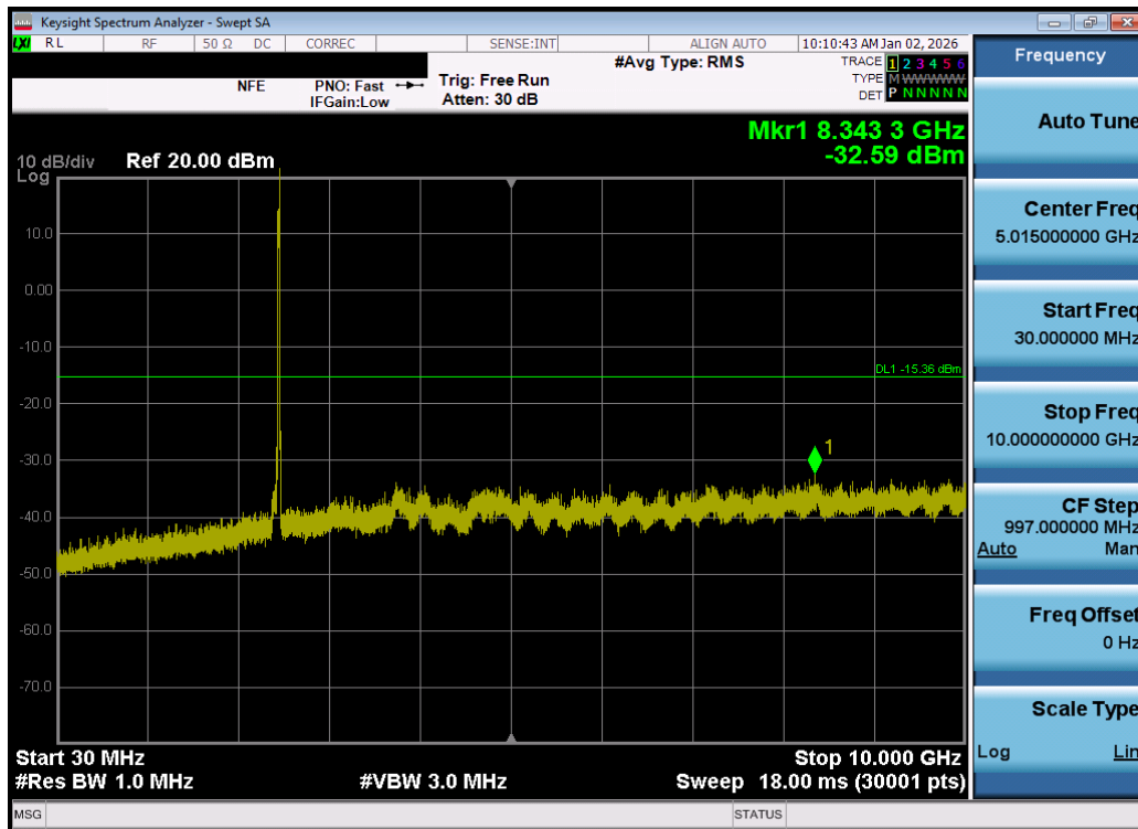
Plot 7-119. Conducted Spurious Plot MIMO ANT1 (802.11be OFDMA – 26 Tones – Ch. 11) – DUAL ANT 1
