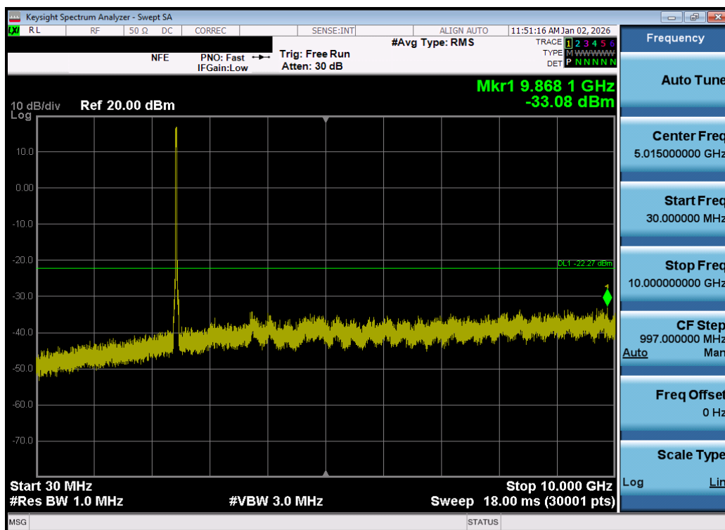
Plot 7-141. Conducted Spurious Plot MIMO ANT2 (802.11be OFDMA – 242 Tones – Ch. 6) – DUAL ANT 2
