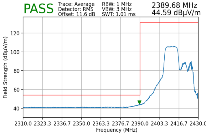
Plot 7-159. Radiated Restricted Lower Band Edge Measurement MIMO (Average – 106 Tones)
