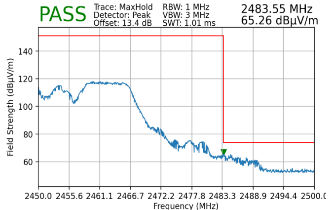
Plot 7-166. Radiated Restricted Upper Band Edge Measurement MIMO (Peak – 106 Tones)
