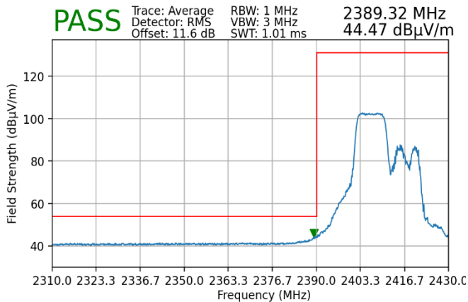
Plot 7-157. Radiated Restricted Lower Band Edge Measurement MIMO (Average – 106 Tones)
