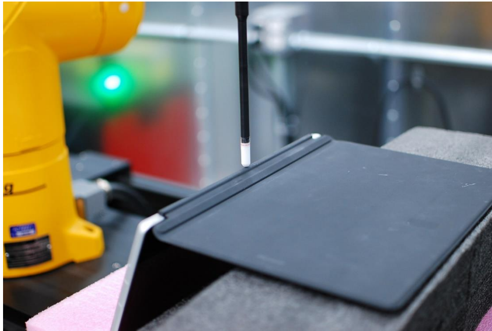
PD Test Setup Photo 34 – Near Field Power Density Laptop Bottom Edge at 2 mm
