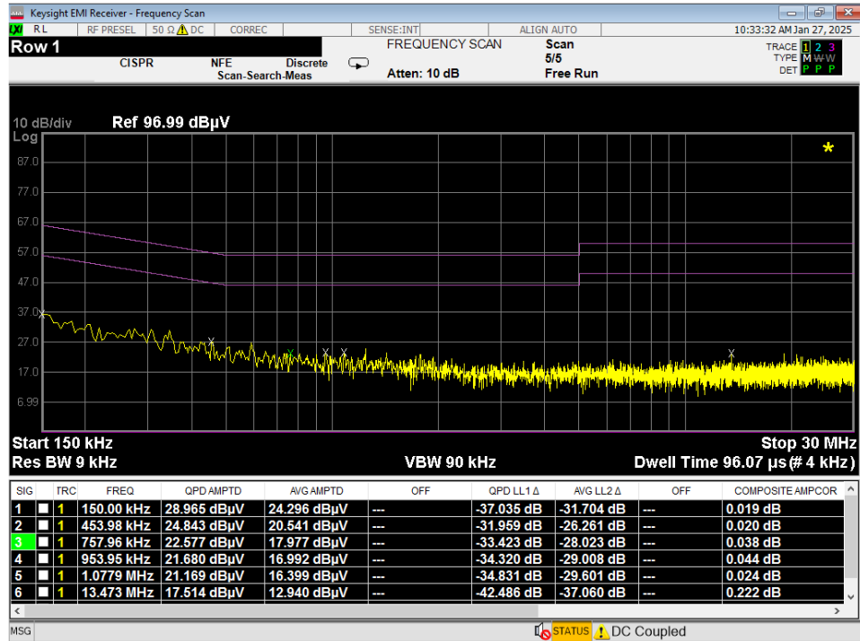
Plot 7-44. Line Conducted Plot with 802.11a UNII Band 2A (L1)
