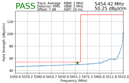
Plot 7-34. Lower Band Edge Plot MIMO (Average – UNII Band 2C)
