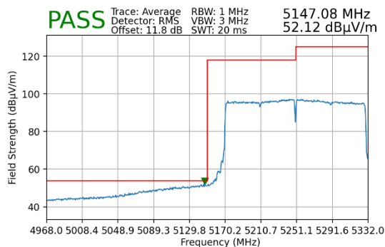
Plot 7-40. Lower Band Edge Plot MIMO (Average – UNII Band 1)
