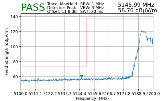
Plot 7-19. Lower Band Edge Plot MIMO (Peak – UNII Band 1)
