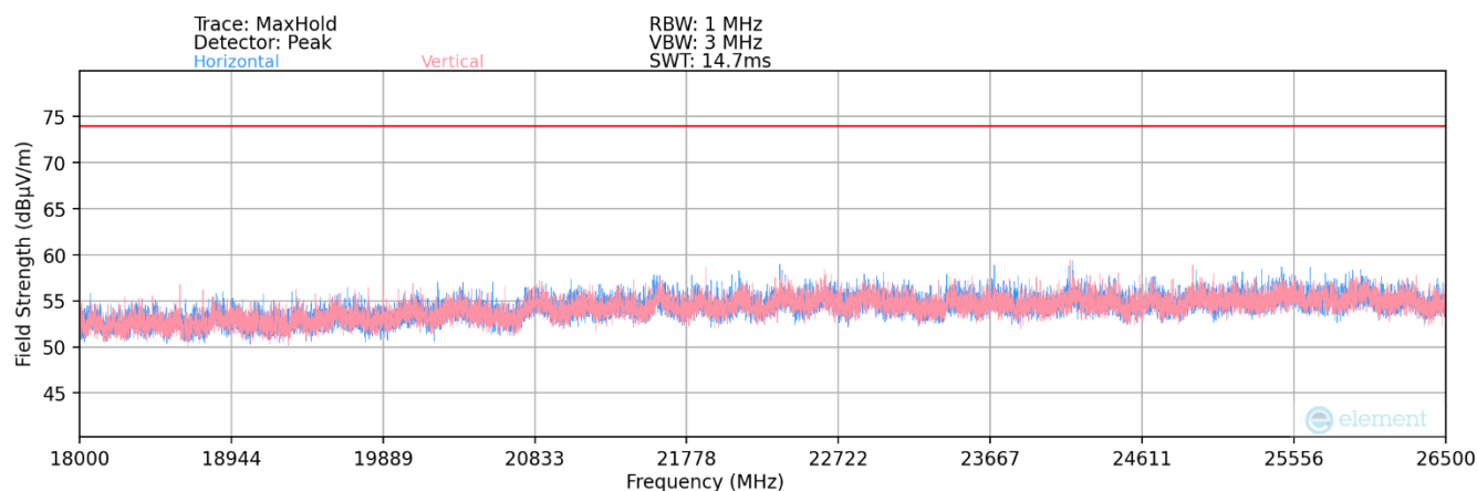
Plot 7-14. Radiated Spurious Plot 18GHz – 26.5GHz MIMO (802.11be 52T – 20MHz)
