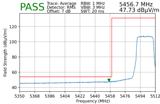
Plot 7-24. Lower Band Edge Plot MIMO (Average – UNII Band 2C)
