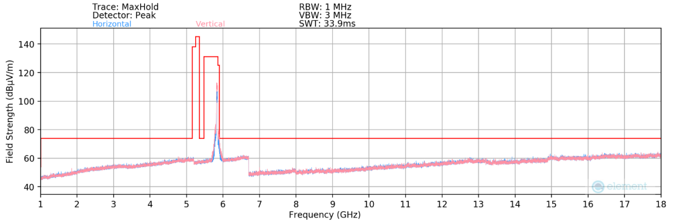
Plot 7-10. Radiated Spurious Plot above 1GHz MIMO (802.11n – UNII Band 4 Ch. 167 – 40MHz)
