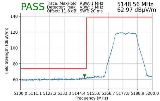
Plot 7-17. Lower Band Edge Plot MIMO (Peak – UNII Band 1)
