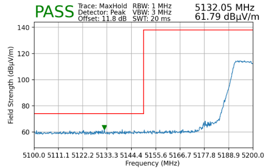
Plot 7-21. Lower Band Edge Plot MIMO (Peak – UNII Band 1)
