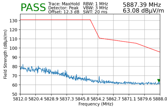
Plot 7-28. Upper Band Edge Plot MIMO (Peak – UNII Band 3)
