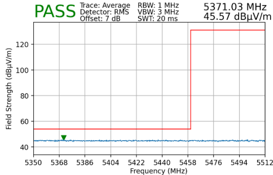
Plot 7-26. Lower Band Edge Plot MIMO (Average – UNII Band 2C)
