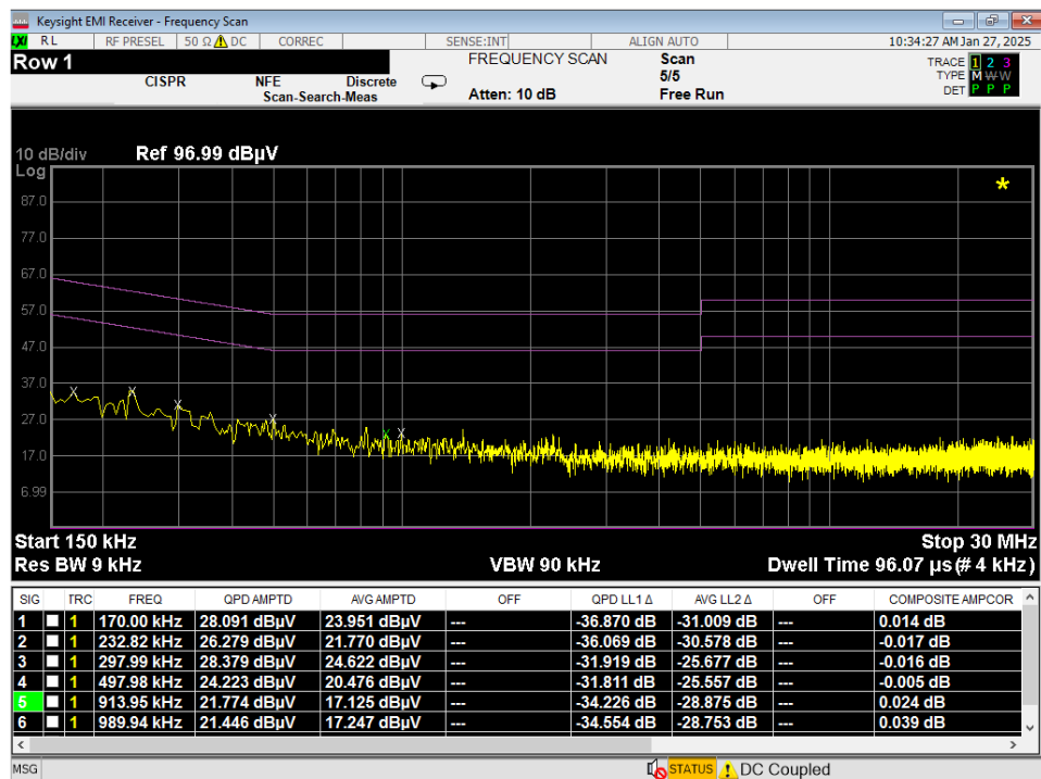
Plot 7-45. Line Conducted Plot with 802.11a UNII Band 2A (N)
