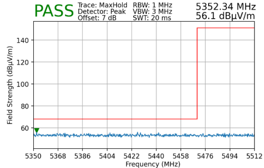
Plot 7-27. Lower Band Edge Plot MIMO (Peak – UNII Band 2C)
