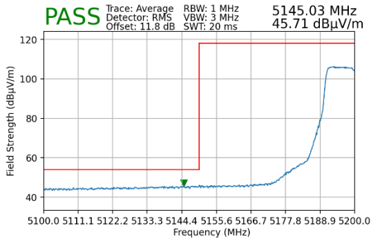
Plot 7-20. Lower Band Edge Plot MIMO (Average – UNII Band 1)
