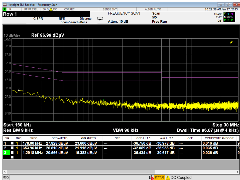
Plot 7-43. Line Conducted Plot with 802.11a UNII Band 1 (N)
