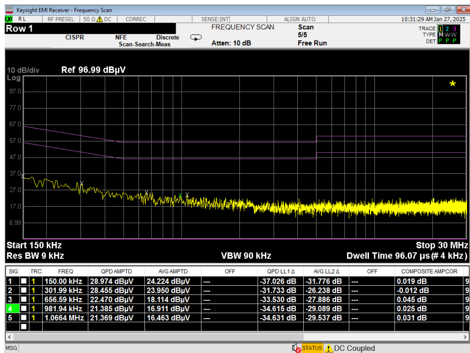
Plot 7-42. Line Conducted Plot with 802.11a UNII Band 1 (L1)
