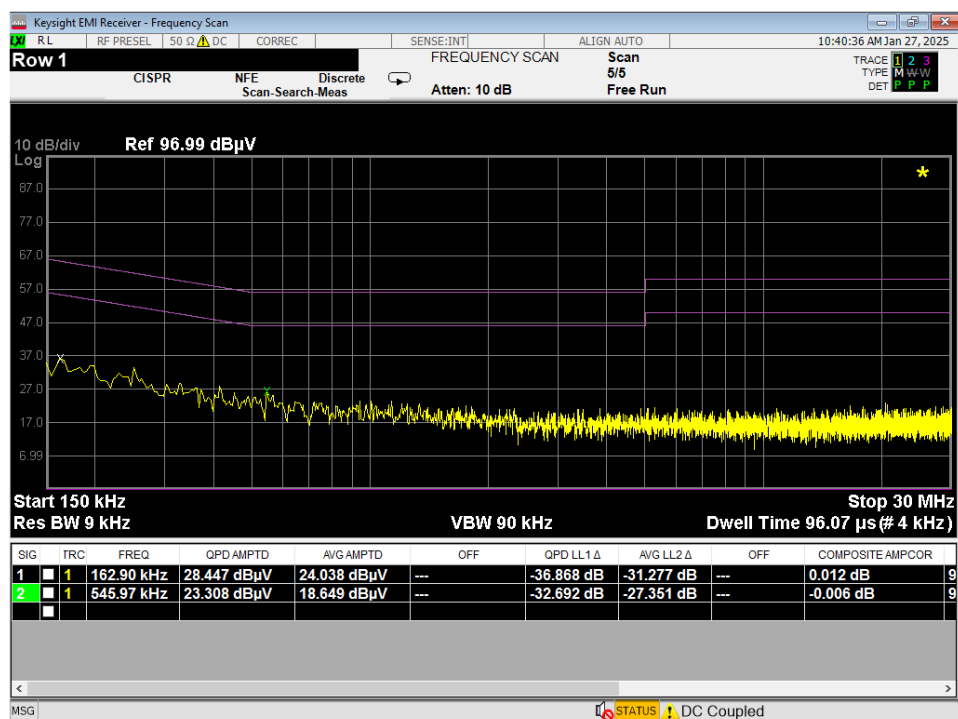
Plot 7-49. Line Conducted Plot with 802.11a UNII Band 3 (N)
