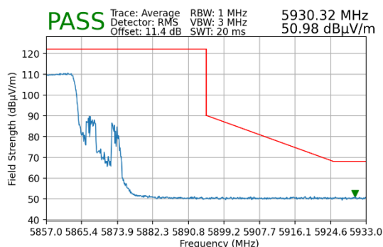
Plot 7-30. Upper Band Edge Plot MIMO (Average – UNII Band 4)
