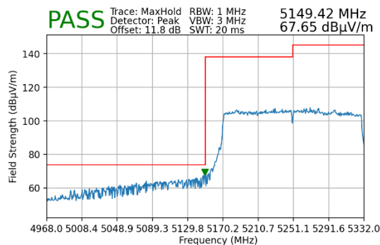
Plot 7-41. Lower Band Edge Plot MIMO (Peak – UNII Band 1)
