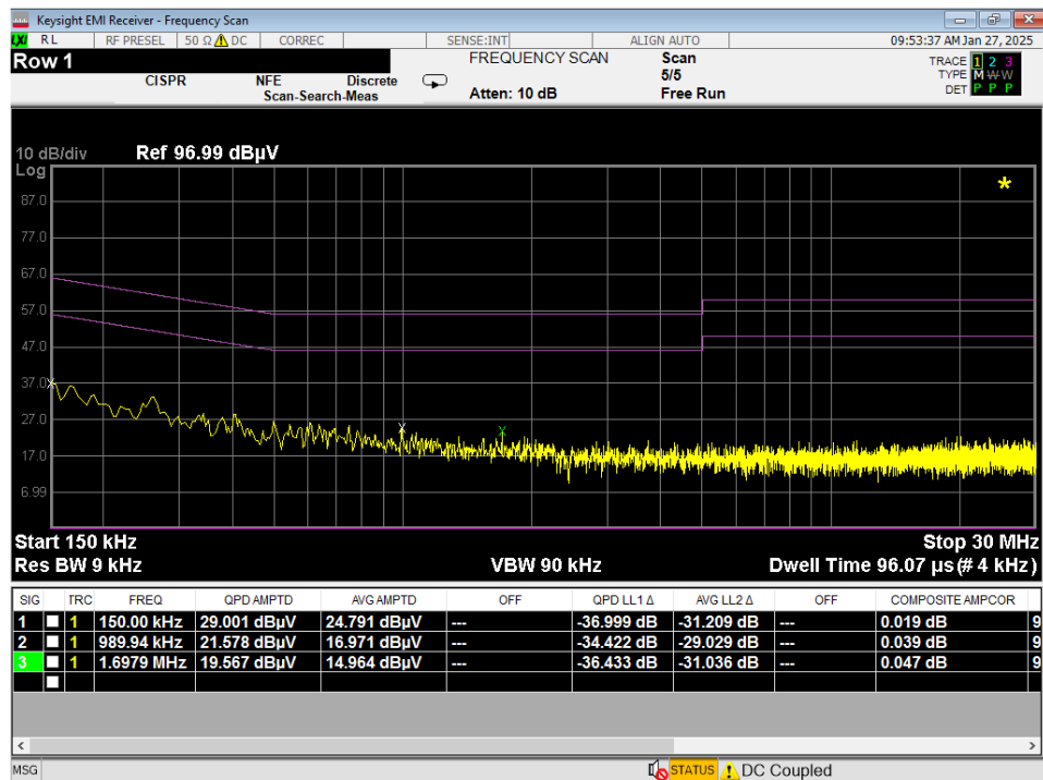
Plot 7-51. Line Conducted Plot with 802.11a UNII Band 4 (N)
