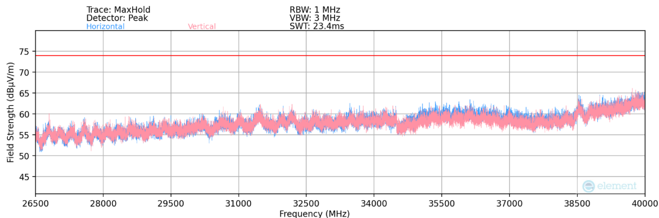
Plot 7-15. Radiated Spurious Plot 26.5GHz – 40GHz MIMO (802.11be 52T – 20MHz)
