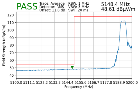
Plot 7-18. Lower Band Edge Plot MIMO (Average – UNII Band 1)
