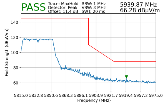
Plot 7-38. Upper Band Edge Plot MIMO (Peak – UNII Band 4)
