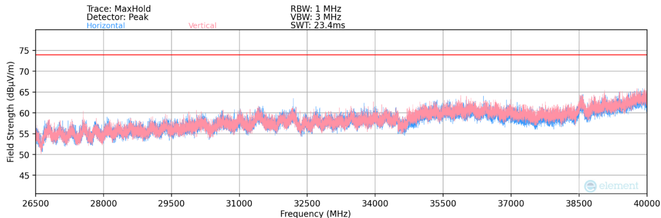
Plot 7-13. Radiated Spurious Plot 26.5GHz – 40GHz MIMO (802.11n – 20MHz)
