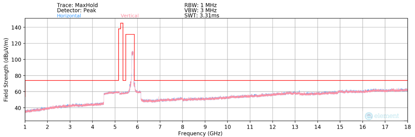
Plot 7-8. Radiated Spurious Plot above 1GHz MIMO (802.11ac – UNII Band 3 Ch. 155 – 80MHz)
