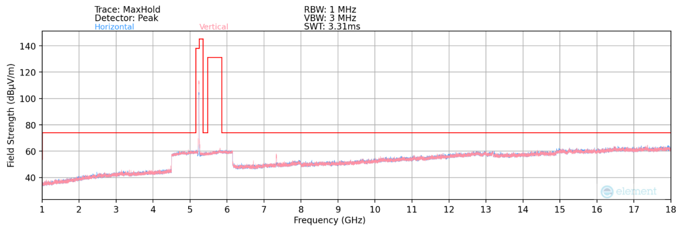
Plot 7-5. Radiated Spurious Plot above 1GHz MIMO (802.11be – UNII Band 2A Ch. 52 – 52T – 20MHz)
