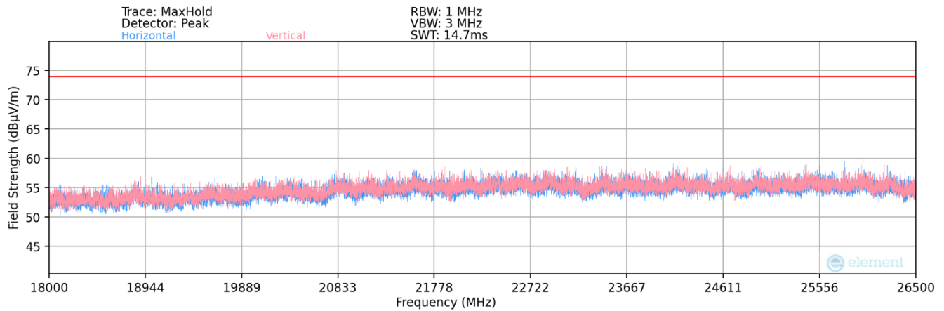
Plot 7-12. Radiated Spurious Plot 18GHz – 26.5GHz MIMO (802.11n – 20MHz)
