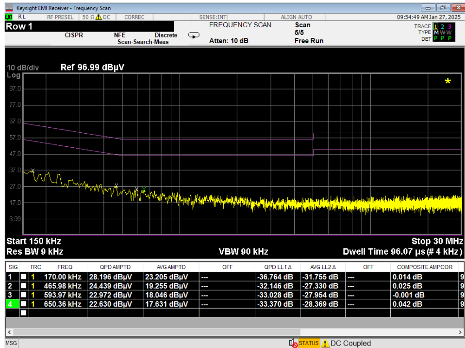
Plot 7-50. Line Conducted Plot with 802.11a UNII Band 4 (L1)
