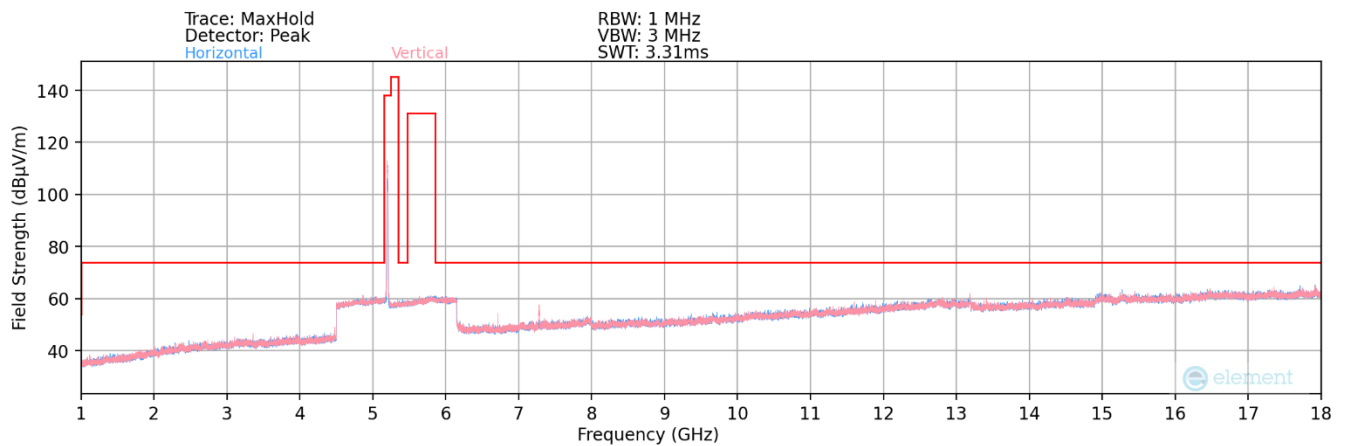
Plot 7-2. Radiated Spurious Plot above 1GHz MIMO (802.11n – UNII Band 1 Ch. 40 – 20MHz)
