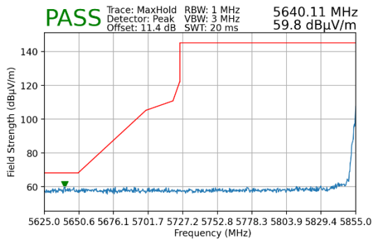
Plot 7-29. Lower Band Edge Plot MIMO (Peak – UNII Band 4)
