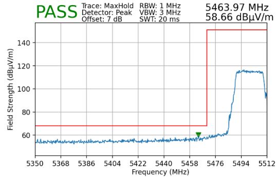
Plot 7-25. Lower Band Edge Plot MIMO (Peak – UNII Band 2C)
