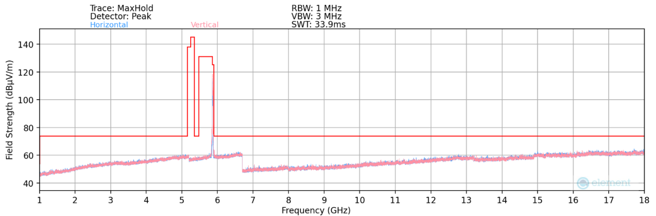
Plot 7-11. Radiated Spurious Plot above 1GHz MIMO (802.11be – UNII Band 4 Ch. 173 – 106T – 20MHz)
