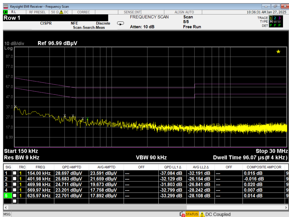
Plot 7-47. Line Conducted Plot with 802.11a UNII Band 2C (N)
