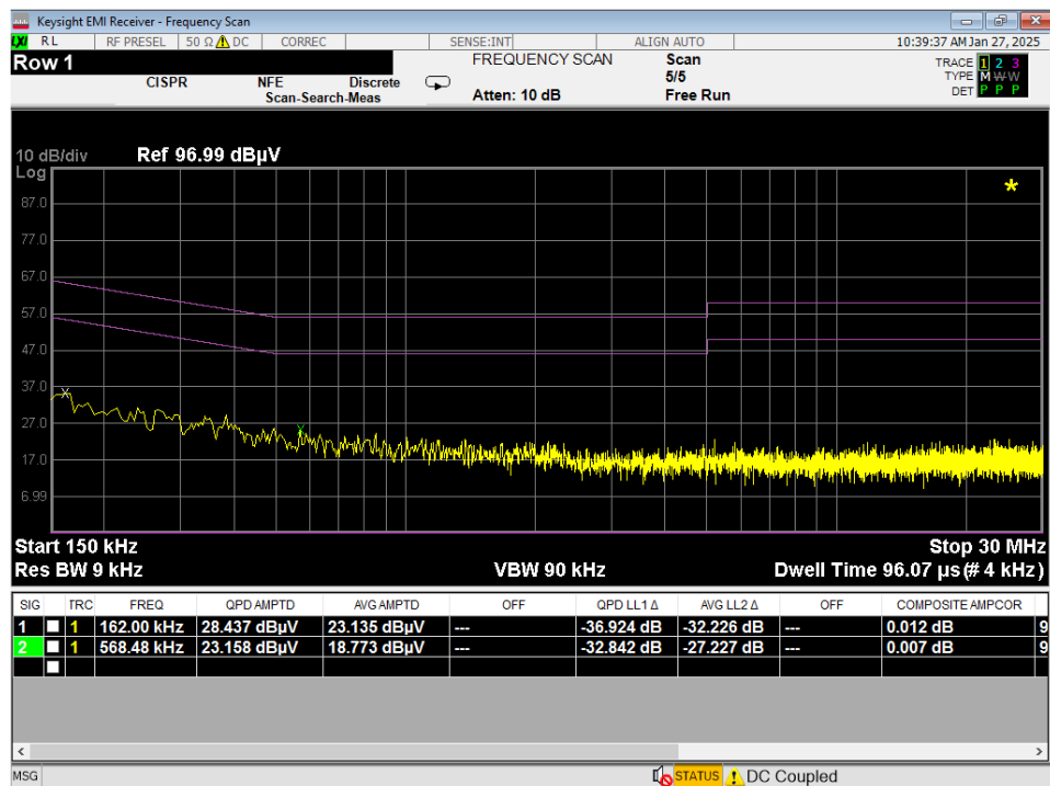
Plot 7-48. Line Conducted Plot with 802.11a UNII Band 3 (L1)
