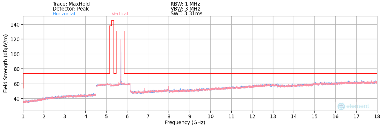
Plot 7-7. Radiated Spurious Plot above 1GHz MIMO (802.11be – UNII Band 2C Ch. 140 – 40MHz)
