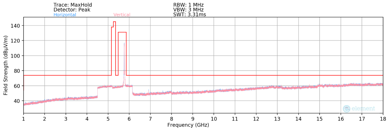
Plot 7-9. Radiated Spurious Plot above 1GHz MIMO (802.11n – UNII Band 3 Ch. 153 – 20MHz)
