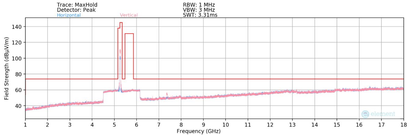
Plot 7-4. Radiated Spurious Plot above 1GHz MIMO (802.11n – UNII Band 2A Ch. 54 – 40MHz)
