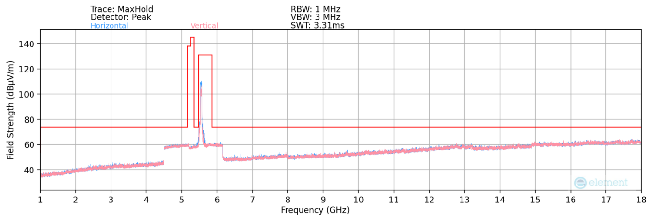
Plot 7-6. Radiated Spurious Plot above 1GHz MIMO (802.11n – UNII Band 2C Ch. 110 – 40MHz)
