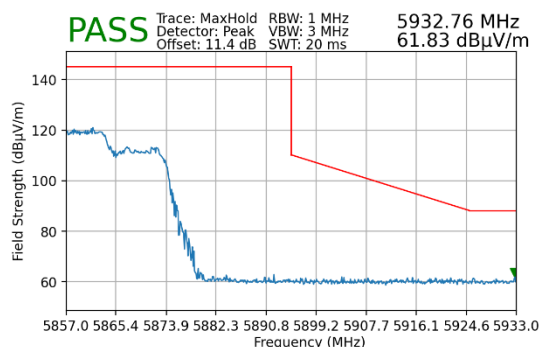
Plot 7-31. Upper Band Edge Plot MIMO (Peak – UNII Band 4)
