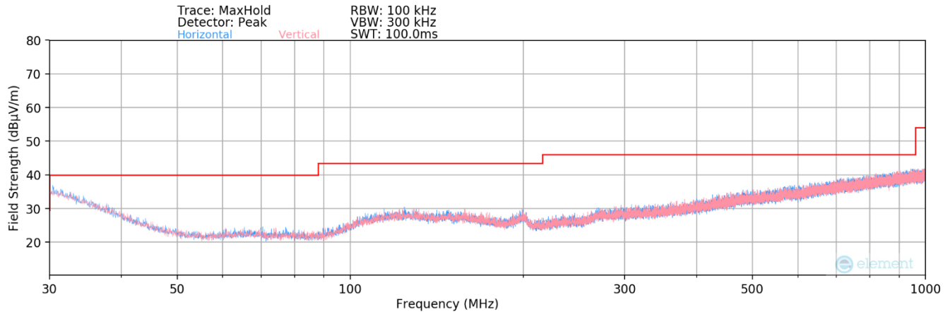
Plot 7-1. Radiated Spurious Plot below 1GHz MIMO (20MHz – 802.11n)
