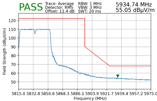
Plot 7-37. Upper Band Edge Plot MIMO (Average – UNII Band 4)
