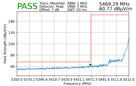
Plot 7-35. Lower Band Edge Plot MIMO (Peak – UNII Band 2C)
