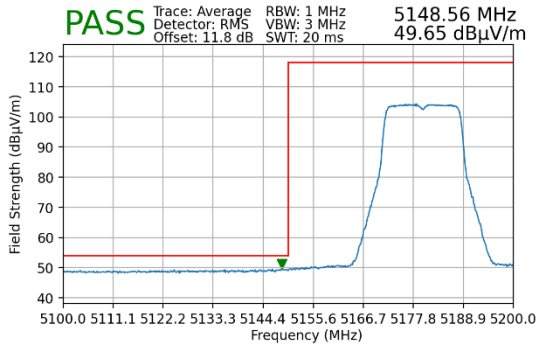
Plot 7-16. Lower Band Edge Plot MIMO (Average – UNII Band 1)
