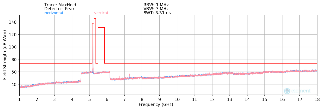
Plot 7-3. Radiated Spurious Plot above 1GHz MIMO (802.11be – UNII Band 1 Ch. 40 – 52T – 20MHz)
