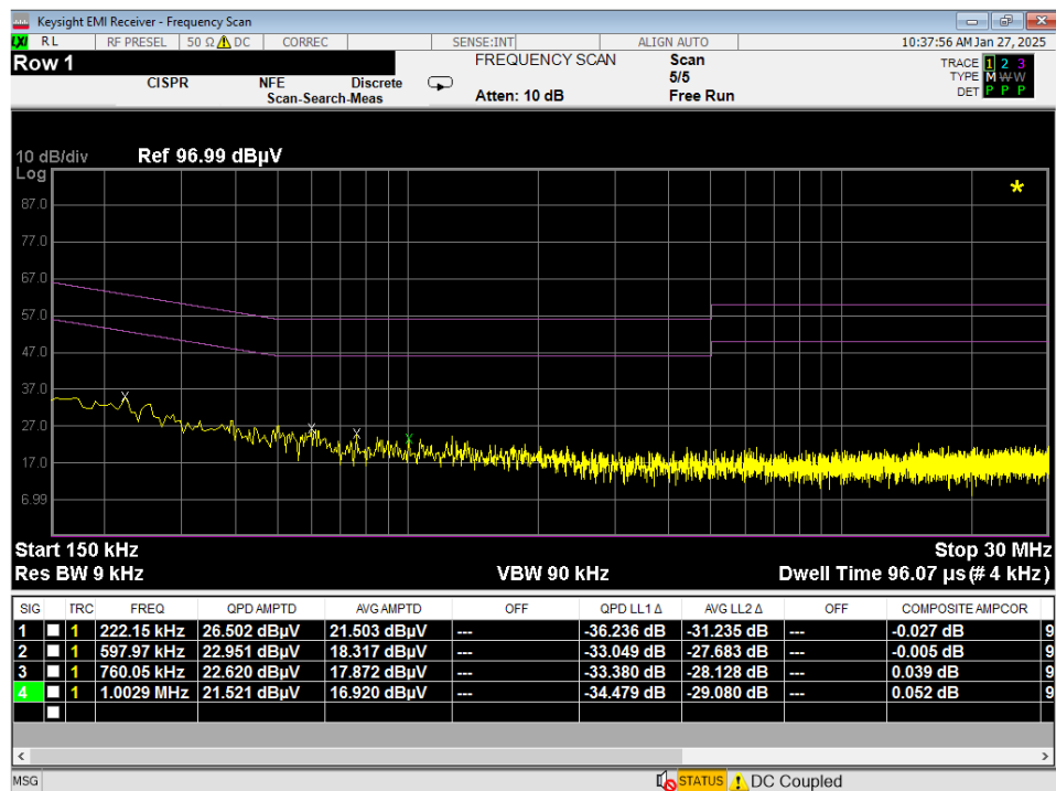
Plot 7-46. Line Conducted Plot with 802.11a UNII Band 2C (L1)
