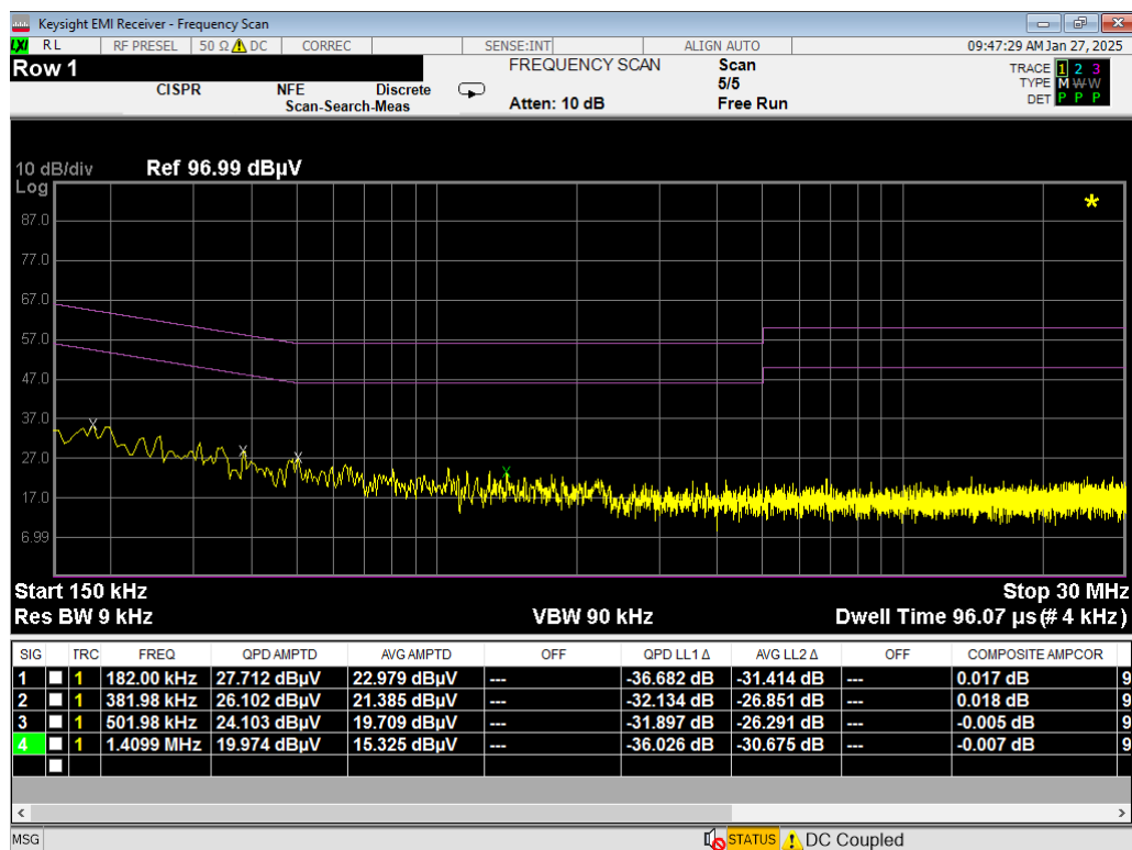
Plot 7-21. Line Conducted Plot with 802.11b (L1)
