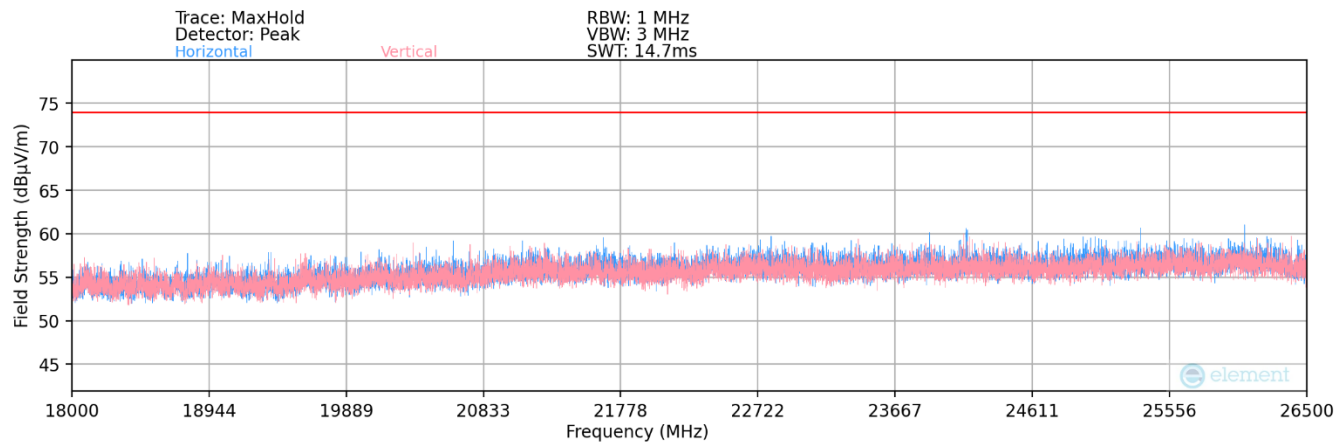
Plot 7-4. Radiated Spurious Plot above 18GHz MIMO
