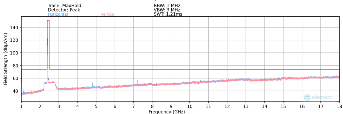
Plot 7-2. Radiated Spurious Plot above 1GHz MIMO (802.11be 26T – Ch. 1)
