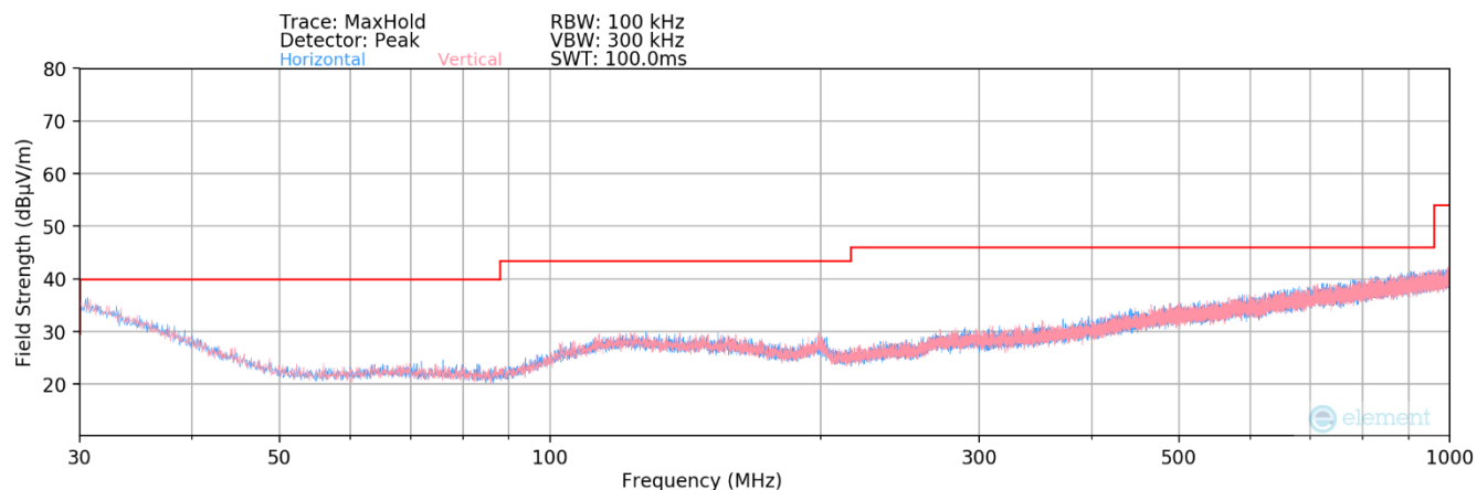
Plot 7-1. Radiated Spurious Plot below 1GHz MIMO
