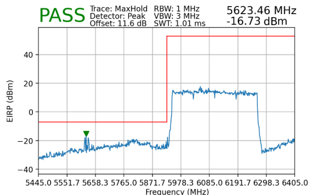
Plot 7-13. Lower Band Edge Plot MIMO (Peak – UNII Band 5)
