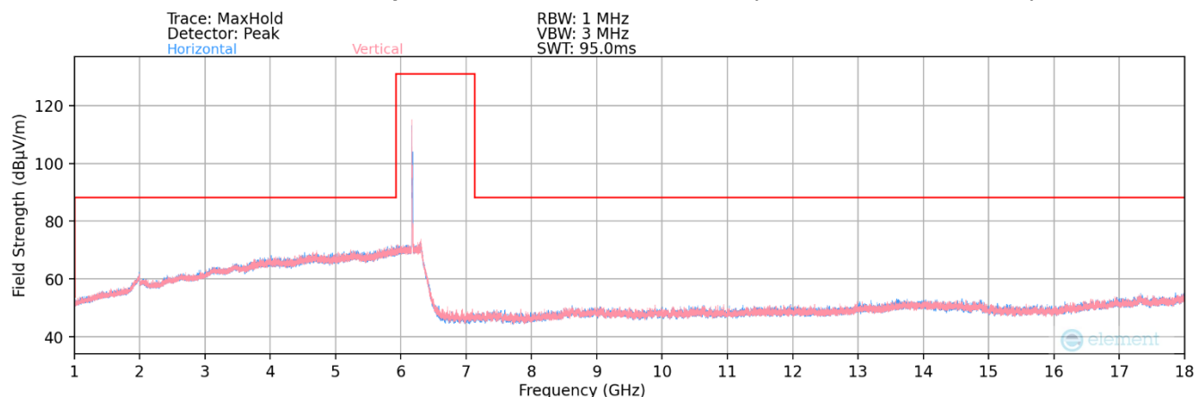
Plot 7-2. Radiated Spurious Plot 1GHz – 18GHz MIMO (802.11be – UNII Band 5 Ch. 49 52T – 20MHz)
