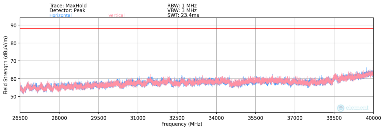
Plot 7-5. Radiated Spurious Plot 26.5GHz - 40GHz (802.11be(20MHz 52T))
