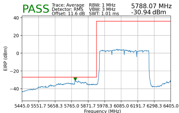
Plot 7-12. Lower Band Edge Plot MIMO (Average – UNII Band 5)
