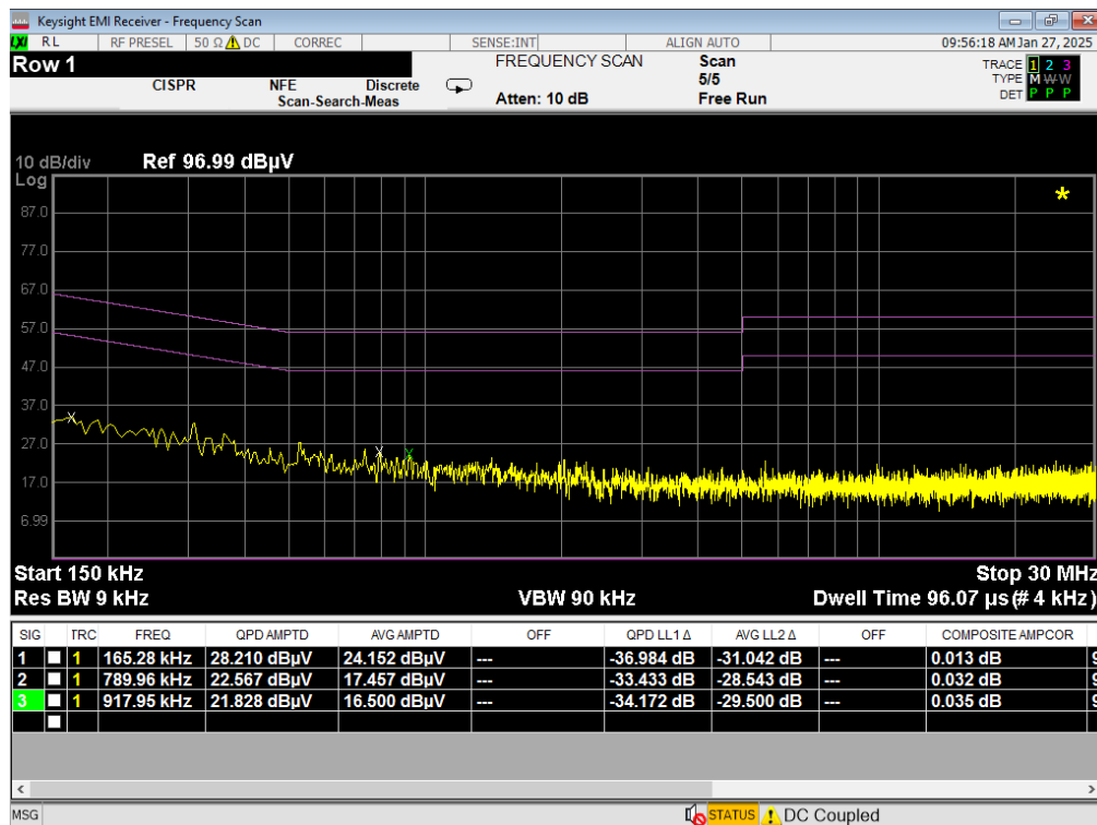
Plot 7-15. Line Conducted Plot with 802.11a UNII Band 5 (N)
