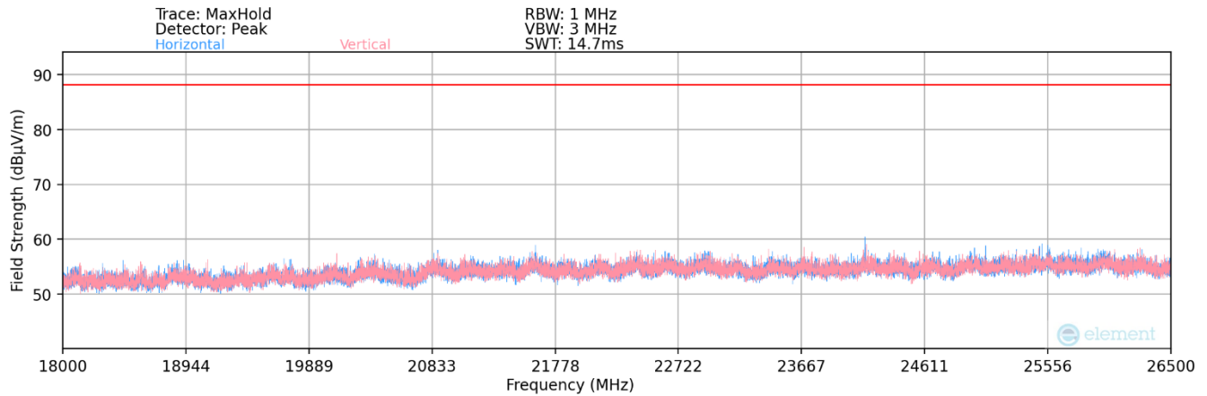
Plot 7-4. Radiated Spurious Plot 18GHz - 26.5GHz (802.11be (20MHz 52T))
