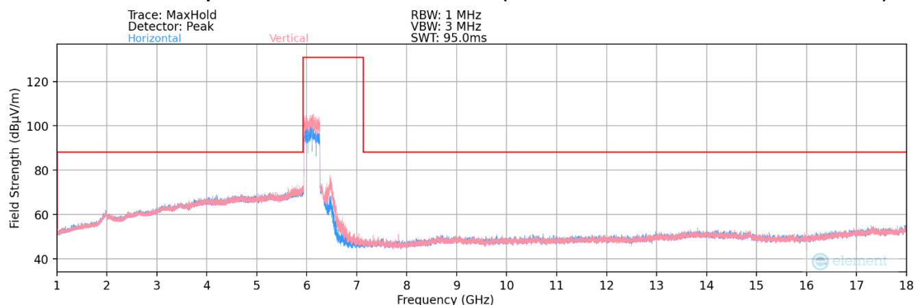
Plot 7-3. Radiated Spurious Plot 1GHz – 18GHz MIMO (802.11be – UNII Band 5 Ch. 31 – 320MHz)
