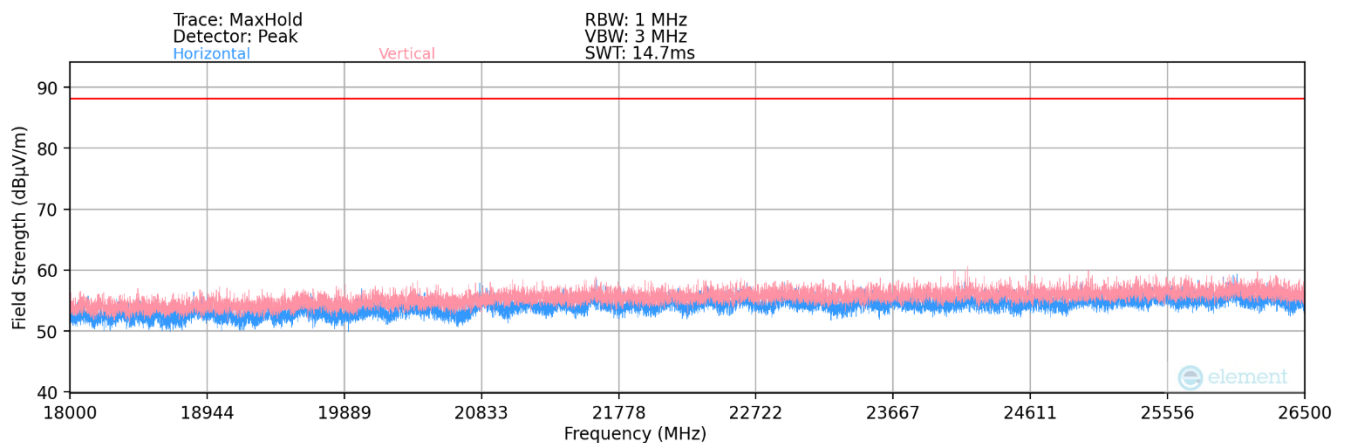
Plot 7-6. Radiated Spurious Plot 18GHz - 26.5GHz (802.11be (320MHz))
