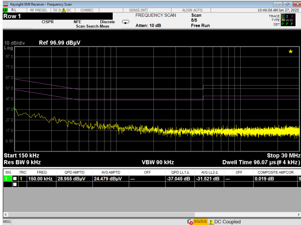
Plot 7-16. Line Conducted Plot with 802.11a UNII Band 6 (L1)
