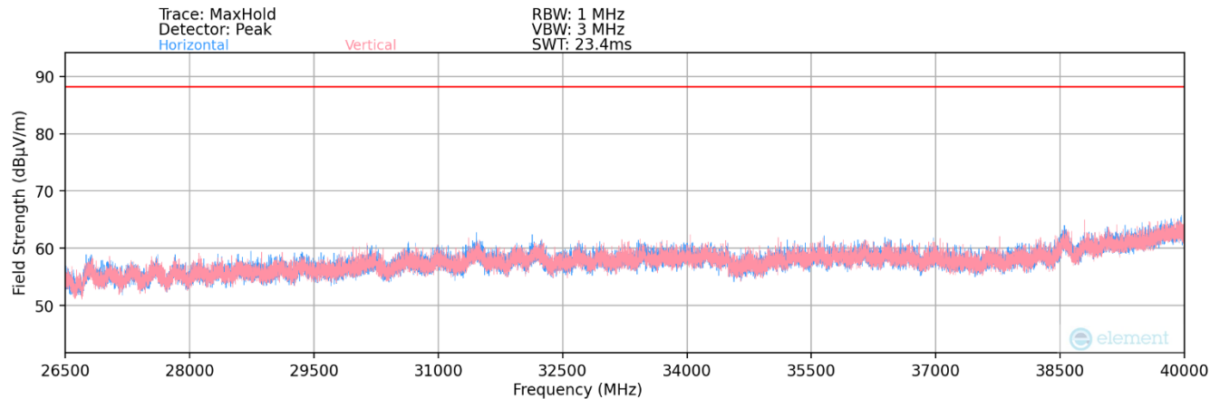
Plot 7-7. Radiated Spurious Plot 26.5GHz - 40GHz (802.11be(320MHz))
