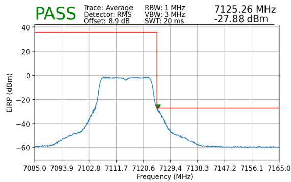
Plot 7-10. Upper Band Edge Plot MIMO (Average – UNII Band 8)
