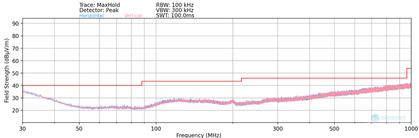
Plot 7-1. Radiated Spurious Plot below 1GHz MIMO (802.11be – 52T – 20MHz)
