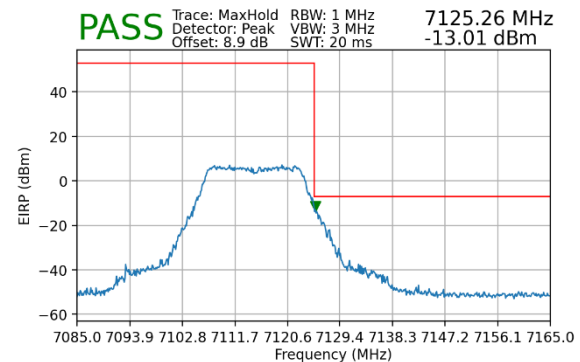
Plot 7-11. Upper Band Edge Plot MIMO (Peak – UNII Band 8)
