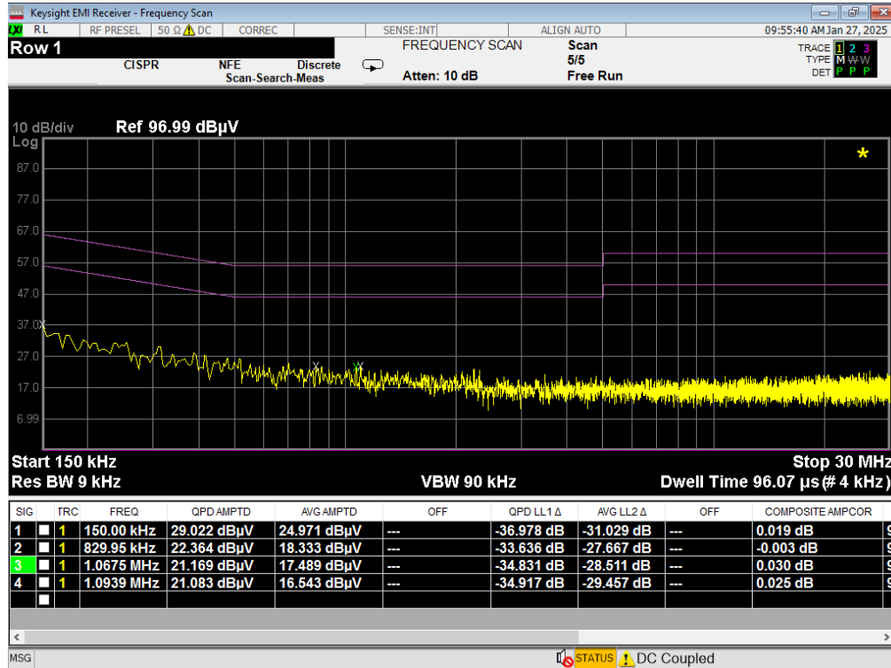
Plot 7-14. Line Conducted Plot with 802.11a UNII Band 5 (L1)
