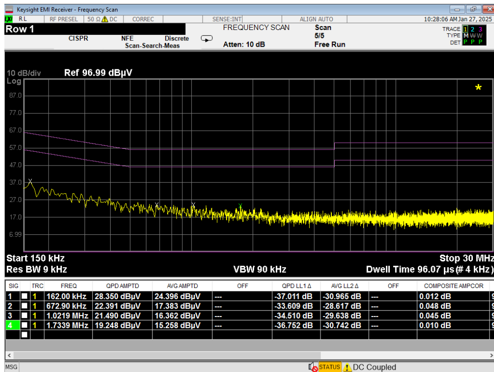
Plot 7-21. Line Conducted Plot with 802.11a UNII Band 8 (N)
