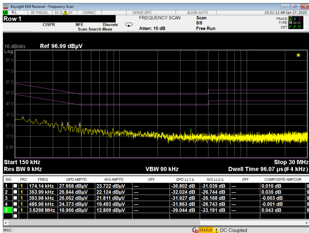
Plot 7-17. Line Conducted Plot with 802.11a UNII Band 6 (N)
