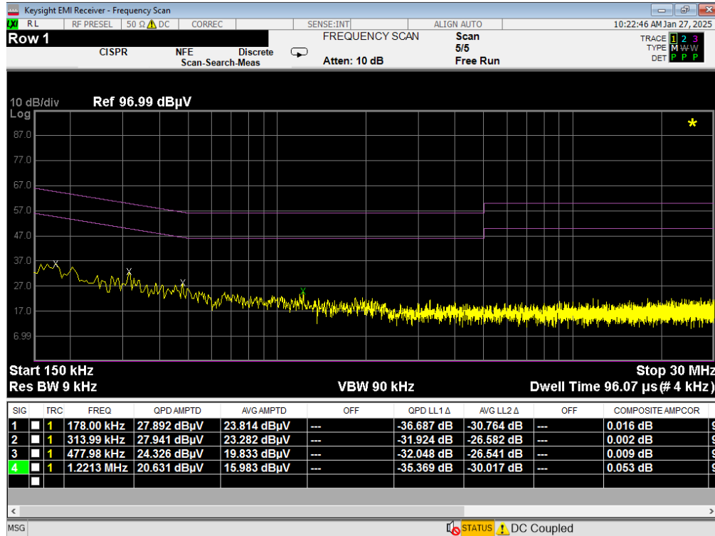
Plot 7-18. Line Conducted Plot with 802.11a UNII Band 7 (L1)
