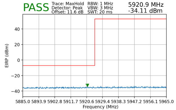
Plot 7-9. Lower Band Edge Plot MIMO (Peak – UNII Band 5)
