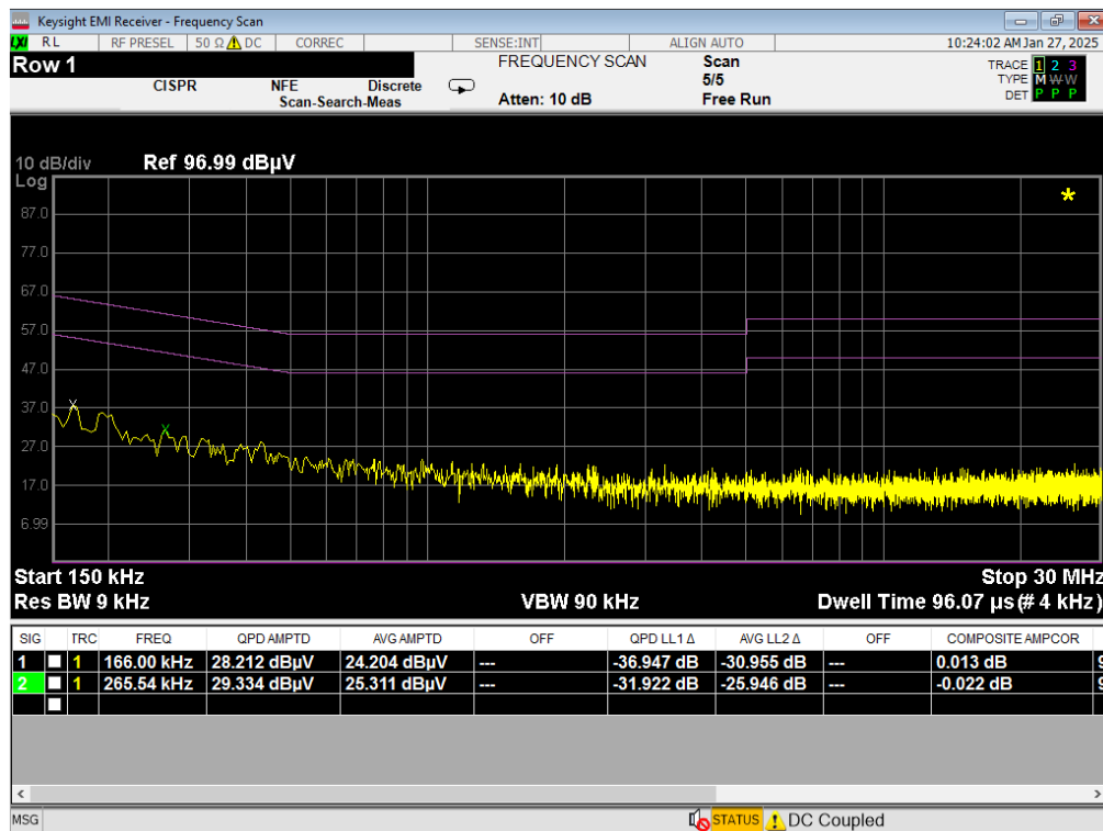
Plot 7-19. Line Conducted Plot with 802.11a UNII Band 7 (N)
