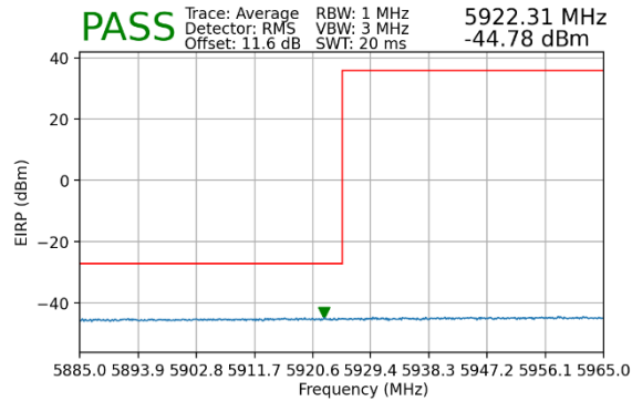
Plot 7-8. Lower Band Edge Plot MIMO (Average – UNII Band 5)
