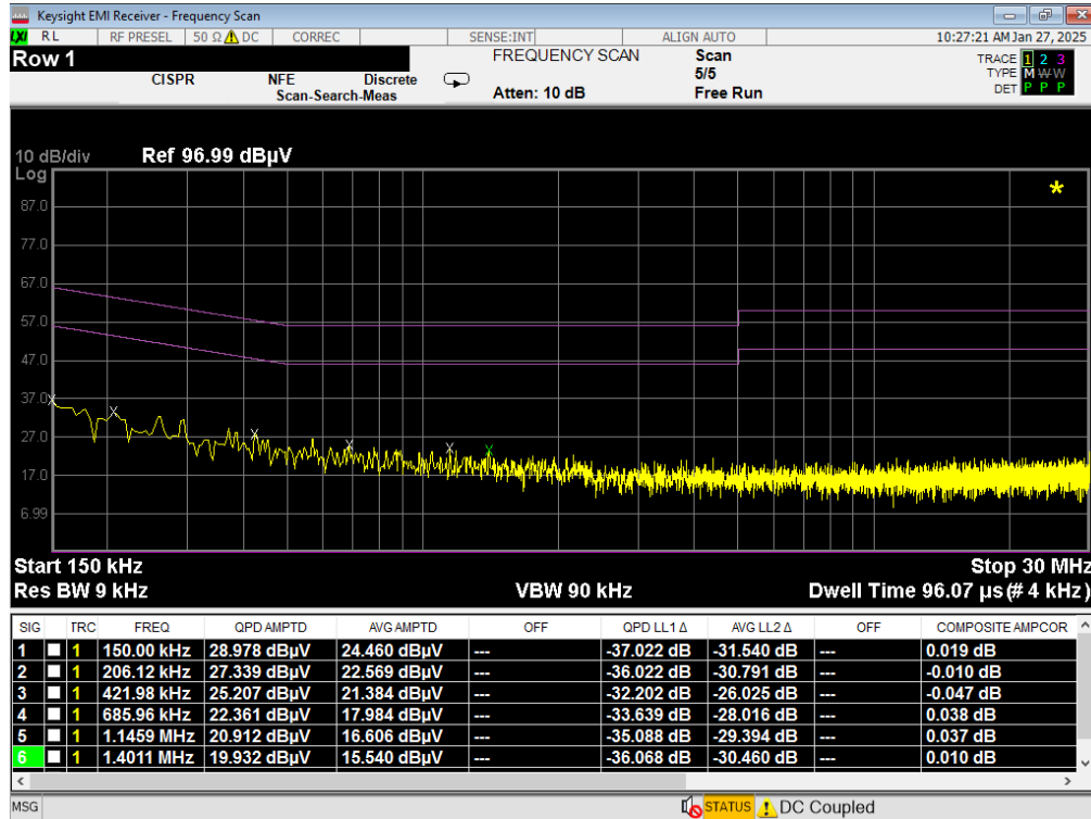
Plot 7-20. Line Conducted Plot with 802.11a UNII Band 8 (L1)
