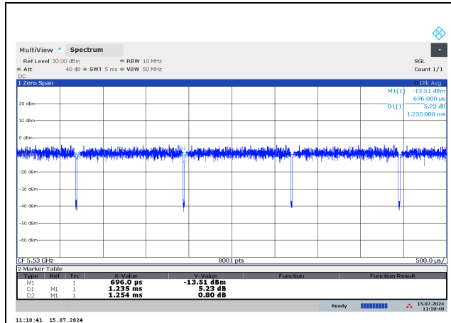
802.11be EHT80 484T+242T (N) MODE
