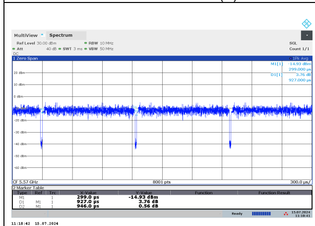
802.11be EHT160 996T+484T (C) MODE
