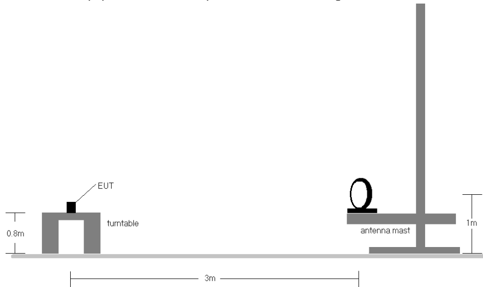
Figure 7-8. Radiated Test Setup
