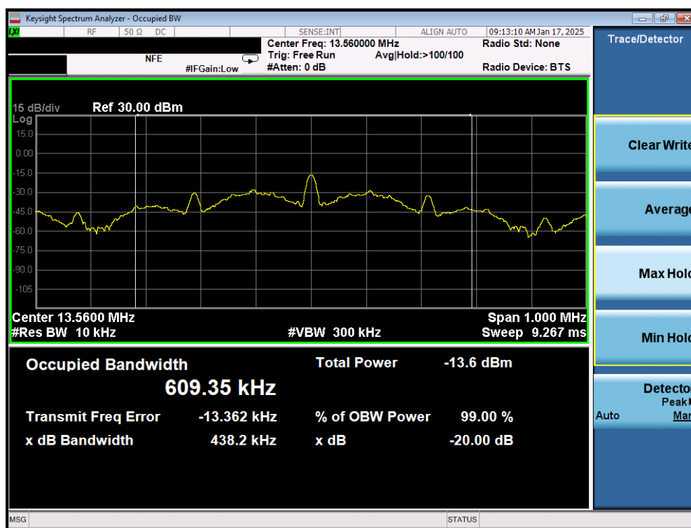
Figure 7-2. Occupied Bandwidth Plot – NFC A
