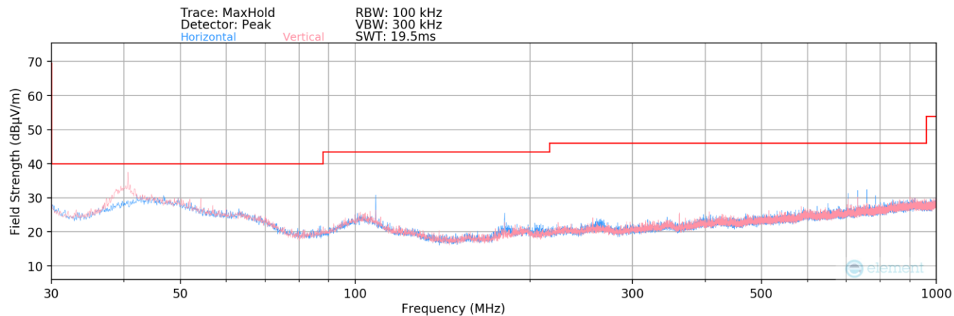
Plot 7-8. Radiated Spurious Plot 30MHz – 1GHz
