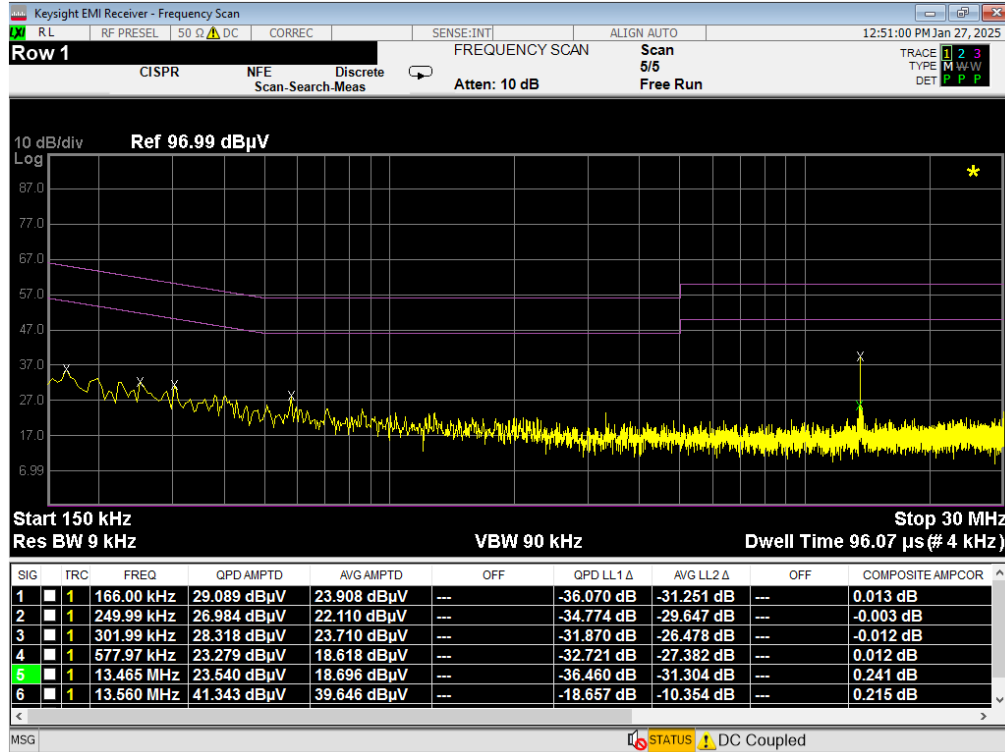
Plot 7-9. Line-Conducted Test Plot (L1) – NFC – A
