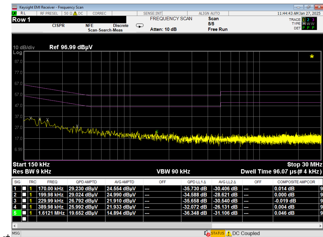
Plot 7-12. Line-Conducted Test Plot (N) – Pen Charging
