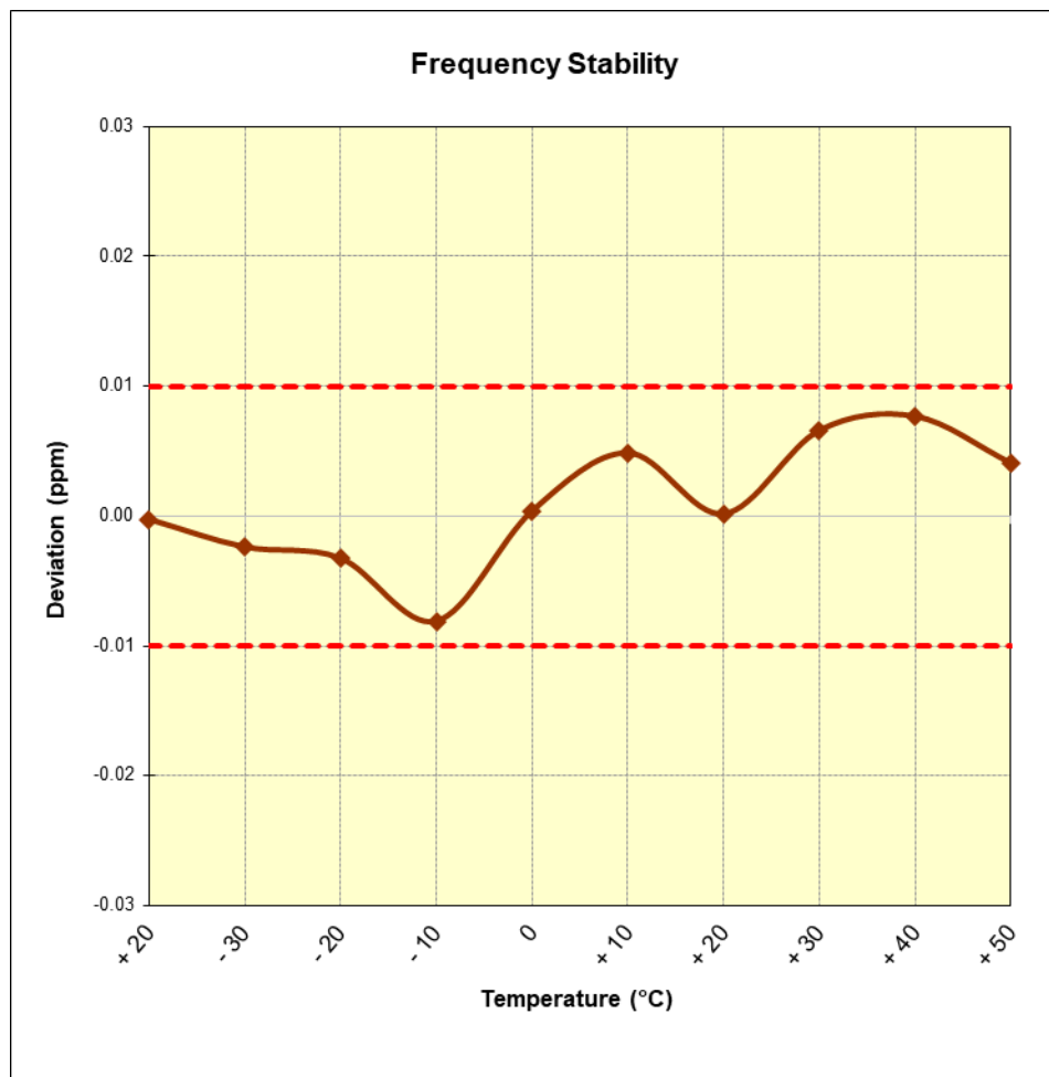
Figure 7-7. Frequency Stability Plot
