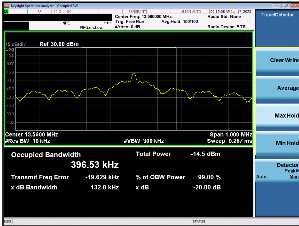
Figure 7-5. Occupied Bandwidth Plot – NFC V
