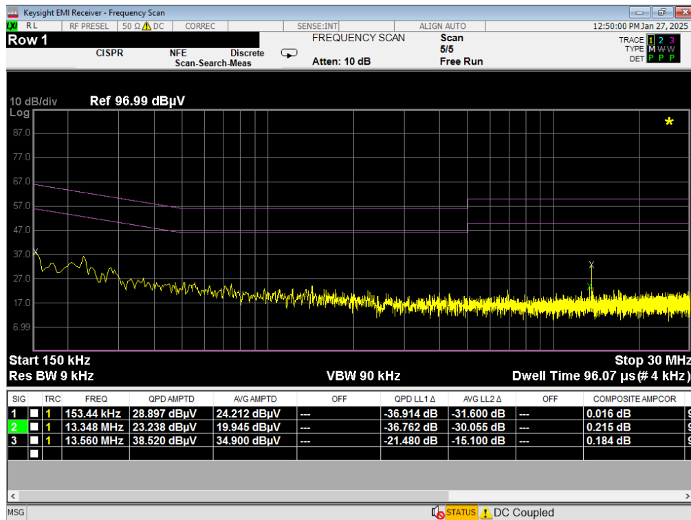
Plot 7-10. Line-Conducted Test Plot (N) – NFC – A
