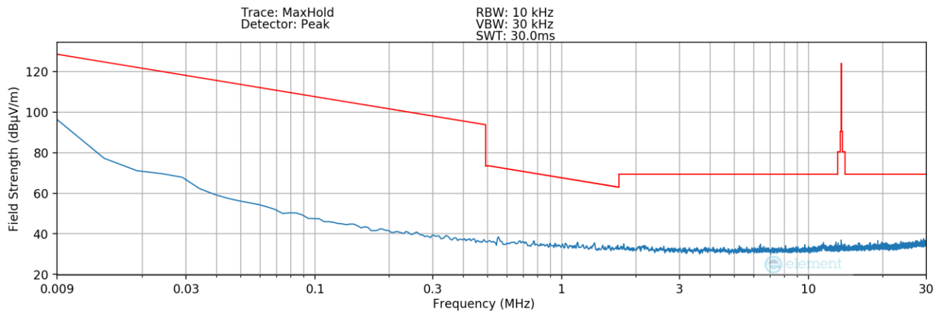
Plot 7-6. Radiated Spurious Plot 9kHz – 30MHz (Pol. Y)
