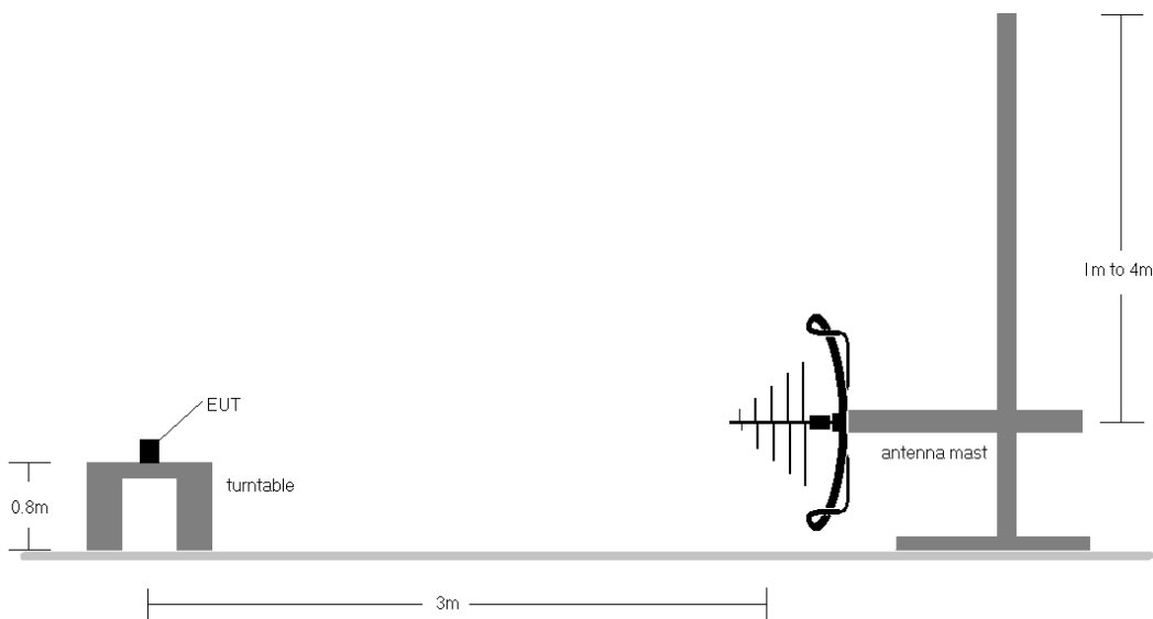
Figure 7-10. Radiated Test Setup > 30MHz
