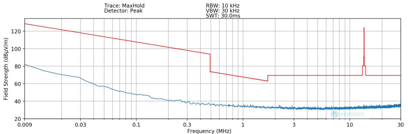
Plot 7-7. Radiated Spurious Plot 9kHz – 30MHz (Pol. Z)
