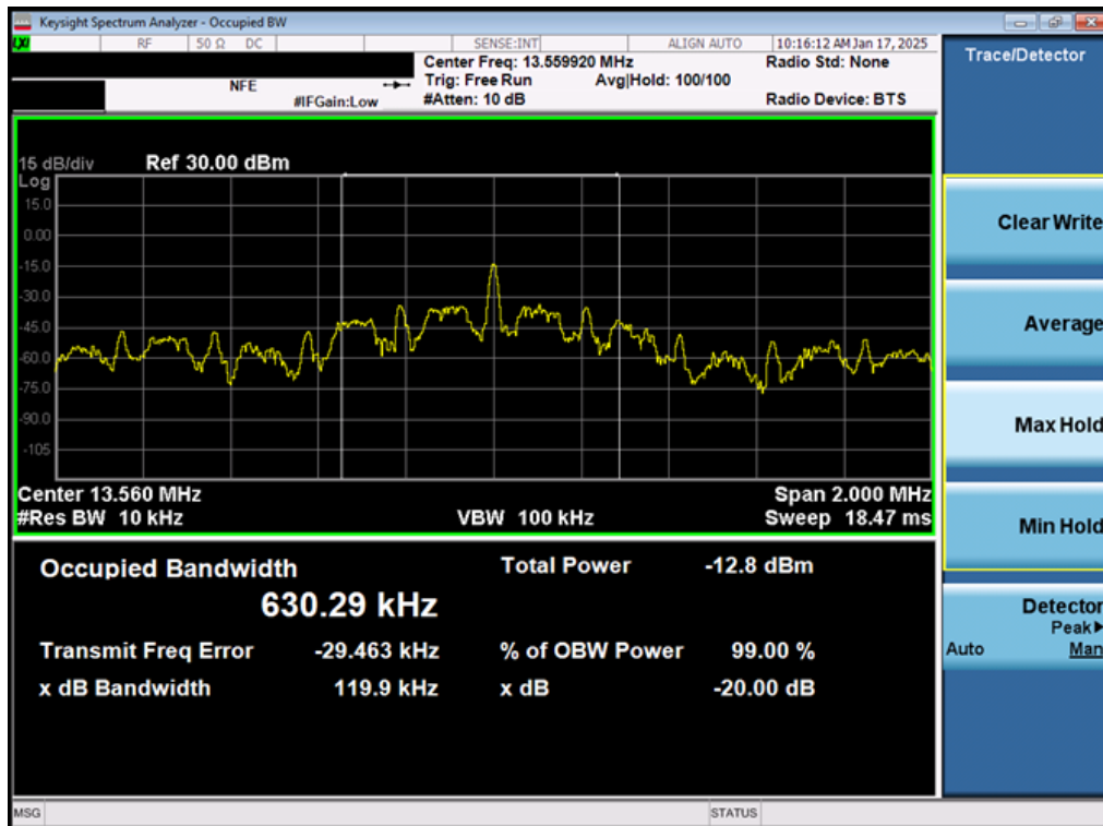
Figure 7-6. Occupied Bandwidth Plot – Pen Wireless Charging
