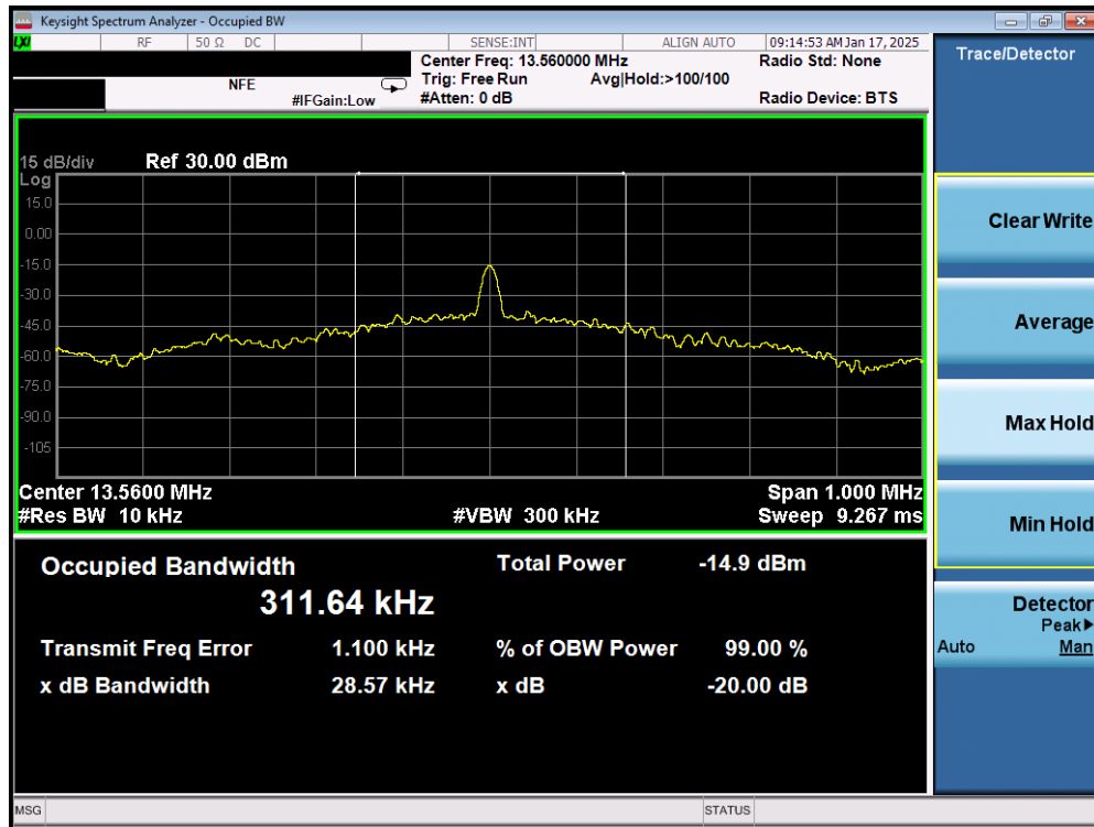
Figure 7-3. Occupied Bandwidth Plot – NFC B
