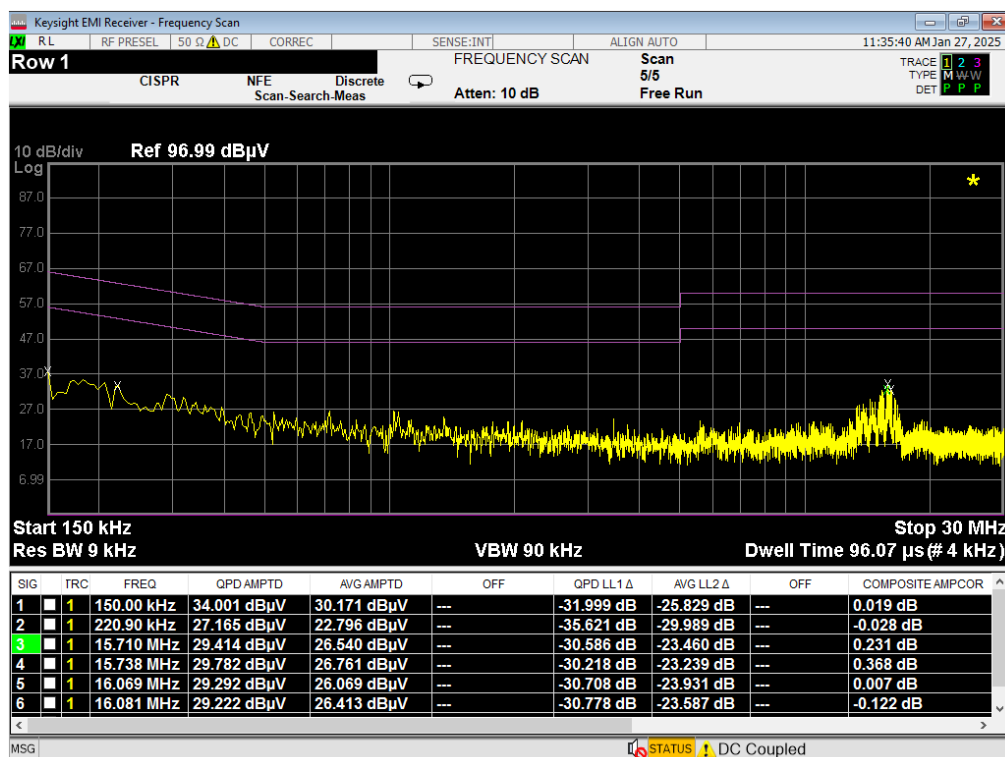
Plot 7-11. Line-Conducted Test Plot (L1) – Pen Charging
