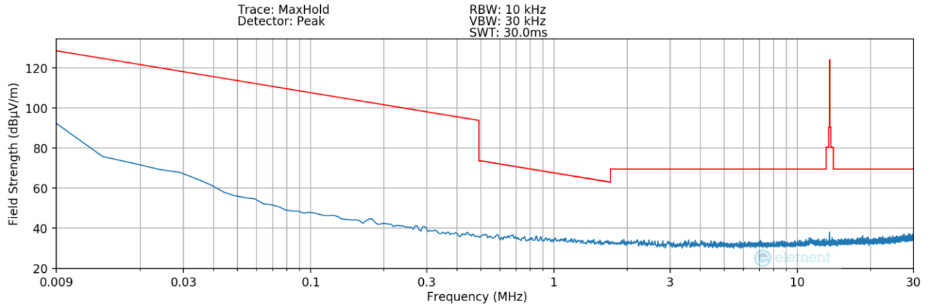
Plot 7-5. Radiated Spurious Plot 9kHz – 30MHz (Pol. X)
