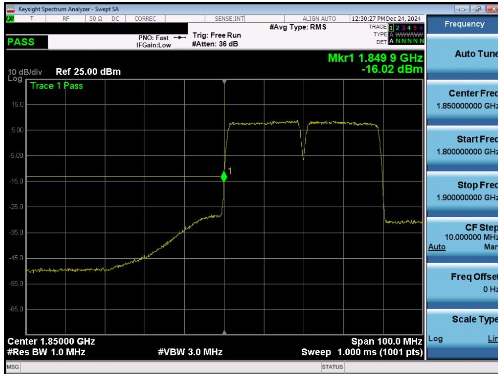
Plot 7-60. Lower Band Edge Plot (ULCA LTE Band 2 – 20+20MHz QPSK – Full RB - Ant 1)
