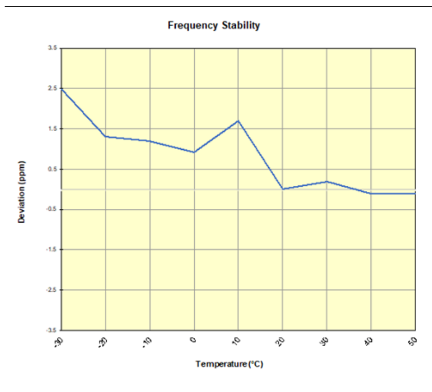
Plot 7-87. NR Band n25/2 Frequency Stability Chart
