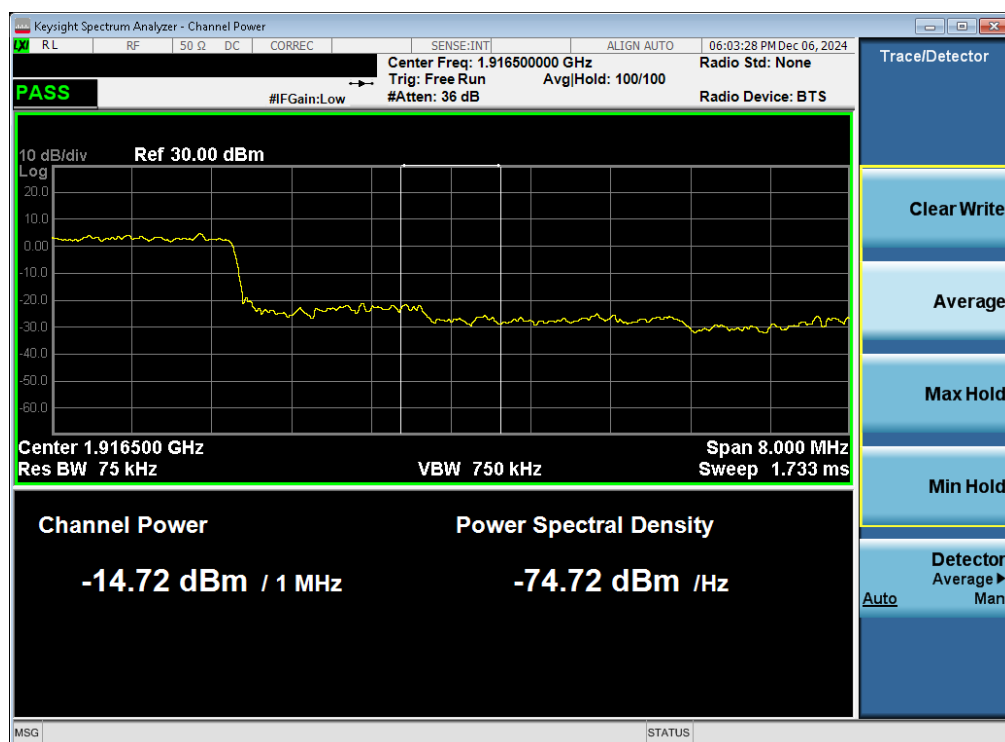
Plot 7-69. Extended Upper Band Edge Plot (NR Band n25 - 10MHz QPSK – Full RB - Ant 1)
