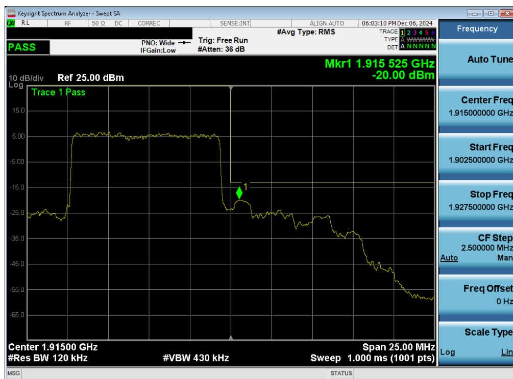
Plot 7-68. Upper Band Edge Plot (NR Band n25 - 10MHz QPSK – Full RB - Ant 1)
