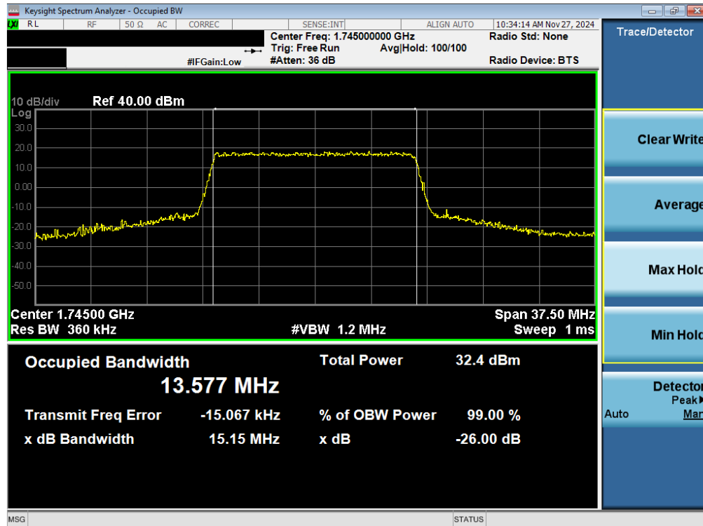
Plot 7-86. Occupied Bandwidth Plot (LTE Band 66/4 - 15MHz QPSK - Full RB - Ant 1)
