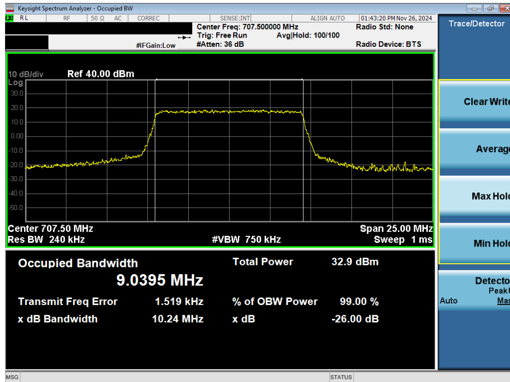
Plot 7-50. Occupied Bandwidth Plot (LTE Band 12 - 10MHz QPSK - Full RB – Ant 2)
