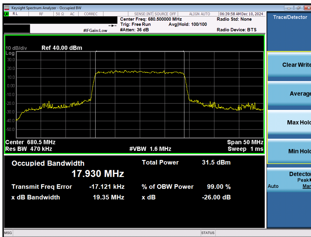
Plot 7-30. Occupied Bandwidth Plot (NR Band n71 - 20MHz DFT-s-OFDM BPSK - Full RB – Ant 5)
