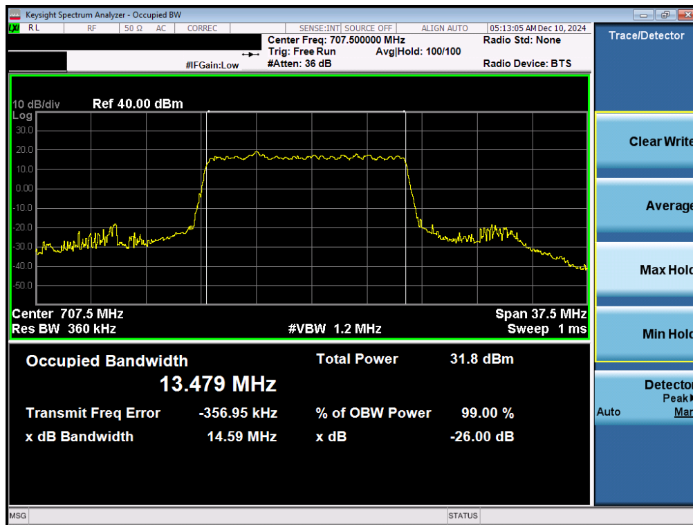
Plot 7-62. Occupied Bandwidth Plot (NR Band n12 - 15MHz DFT-s-OFDM BPSK - Full RB – Ant 2)
