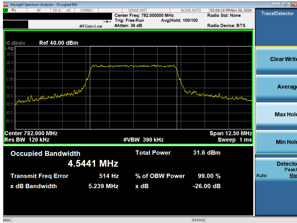
Plot 7-60. Occupied Bandwidth Plot (LTE Band 13 - 5MHz QPSK - Full RB – Ant 2)
