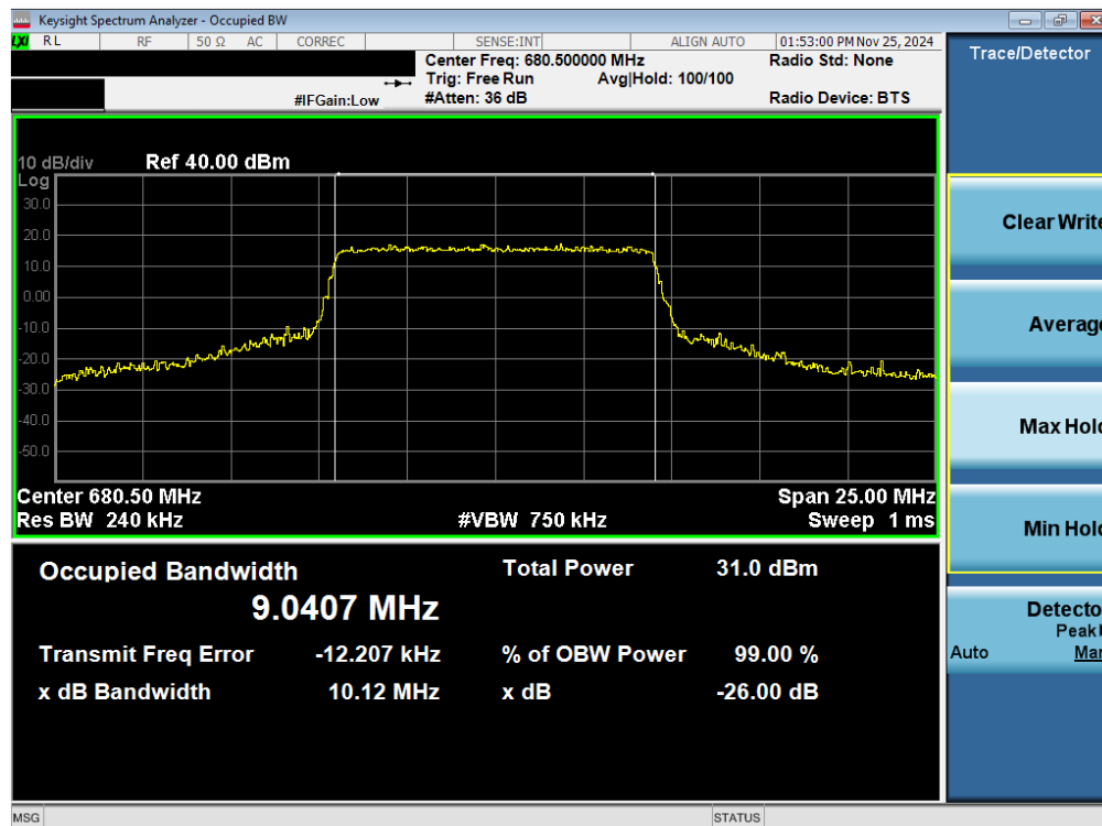
Plot 7-47. Occupied Bandwidth Plot (LTE Band 71 - 10MHz 16-QAM - Full RB – Ant 2)
