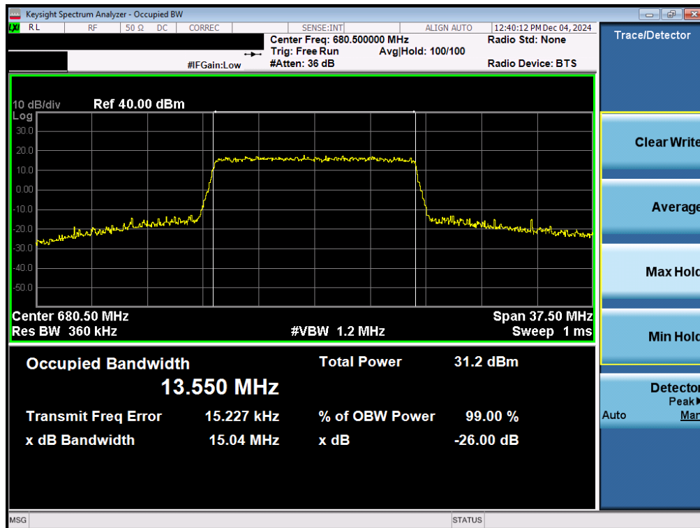
Plot 7-4. Occupied Bandwidth Plot (LTE Band 71 - 15MHz 16-QAM - Full RB – Ant 5)
