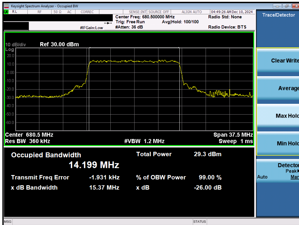
Plot 7-76. Occupied Bandwidth Plot (NR Band n71 - 15MHz CP-OFDM 16-QAM - Full RB – Ant 2)
