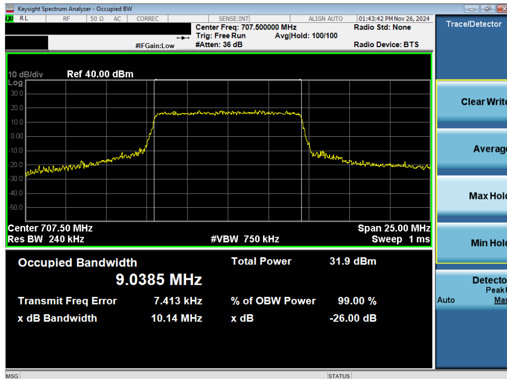
Plot 7-51. Occupied Bandwidth Plot (LTE Band 12 - 10MHz 16-QAM - Full RB – Ant 2)
